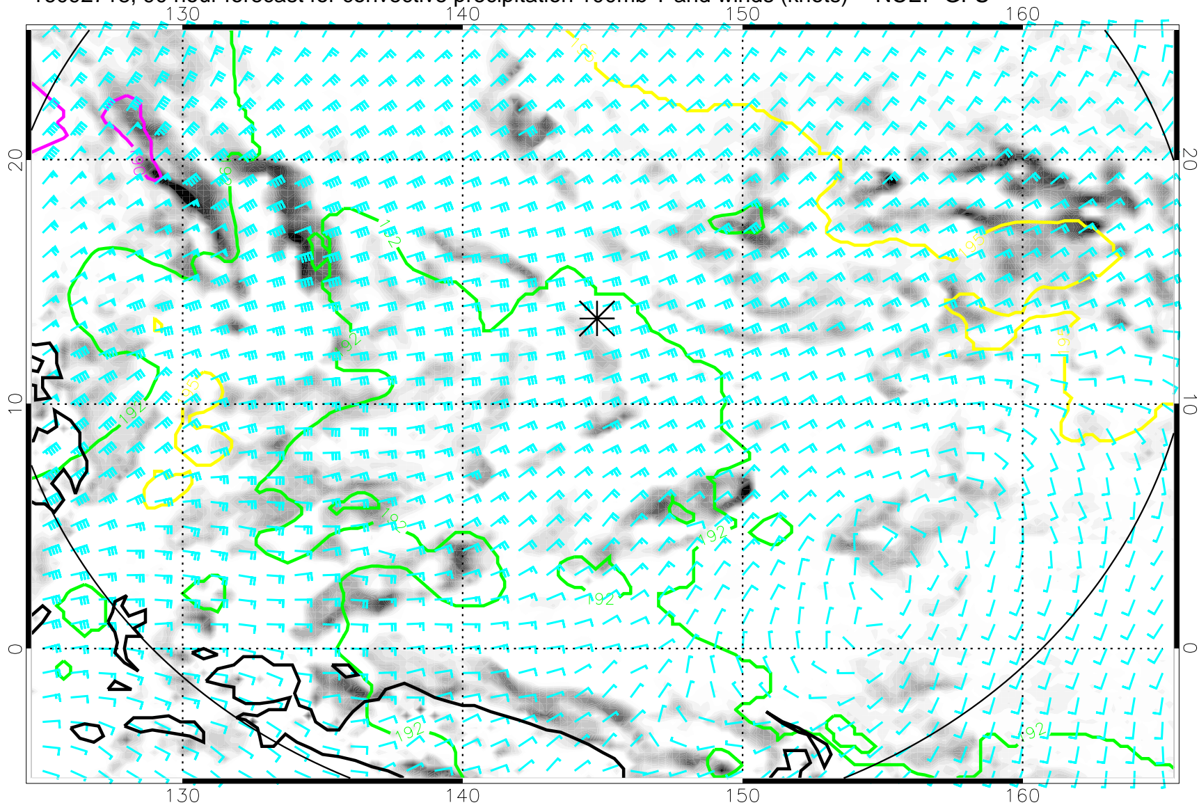
16092718, 90 hour forecast for convective precipitation 100mb T and winds (knots) -- NCEP GFS
