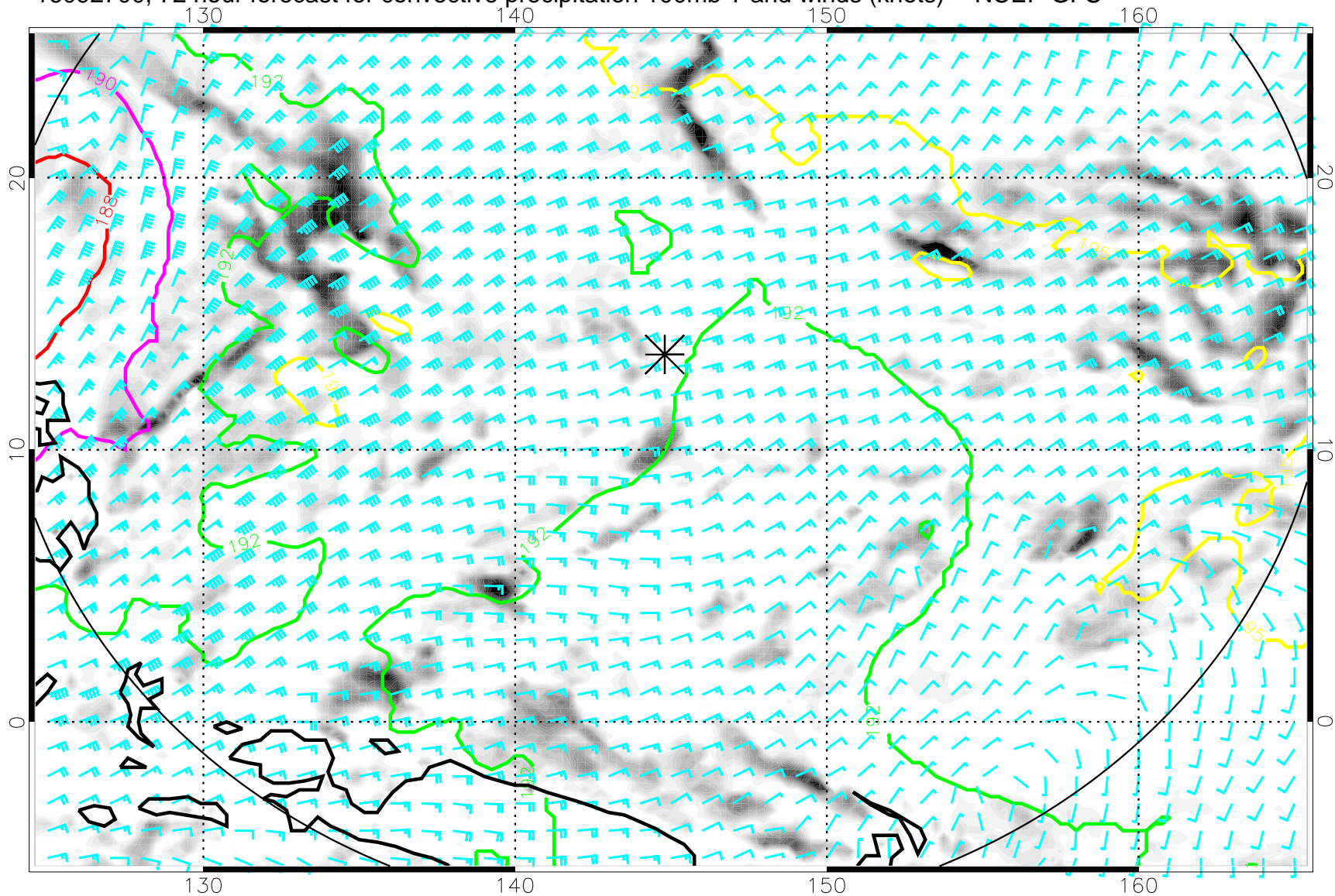
16092700, 72 hour forecast for convective precipitation 100mb T and winds (knots) -- NCEP GFS
