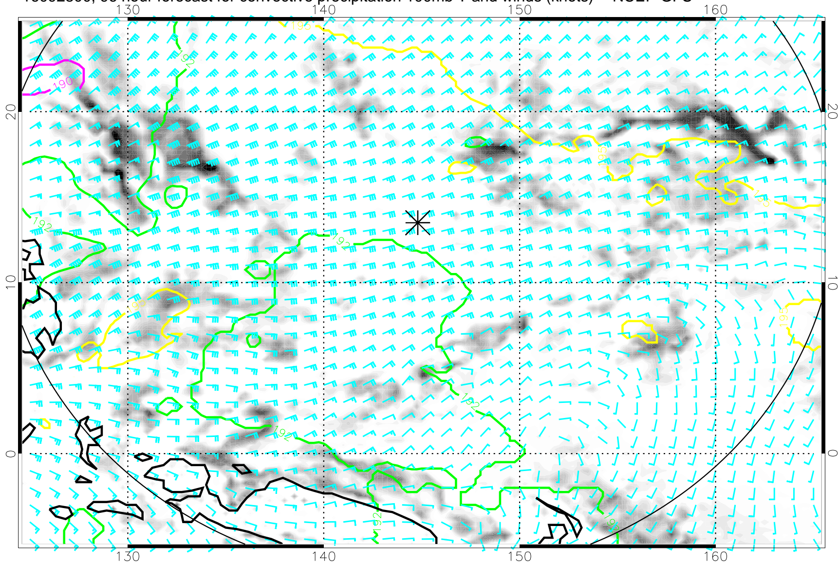
16092800, 96 hour forecast for convective precipitation 100mb T and winds (knots) -- NCEP GFS
