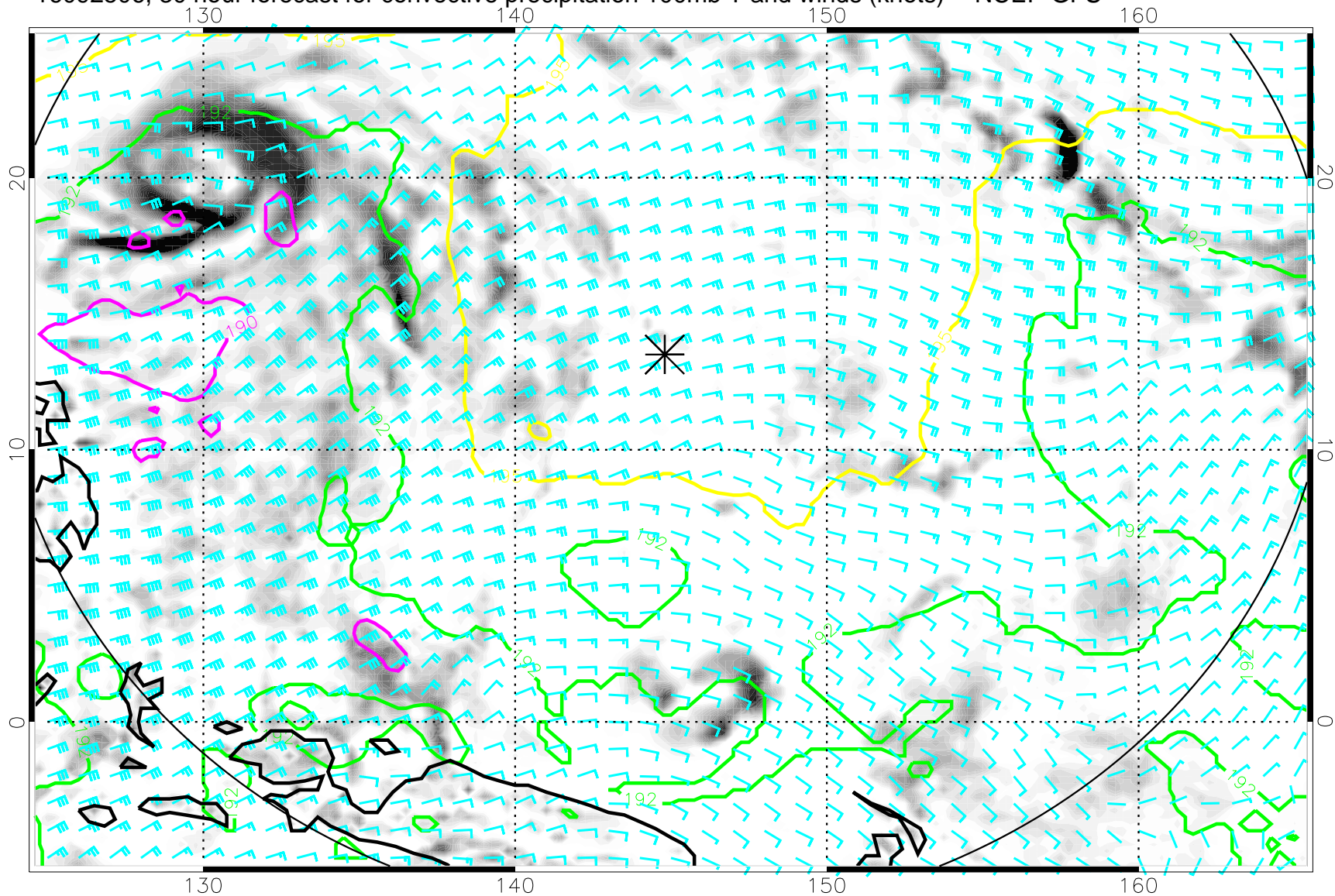
16092506, 30 hour forecast for convective precipitation 100mb T and winds (knots) -- NCEP GFS
