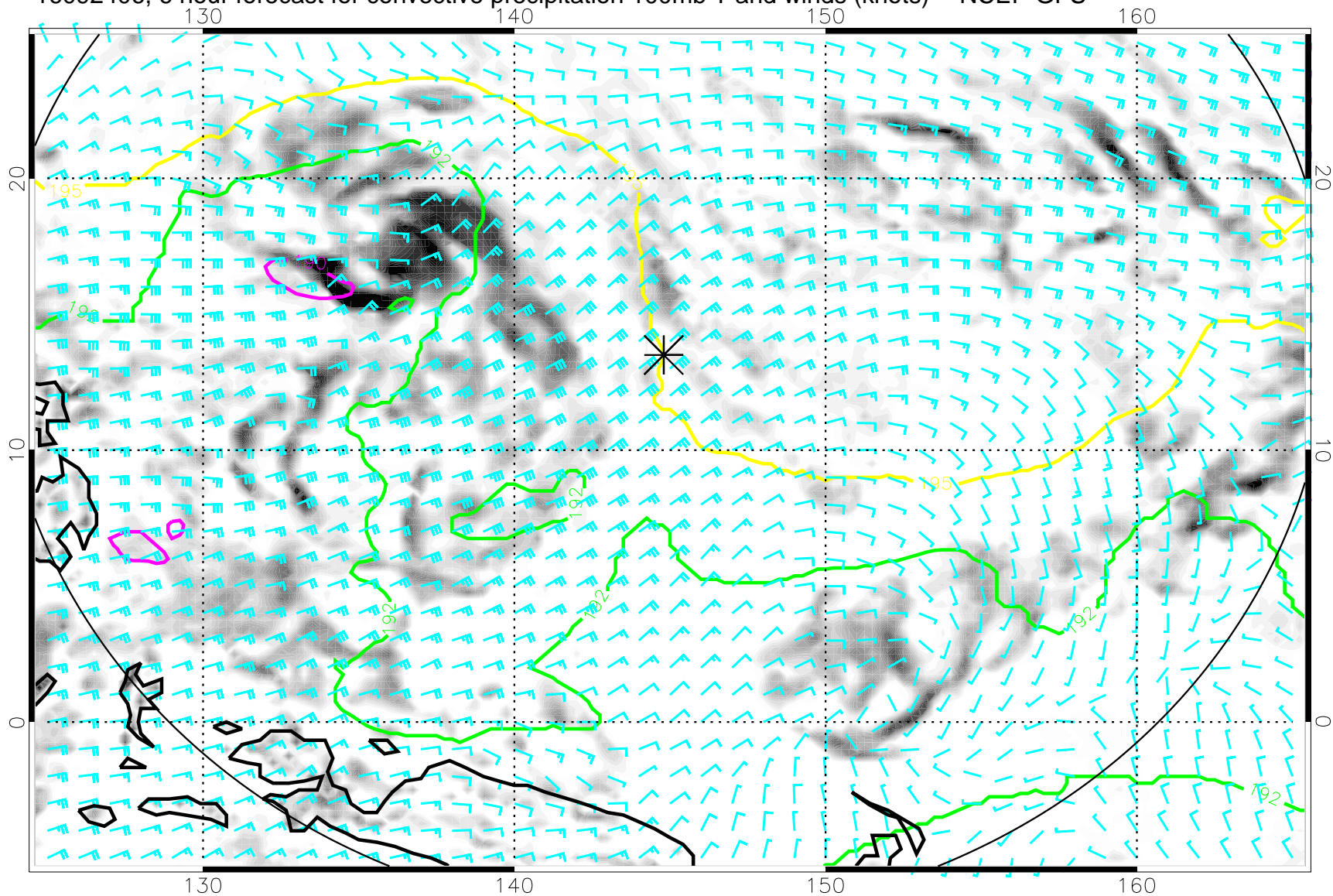
16092406, 6 hour forecast for convective precipitation 100mb T and winds (knots) -- NCEP GFS
