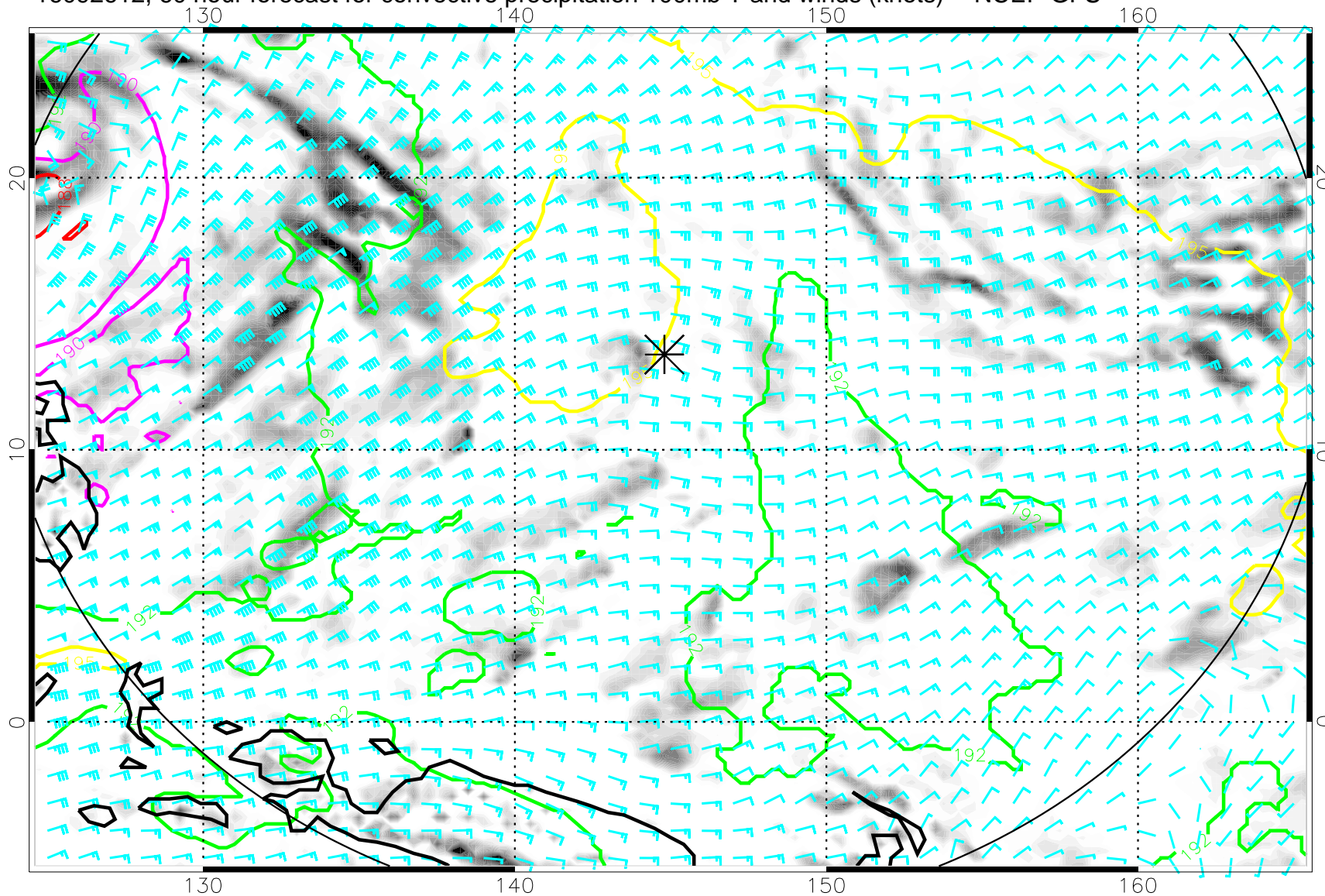
16092612, 60 hour forecast for convective precipitation 100mb T and winds (knots) -- NCEP GFS
