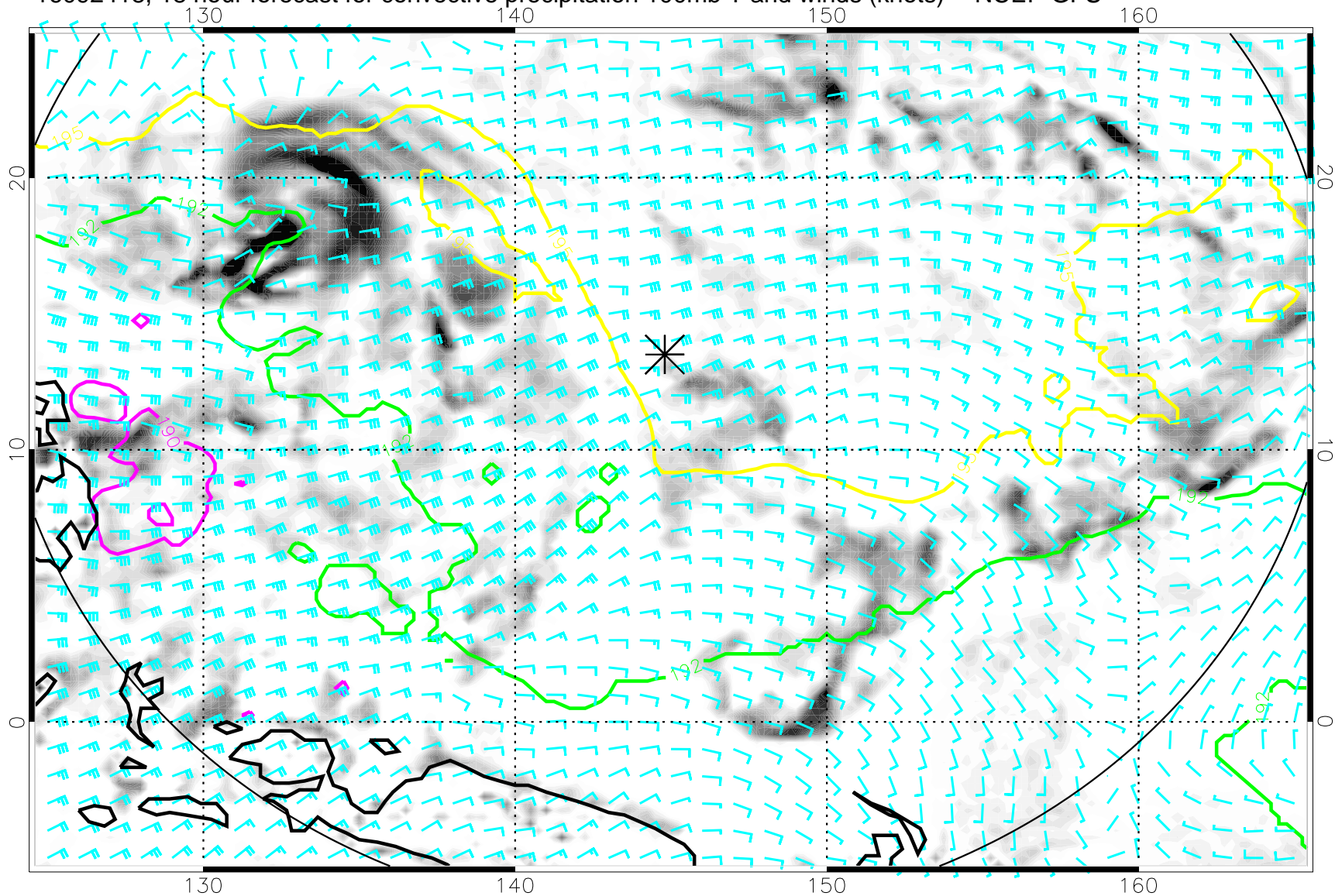
16092418, 18 hour forecast for convective precipitation 100mb T and winds (knots) -- NCEP GFS
