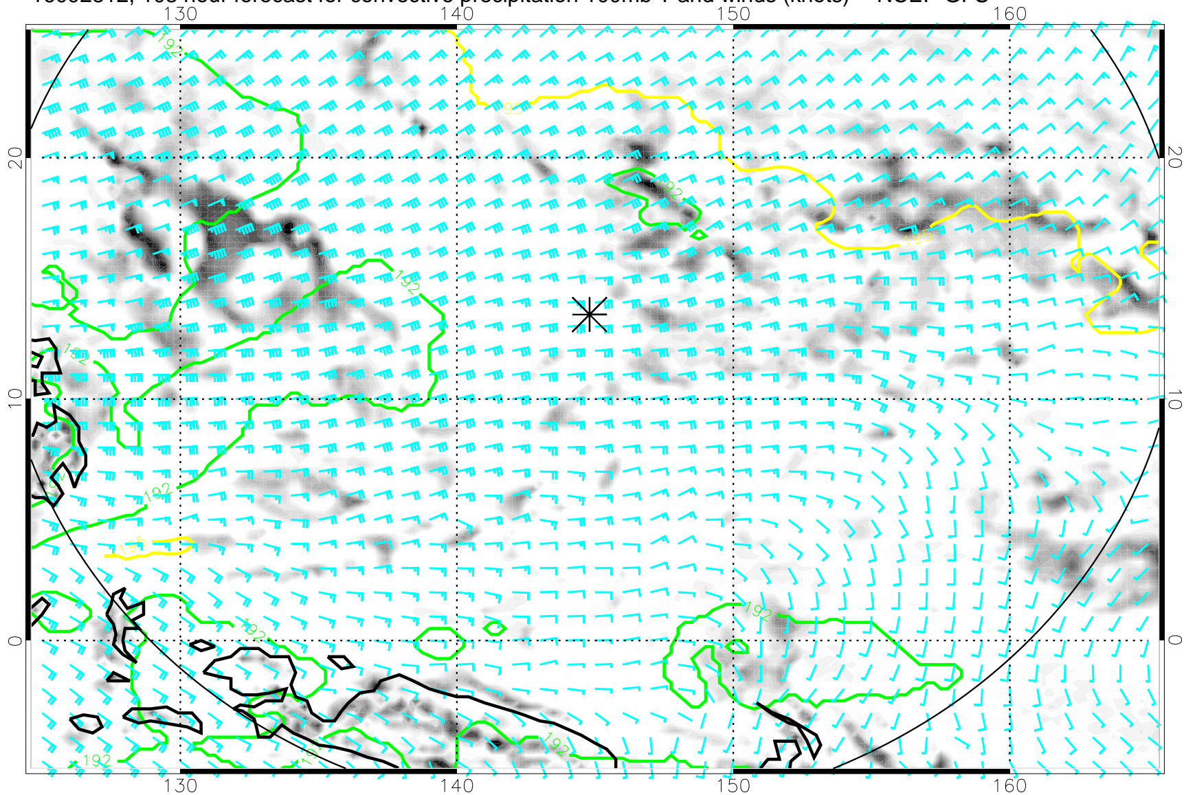
16092812, 108 hour forecast for convective precipitation 100mb T and winds (knots) -- NCEP GFS
