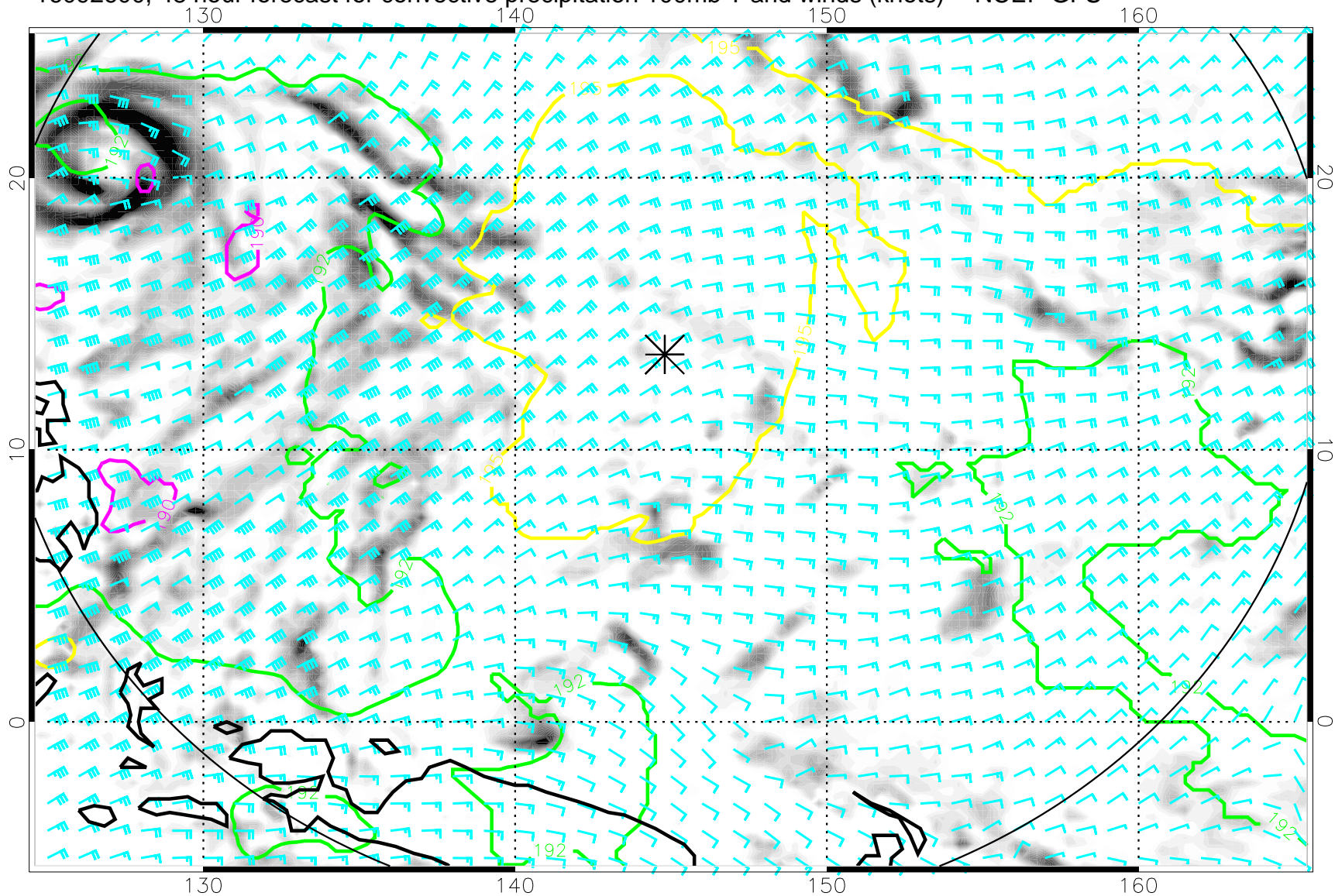
16092600, 48 hour forecast for convective precipitation 100mb T and winds (knots) -- NCEP GFS
