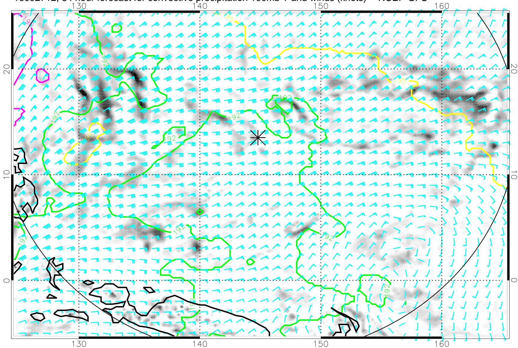
16092712, 84 hour forecast for convective precipitation 100mb T and winds (knots) -- NCEP GFS
