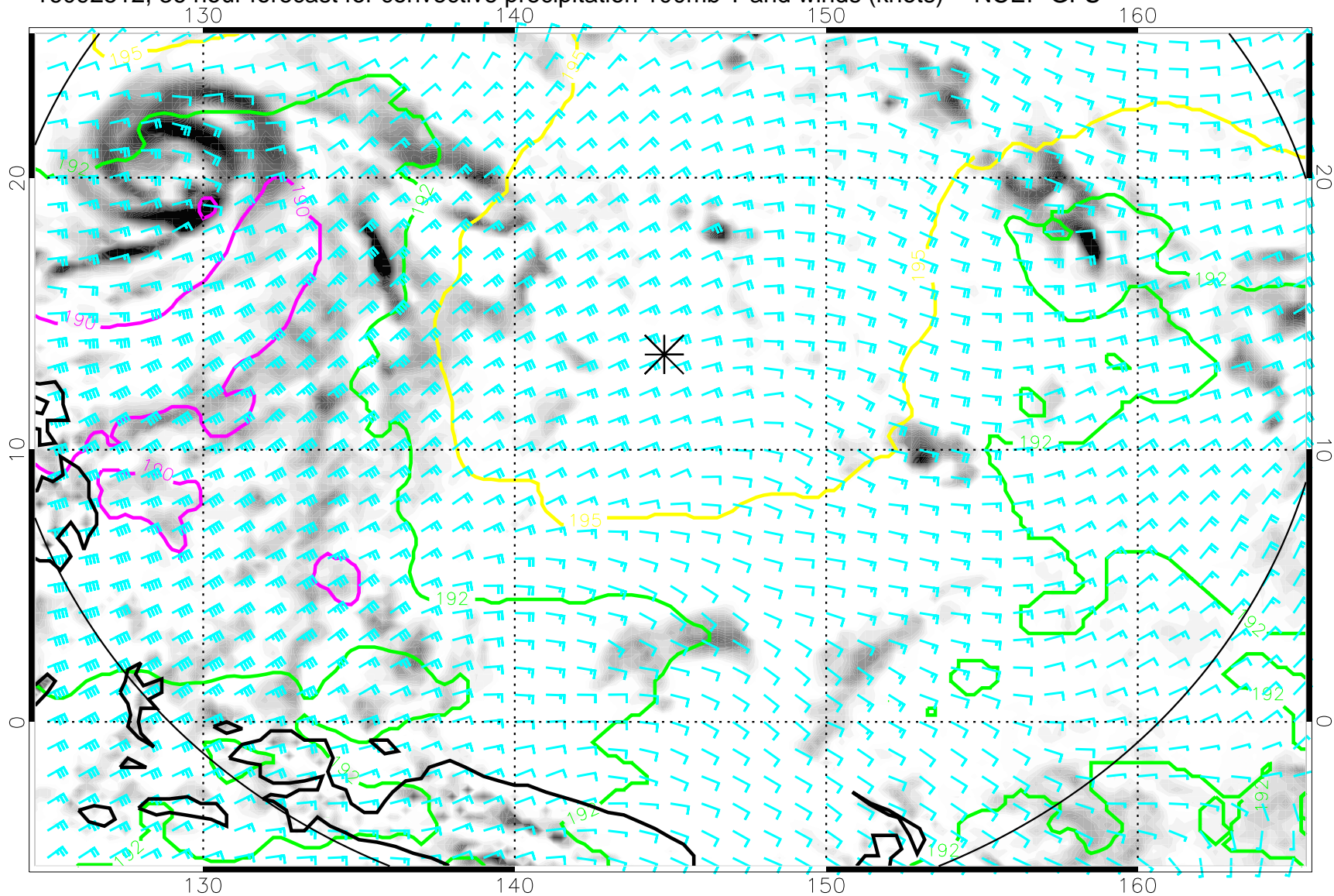
16092512, 36 hour forecast for convective precipitation 100mb T and winds (knots) -- NCEP GFS
