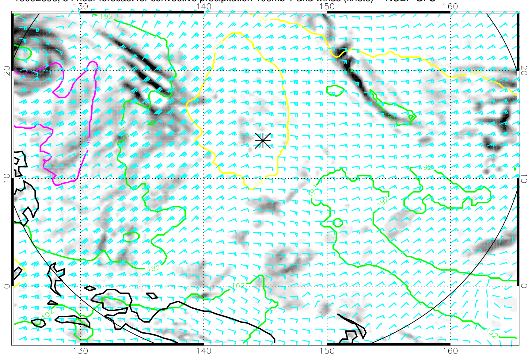
16092606, 54 hour forecast for convective precipitation 100mb T and winds (knots) -- NCEP GFS
