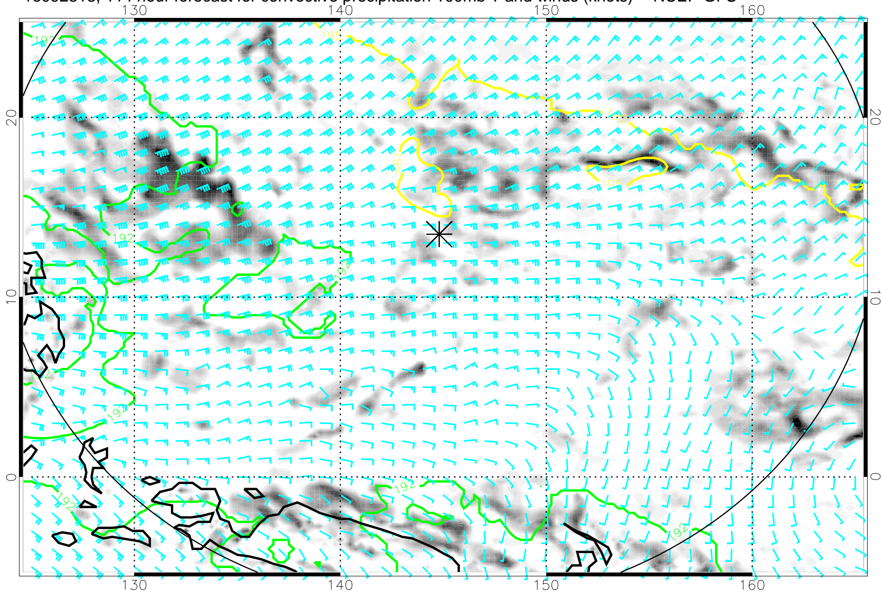
16092818, 114 hour forecast for convective precipitation 100mb T and winds (knots) -- NCEP GFS
