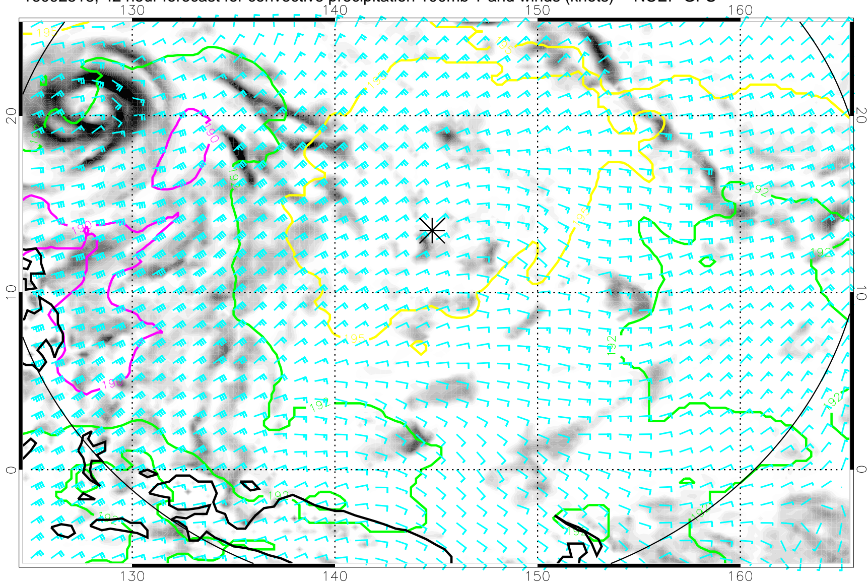
16092518, 42 hour forecast for convective precipitation 100mb T and winds (knots) -- NCEP GFS
