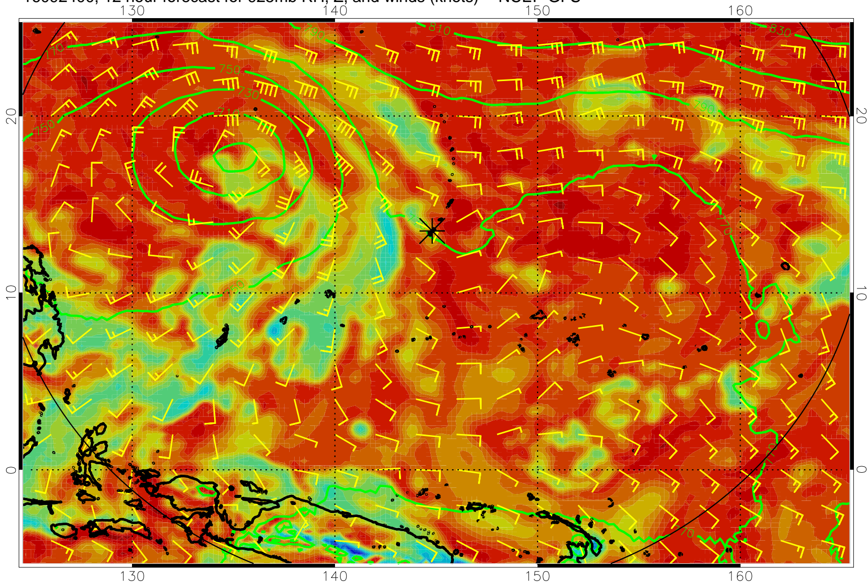
16092400, 12 hour forecast for 925mb RH, Z, and winds (knots) -- NCEP GFS
