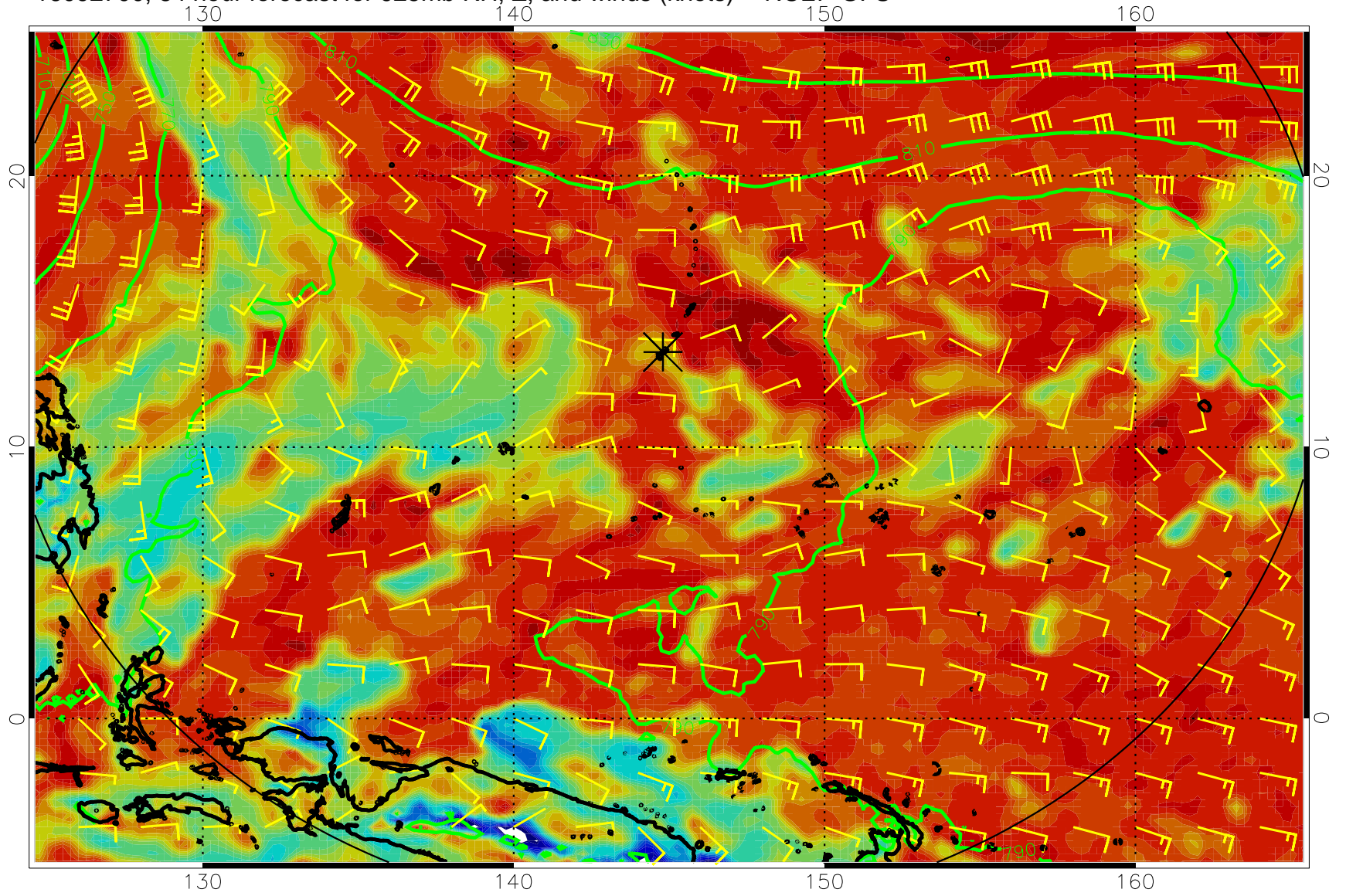
16092700, 84 hour forecast for 925mb RH, Z, and winds (knots) -- NCEP GFS
