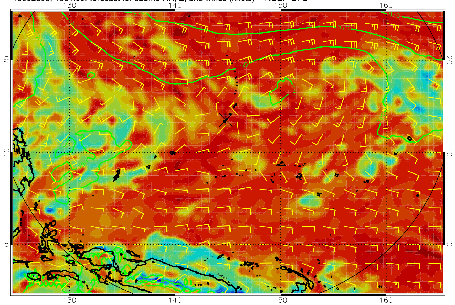
16092800, 108 hour forecast for 925mb RH, Z, and winds (knots) -- NCEP GFS
