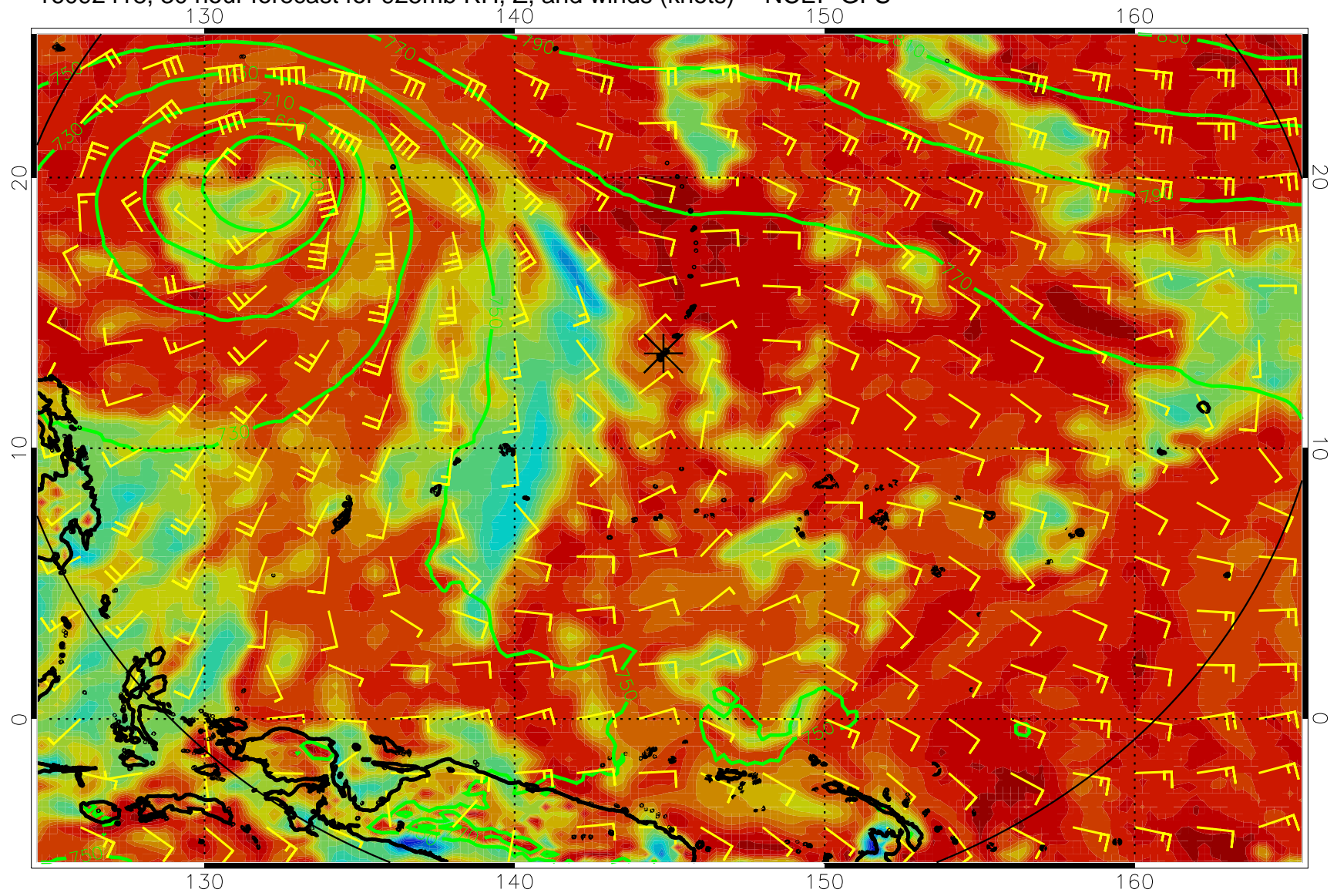
16092418, 30 hour forecast for 925mb RH, Z, and winds (knots) -- NCEP GFS
