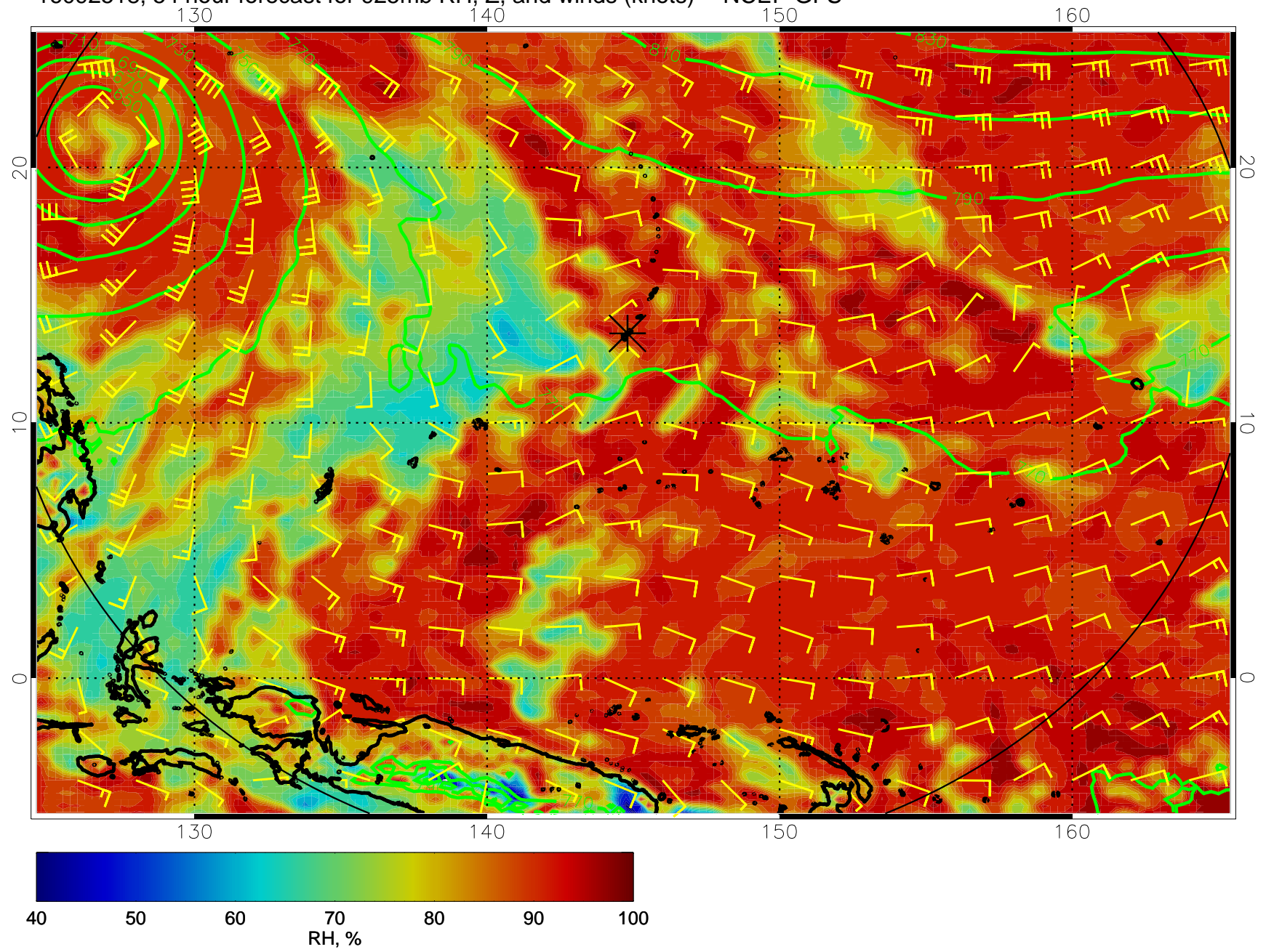
16092518, 54 hour forecast for 925mb RH, Z, and winds (knots) -- NCEP GFS
