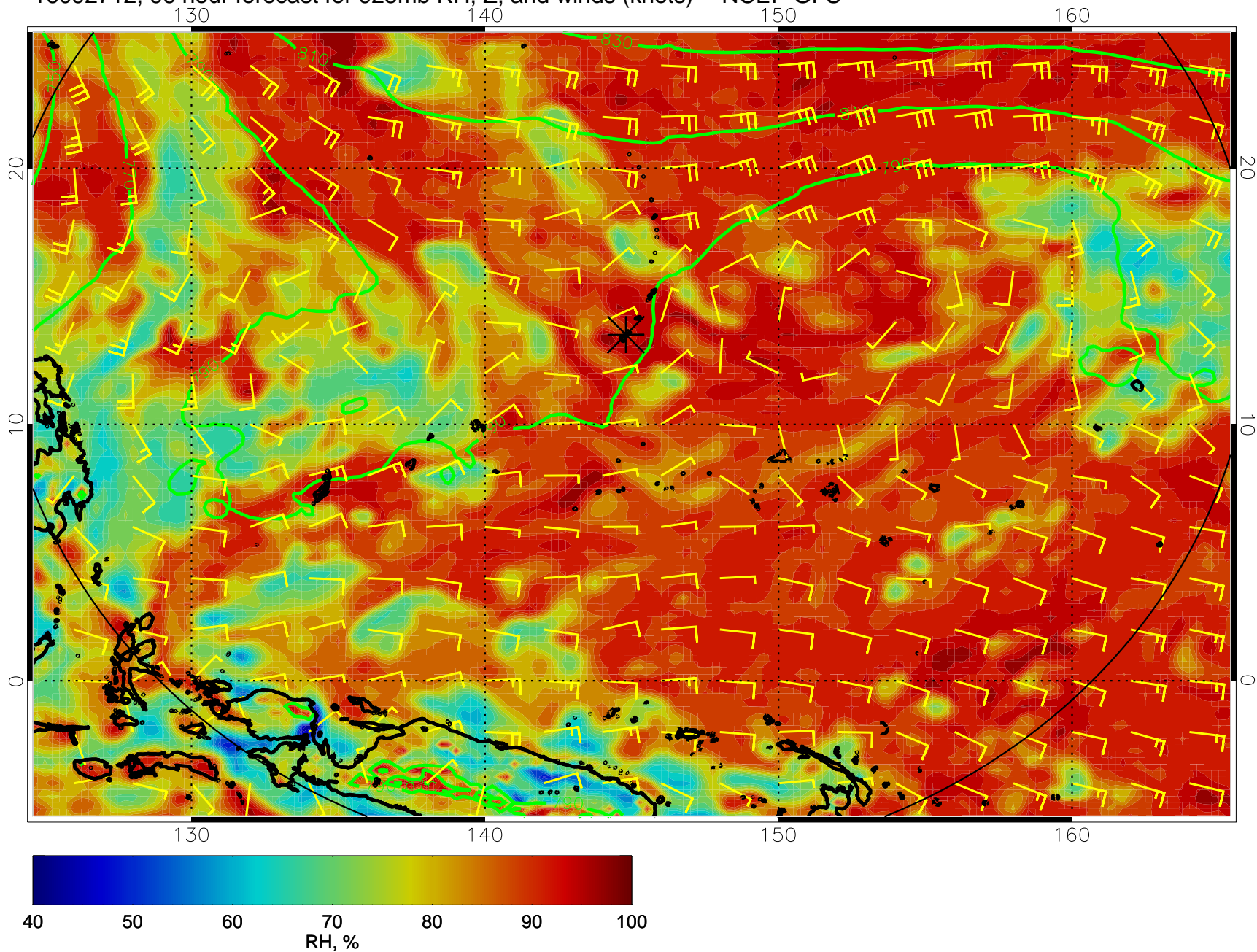
16092712, 96 hour forecast for 925mb RH, Z, and winds (knots) -- NCEP GFS
