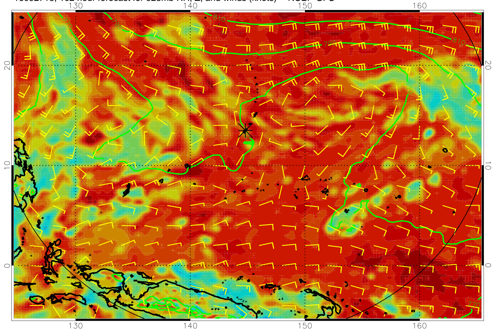
16092718, 102 hour forecast for 925mb RH, Z, and winds (knots) -- NCEP GFS
