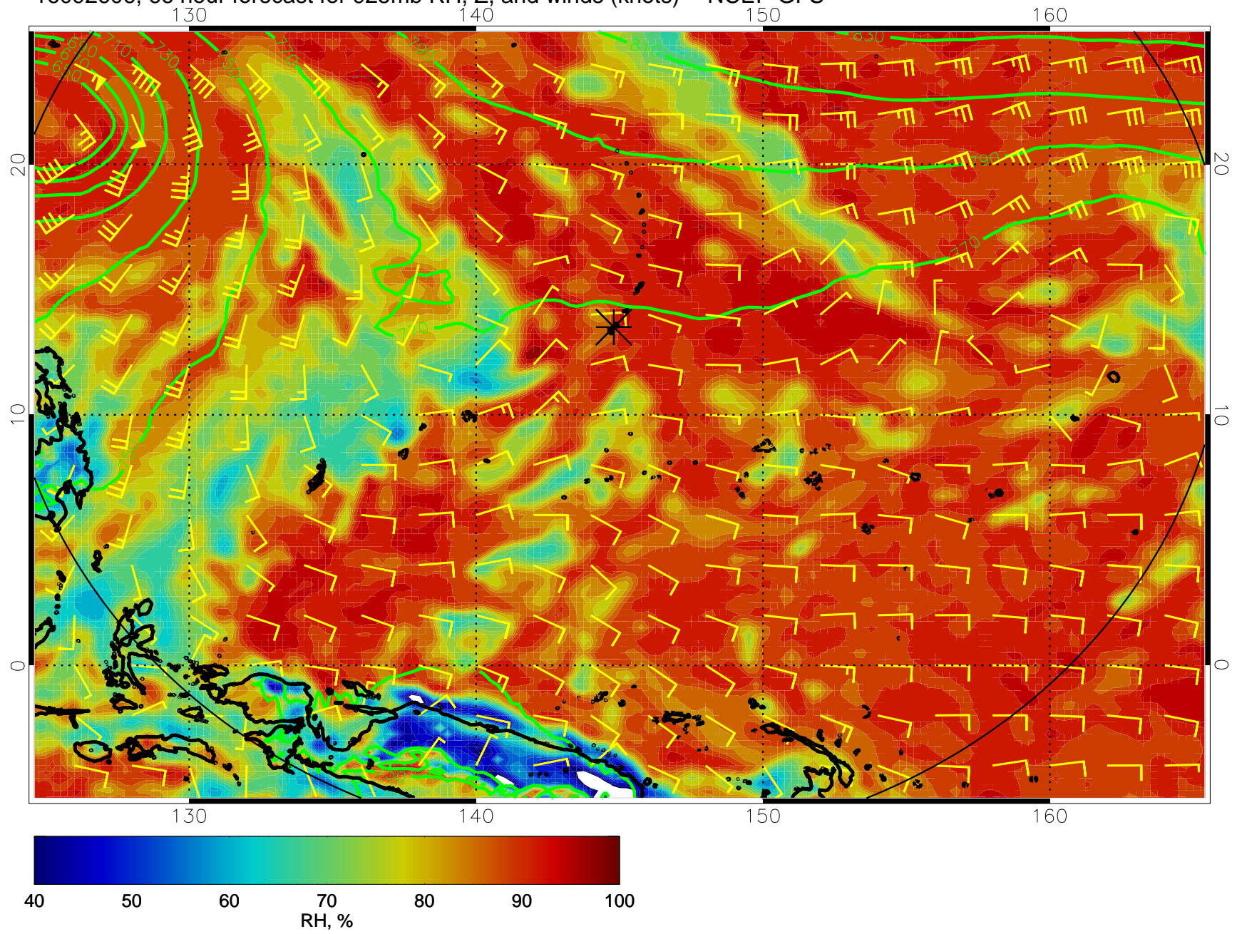
16092606, 66 hour forecast for 925mb RH, Z, and winds (knots) -- NCEP GFS
