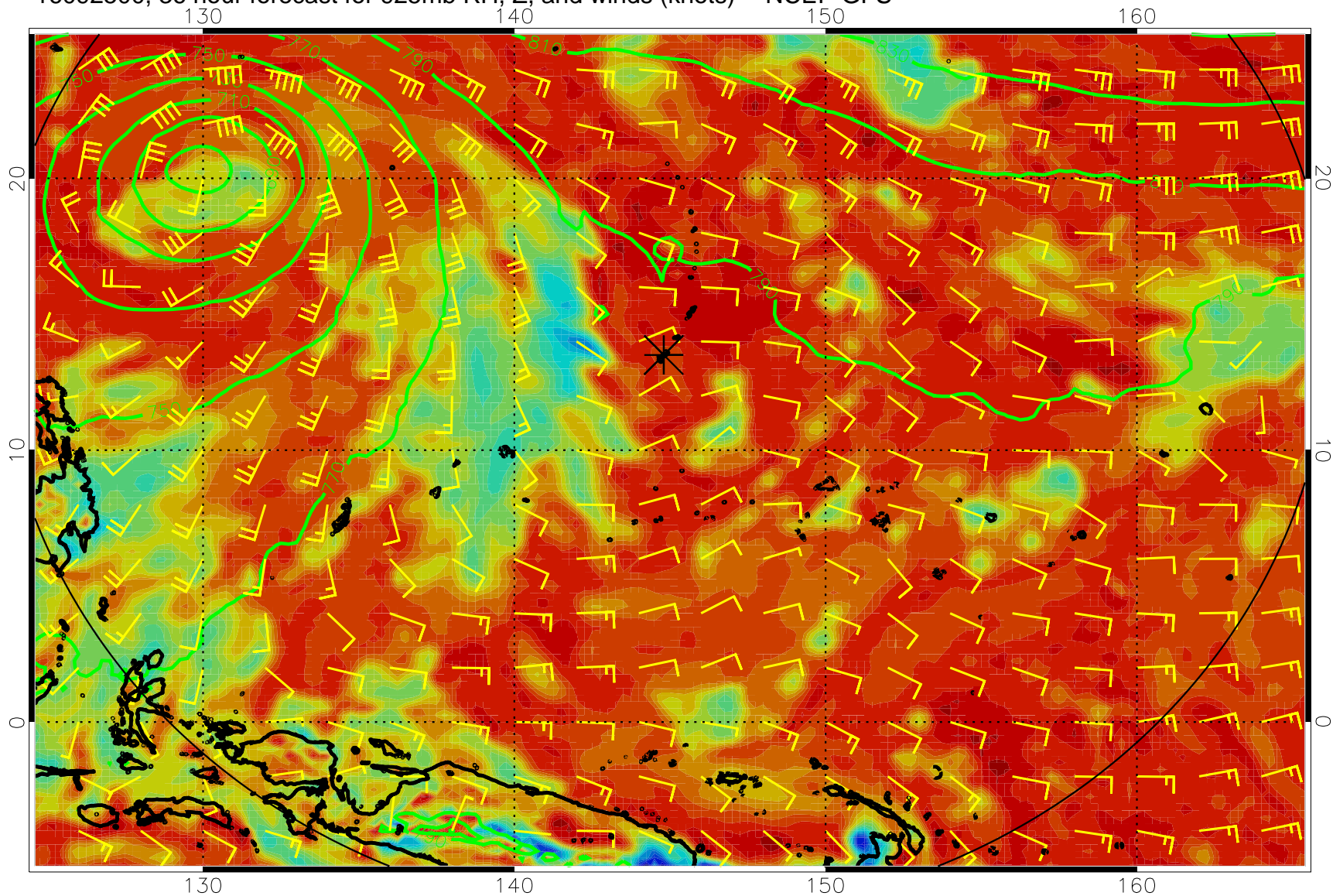
16092500, 36 hour forecast for 925mb RH, Z, and winds (knots) -- NCEP GFS
