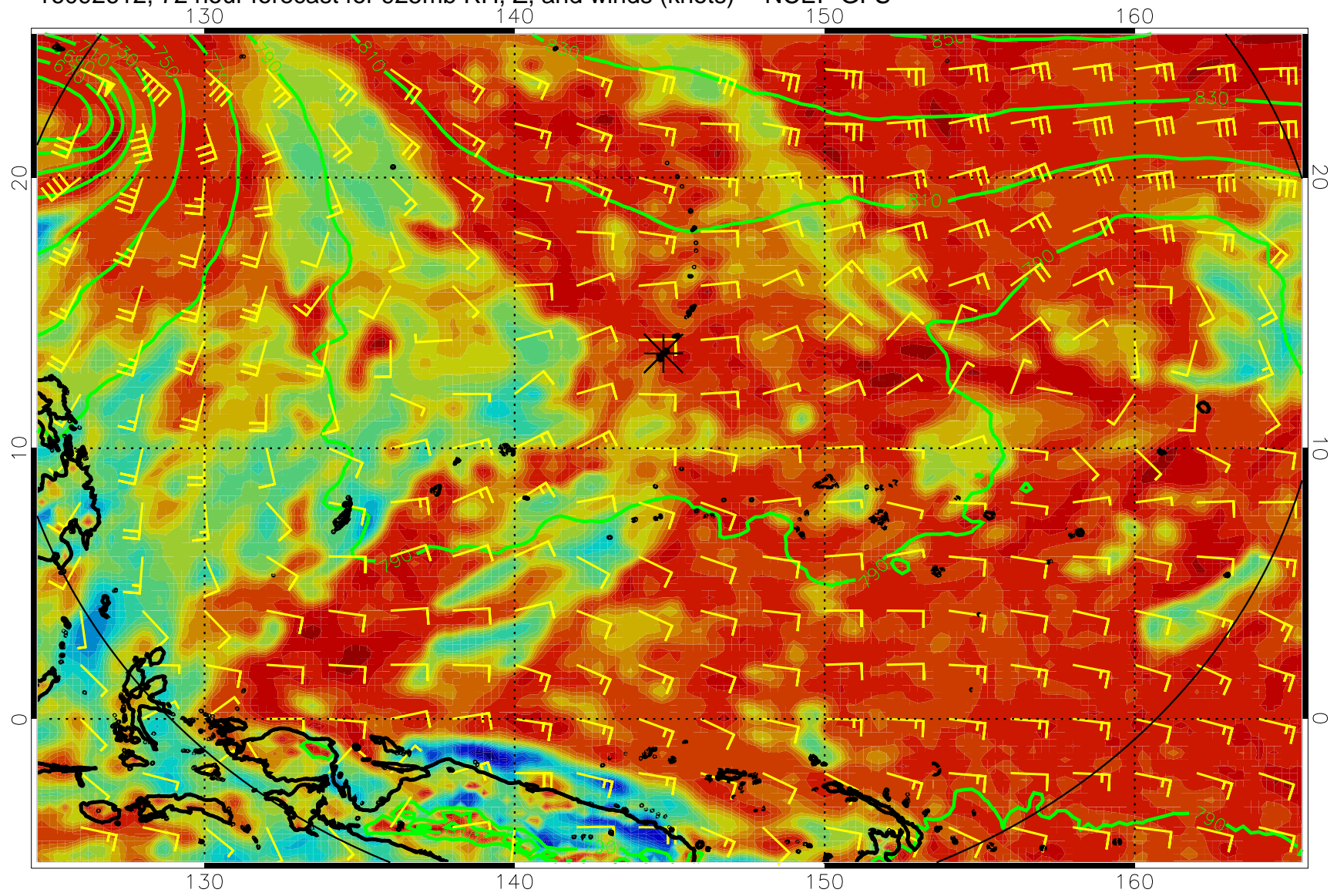
16092612, 72 hour forecast for 925mb RH, Z, and winds (knots) -- NCEP GFS
