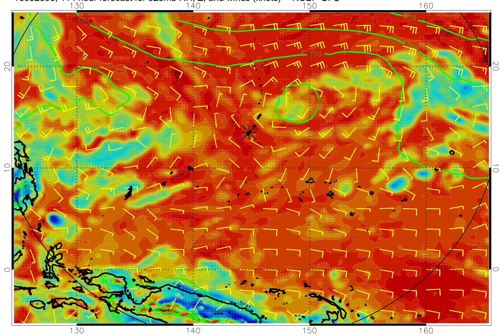
16092806, 114 hour forecast for 925mb RH, Z, and winds (knots) -- NCEP GFS
