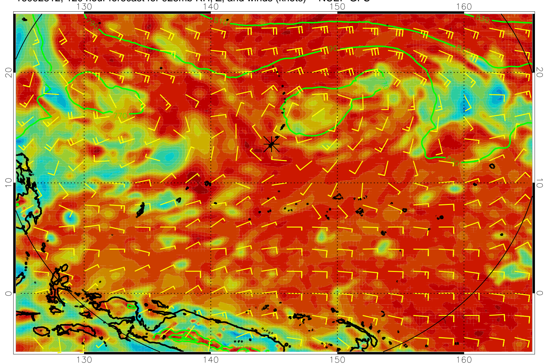
16092812, 120 hour forecast for 925mb RH, Z, and winds (knots) -- NCEP GFS
