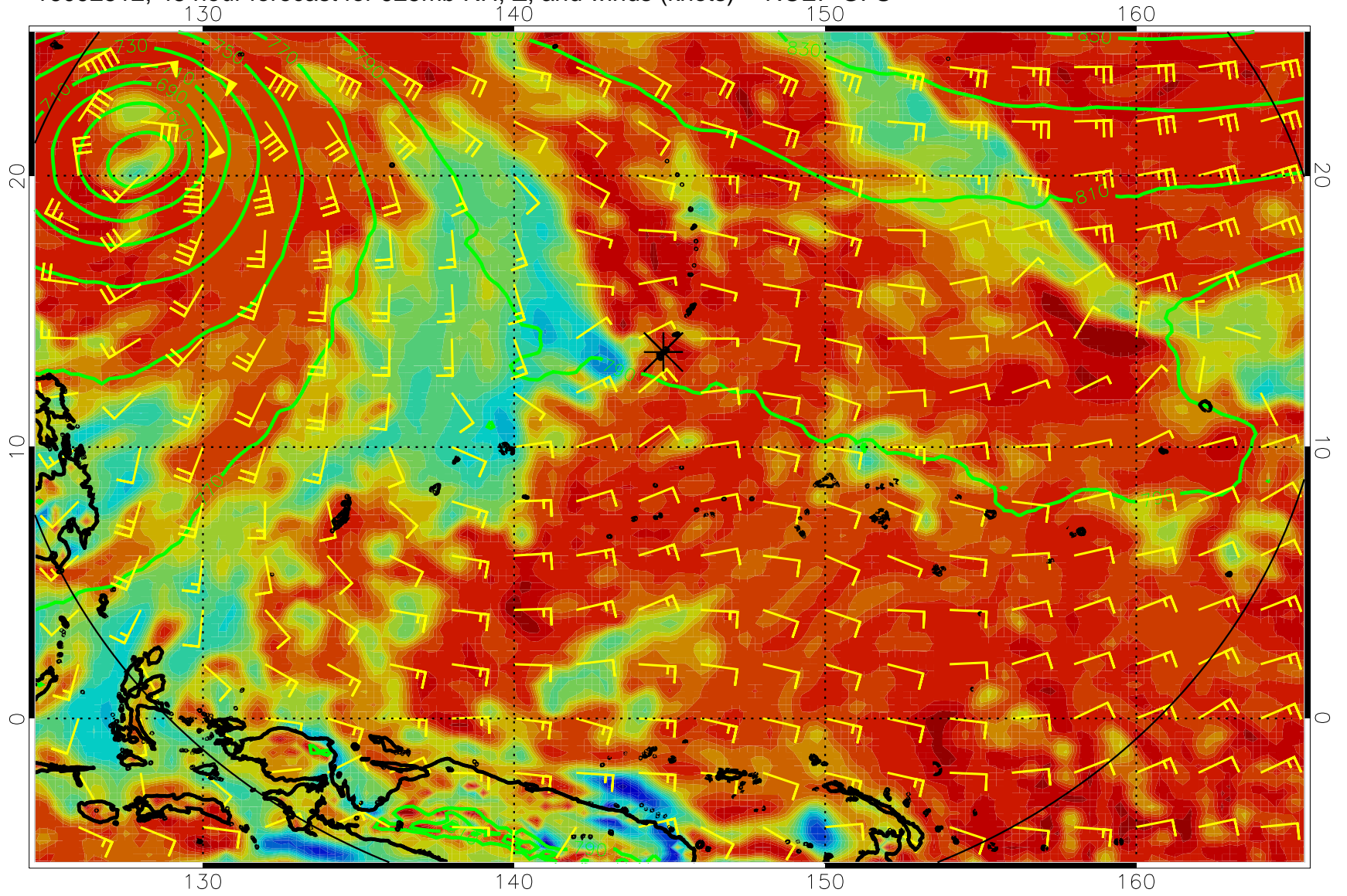
16092512, 48 hour forecast for 925mb RH, Z, and winds (knots) -- NCEP GFS
