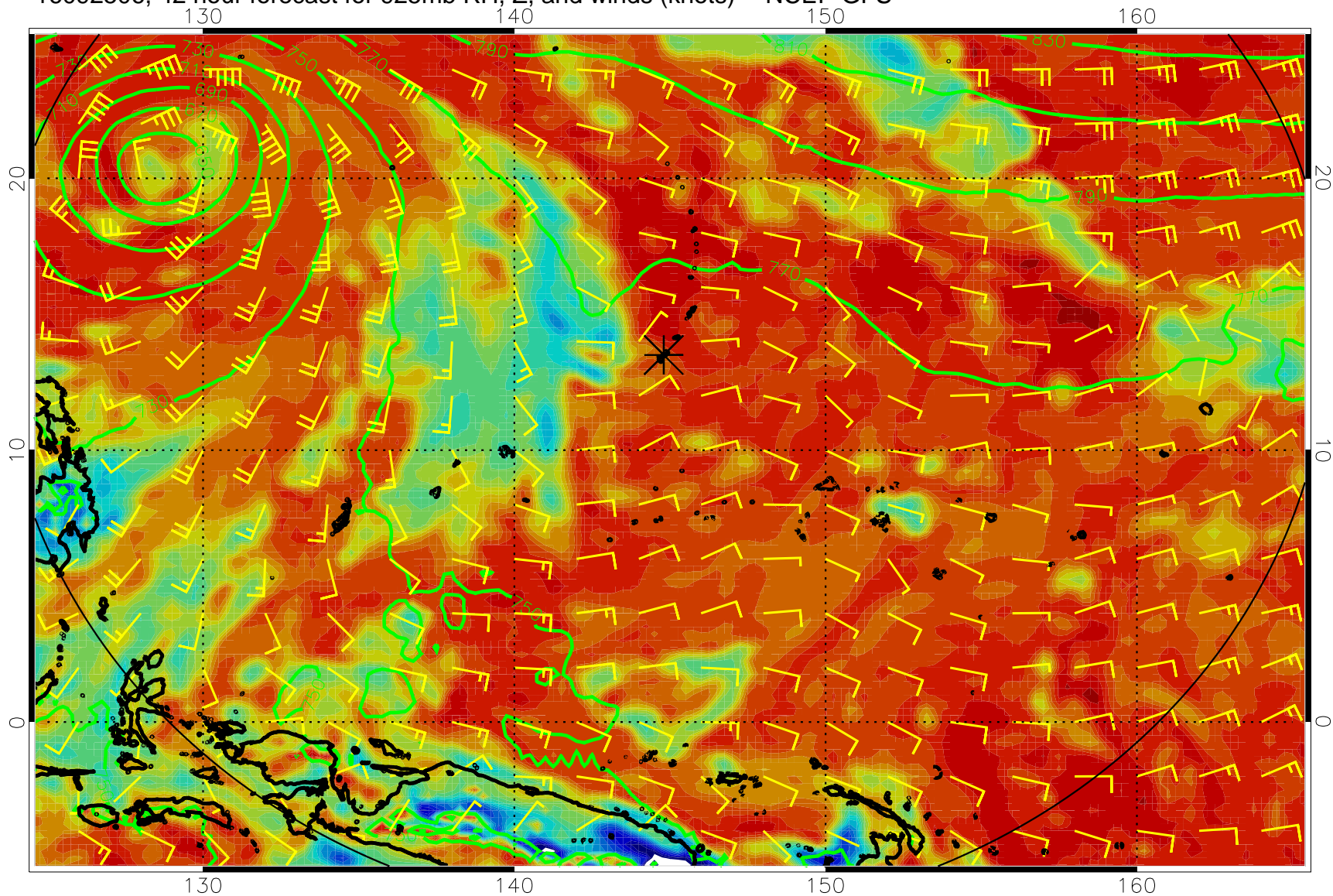
16092506, 42 hour forecast for 925mb RH, Z, and winds (knots) -- NCEP GFS
