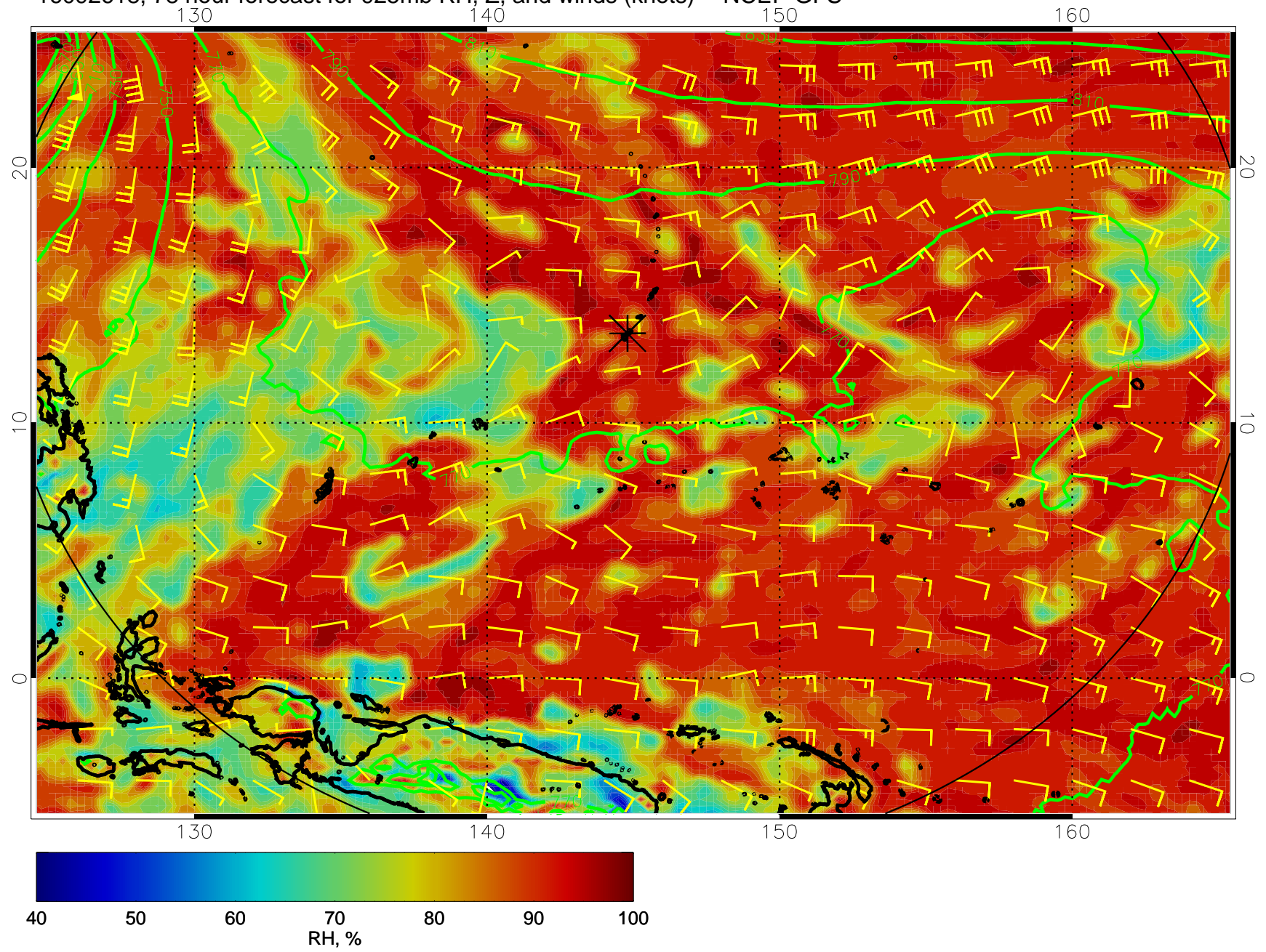
16092618, 78 hour forecast for 925mb RH, Z, and winds (knots) -- NCEP GFS
