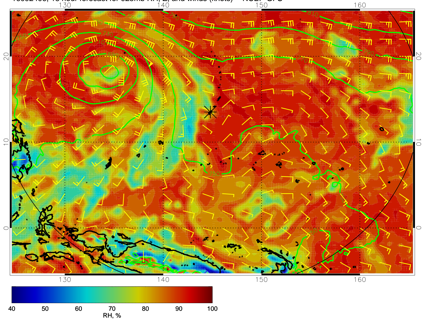
16092406, 18 hour forecast for 925mb RH, Z, and winds (knots) -- NCEP GFS
