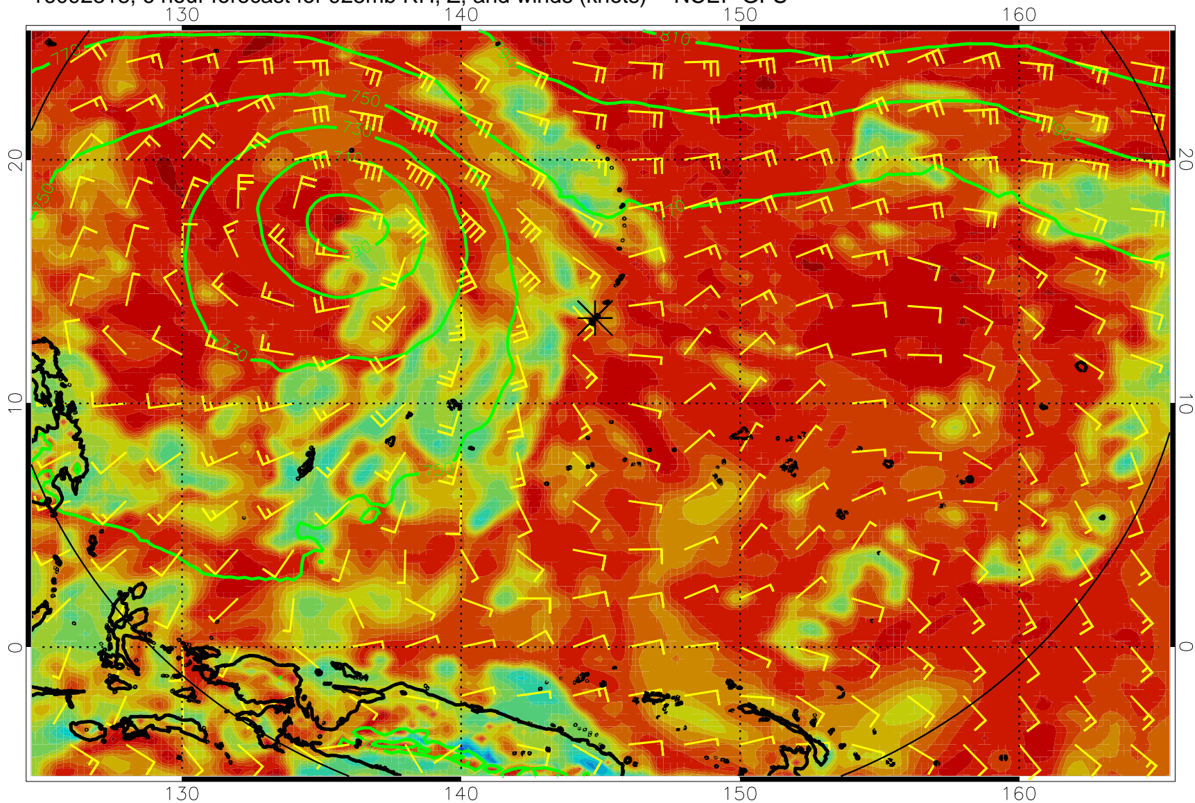
16092318, 6 hour forecast for 925mb RH, Z, and winds (knots) -- NCEP GFS
