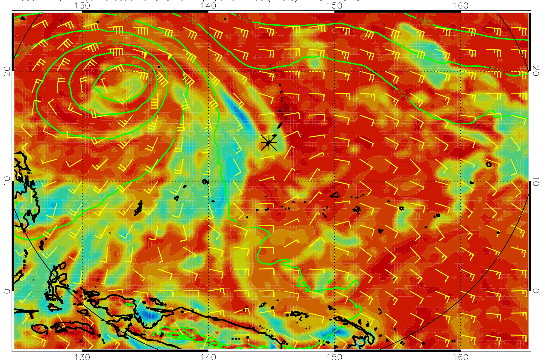
16092412, 24 hour forecast for 925mb RH, Z, and winds (knots) -- NCEP GFS
