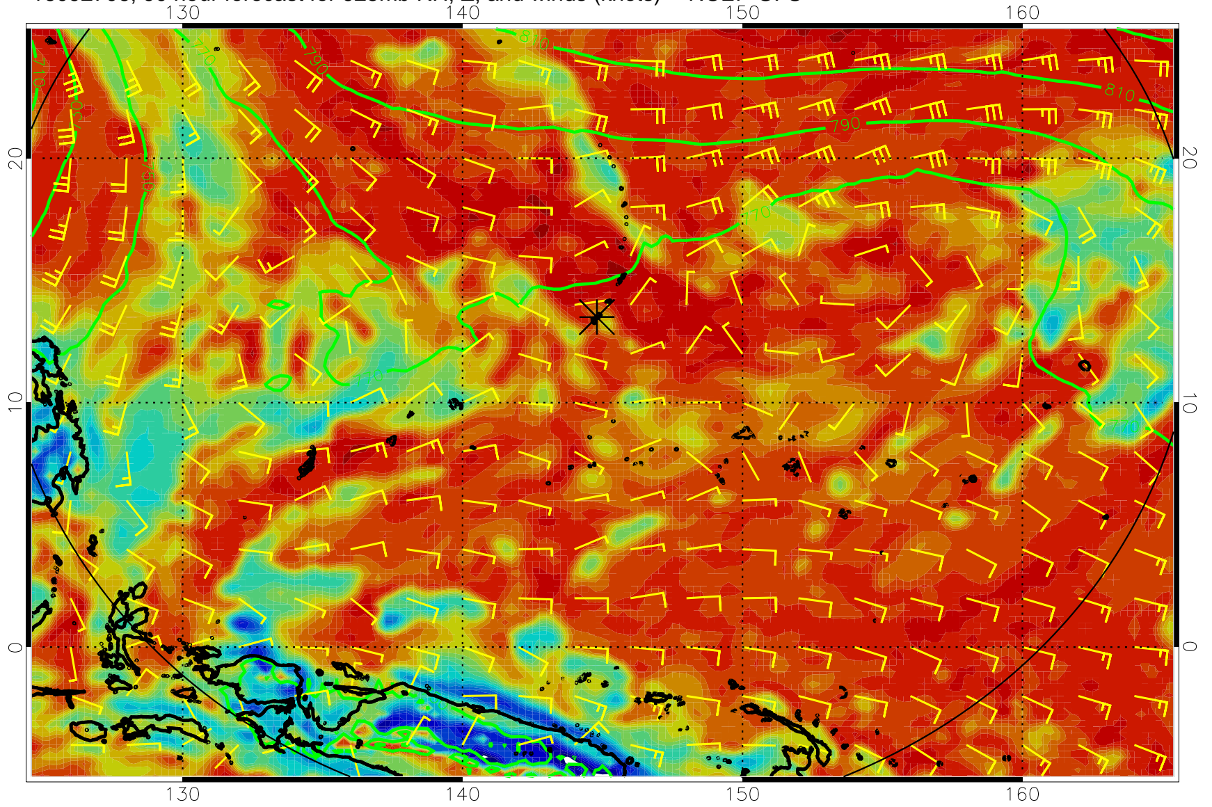
16092706, 90 hour forecast for 925mb RH, Z, and winds (knots) -- NCEP GFS
