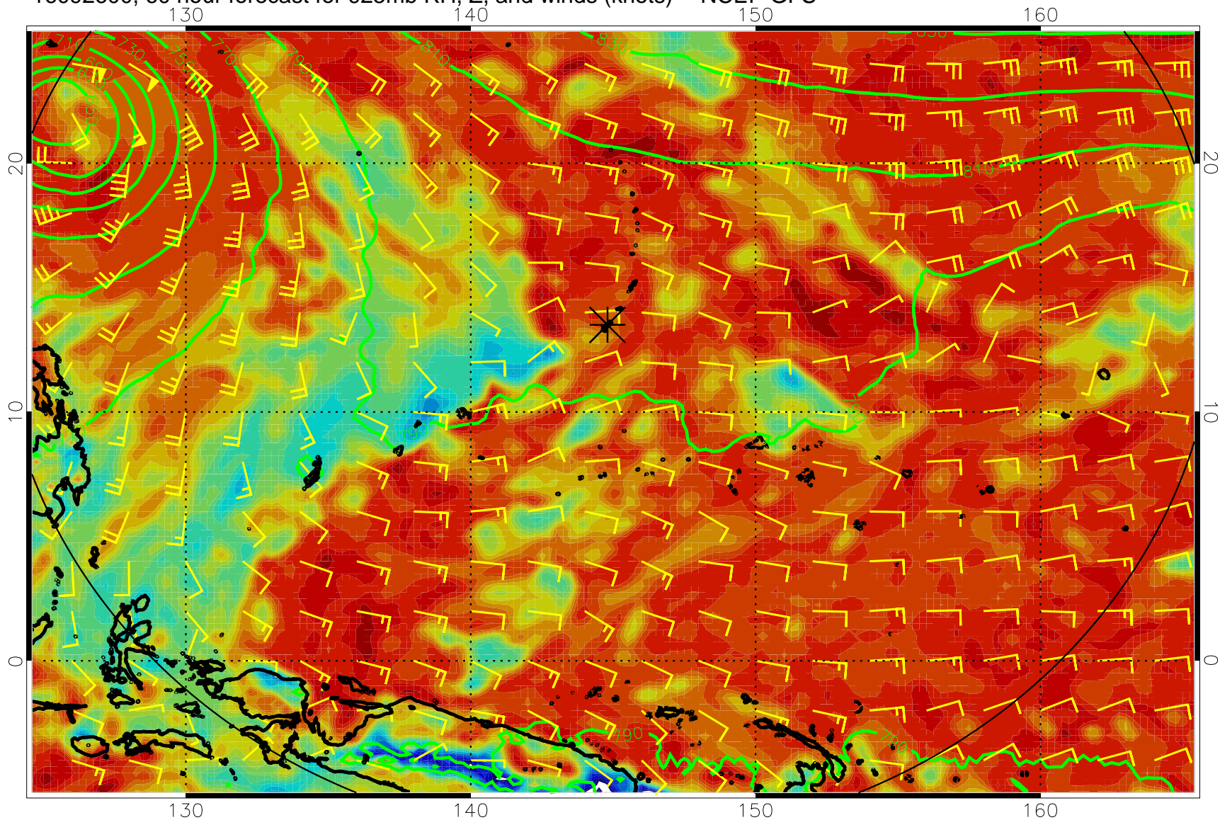
16092600, 60 hour forecast for 925mb RH, Z, and winds (knots) -- NCEP GFS
