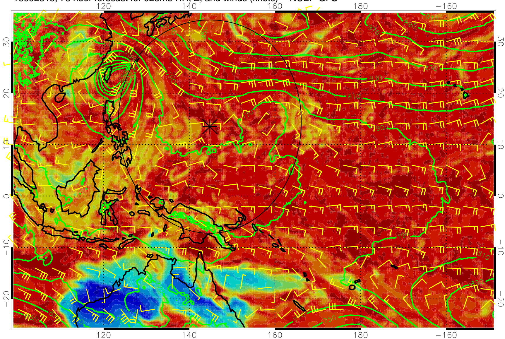
16092618, 78 hour forecast for 925mb RH, Z, and winds (knots) -- NCEP GFS
