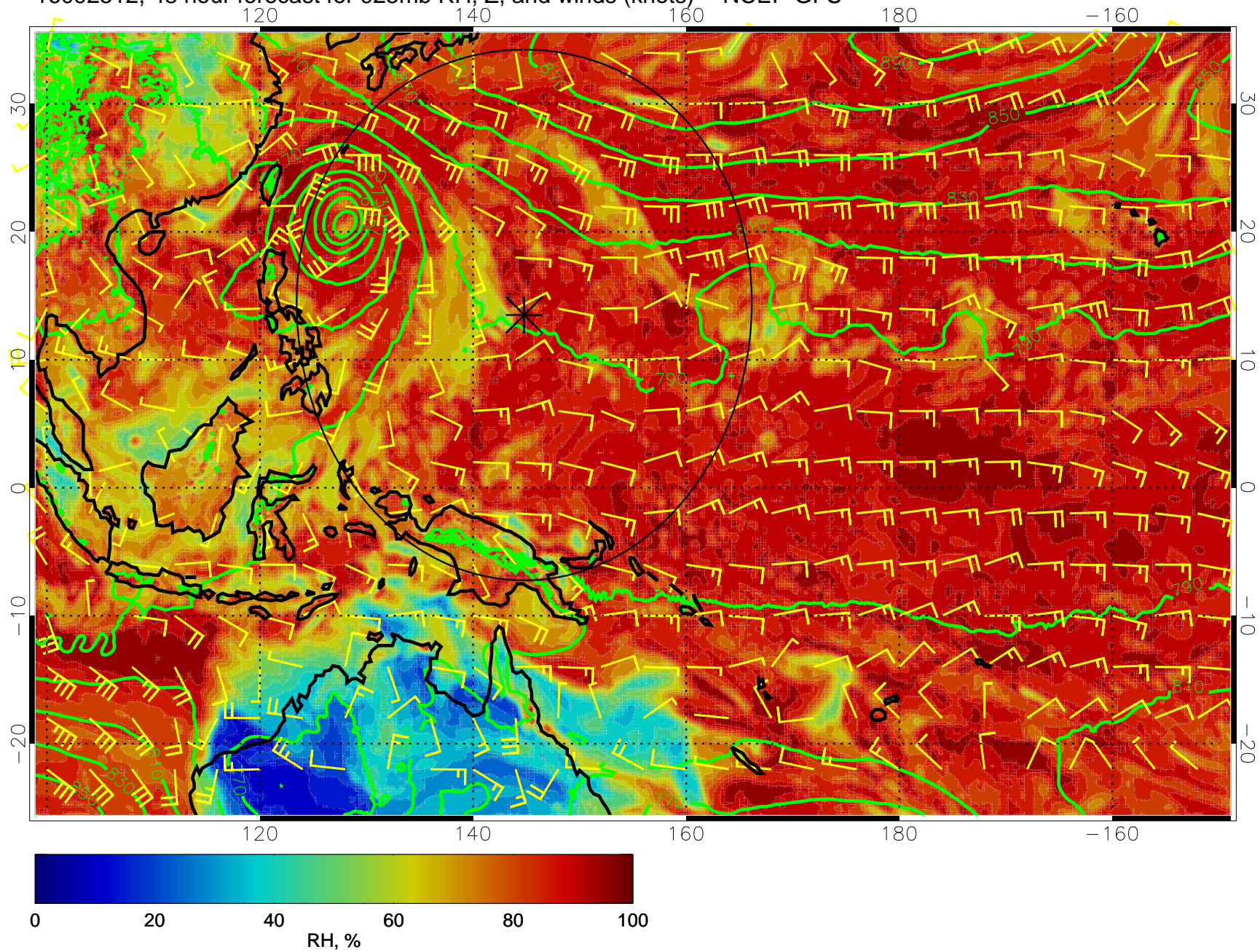
16092512, 48 hour forecast for 925mb RH, Z, and winds (knots) -- NCEP GFS
