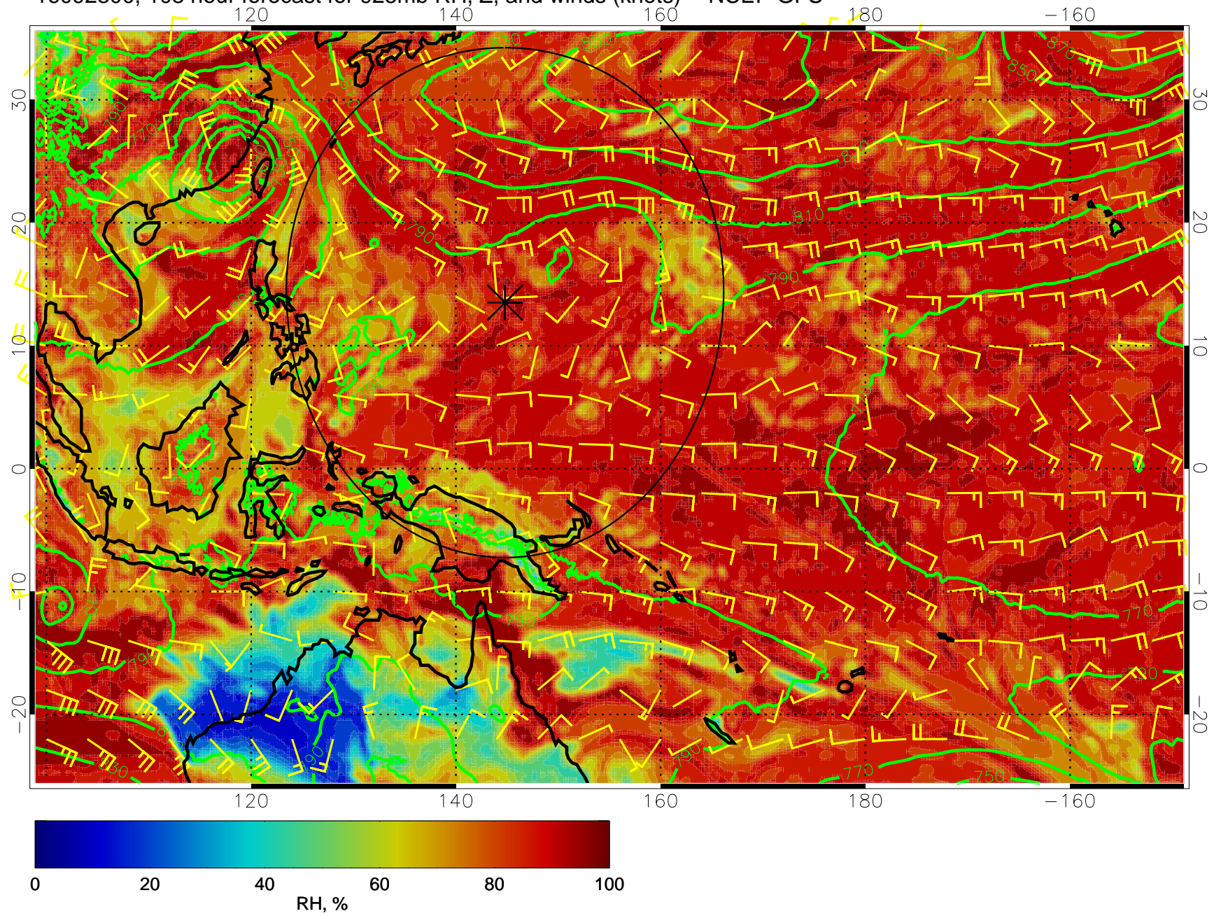
16092800, 108 hour forecast for 925mb RH, Z, and winds (knots) -- NCEP GFS
