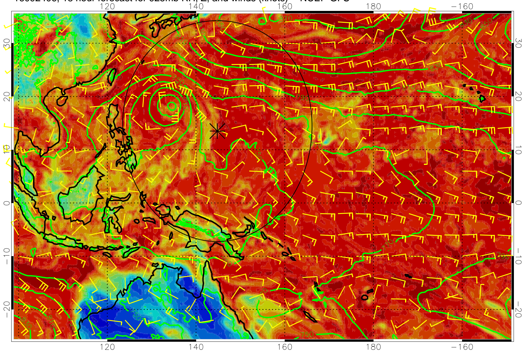
16092406, 18 hour forecast for 925mb RH, Z, and winds (knots) -- NCEP GFS
