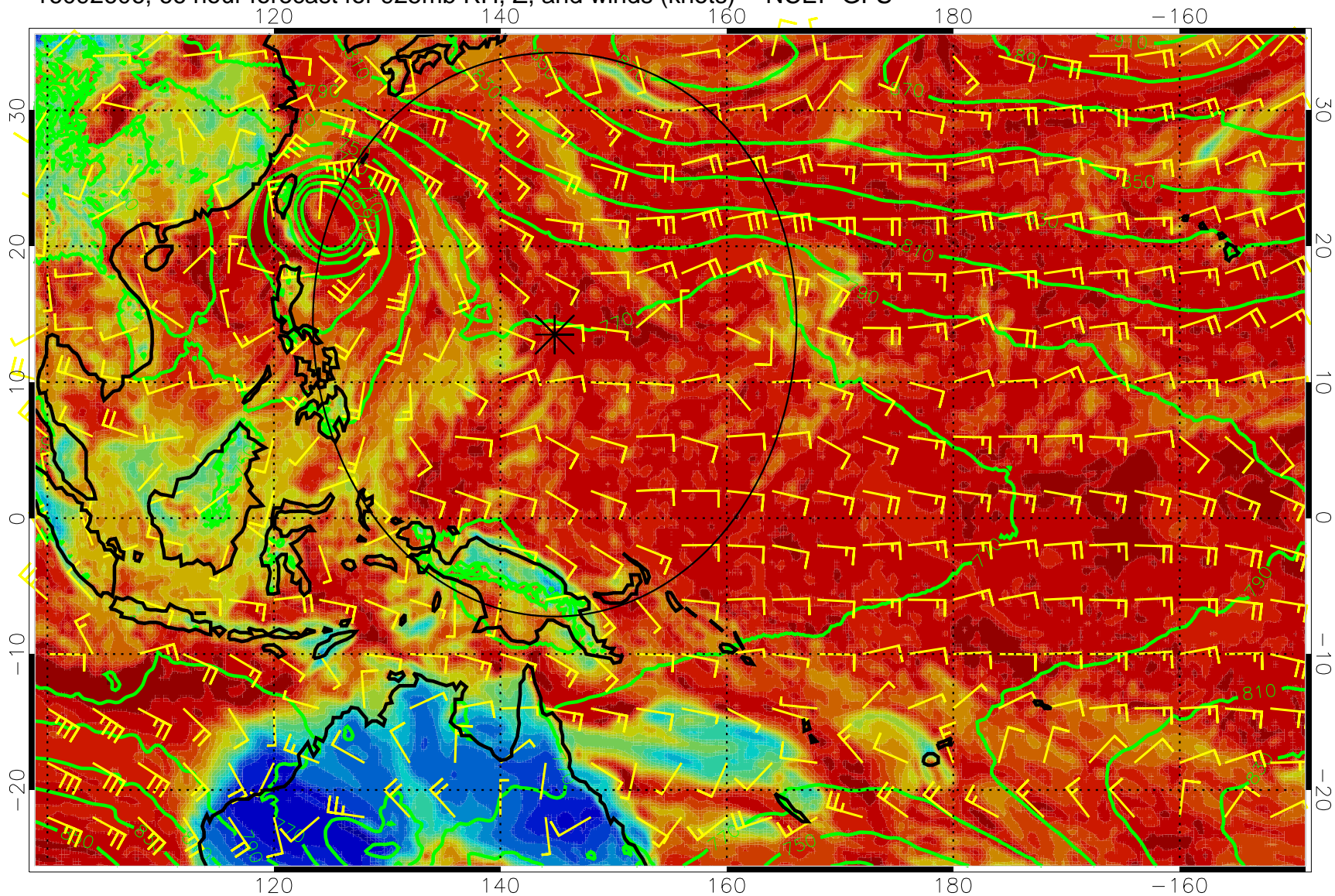
16092606, 66 hour forecast for 925mb RH, Z, and winds (knots) -- NCEP GFS
