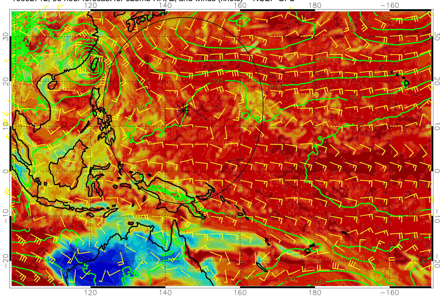
16092712, 96 hour forecast for 925mb RH, Z, and winds (knots) -- NCEP GFS
