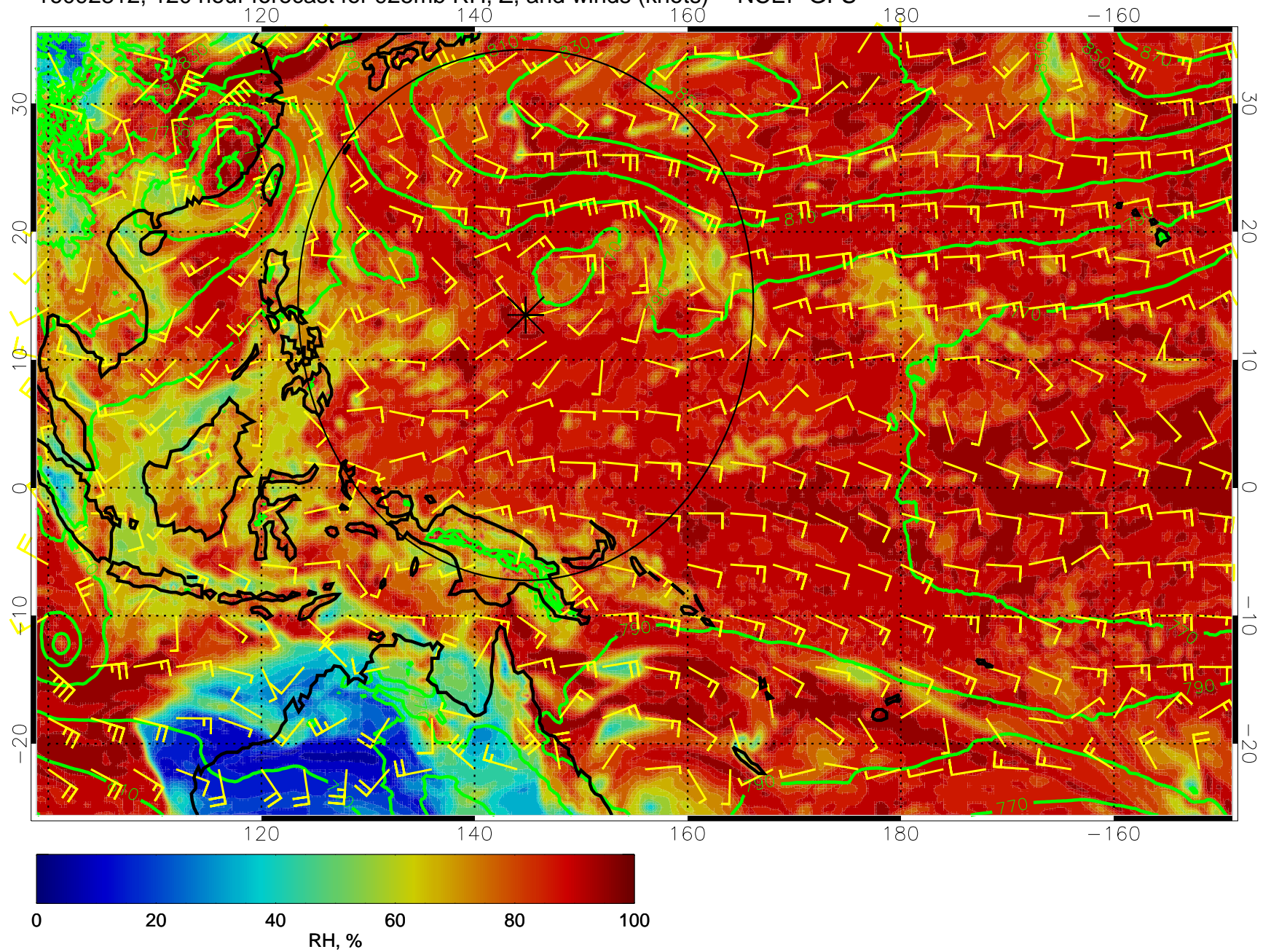
16092812, 120 hour forecast for 925mb RH, Z, and winds (knots) -- NCEP GFS
