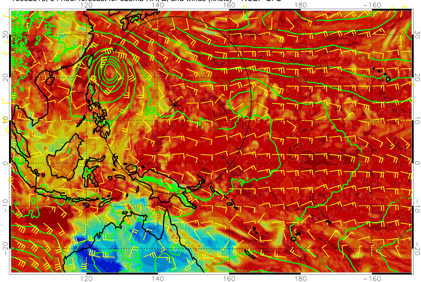
16092518, 54 hour forecast for 925mb RH, Z, and winds (knots) -- NCEP GFS
