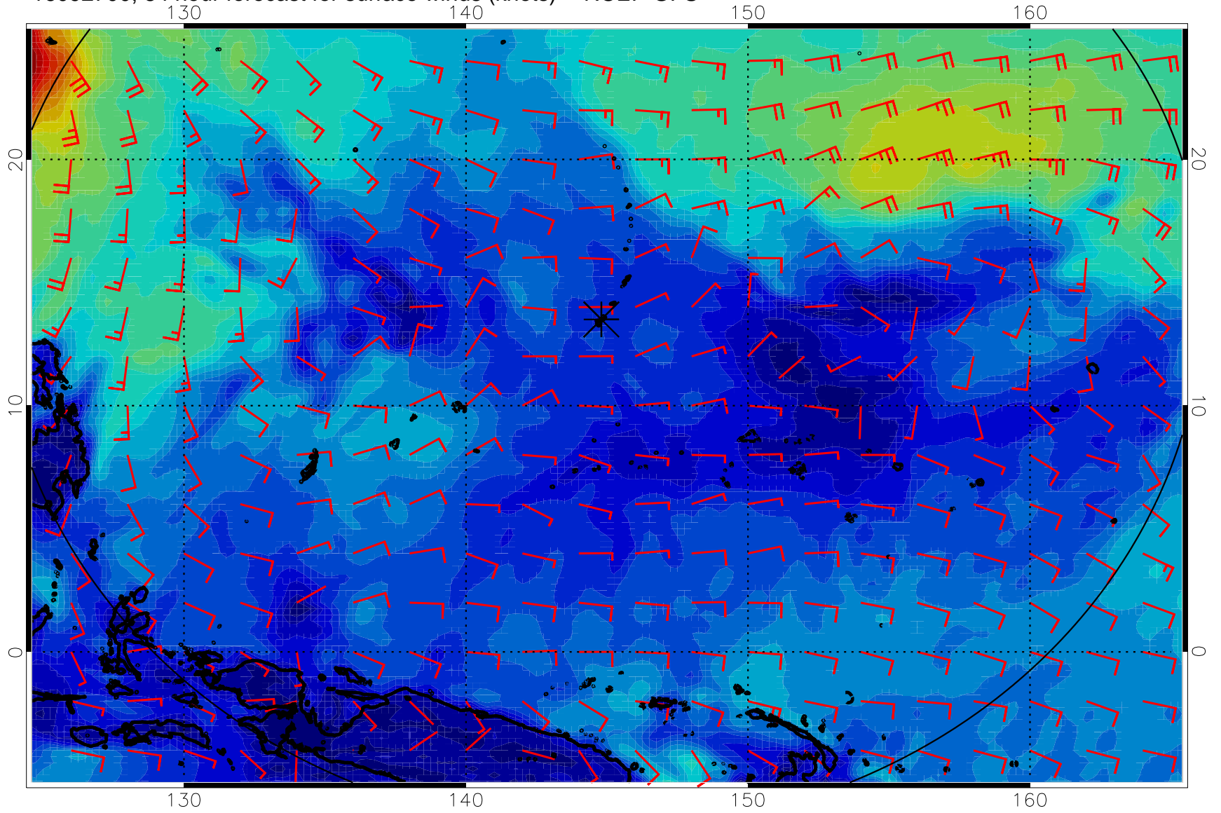
16092700, 84 hour forecast for surface winds (knots) -- NCEP GFS
