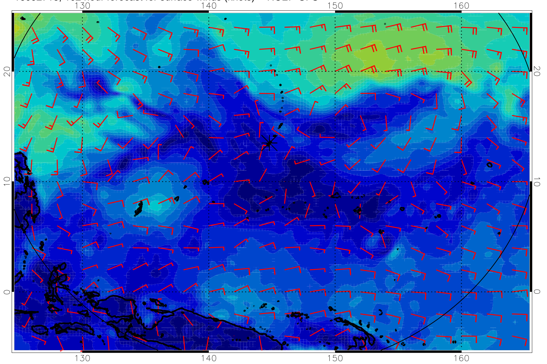
16092718, 102 hour forecast for surface winds (knots) -- NCEP GFS
