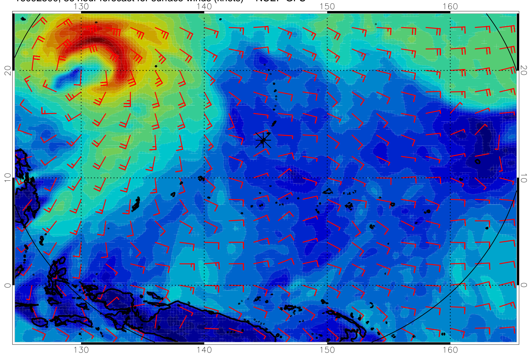
16092500, 36 hour forecast for surface winds (knots) -- NCEP GFS
