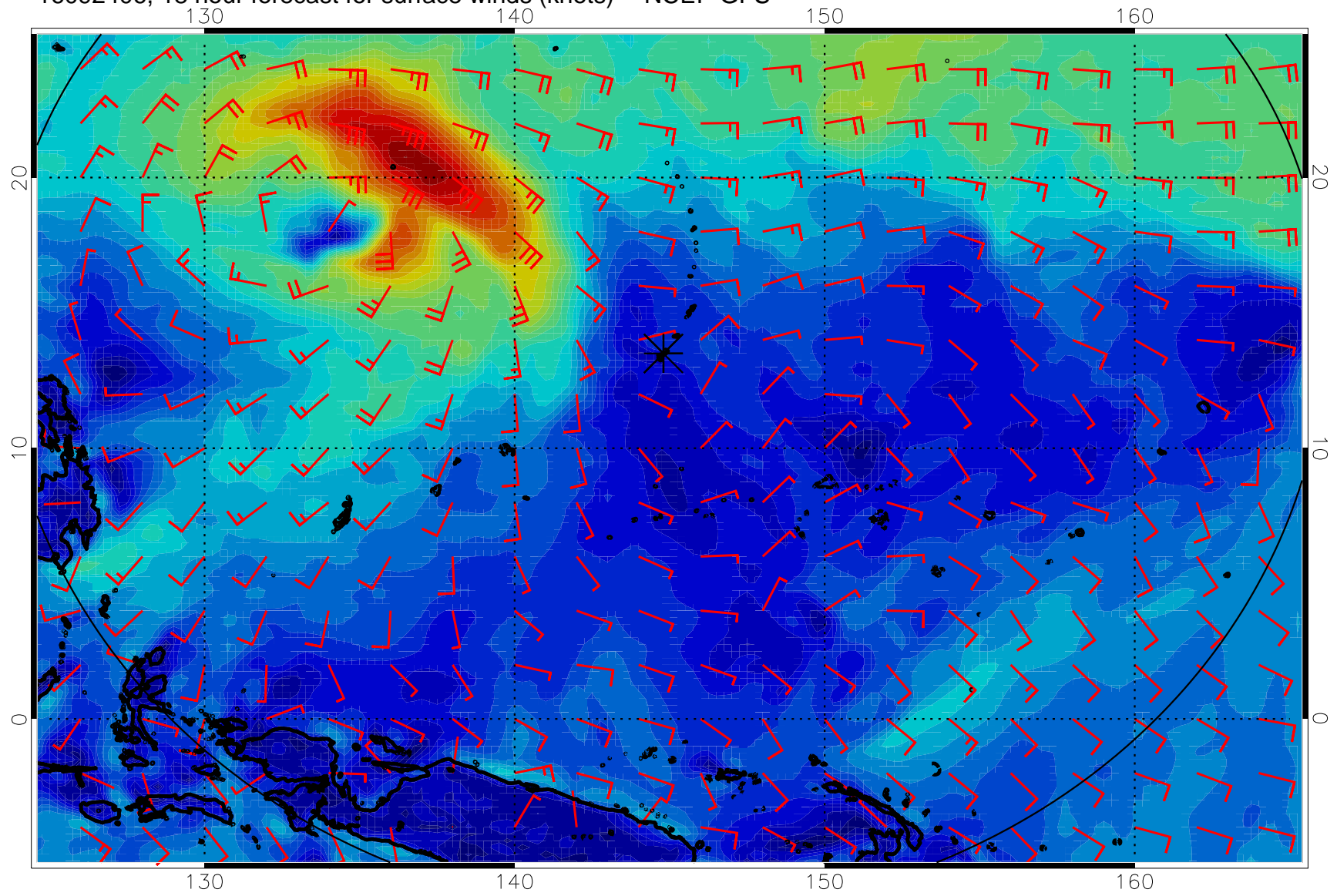
16092406, 18 hour forecast for surface winds (knots) -- NCEP GFS
