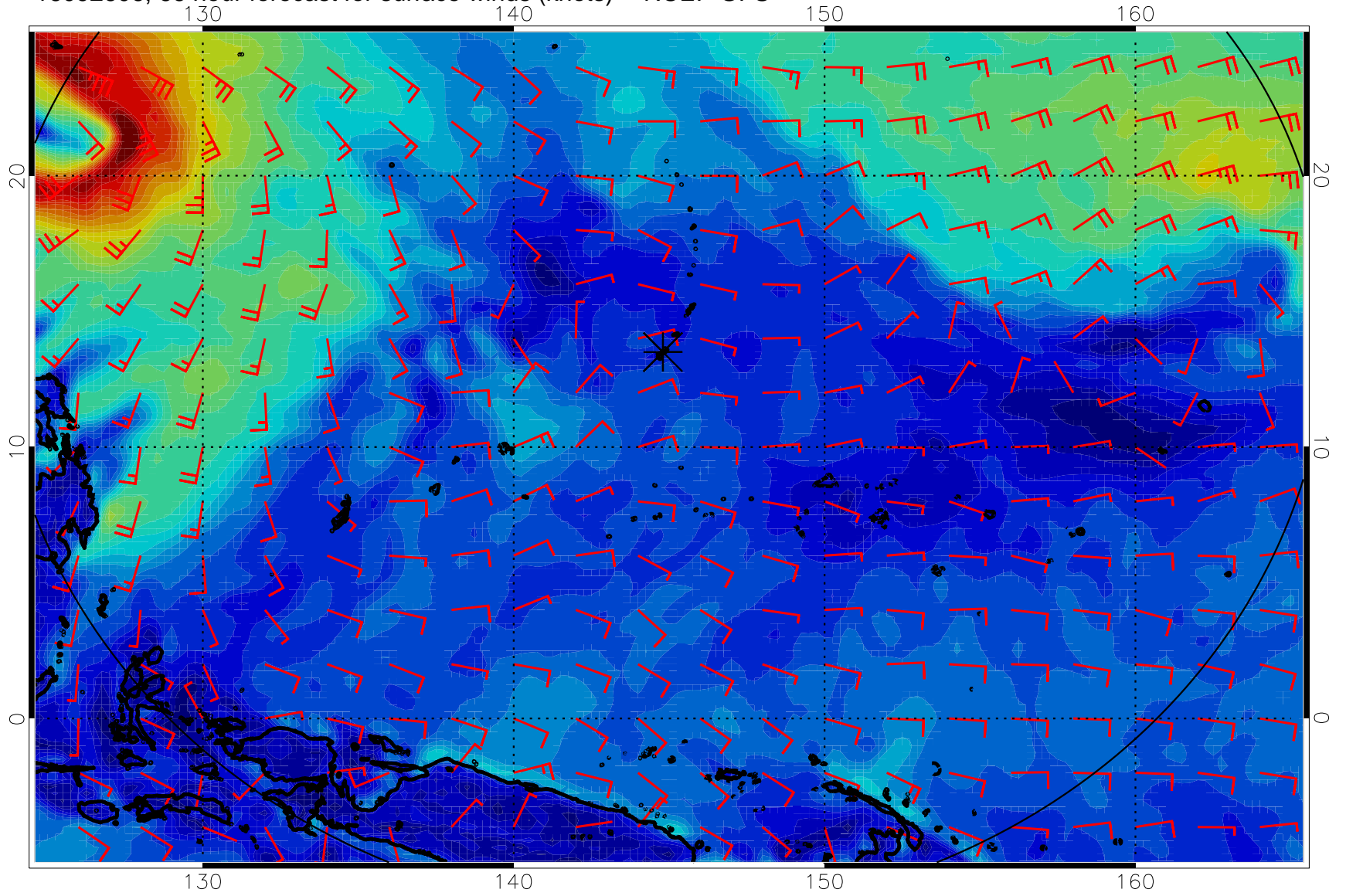
16092606, 66 hour forecast for surface winds (knots) -- NCEP GFS
