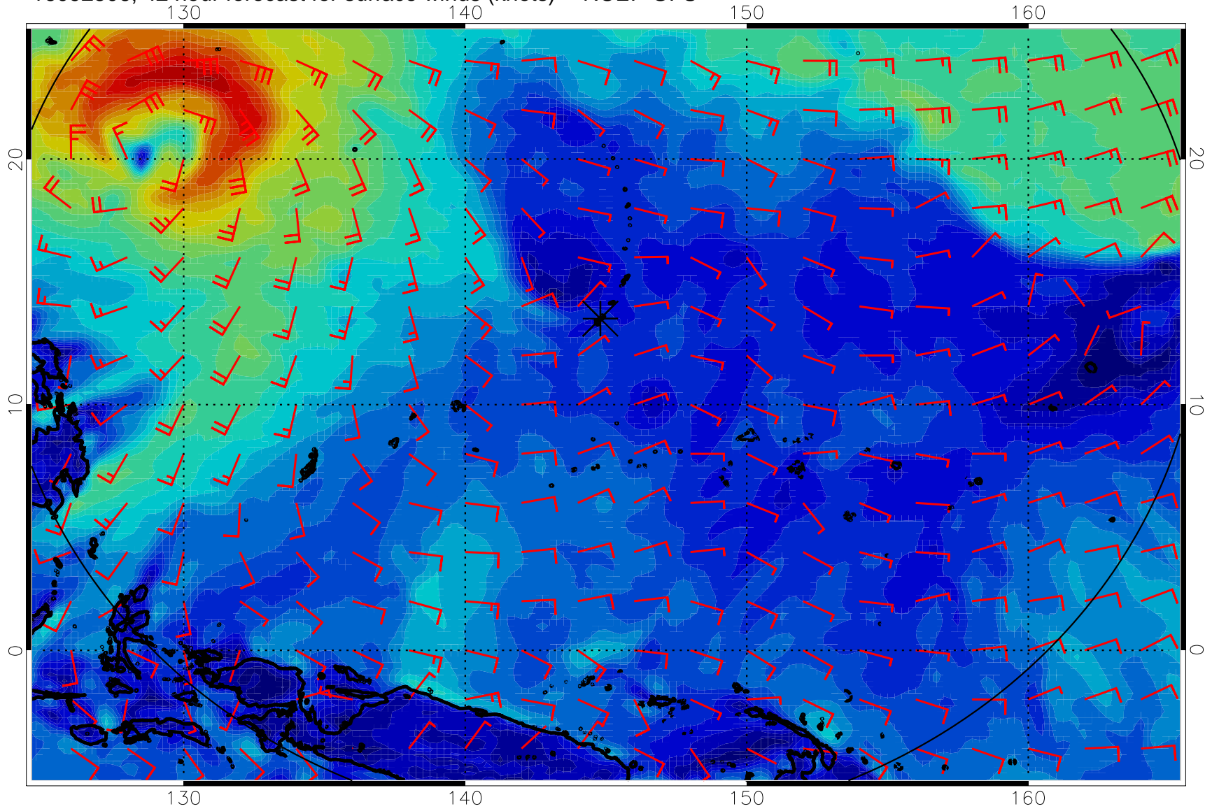
16092506, 42 hour forecast for surface winds (knots) -- NCEP GFS
