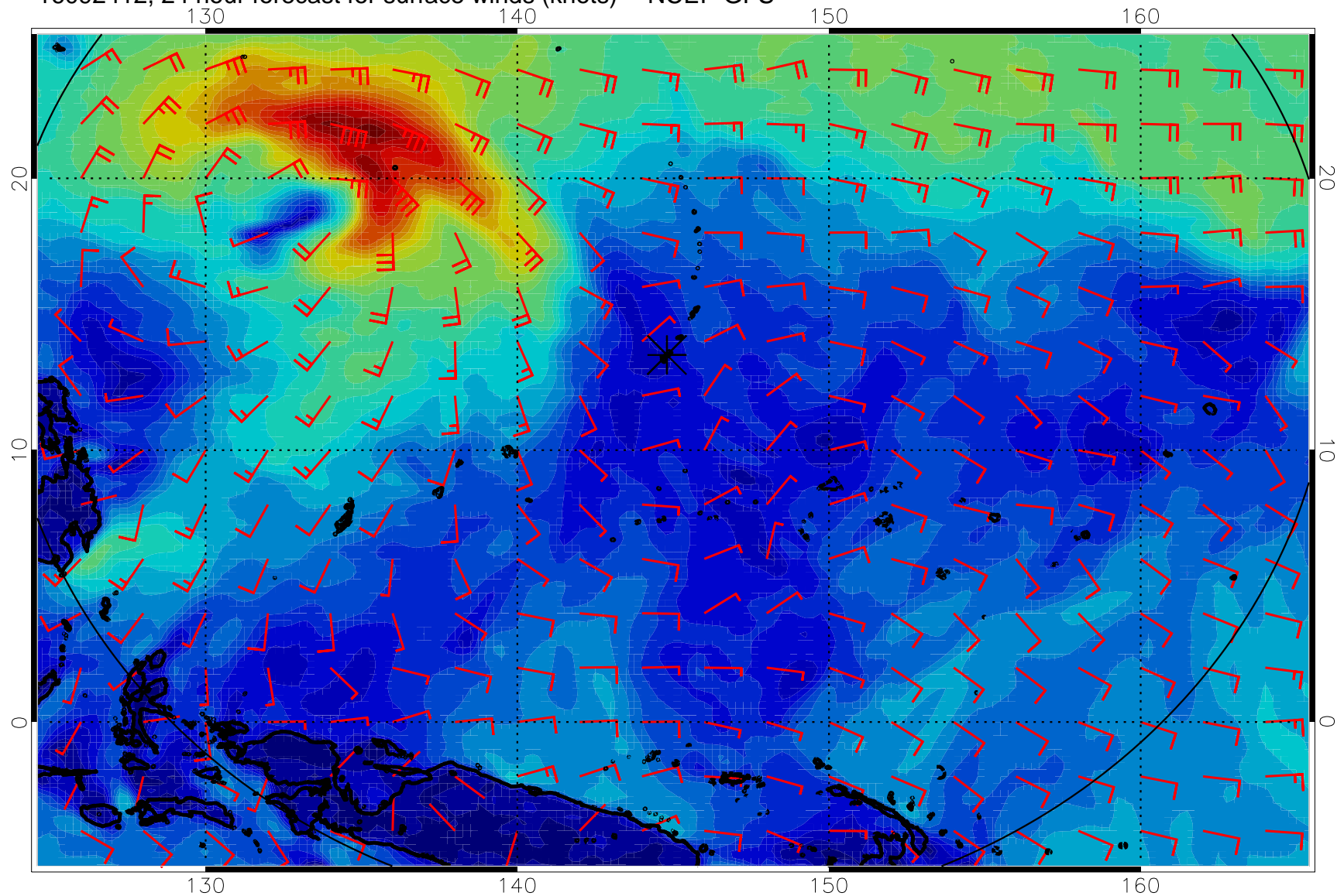
16092412, 24 hour forecast for surface winds (knots) -- NCEP GFS
