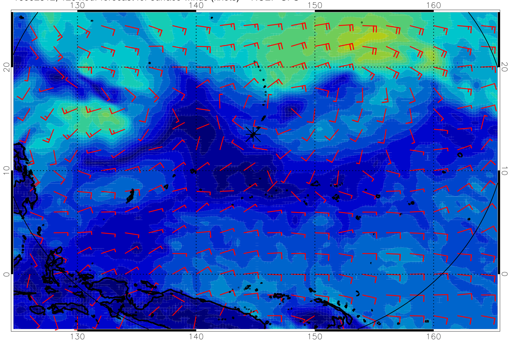
16092812, 120 hour forecast for surface winds (knots) -- NCEP GFS
