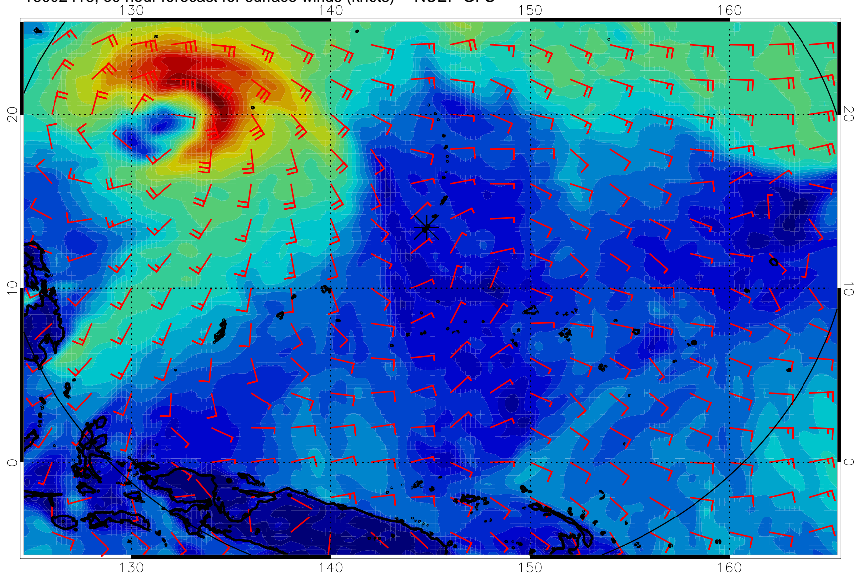
16092418, 30 hour forecast for surface winds (knots) -- NCEP GFS
