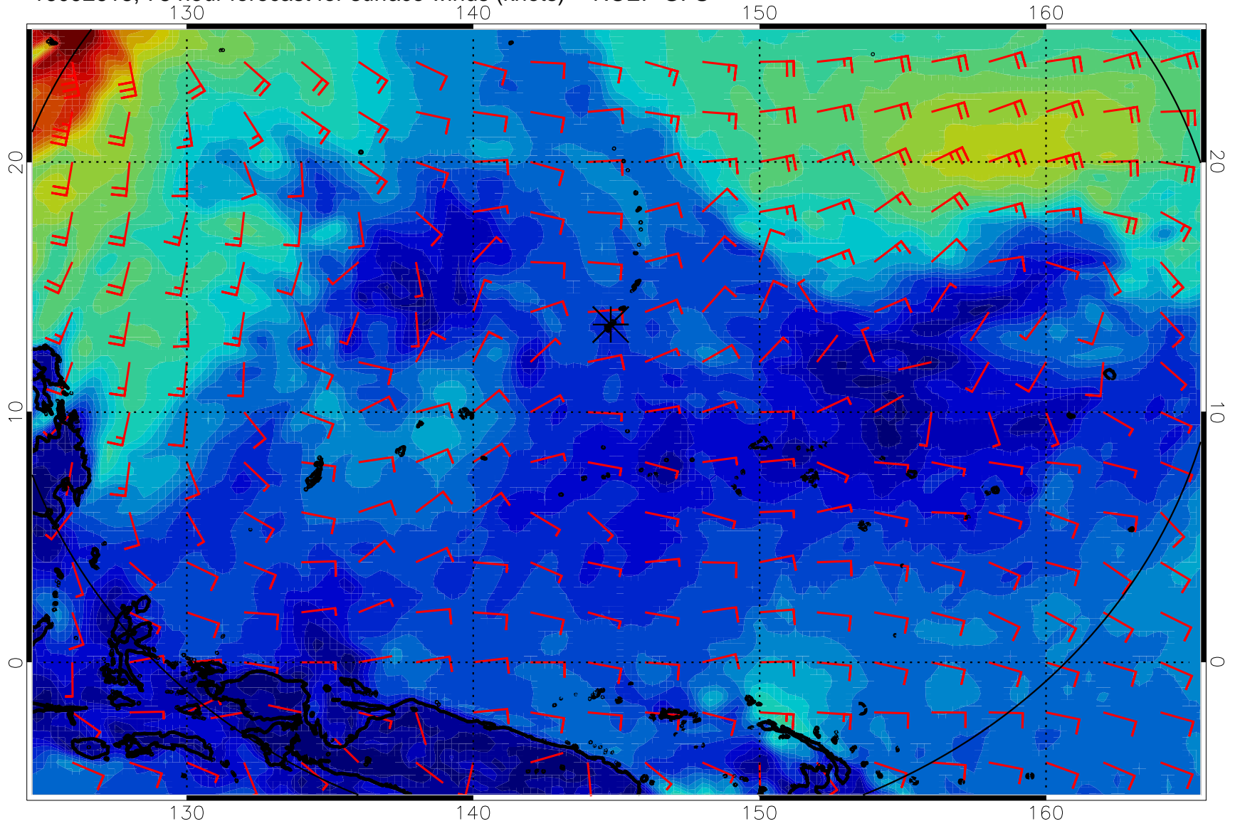
16092618, 78 hour forecast for surface winds (knots) -- NCEP GFS
