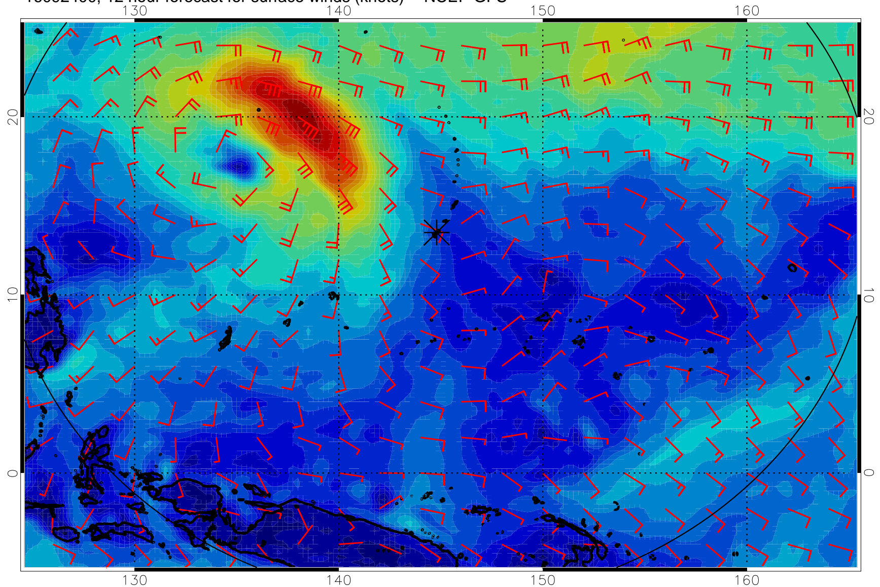
16092400, 12 hour forecast for surface winds (knots) -- NCEP GFS
