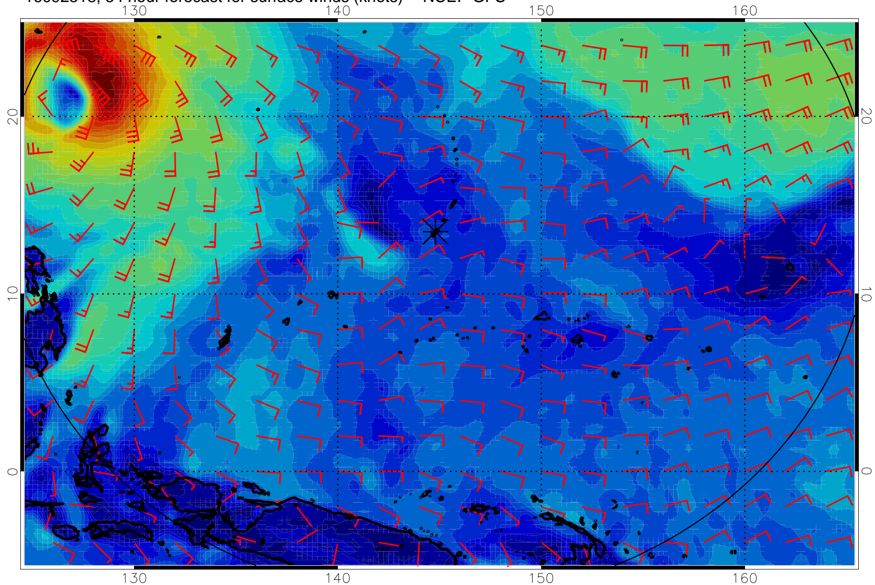
16092518, 54 hour forecast for surface winds (knots) -- NCEP GFS
