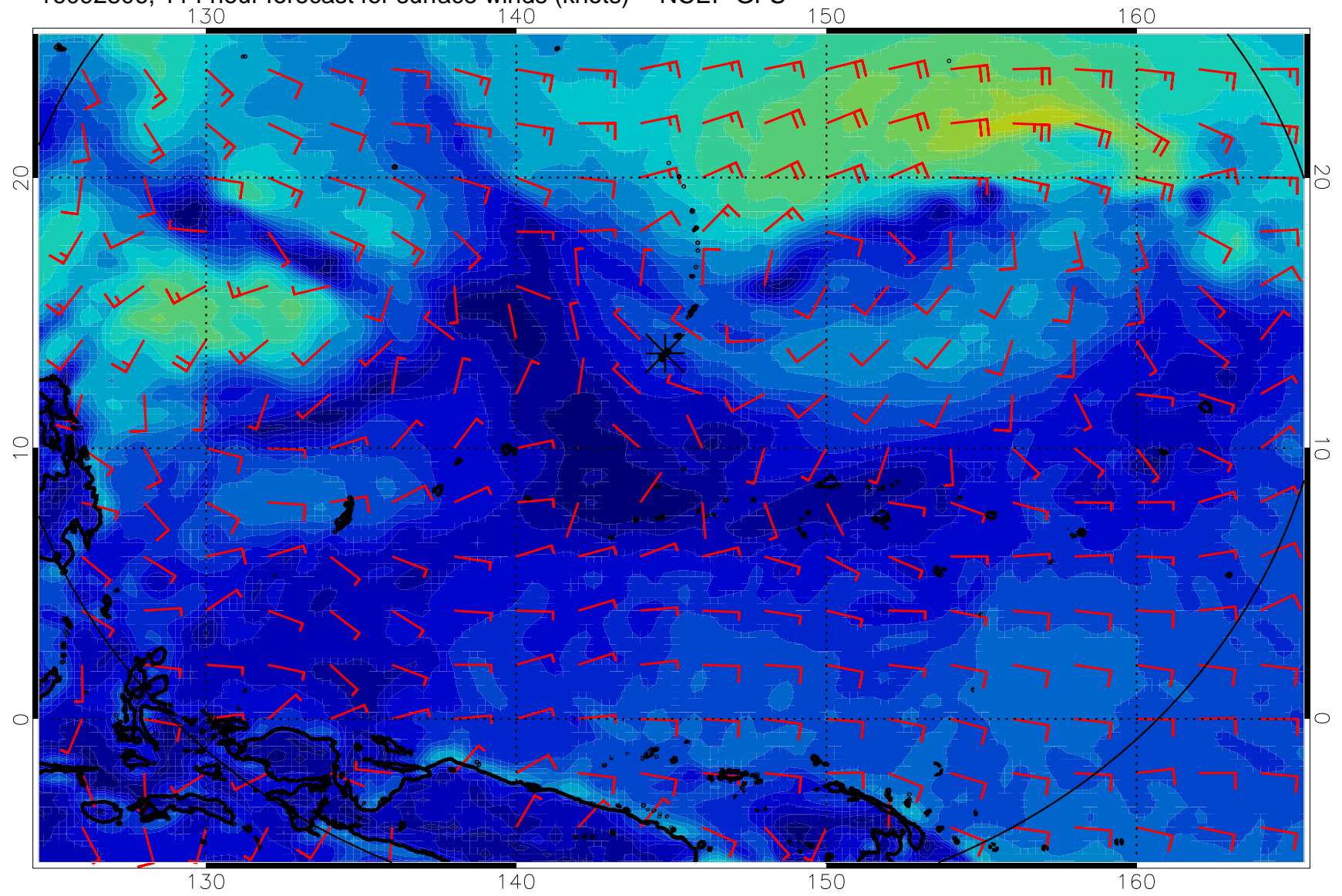
16092806, 114 hour forecast for surface winds (knots) -- NCEP GFS
