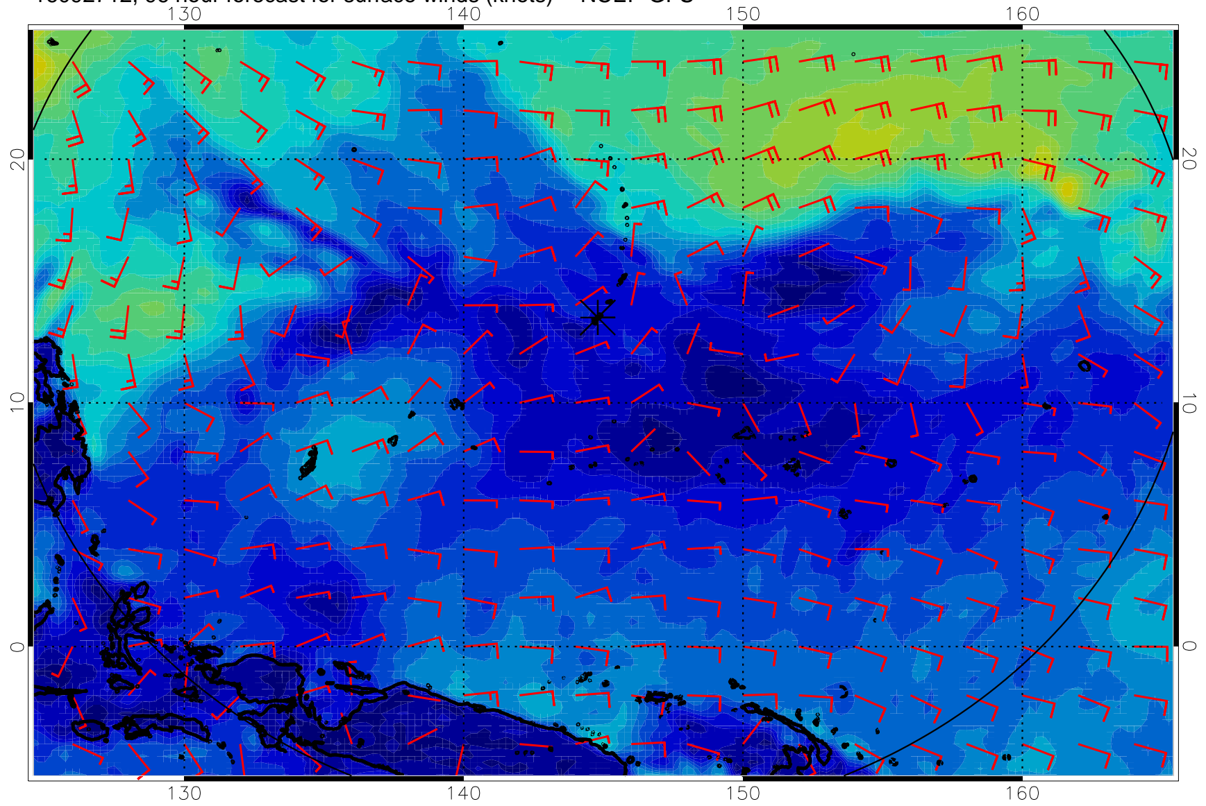
16092712, 96 hour forecast for surface winds (knots) -- NCEP GFS
