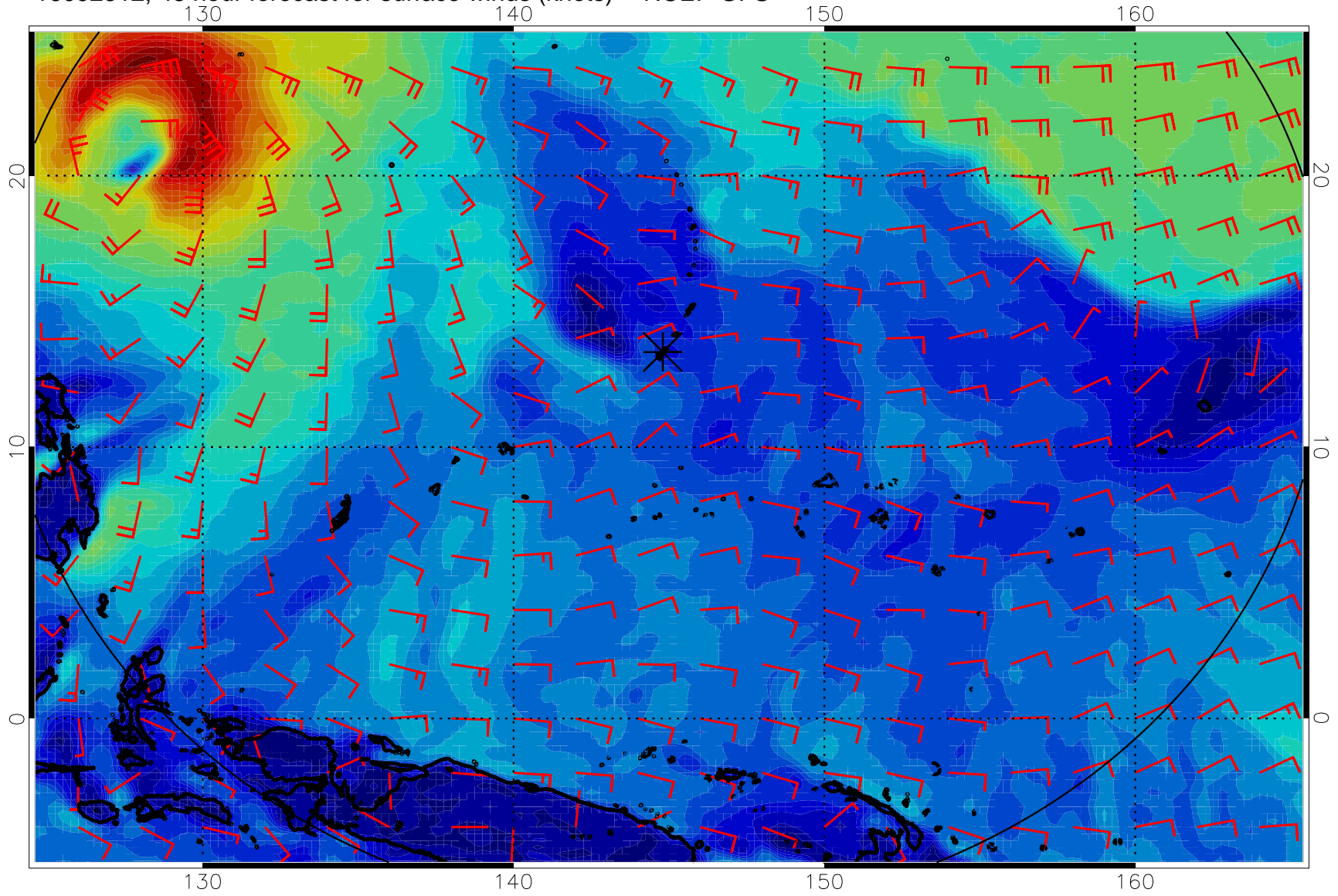
16092512, 48 hour forecast for surface winds (knots) -- NCEP GFS
