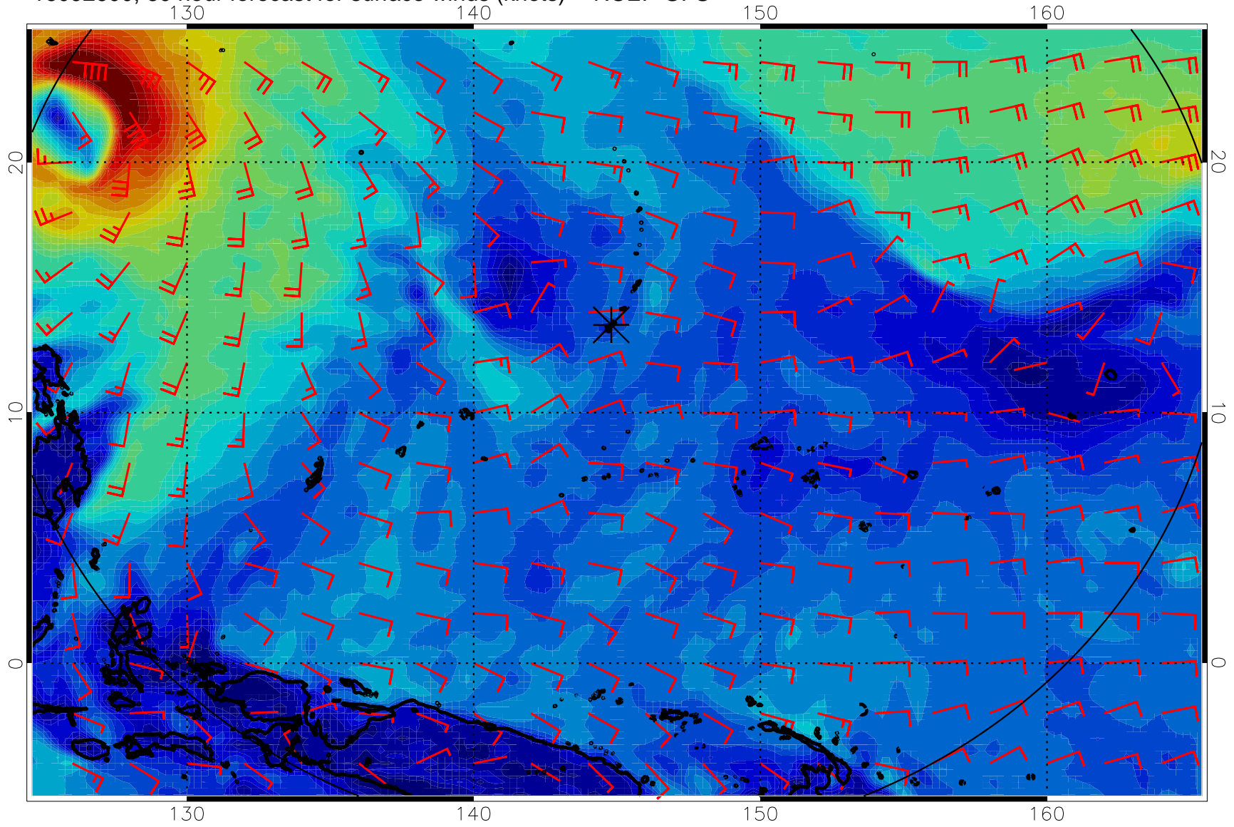
16092600, 60 hour forecast for surface winds (knots) -- NCEP GFS
