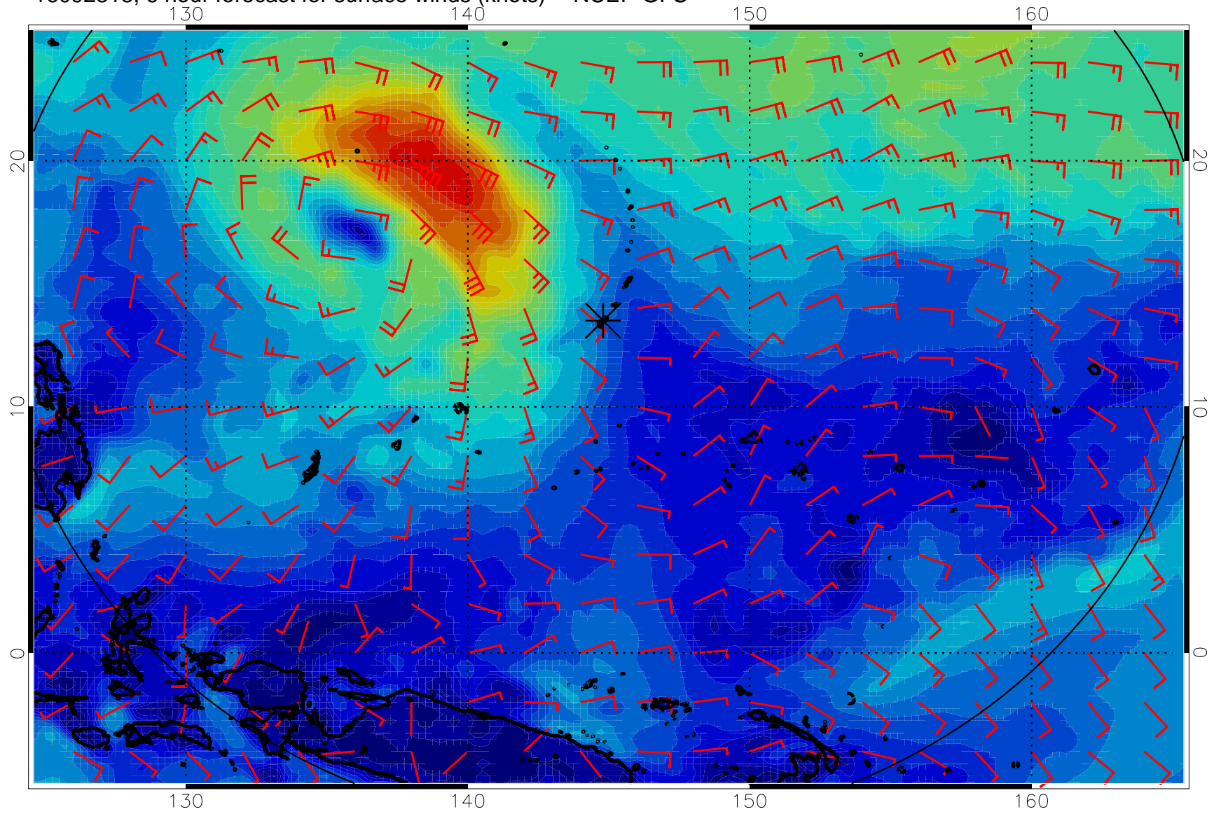
16092318, 6 hour forecast for surface winds (knots) -- NCEP GFS
