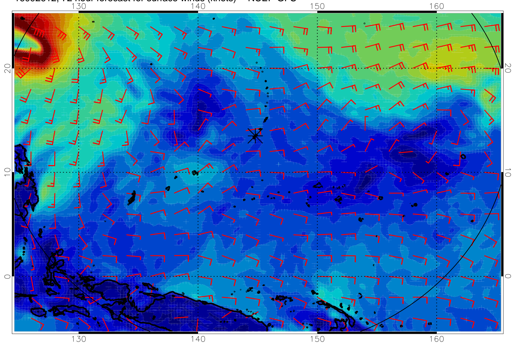
16092612, 72 hour forecast for surface winds (knots) -- NCEP GFS
