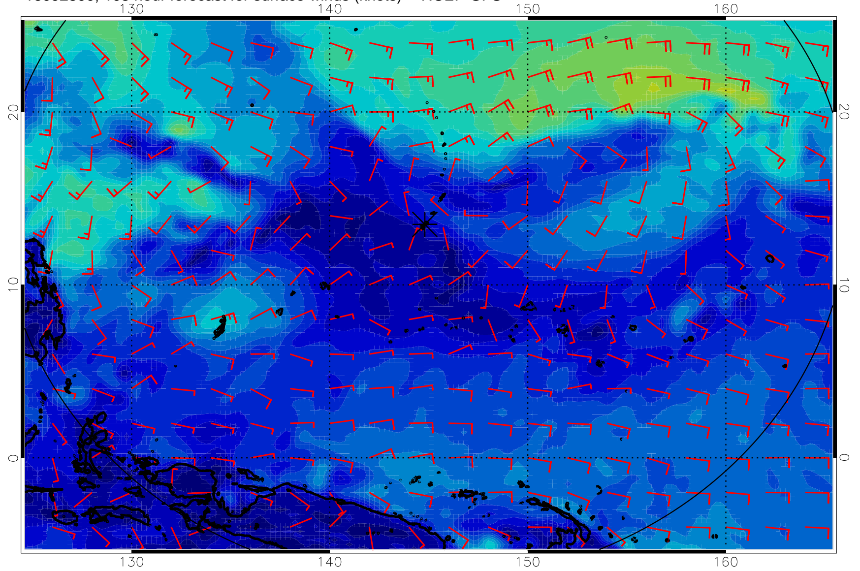
16092800, 108 hour forecast for surface winds (knots) -- NCEP GFS
