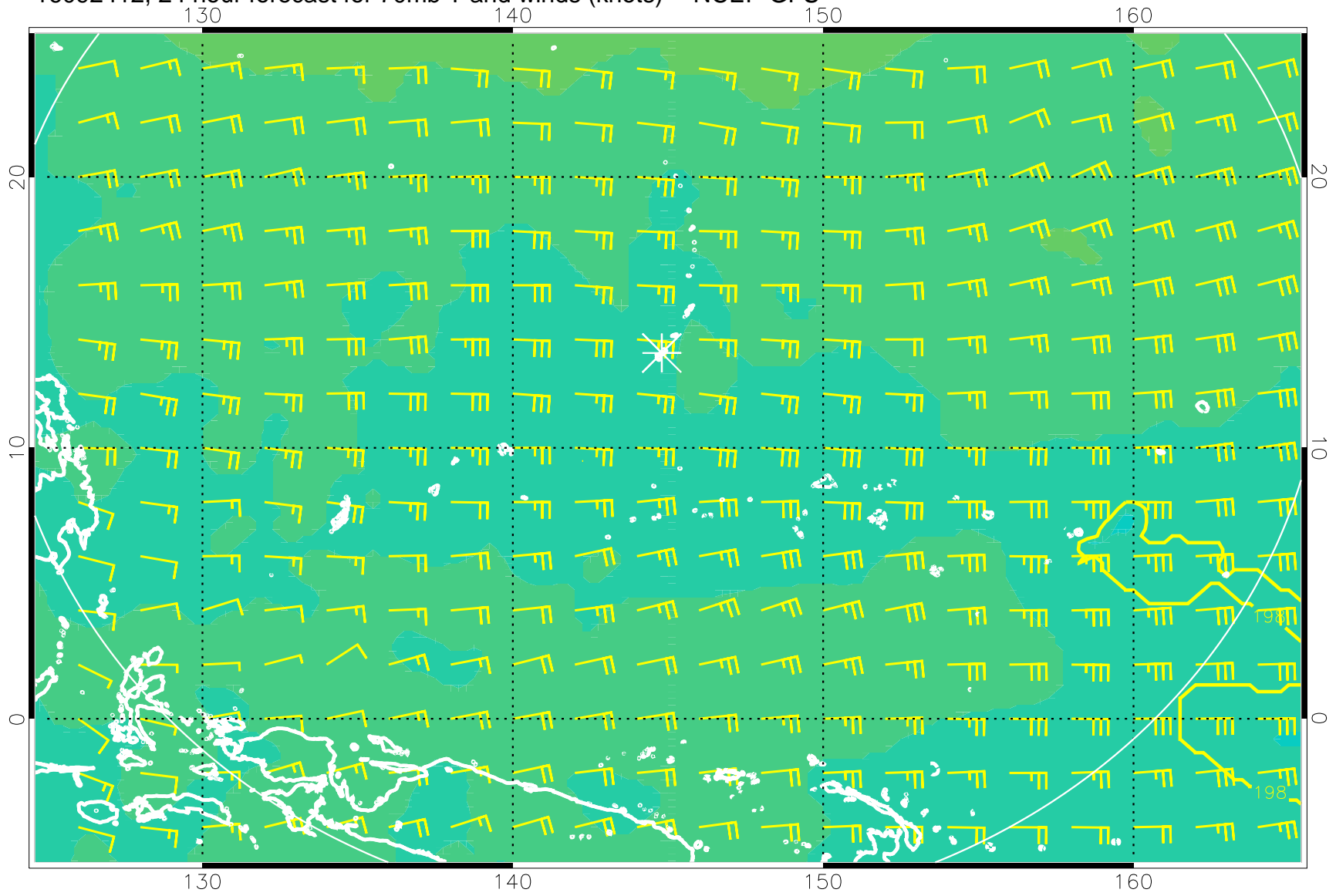
16092412, 24 hour forecast for 70mb T and winds (knots) -- NCEP GFS
