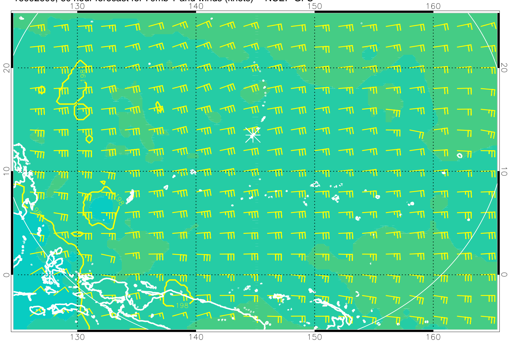
16092600, 60 hour forecast for 70mb T and winds (knots) -- NCEP GFS
