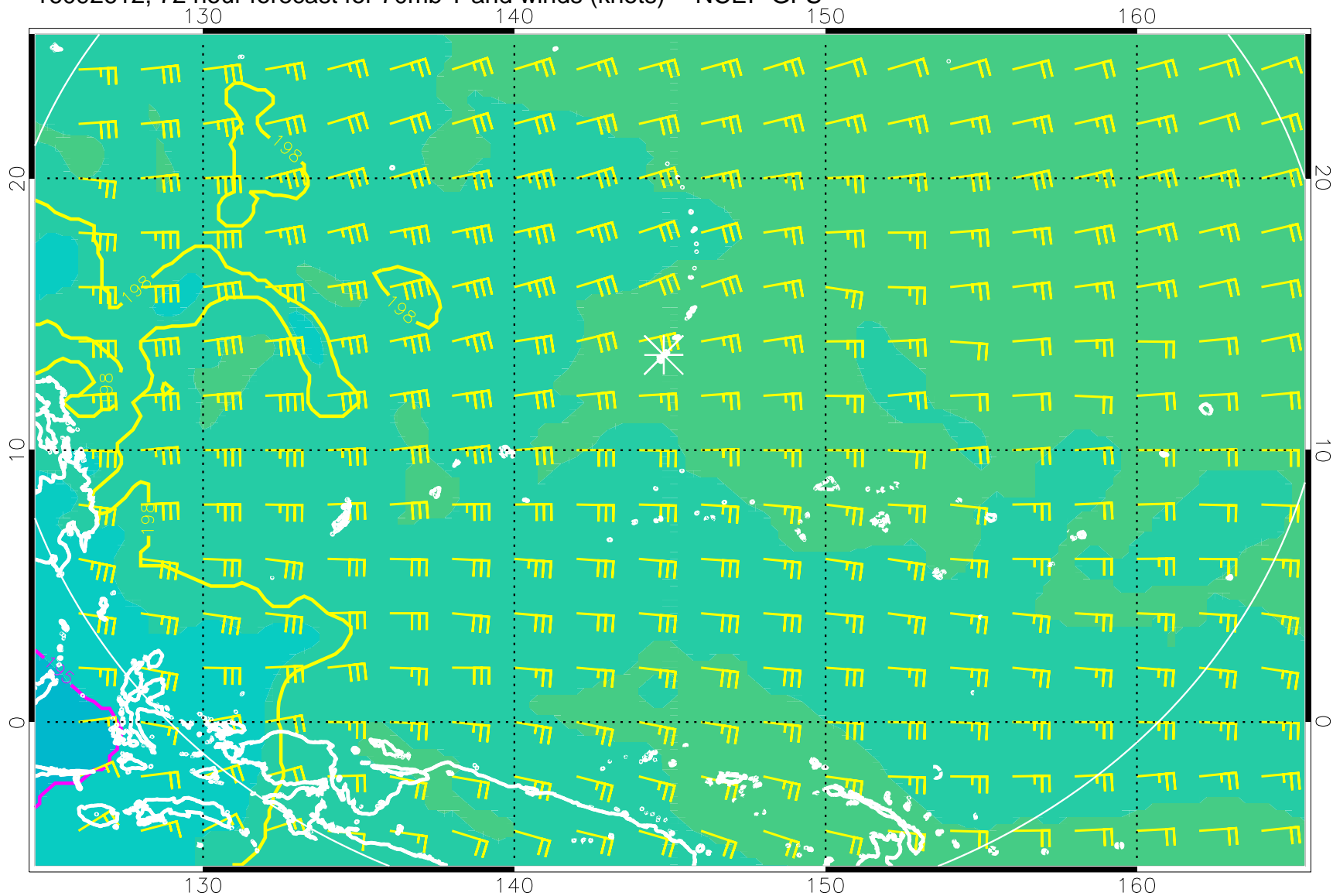
16092612, 72 hour forecast for 70mb T and winds (knots) -- NCEP GFS
