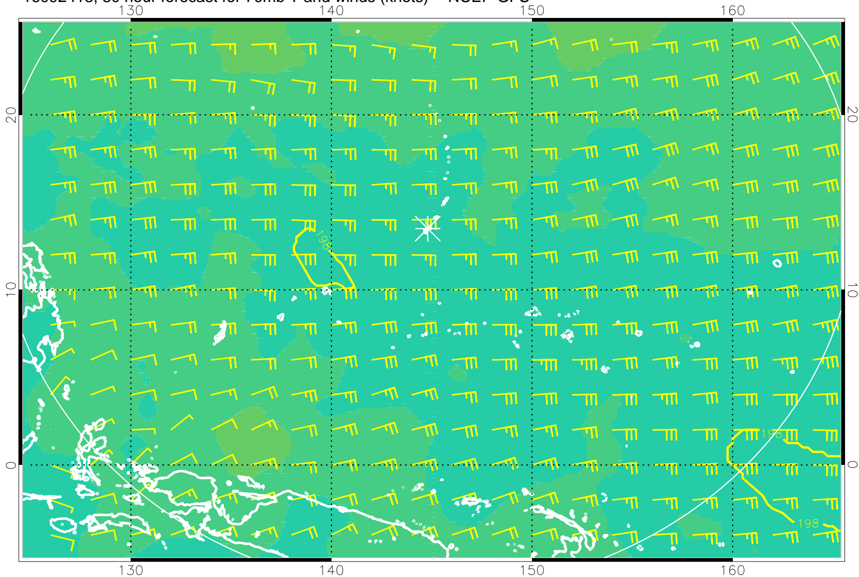
16092418, 30 hour forecast for 70mb T and winds (knots) -- NCEP GFS
