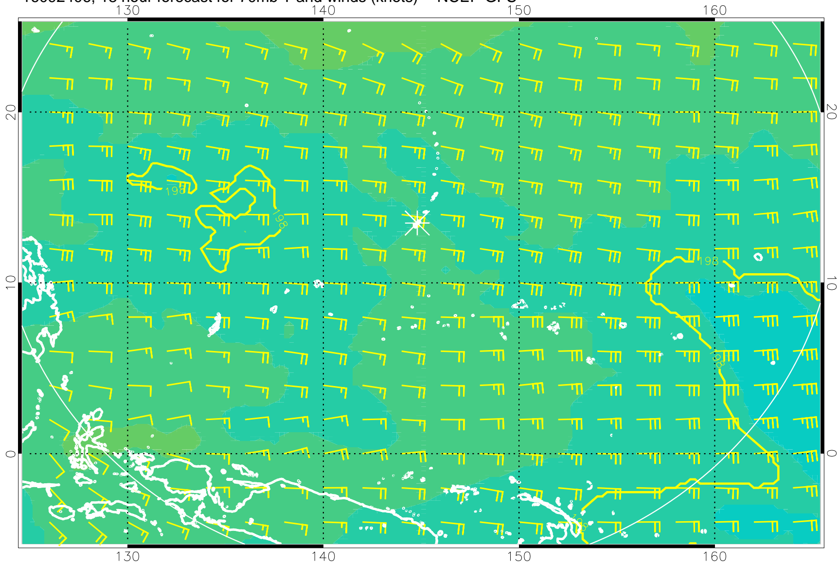
16092406, 18 hour forecast for 70mb T and winds (knots) -- NCEP GFS
