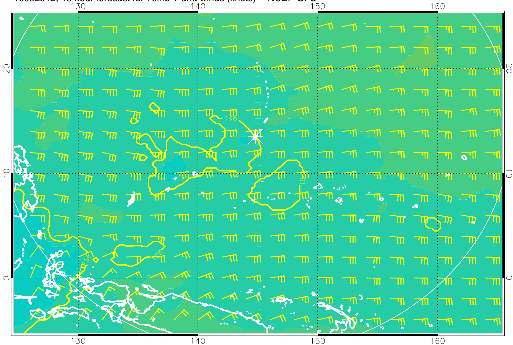
16092512, 48 hour forecast for 70mb T and winds (knots) -- NCEP GFS
