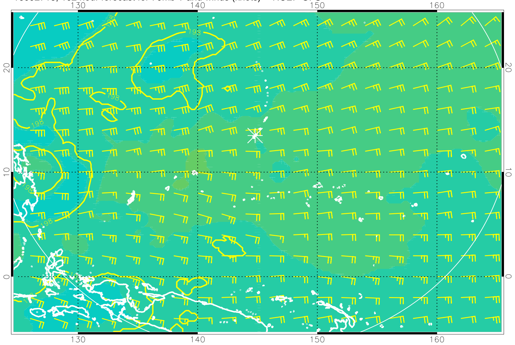
16092718, 102 hour forecast for 70mb T and winds (knots) -- NCEP GFS
