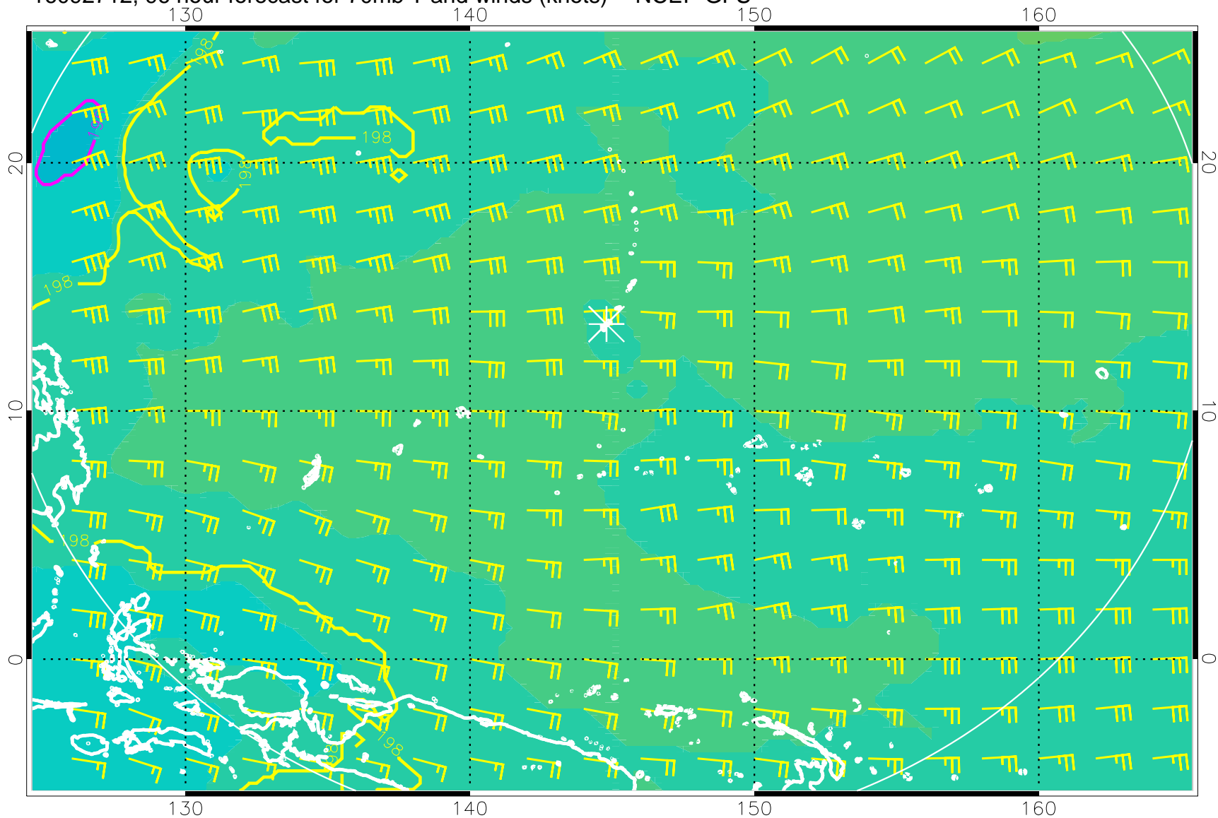
16092712, 96 hour forecast for 70mb T and winds (knots) -- NCEP GFS
