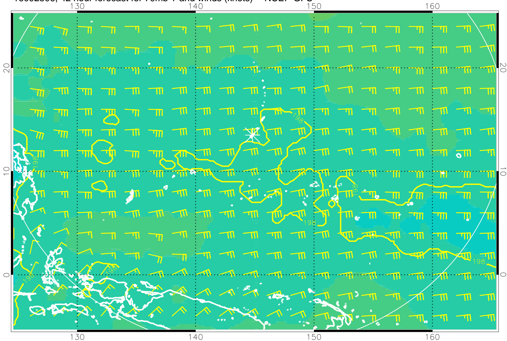
16092506, 42 hour forecast for 70mb T and winds (knots) -- NCEP GFS
