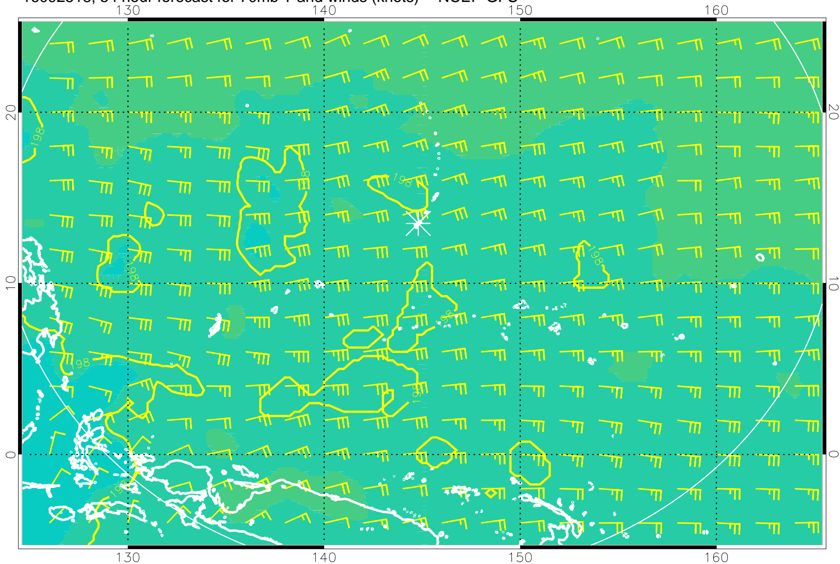
16092518, 54 hour forecast for 70mb T and winds (knots) -- NCEP GFS
