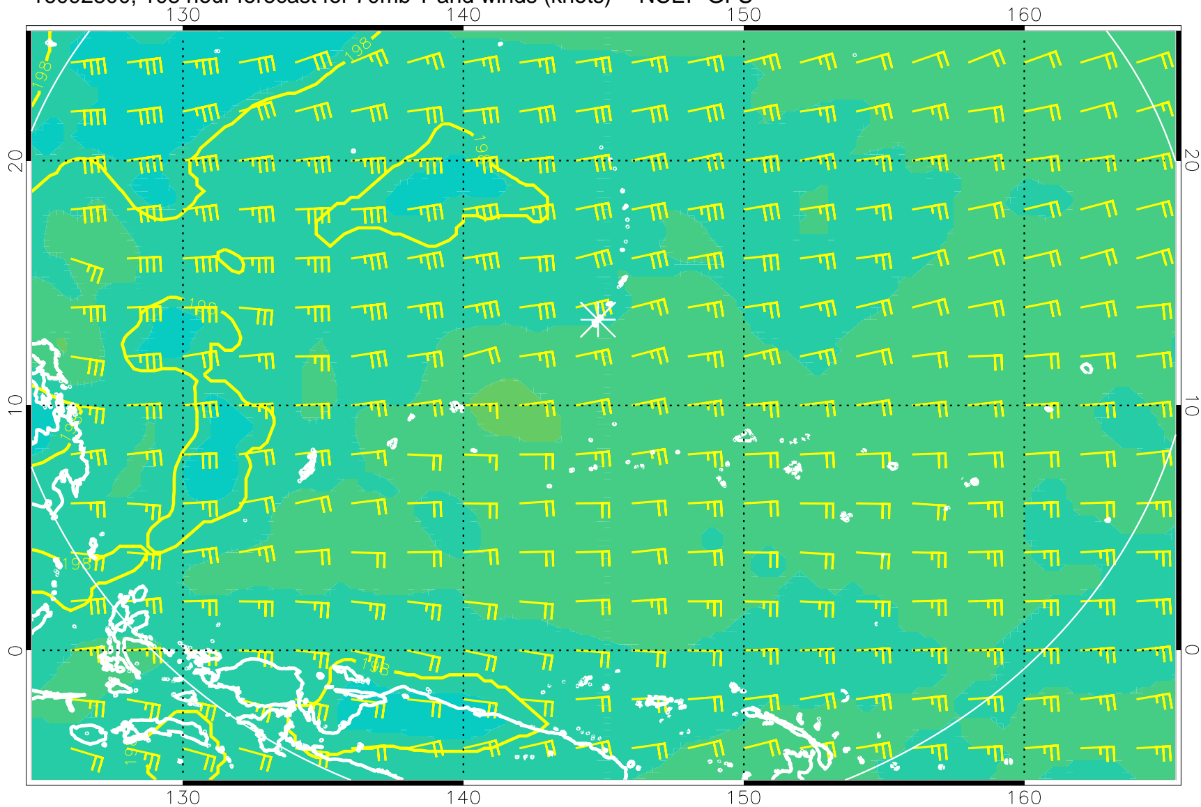
16092800, 108 hour forecast for 70mb T and winds (knots) -- NCEP GFS
