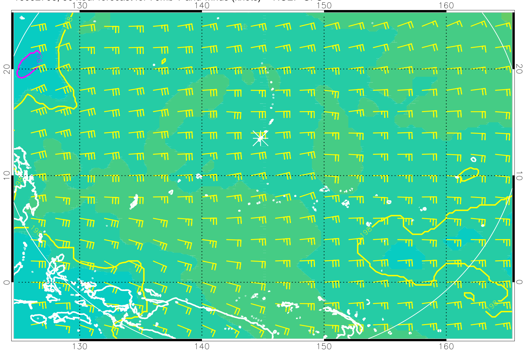
16092706, 90 hour forecast for 70mb T and winds (knots) -- NCEP GFS
