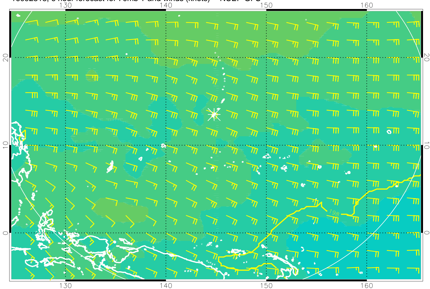
16092318, 6 hour forecast for 70mb T and winds (knots) -- NCEP GFS
