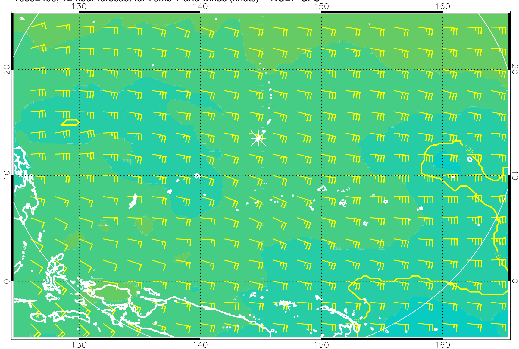
16092400, 12 hour forecast for 70mb T and winds (knots) -- NCEP GFS
