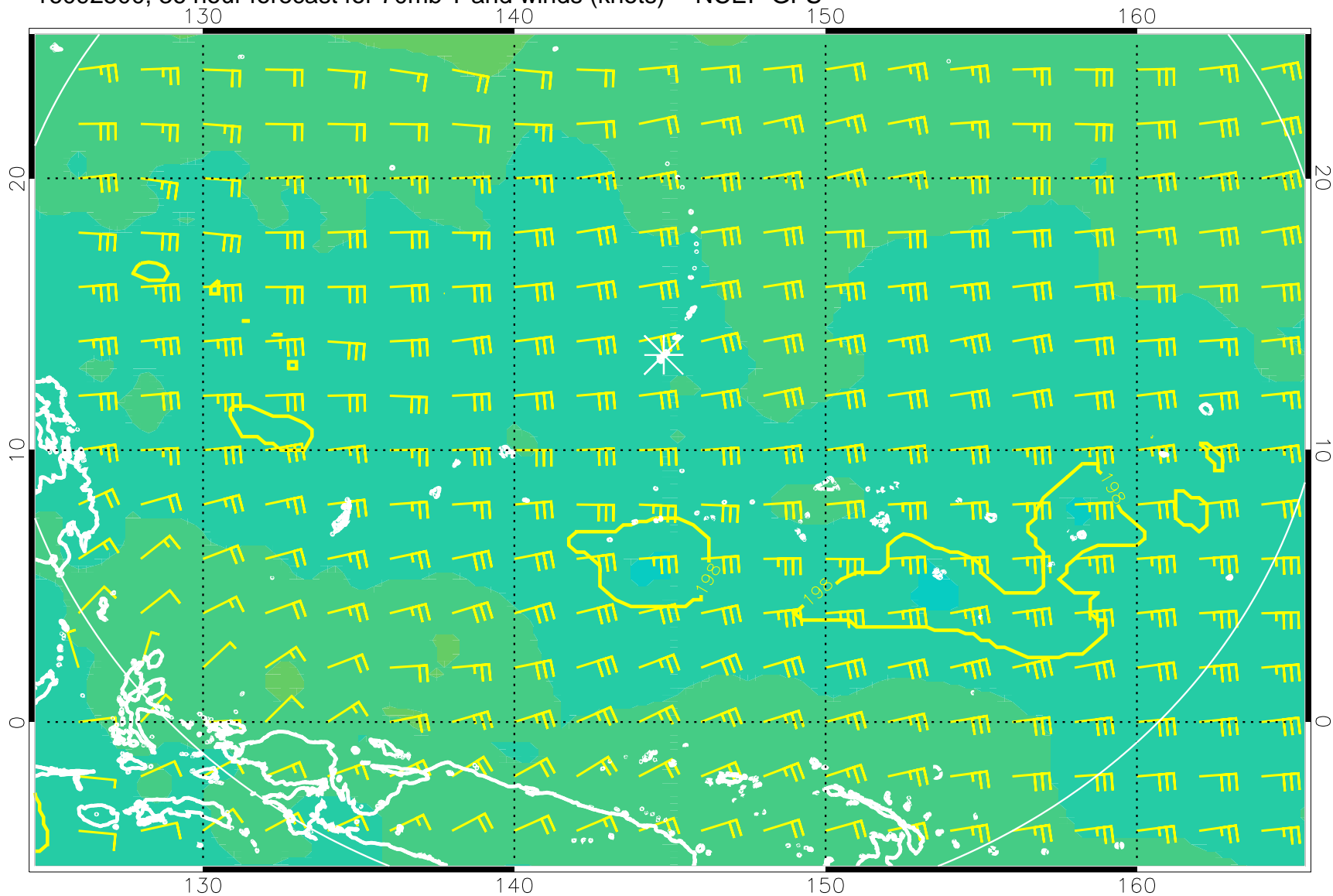
16092500, 36 hour forecast for 70mb T and winds (knots) -- NCEP GFS
