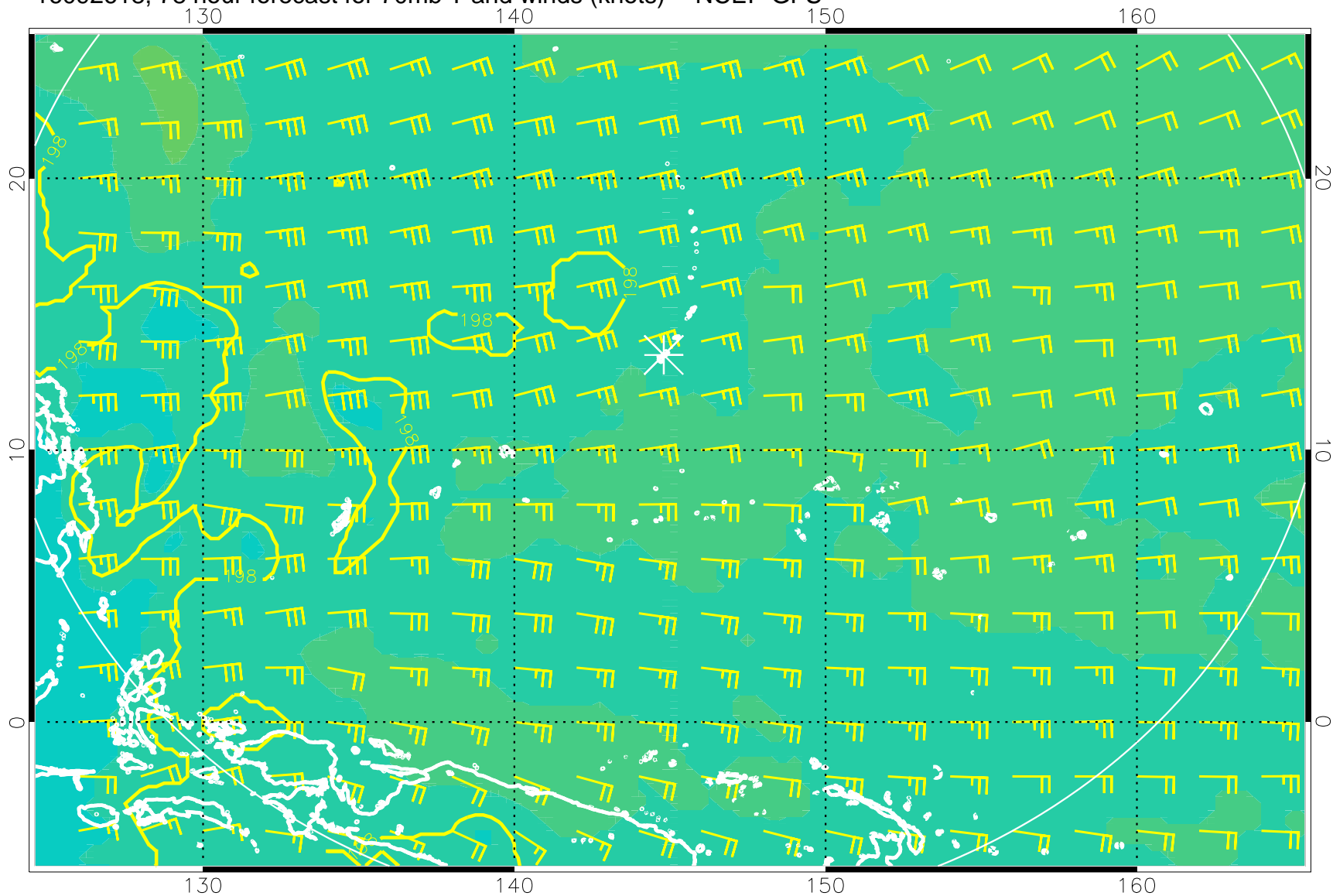
16092618, 78 hour forecast for 70mb T and winds (knots) -- NCEP GFS
