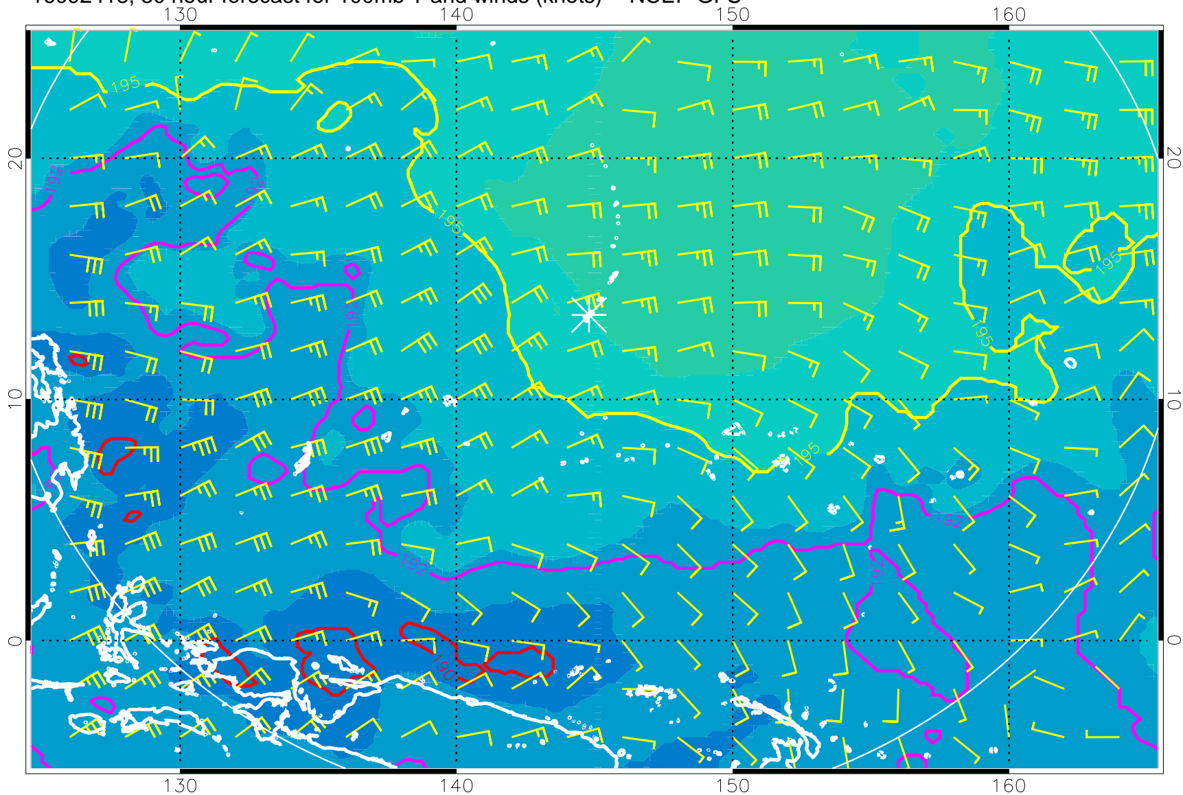
16092418, 30 hour forecast for 100mb T and winds (knots) -- NCEP GFS
