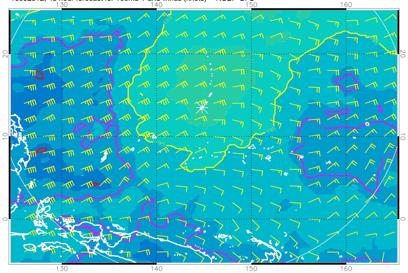
16092512, 48 hour forecast for 100mb T and winds (knots) -- NCEP GFS
