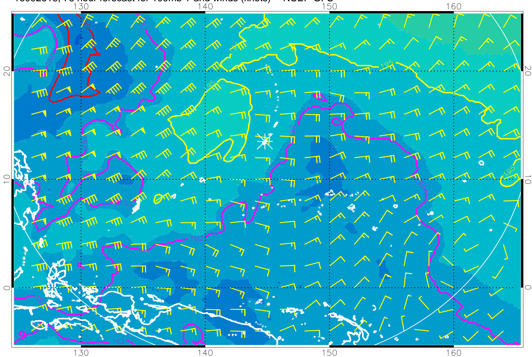
16092618, 78 hour forecast for 100mb T and winds (knots) -- NCEP GFS
