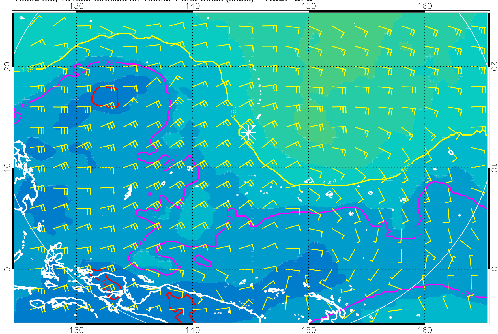
16092406, 18 hour forecast for 100mb T and winds (knots) -- NCEP GFS
