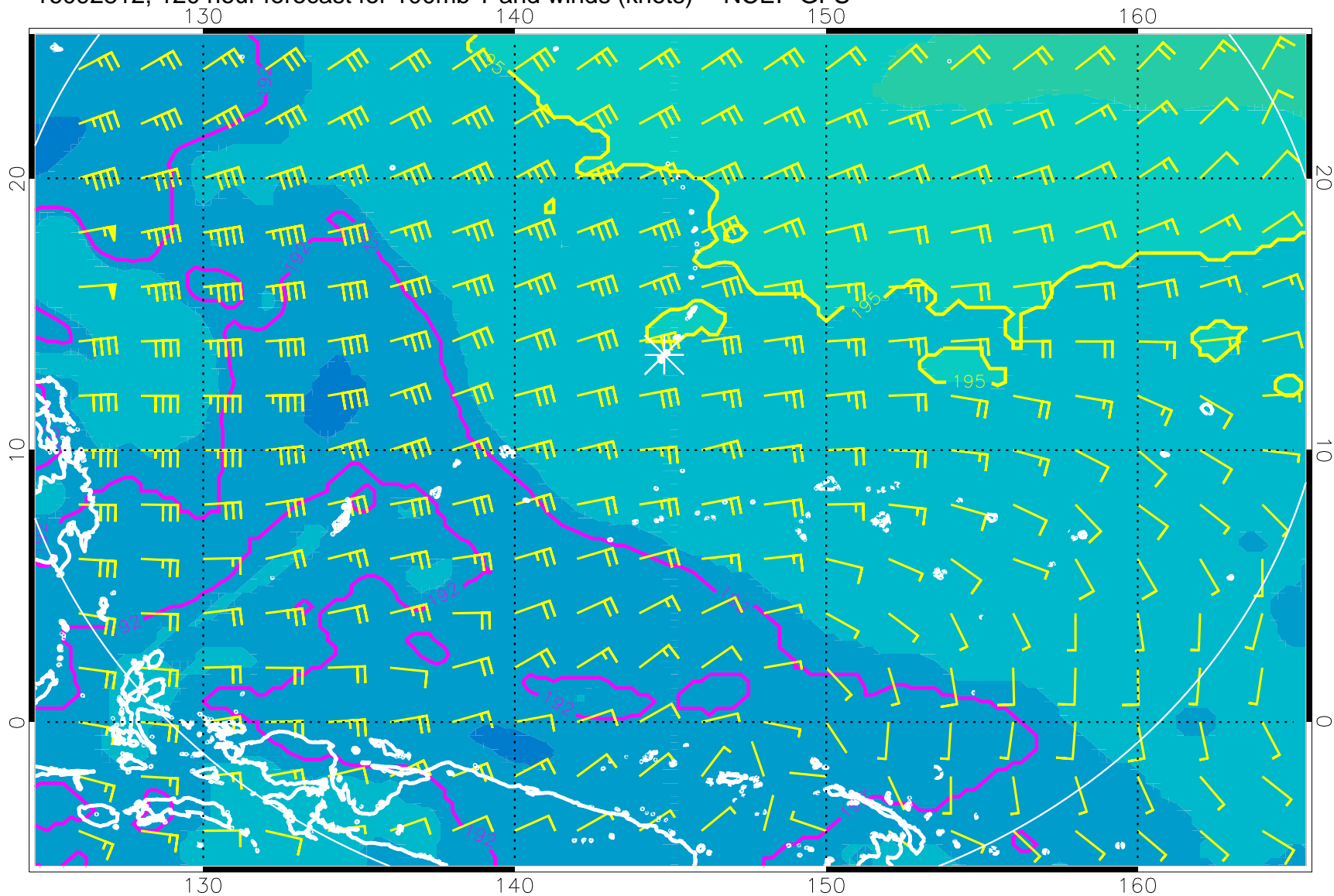
16092812, 120 hour forecast for 100mb T and winds (knots) -- NCEP GFS
