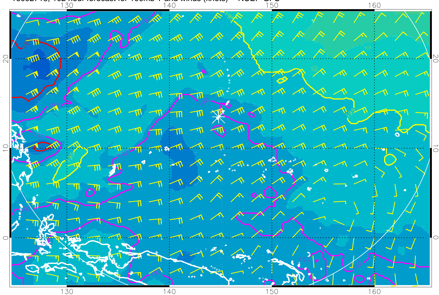
16092718, 102 hour forecast for 100mb T and winds (knots) -- NCEP GFS
