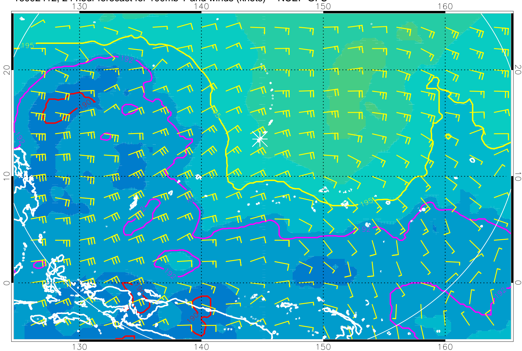
16092412, 24 hour forecast for 100mb T and winds (knots) -- NCEP GFS
