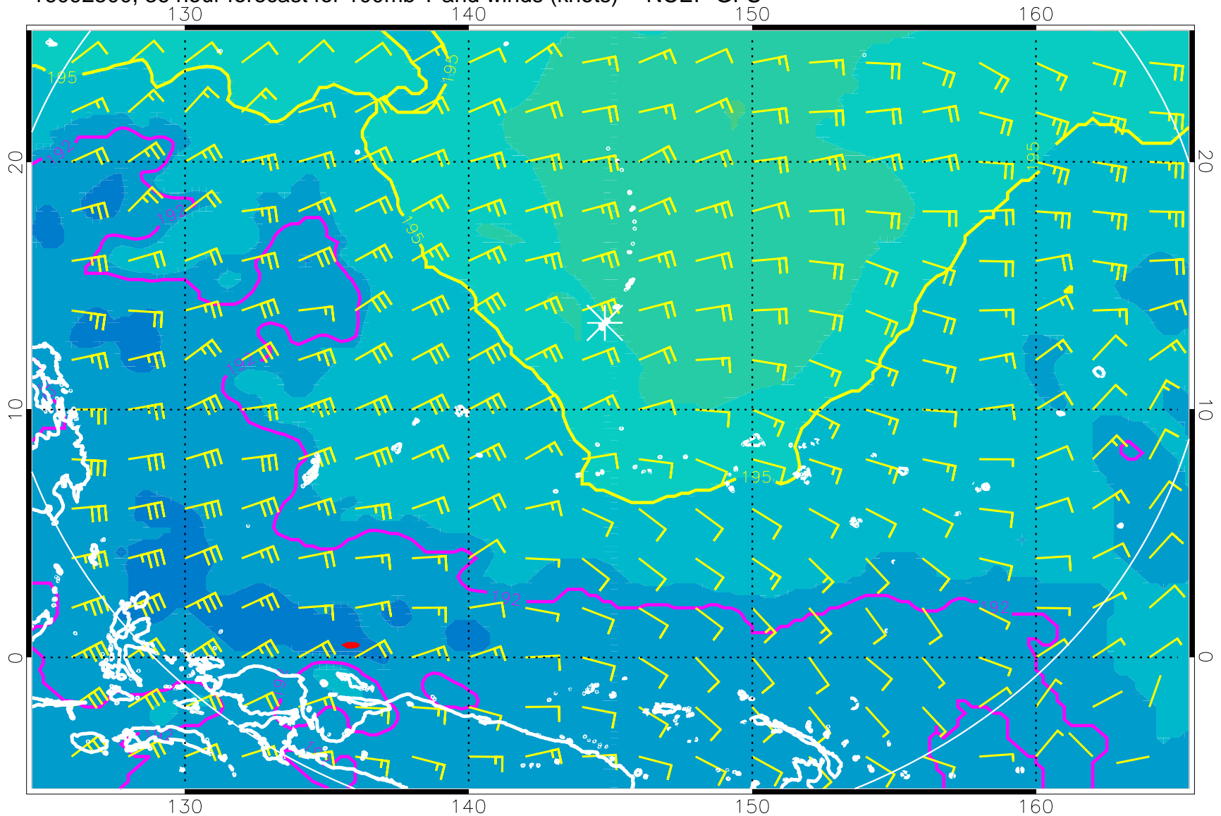
16092500, 36 hour forecast for 100mb T and winds (knots) -- NCEP GFS
