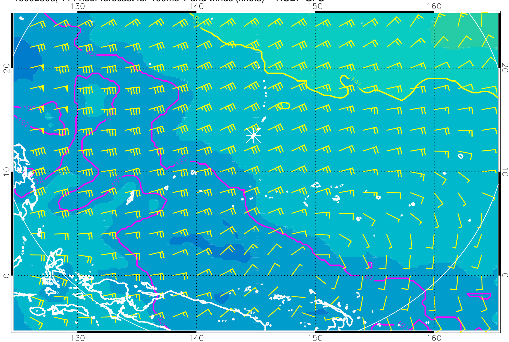
16092806, 114 hour forecast for 100mb T and winds (knots) -- NCEP GFS
