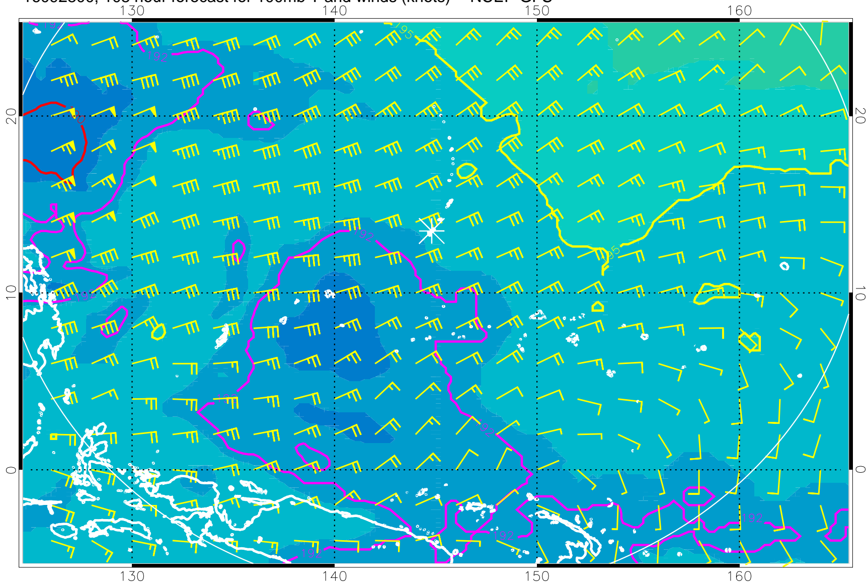
16092800, 108 hour forecast for 100mb T and winds (knots) -- NCEP GFS
