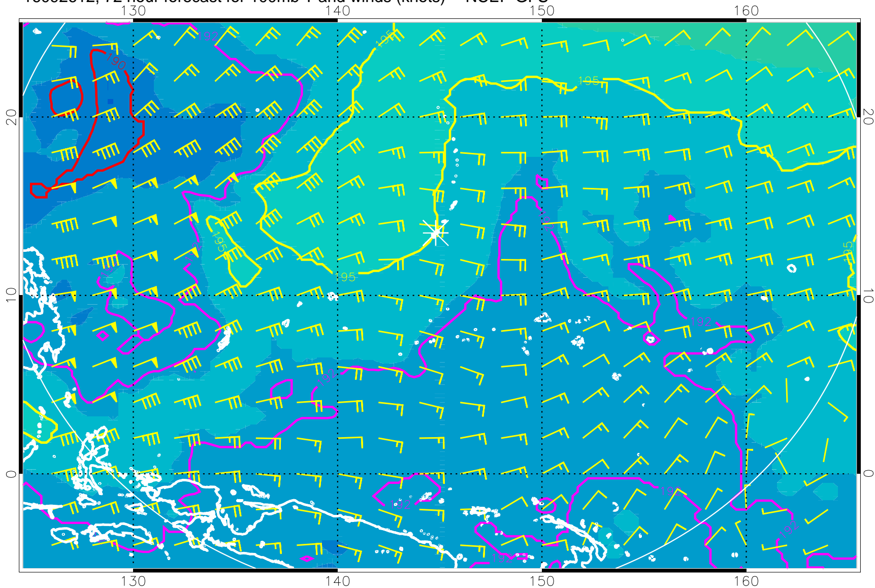
16092612, 72 hour forecast for 100mb T and winds (knots) -- NCEP GFS
