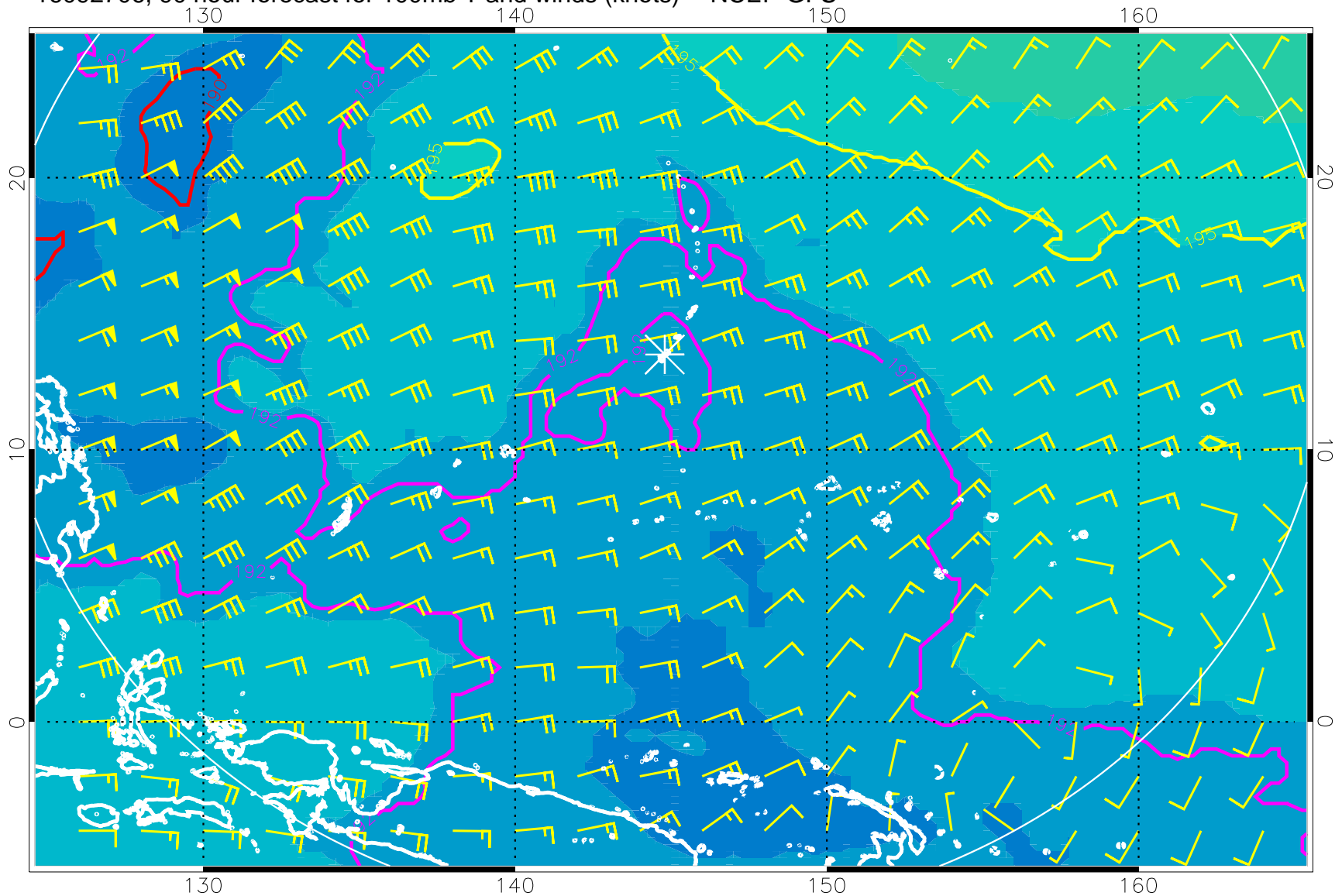
16092706, 90 hour forecast for 100mb T and winds (knots) -- NCEP GFS
