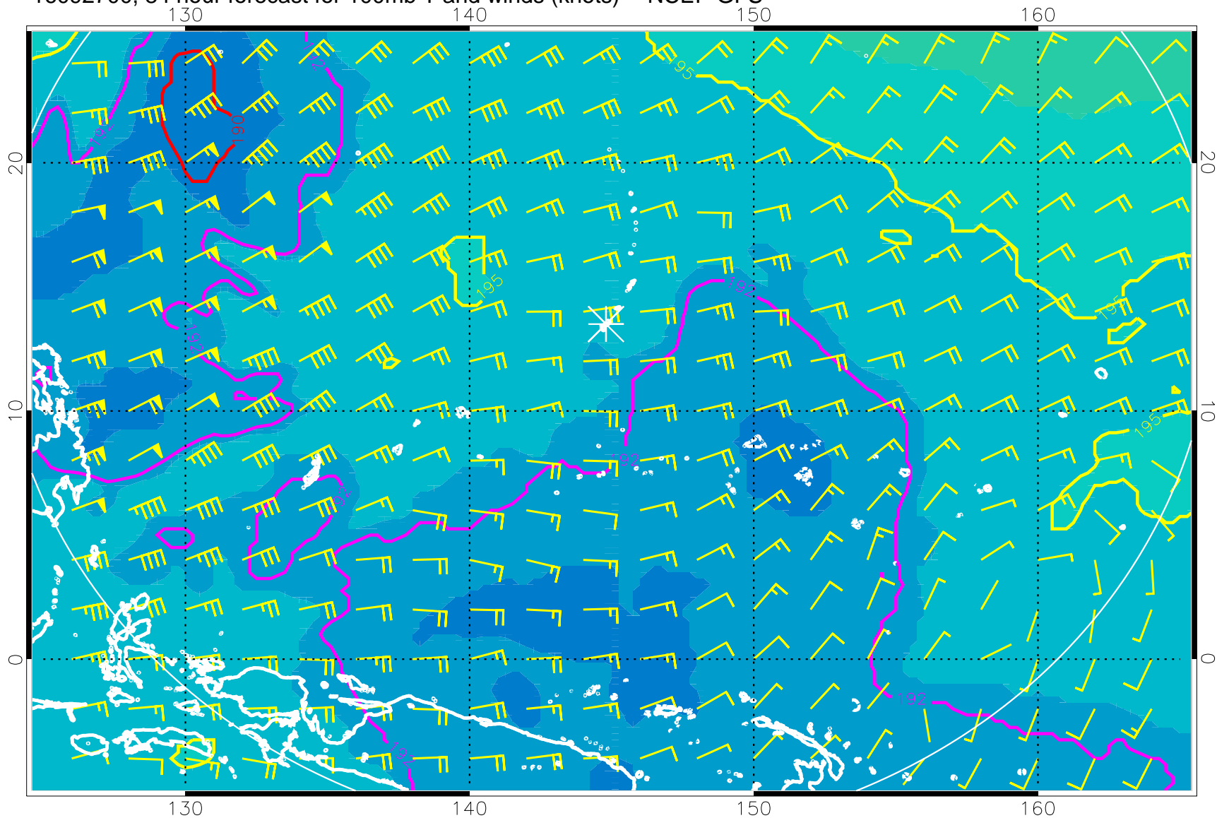
16092700, 84 hour forecast for 100mb T and winds (knots) -- NCEP GFS
