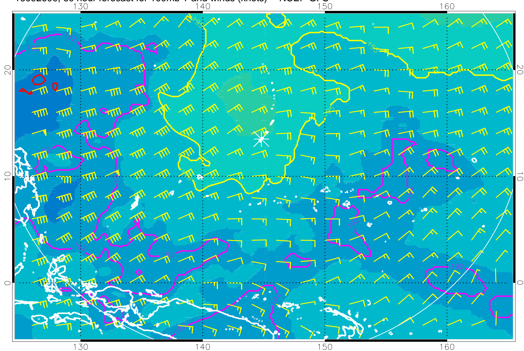
16092600, 60 hour forecast for 100mb T and winds (knots) -- NCEP GFS
