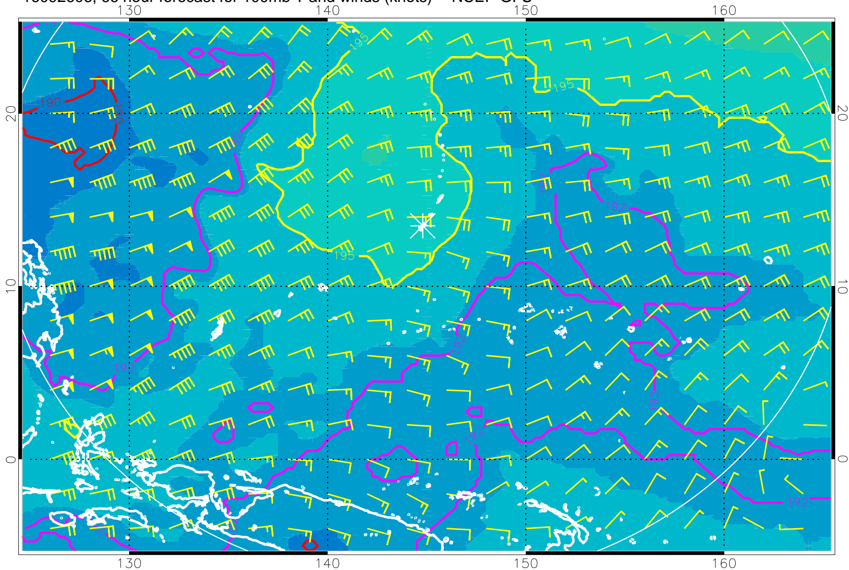
16092606, 66 hour forecast for 100mb T and winds (knots) -- NCEP GFS
