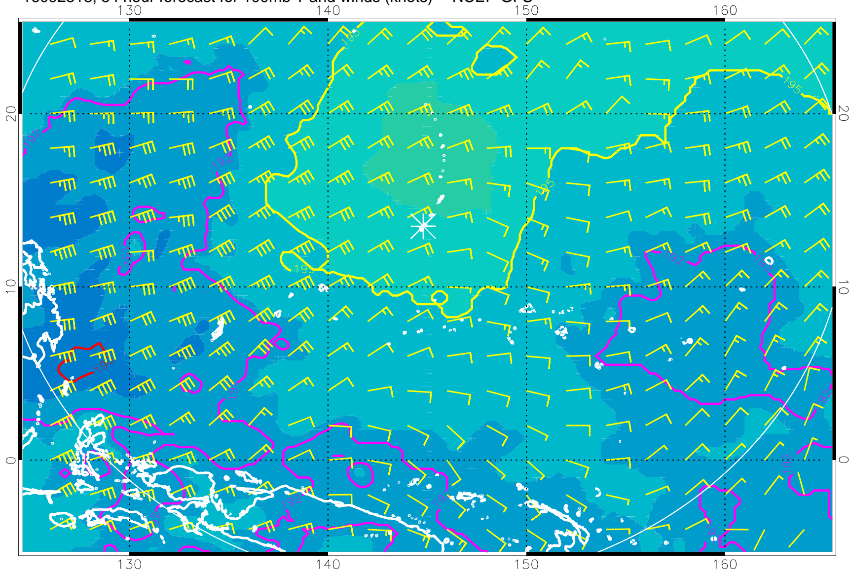
16092518, 54 hour forecast for 100mb T and winds (knots) -- NCEP GFS
