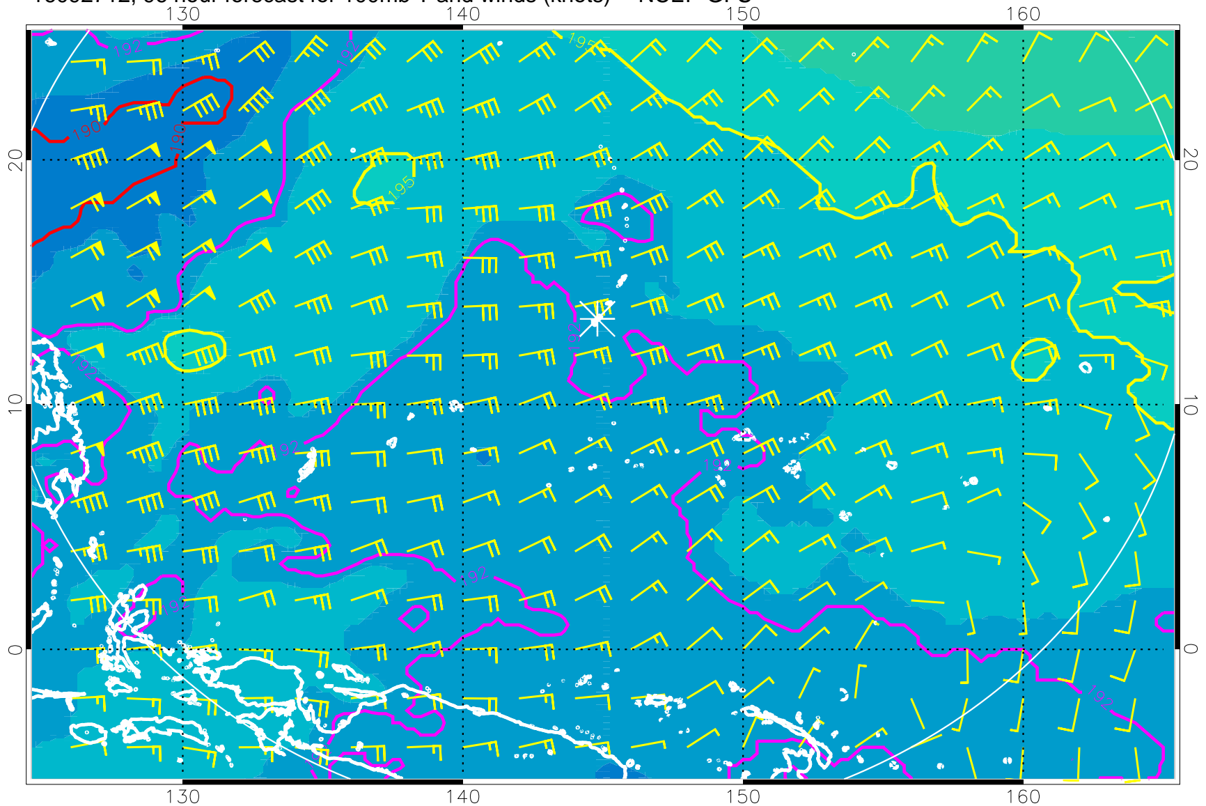
16092712, 96 hour forecast for 100mb T and winds (knots) -- NCEP GFS
