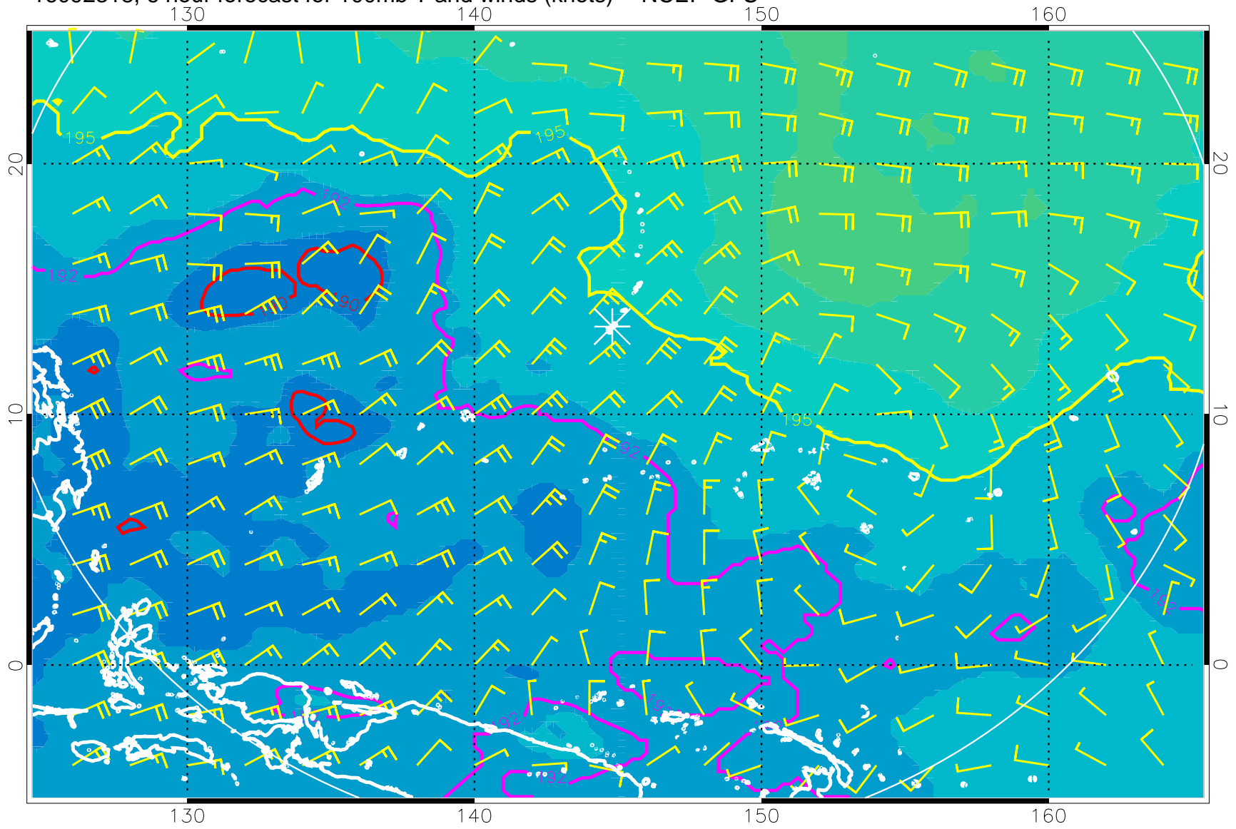
16092318, 6 hour forecast for 100mb T and winds (knots) -- NCEP GFS
