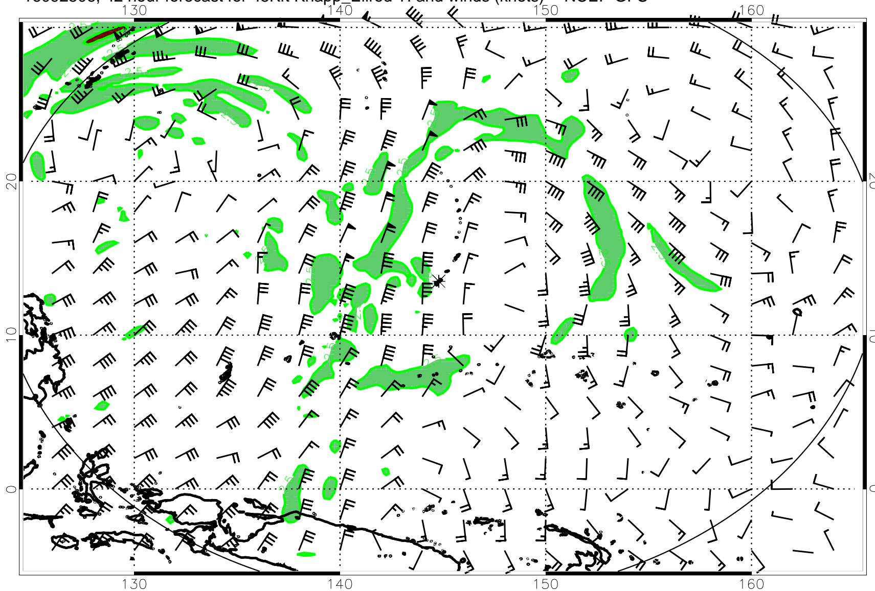
16092506, 42 hour forecast for 45Kft Knapp_Ellrod TI and winds (knots) -- NCEP GFS
