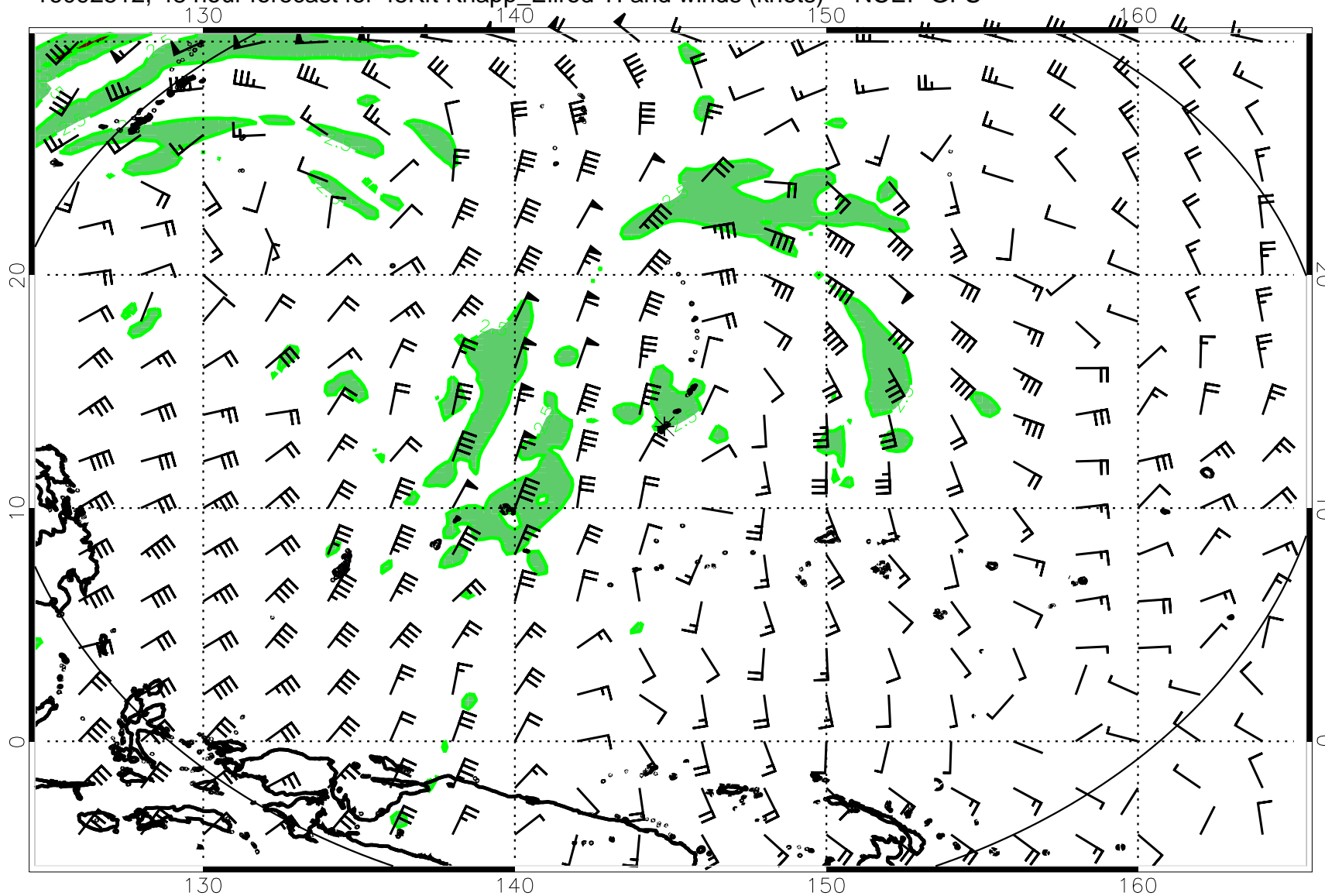
16092512, 48 hour forecast for 45Kft Knapp_Ellrod TI and winds (knots) -- NCEP GFS
