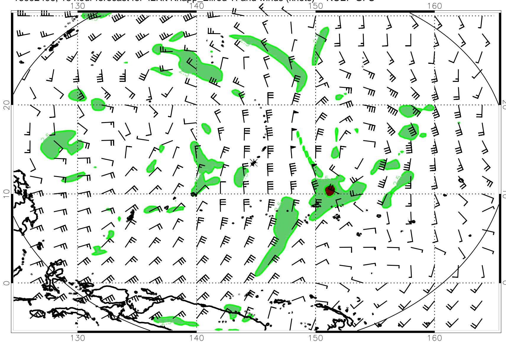
16092406, 18 hour forecast for 42Kft Knapp_Ellrod TI and winds (knots) -- NCEP GFS
