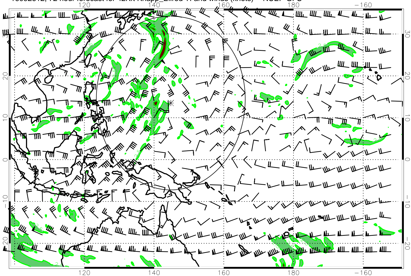
16092612, 72 hour forecast for 42Kft Knapp_Ellrod TI and winds (knots) -- NCEP GFS
