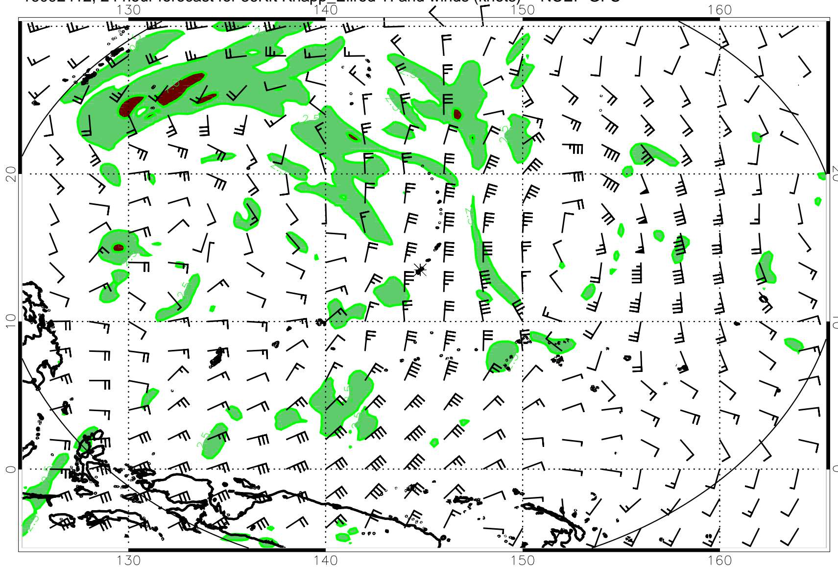
16092412, 24 hour forecast for 36Kft Knapp_Ellrod TI and winds (knots) -- NCEP GFS
