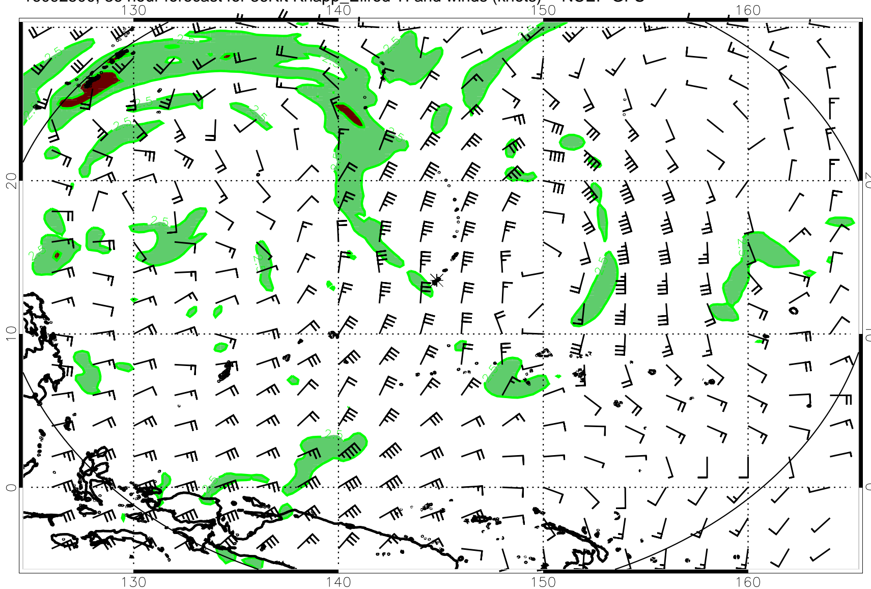
16092500, 36 hour forecast for 36Kft Knapp_Ellrod TI and winds (knots) -- NCEP GFS
