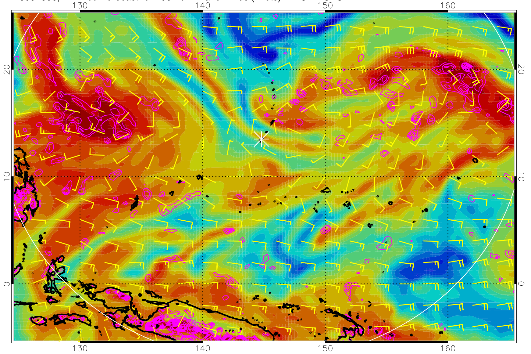
16092806, 114 hour forecast for 700mb RH and winds (knots) -- NCEP GFS
