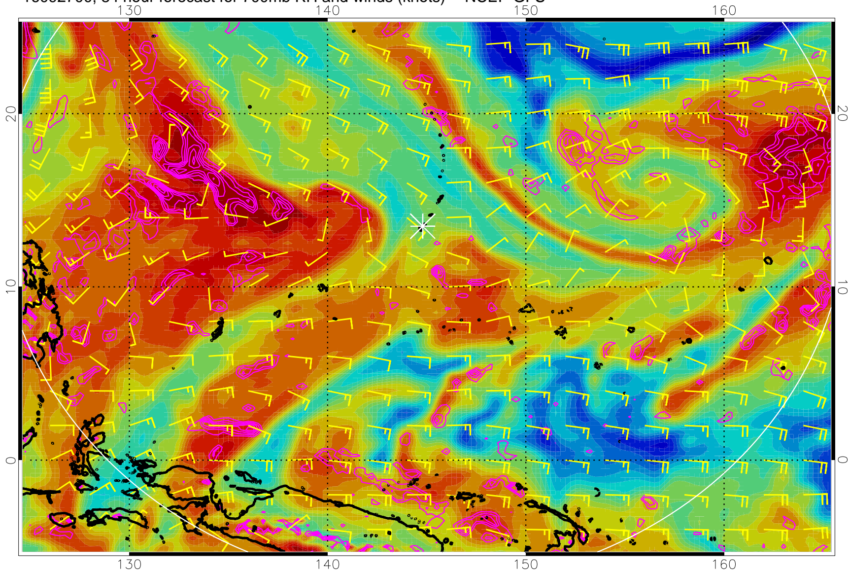
16092700, 84 hour forecast for 700mb RH and winds (knots) -- NCEP GFS
