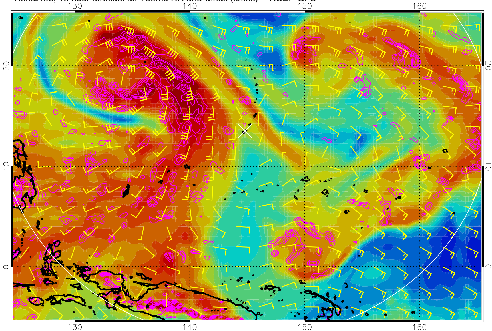
16092406, 18 hour forecast for 700mb RH and winds (knots) -- NCEP GFS
