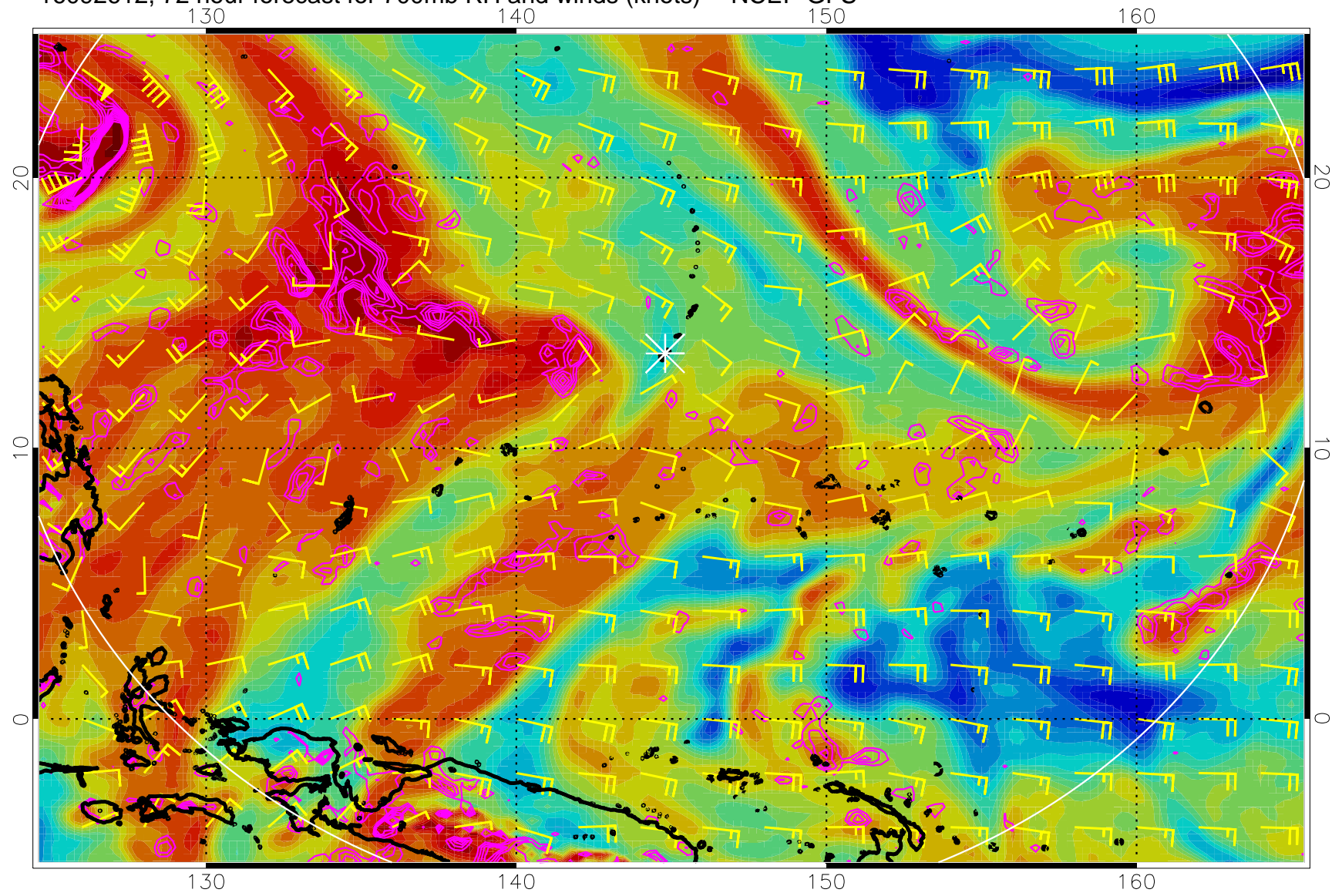
16092612, 72 hour forecast for 700mb RH and winds (knots) -- NCEP GFS
