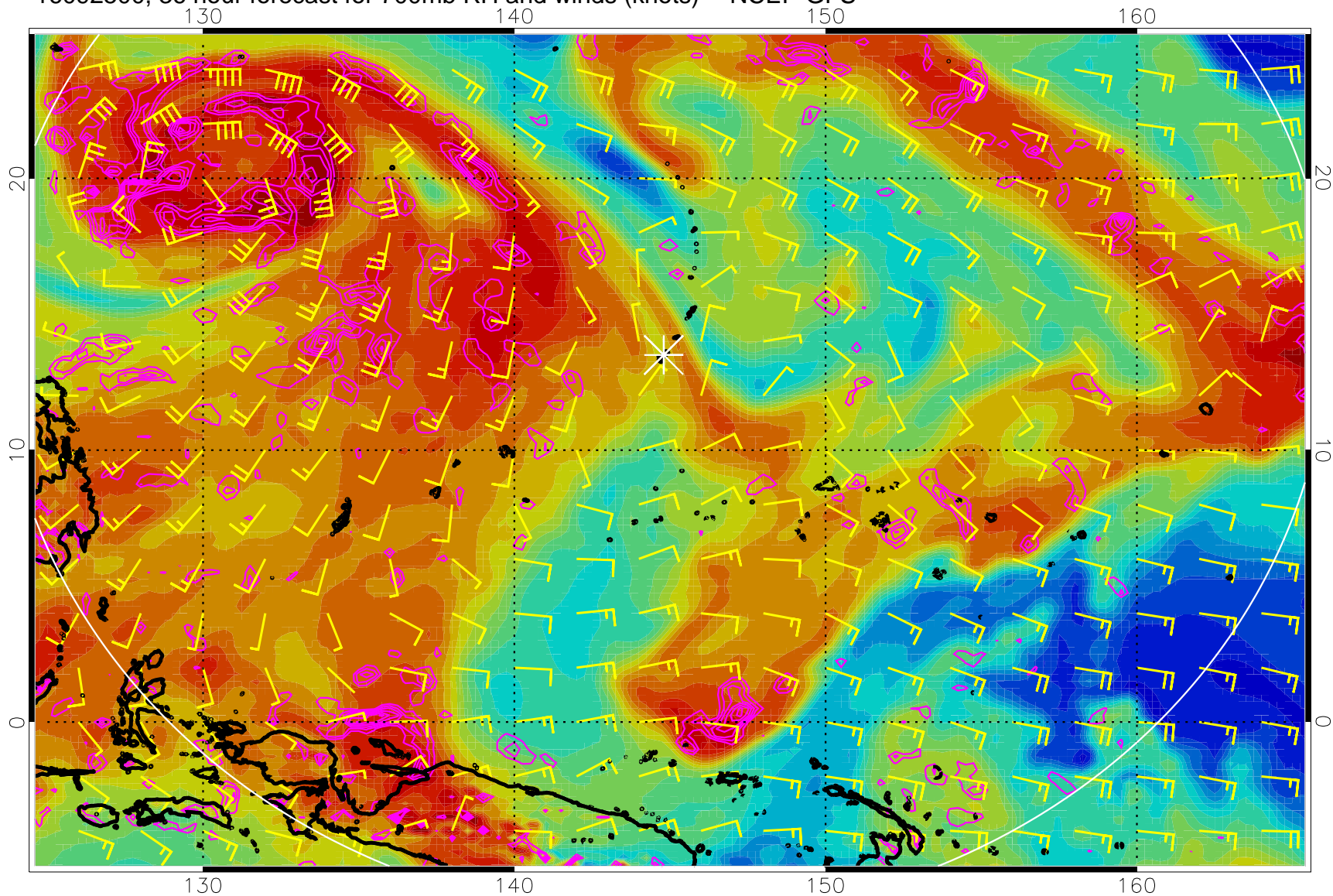
16092500, 36 hour forecast for 700mb RH and winds (knots) -- NCEP GFS
