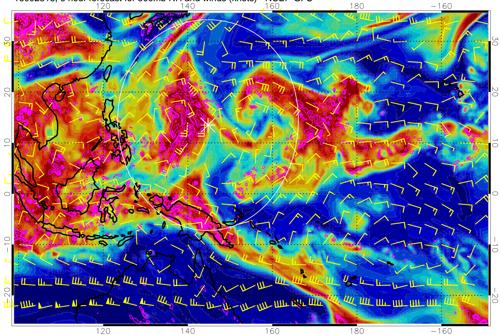
16092318, 6 hour forecast for 500mb RH and winds (knots) - NCEP GFS
