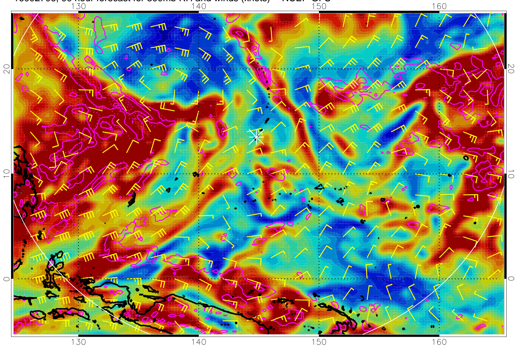
16092706, 90 hour forecast for 300mb RH and winds (knots) -- NCEP GFS
