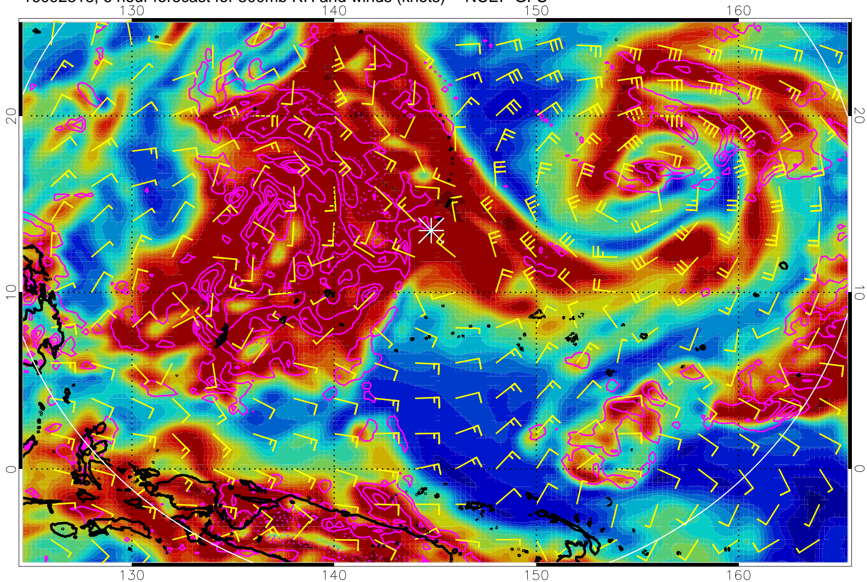
16092318, 6 hour forecast for 300mb RH and winds (knots) -- NCEP GFS
