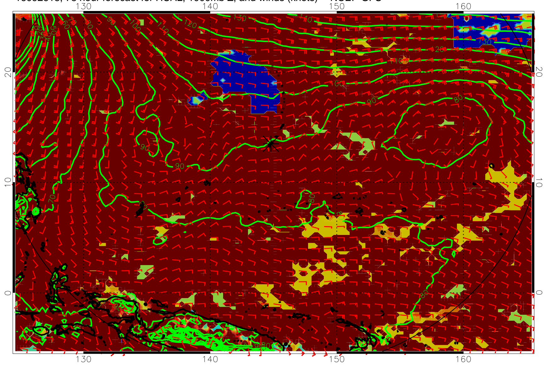
16092618, 78 hour forecast for HCAL, 1000mb Z, and winds (knots) -- NCEP GFS
