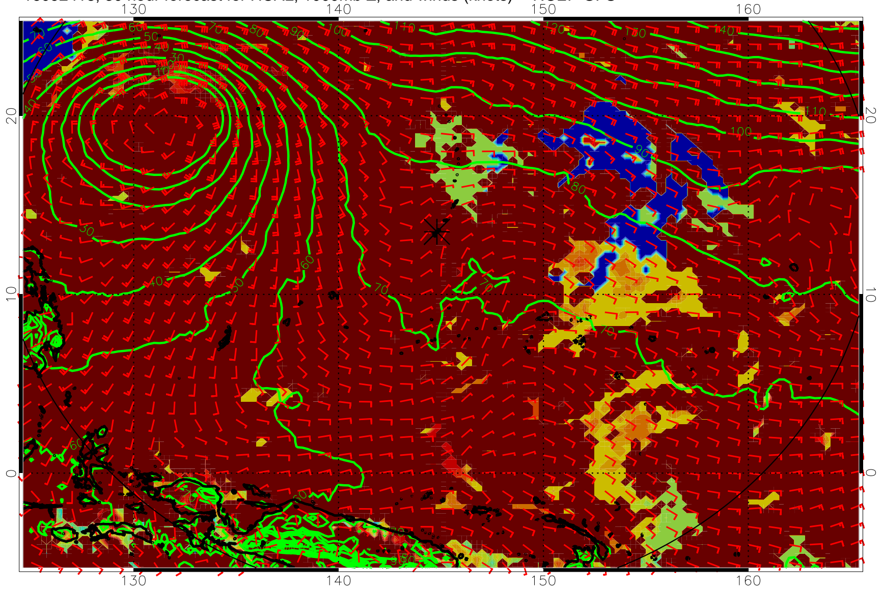
16092418, 30 hour forecast for HCAL, 1000mb Z, and winds (knots) -- NCEP GFS
