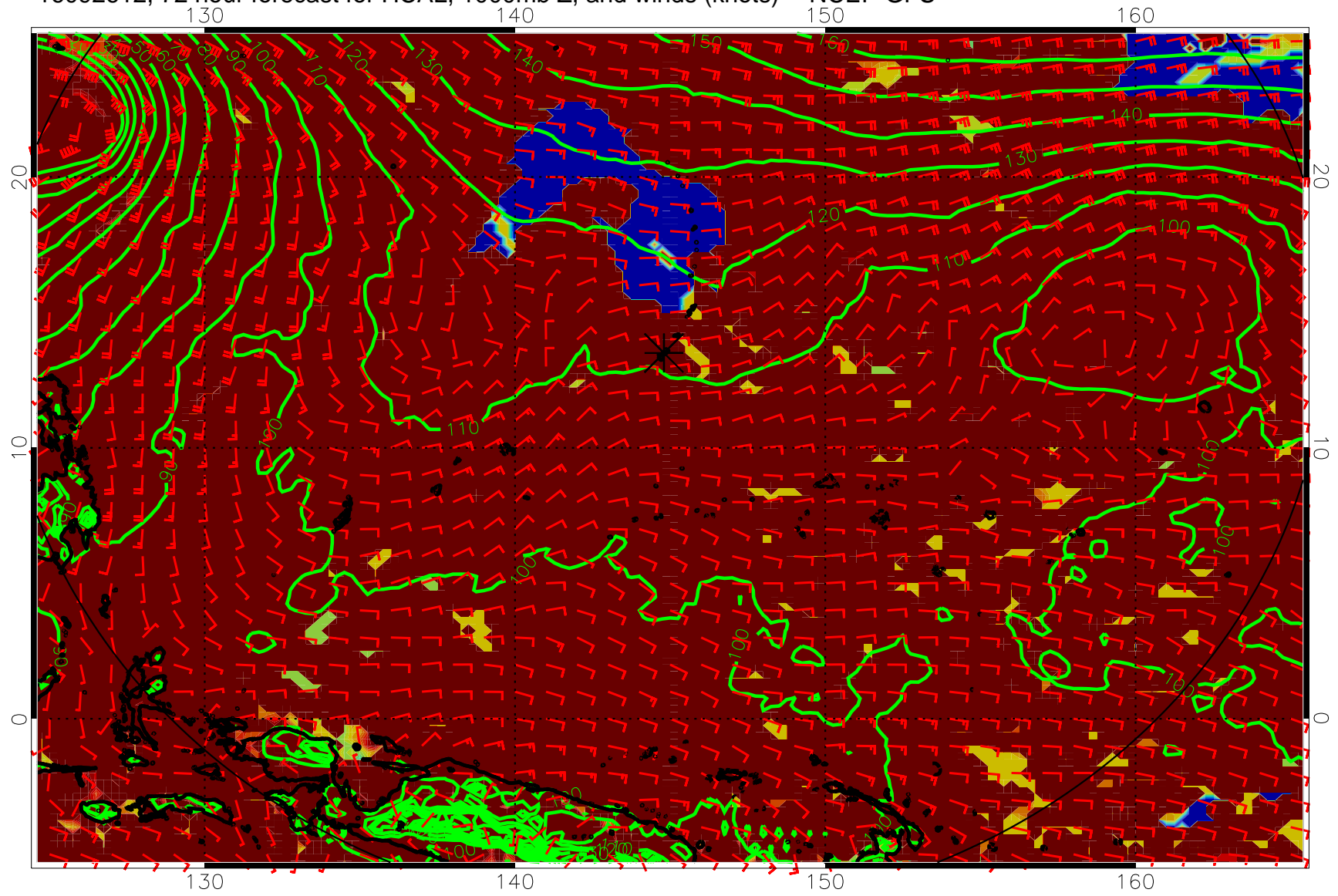
16092612, 72 hour forecast for HCAL, 1000mb Z, and winds (knots) -- NCEP GFS
