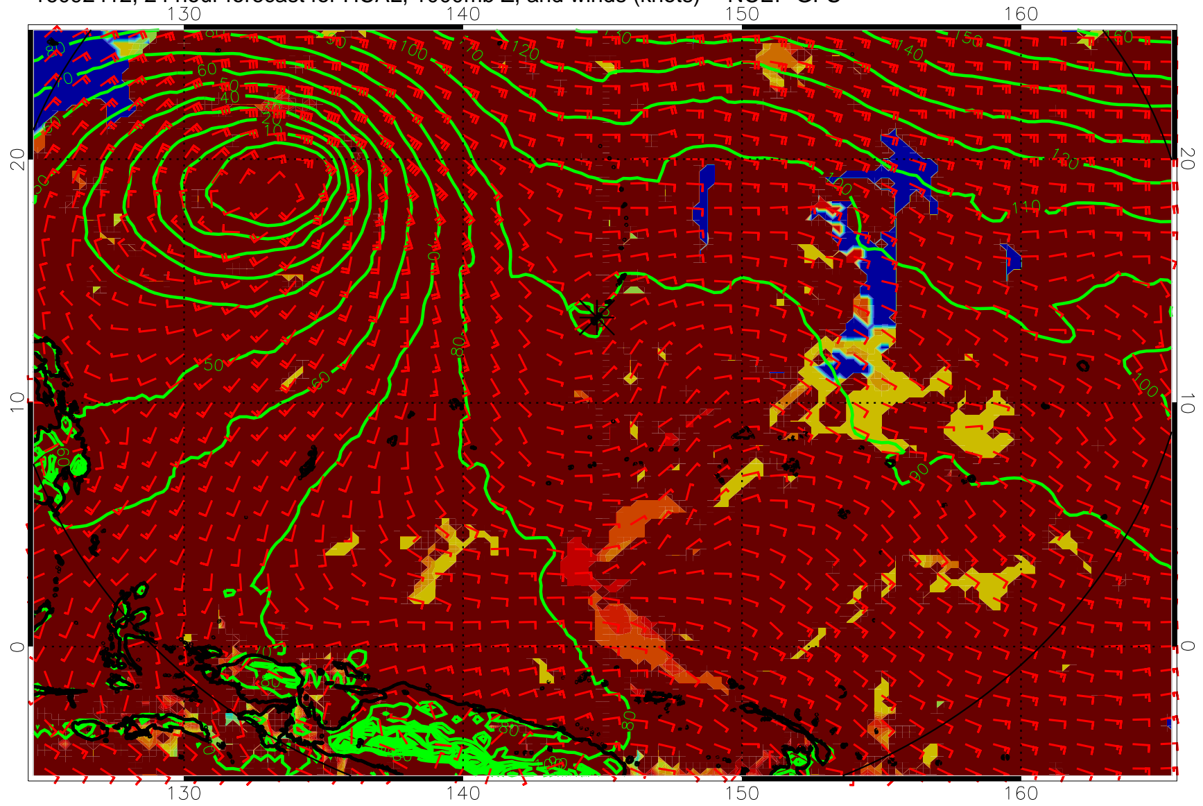
16092412, 24 hour forecast for HCAL, 1000mb Z, and winds (knots) -- NCEP GFS
