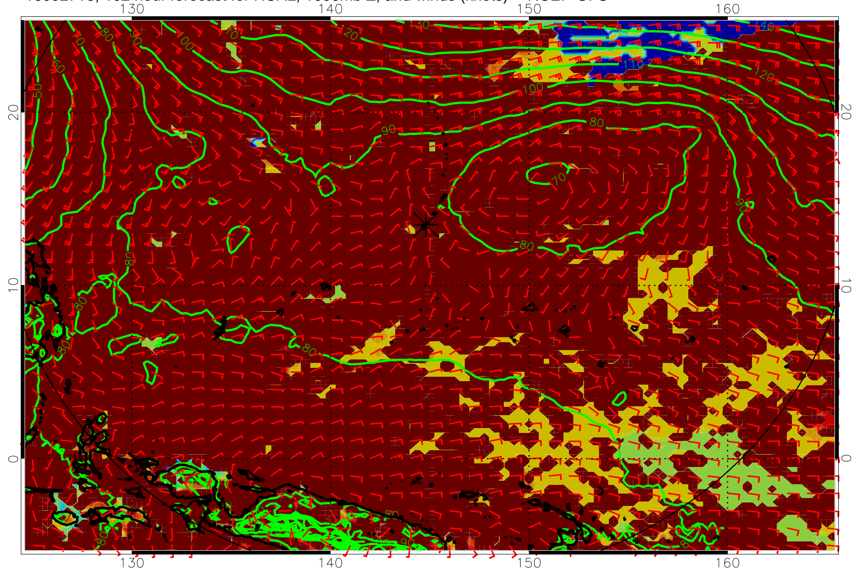
16092718, 102 hour forecast for HCAL, 1000mb Z, and winds (knots) -- NCEP GFS
