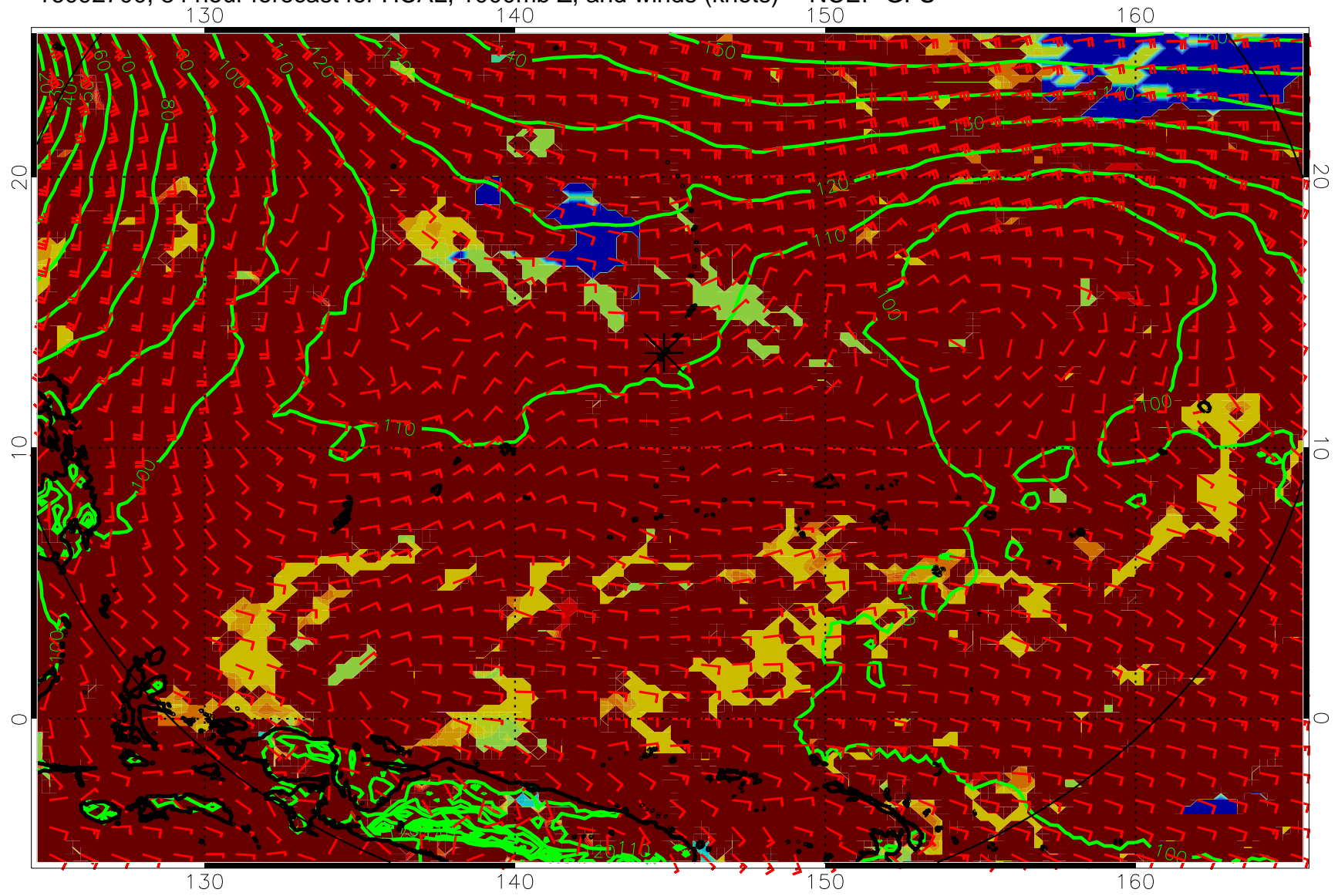
16092700, 84 hour forecast for HCAL, 1000mb Z, and winds (knots) -- NCEP GFS
