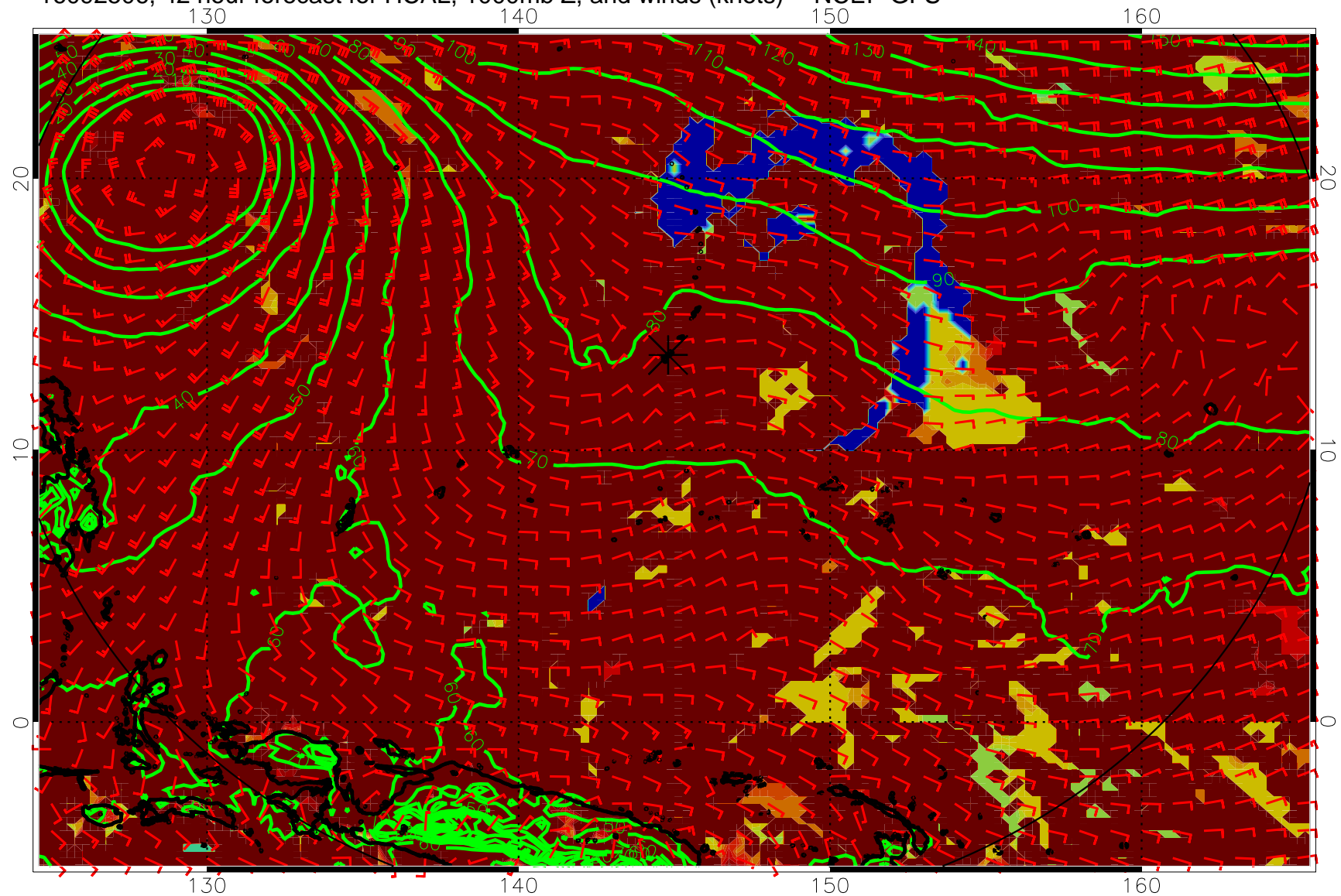
16092506, 42 hour forecast for HCAL, 1000mb Z, and winds (knots) -- NCEP GFS
