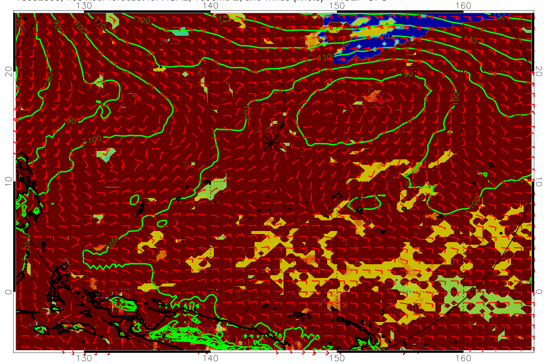
16092800, 108 hour forecast for HCAL, 1000mb Z, and winds (knots) -- NCEP GFS
