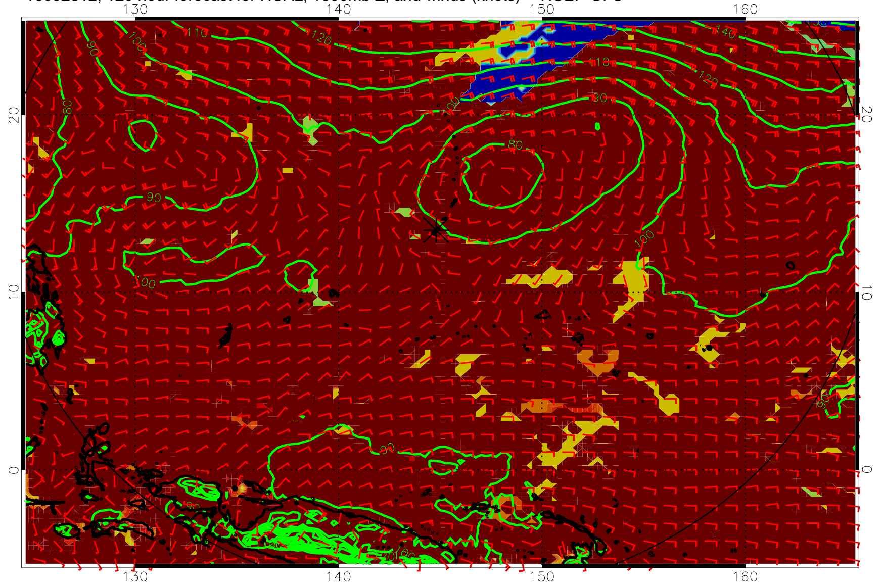
16092812, 120 hour forecast for HCAL, 1000mb Z, and winds (knots) -- NCEP GFS
