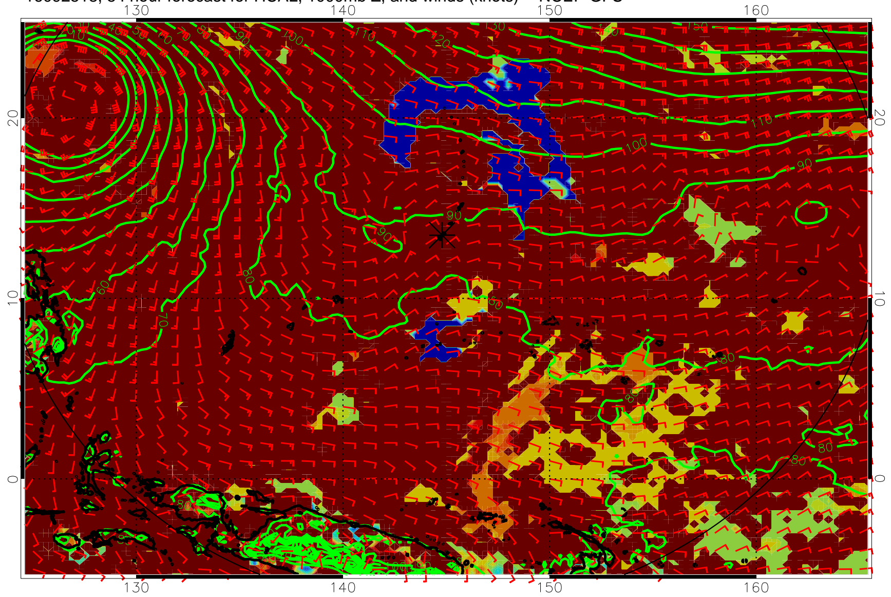
16092518, 54 hour forecast for HCAL, 1000mb Z, and winds (knots) -- NCEP GFS
