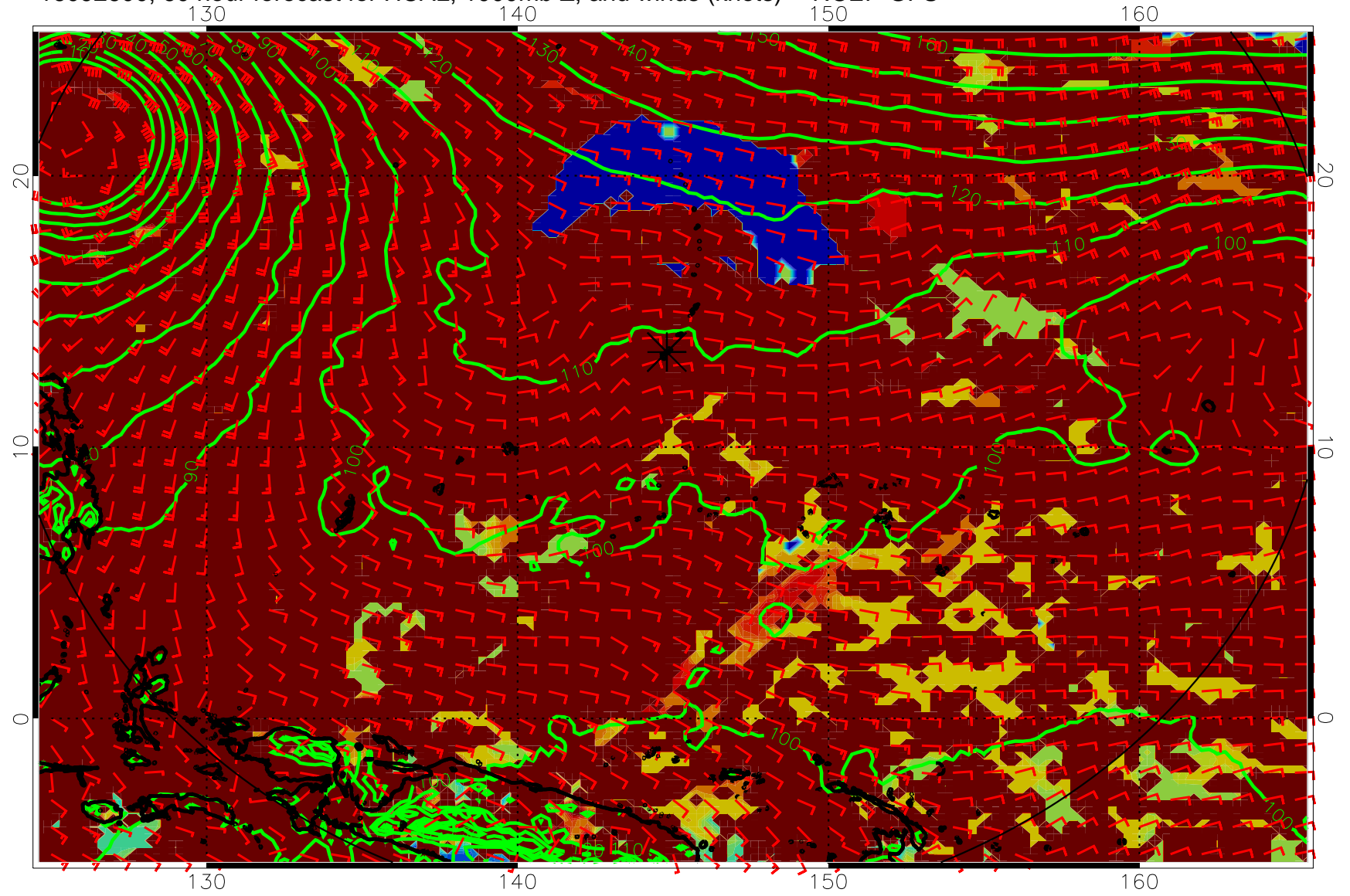
16092600, 60 hour forecast for HCAL, 1000mb Z, and winds (knots) -- NCEP GFS
