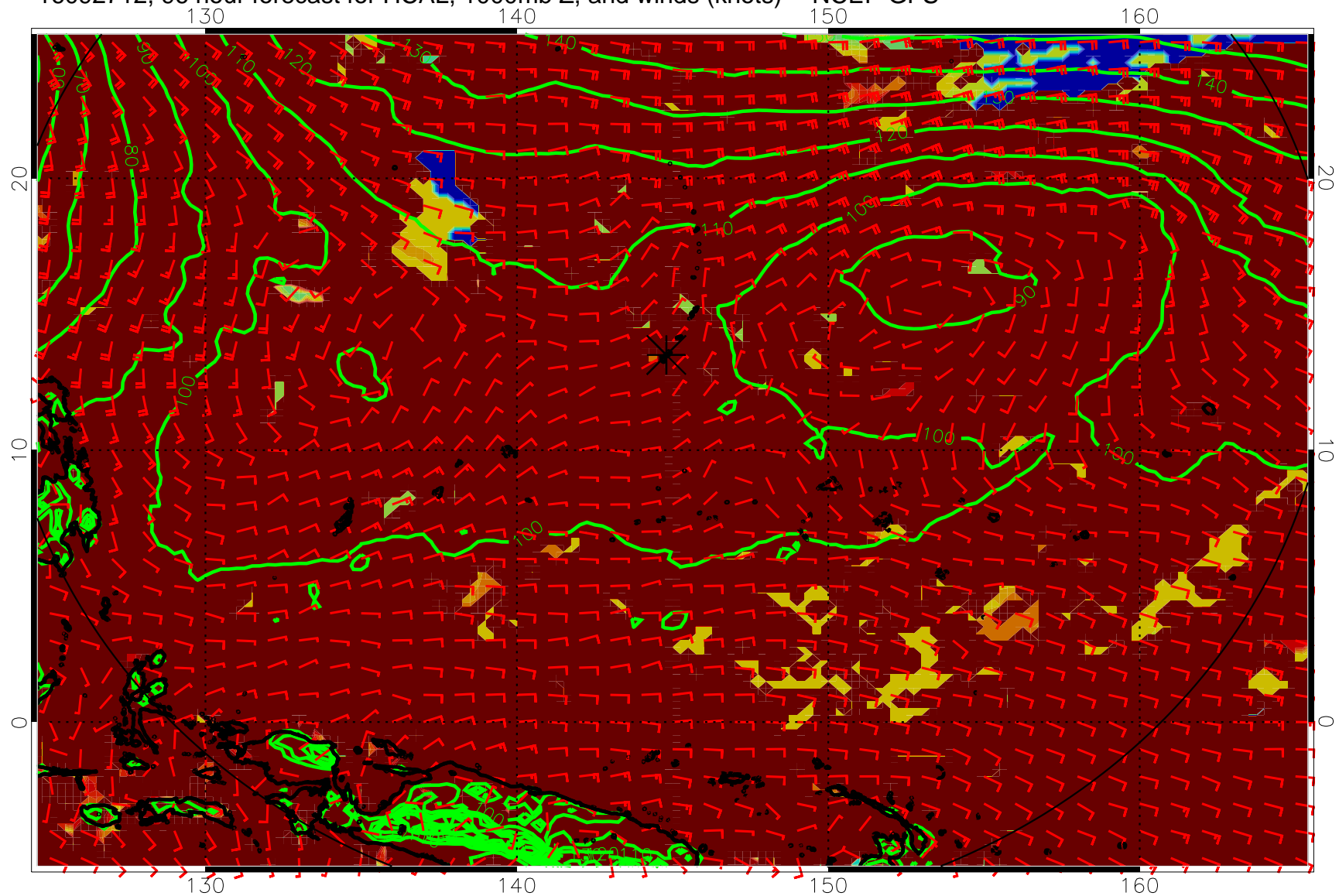
16092712, 96 hour forecast for HCAL, 1000mb Z, and winds (knots) -- NCEP GFS
