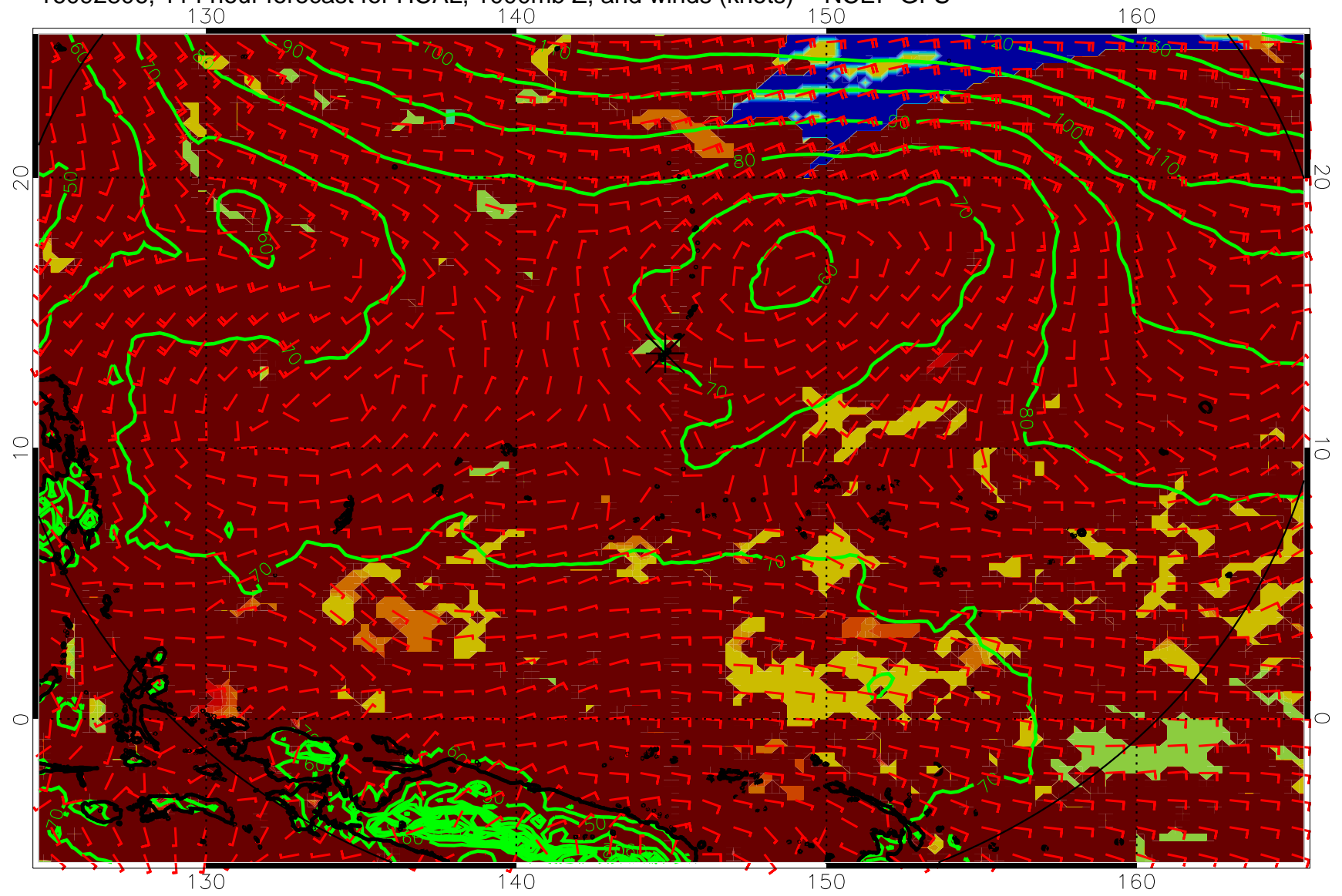
16092806, 114 hour forecast for HCAL, 1000mb Z, and winds (knots) -- NCEP GFS
