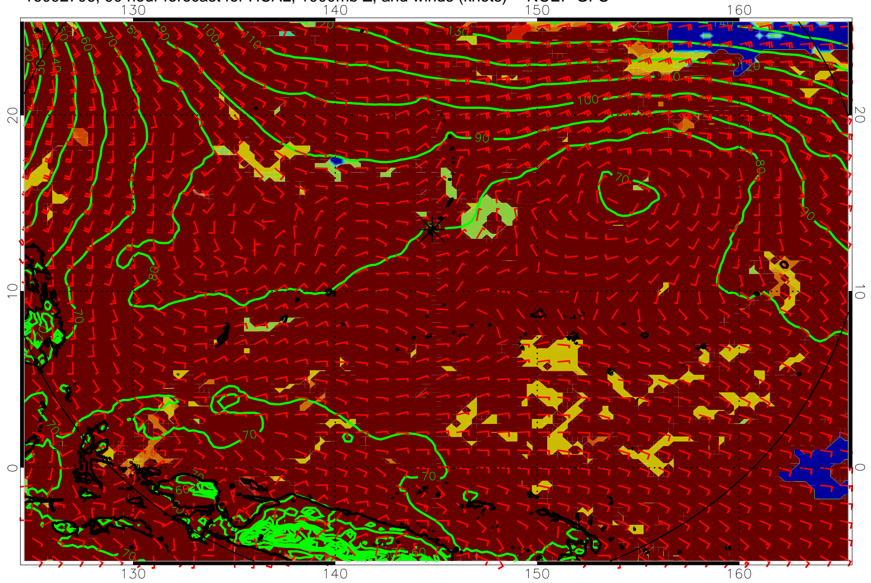
16092706, 90 hour forecast for HCAL, 1000mb Z, and winds (knots) -- NCEP GFS
