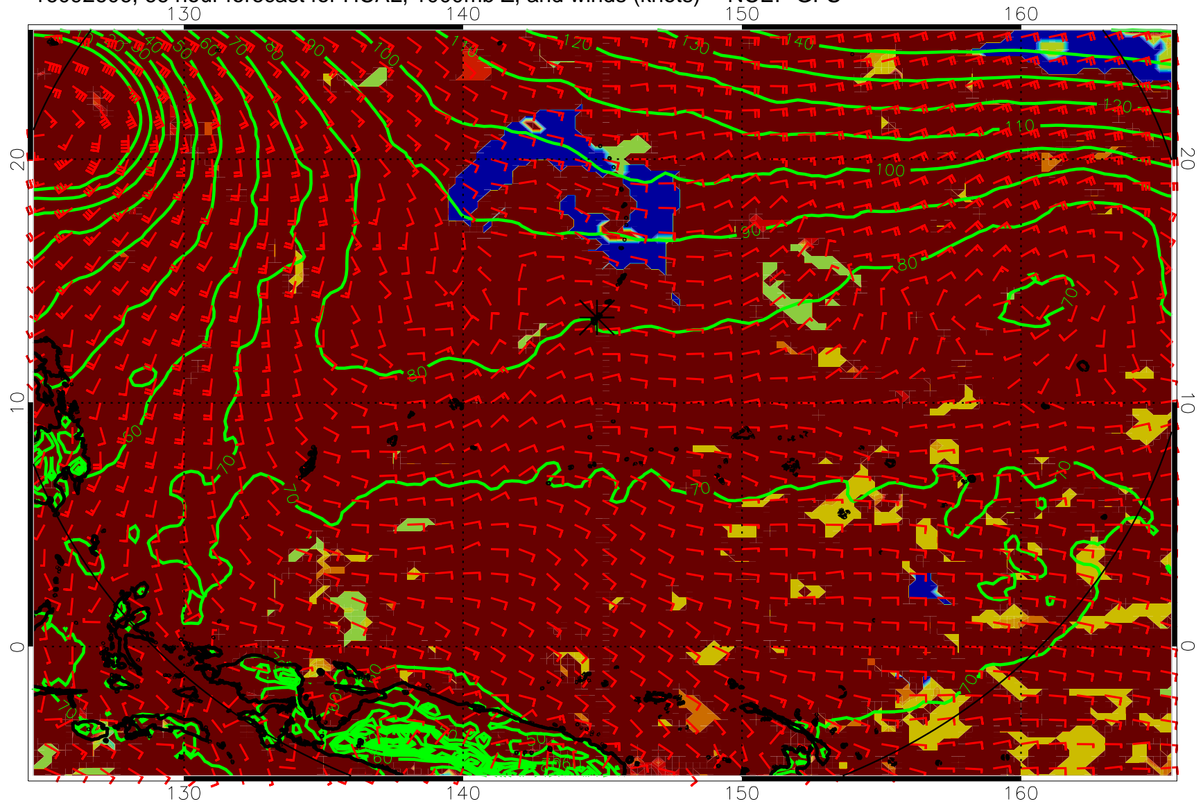
16092606, 66 hour forecast for HCAL, 1000mb Z, and winds (knots) -- NCEP GFS
