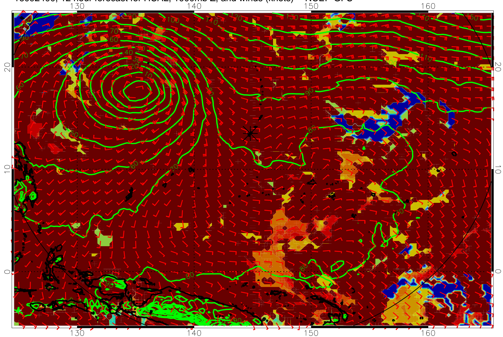
16092400, 12 hour forecast for HCAL, 1000mb Z, and winds (knots) -- NCEP GFS
