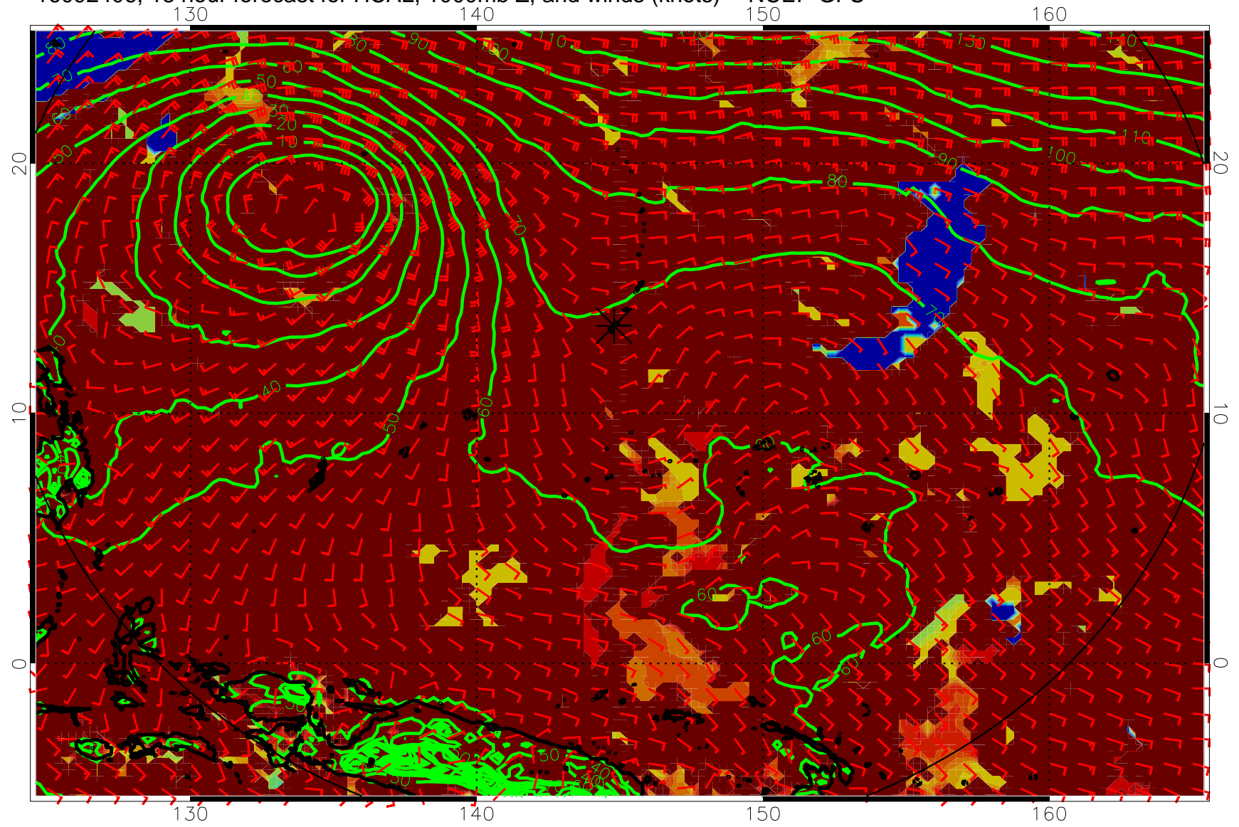
16092406, 18 hour forecast for HCAL, 1000mb Z, and winds (knots) -- NCEP GFS
