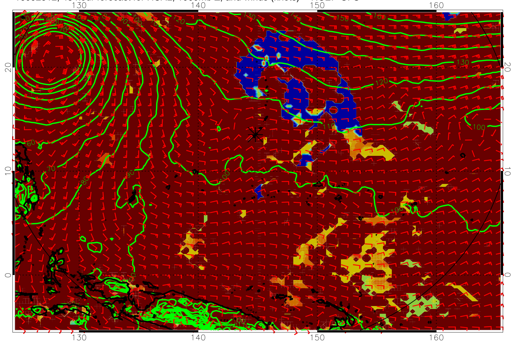
16092512, 48 hour forecast for HCAL, 1000mb Z, and winds (knots) -- NCEP GFS
