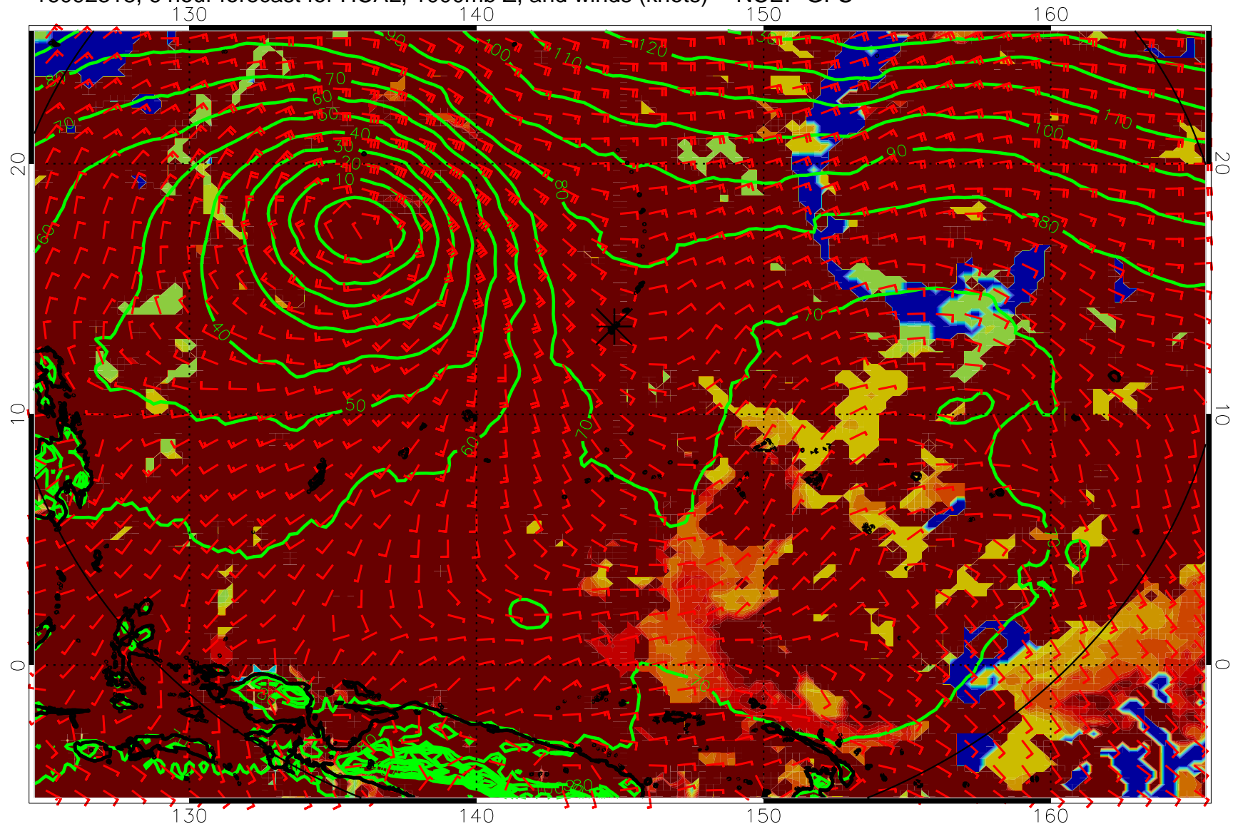
16092318, 6 hour forecast for HCAL, 1000mb Z, and winds (knots) -- NCEP GFS
