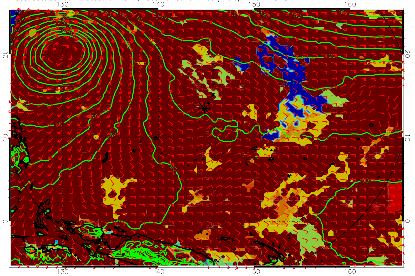
16092500, 36 hour forecast for HCAL, 1000mb Z, and winds (knots) -- NCEP GFS
