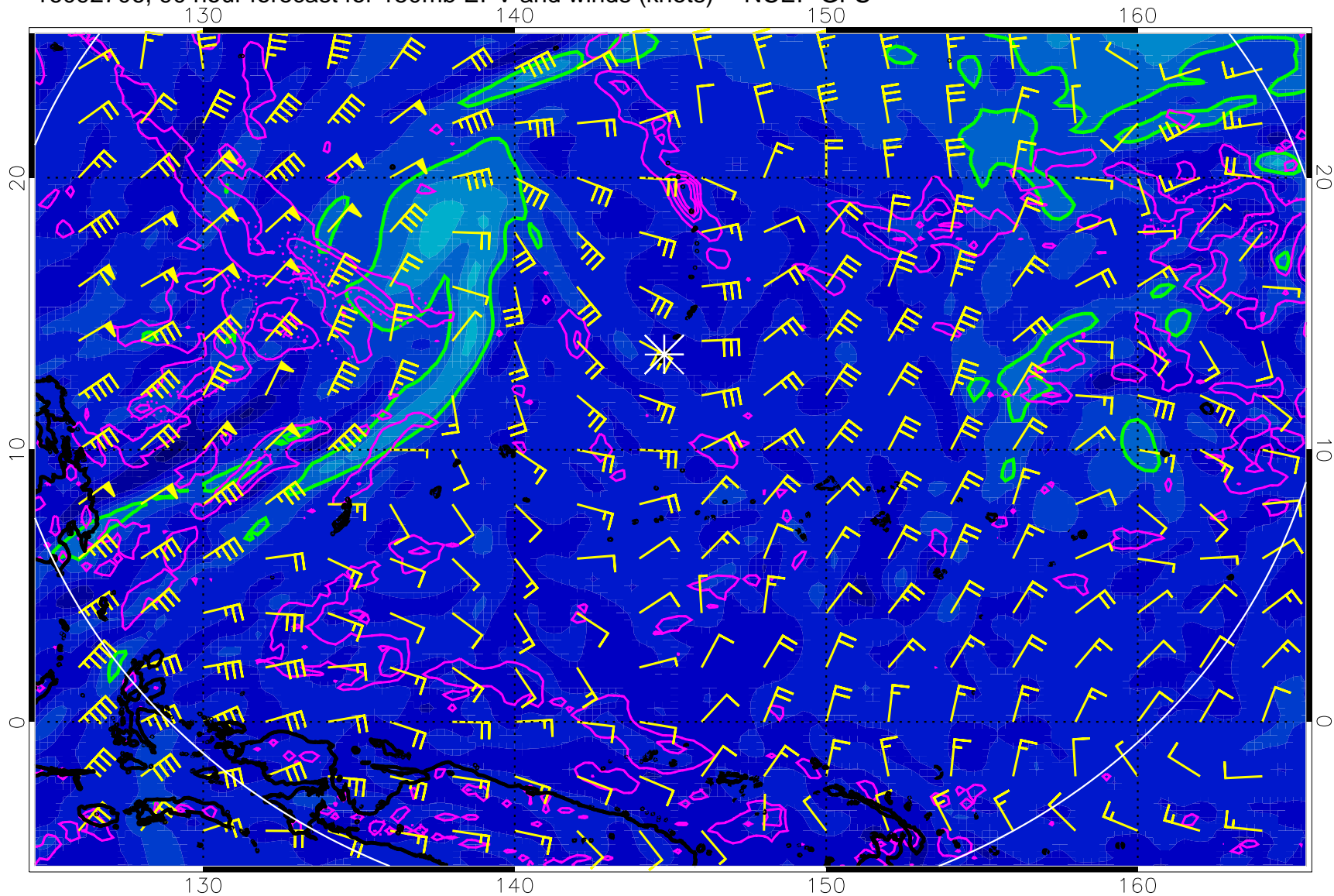
16092706, 90 hour forecast for 150mb EPV and winds (knots) -- NCEP GFS
