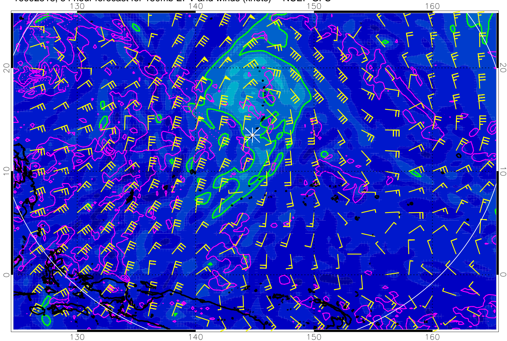
16092518, 54 hour forecast for 150mb EPV and winds (knots) -- NCEP GFS
