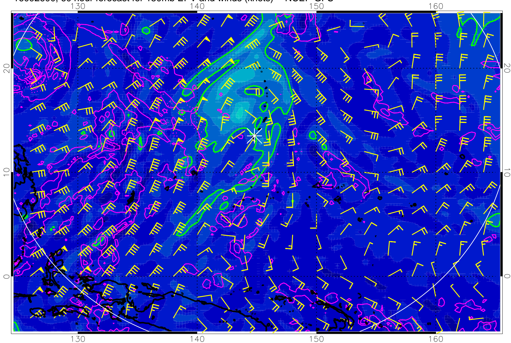
16092600, 60 hour forecast for 150mb EPV and winds (knots) -- NCEP GFS
