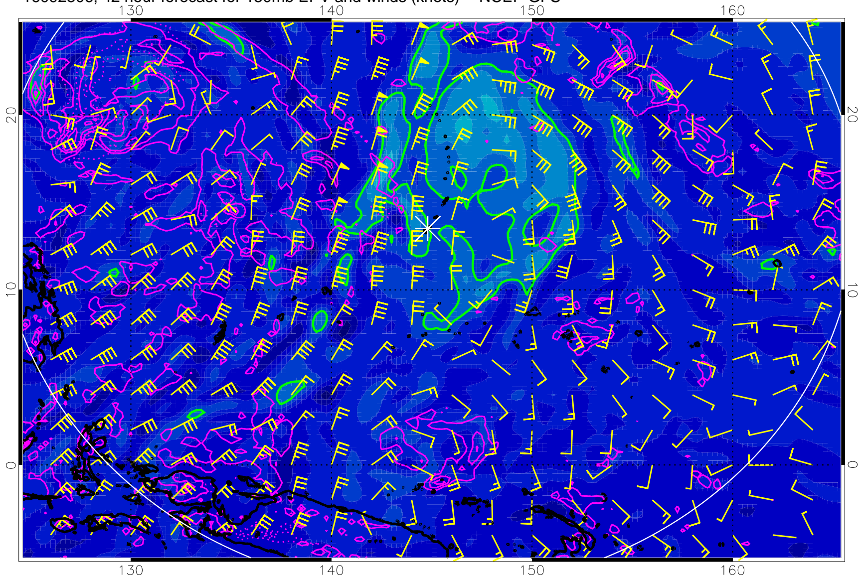
16092506, 42 hour forecast for 150mb EPV and winds (knots) -- NCEP GFS
