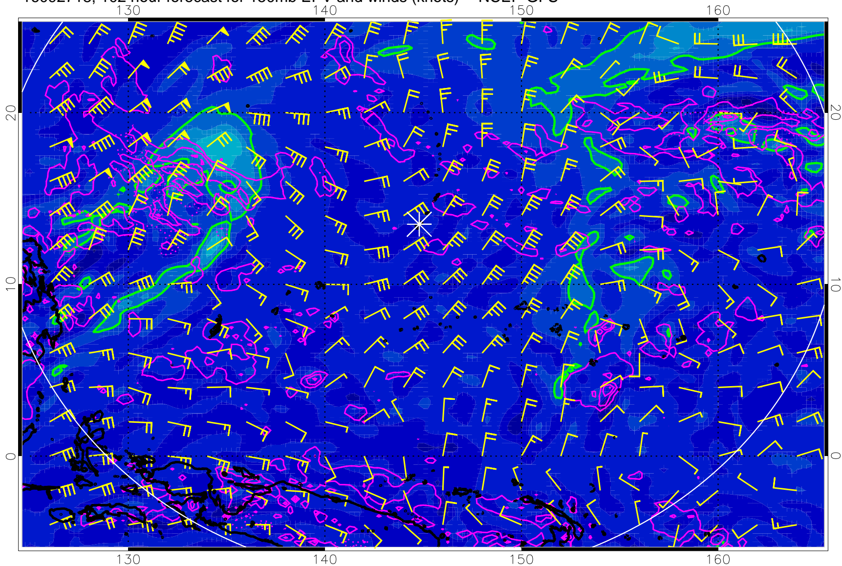
16092718, 102 hour forecast for 150mb EPV and winds (knots) -- NCEP GFS
