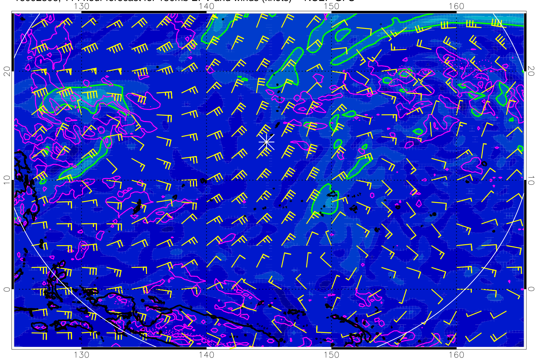
16092806, 114 hour forecast for 150mb EPV and winds (knots) -- NCEP GFS
