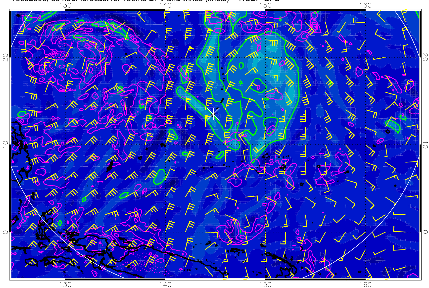
16092500, 36 hour forecast for 150mb EPV and winds (knots) -- NCEP GFS
