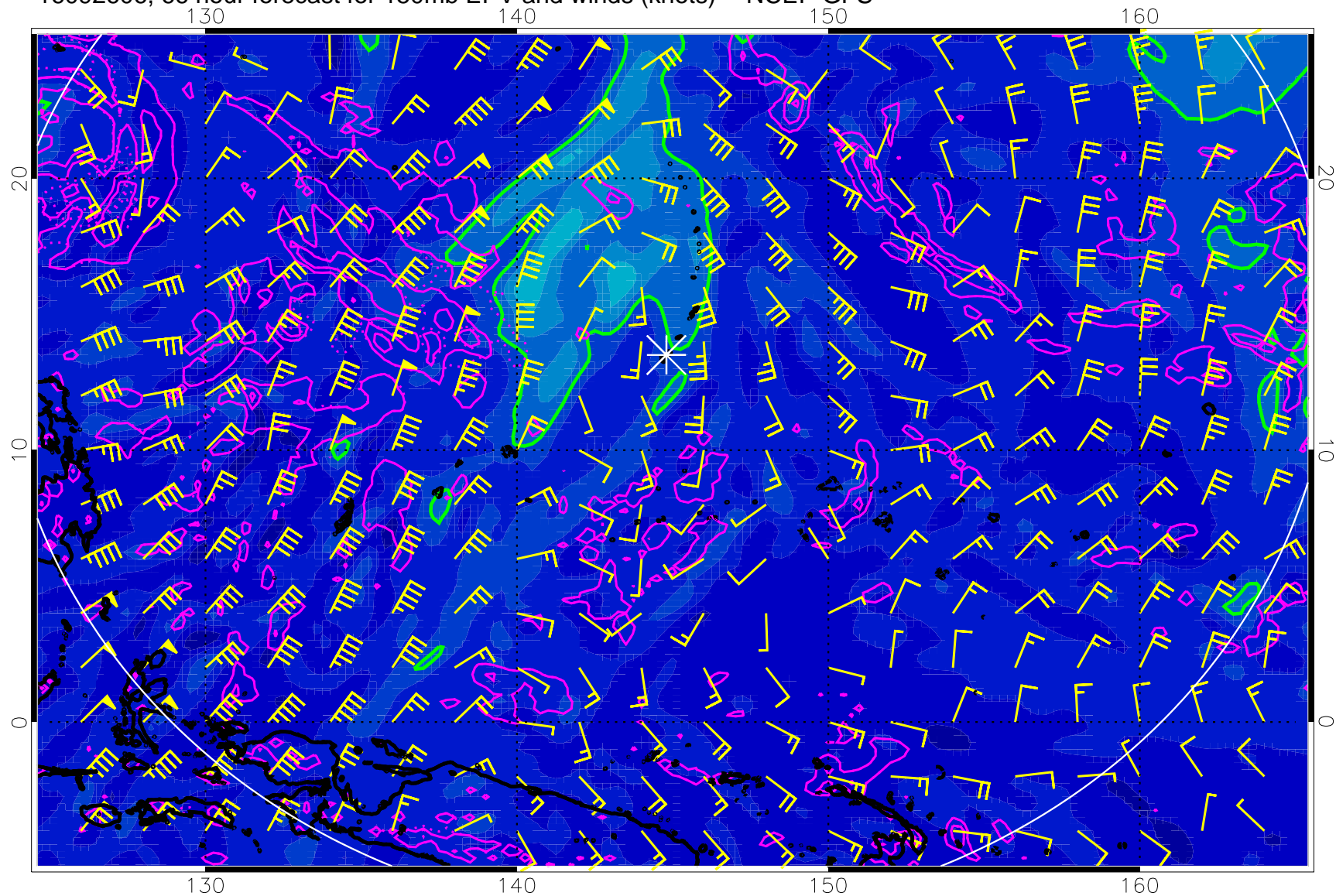
16092606, 66 hour forecast for 150mb EPV and winds (knots) -- NCEP GFS
