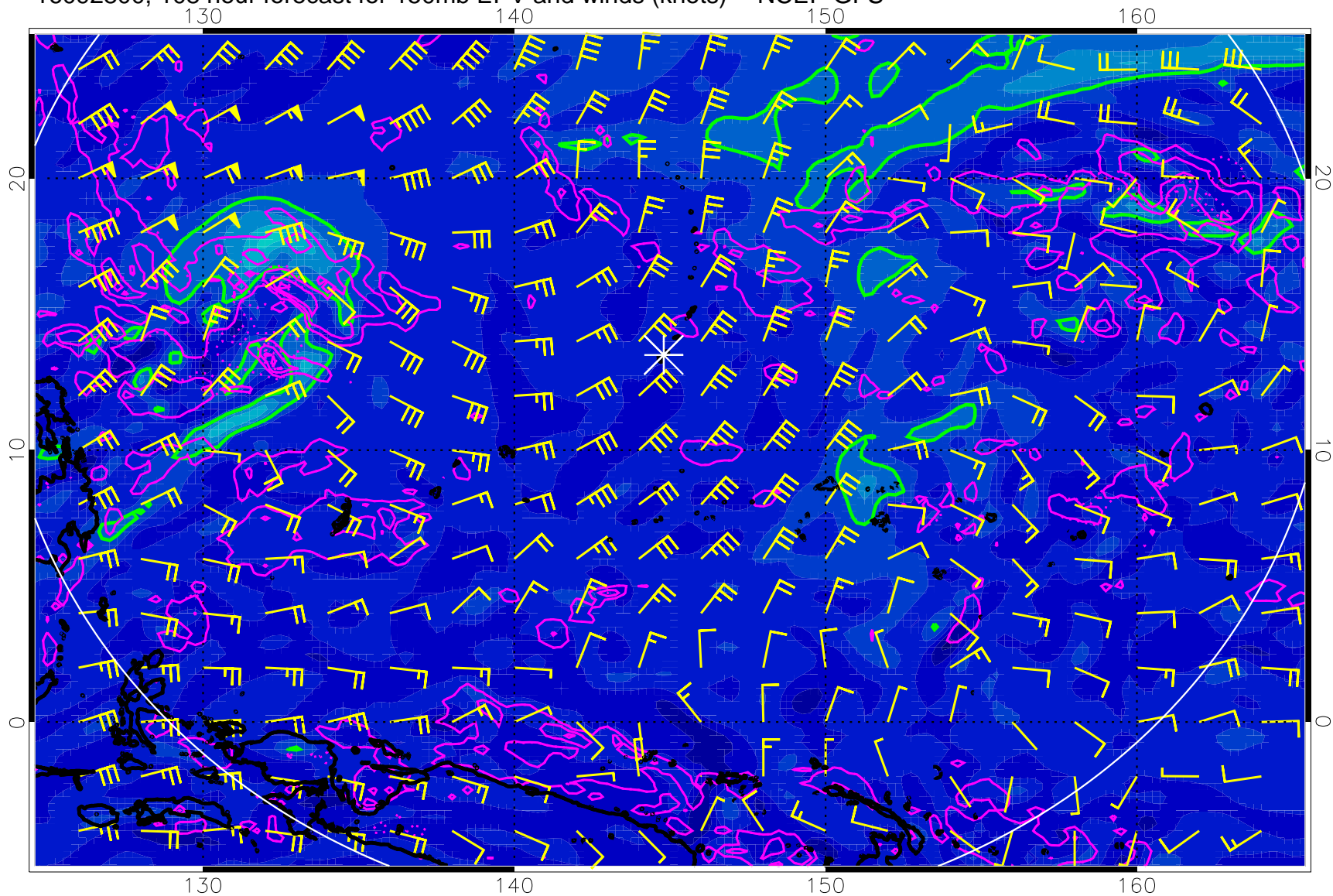
16092800, 108 hour forecast for 150mb EPV and winds (knots) -- NCEP GFS
