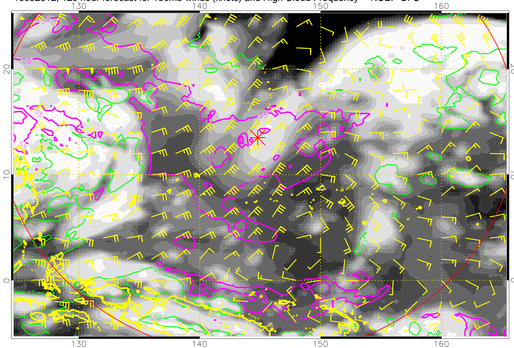
16092812, 120 hour forecast for 150mb winds (knots) and High Cloud Frequency -- NCEP GFS
