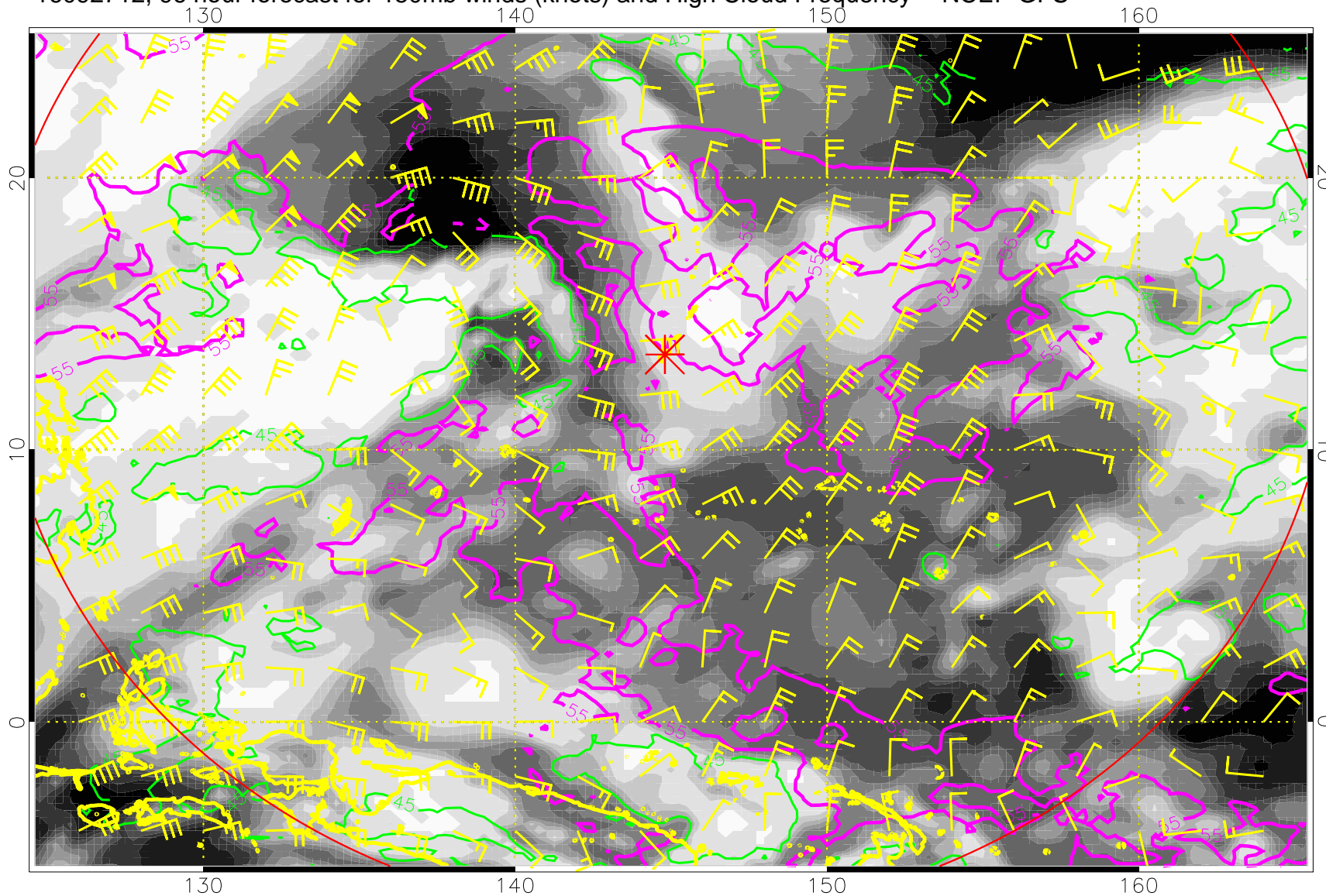
16092712, 96 hour forecast for 150mb winds (knots) and High Cloud Frequency -- NCEP GFS
