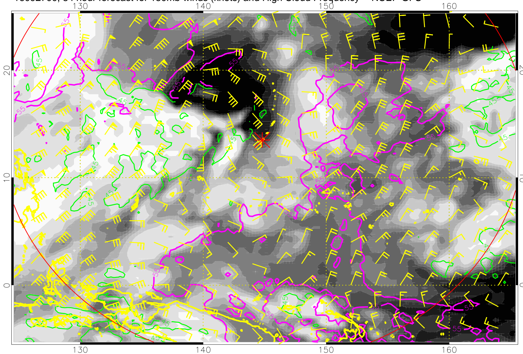
16092700, 84 hour forecast for 150mb winds (knots) and High Cloud Frequency -- NCEP GFS
