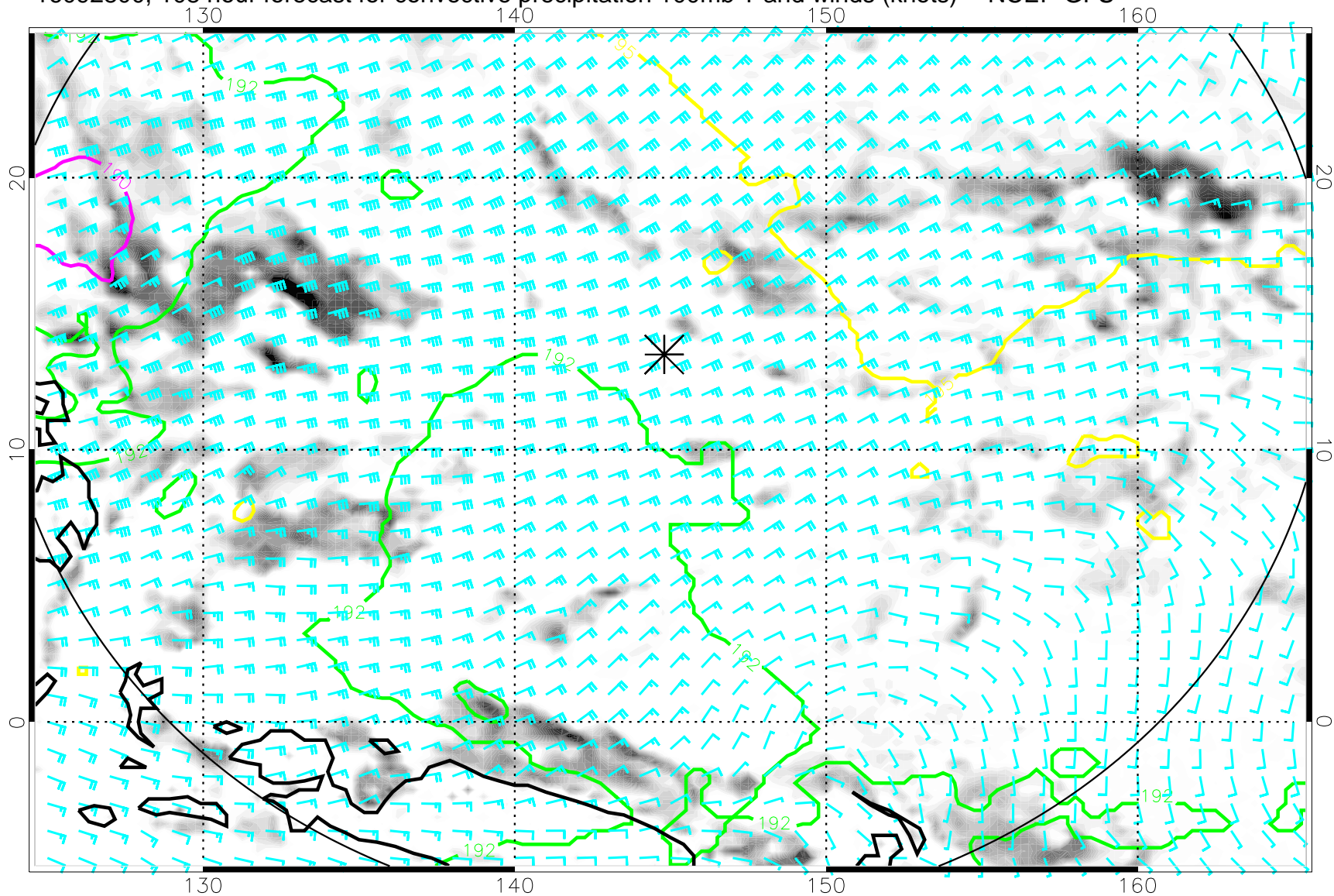
16092800, 108 hour forecast for convective precipitation 100mb T and winds (knots) -- NCEP GFS
