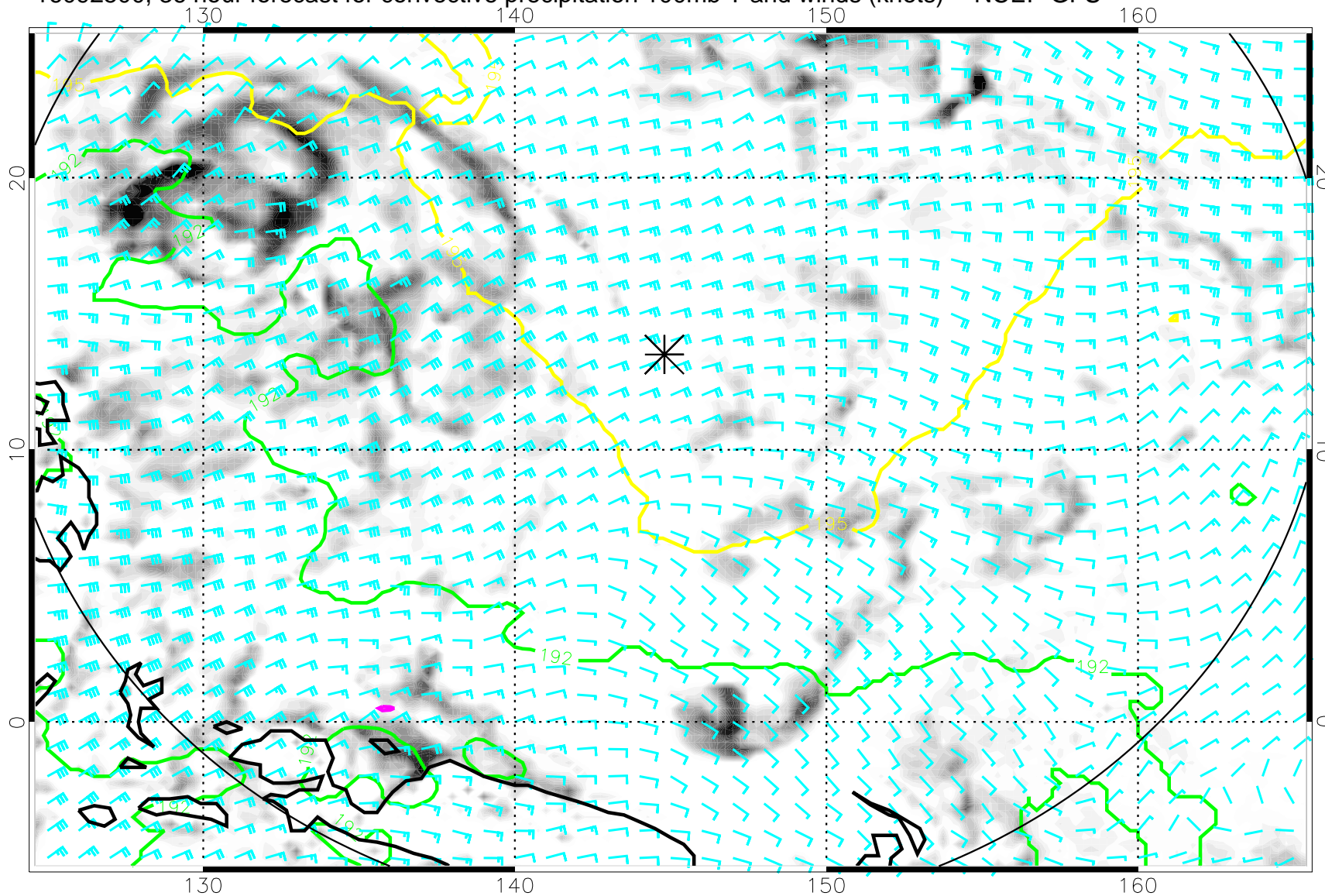
16092500, 36 hour forecast for convective precipitation 100mb T and winds (knots) -- NCEP GFS
