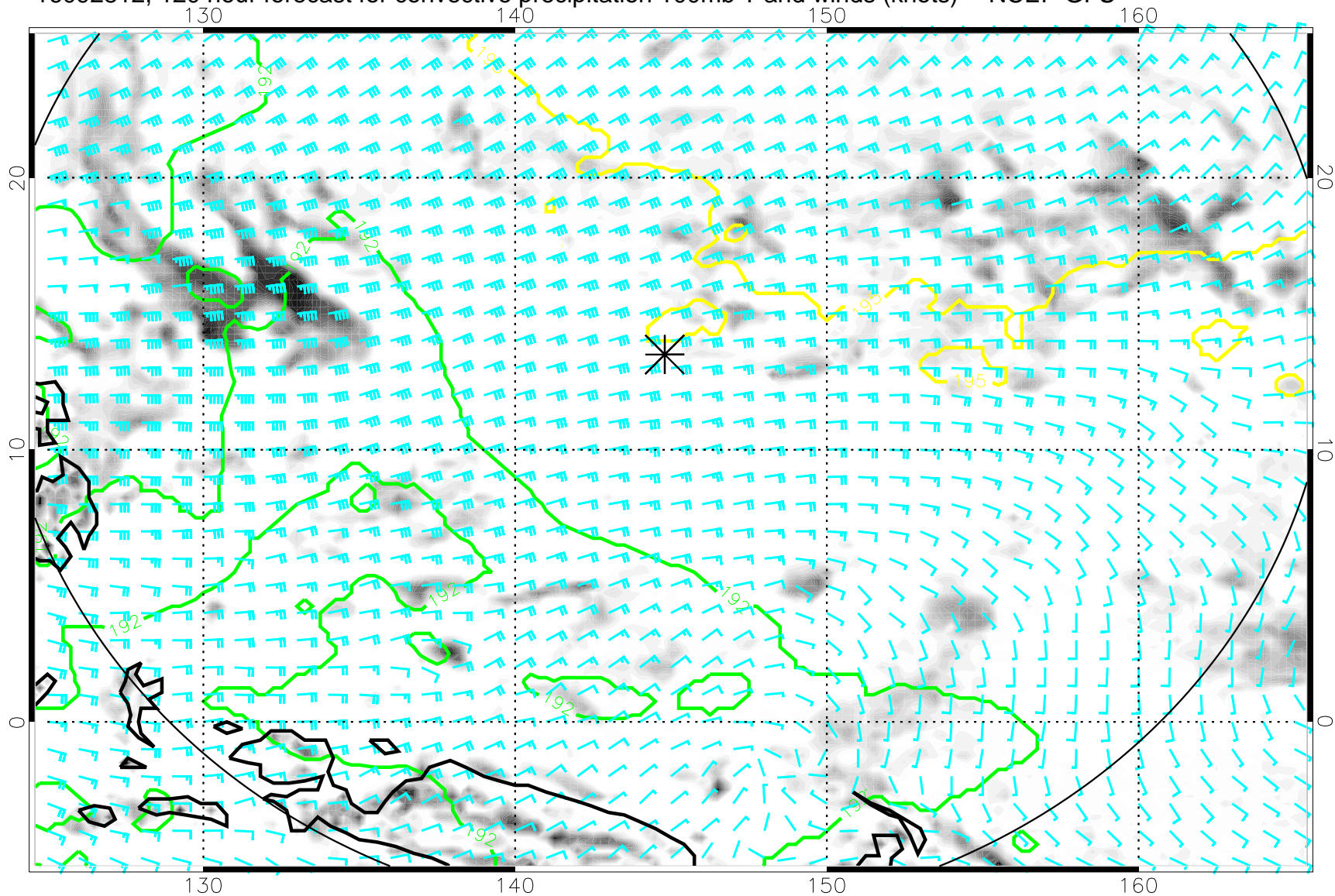
16092812, 120 hour forecast for convective precipitation 100mb T and winds (knots) -- NCEP GFS
