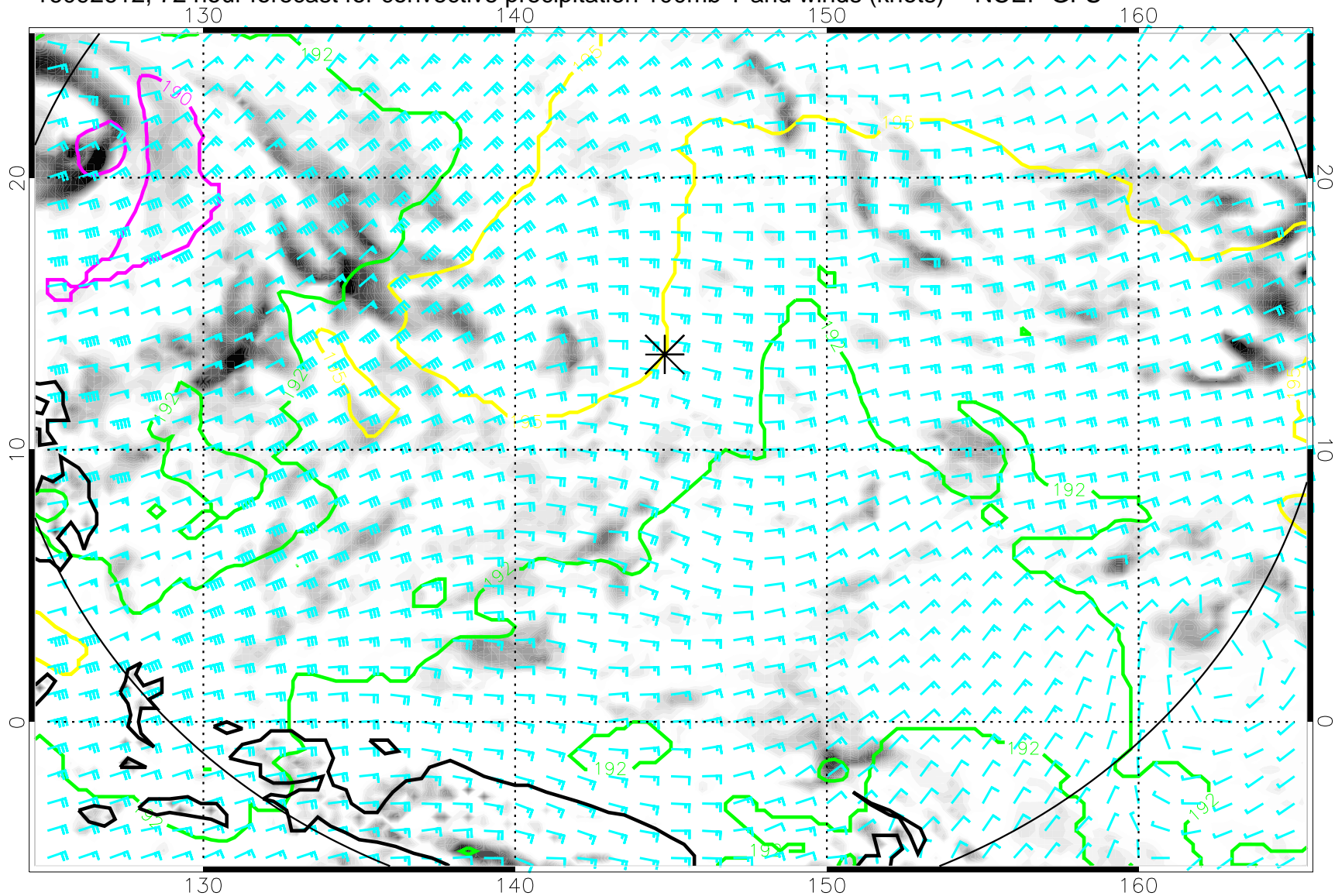
16092612, 72 hour forecast for convective precipitation 100mb T and winds (knots) -- NCEP GFS
