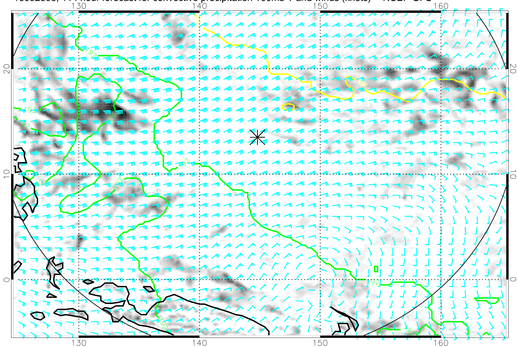
16092806, 114 hour forecast for convective precipitation 100mb T and winds (knots) -- NCEP GFS
