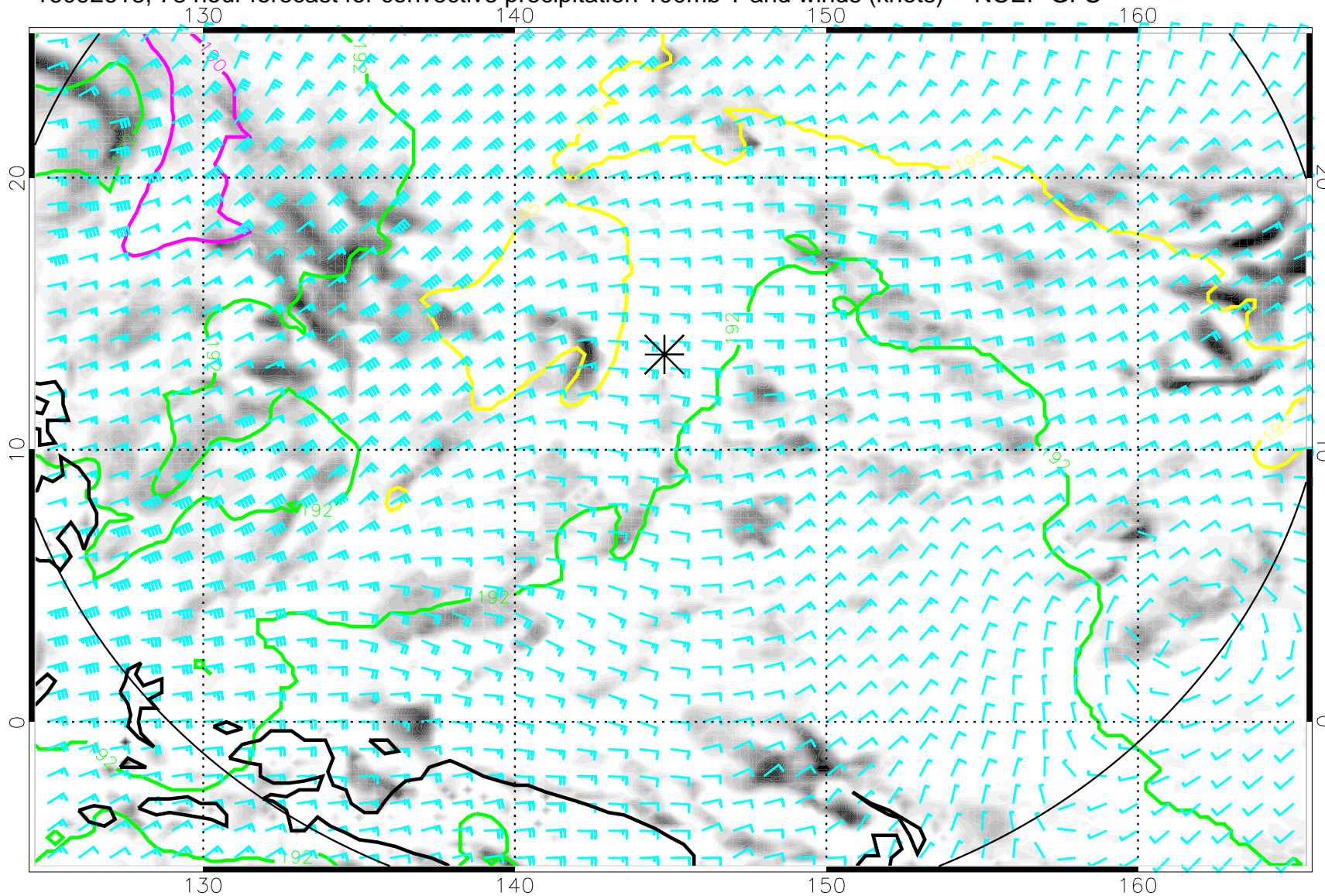
16092618, 78 hour forecast for convective precipitation 100mb T and winds (knots) -- NCEP GFS
