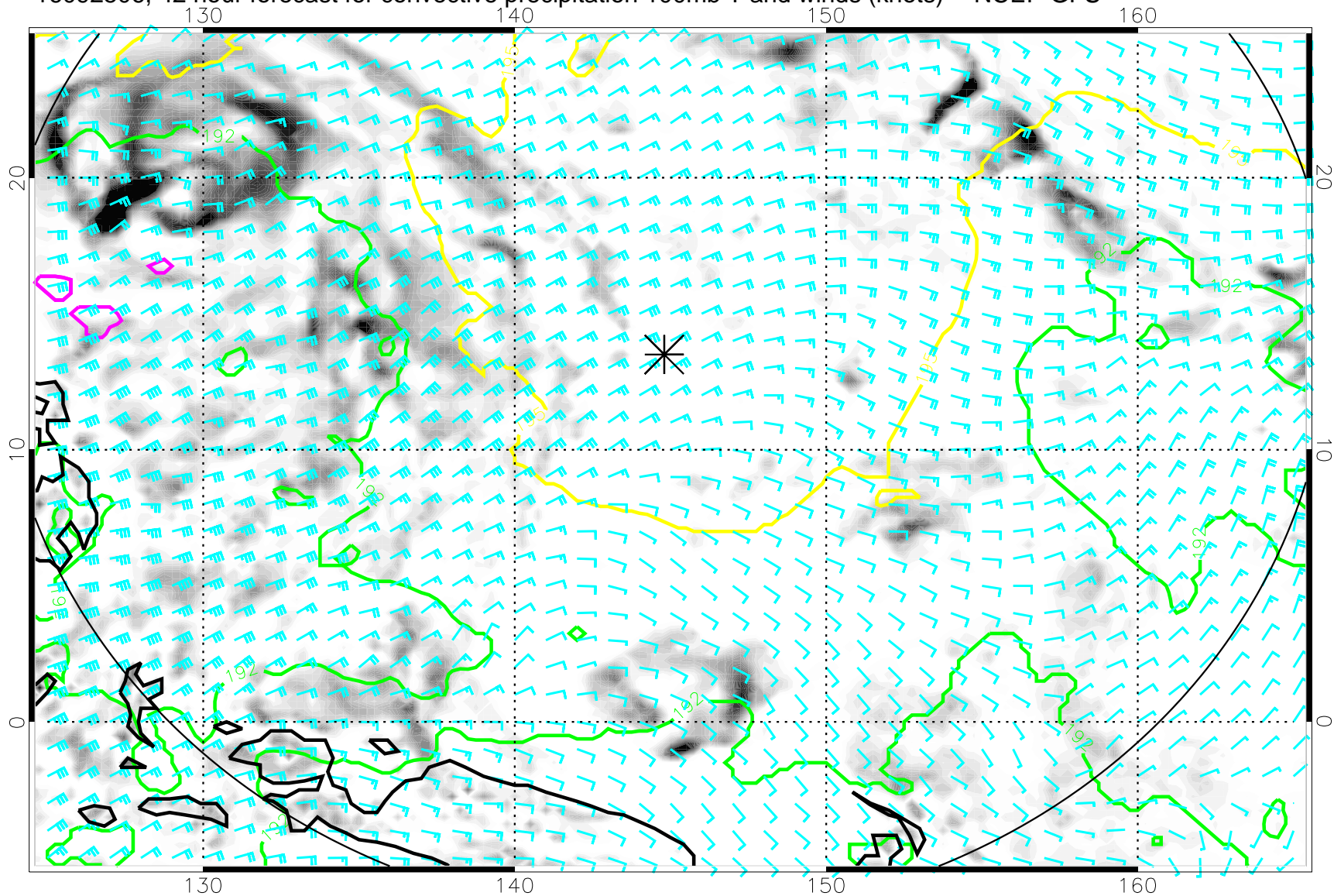
16092506, 42 hour forecast for convective precipitation 100mb T and winds (knots) -- NCEP GFS
