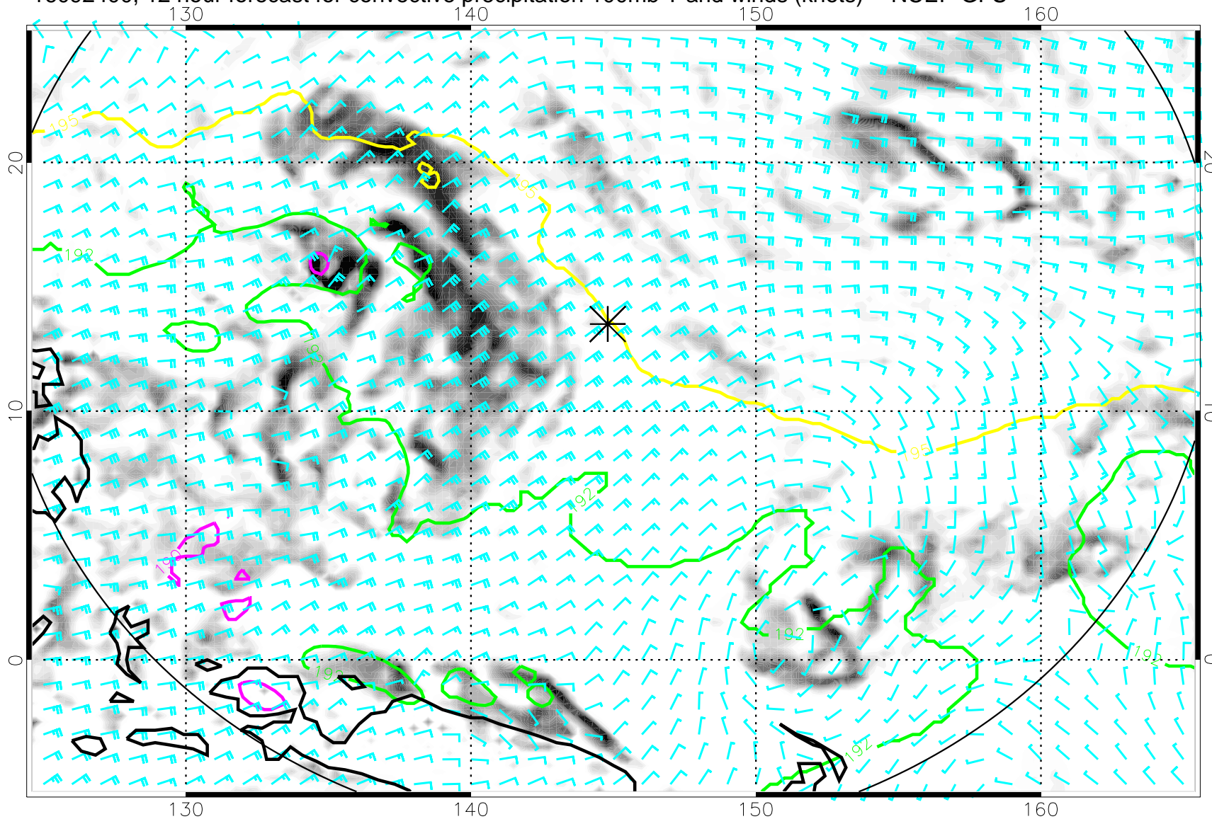
16092400, 12 hour forecast for convective precipitation 100mb T and winds (knots) -- NCEP GFS
