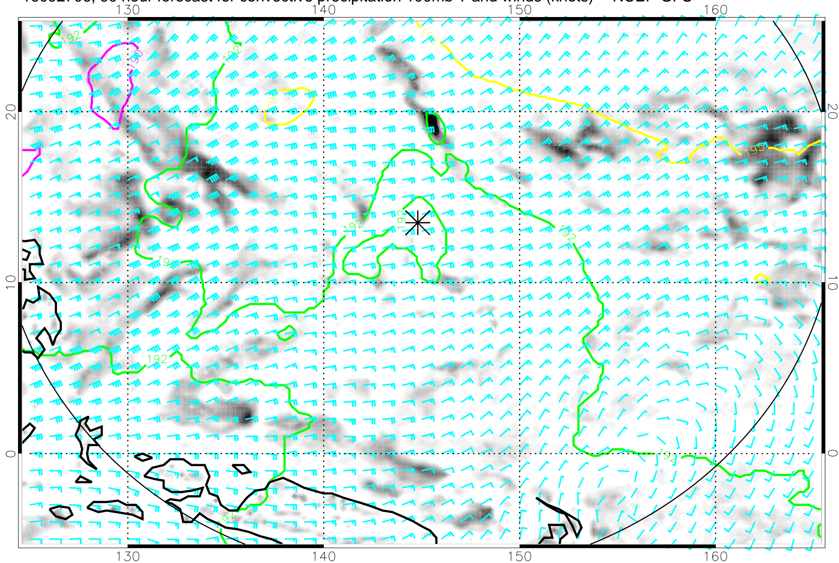
16092706, 90 hour forecast for convective precipitation 100mb T and winds (knots) -- NCEP GFS
