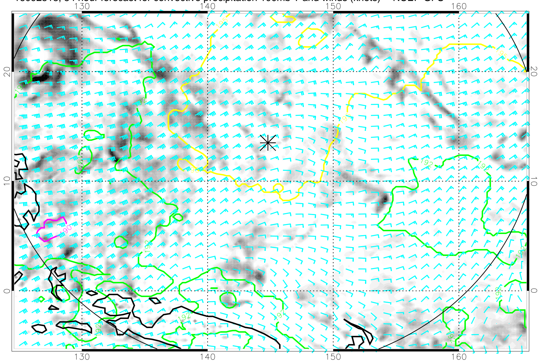
16092518, 54 hour forecast for convective precipitation 100mb T and winds (knots) -- NCEP GFS
