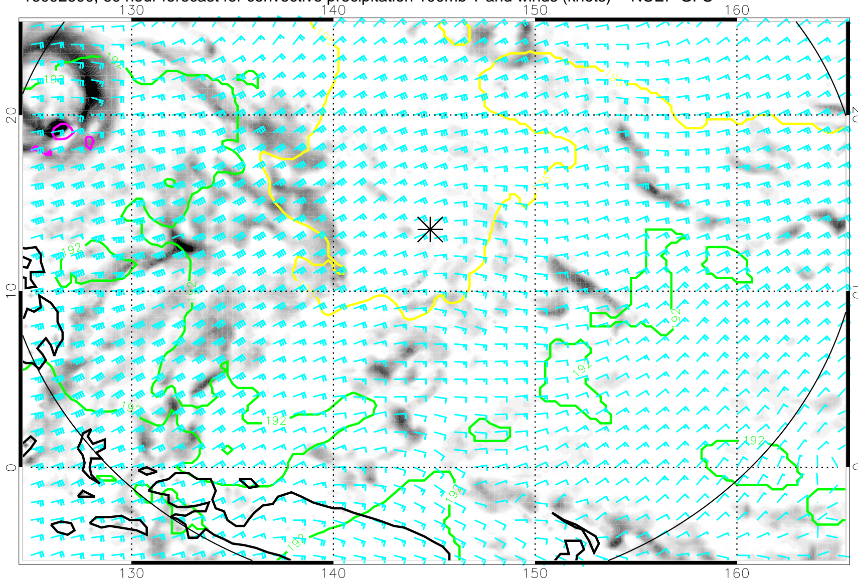
16092600, 60 hour forecast for convective precipitation 100mb T and winds (knots) -- NCEP GFS
