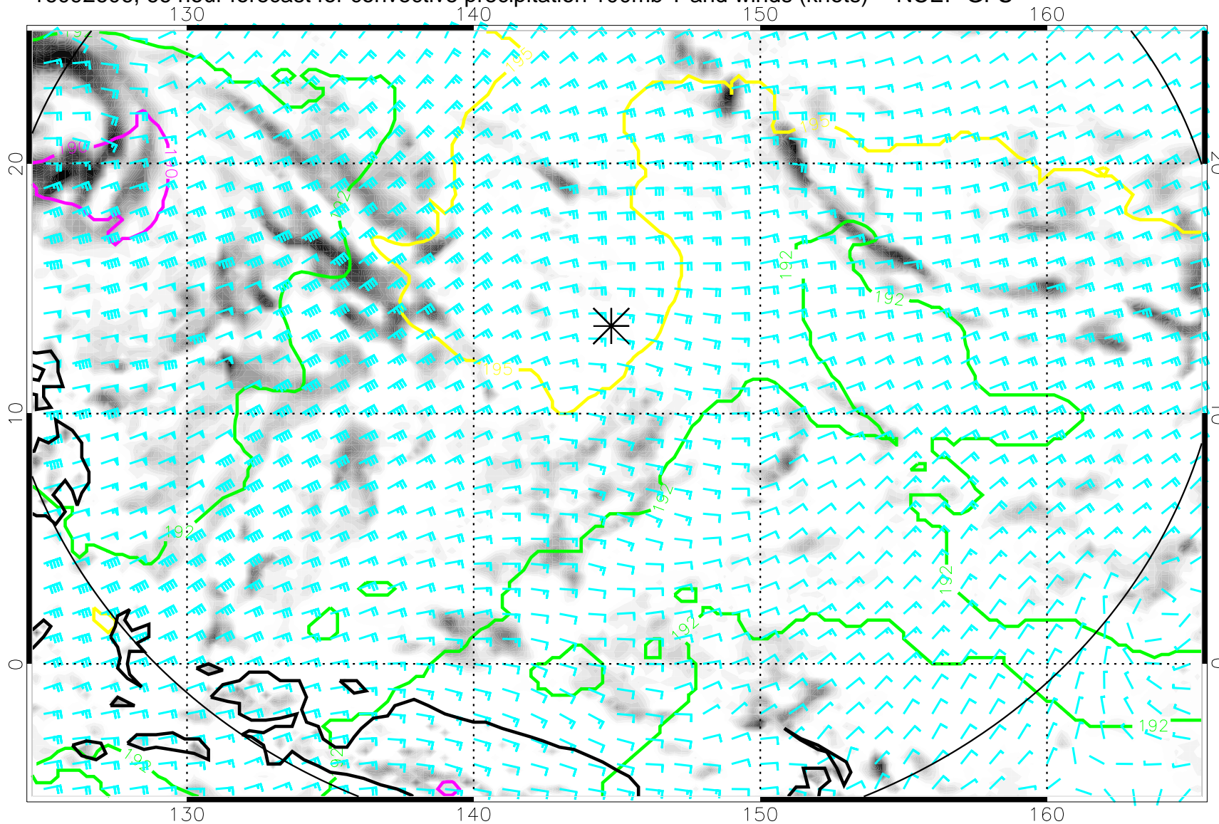
16092606, 66 hour forecast for convective precipitation 100mb T and winds (knots) -- NCEP GFS
