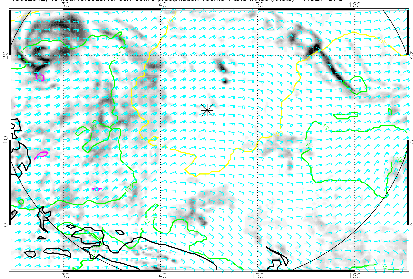
16092512, 48 hour forecast for convective precipitation 100mb T and winds (knots) -- NCEP GFS
