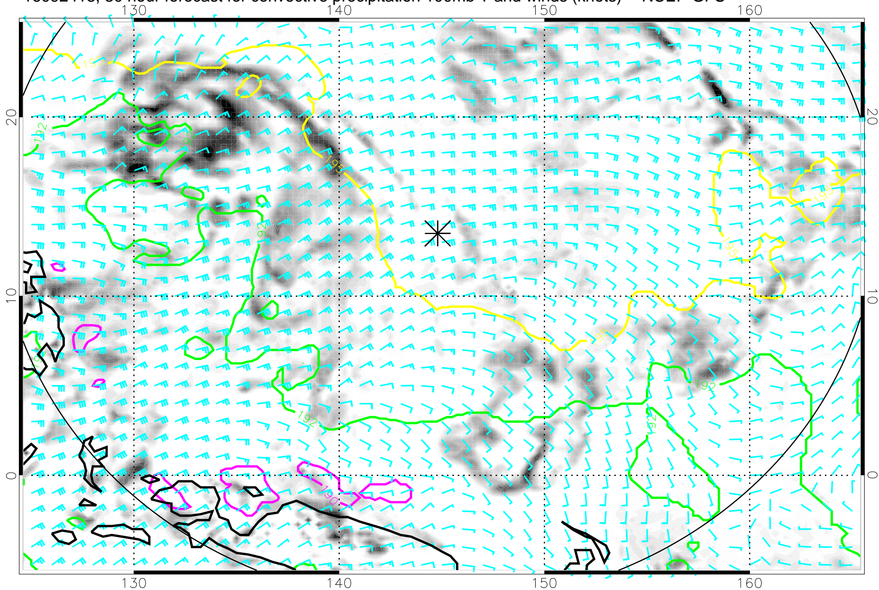
16092418, 30 hour forecast for convective precipitation 100mb T and winds (knots) -- NCEP GFS
