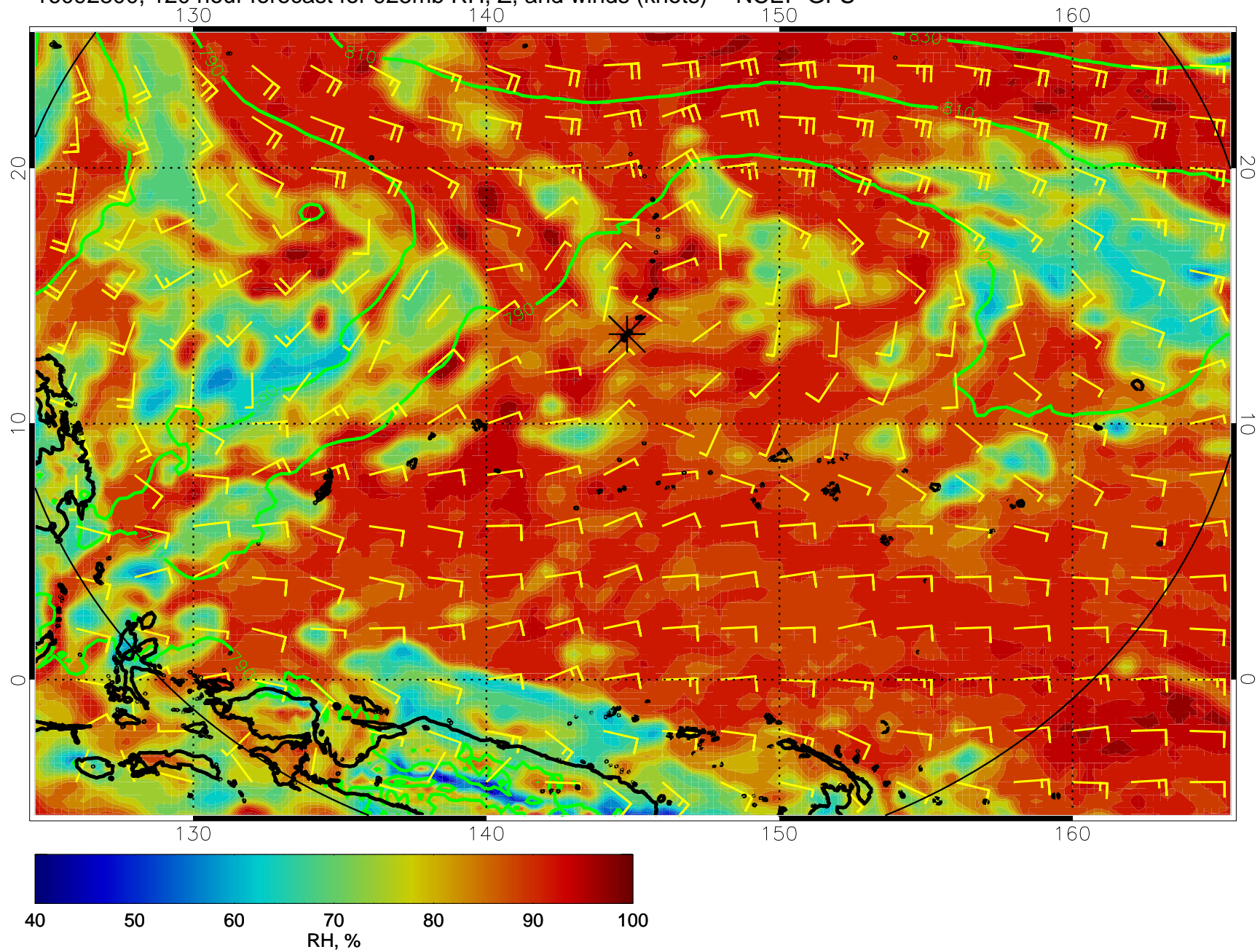
16092800, 120 hour forecast for 925mb RH, Z, and winds (knots) -- NCEP GFS
