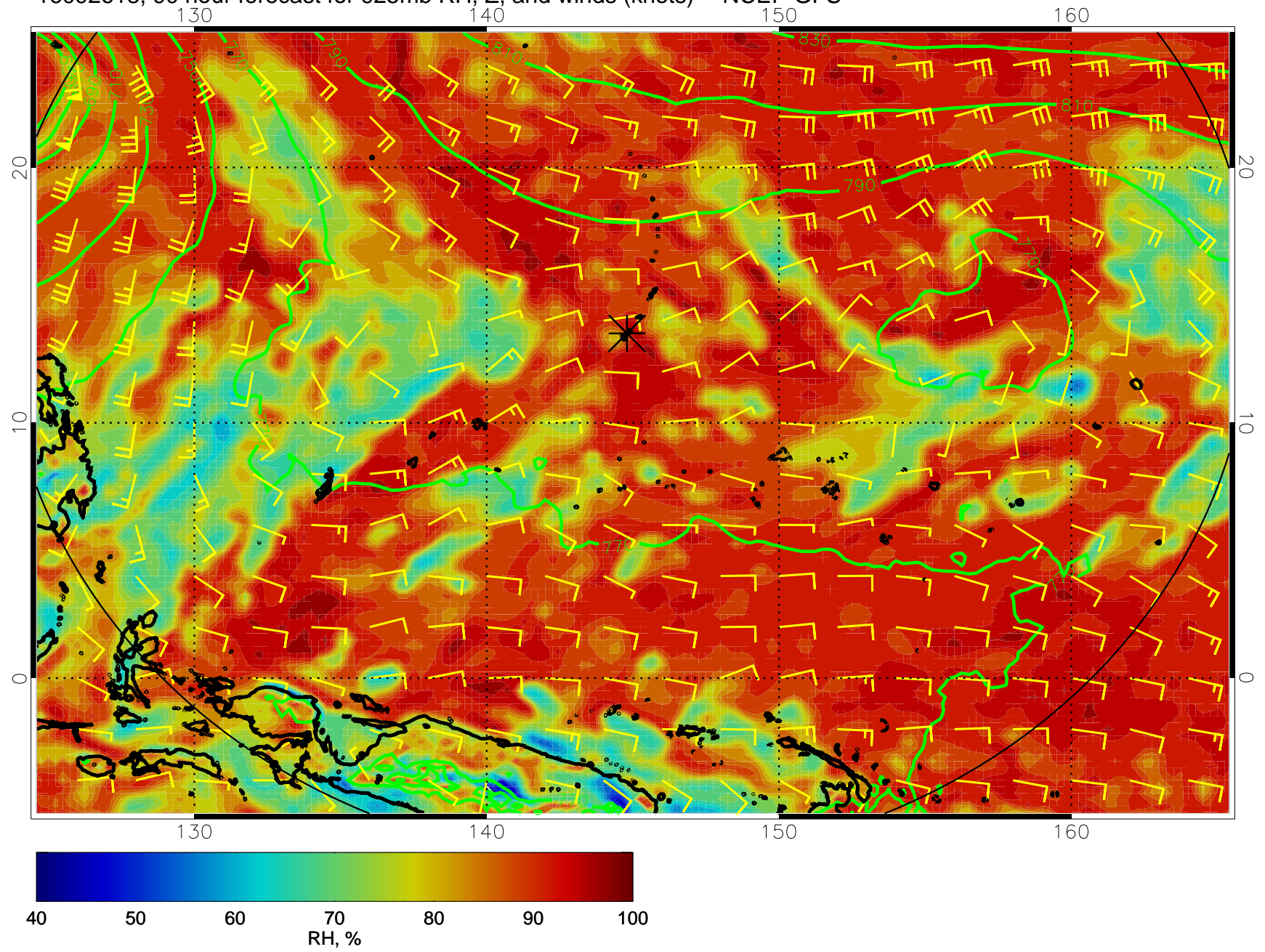
16092618, 90 hour forecast for 925mb RH, Z, and winds (knots) -- NCEP GFS
