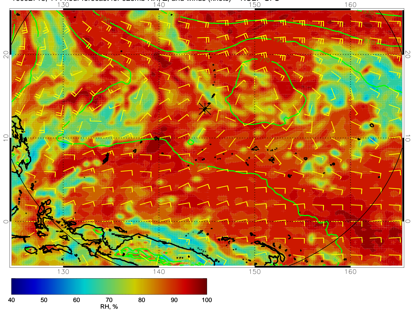
16092718, 114 hour forecast for 925mb RH, Z, and winds (knots) -- NCEP GFS
