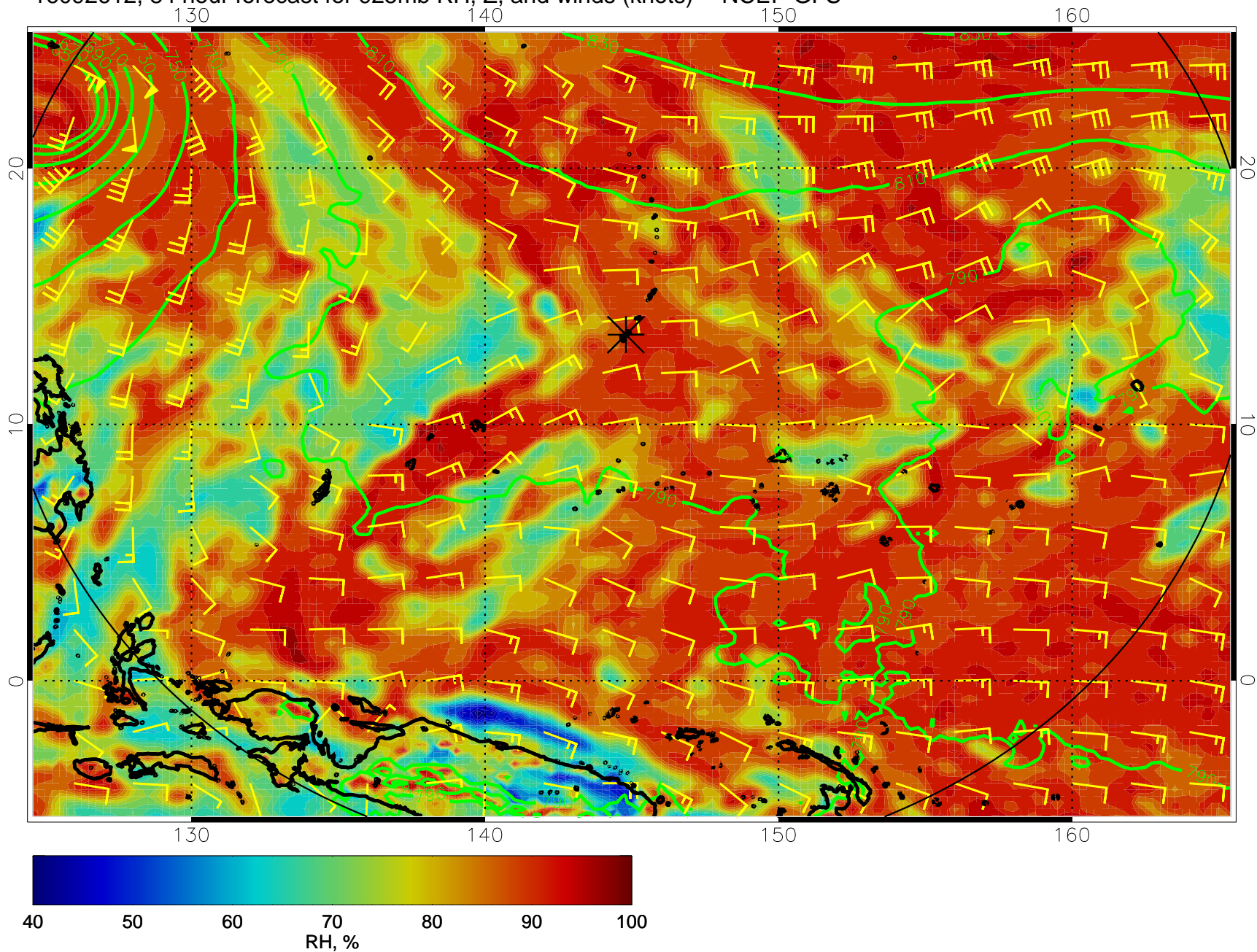
16092612, 84 hour forecast for 925mb RH, Z, and winds (knots) -- NCEP GFS
