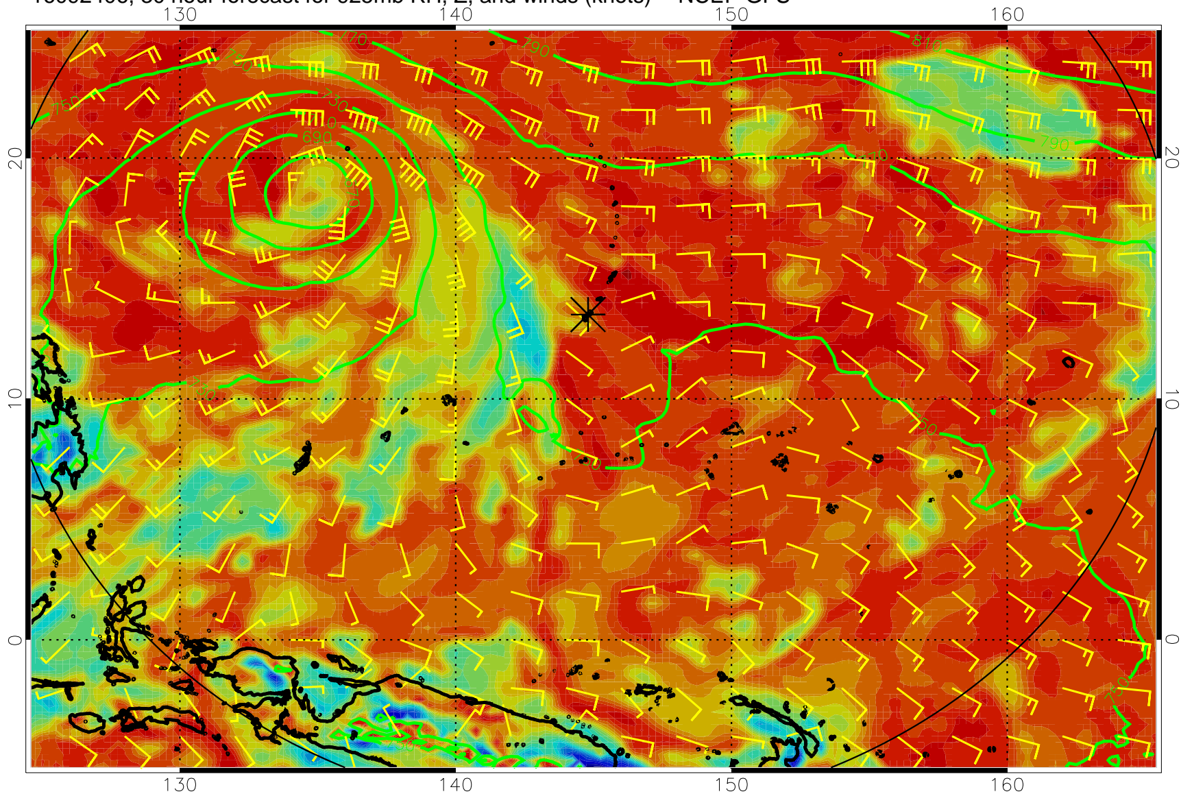
16092406, 30 hour forecast for 925mb RH, Z, and winds (knots) -- NCEP GFS
