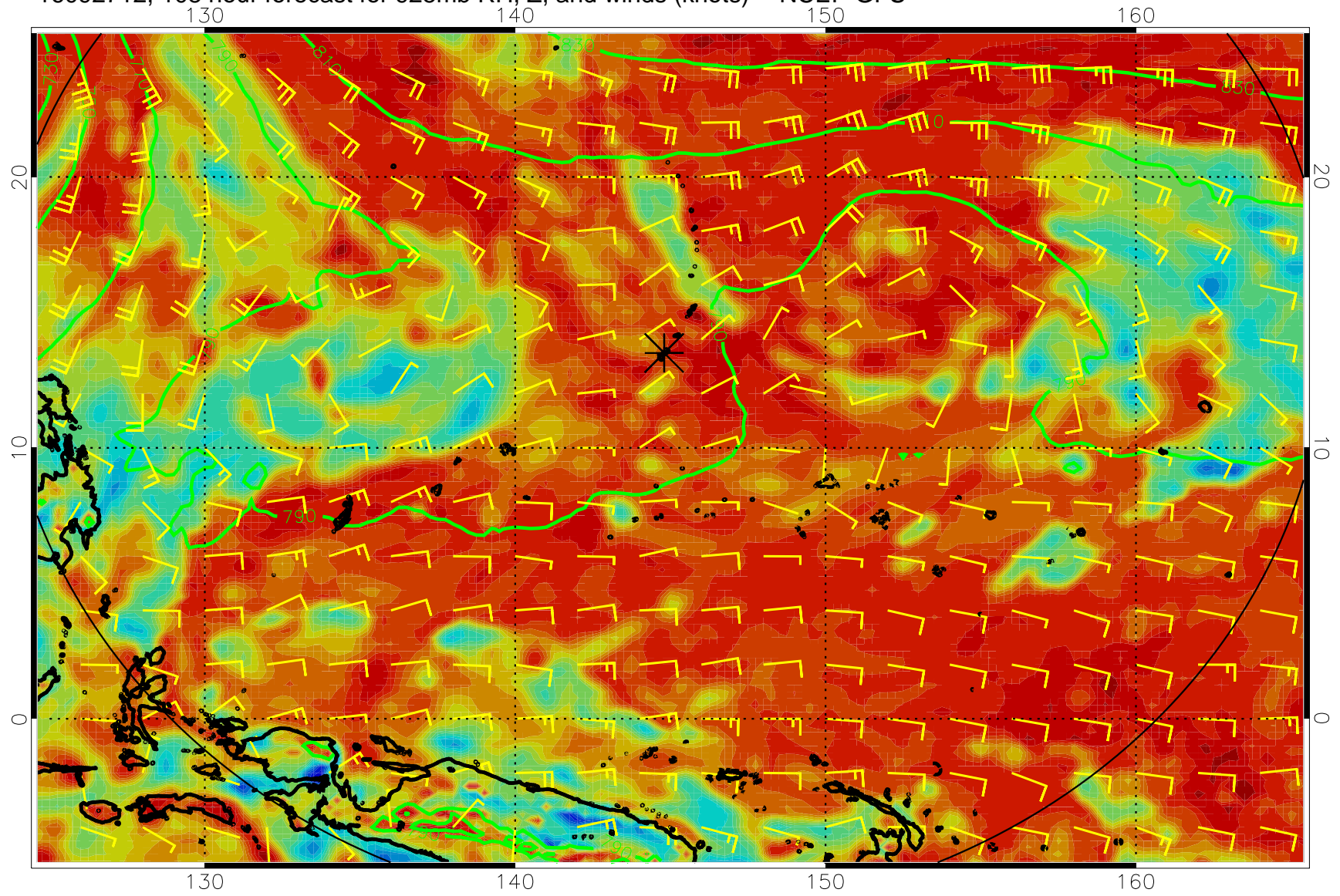
16092712, 108 hour forecast for 925mb RH, Z, and winds (knots) -- NCEP GFS
