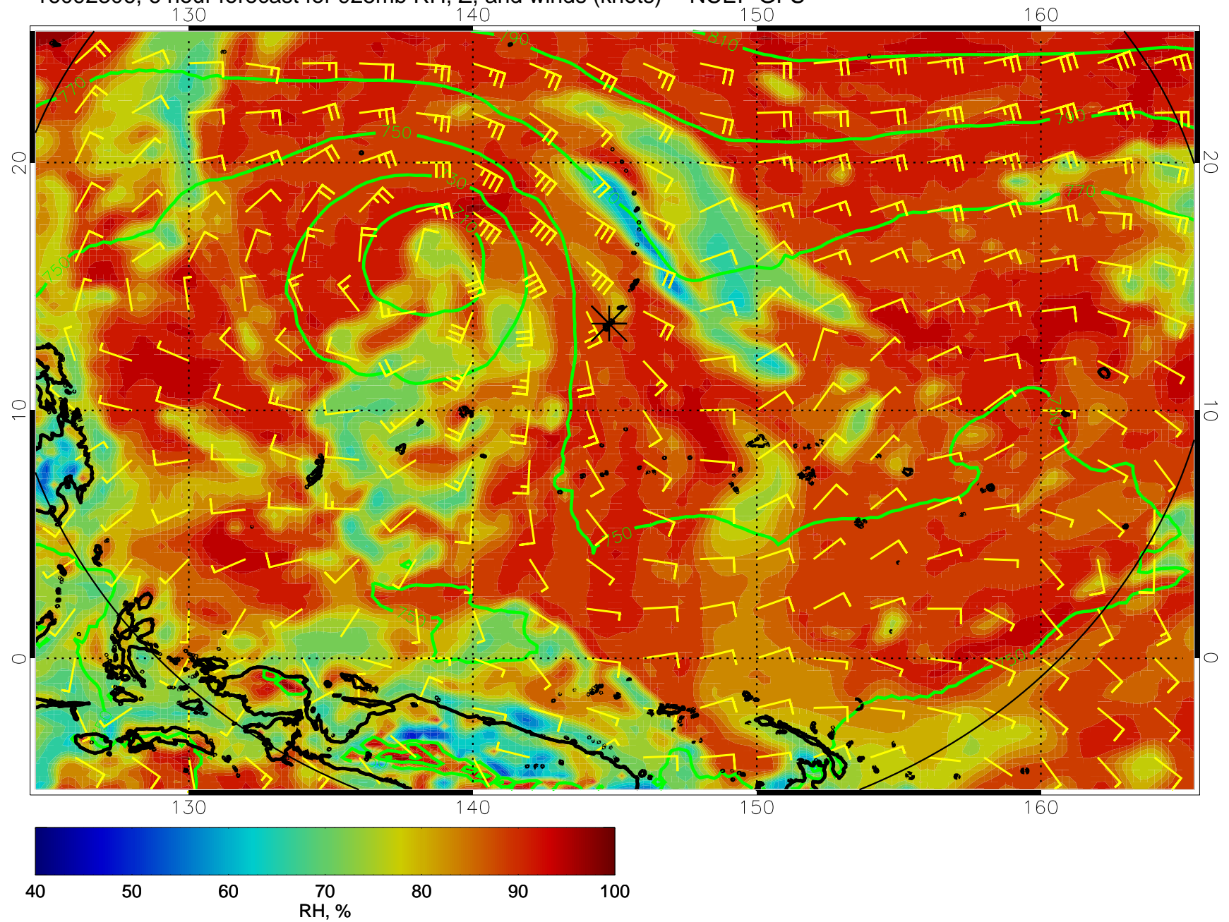
16092306, 6 hour forecast for 925mb RH, Z, and winds (knots) -- NCEP GFS
