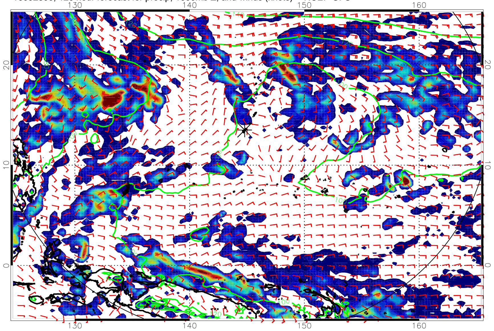
16092800, 120 hour forecast for precip, 1000mb Z, and winds (knots) -- NCEP GFS
