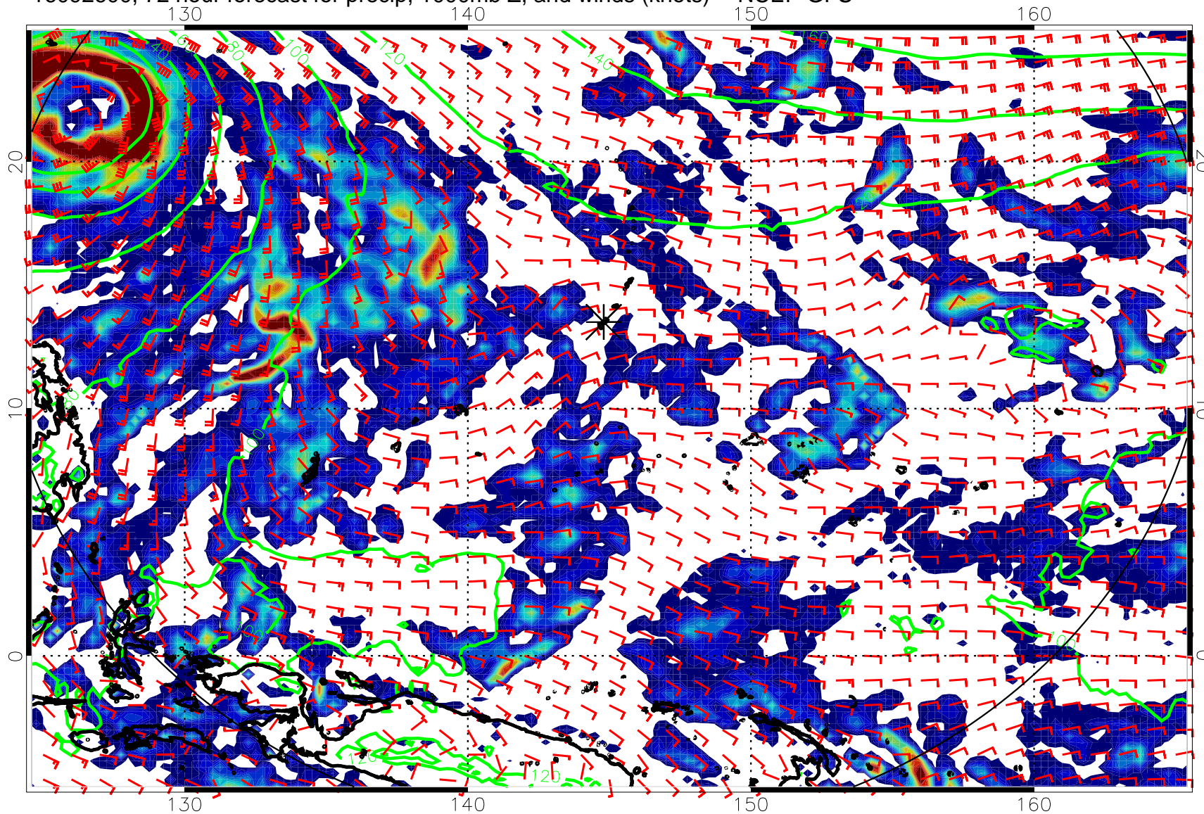
16092600, 72 hour forecast for precip, 1000mb Z, and winds (knots) -- NCEP GFS
