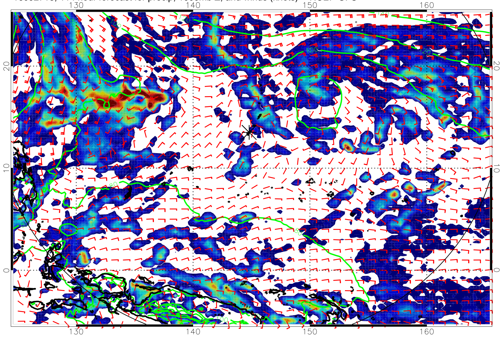
16092718, 114 hour forecast for precip, 1000mb Z, and winds (knots) -- NCEP GFS
