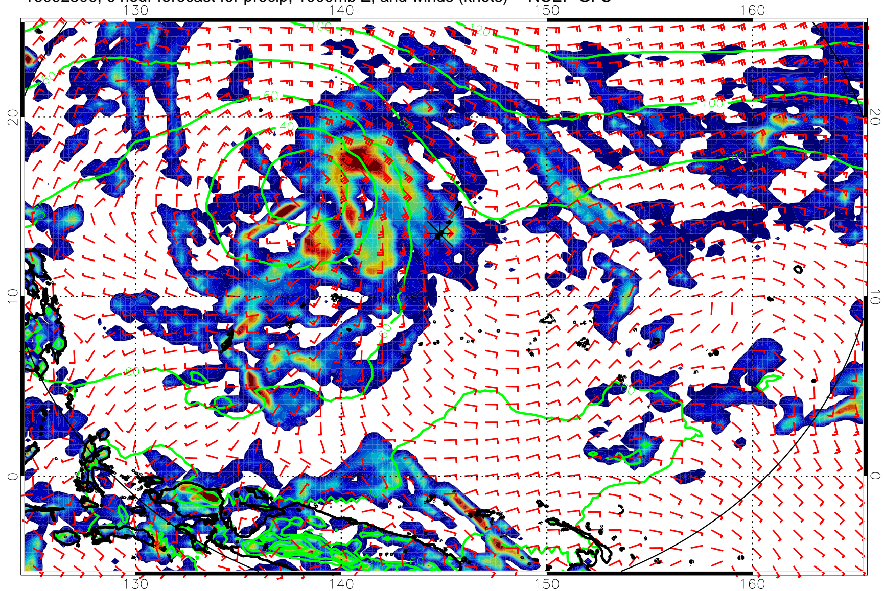
16092306, 6 hour forecast for precip, 1000mb Z, and winds (knots) -- NCEP GFS
