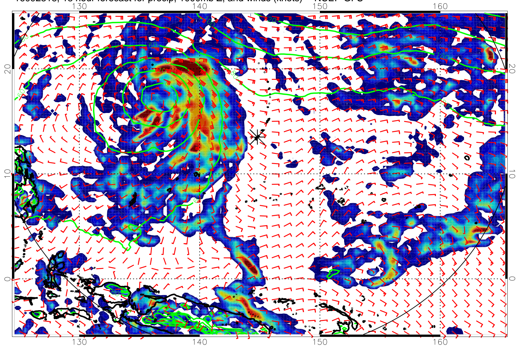
16092318, 18 hour forecast for precip, 1000mb Z, and winds (knots) -- NCEP GFS
