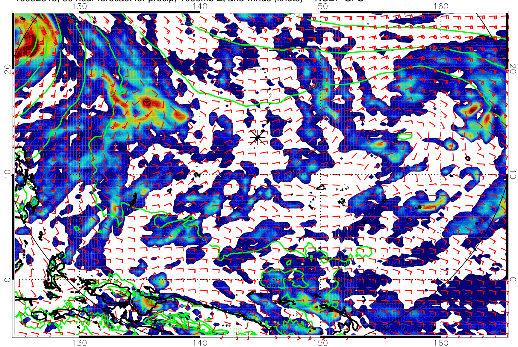
16092618, 90 hour forecast for precip, 1000mb Z, and winds (knots) -- NCEP GFS
