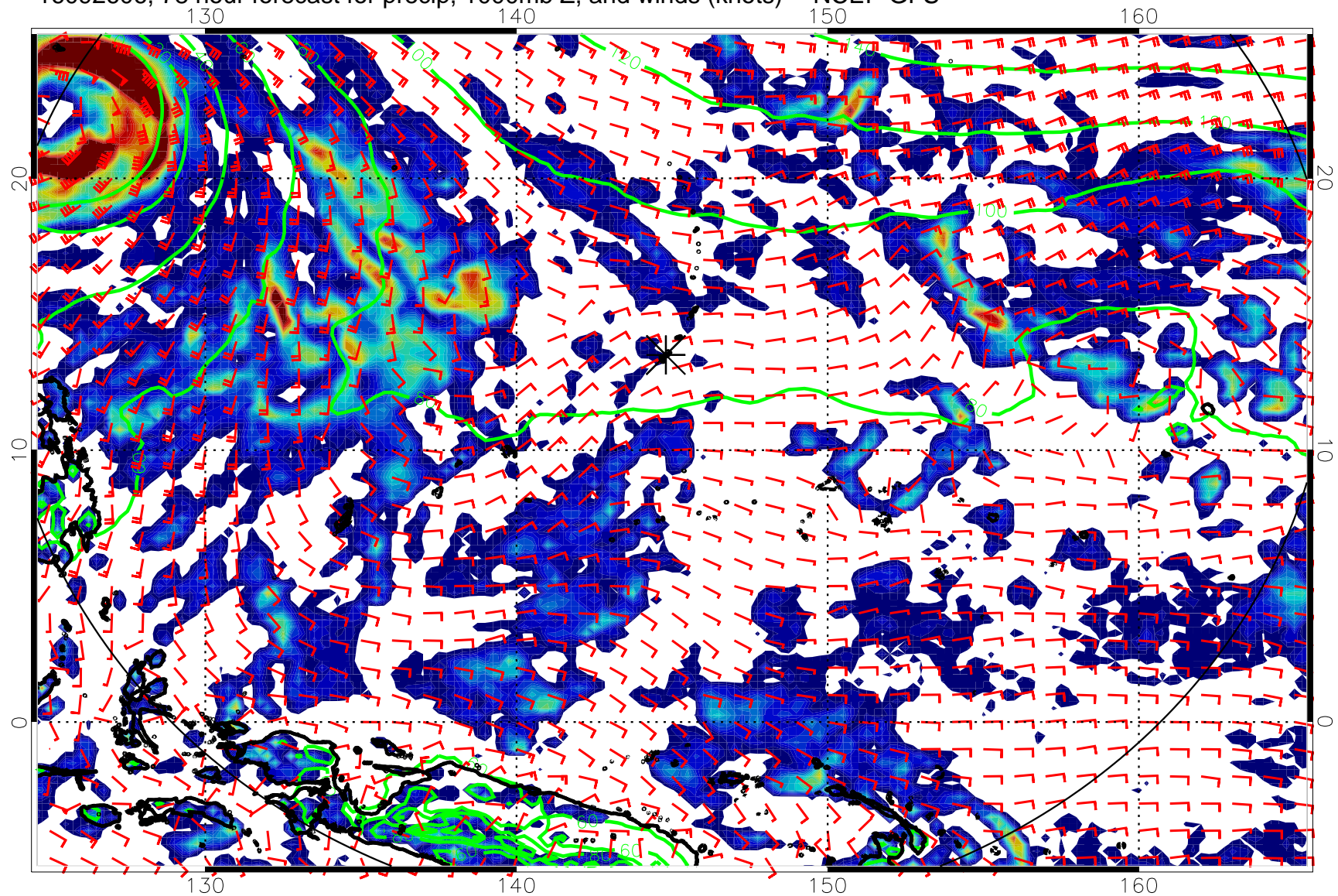
16092606, 78 hour forecast for precip, 1000mb Z, and winds (knots) -- NCEP GFS
