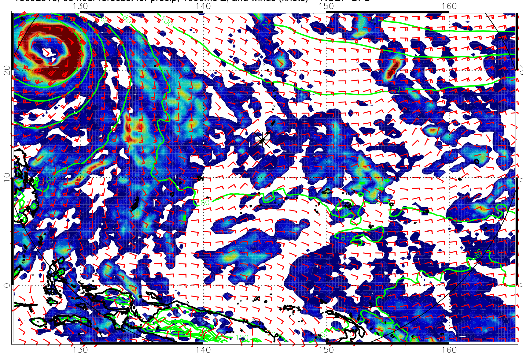
16092518, 66 hour forecast for precip, 1000mb Z, and winds (knots) -- NCEP GFS
