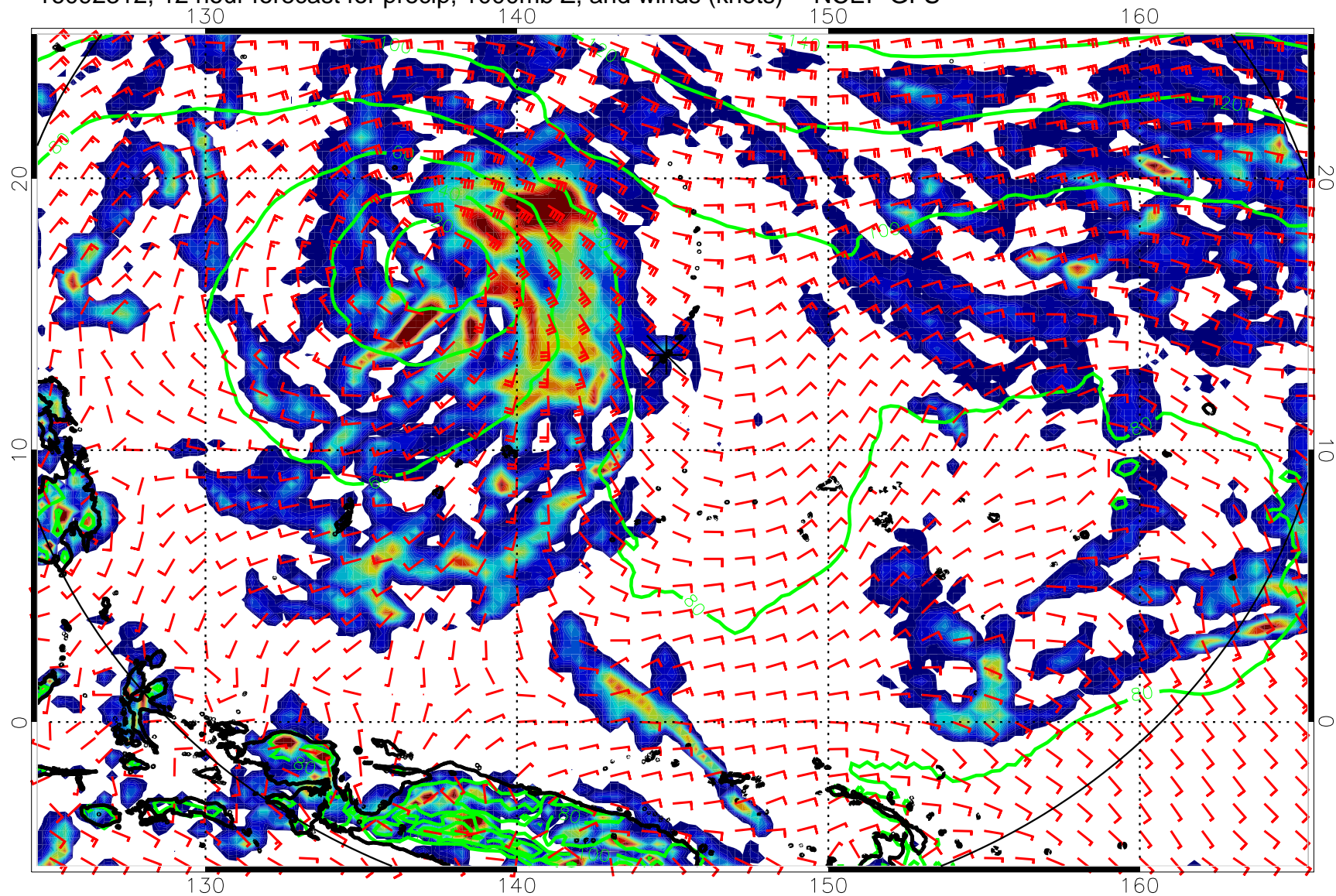
16092312, 12 hour forecast for precip, 1000mb Z, and winds (knots) -- NCEP GFS
