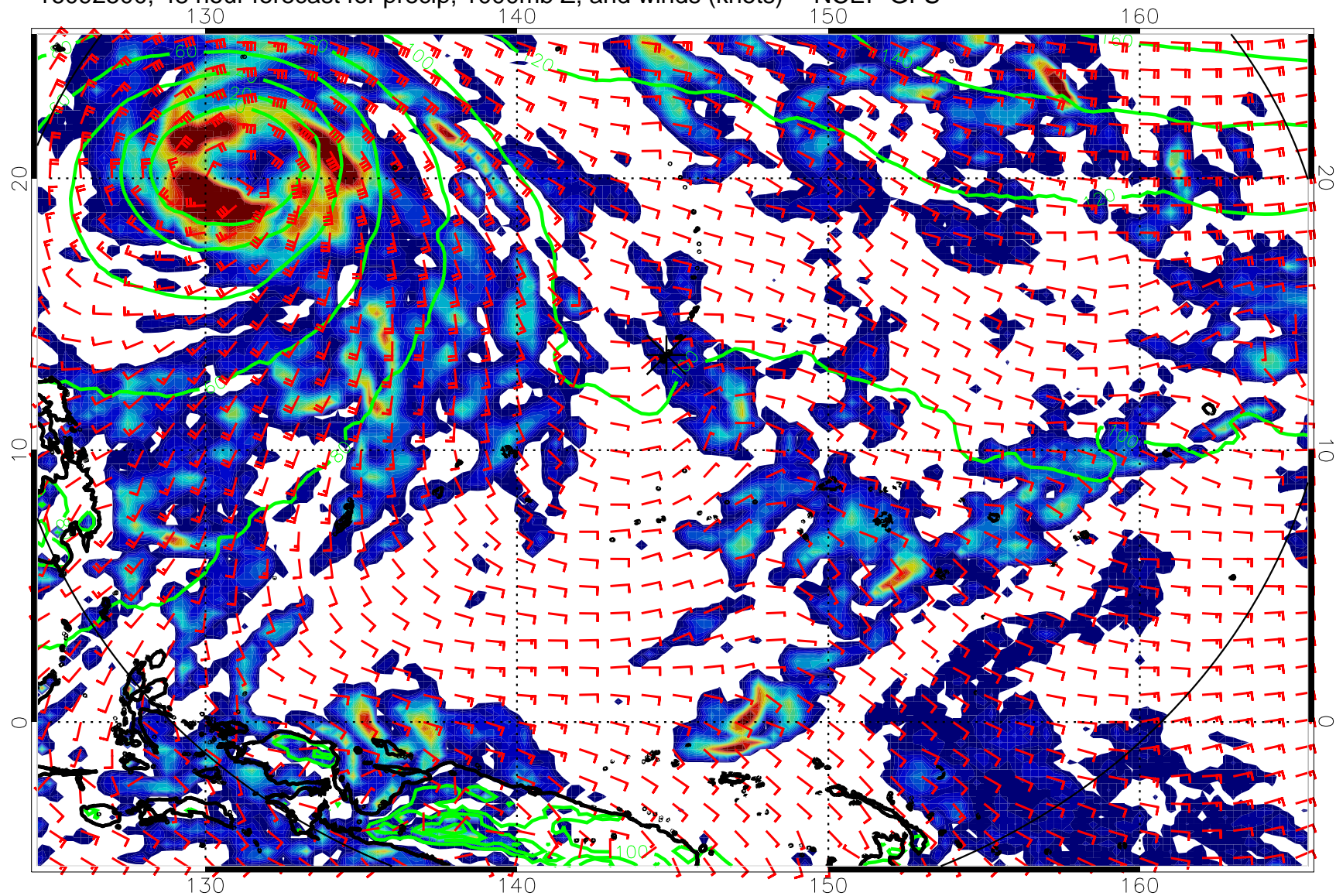
16092500, 48 hour forecast for precip, 1000mb Z, and winds (knots) -- NCEP GFS
