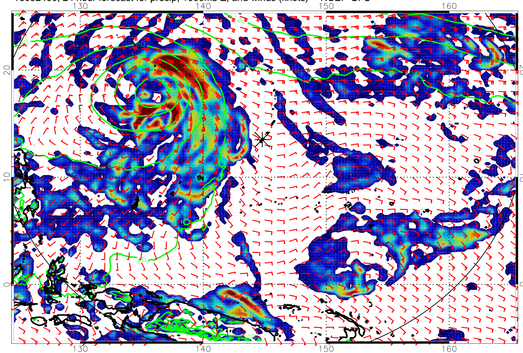
16092400, 24 hour forecast for precip, 1000mb Z, and winds (knots) -- NCEP GFS
