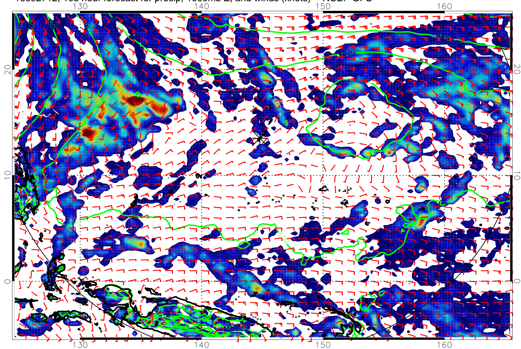
16092712, 108 hour forecast for precip, 1000mb Z, and winds (knots) -- NCEP GFS
