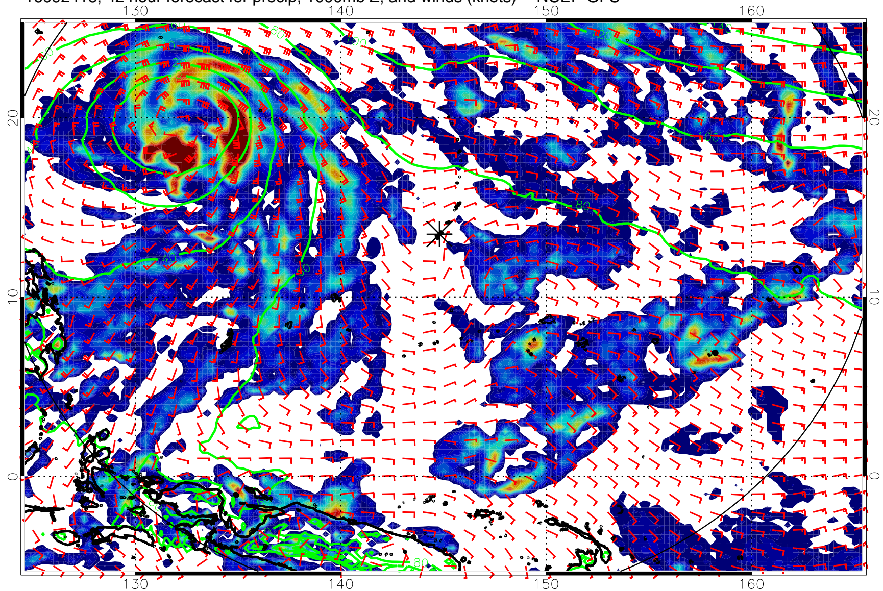
16092418, 42 hour forecast for precip, 1000mb Z, and winds (knots) -- NCEP GFS
