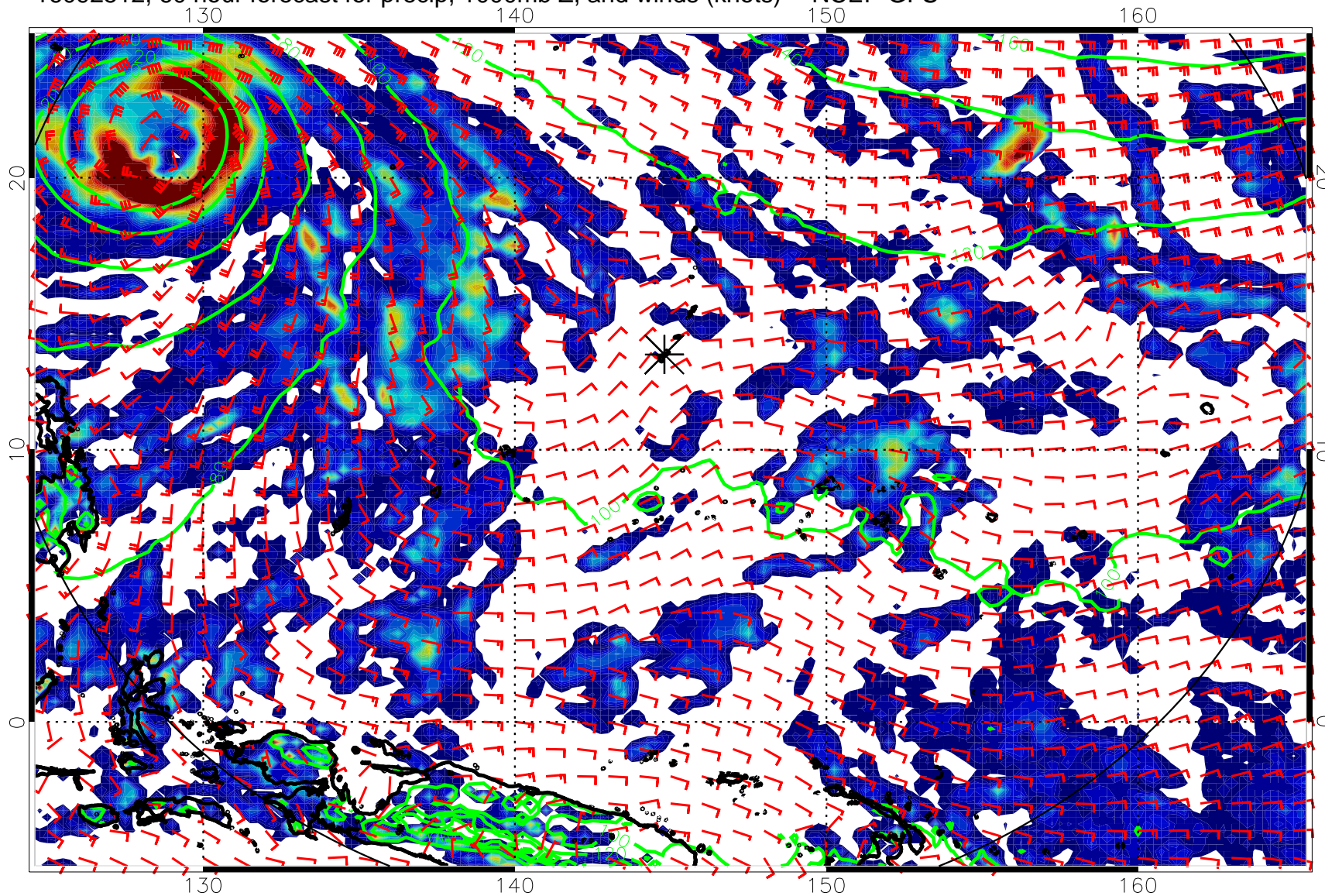
16092512, 60 hour forecast for precip, 1000mb Z, and winds (knots) -- NCEP GFS
