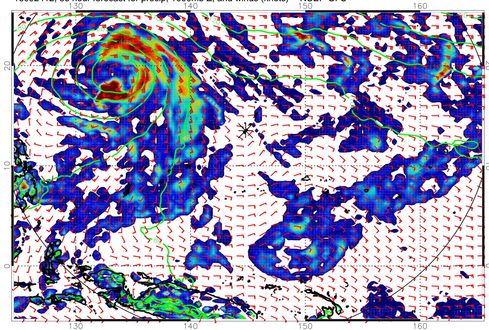
16092412, 36 hour forecast for precip, 1000mb Z, and winds (knots) -- NCEP GFS
