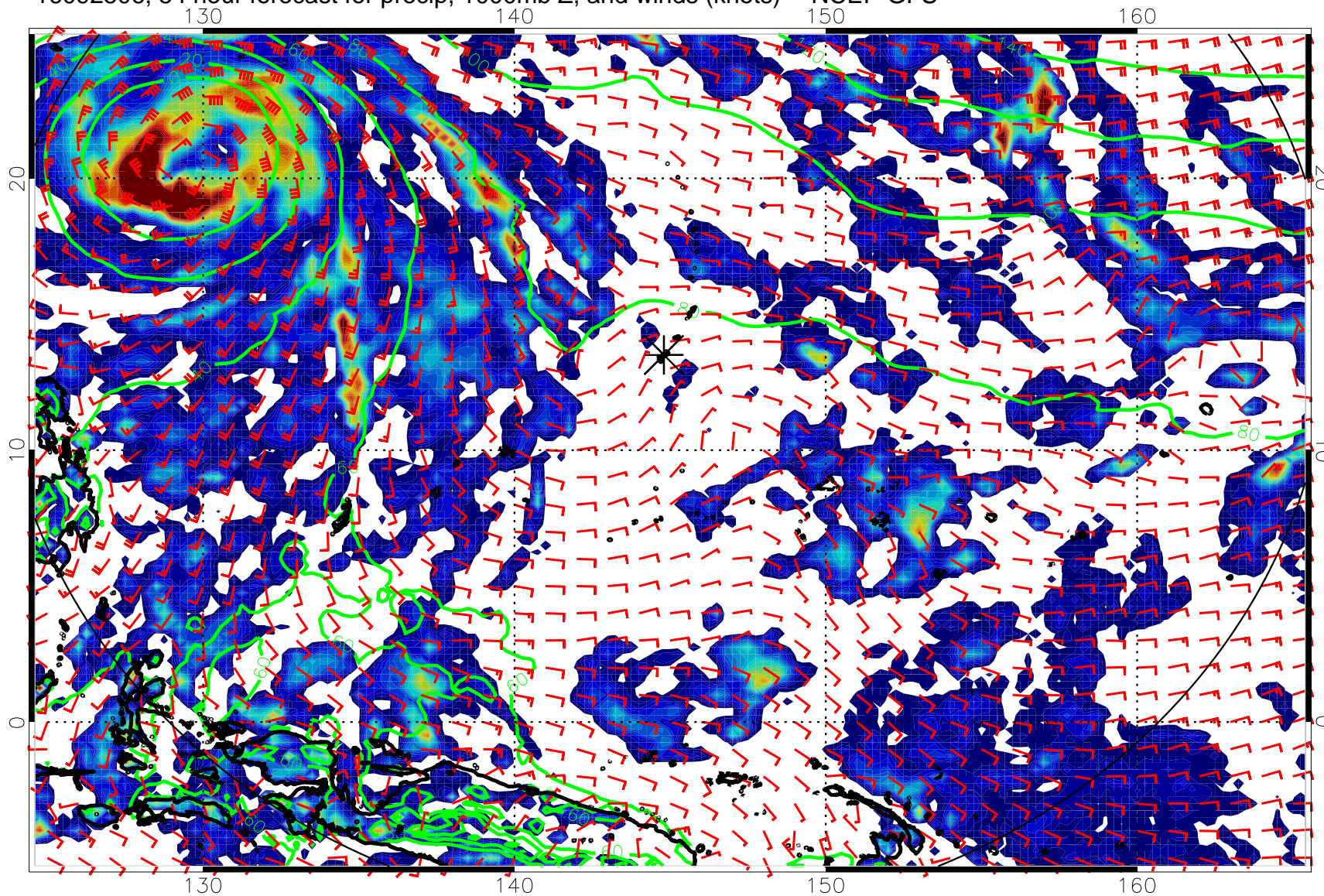
16092506, 54 hour forecast for precip, 1000mb Z, and winds (knots) -- NCEP GFS
