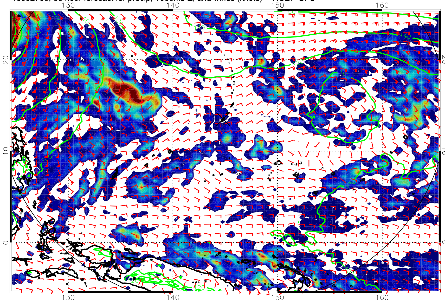
16092700, 96 hour forecast for precip, 1000mb Z, and winds (knots) -- NCEP GFS
