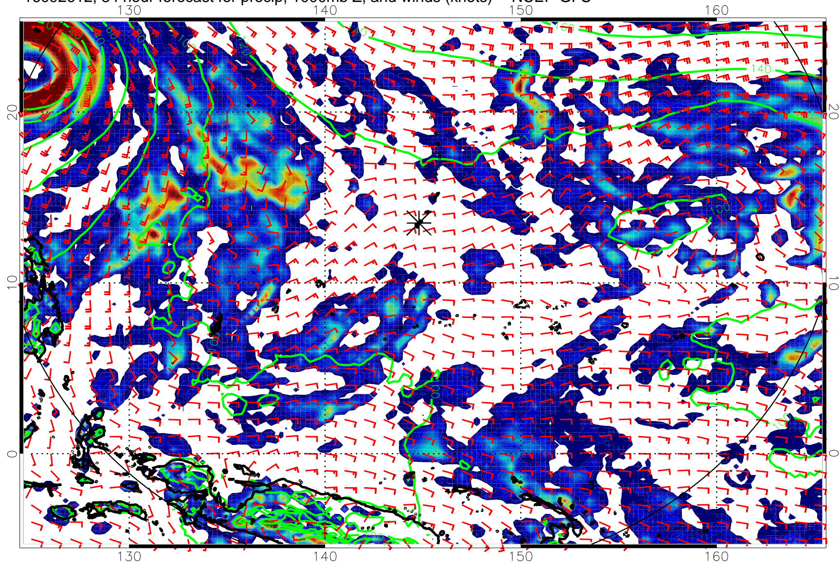
16092612, 84 hour forecast for precip, 1000mb Z, and winds (knots) -- NCEP GFS
