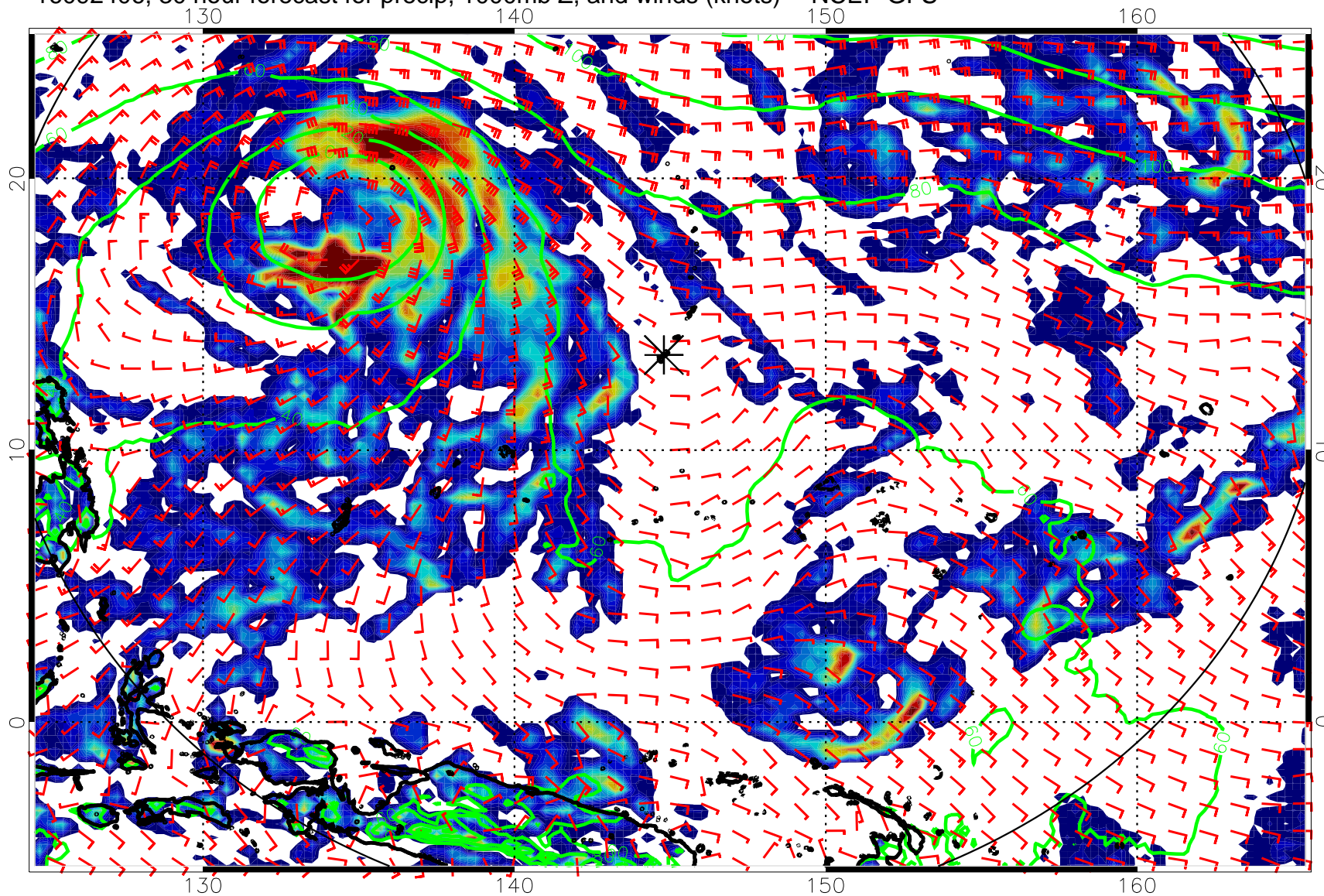
16092406, 30 hour forecast for precip, 1000mb Z, and winds (knots) -- NCEP GFS
