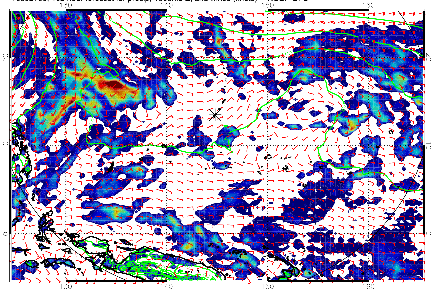
16092706, 102 hour forecast for precip, 1000mb Z, and winds (knots) -- NCEP GFS
