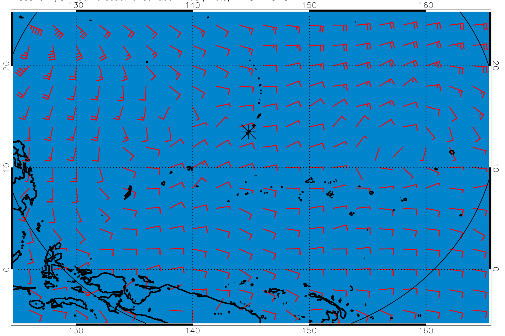
16092612, 84 hour forecast for surface winds (knots) -- NCEP GFS
