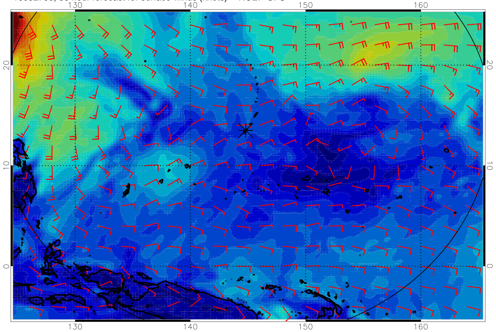
16092700, 96 hour forecast for surface winds (knots) -- NCEP GFS
