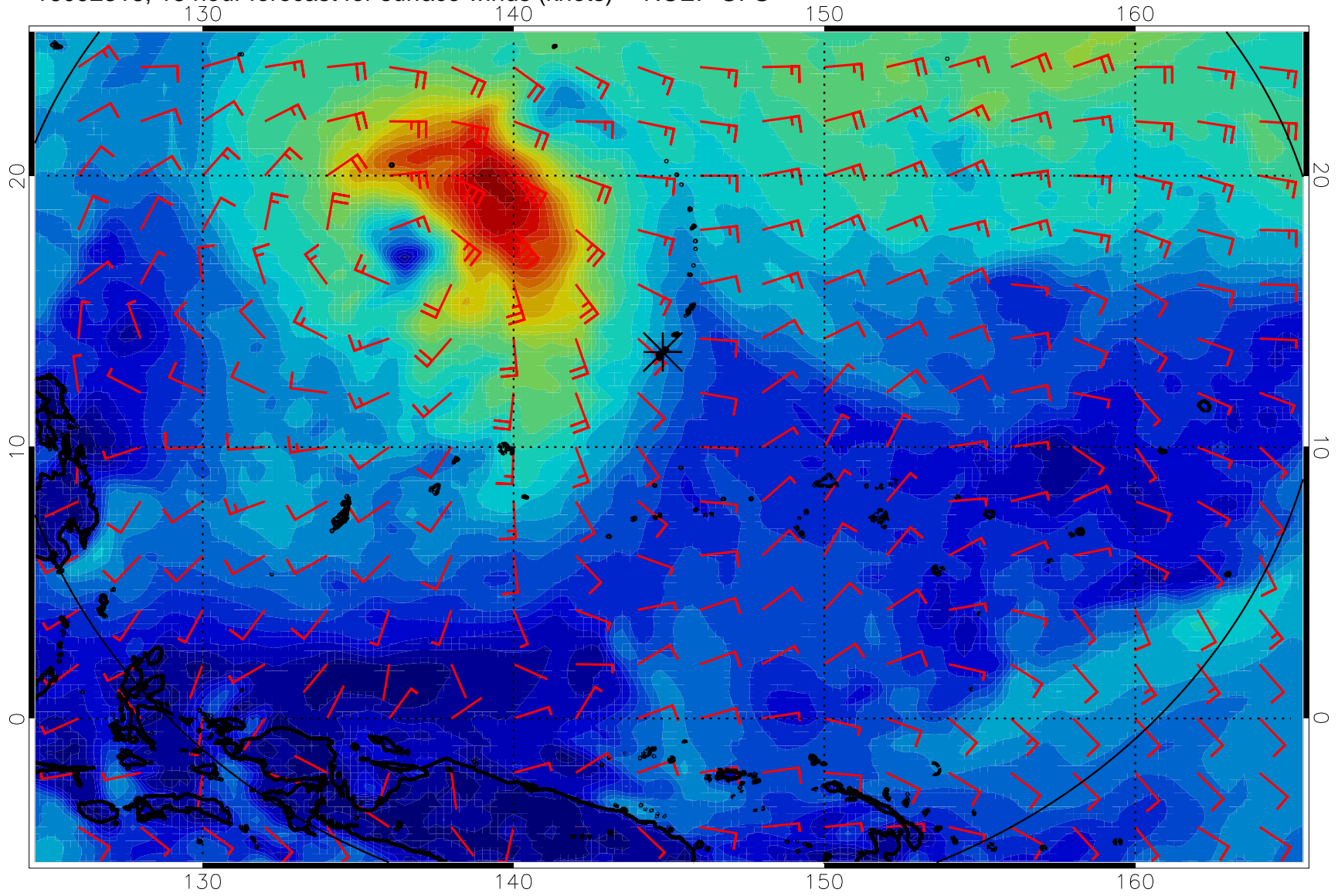
16092318, 18 hour forecast for surface winds (knots) -- NCEP GFS
