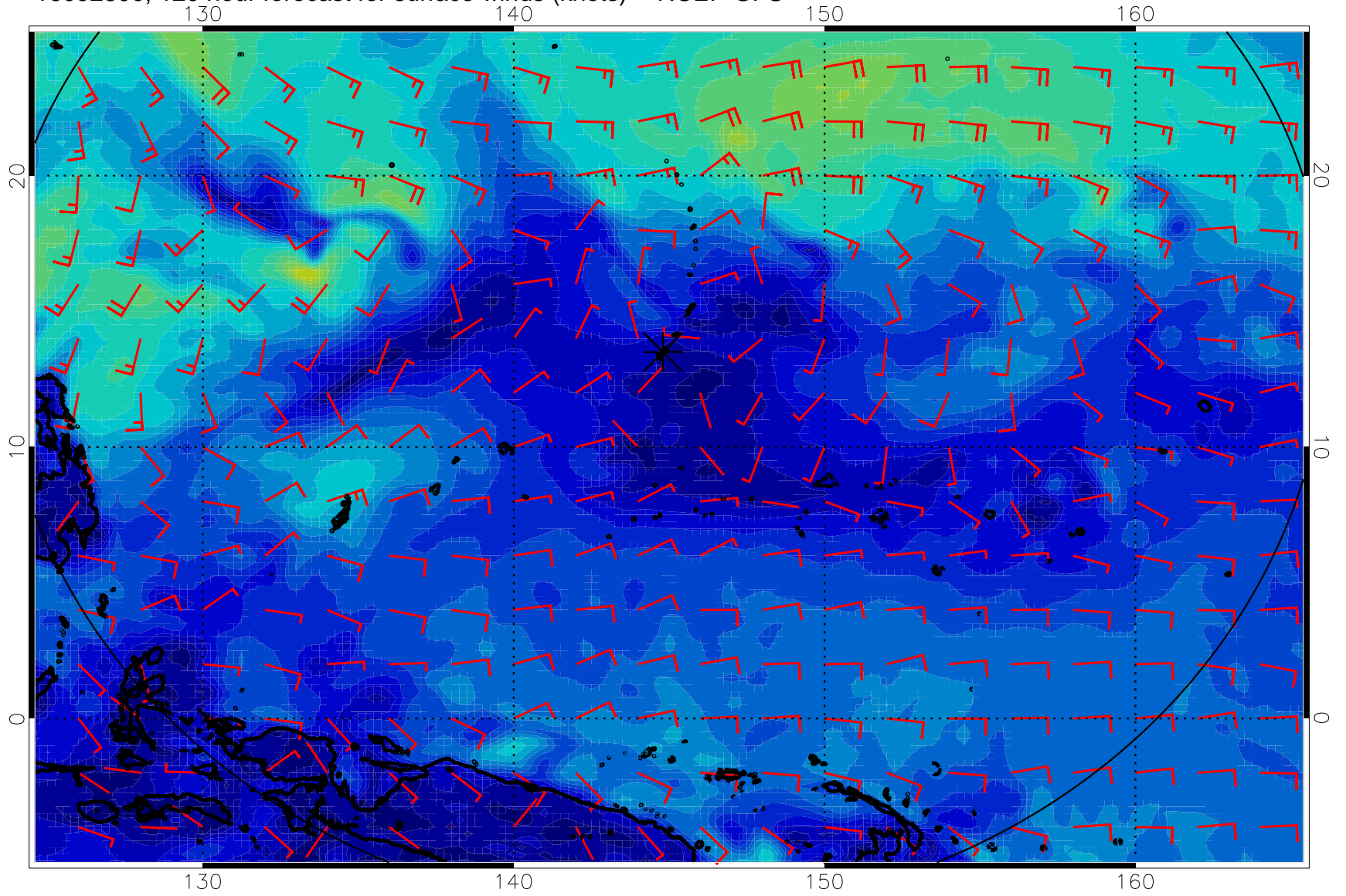
16092800, 120 hour forecast for surface winds (knots) -- NCEP GFS
