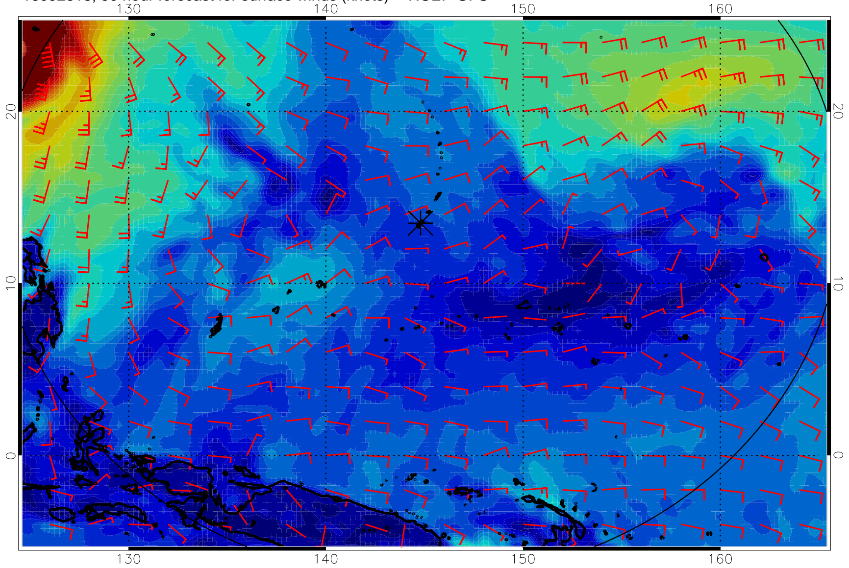
16092618, 90 hour forecast for surface winds (knots) -- NCEP GFS
