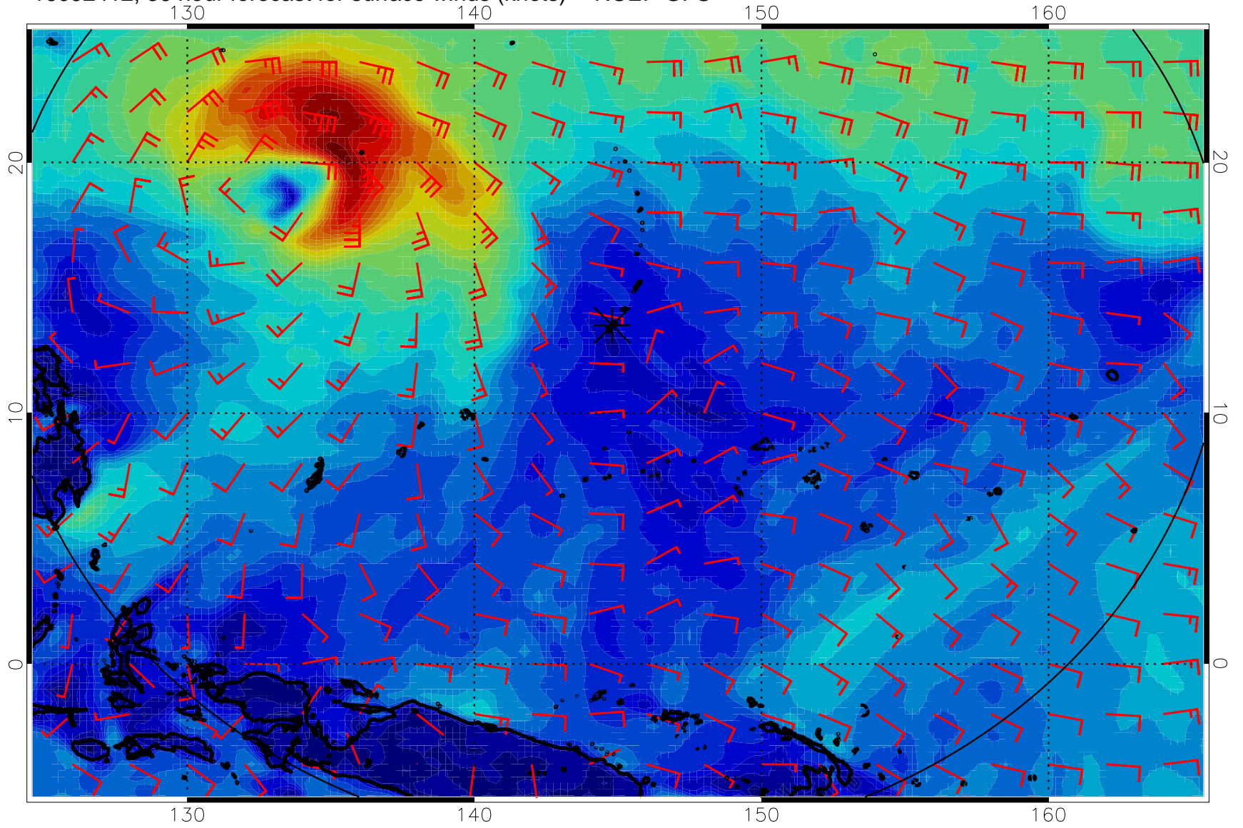
16092412, 36 hour forecast for surface winds (knots) -- NCEP GFS
