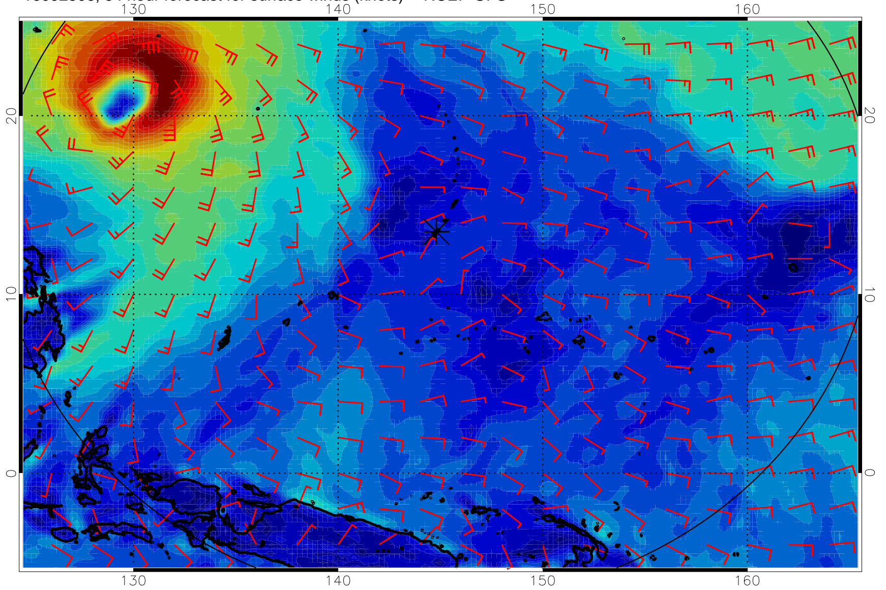
16092506, 54 hour forecast for surface winds (knots) -- NCEP GFS
