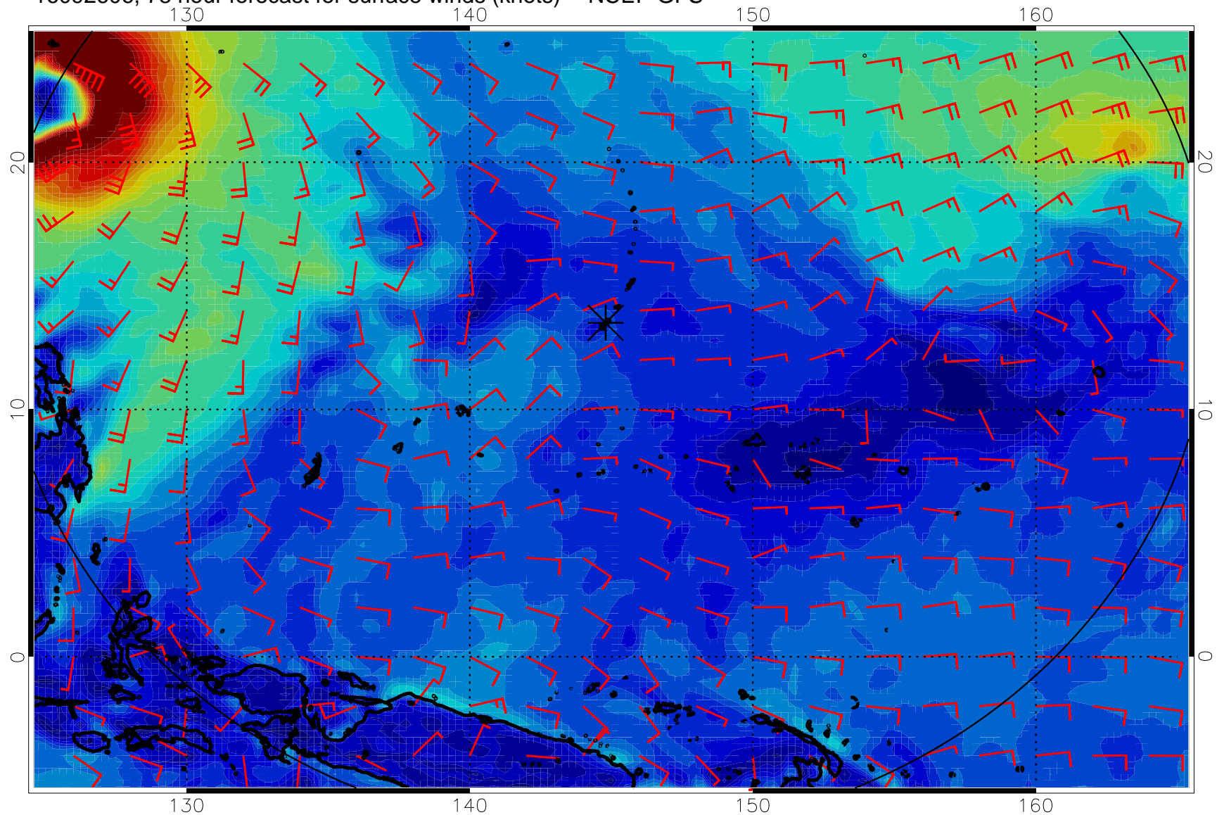
16092606, 78 hour forecast for surface winds (knots) -- NCEP GFS
