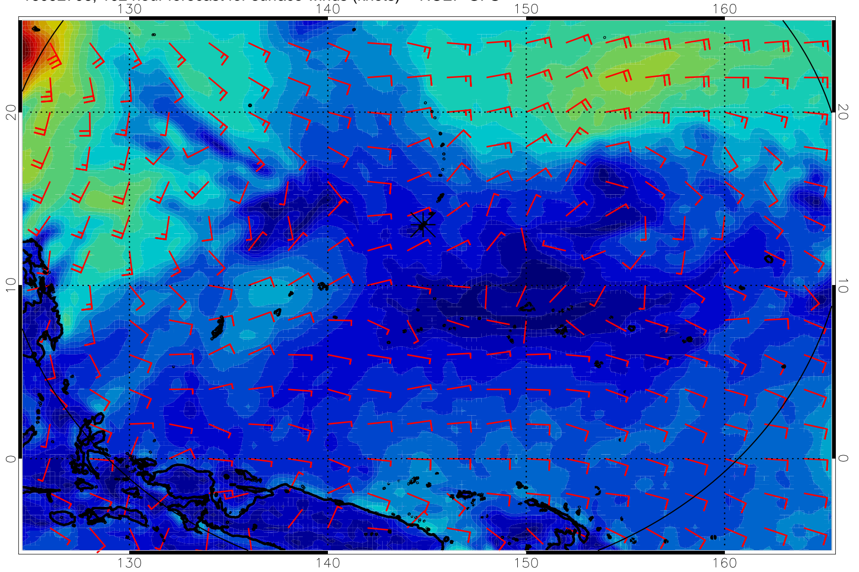
16092706, 102 hour forecast for surface winds (knots) -- NCEP GFS
