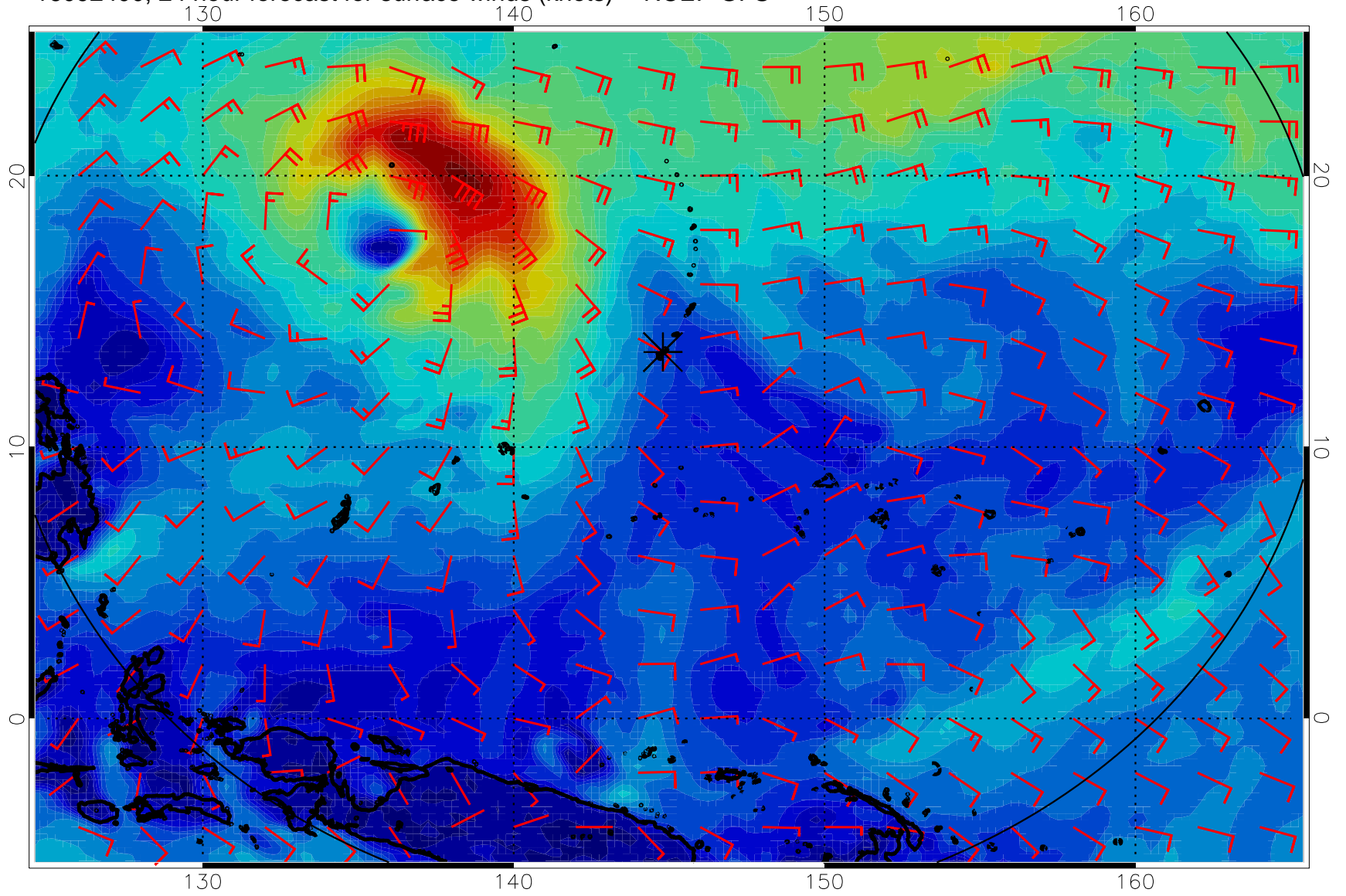
16092400, 24 hour forecast for surface winds (knots) -- NCEP GFS
