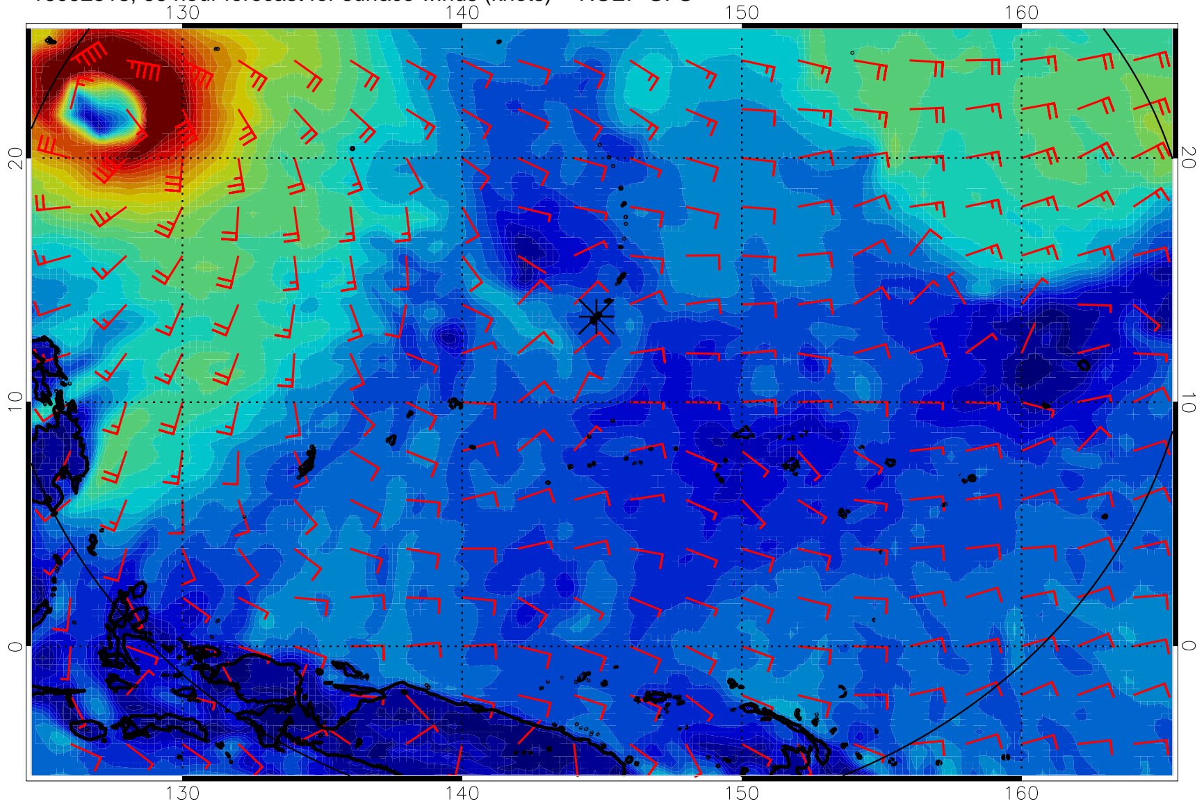
16092518, 66 hour forecast for surface winds (knots) -- NCEP GFS
