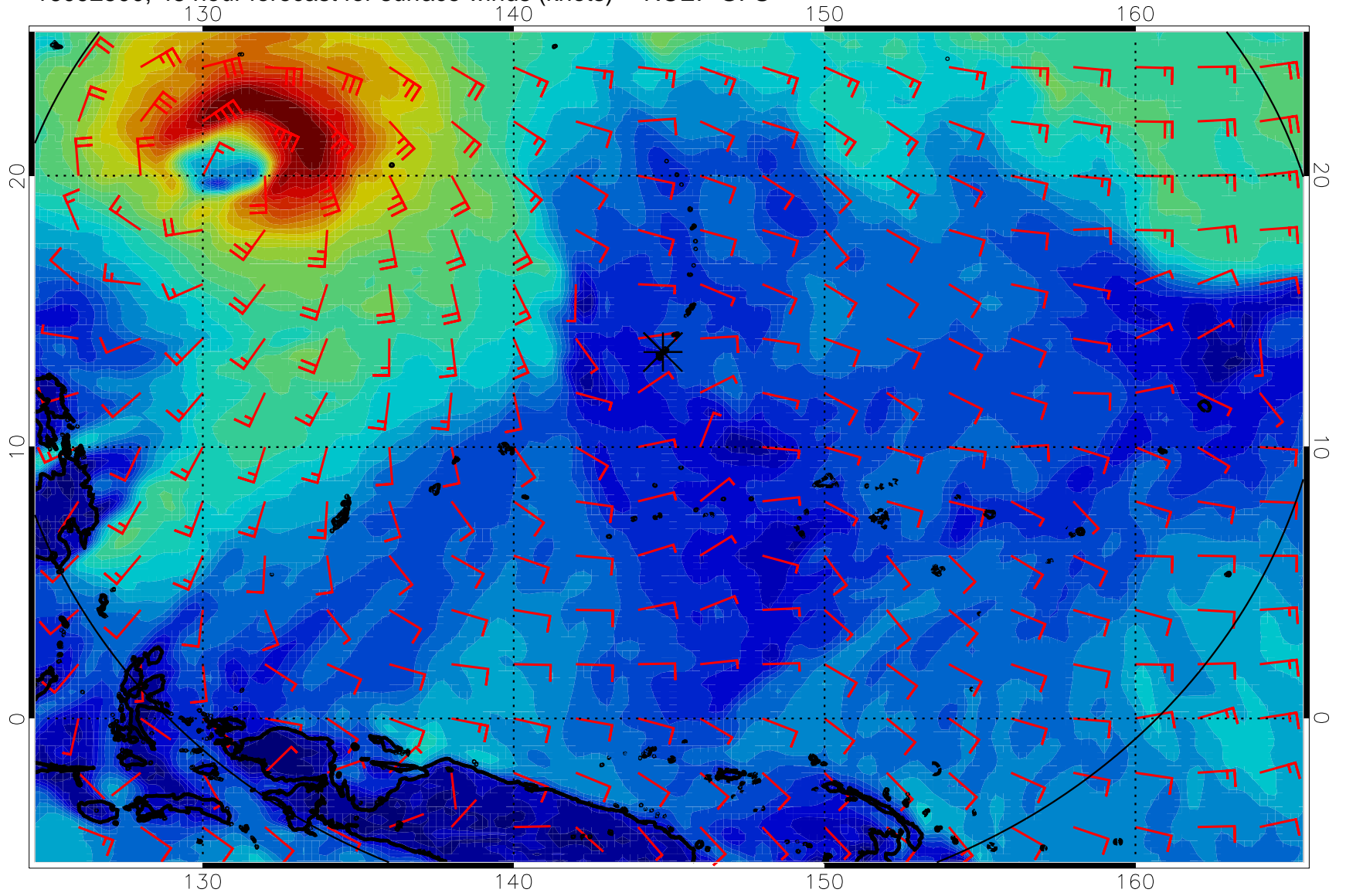
16092500, 48 hour forecast for surface winds (knots) -- NCEP GFS
