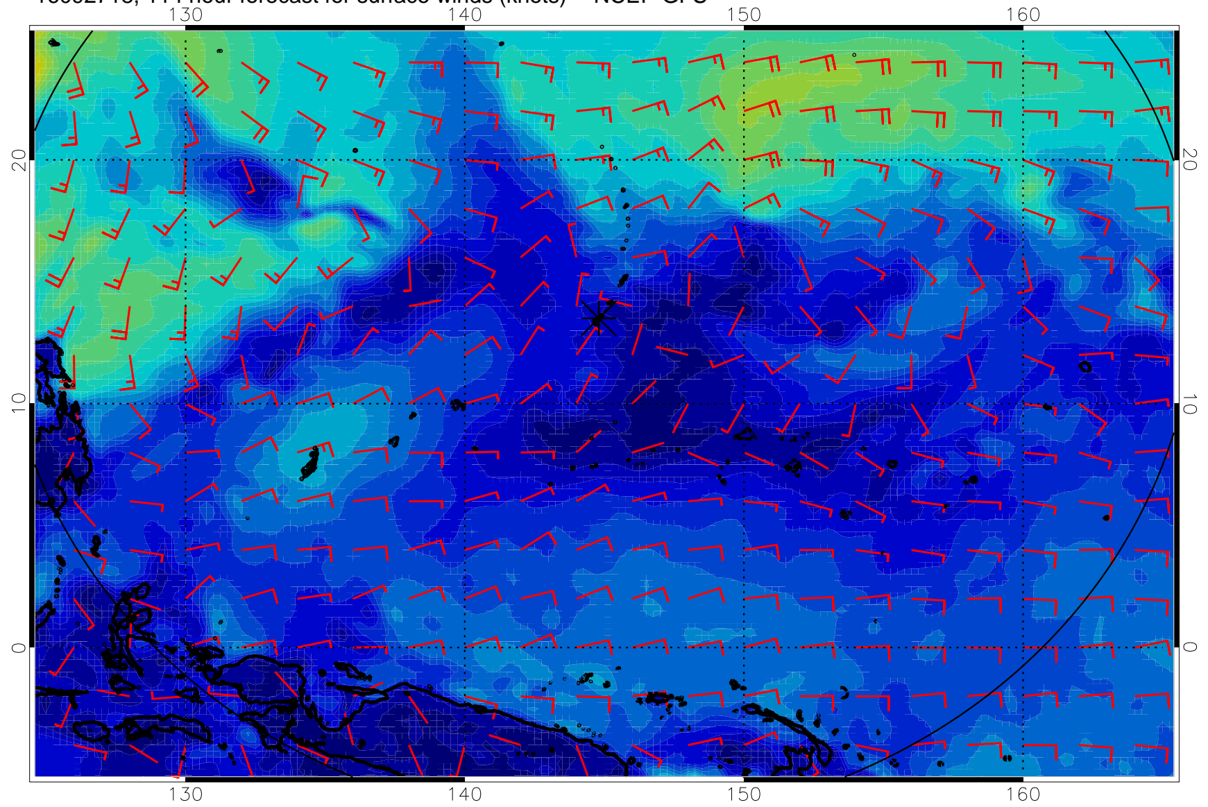
16092718, 114 hour forecast for surface winds (knots) -- NCEP GFS
