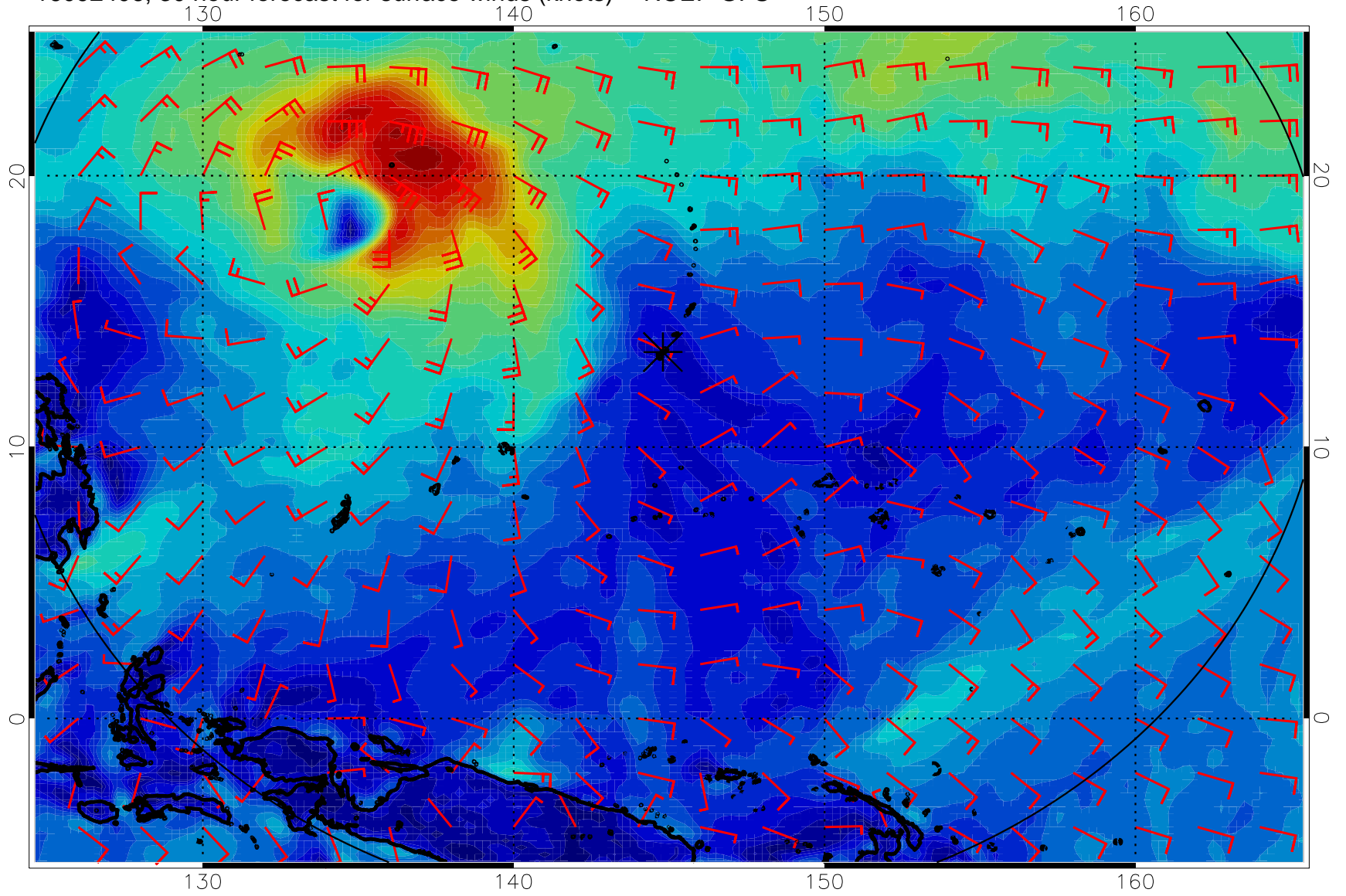
16092406, 30 hour forecast for surface winds (knots) -- NCEP GFS
