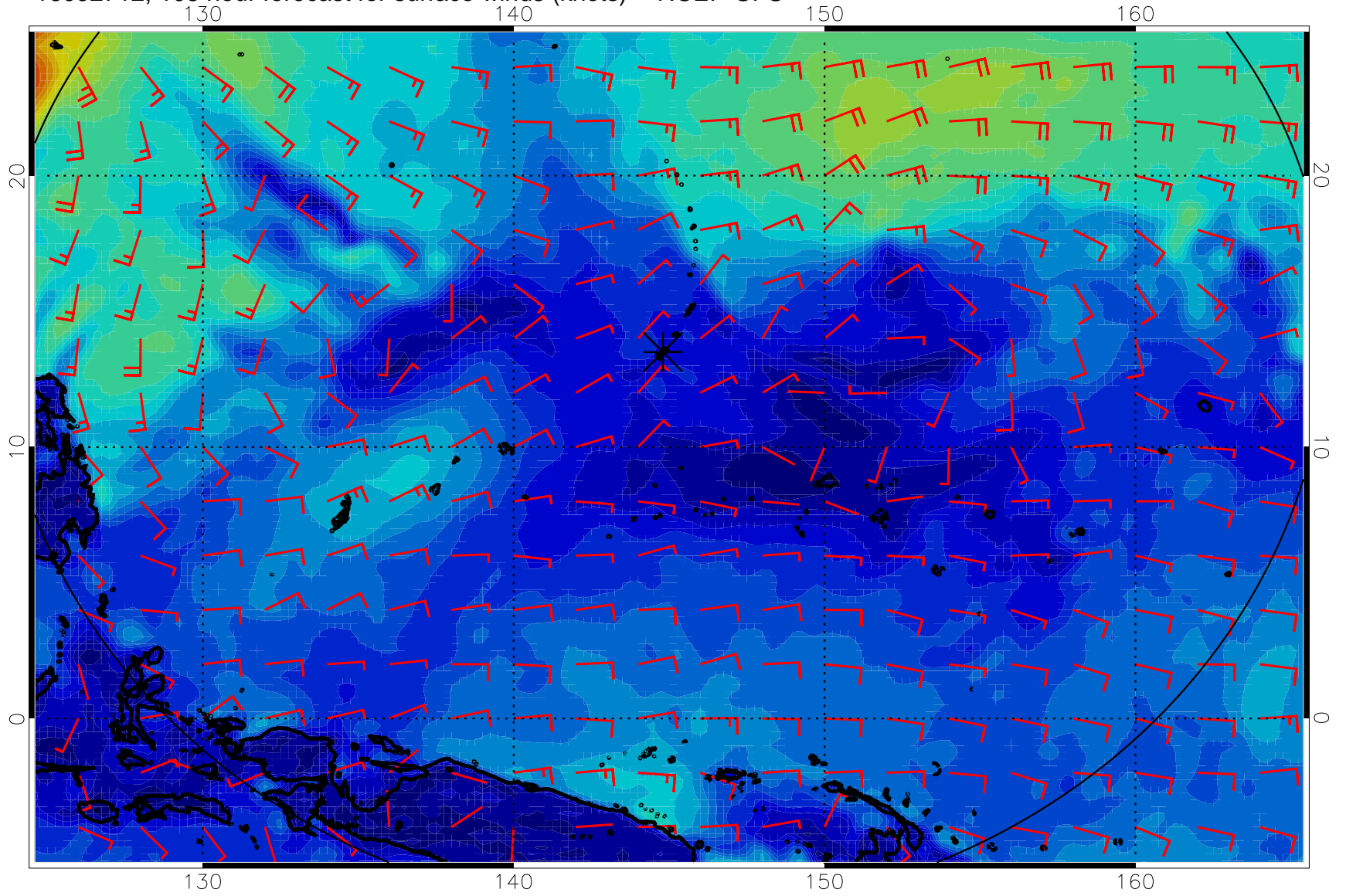
16092712, 108 hour forecast for surface winds (knots) -- NCEP GFS
