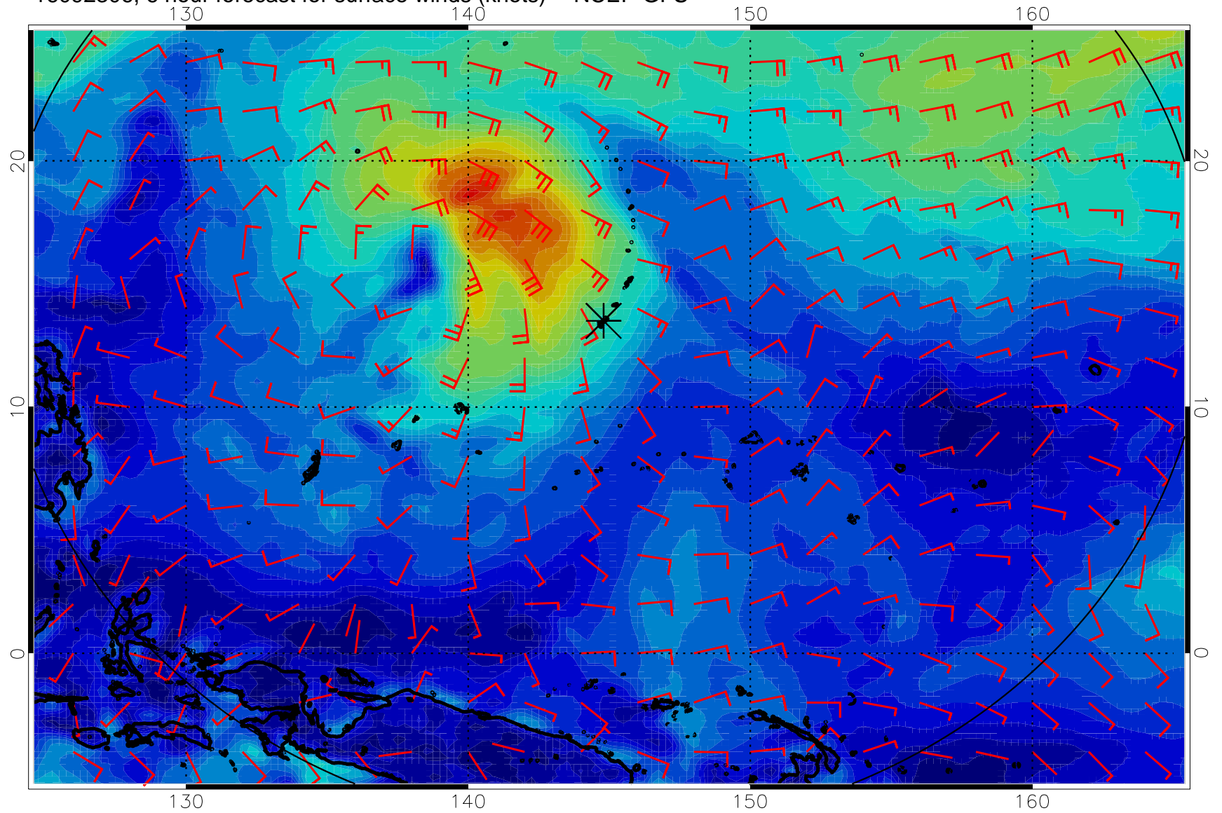
16092306, 6 hour forecast for surface winds (knots) -- NCEP GFS
