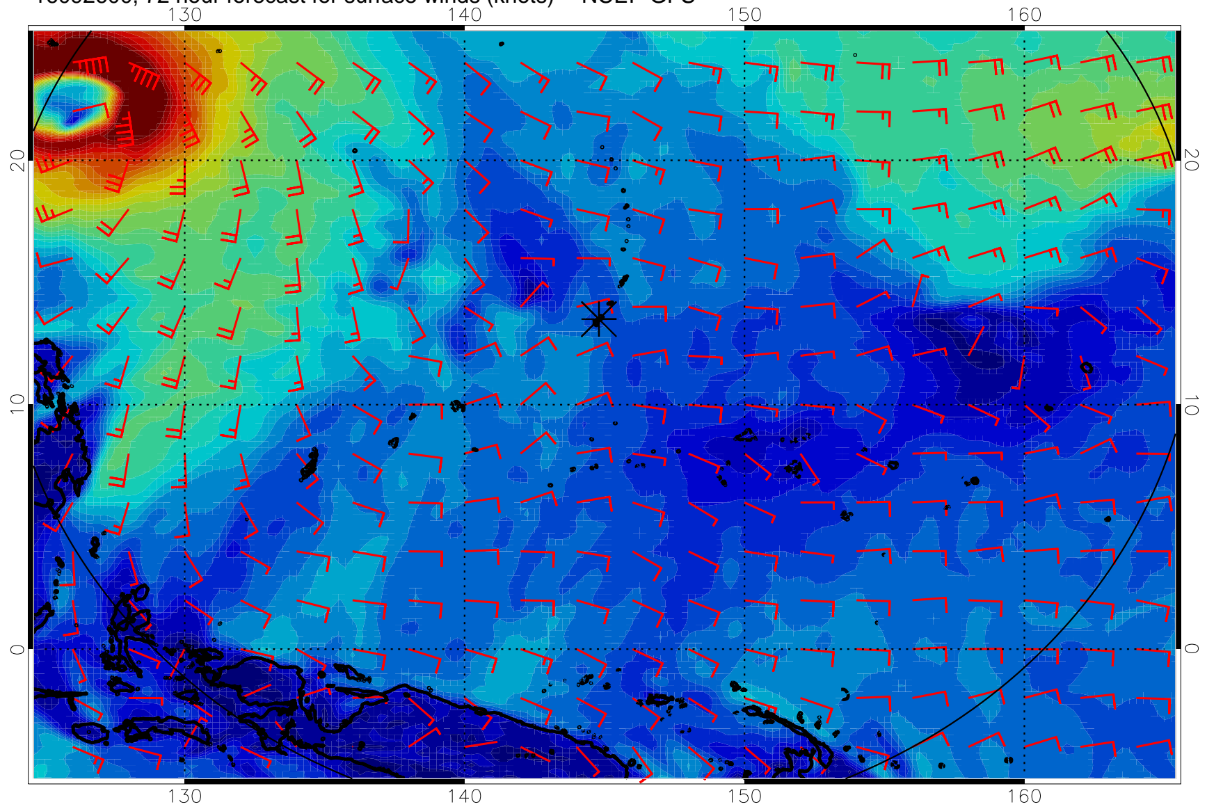
16092600, 72 hour forecast for surface winds (knots) -- NCEP GFS
