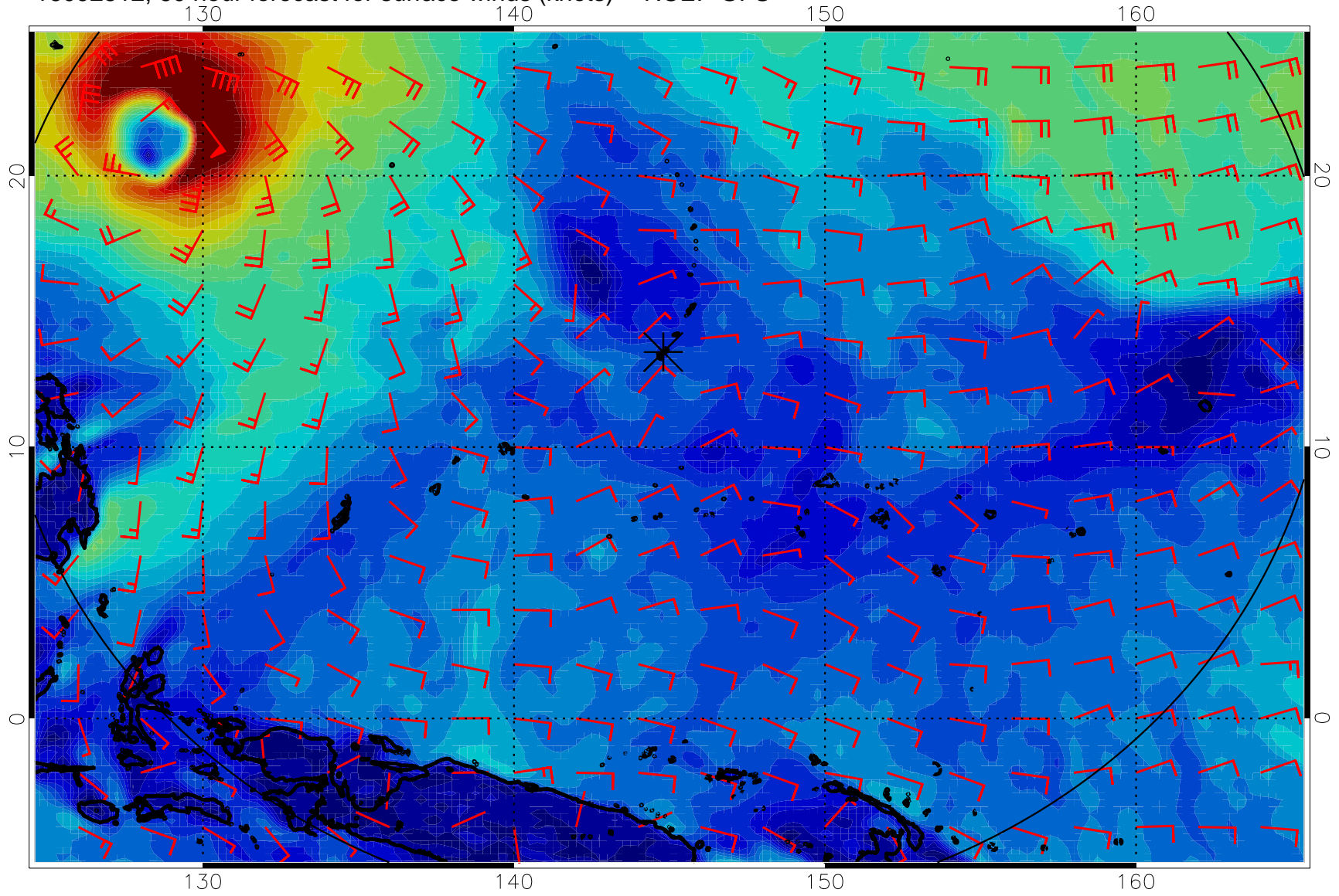
16092512, 60 hour forecast for surface winds (knots) -- NCEP GFS
