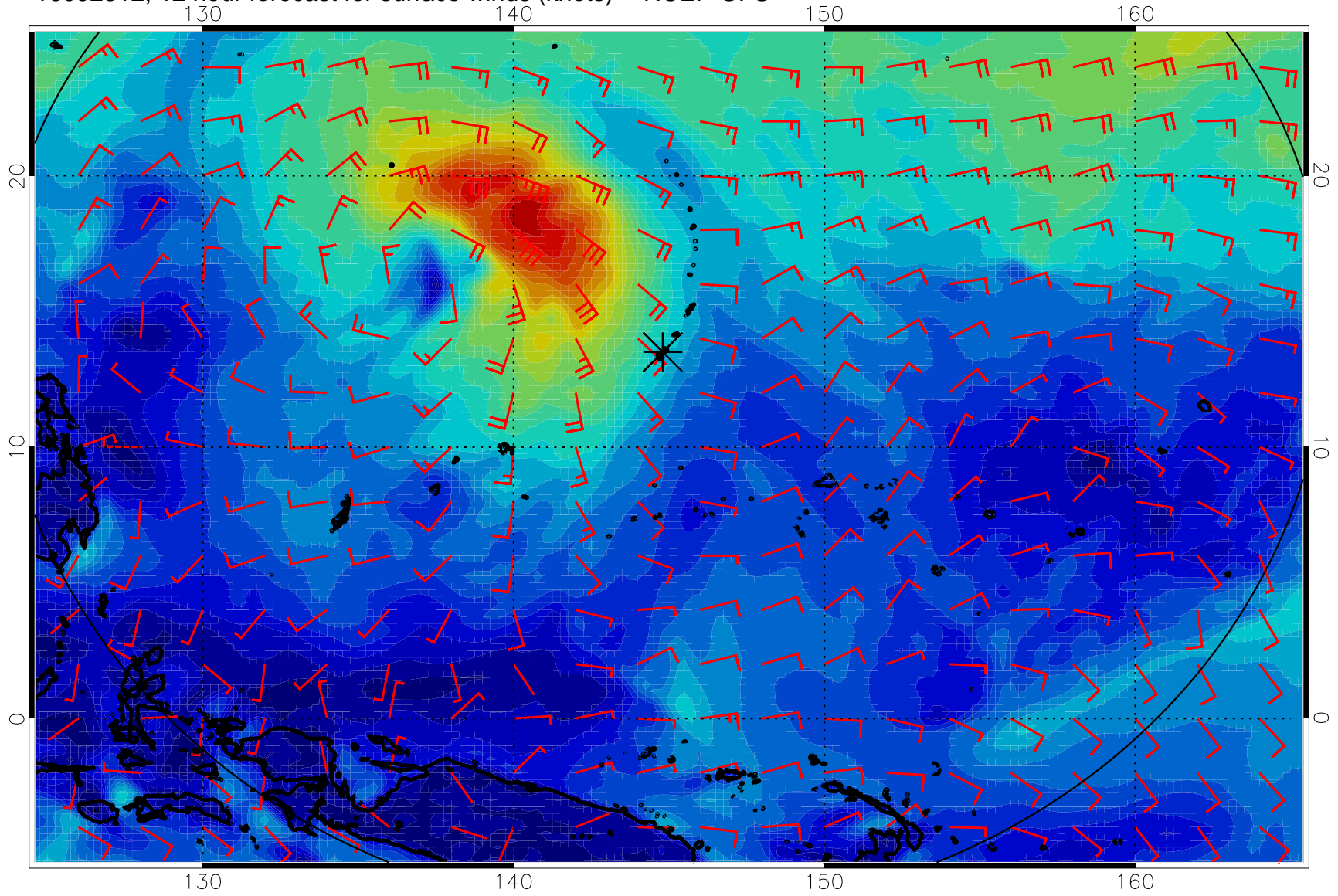
16092312, 12 hour forecast for surface winds (knots) -- NCEP GFS
