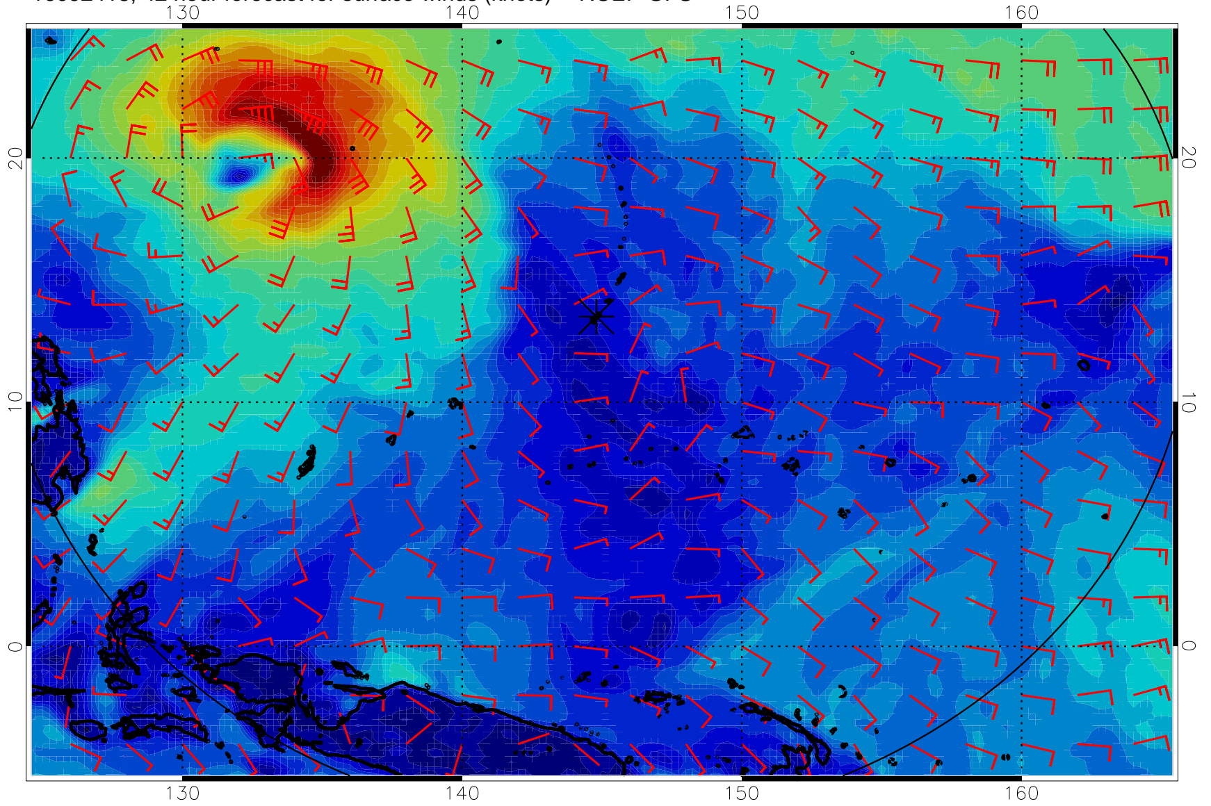
16092418, 42 hour forecast for surface winds (knots) -- NCEP GFS
