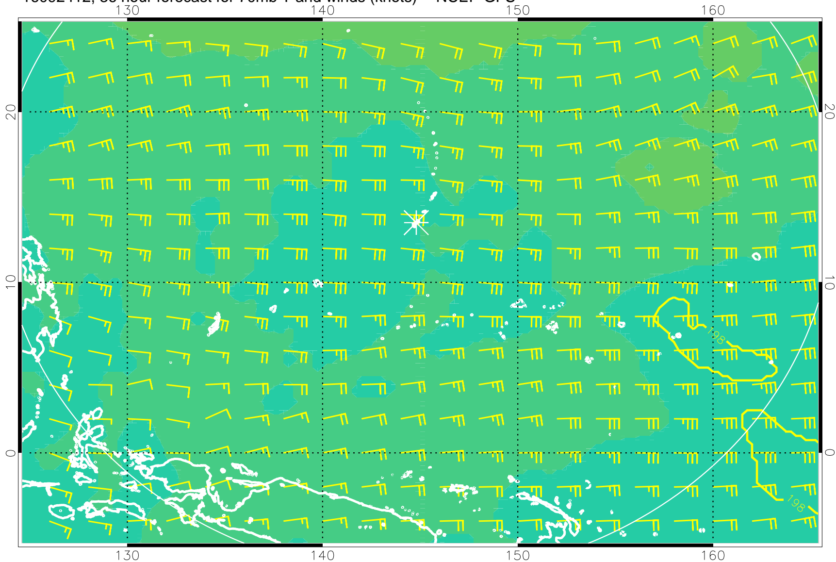
16092412, 36 hour forecast for 70mb T and winds (knots) -- NCEP GFS
