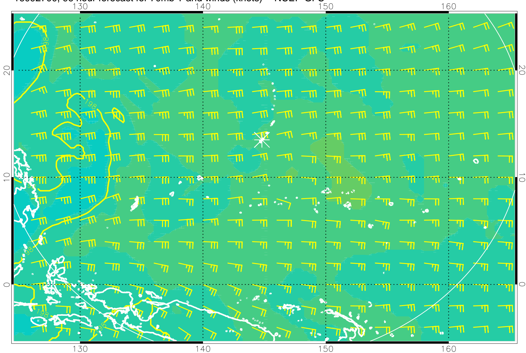
16092700, 96 hour forecast for 70mb T and winds (knots) -- NCEP GFS
