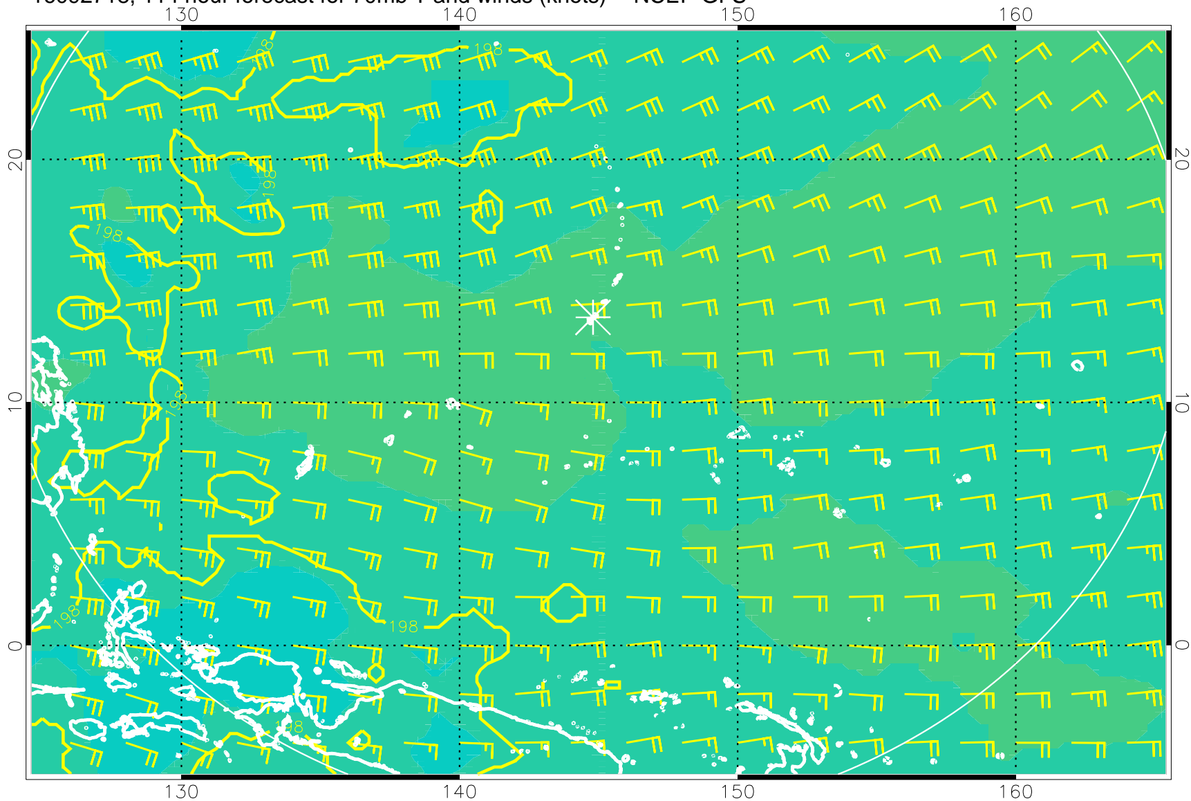
16092718, 114 hour forecast for 70mb T and winds (knots) -- NCEP GFS
