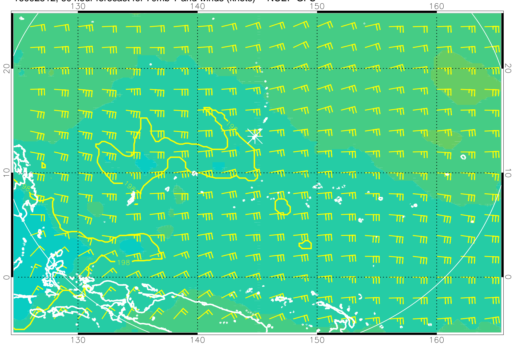
16092512, 60 hour forecast for 70mb T and winds (knots) -- NCEP GFS
