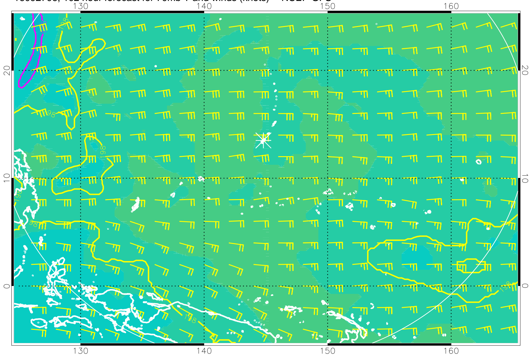
16092706, 102 hour forecast for 70mb T and winds (knots) -- NCEP GFS
