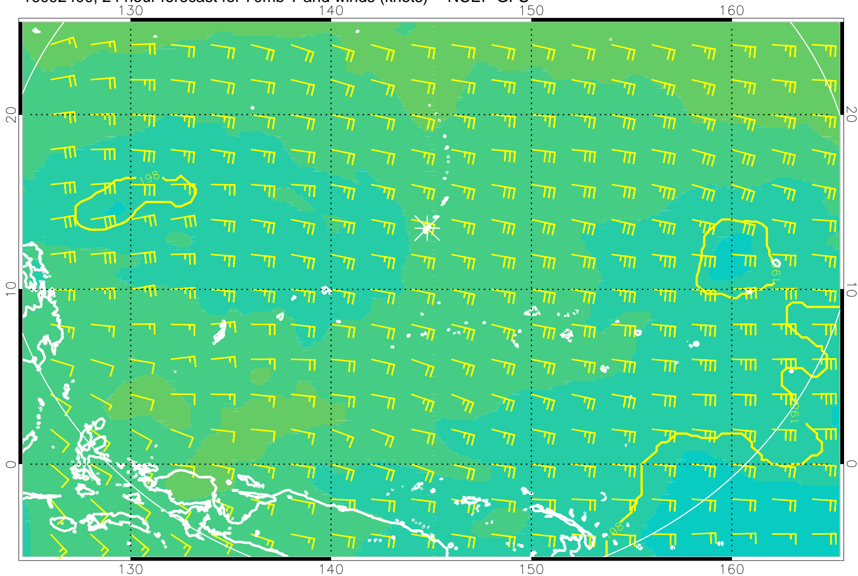
16092400, 24 hour forecast for 70mb T and winds (knots) -- NCEP GFS
