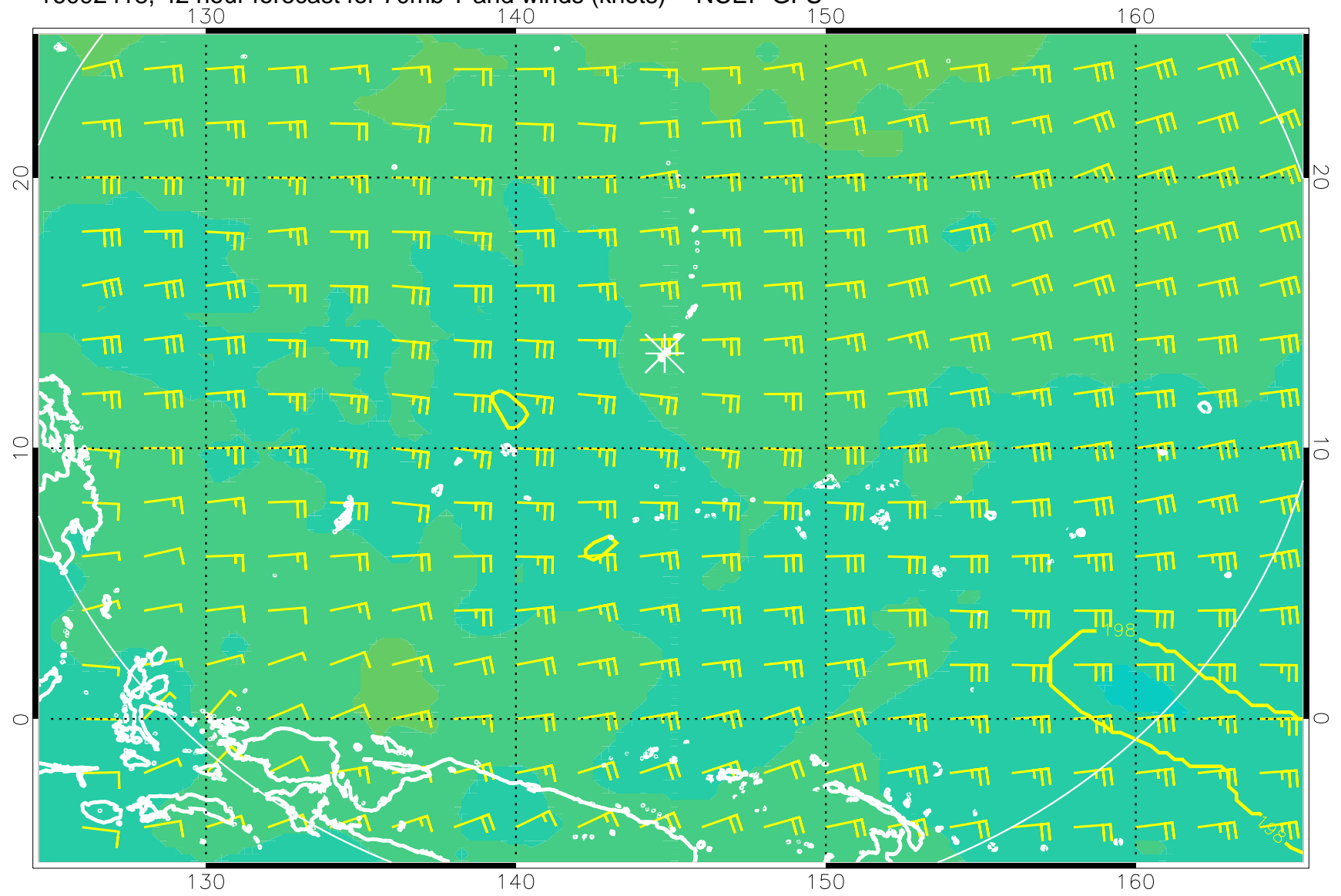
16092418, 42 hour forecast for 70mb T and winds (knots) -- NCEP GFS
