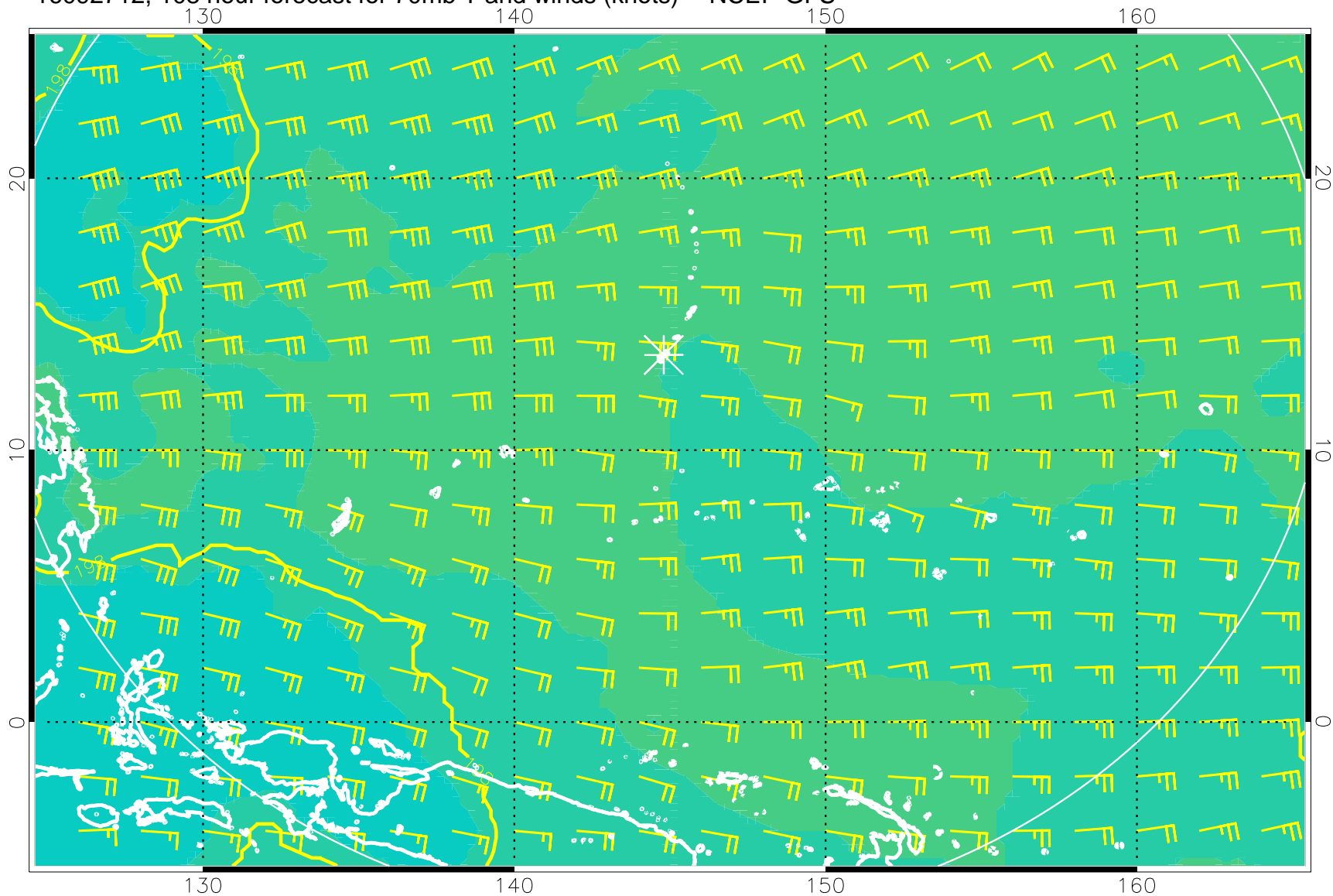
16092712, 108 hour forecast for 70mb T and winds (knots) -- NCEP GFS
