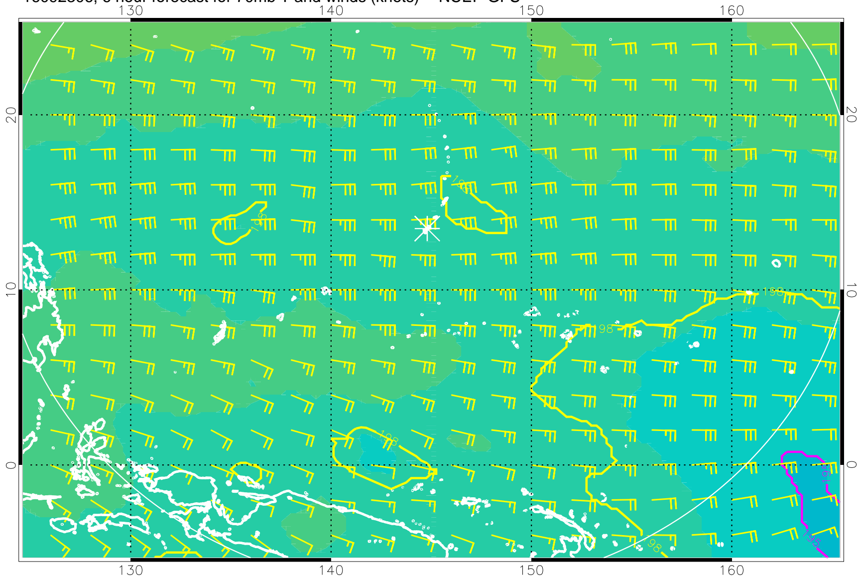
16092306, 6 hour forecast for 70mb T and winds (knots) -- NCEP GFS
