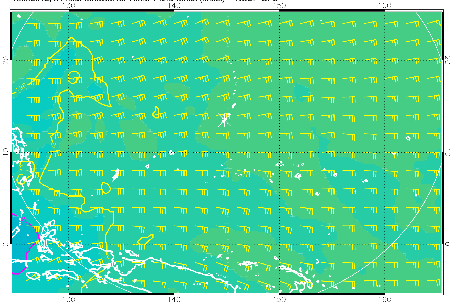
16092612, 84 hour forecast for 70mb T and winds (knots) -- NCEP GFS
