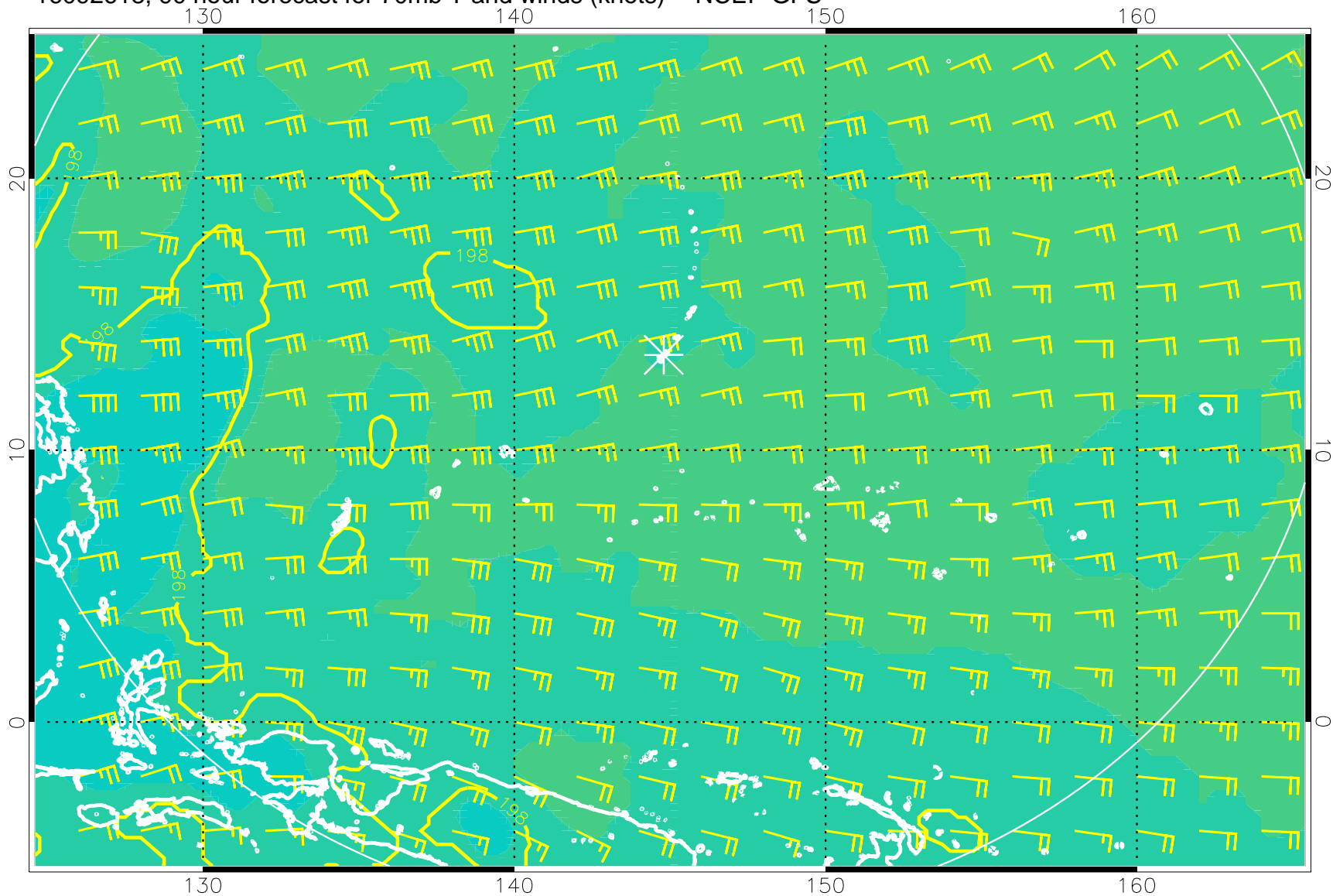
16092618, 90 hour forecast for 70mb T and winds (knots) -- NCEP GFS
