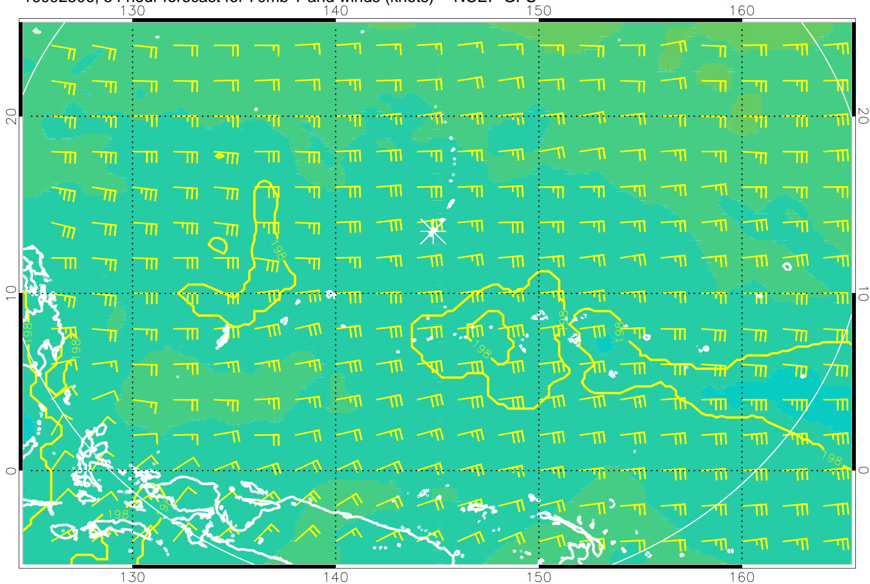
16092506, 54 hour forecast for 70mb T and winds (knots) -- NCEP GFS
