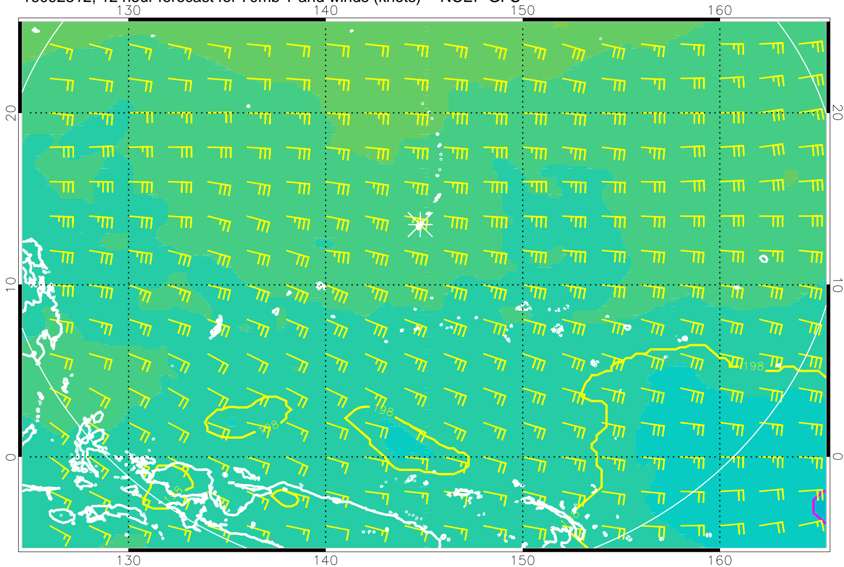
16092312, 12 hour forecast for 70mb T and winds (knots) -- NCEP GFS
