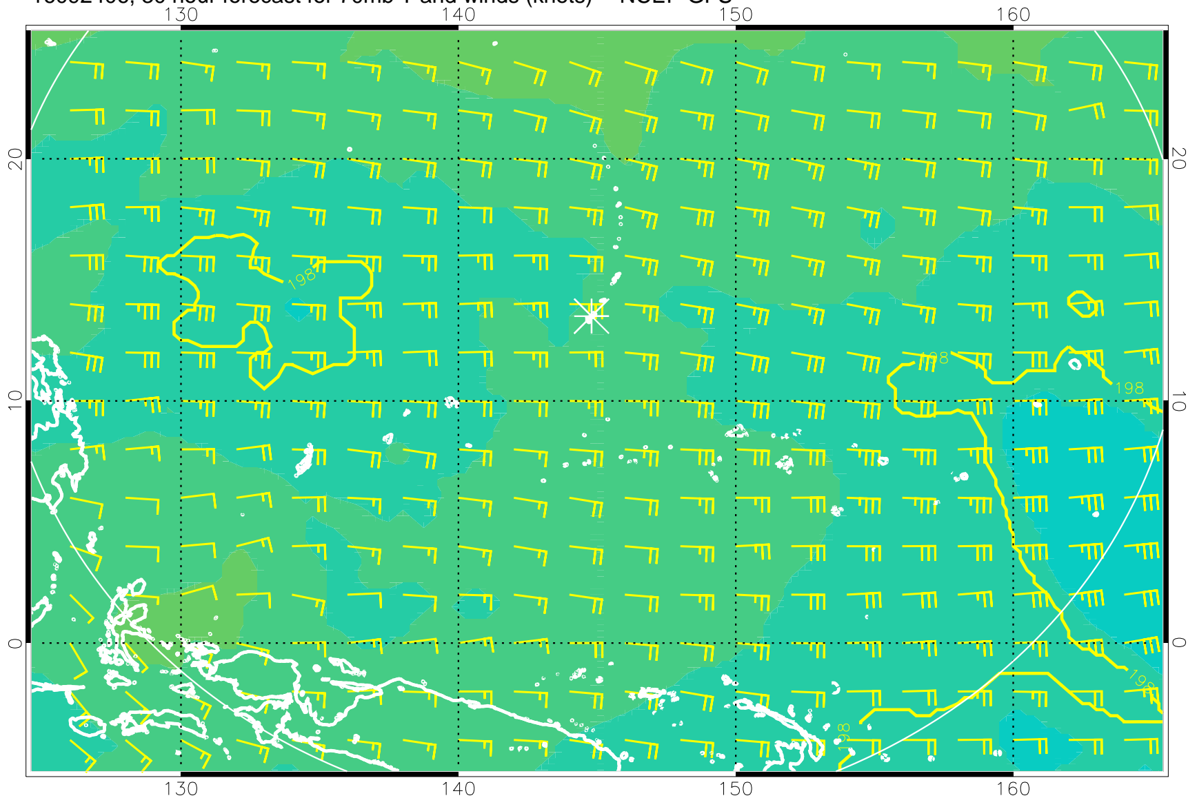
16092406, 30 hour forecast for 70mb T and winds (knots) -- NCEP GFS
