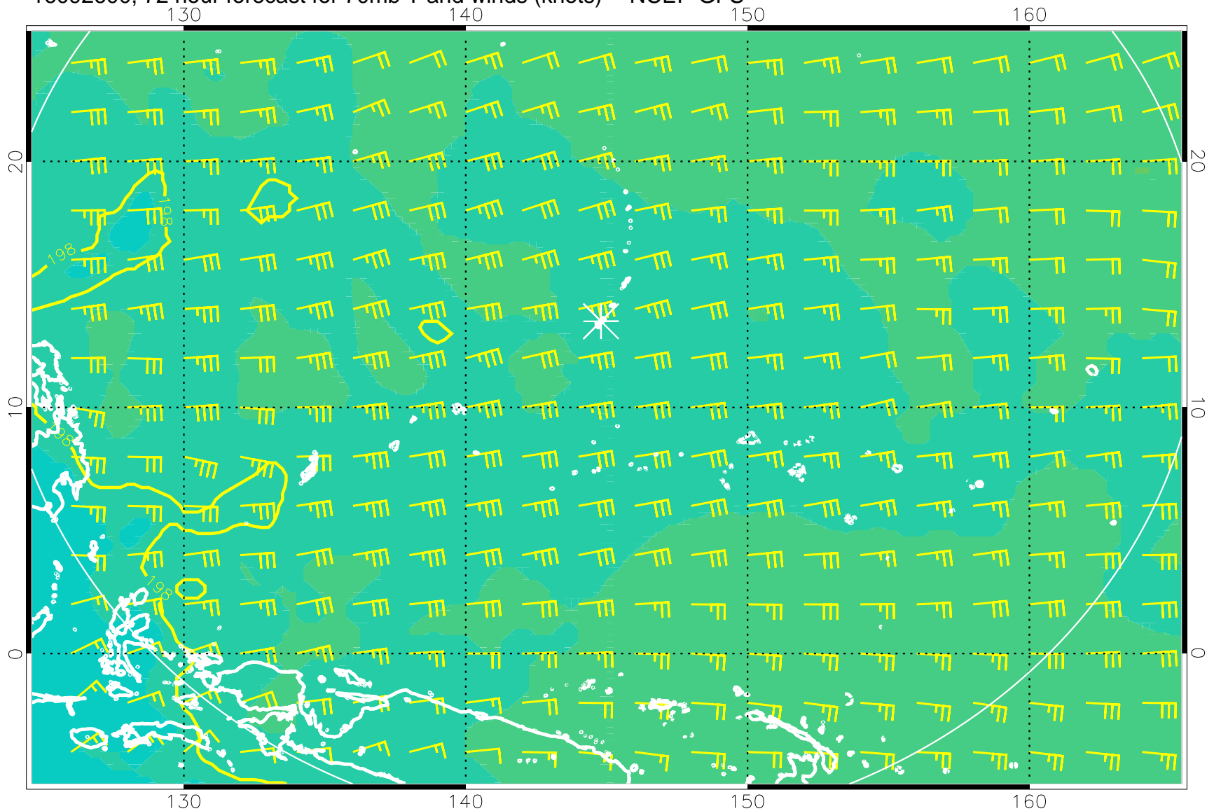
16092600, 72 hour forecast for 70mb T and winds (knots) -- NCEP GFS
