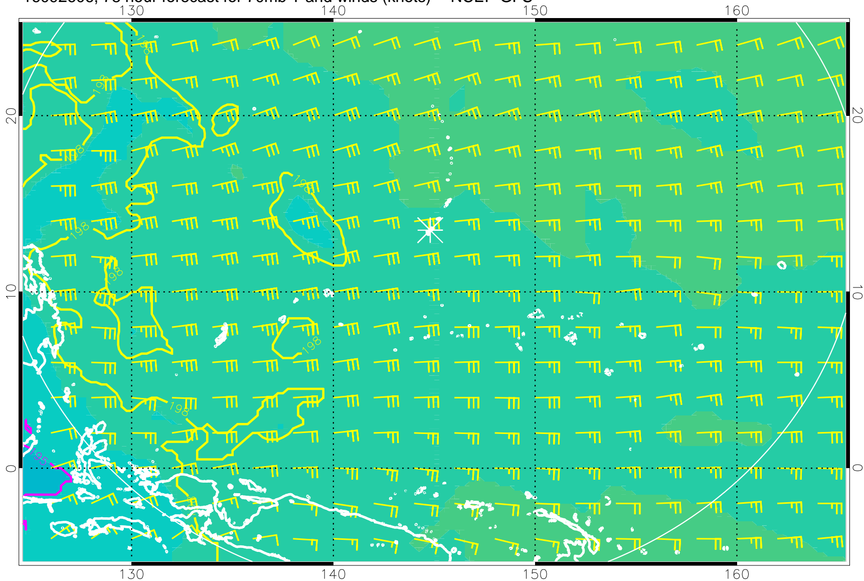
16092606, 78 hour forecast for 70mb T and winds (knots) -- NCEP GFS
