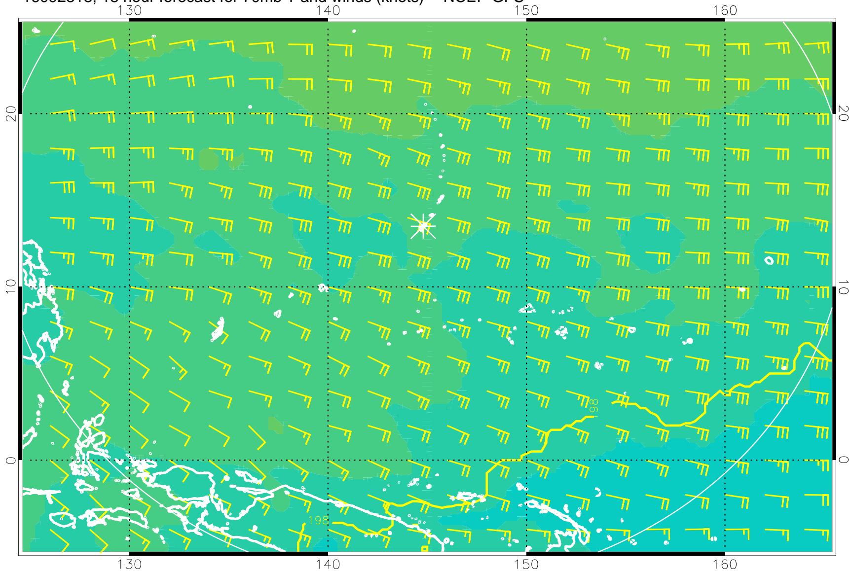
16092318, 18 hour forecast for 70mb T and winds (knots) -- NCEP GFS
