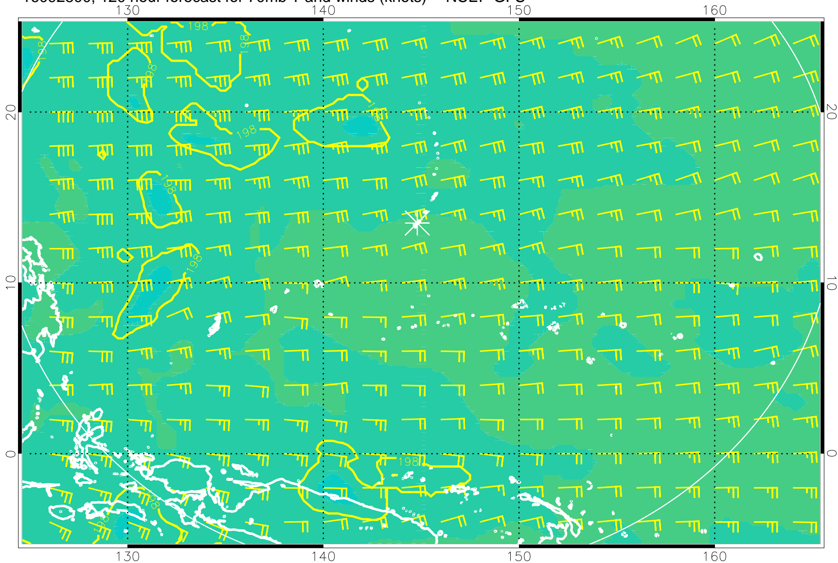
16092800, 120 hour forecast for 70mb T and winds (knots) -- NCEP GFS
