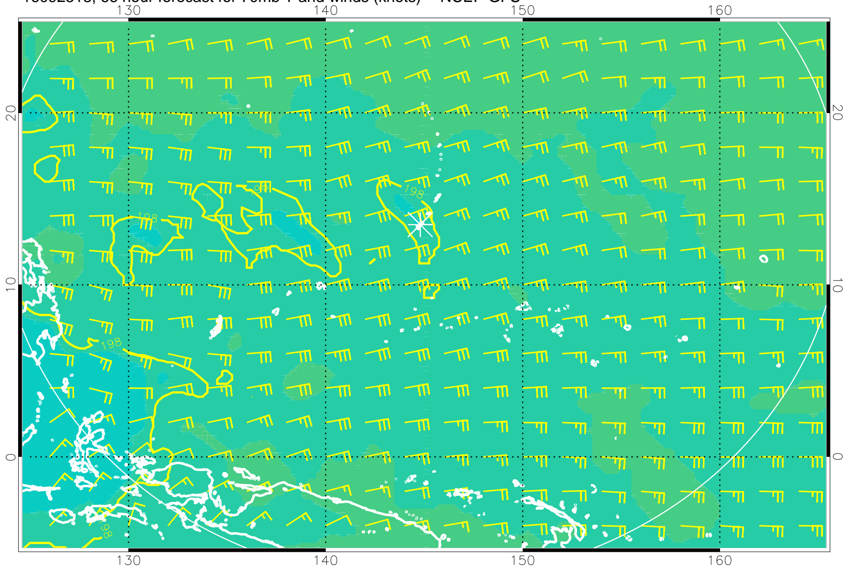
16092518, 66 hour forecast for 70mb T and winds (knots) -- NCEP GFS
