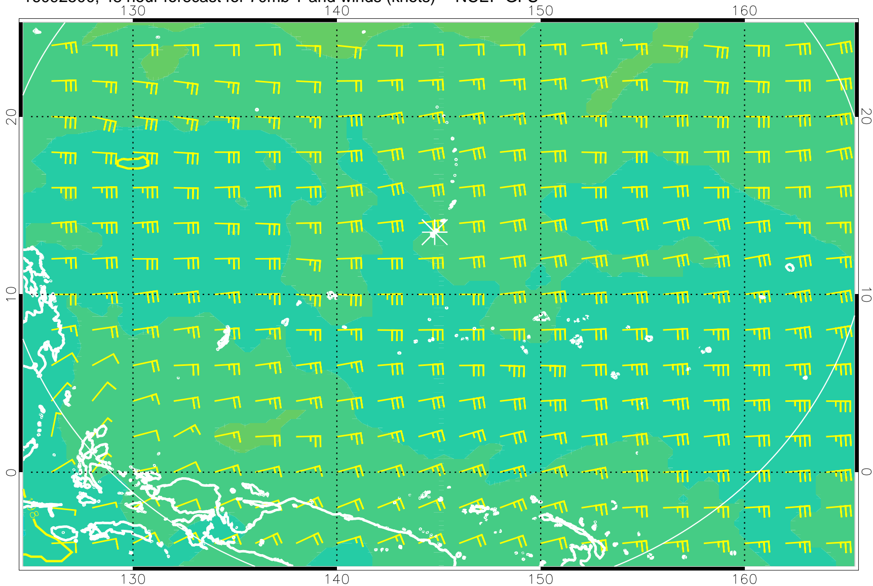
16092500, 48 hour forecast for 70mb T and winds (knots) -- NCEP GFS
