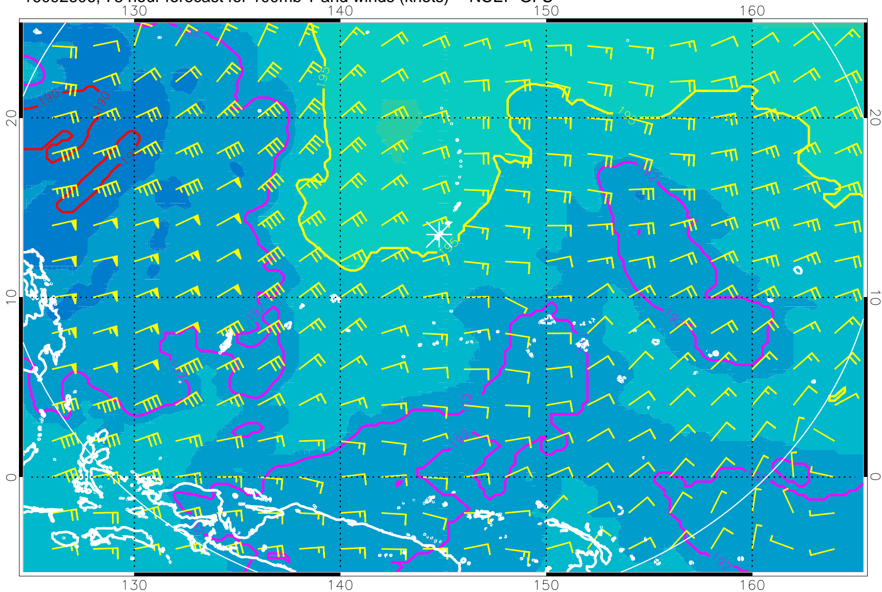
16092606, 78 hour forecast for 100mb T and winds (knots) -- NCEP GFS
