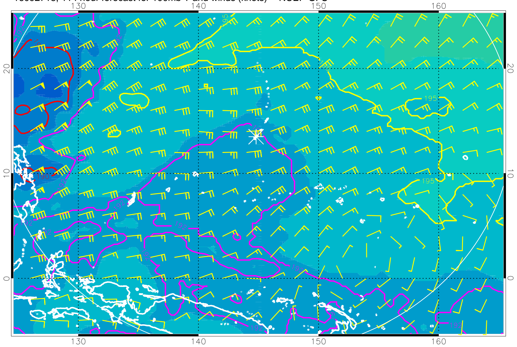
16092718, 114 hour forecast for 100mb T and winds (knots) -- NCEP GFS
