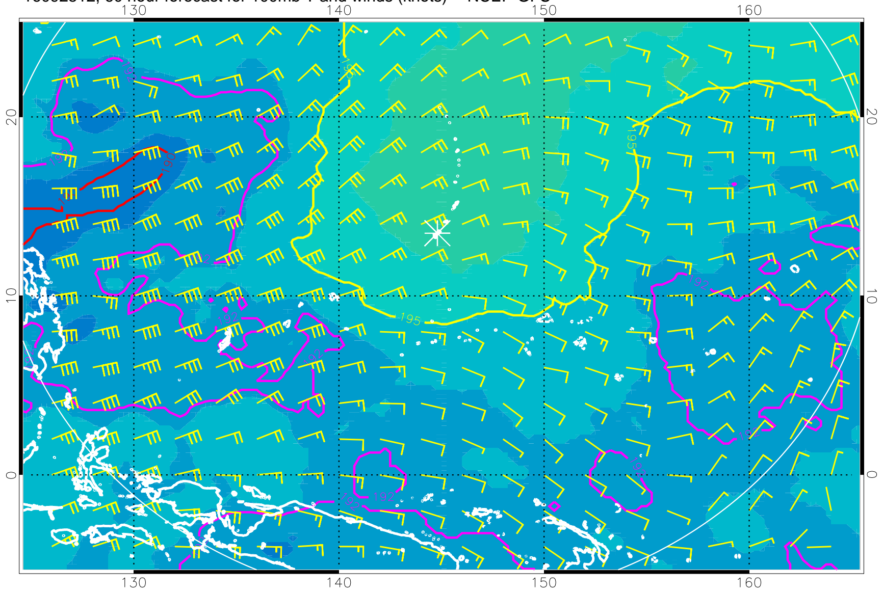
16092512, 60 hour forecast for 100mb T and winds (knots) -- NCEP GFS
