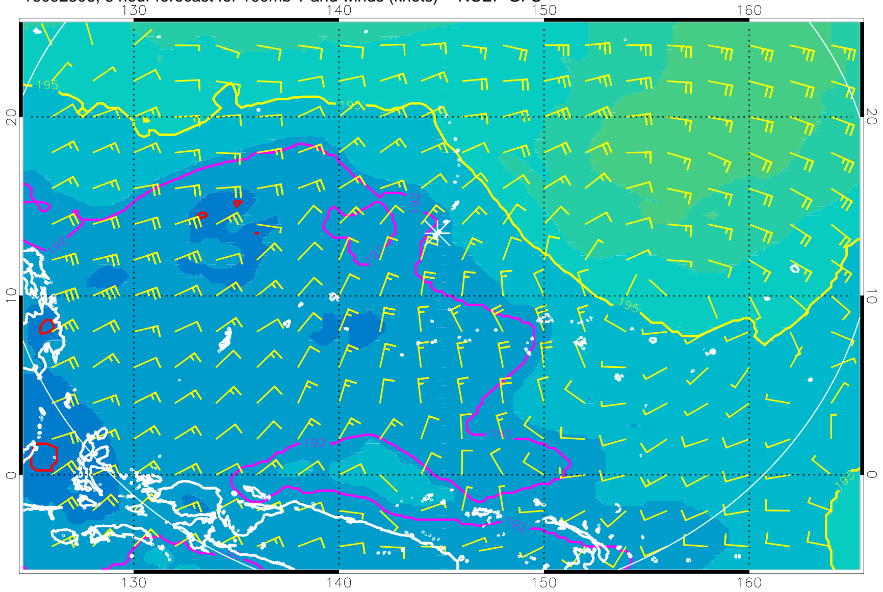
16092306, 6 hour forecast for 100mb T and winds (knots) -- NCEP GFS
