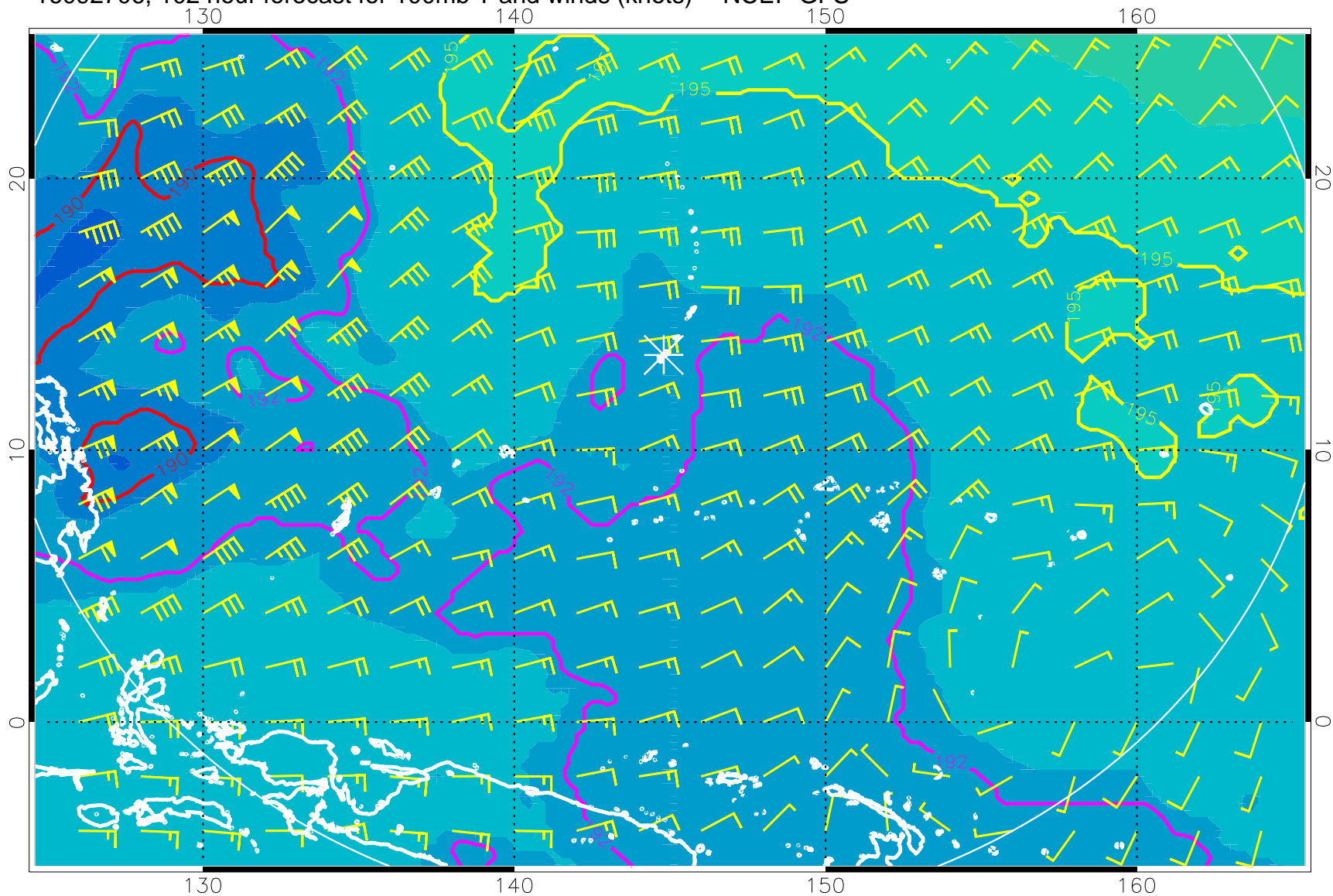
16092706, 102 hour forecast for 100mb T and winds (knots) -- NCEP GFS
