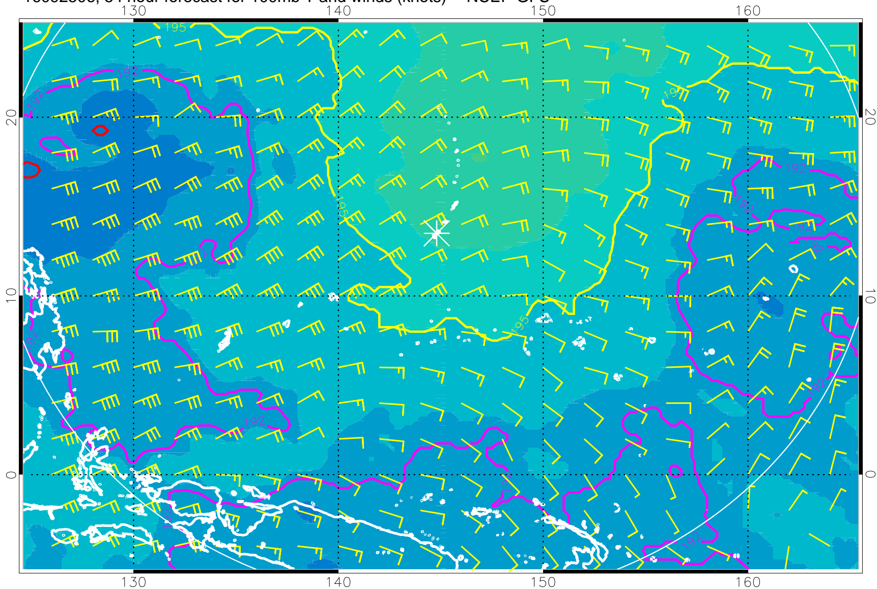
16092506, 54 hour forecast for 100mb T and winds (knots) -- NCEP GFS
