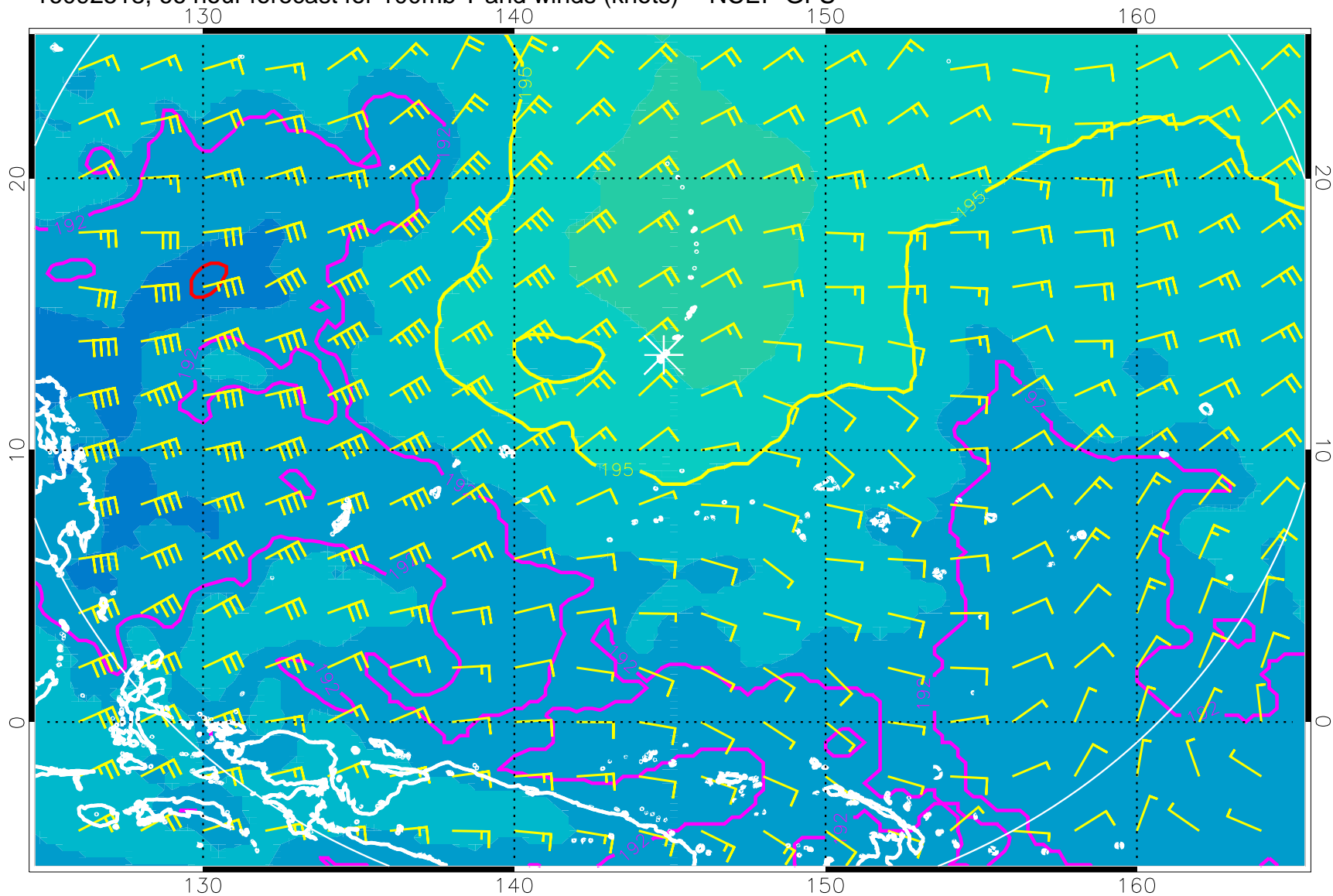
16092518, 66 hour forecast for 100mb T and winds (knots) -- NCEP GFS
