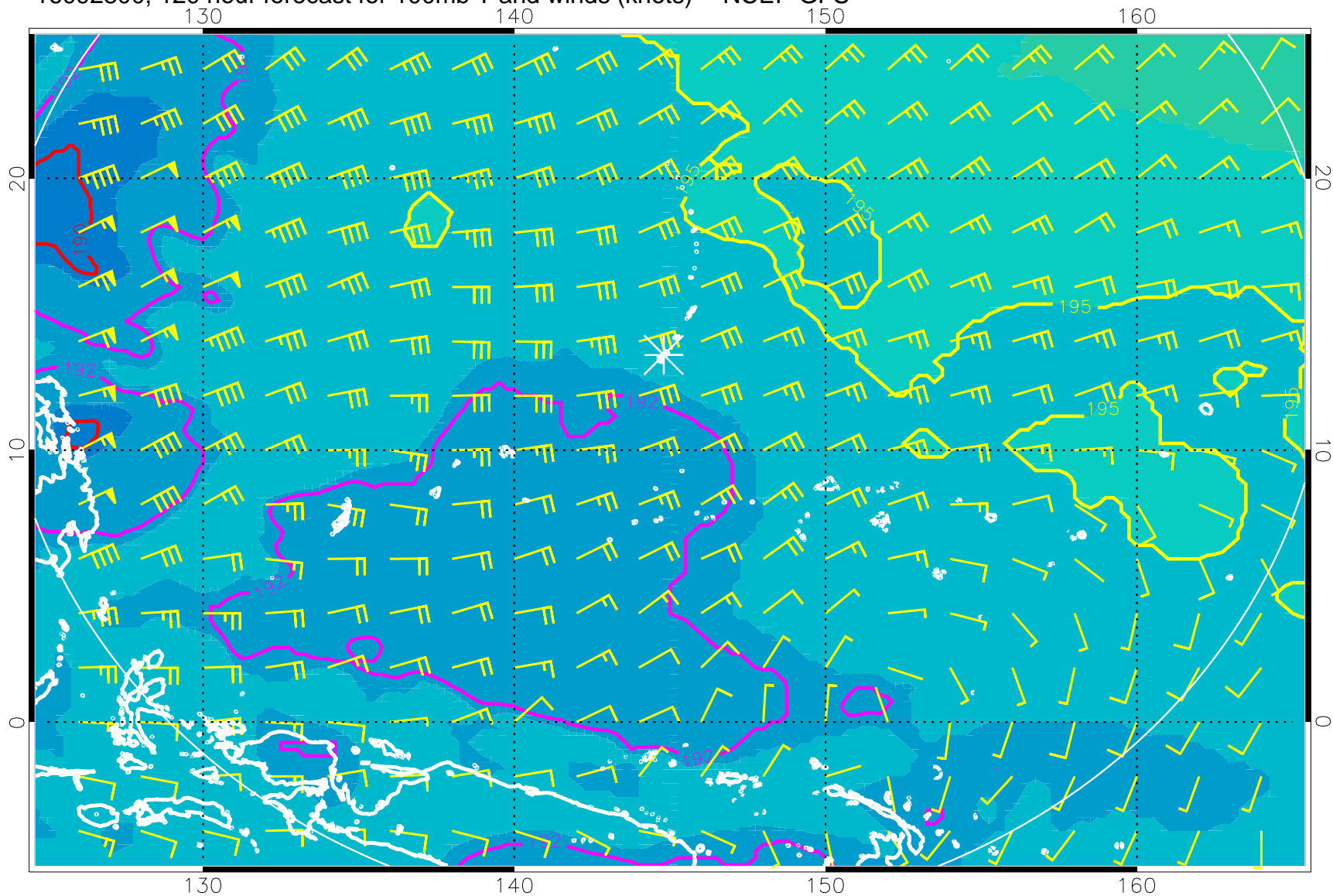
16092800, 120 hour forecast for 100mb T and winds (knots) -- NCEP GFS
