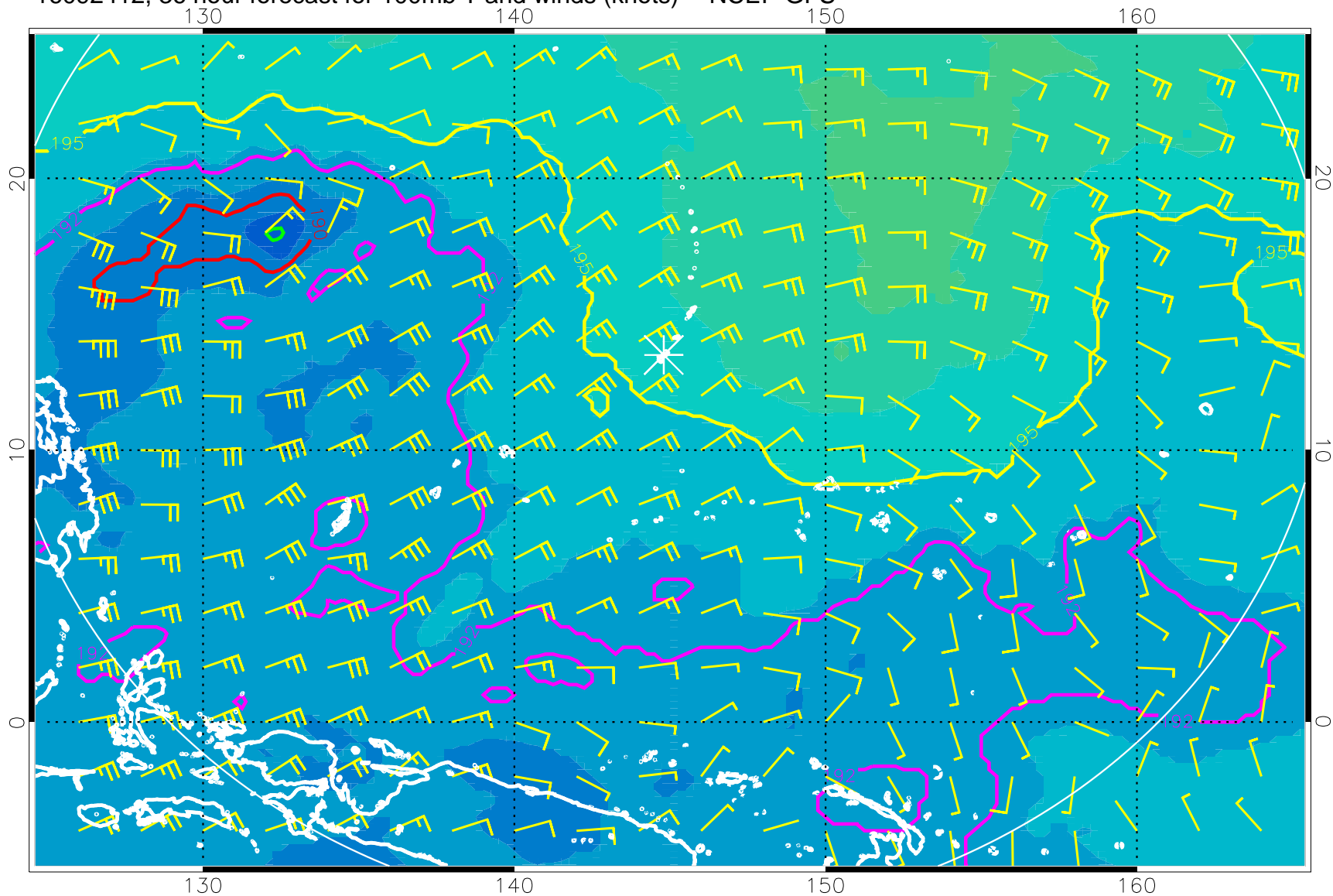
16092412, 36 hour forecast for 100mb T and winds (knots) -- NCEP GFS
