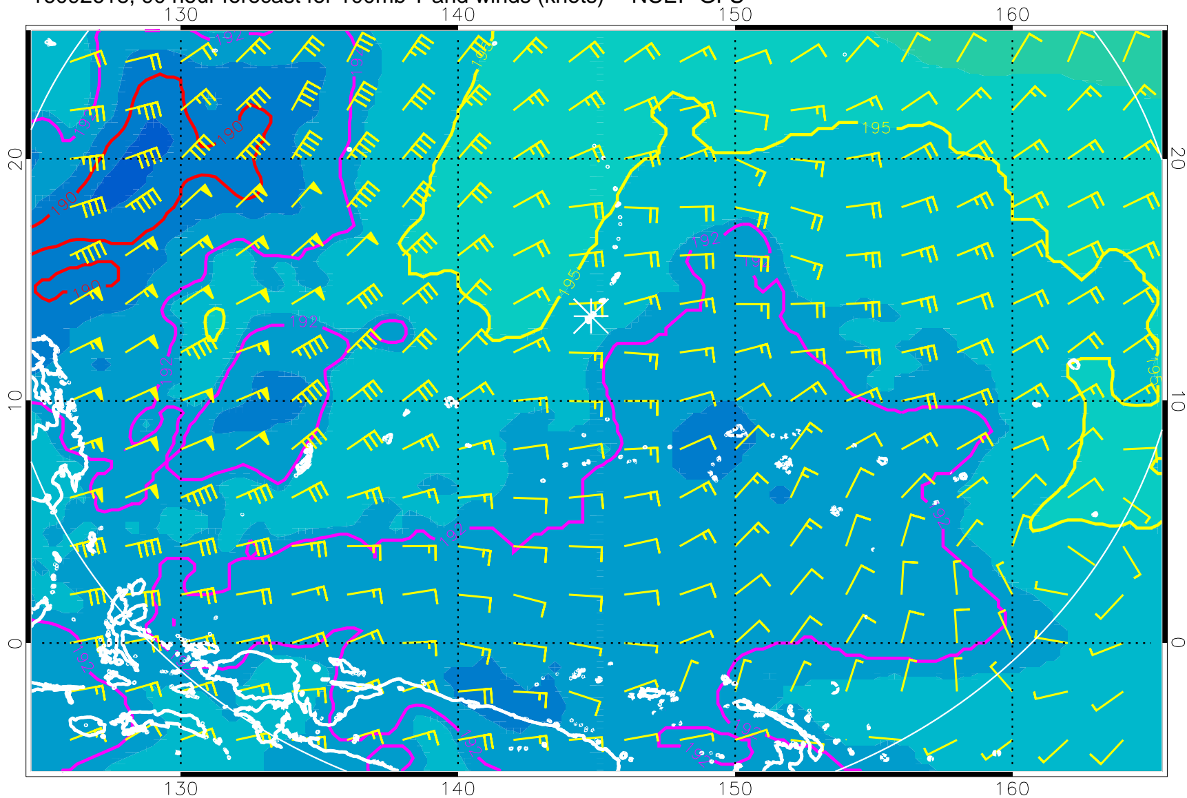
16092618, 90 hour forecast for 100mb T and winds (knots) -- NCEP GFS
