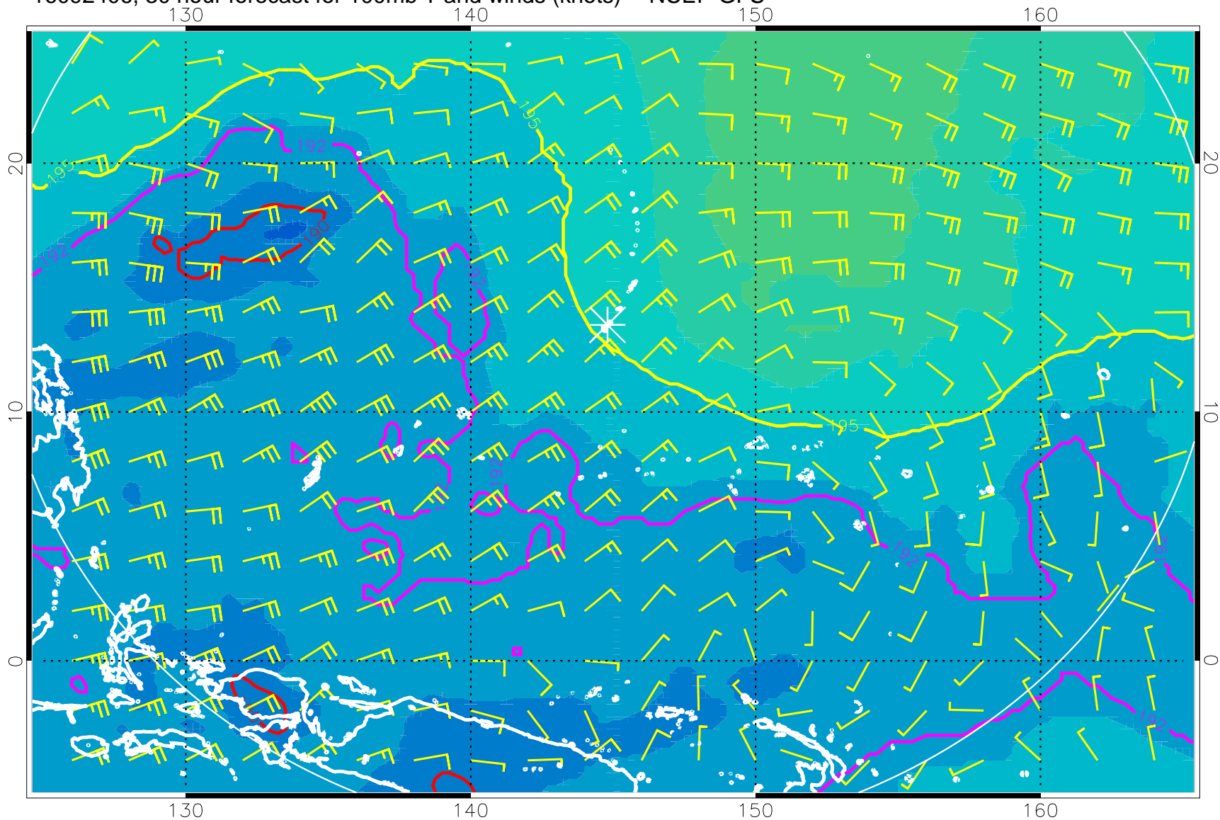
16092406, 30 hour forecast for 100mb T and winds (knots) -- NCEP GFS
