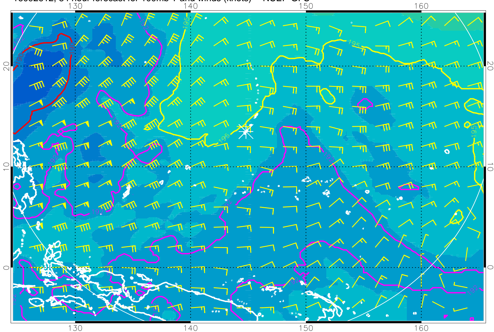
16092612, 84 hour forecast for 100mb T and winds (knots) -- NCEP GFS
