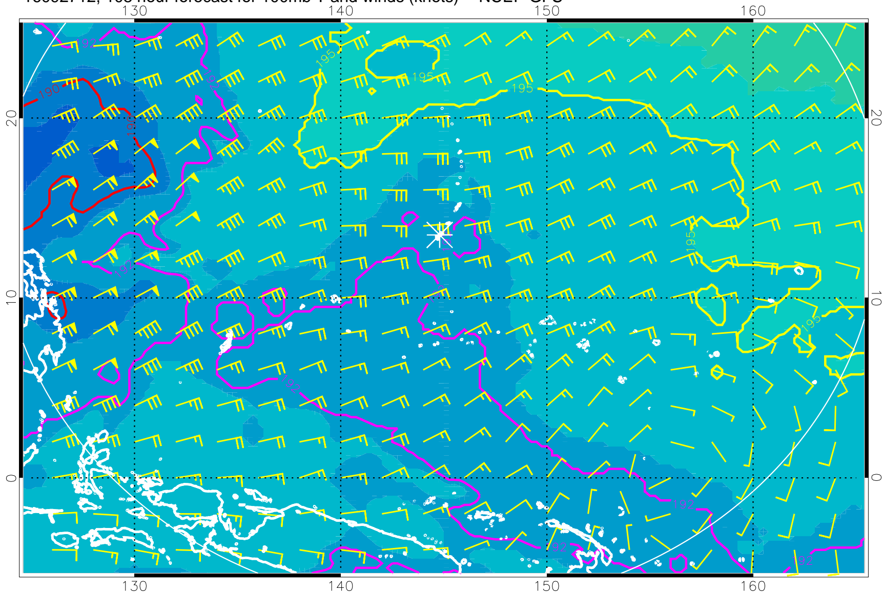
16092712, 108 hour forecast for 100mb T and winds (knots) -- NCEP GFS
