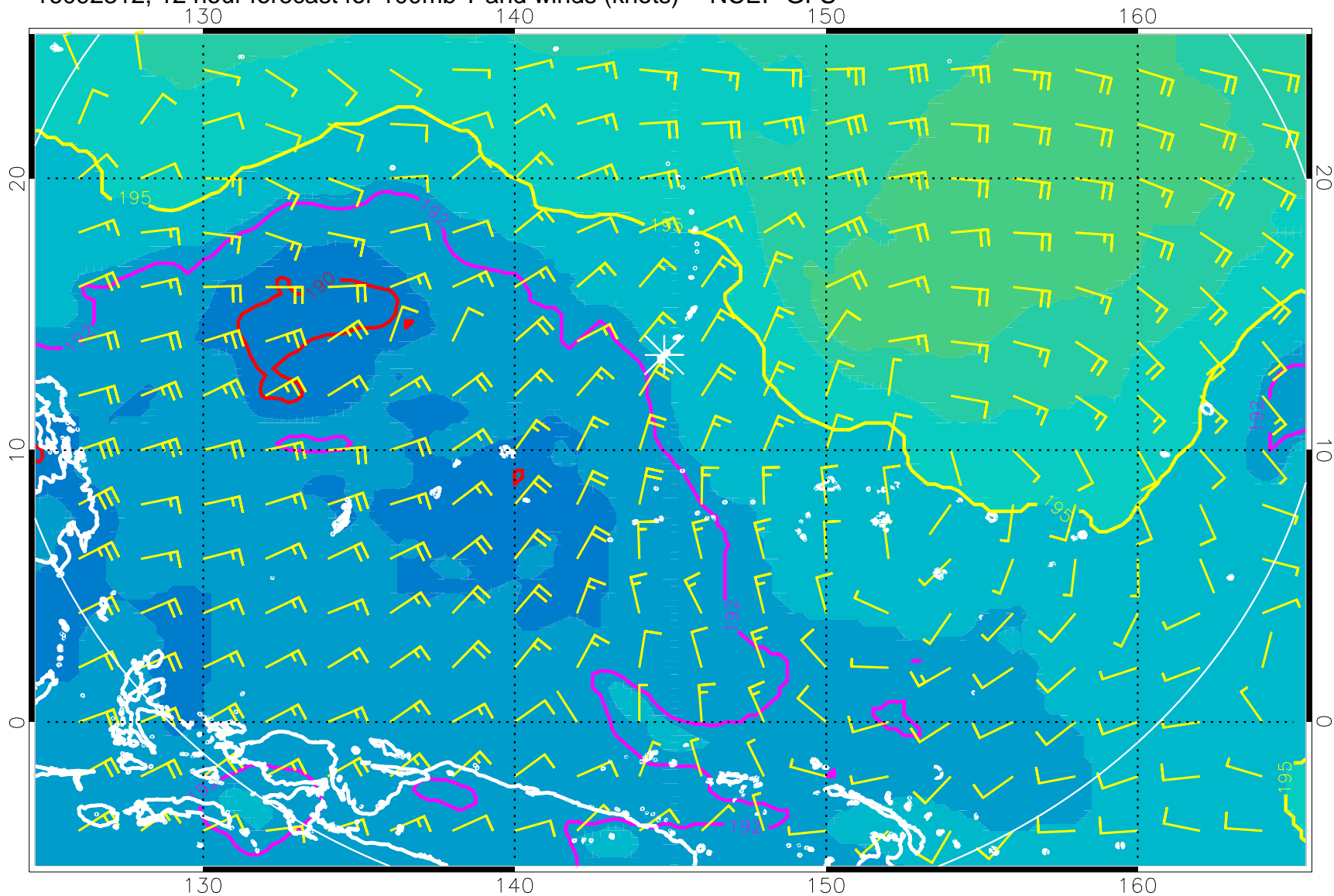
16092312, 12 hour forecast for 100mb T and winds (knots) -- NCEP GFS
