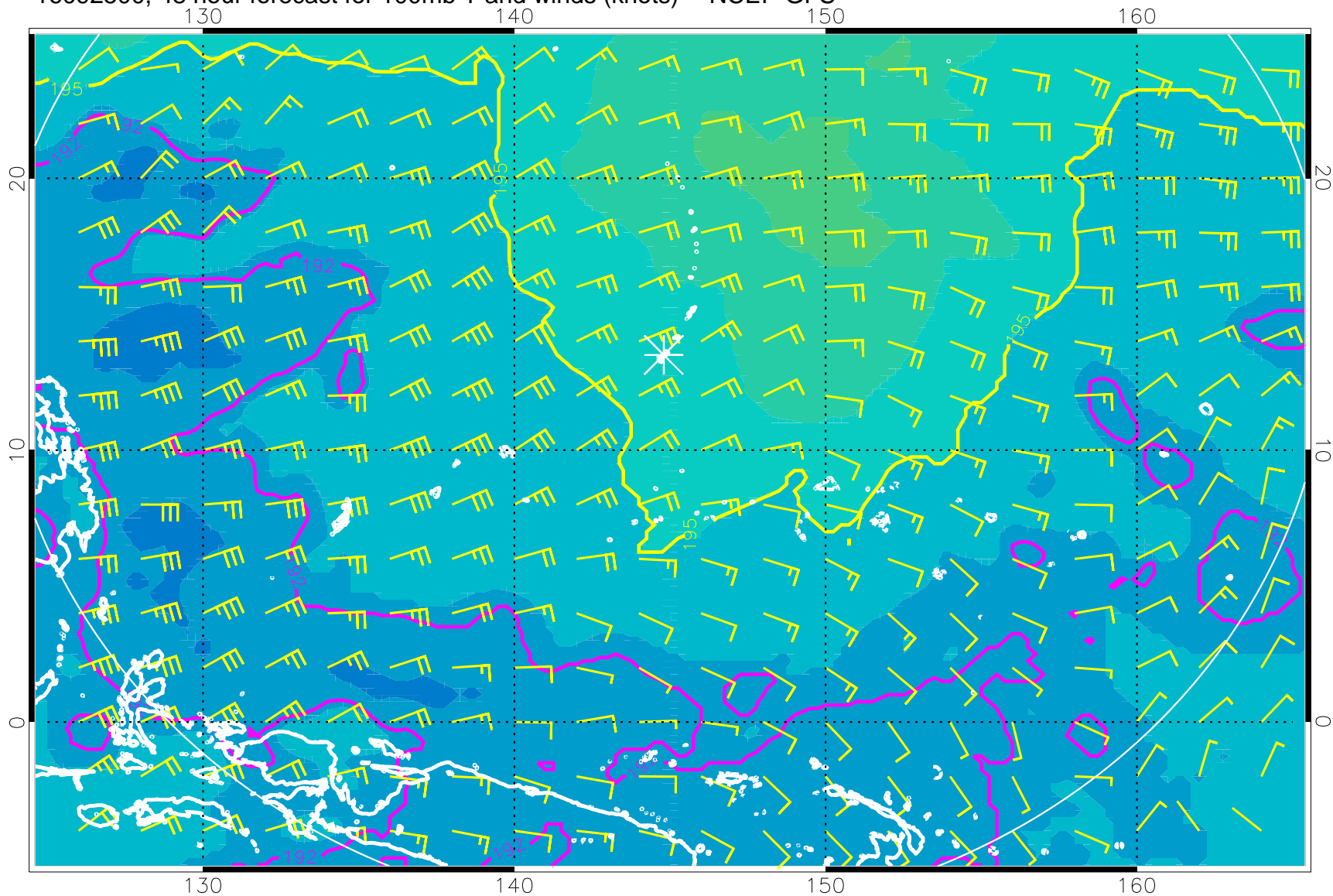
16092500, 48 hour forecast for 100mb T and winds (knots) -- NCEP GFS
