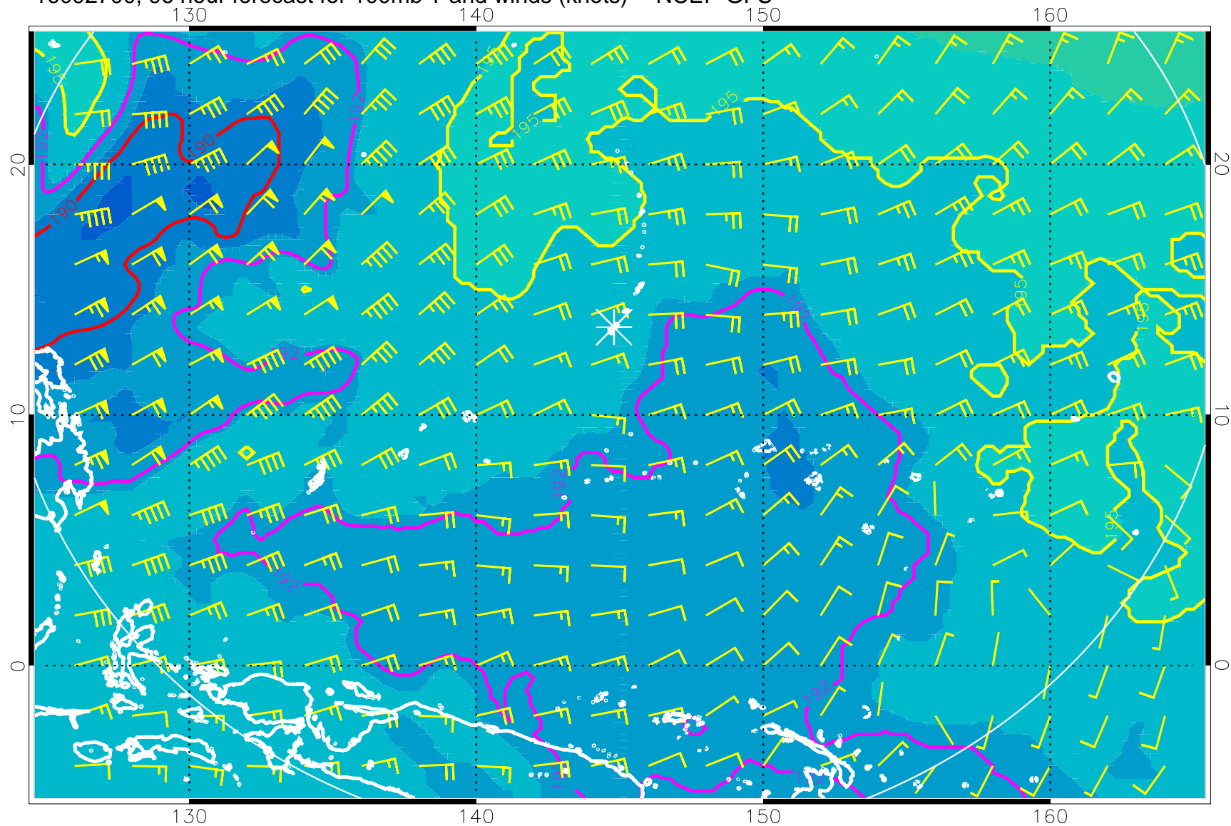
16092700, 96 hour forecast for 100mb T and winds (knots) -- NCEP GFS
