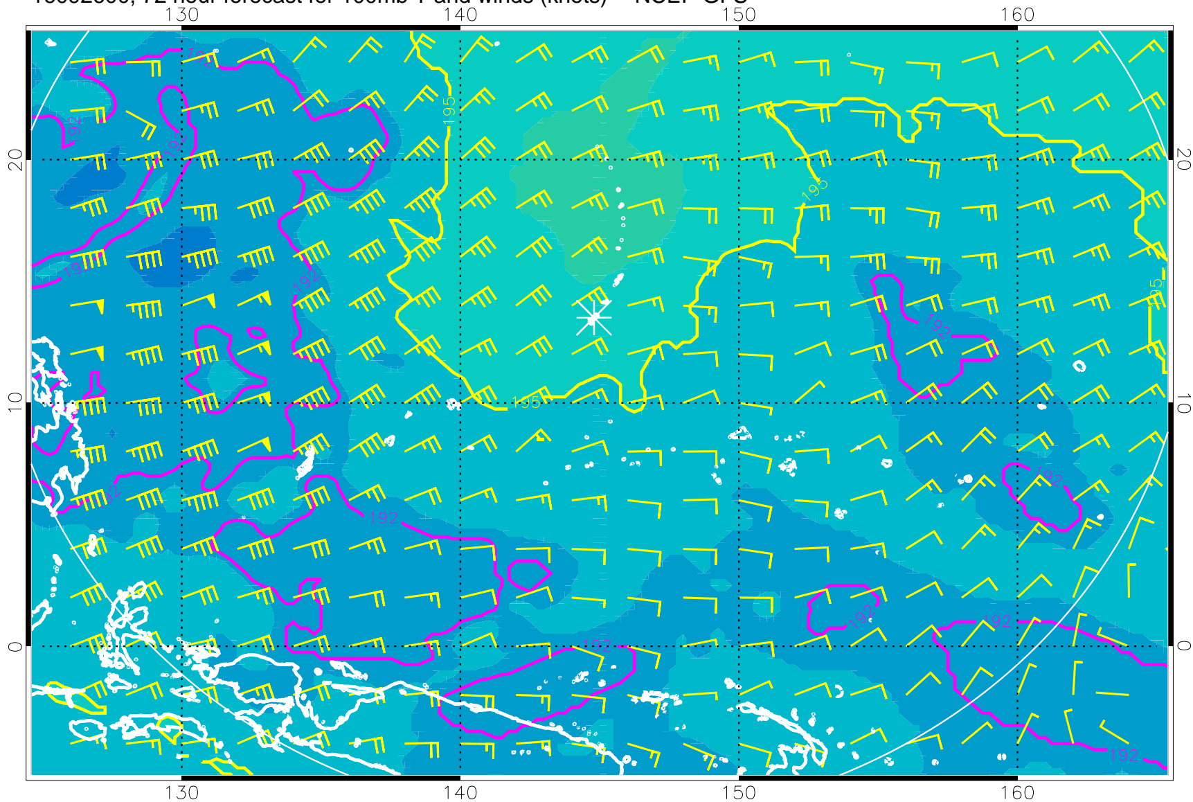
16092600, 72 hour forecast for 100mb T and winds (knots) -- NCEP GFS
