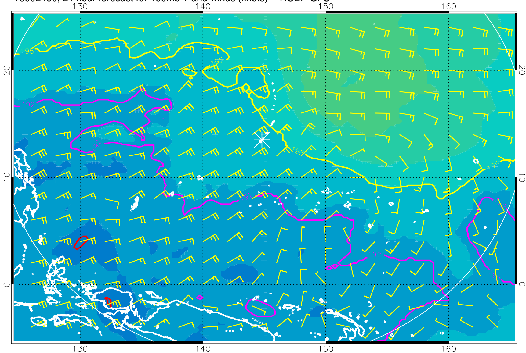
16092400, 24 hour forecast for 100mb T and winds (knots) -- NCEP GFS
