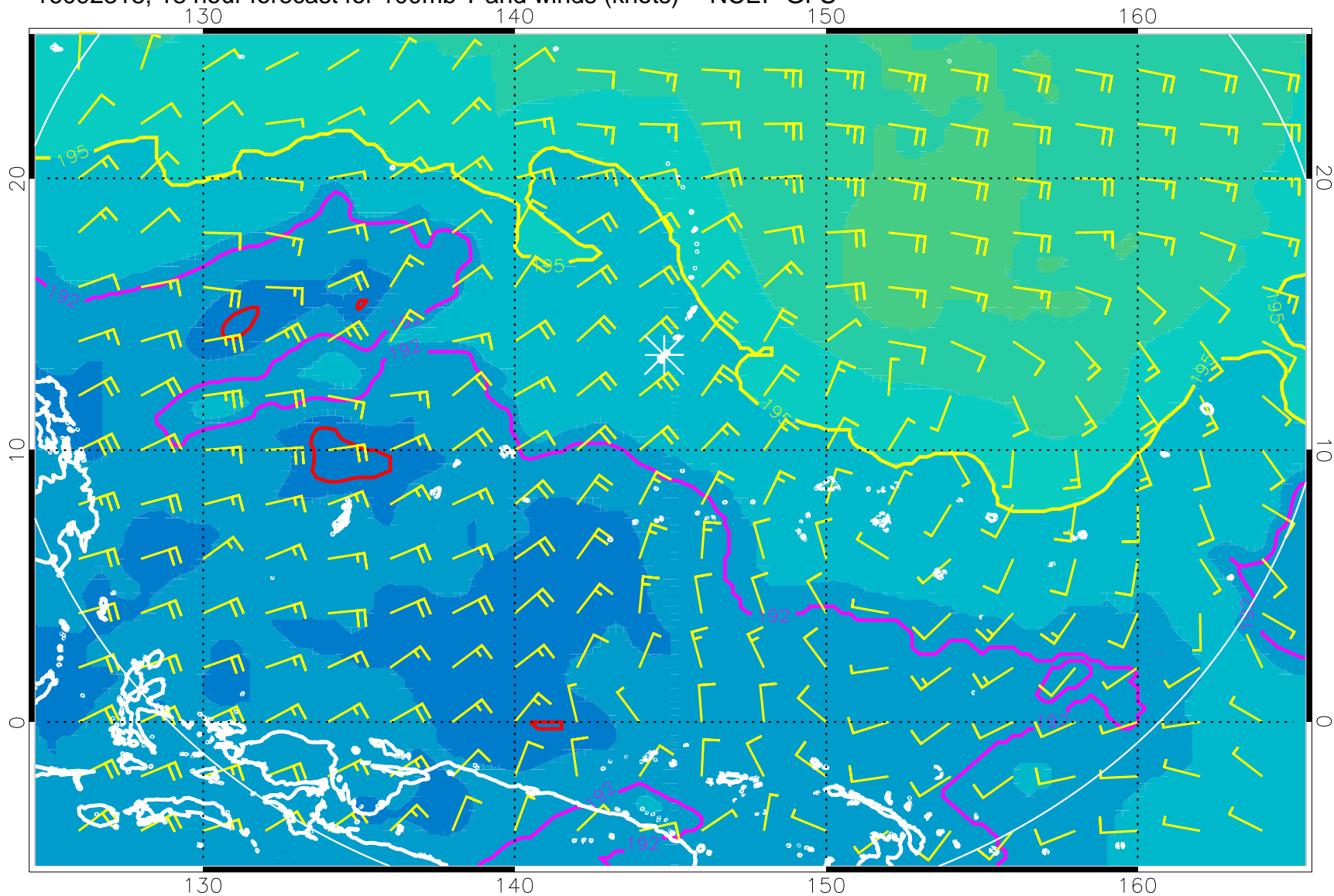
16092318, 18 hour forecast for 100mb T and winds (knots) -- NCEP GFS
