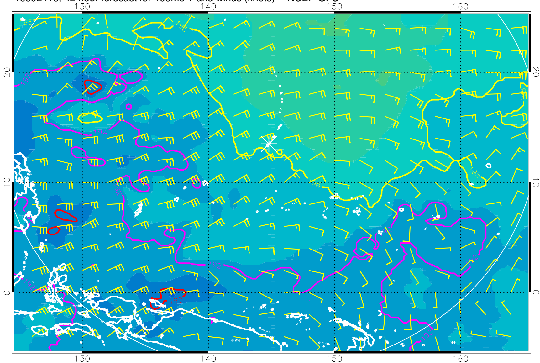
16092418, 42 hour forecast for 100mb T and winds (knots) -- NCEP GFS
