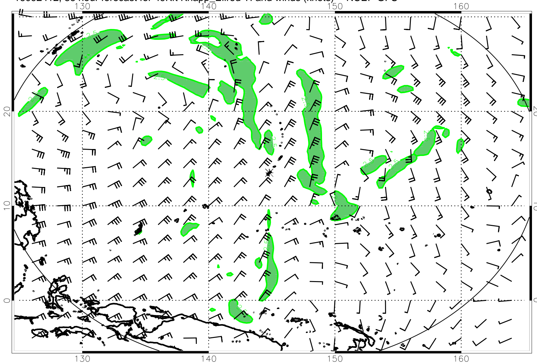
16092412, 36 hour forecast for 49Kft Knapp_Ellrod TI and winds (knots) -- NCEP GFS
