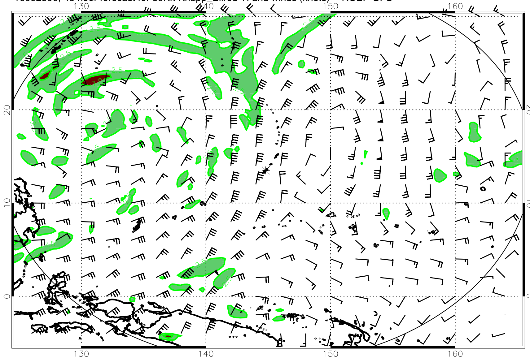
16092500, 48 hour forecast for 39Kft Knapp_Ellrod TI and winds (knots) -- NCEP GFS
