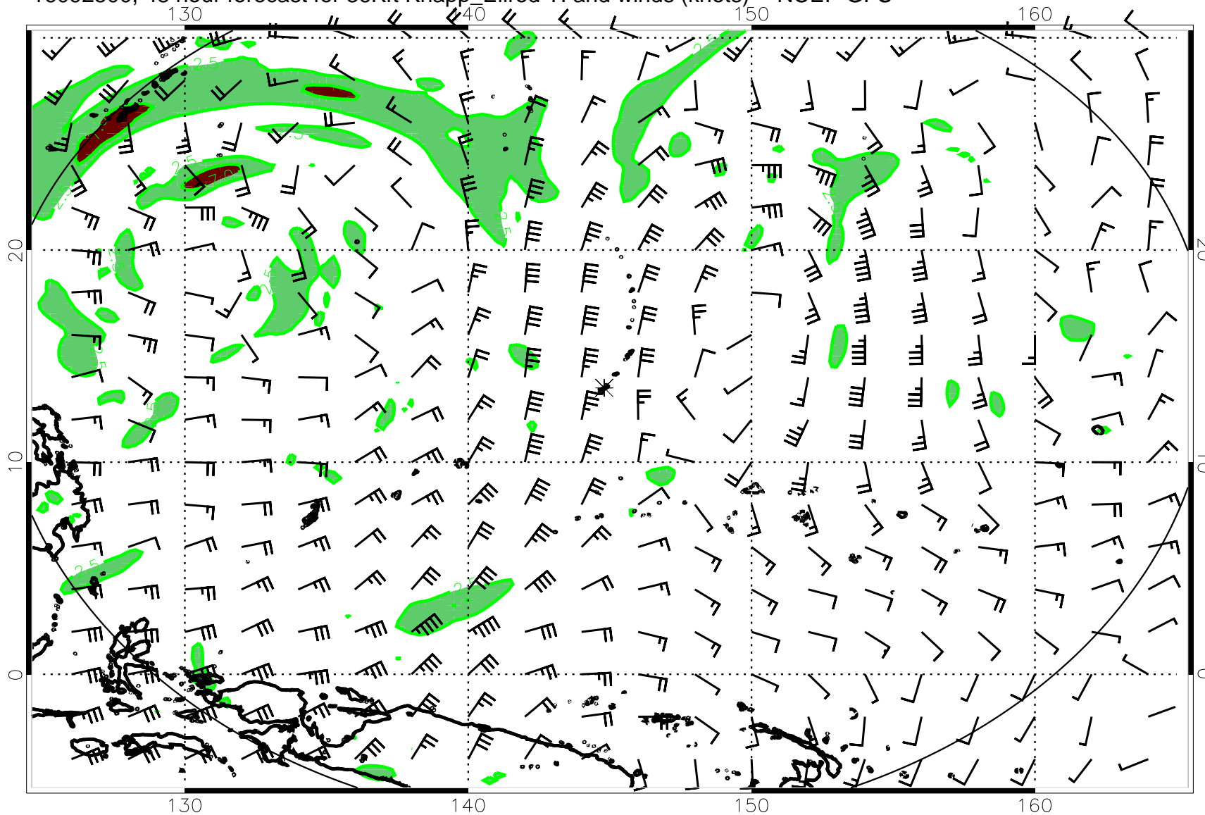
16092500, 48 hour forecast for 36Kft Knapp_Ellrod TI and winds (knots) -- NCEP GFS
