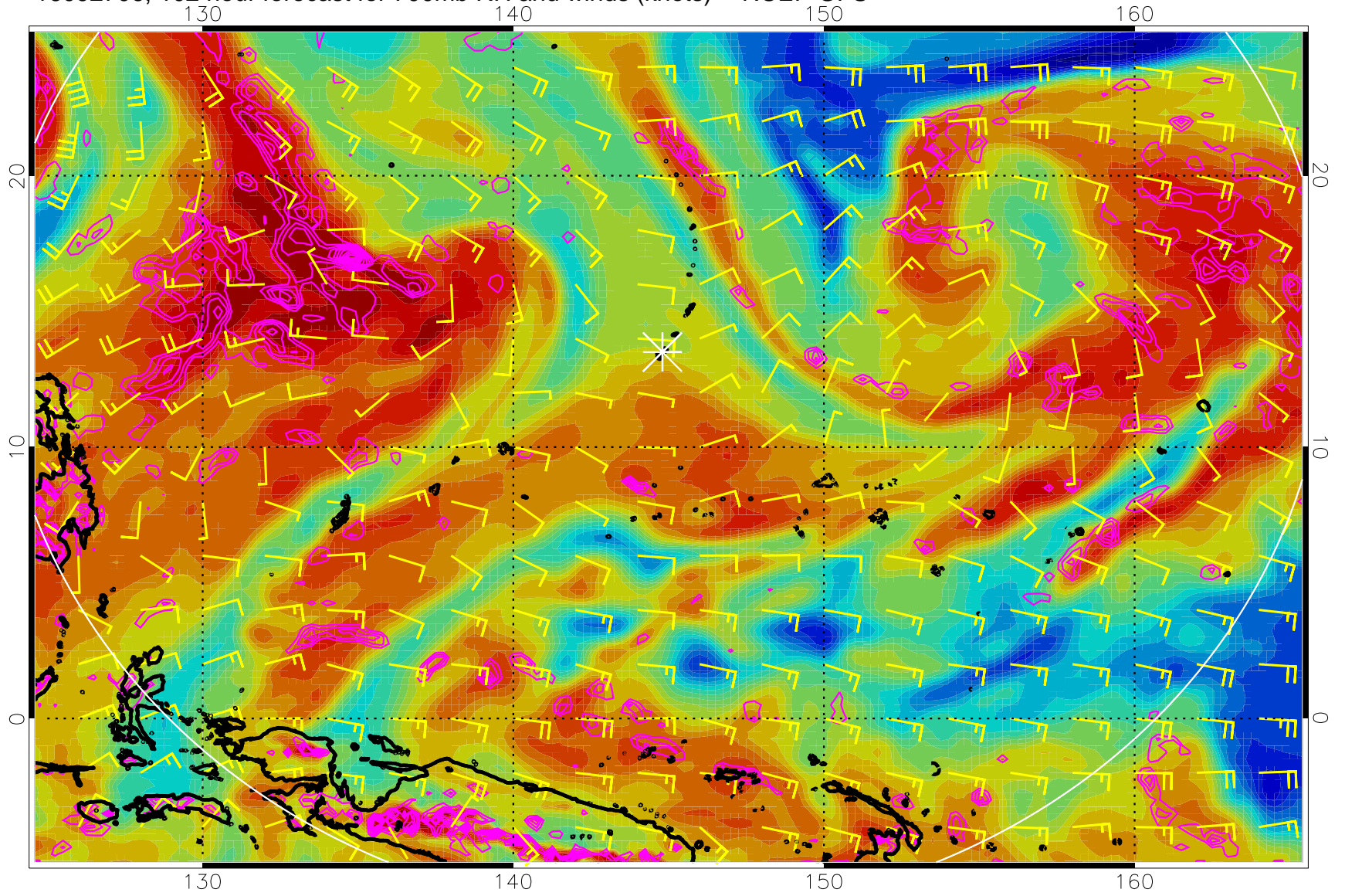
16092706, 102 hour forecast for 700mb RH and winds (knots) -- NCEP GFS
