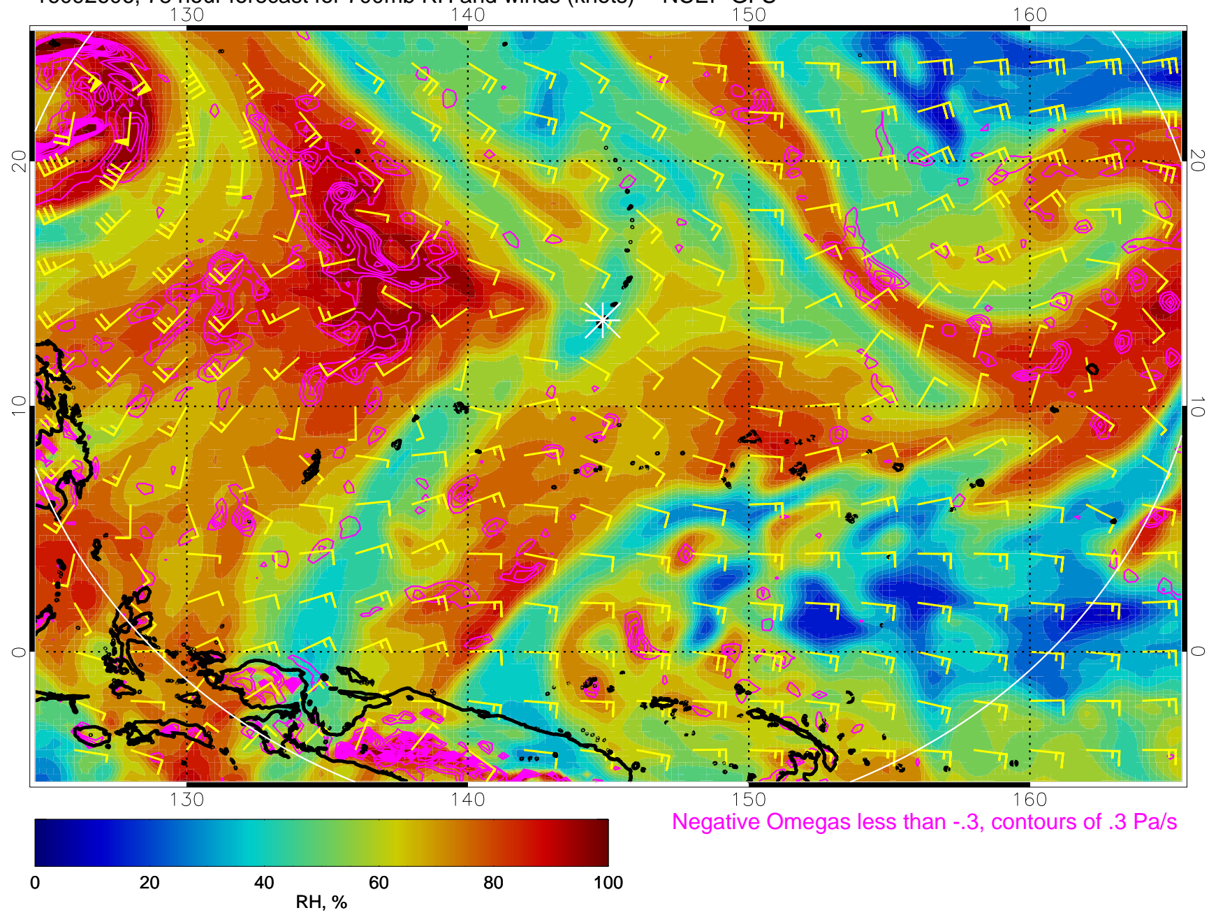
16092606, 78 hour forecast for 700mb RH and winds (knots) -- NCEP GFS
