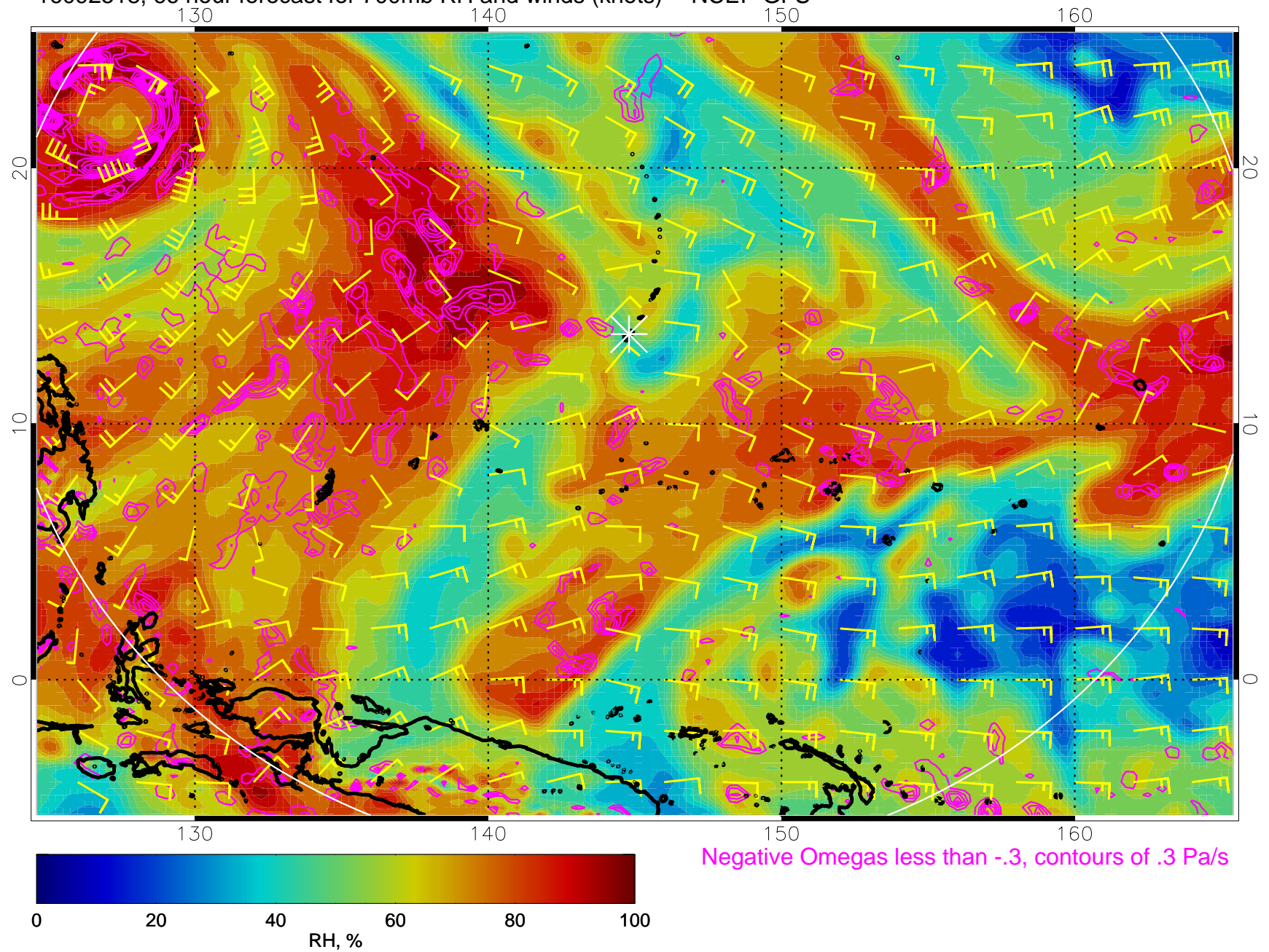
16092518, 66 hour forecast for 700mb RH and winds (knots) -- NCEP GFS
