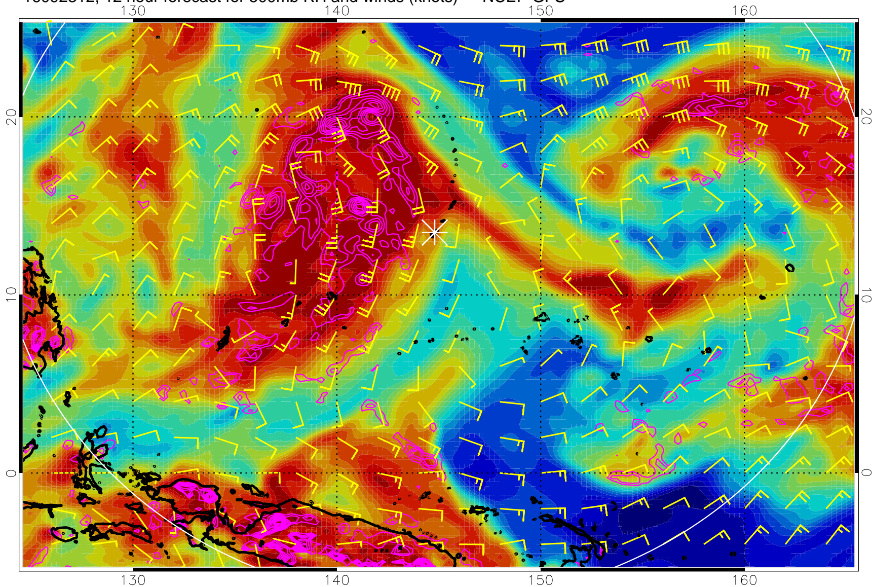
16092312, 12 hour forecast for 500mb RH and winds (knots) -- NCEP GFS
