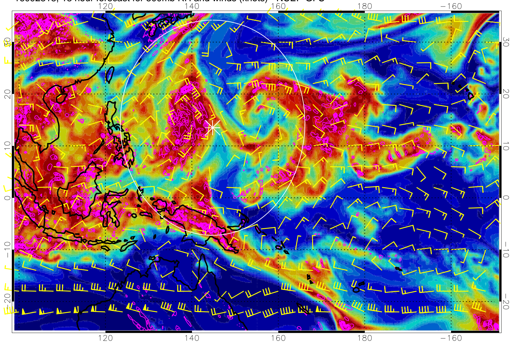
16092318, 18 hour forecast for 500mb RH and winds (knots) - NCEP GFS
