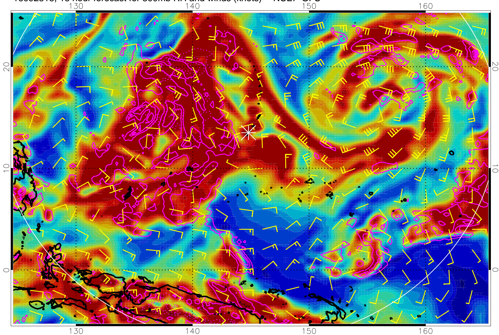
16092318, 18 hour forecast for 300mb RH and winds (knots) -- NCEP GFS
