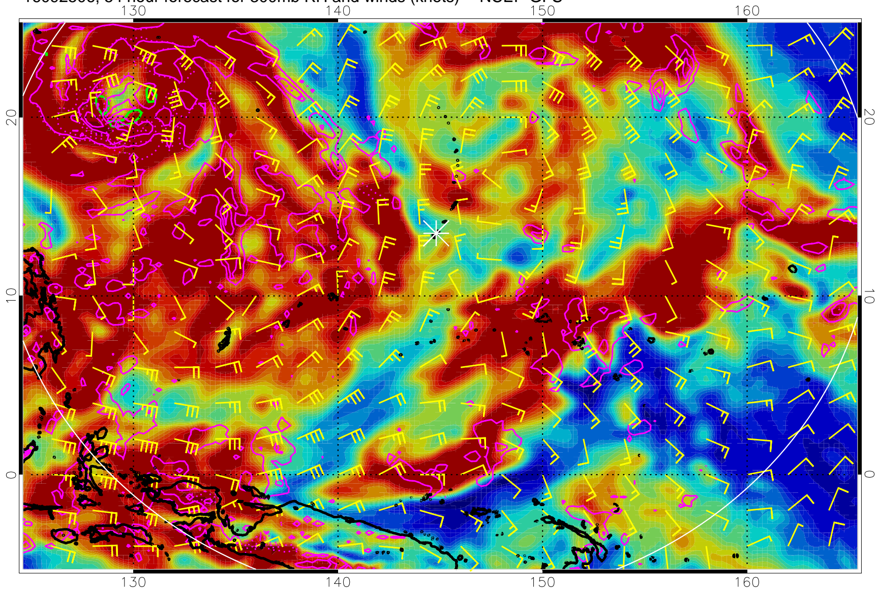
16092506, 54 hour forecast for 300mb RH and winds (knots) -- NCEP GFS
