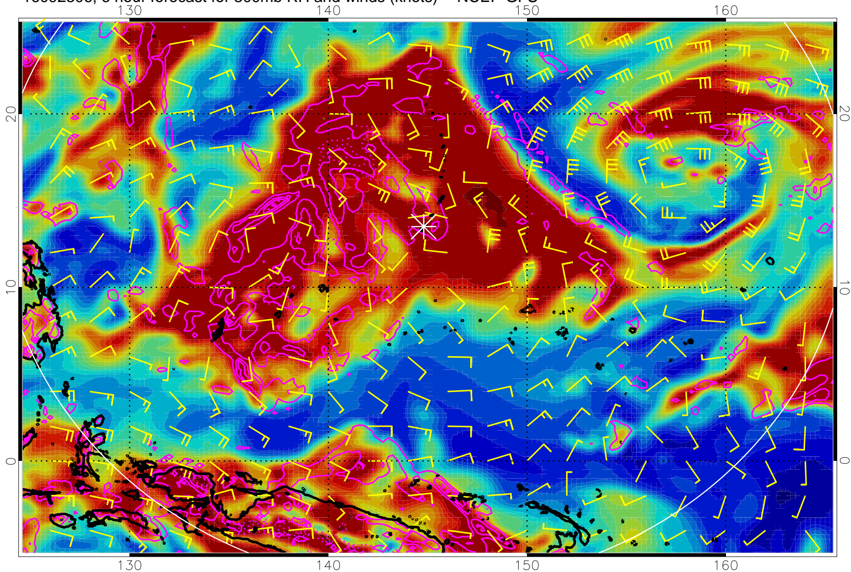
16092306, 6 hour forecast for 300mb RH and winds (knots) -- NCEP GFS
