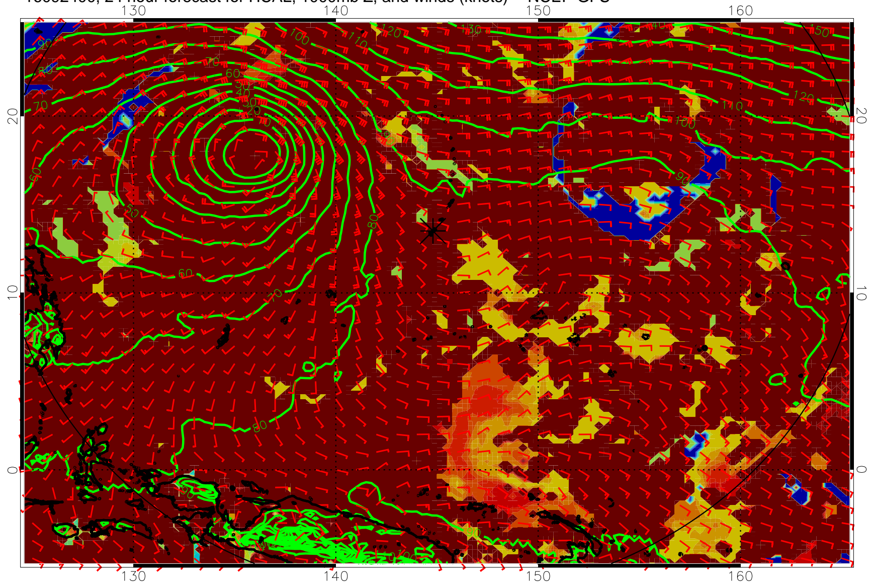
16092400, 24 hour forecast for HCAL, 1000mb Z, and winds (knots) -- NCEP GFS
