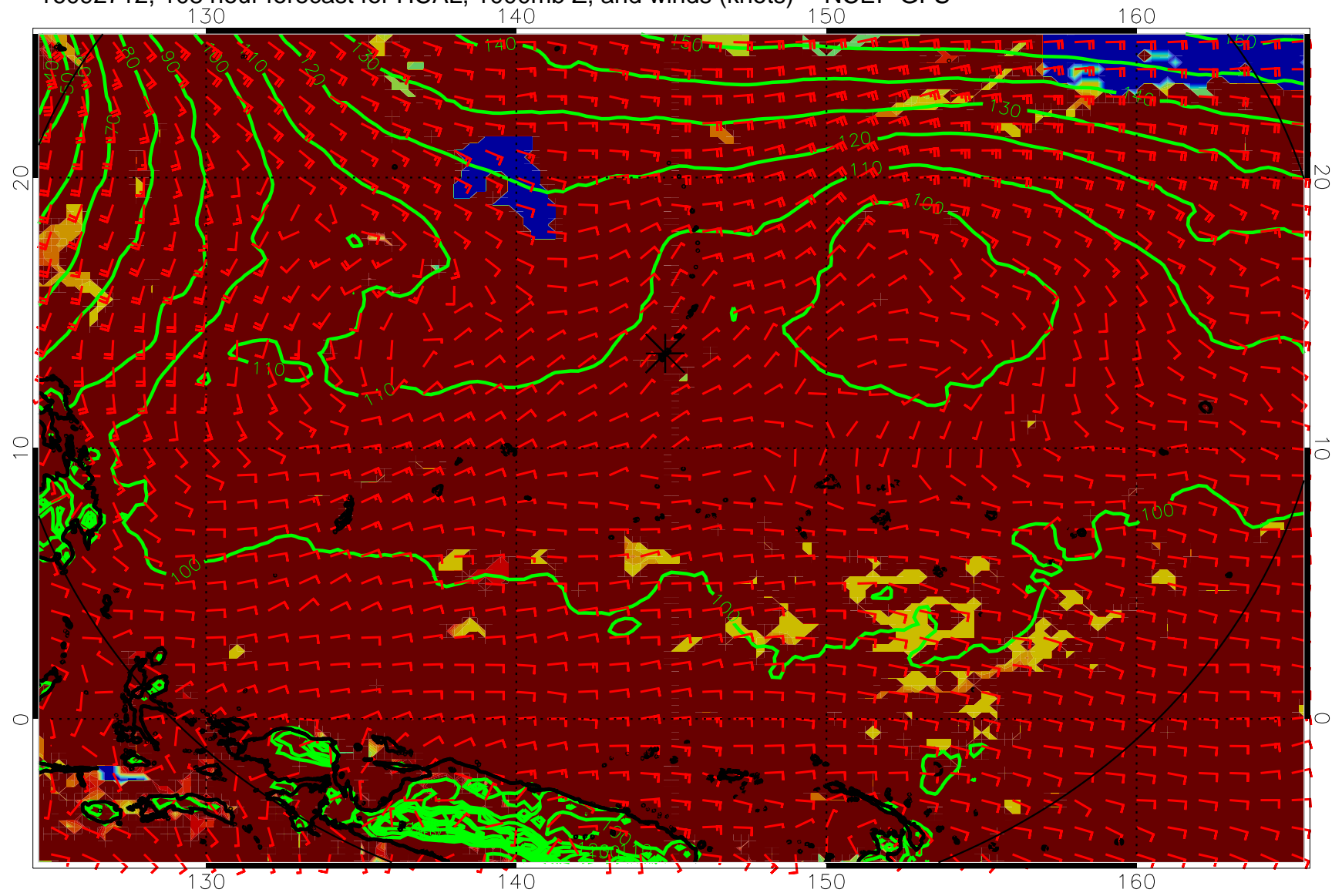
16092712, 108 hour forecast for HCAL, 1000mb Z, and winds (knots) -- NCEP GFS
