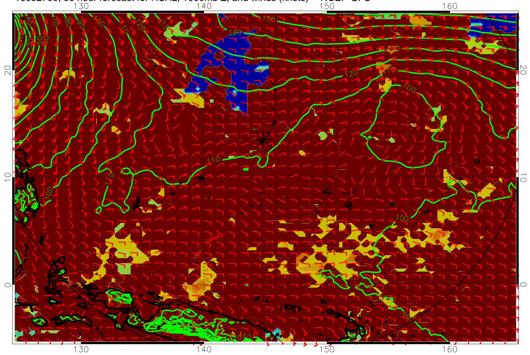
16092700, 96 hour forecast for HCAL, 1000mb Z, and winds (knots) -- NCEP GFS
