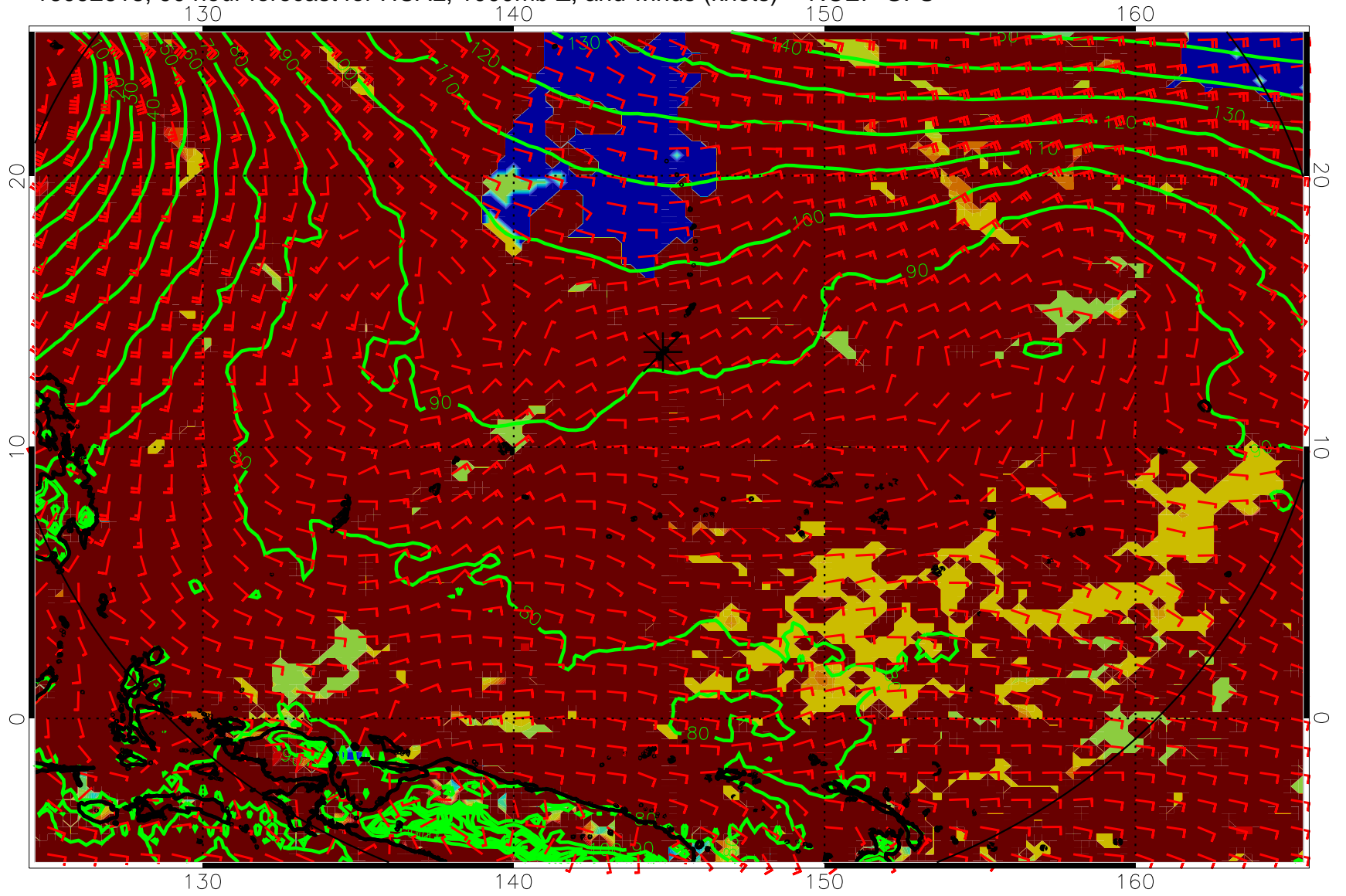
16092618, 90 hour forecast for HCAL, 1000mb Z, and winds (knots) -- NCEP GFS
