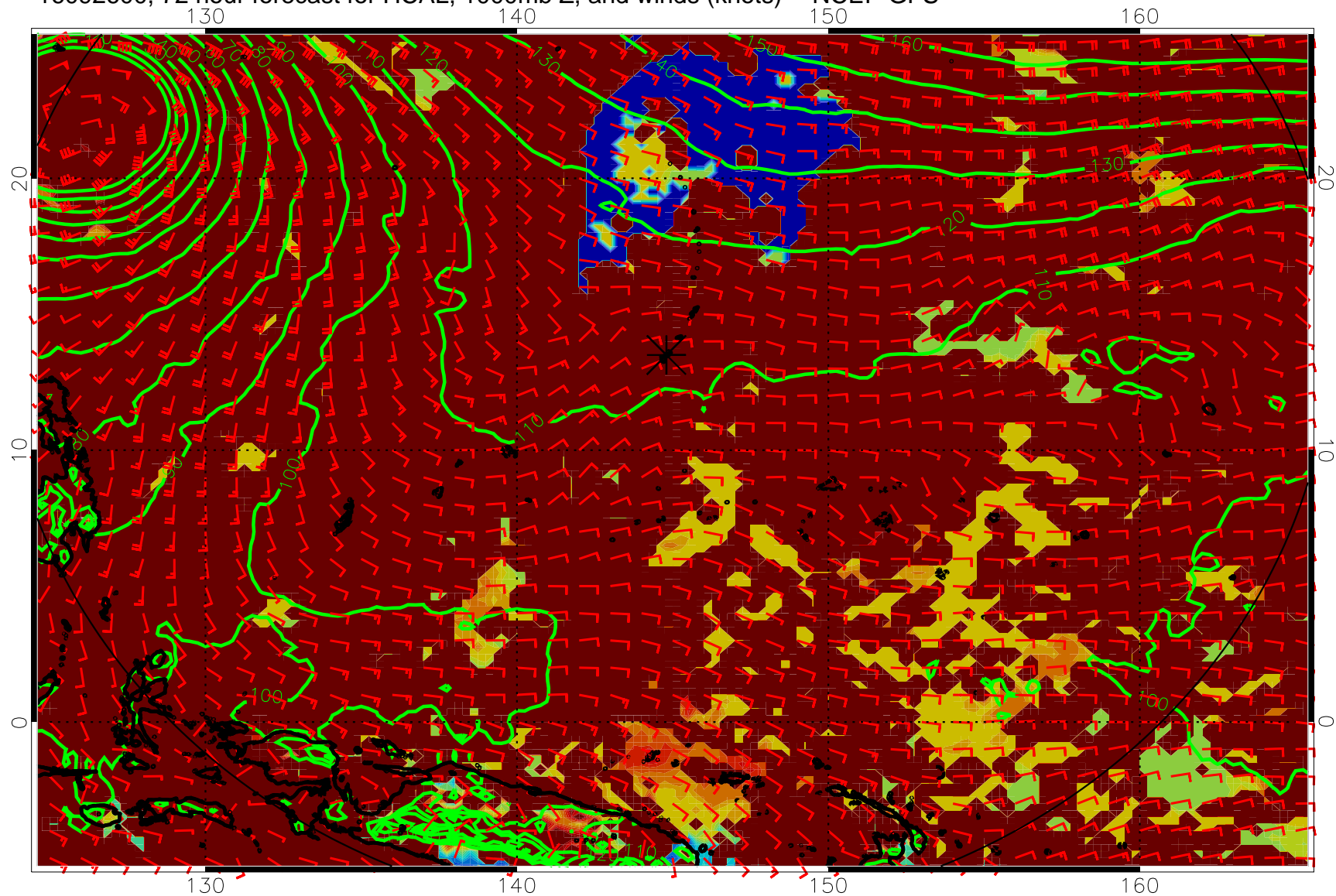
16092600, 72 hour forecast for HCAL, 1000mb Z, and winds (knots) -- NCEP GFS
