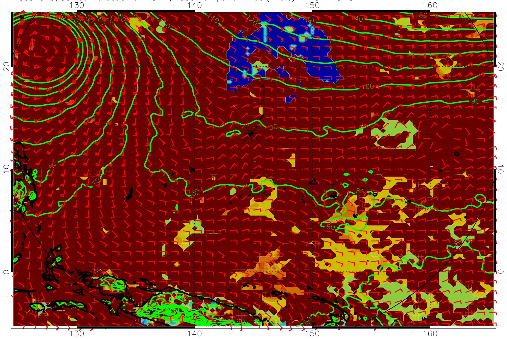
16092518, 66 hour forecast for HCAL, 1000mb Z, and winds (knots) -- NCEP GFS
