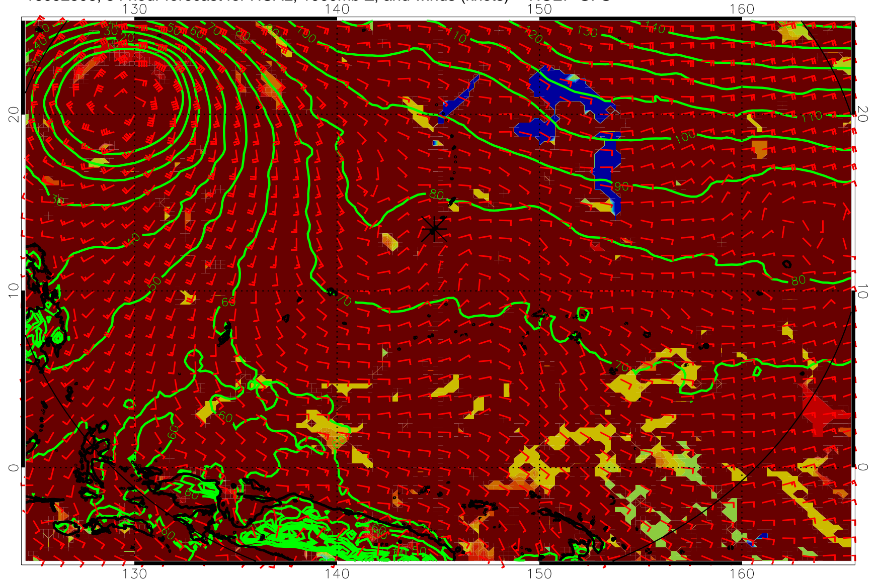
16092506, 54 hour forecast for HCAL, 1000mb Z, and winds (knots) -- NCEP GFS
