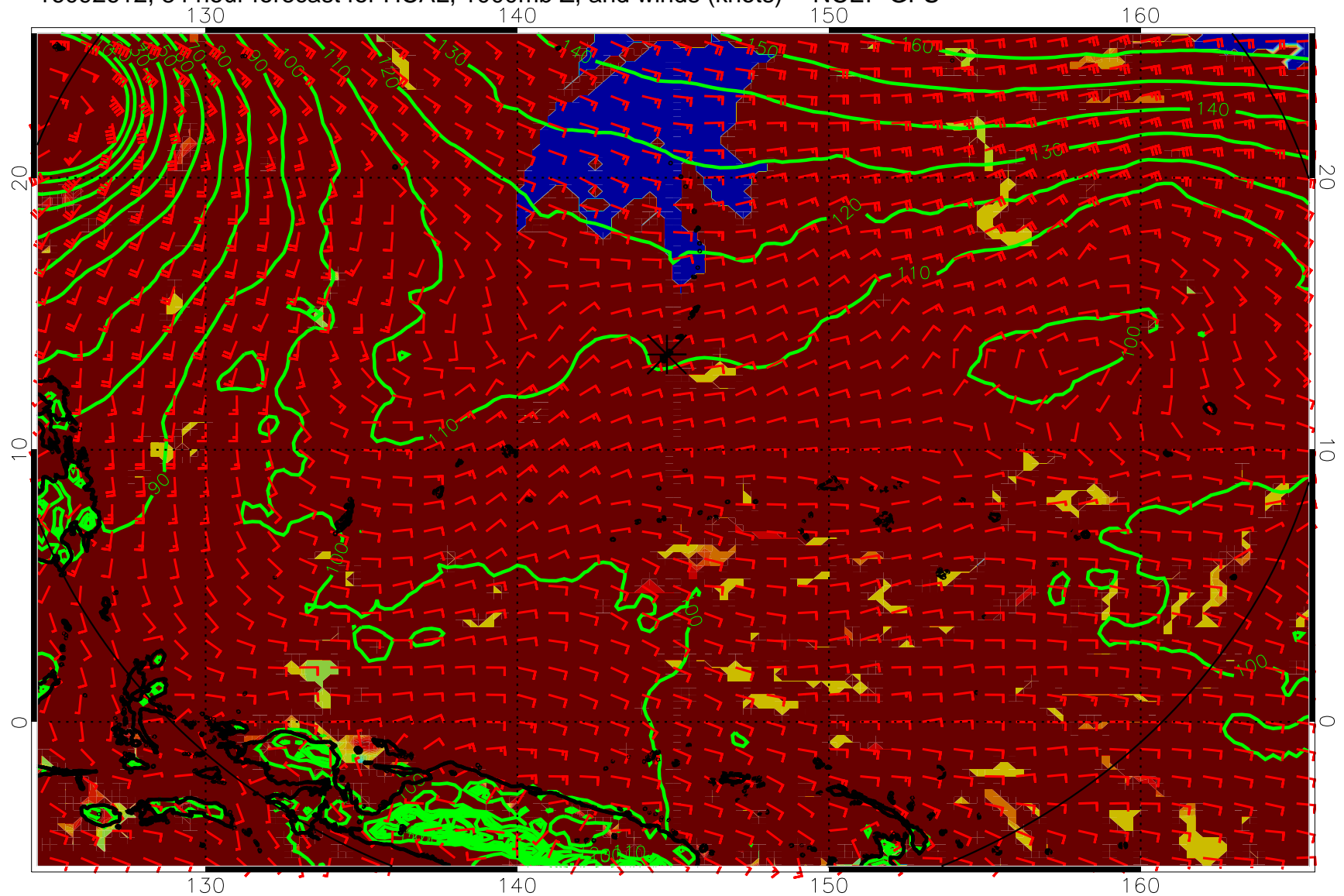
16092612, 84 hour forecast for HCAL, 1000mb Z, and winds (knots) -- NCEP GFS
