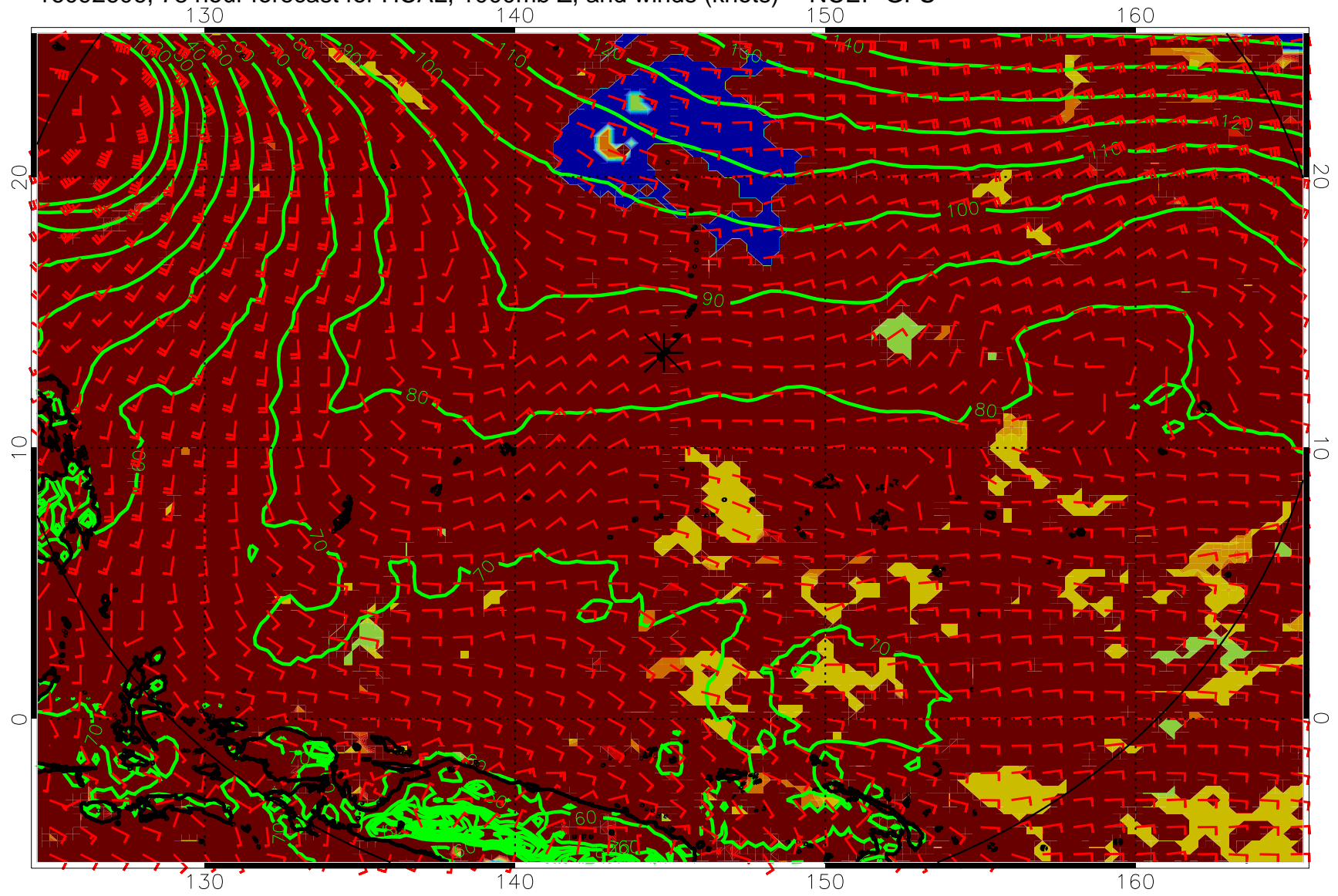
16092606, 78 hour forecast for HCAL, 1000mb Z, and winds (knots) -- NCEP GFS
