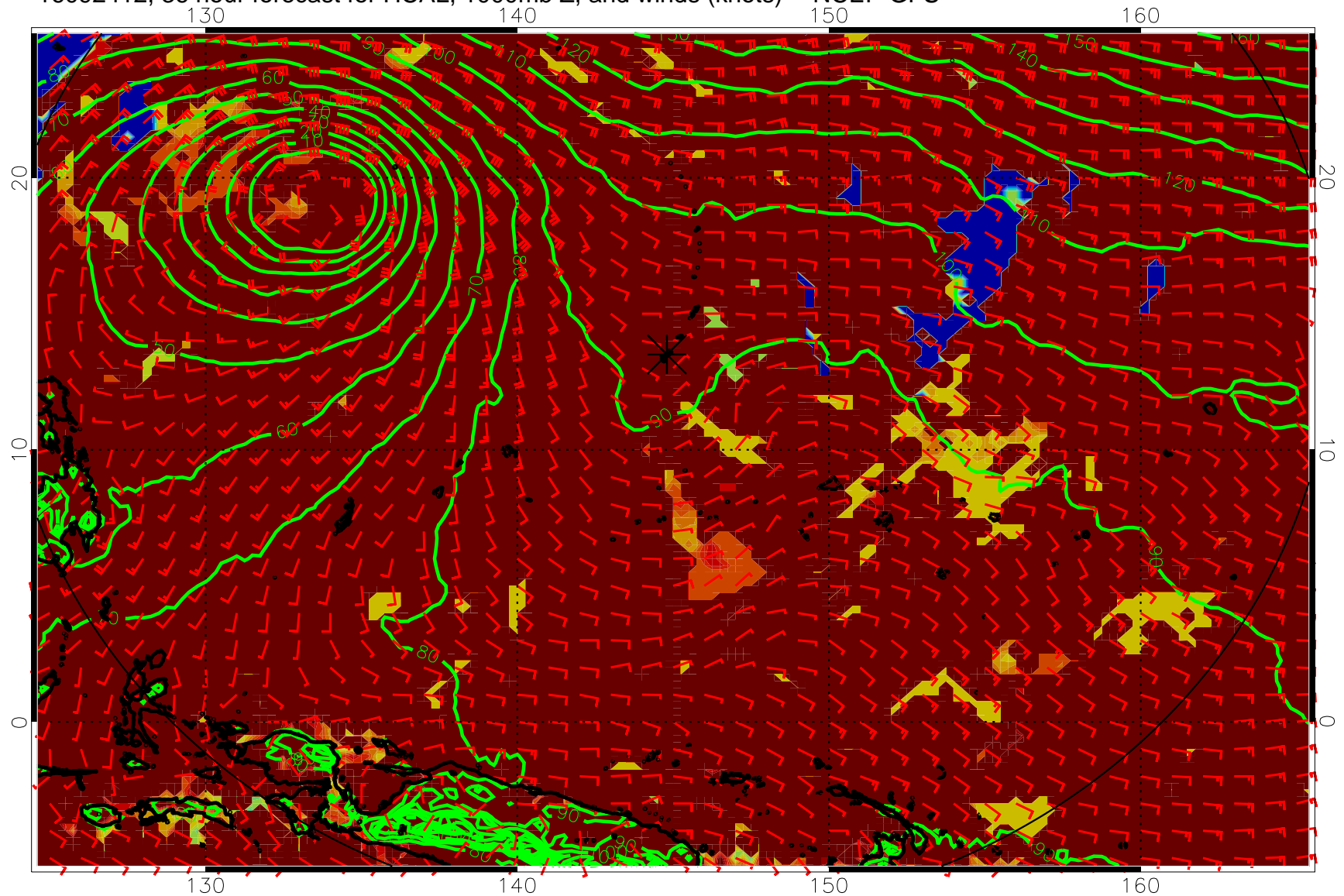
16092412, 36 hour forecast for HCAL, 1000mb Z, and winds (knots) -- NCEP GFS
