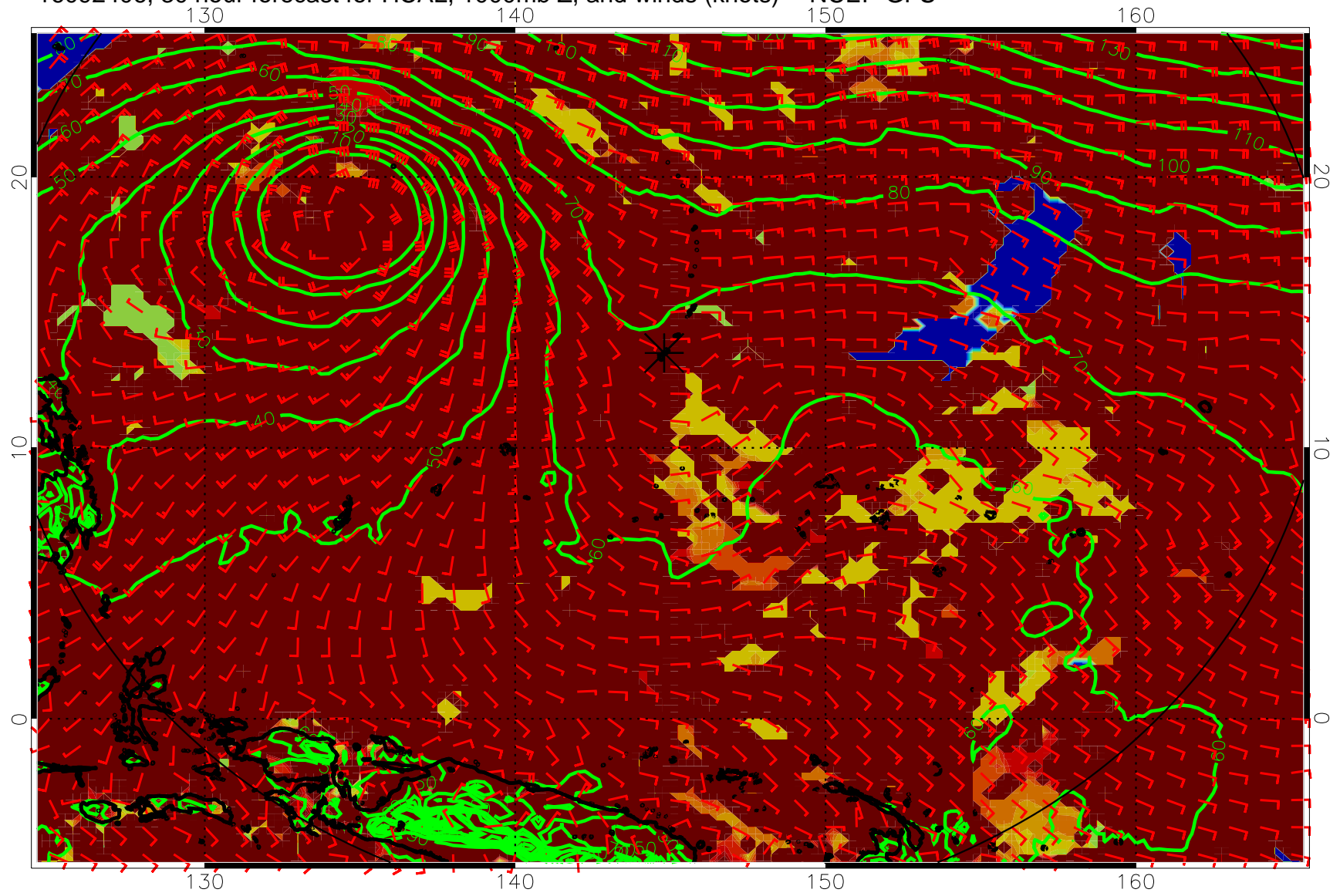
16092406, 30 hour forecast for HCAL, 1000mb Z, and winds (knots) -- NCEP GFS
