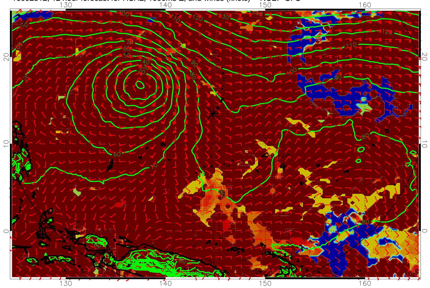
16092312, 12 hour forecast for HCAL, 1000mb Z, and winds (knots) -- NCEP GFS
