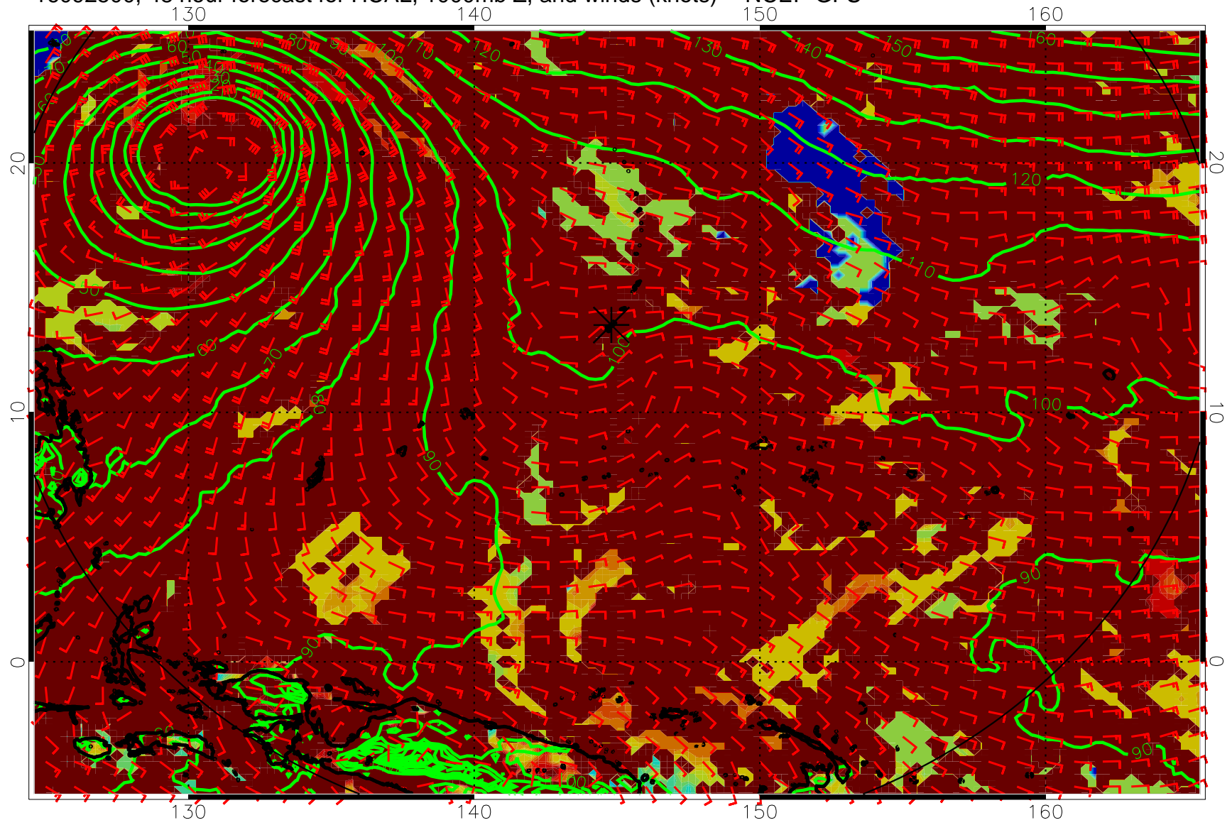
16092500, 48 hour forecast for HCAL, 1000mb Z, and winds (knots) -- NCEP GFS
