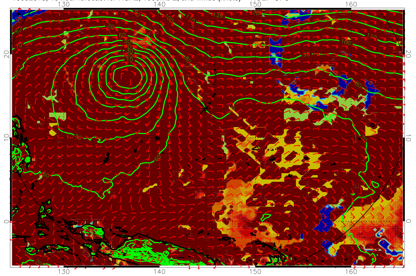
16092318, 18 hour forecast for HCAL, 1000mb Z, and winds (knots) -- NCEP GFS
