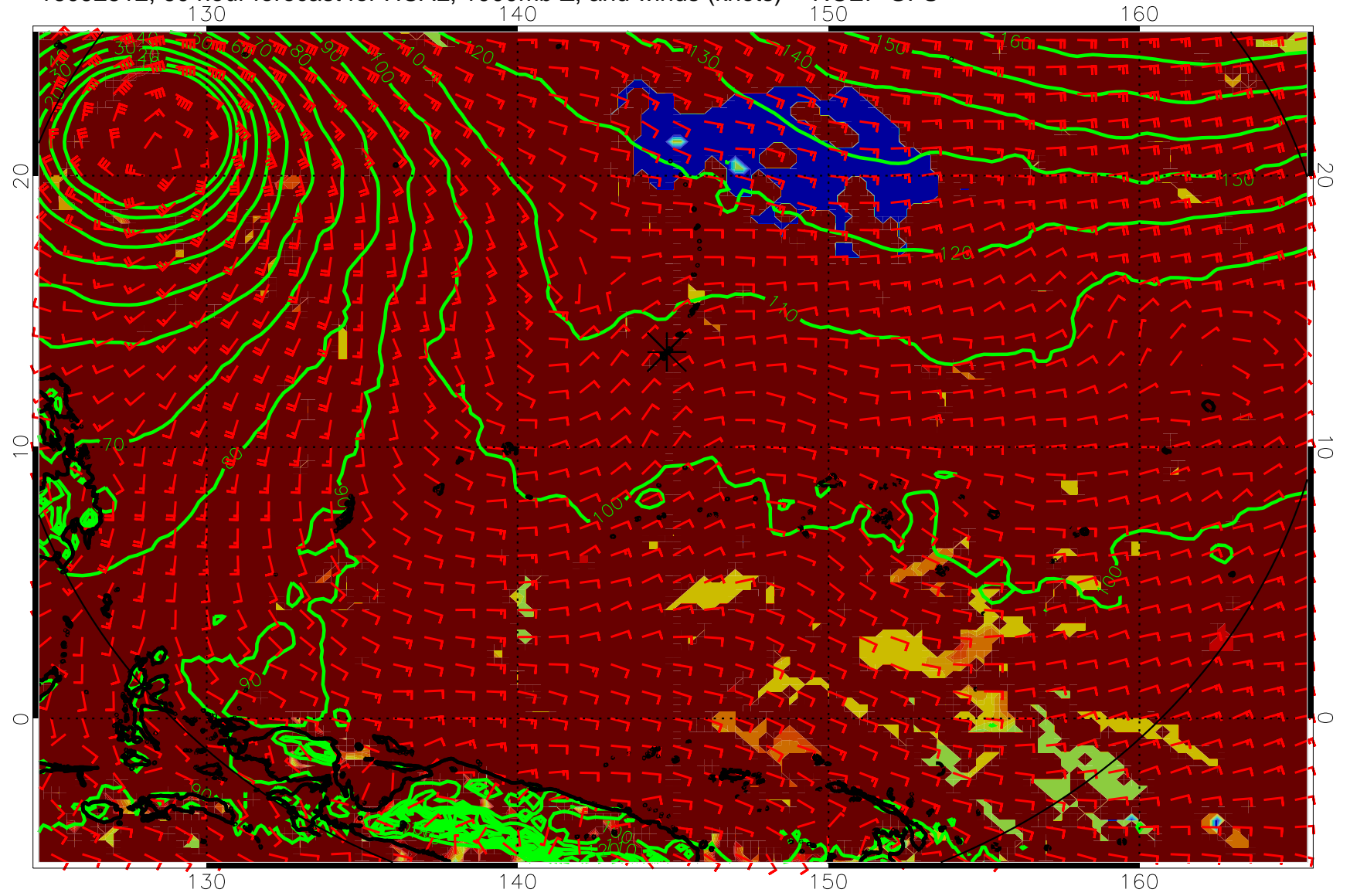
16092512, 60 hour forecast for HCAL, 1000mb Z, and winds (knots) -- NCEP GFS
