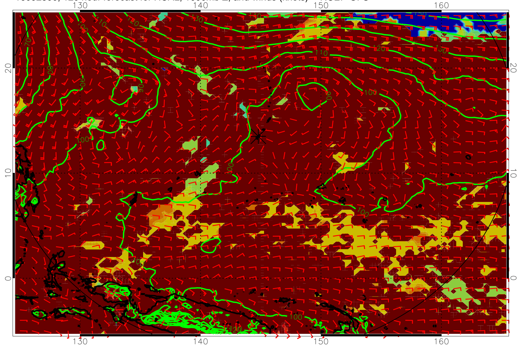
16092800, 120 hour forecast for HCAL, 1000mb Z, and winds (knots) -- NCEP GFS
