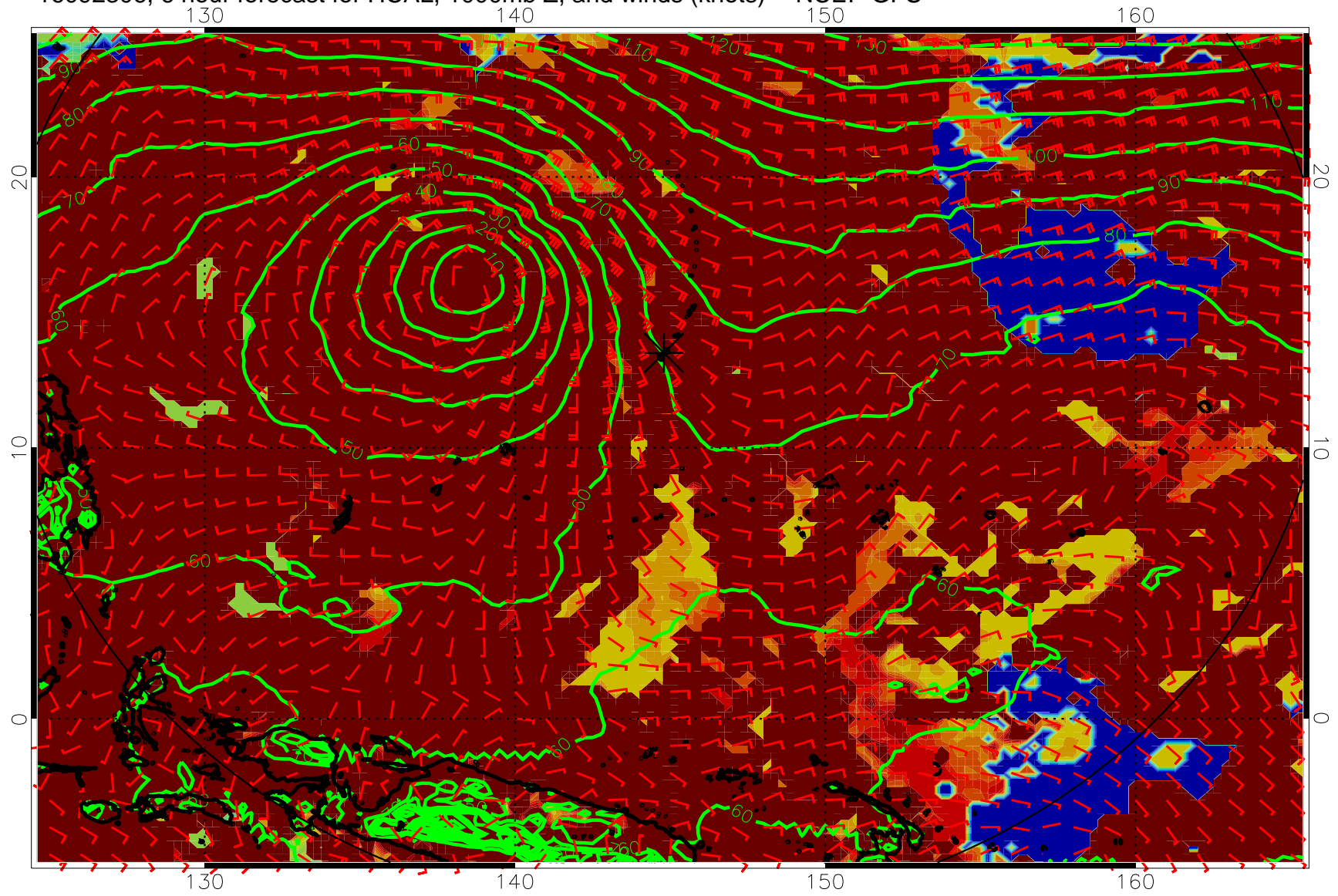
16092306, 6 hour forecast for HCAL, 1000mb Z, and winds (knots) -- NCEP GFS
