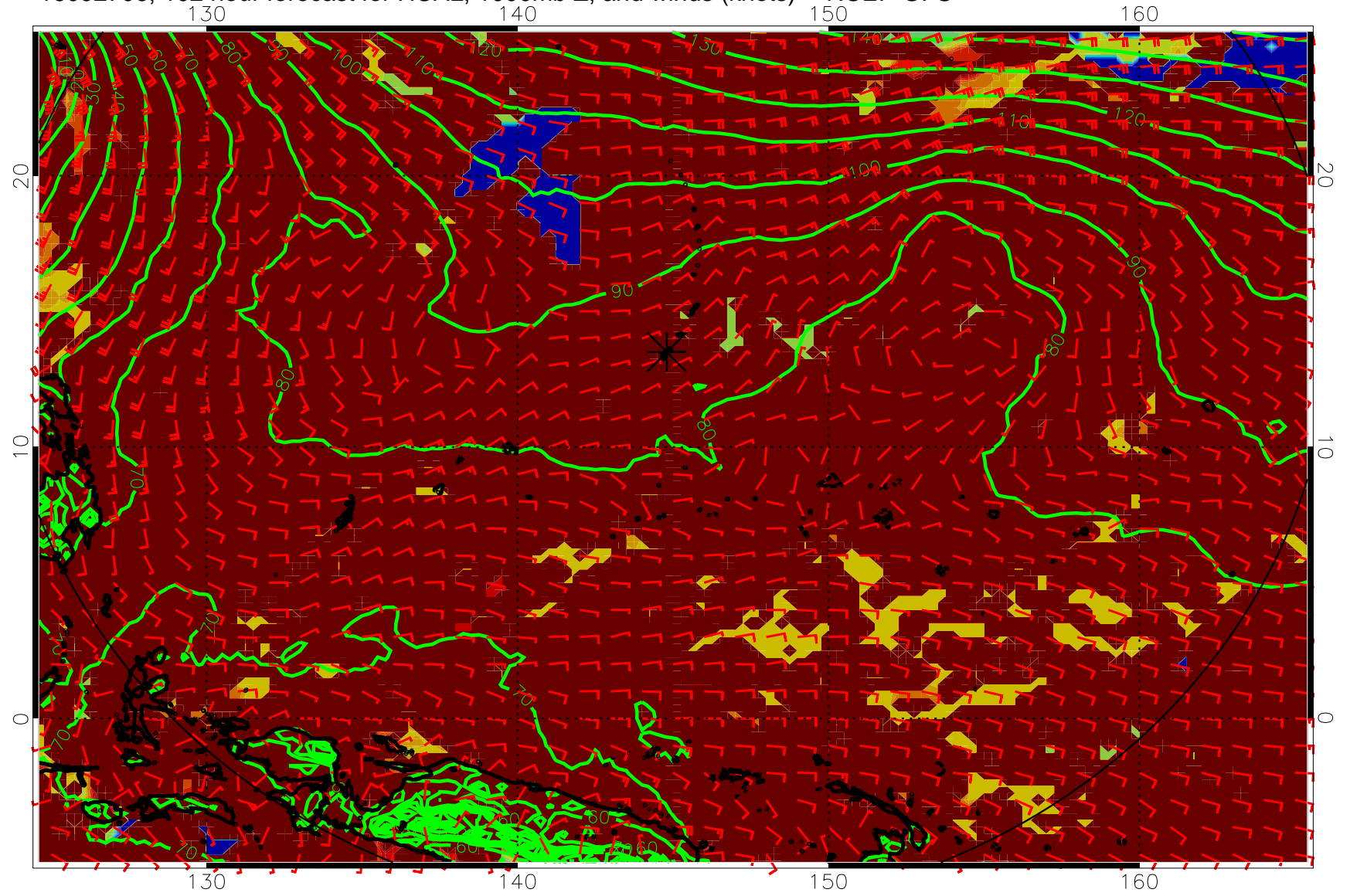
16092706, 102 hour forecast for HCAL, 1000mb Z, and winds (knots) -- NCEP GFS
