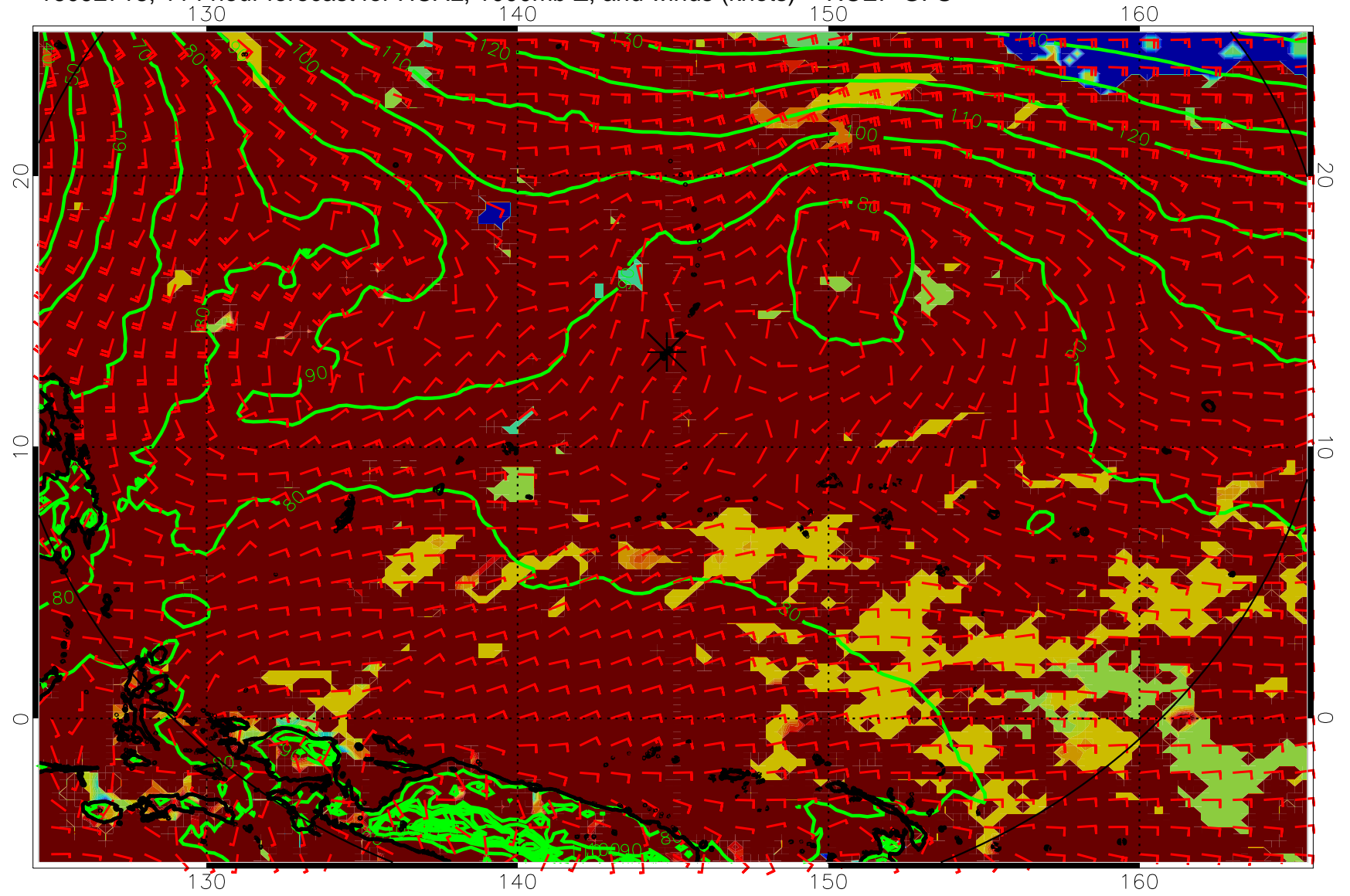
16092718, 114 hour forecast for HCAL, 1000mb Z, and winds (knots) -- NCEP GFS
