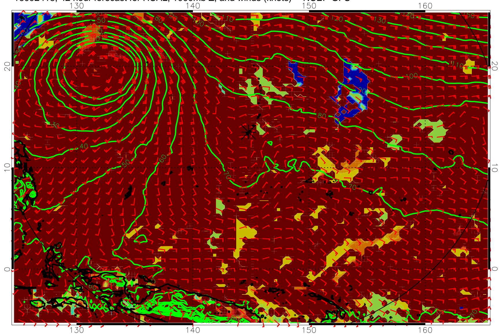
16092418, 42 hour forecast for HCAL, 1000mb Z, and winds (knots) -- NCEP GFS
