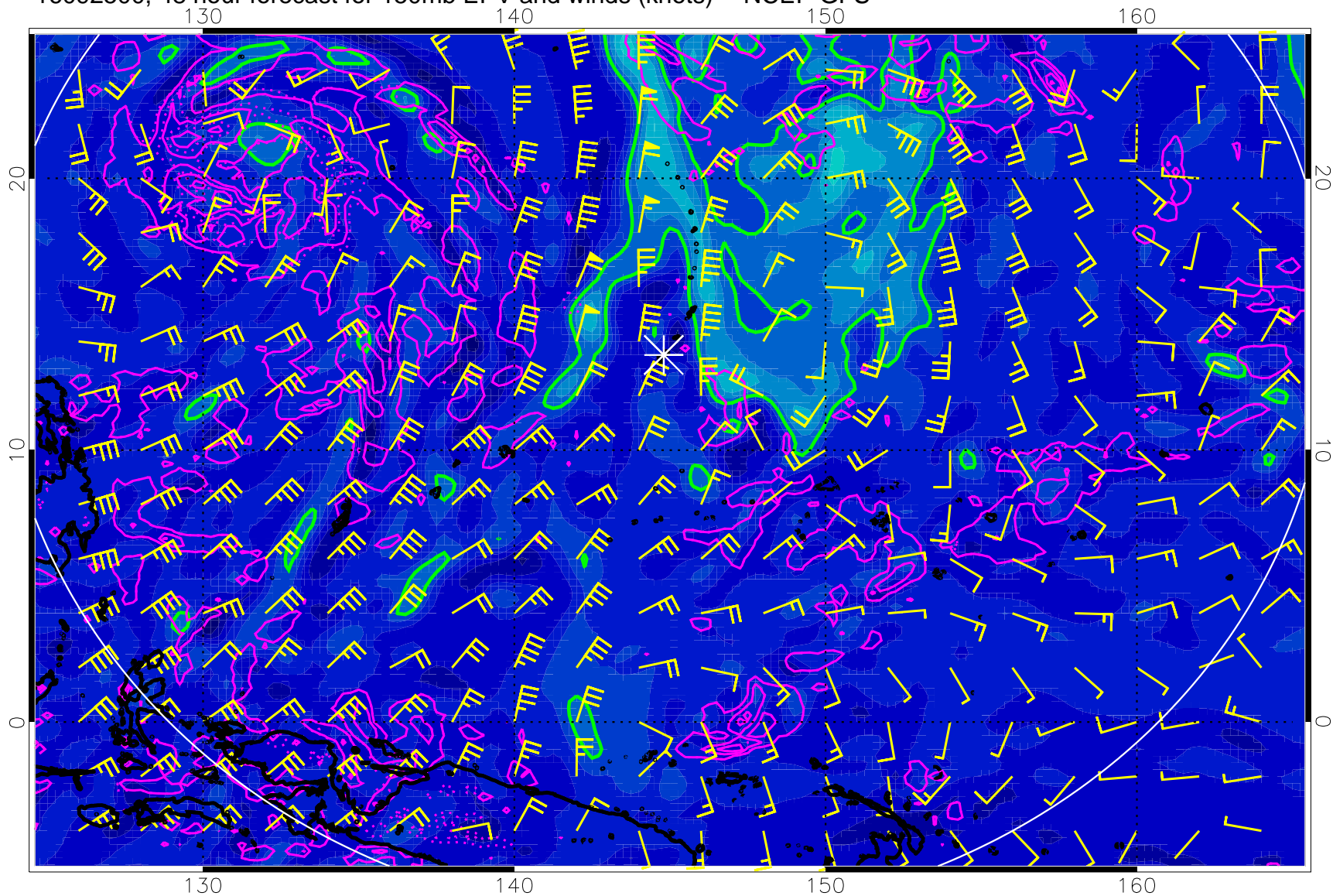
16092500, 48 hour forecast for 150mb EPV and winds (knots) -- NCEP GFS
