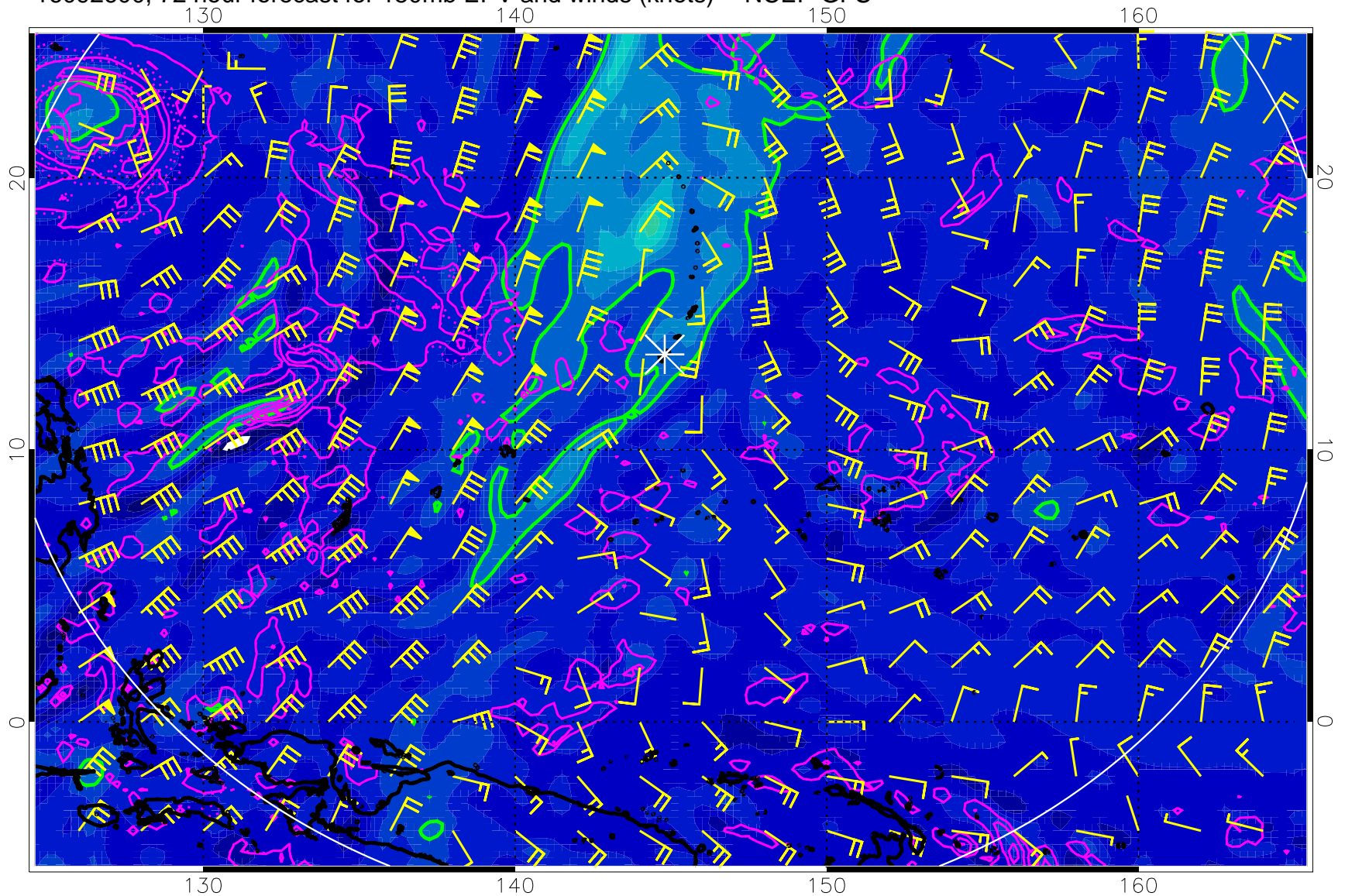
16092600, 72 hour forecast for 150mb EPV and winds (knots) -- NCEP GFS
