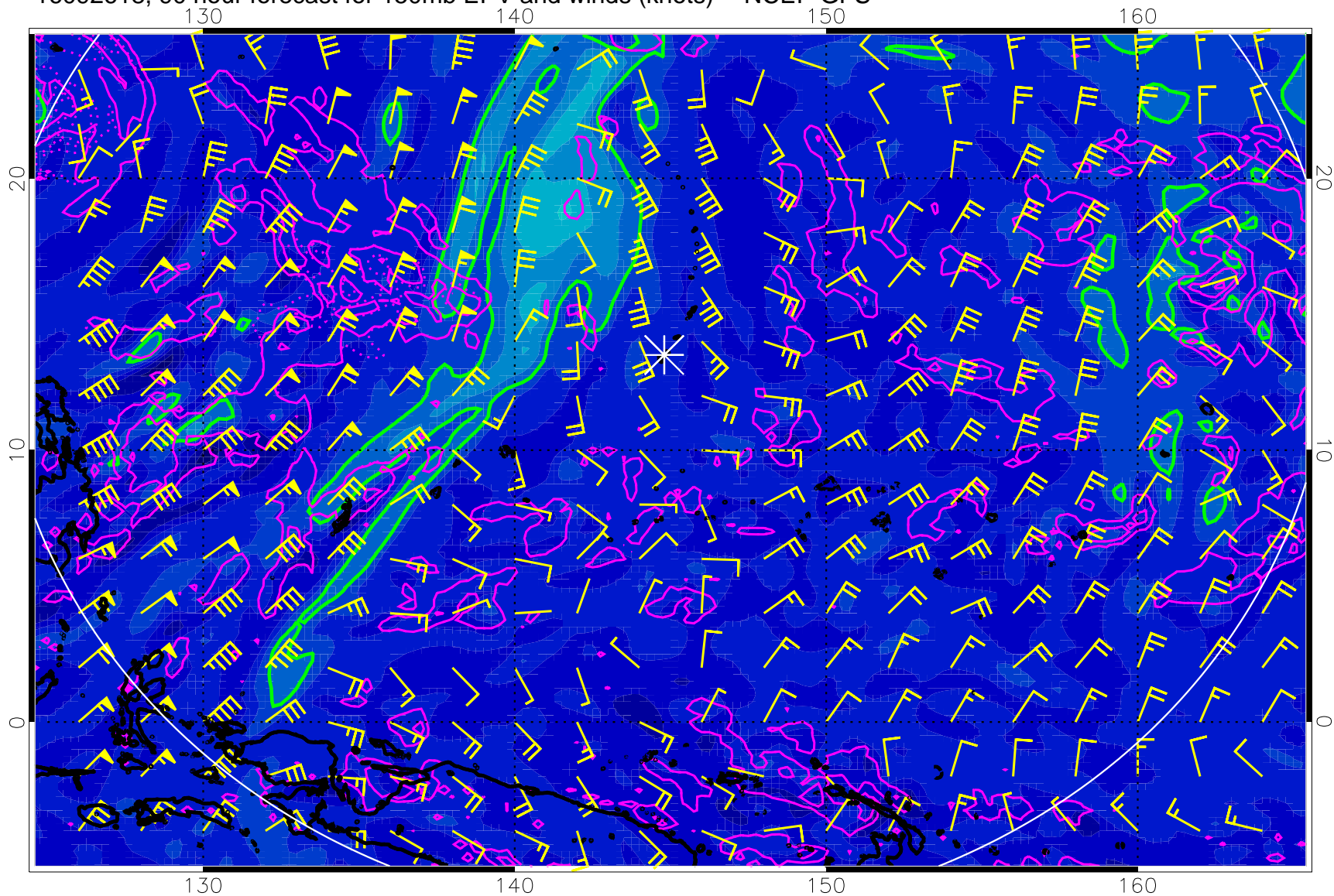
16092618, 90 hour forecast for 150mb EPV and winds (knots) -- NCEP GFS
