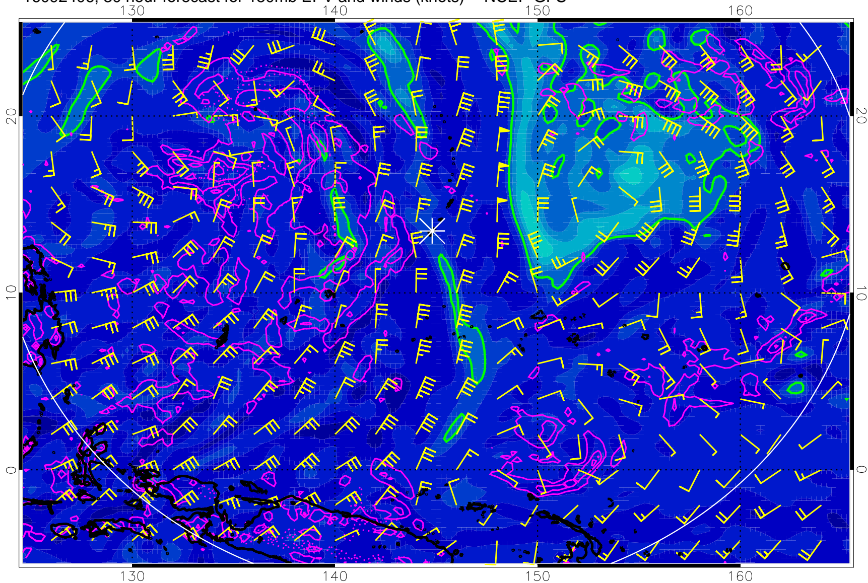
16092406, 30 hour forecast for 150mb EPV and winds (knots) -- NCEP GFS
