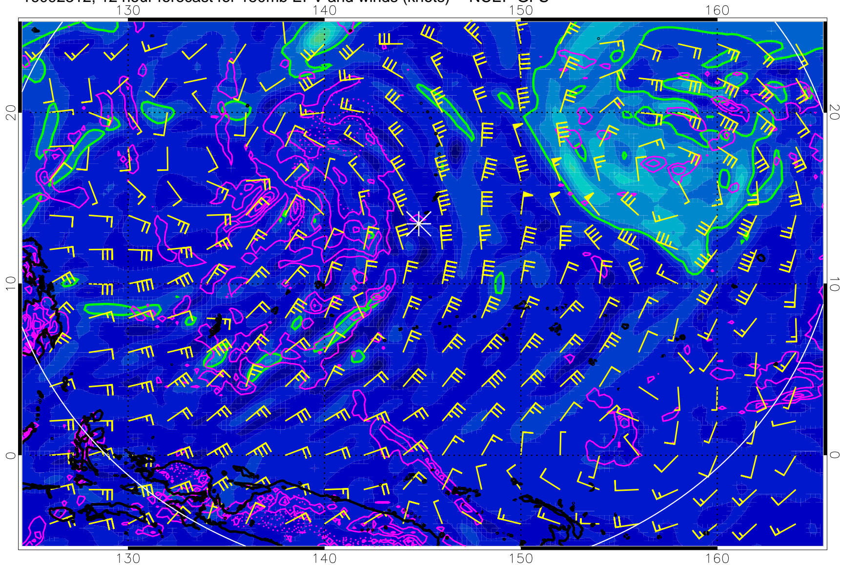
16092312, 12 hour forecast for 150mb EPV and winds (knots) -- NCEP GFS
