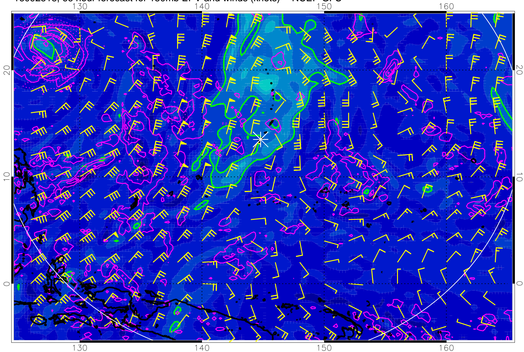
16092518, 66 hour forecast for 150mb EPV and winds (knots) -- NCEP GFS
