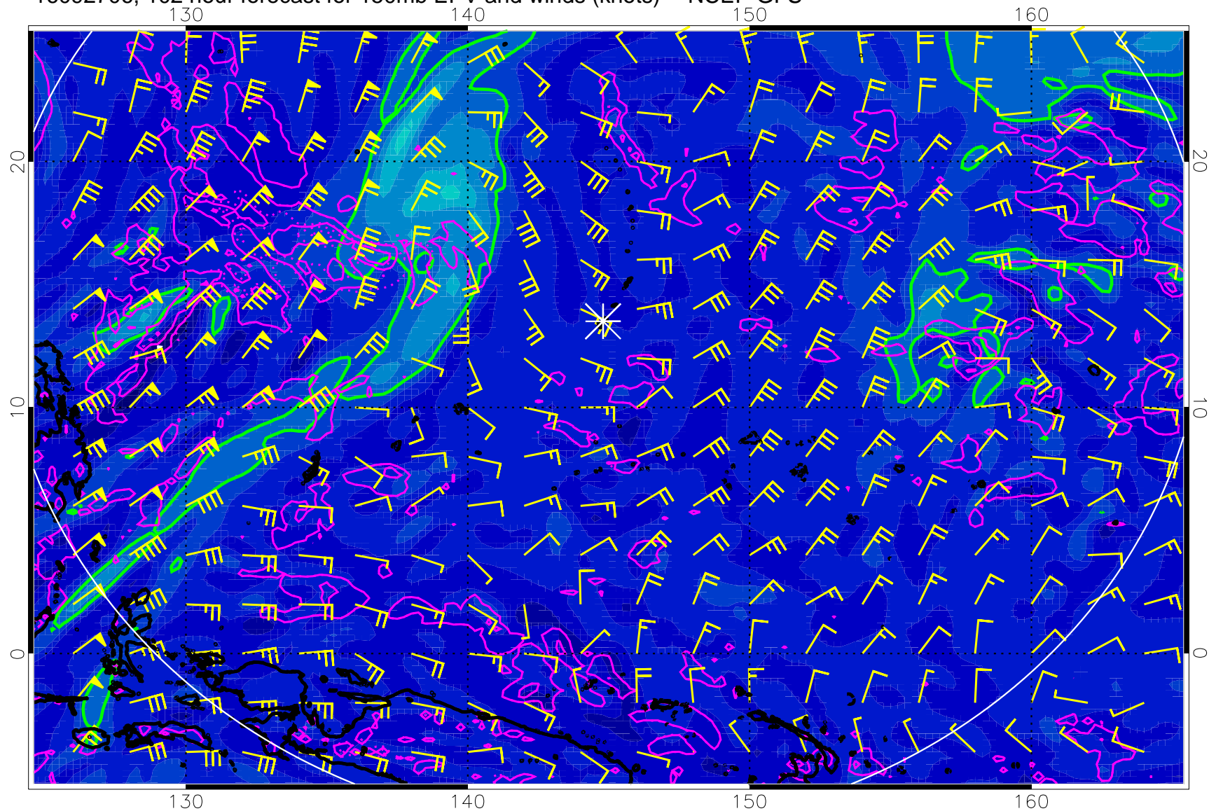
16092706, 102 hour forecast for 150mb EPV and winds (knots) -- NCEP GFS
