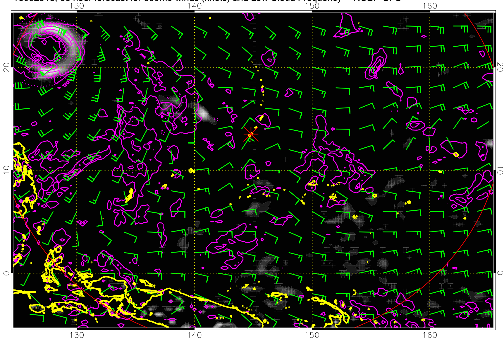
16092518, 66 hour forecast for 850mb winds (knots) and Low Cloud Frequency -- NCEP GFS
