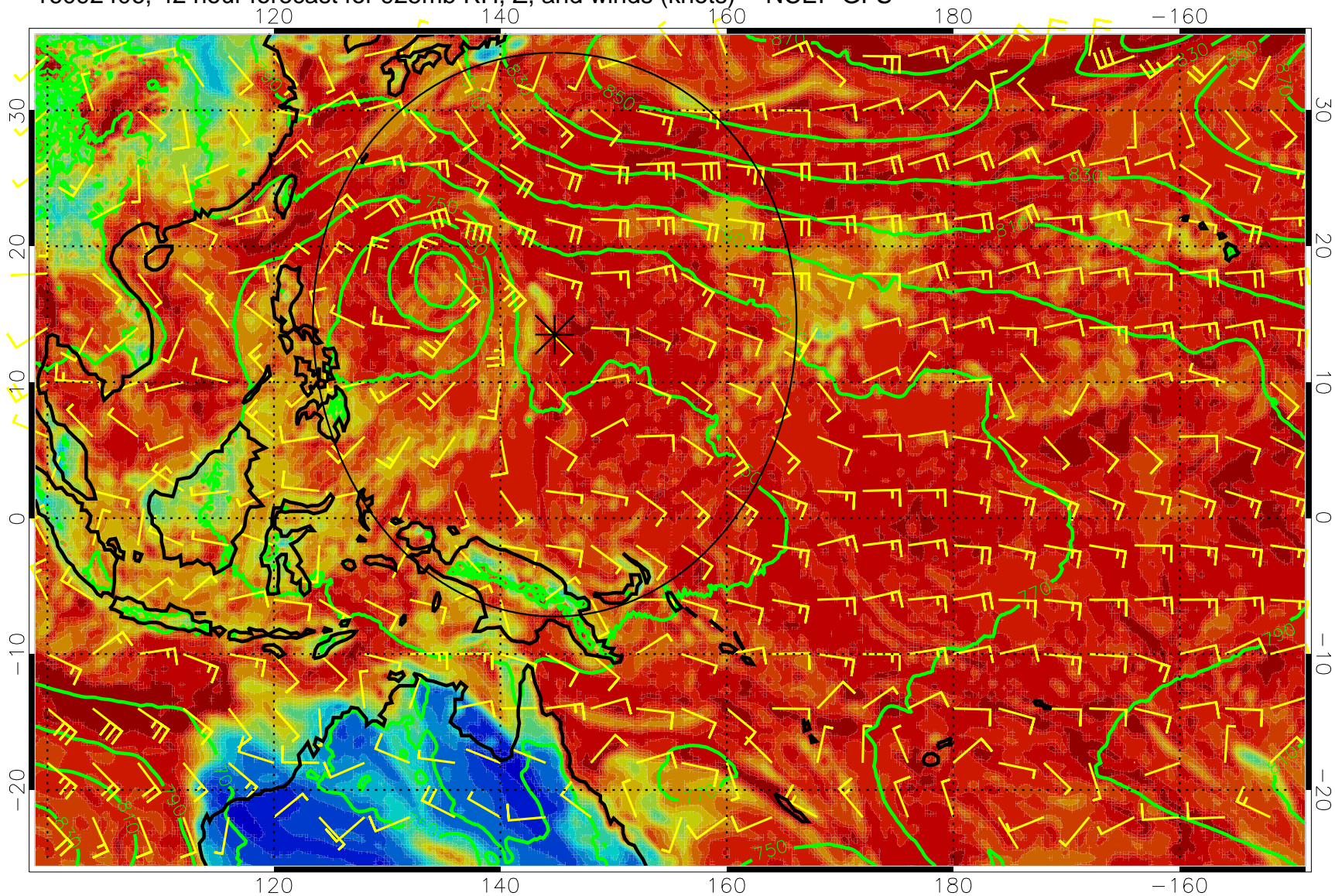
16092406, 42 hour forecast for 925mb RH, Z, and winds (knots) -- NCEP GFS
