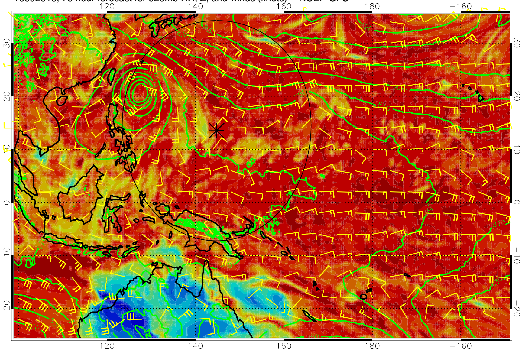
16092518, 78 hour forecast for 925mb RH, Z, and winds (knots) -- NCEP GFS
