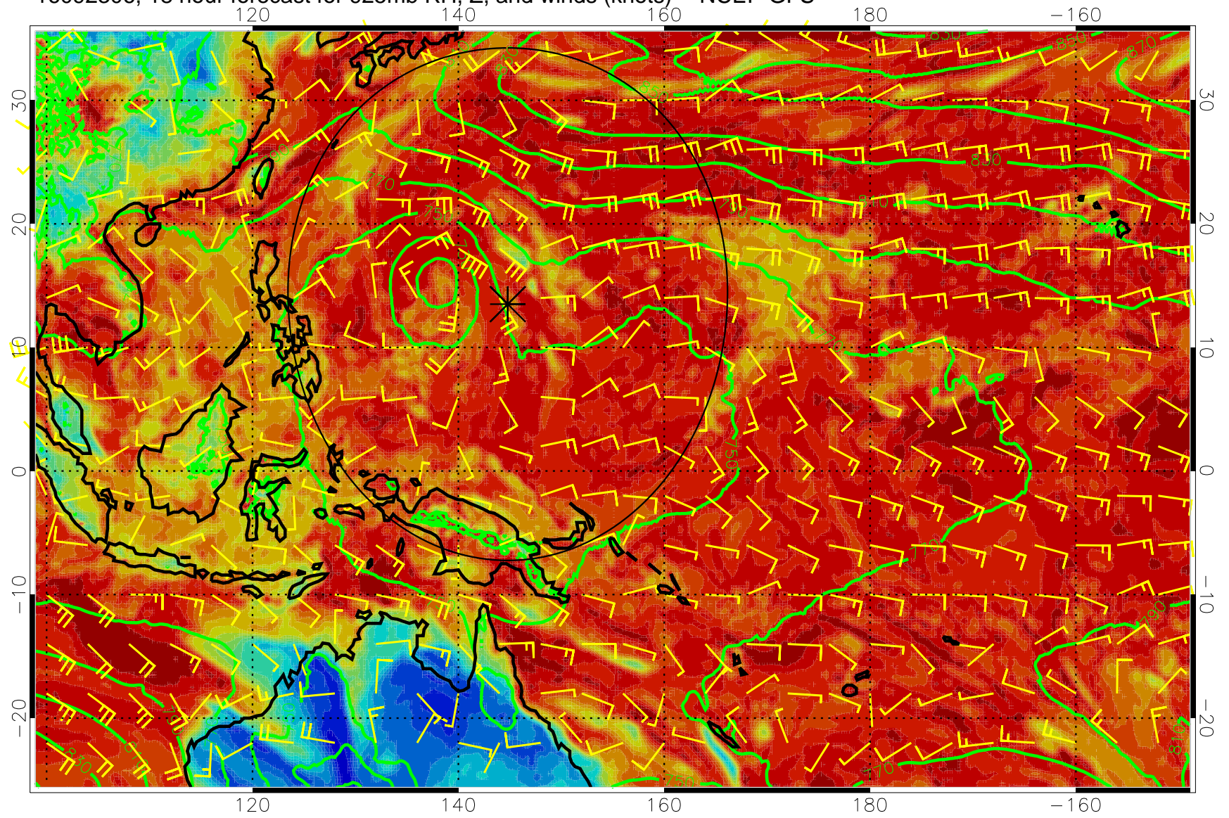
16092306, 18 hour forecast for 925mb RH, Z, and winds (knots) -- NCEP GFS
