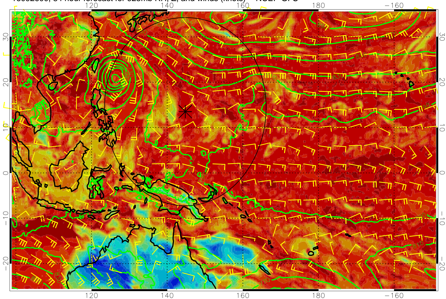
16092600, 84 hour forecast for 925mb RH, Z, and winds (knots) -- NCEP GFS
