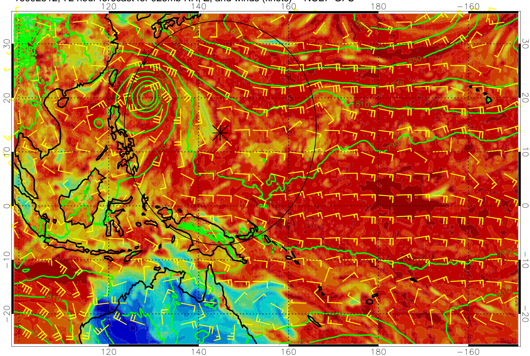
16092512, 72 hour forecast for 925mb RH, Z, and winds (knots) -- NCEP GFS
