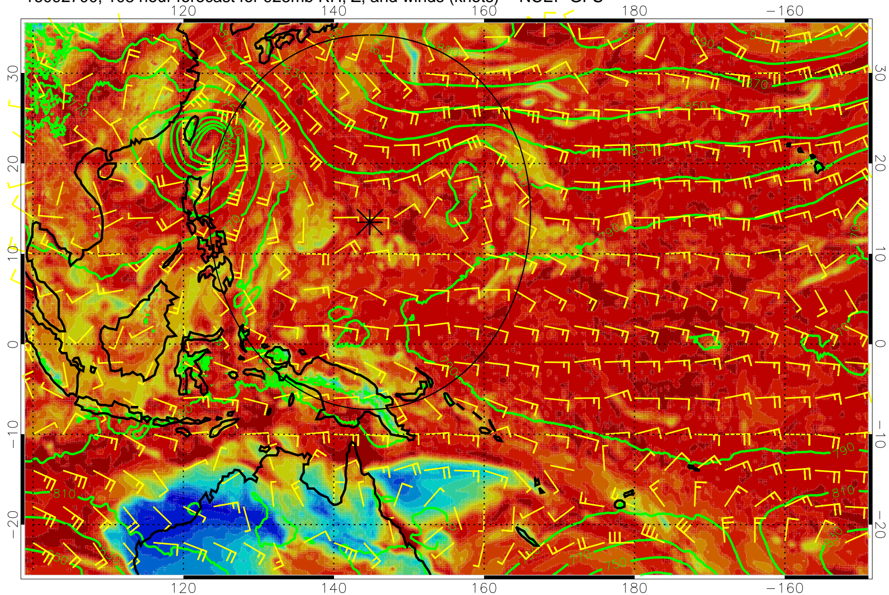
16092700, 108 hour forecast for 925mb RH, Z, and winds (knots) -- NCEP GFS
