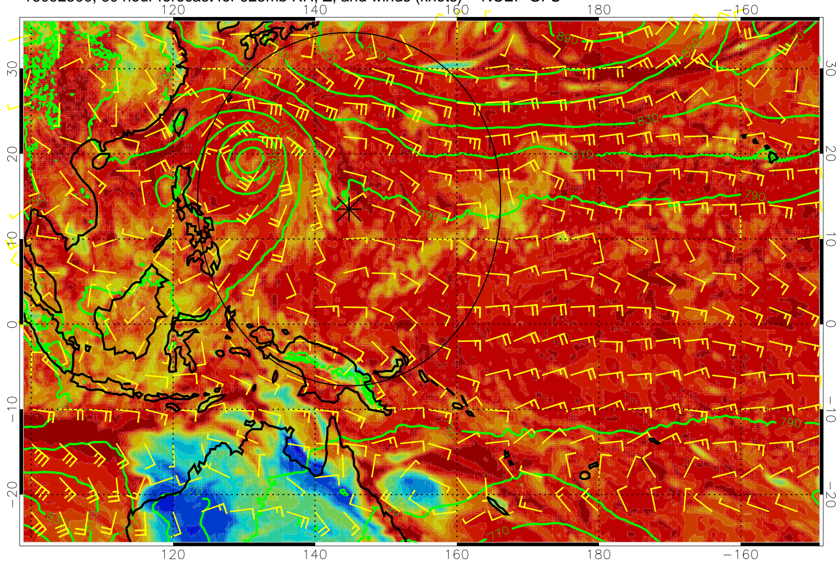
16092500, 60 hour forecast for 925mb RH, Z, and winds (knots) -- NCEP GFS
