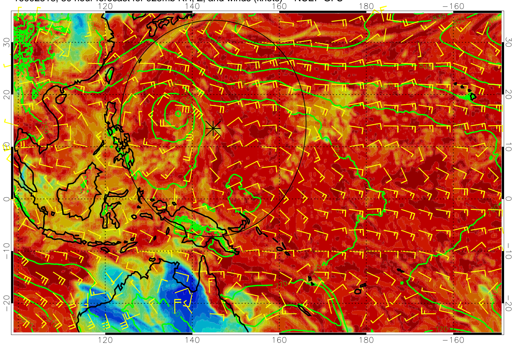
16092318, 30 hour forecast for 925mb RH, Z, and winds (knots) -- NCEP GFS
