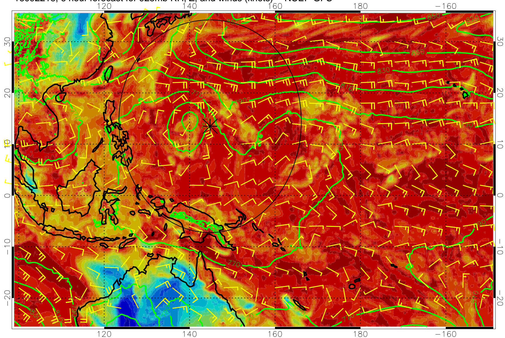
16092218, 6 hour forecast for 925mb RH, Z, and winds (knots) -- NCEP GFS
