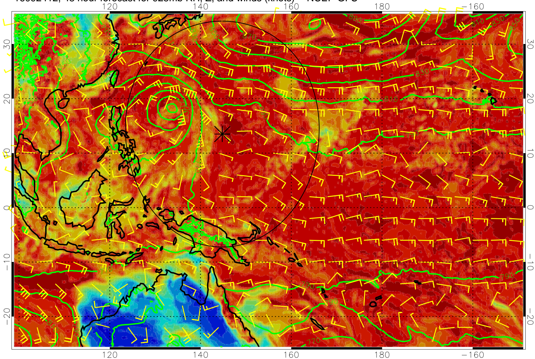
16092412, 48 hour forecast for 925mb RH, Z, and winds (knots) -- NCEP GFS
