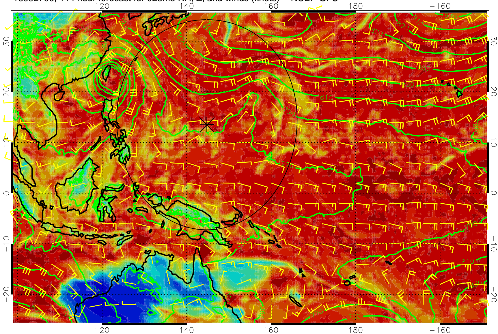
16092706, 114 hour forecast for 925mb RH, Z, and winds (knots) -- NCEP GFS
