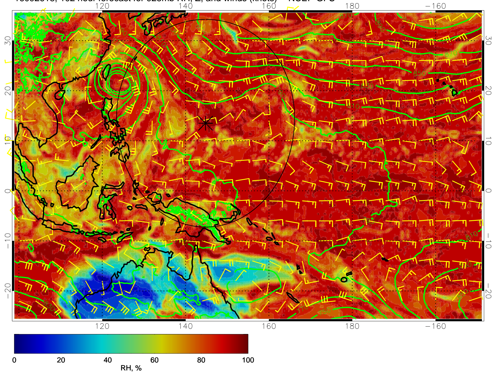
16092618, 102 hour forecast for 925mb RH, Z, and winds (knots) -- NCEP GFS
