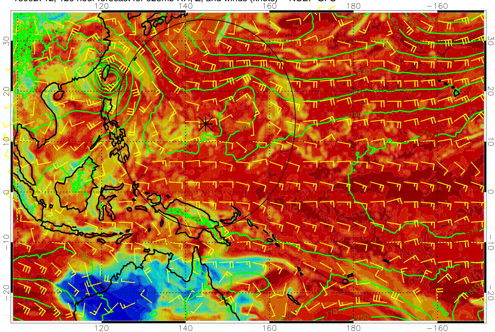
16092712, 120 hour forecast for 925mb RH, Z, and winds (knots) -- NCEP GFS
