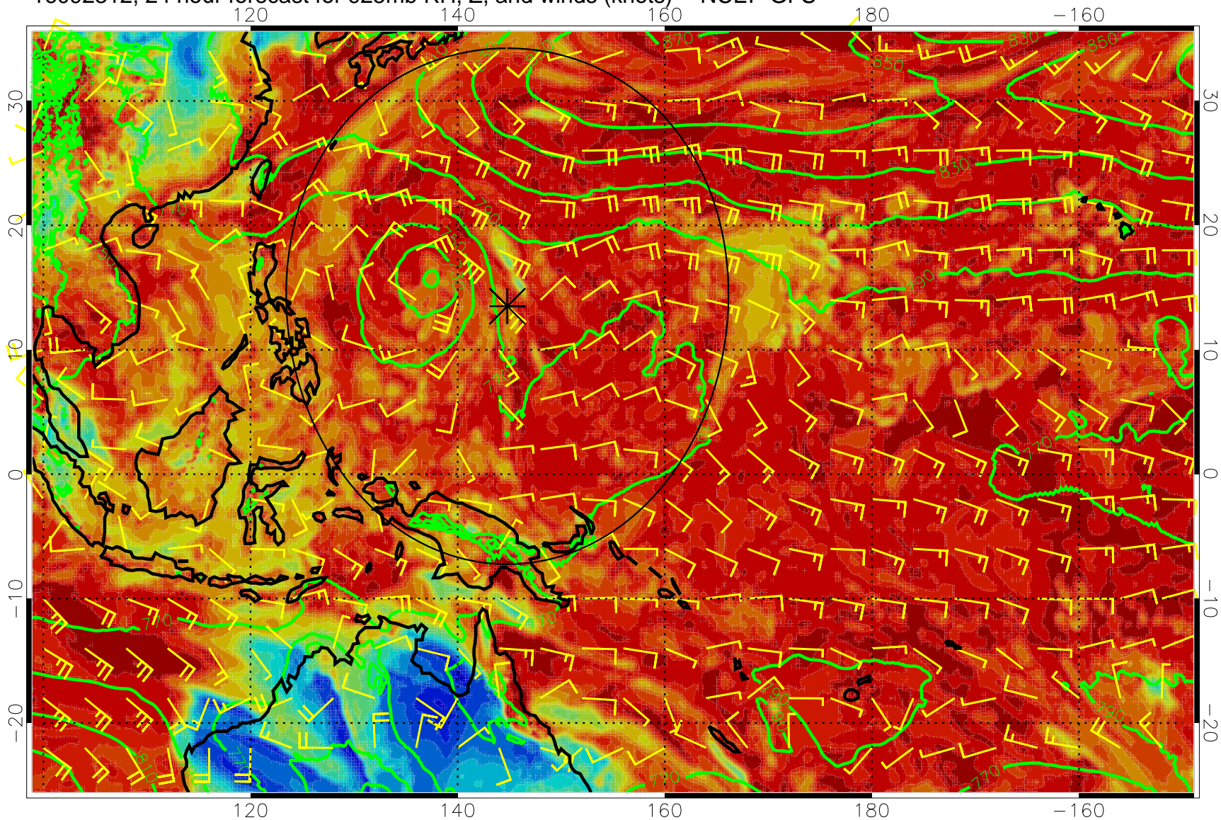
16092312, 24 hour forecast for 925mb RH, Z, and winds (knots) -- NCEP GFS
