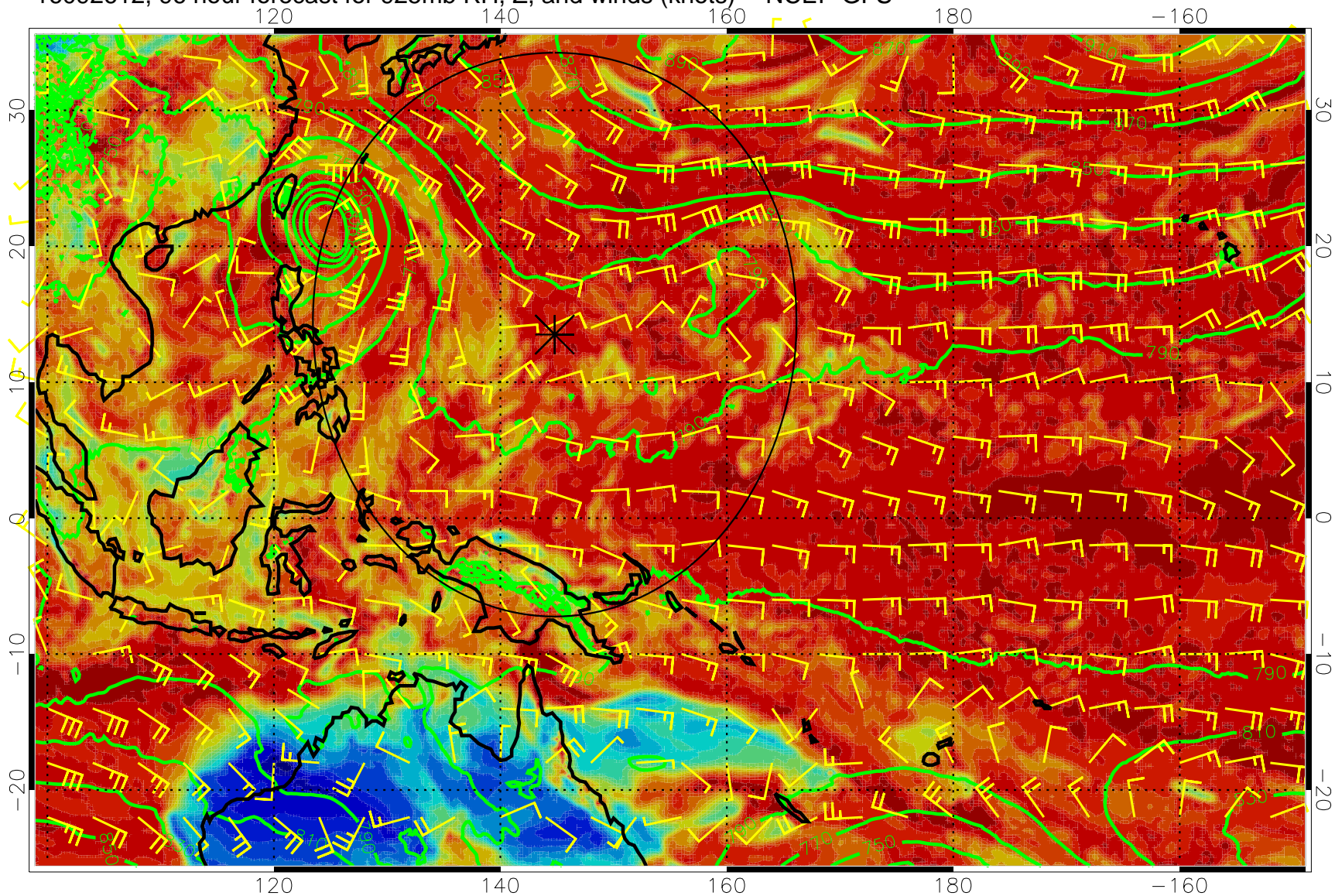
16092612, 96 hour forecast for 925mb RH, Z, and winds (knots) -- NCEP GFS
