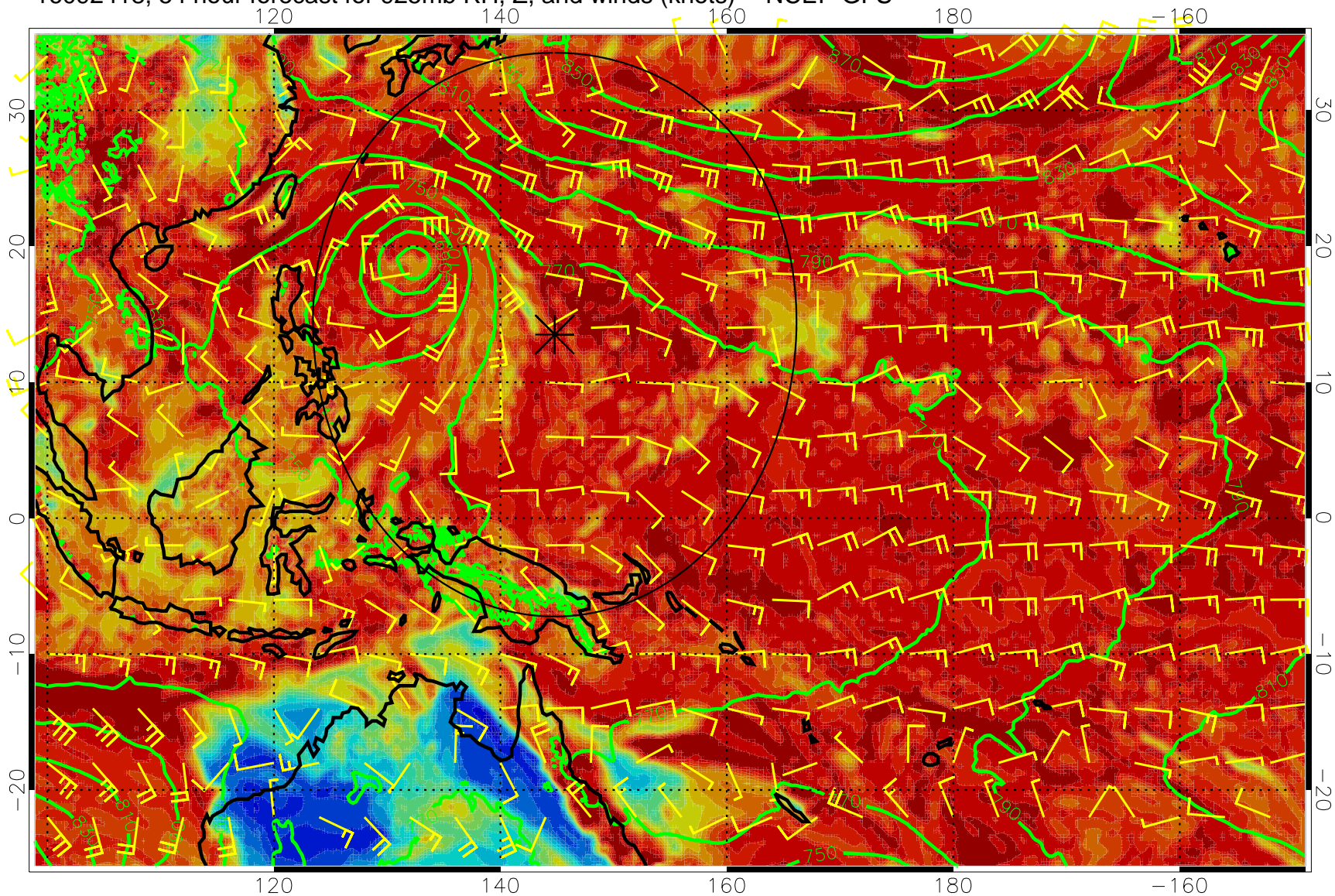
16092418, 54 hour forecast for 925mb RH, Z, and winds (knots) -- NCEP GFS
