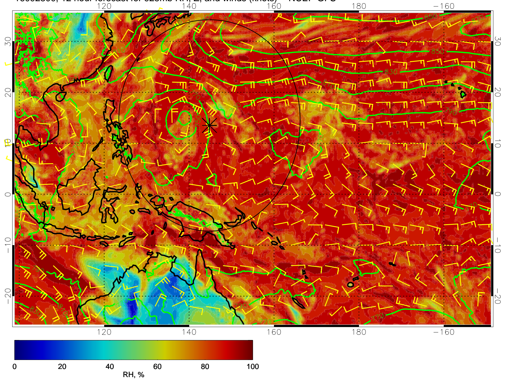
16092300, 12 hour forecast for 925mb RH, Z, and winds (knots) -- NCEP GFS
