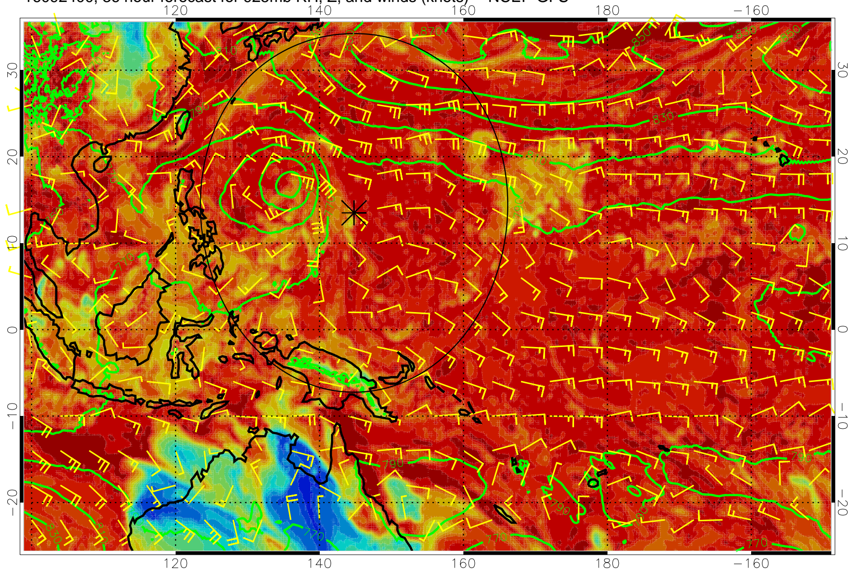
16092400, 36 hour forecast for 925mb RH, Z, and winds (knots) -- NCEP GFS
