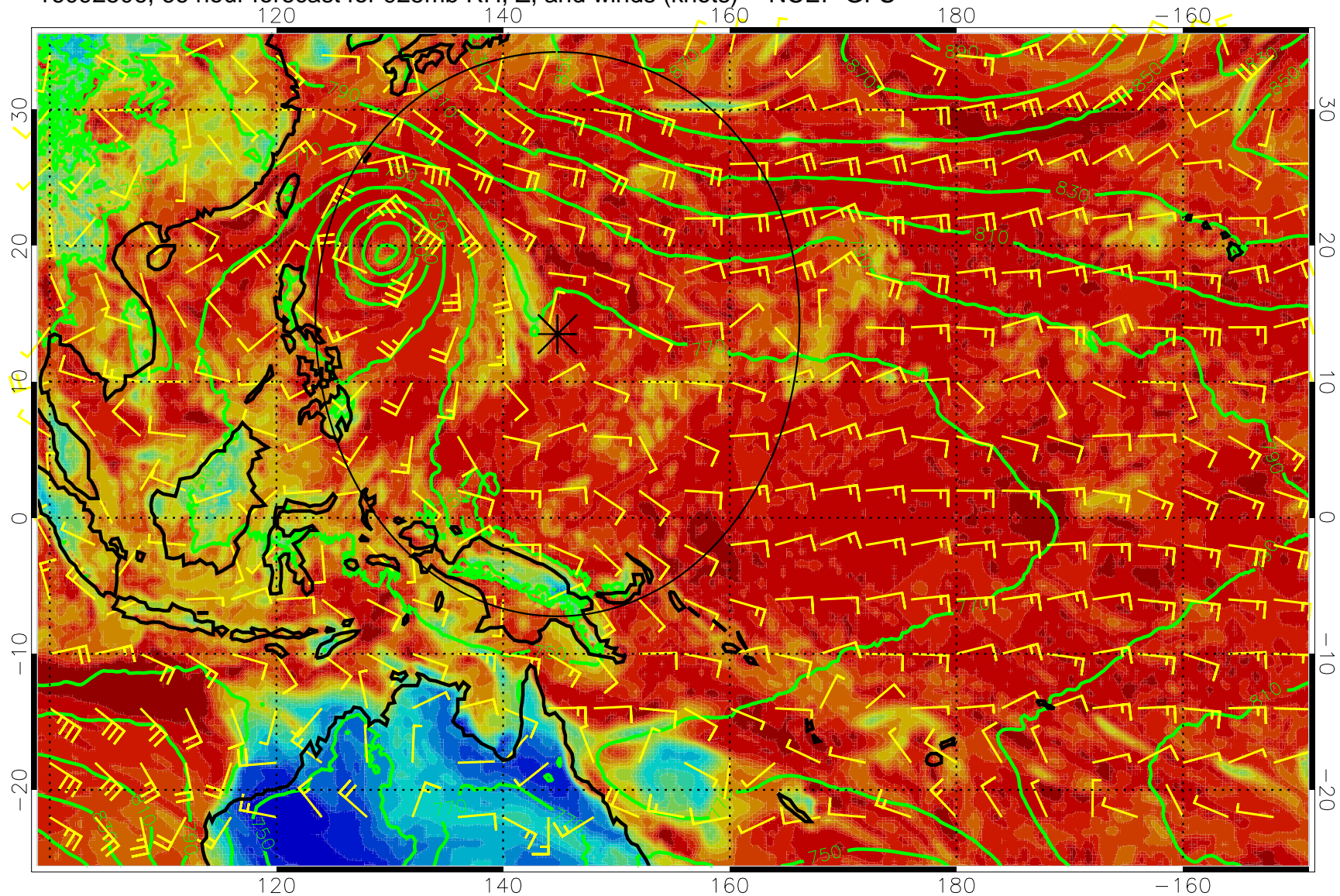
16092506, 66 hour forecast for 925mb RH, Z, and winds (knots) -- NCEP GFS
