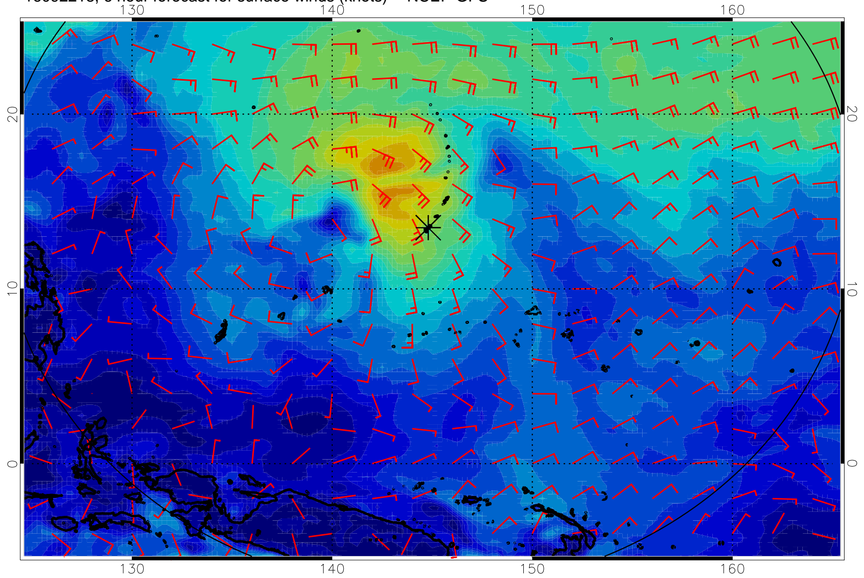
16092218, 6 hour forecast for surface winds (knots) -- NCEP GFS
