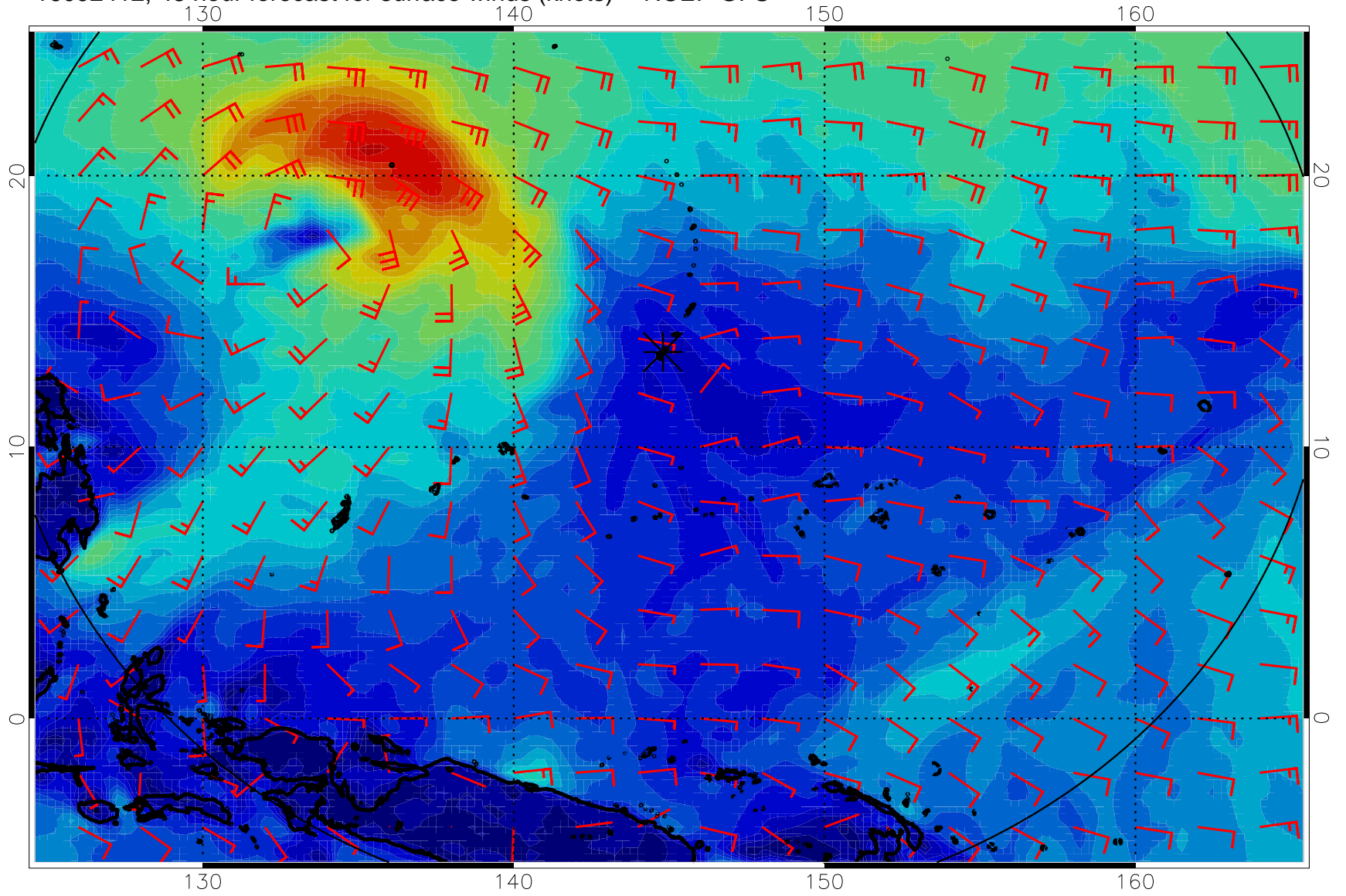
16092412, 48 hour forecast for surface winds (knots) -- NCEP GFS
