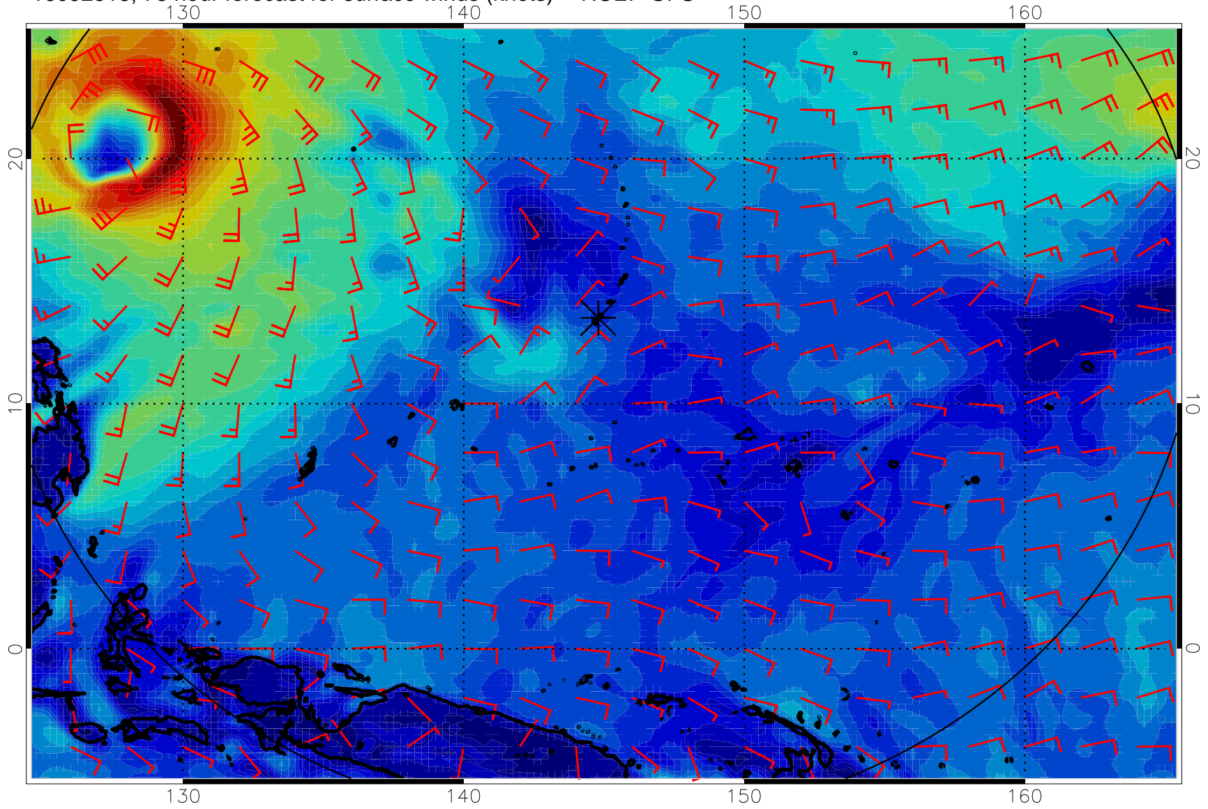
16092518, 78 hour forecast for surface winds (knots) -- NCEP GFS
