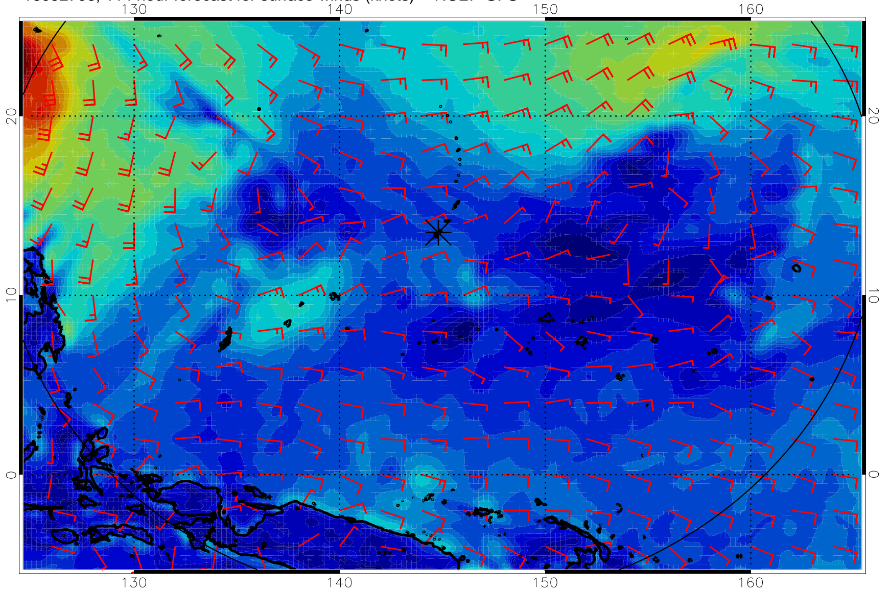
16092706, 114 hour forecast for surface winds (knots) -- NCEP GFS
