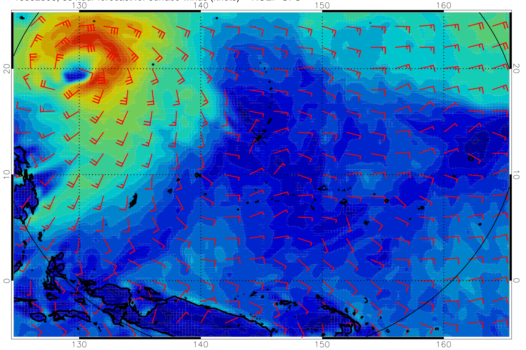
16092506, 66 hour forecast for surface winds (knots) -- NCEP GFS
