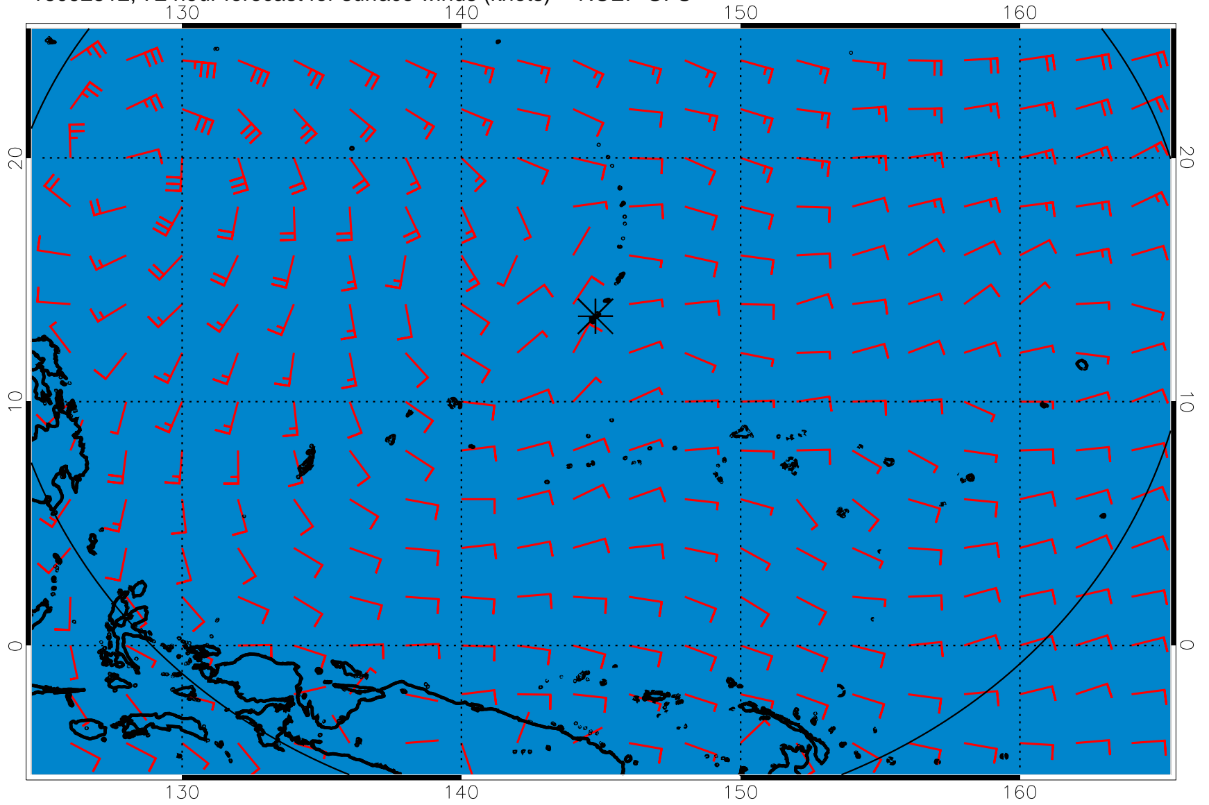
16092512, 72 hour forecast for surface winds (knots) -- NCEP GFS
