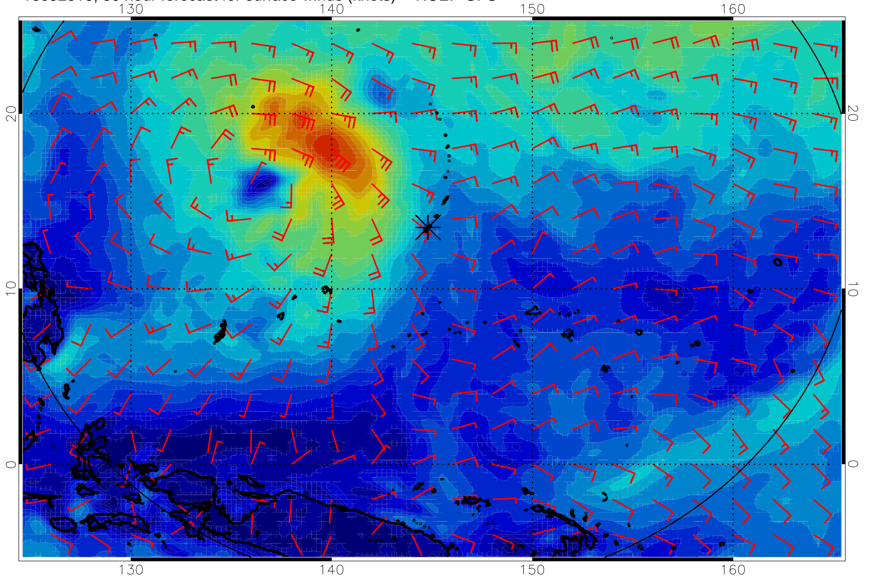
16092318, 30 hour forecast for surface winds (knots) -- NCEP GFS
