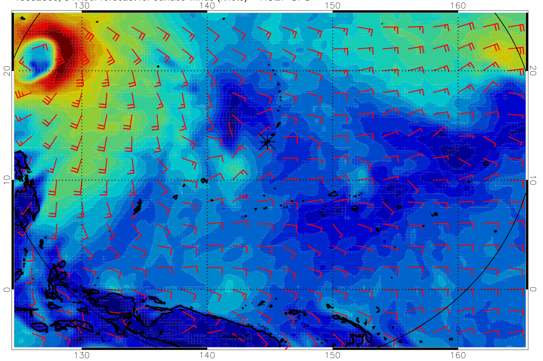
16092600, 84 hour forecast for surface winds (knots) -- NCEP GFS
