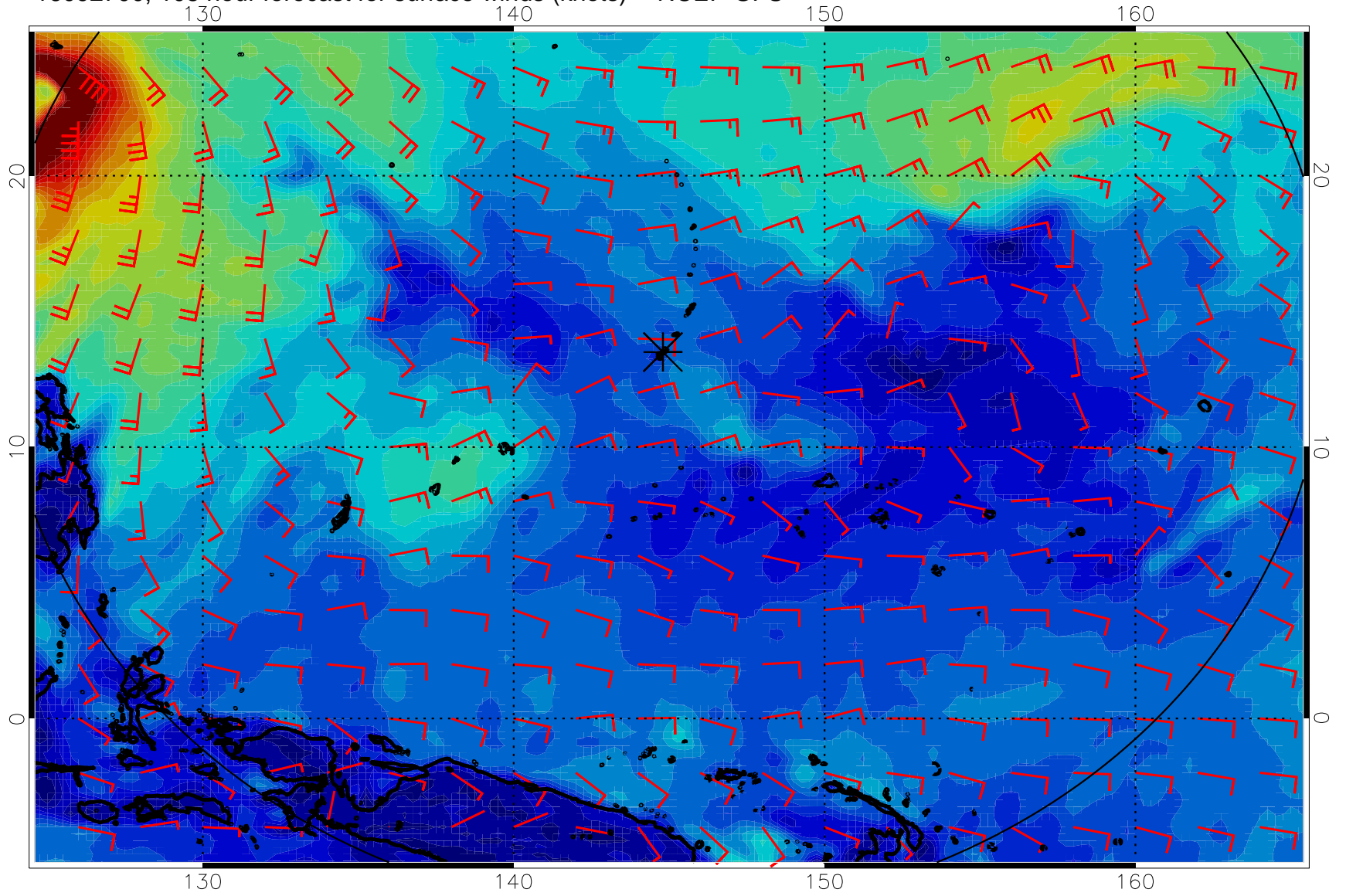
16092700, 108 hour forecast for surface winds (knots) -- NCEP GFS
