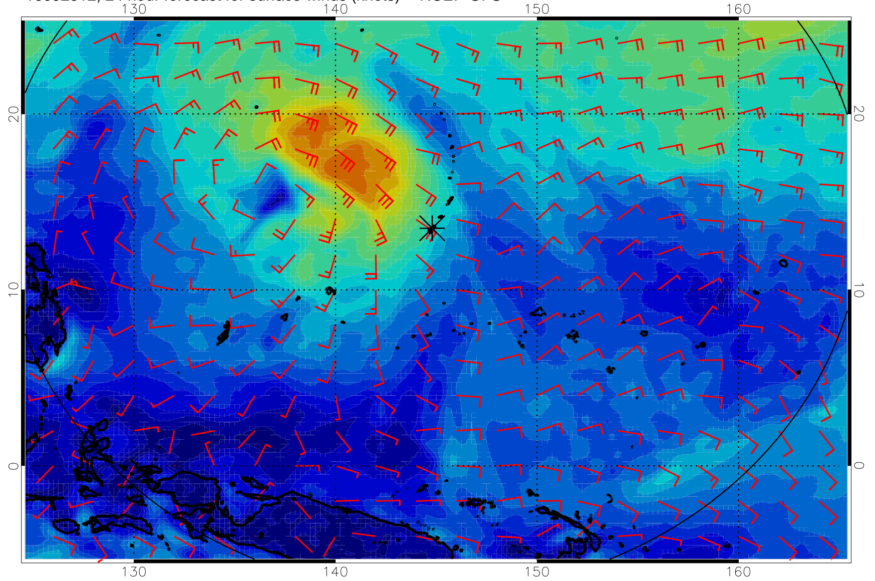
16092312, 24 hour forecast for surface winds (knots) -- NCEP GFS
