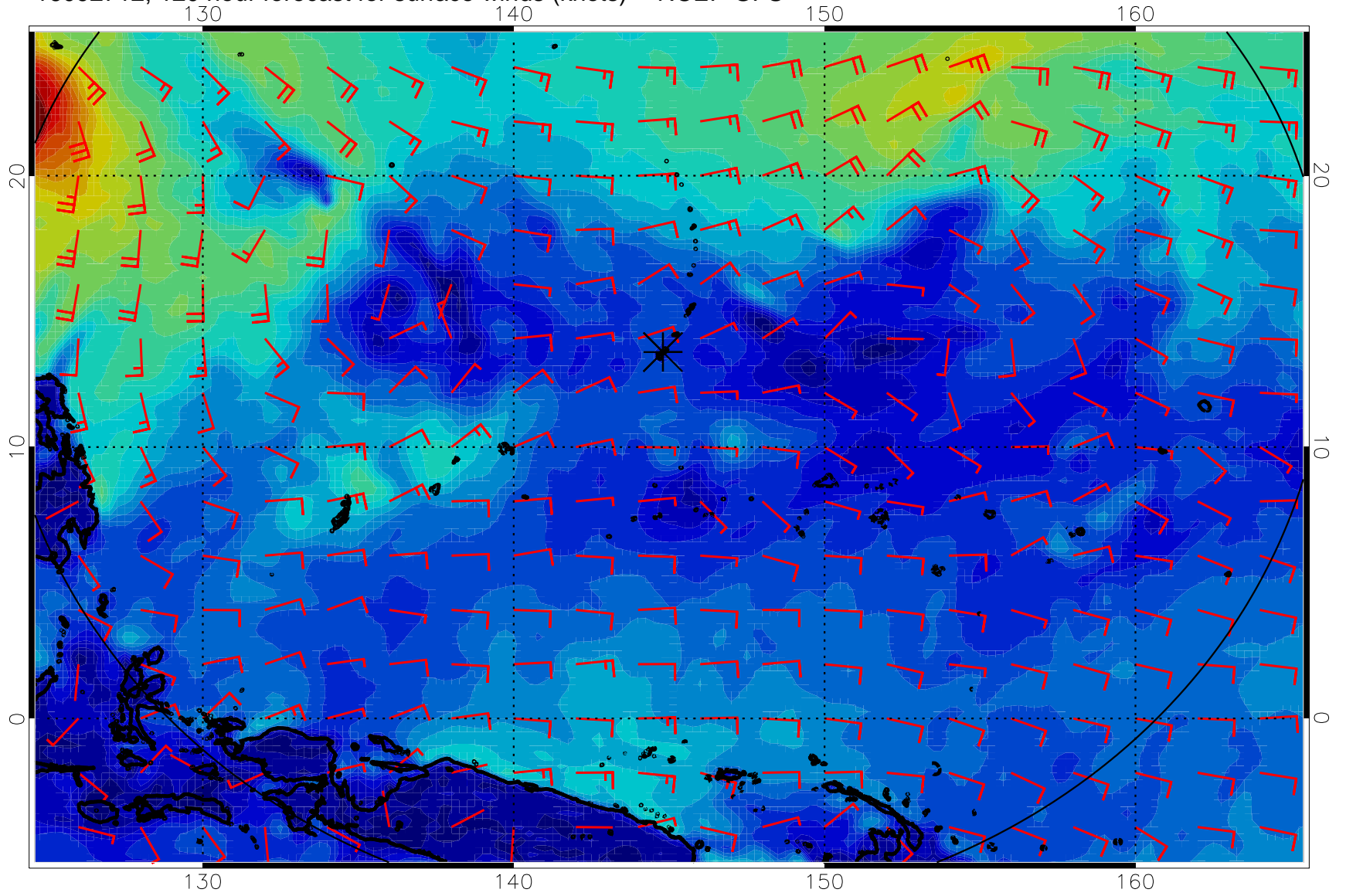
16092712, 120 hour forecast for surface winds (knots) -- NCEP GFS
