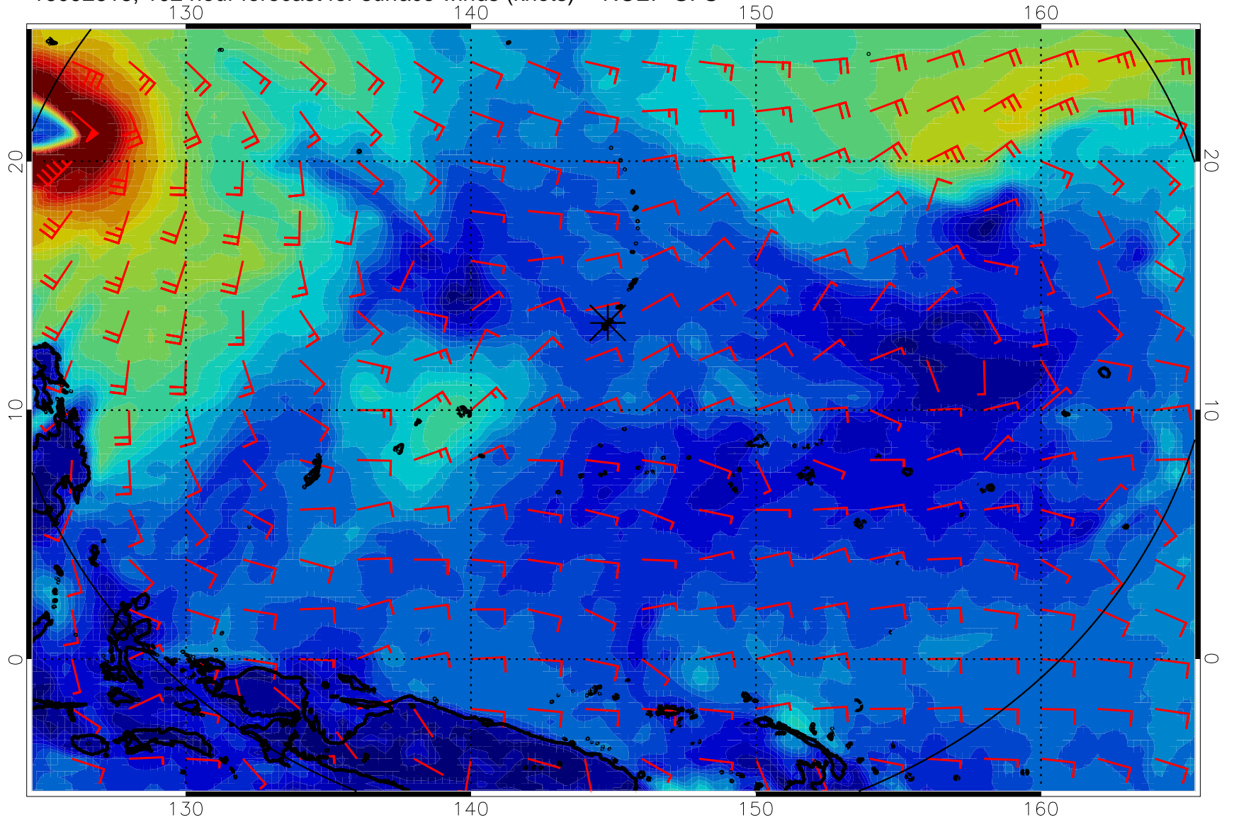
16092618, 102 hour forecast for surface winds (knots) -- NCEP GFS
