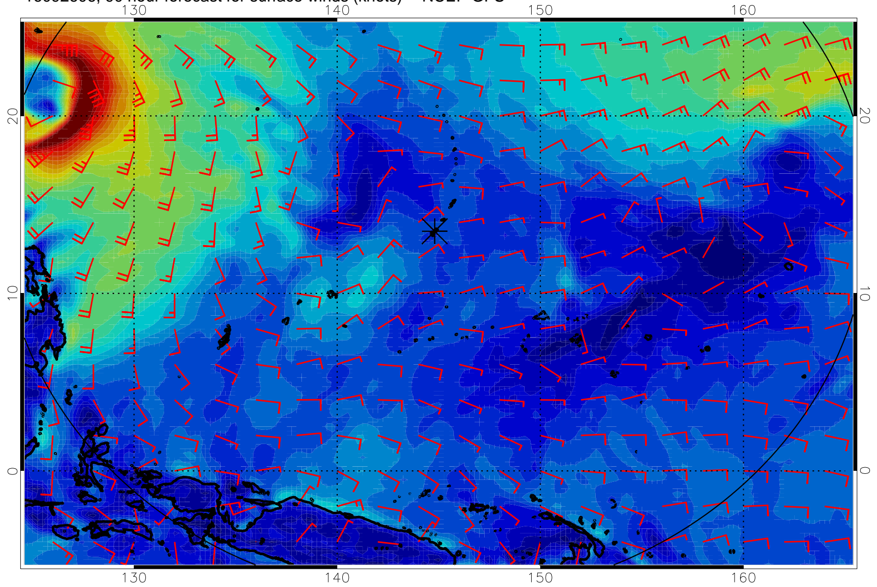
16092606, 90 hour forecast for surface winds (knots) -- NCEP GFS
