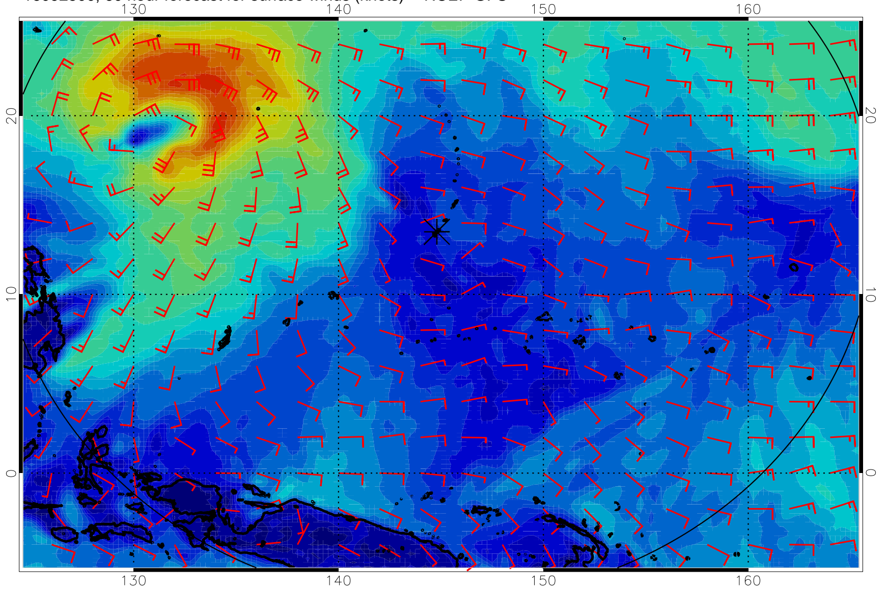
16092500, 60 hour forecast for surface winds (knots) -- NCEP GFS
