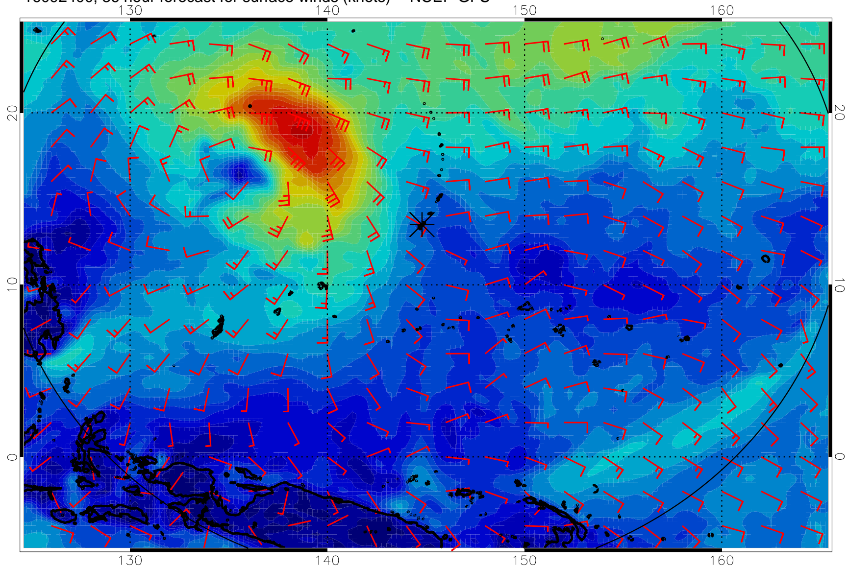
16092400, 36 hour forecast for surface winds (knots) -- NCEP GFS
