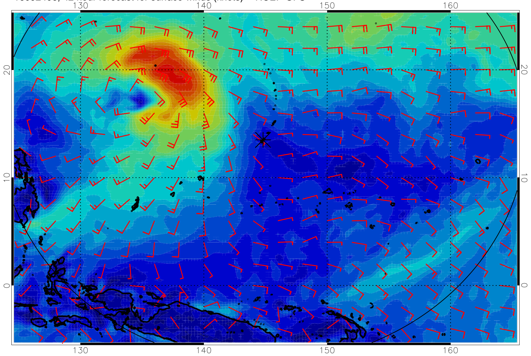
16092406, 42 hour forecast for surface winds (knots) -- NCEP GFS
