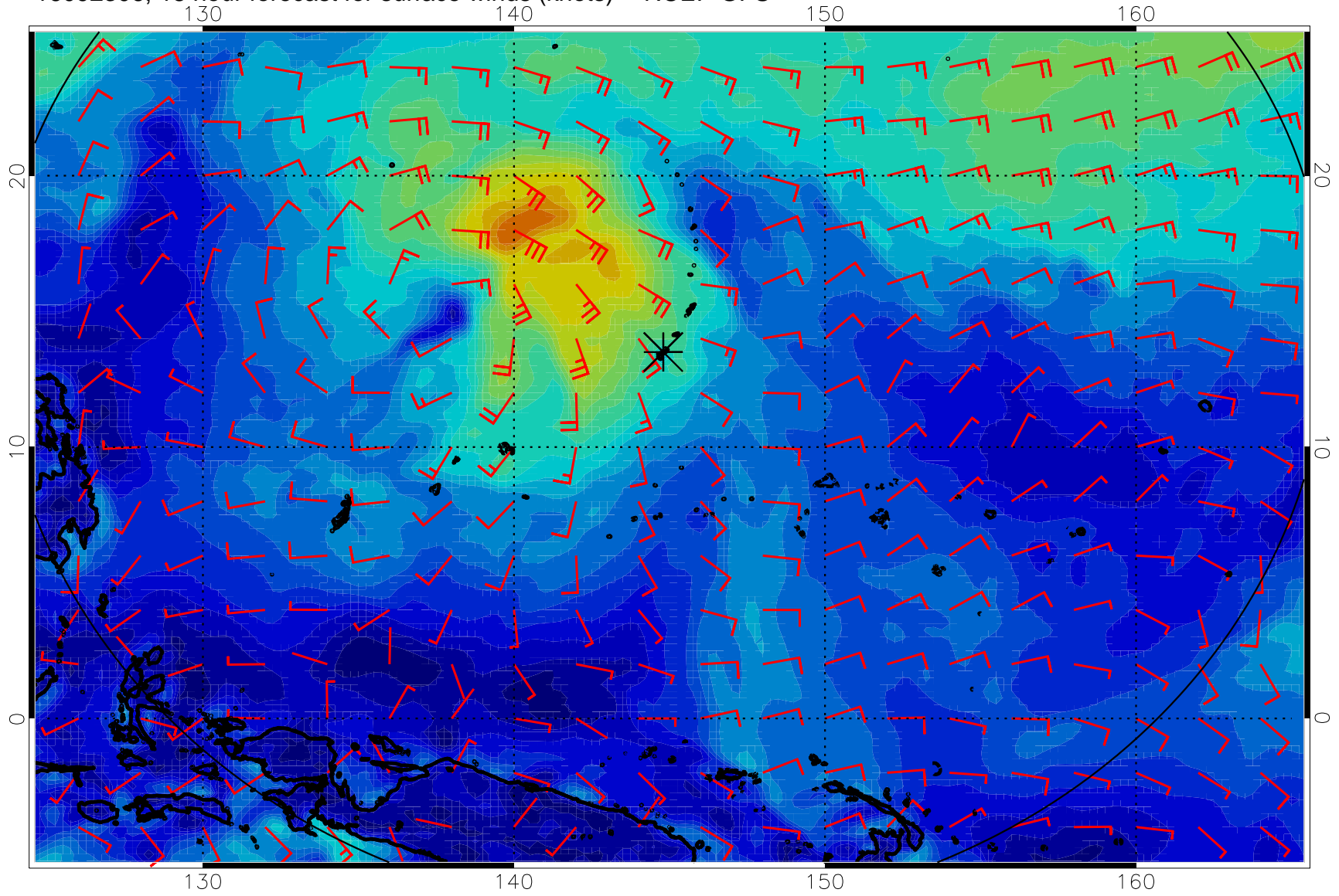
16092306, 18 hour forecast for surface winds (knots) -- NCEP GFS
