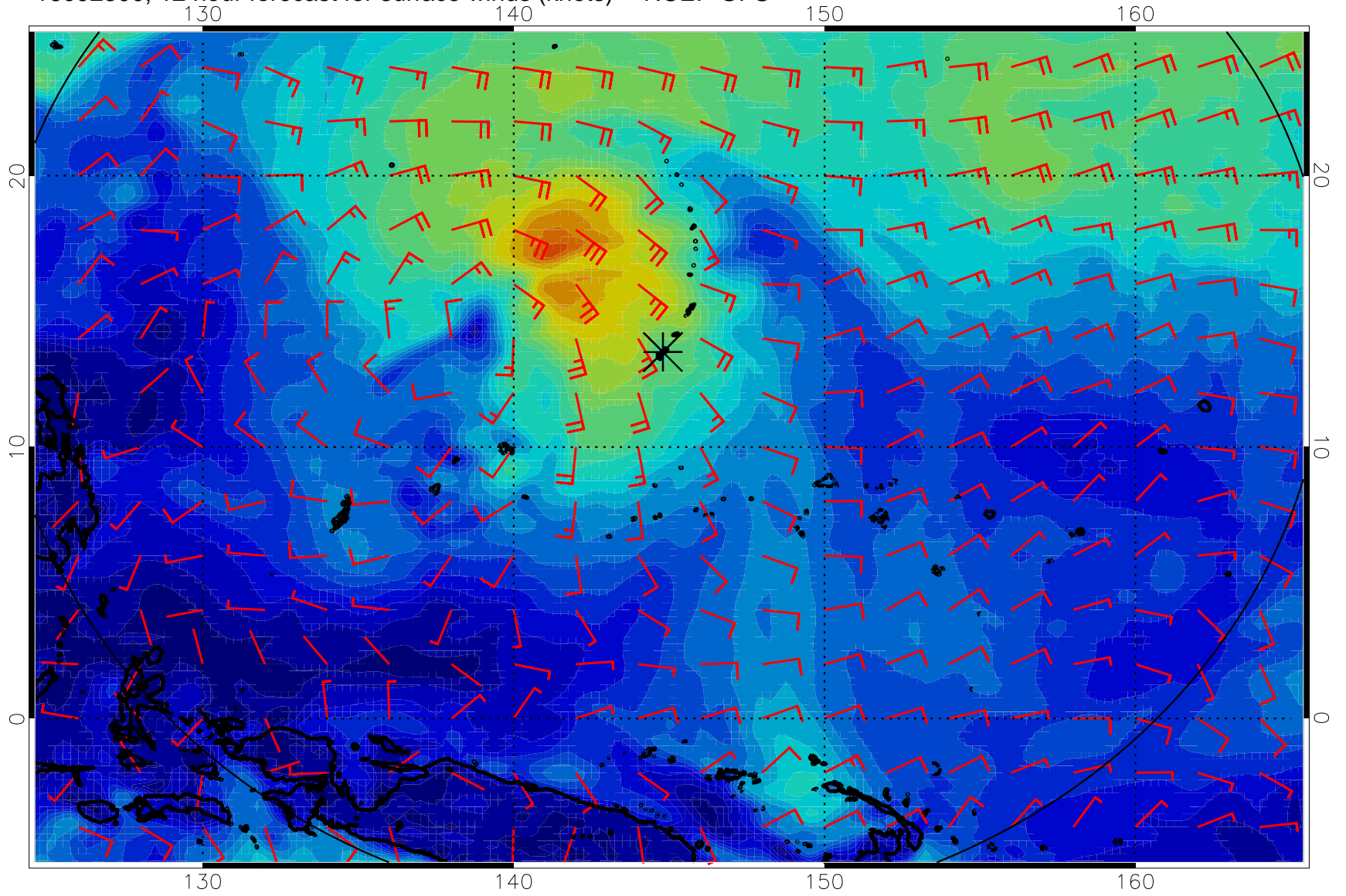
16092300, 12 hour forecast for surface winds (knots) -- NCEP GFS
