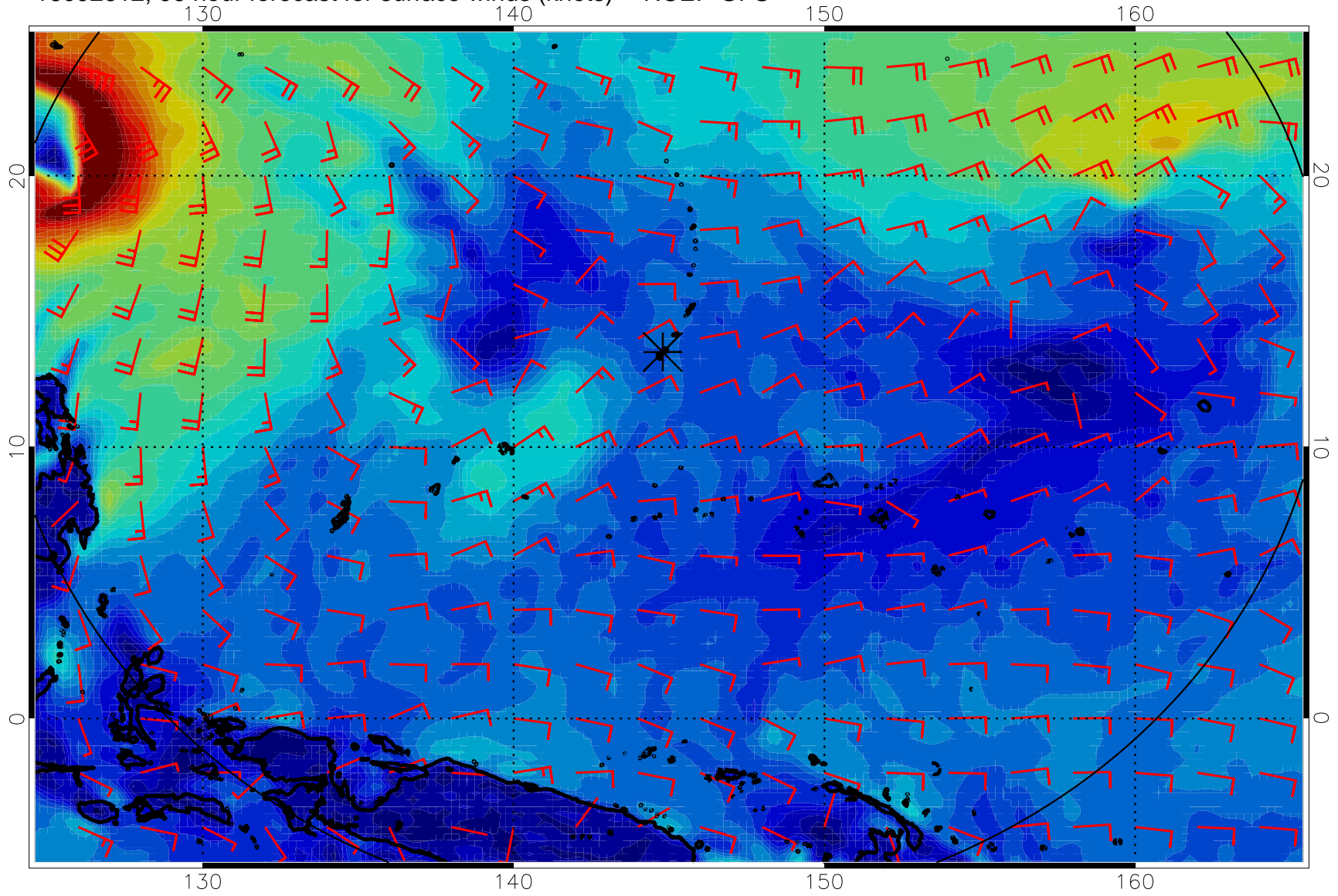
16092612, 96 hour forecast for surface winds (knots) -- NCEP GFS
