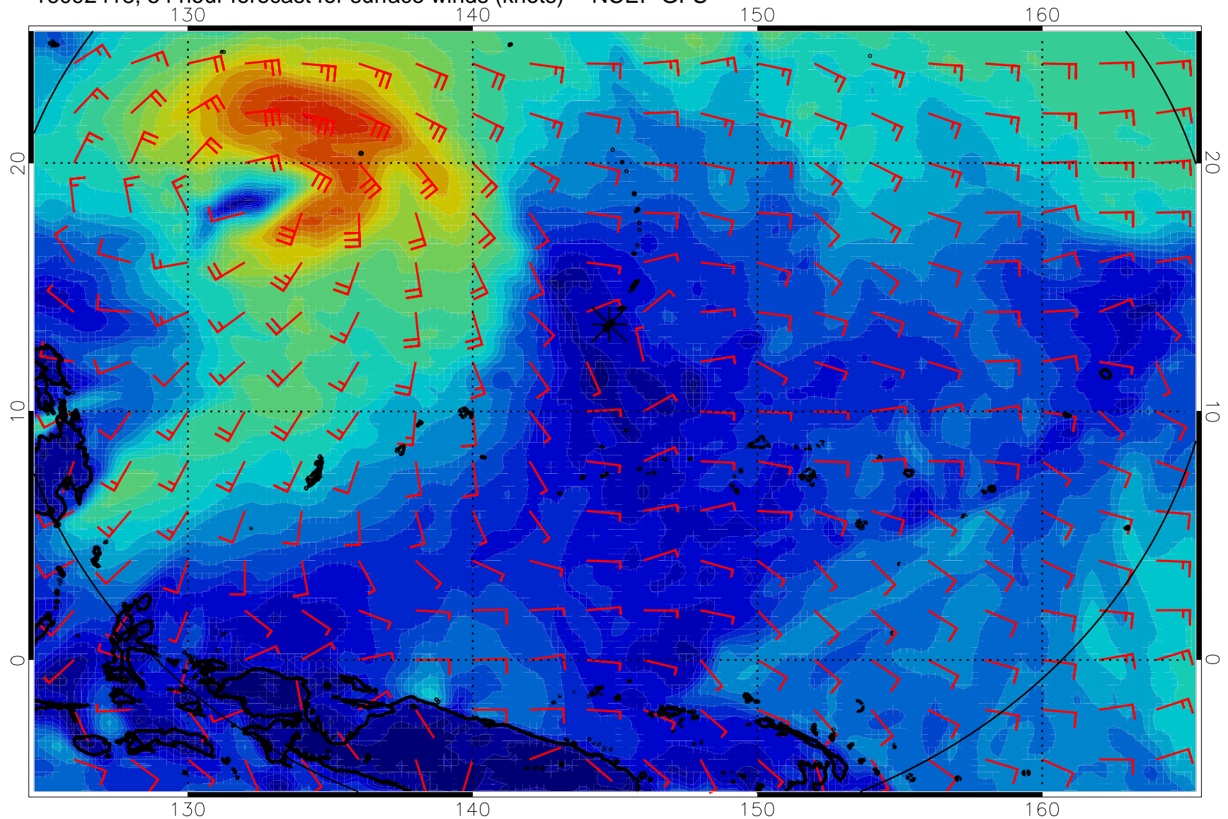
16092418, 54 hour forecast for surface winds (knots) -- NCEP GFS
