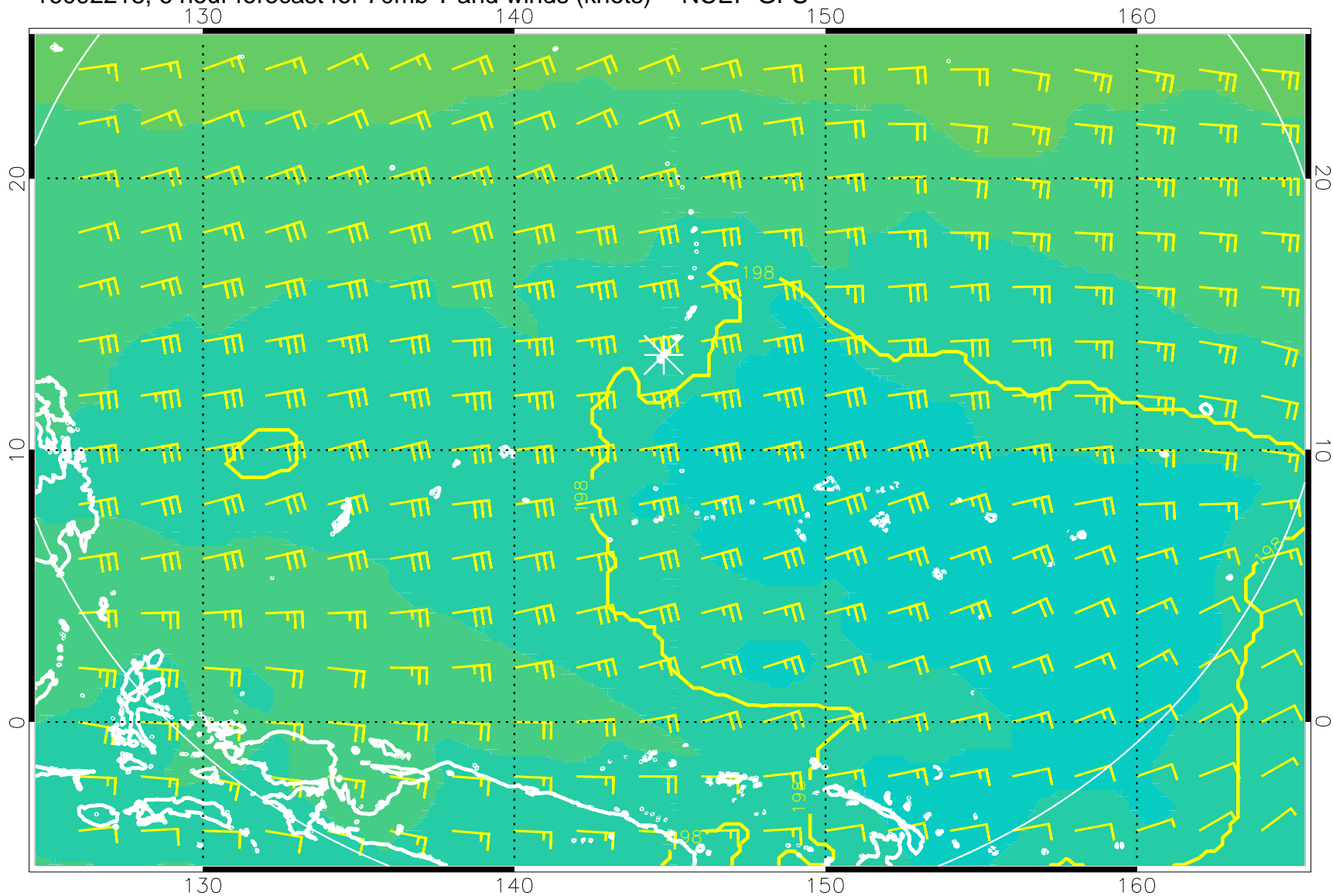
16092218, 6 hour forecast for 70mb T and winds (knots) -- NCEP GFS
