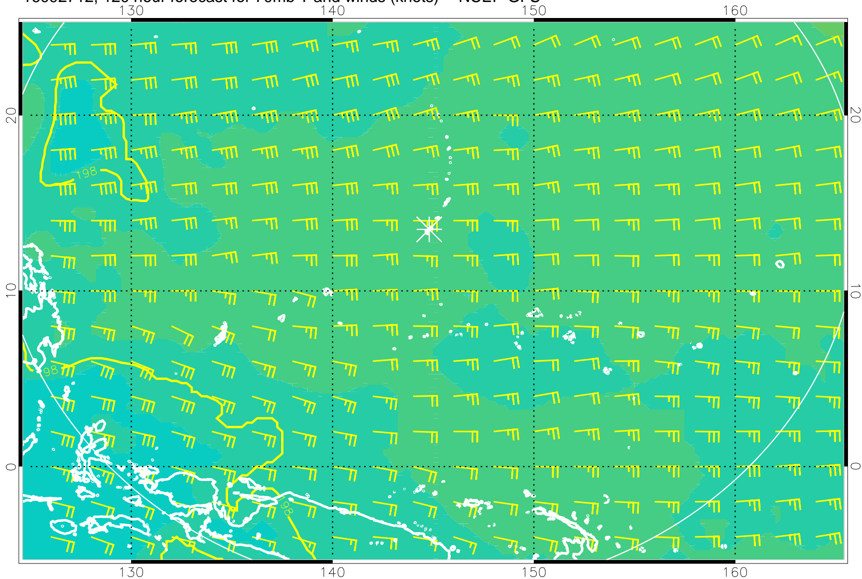
16092712, 120 hour forecast for 70mb T and winds (knots) -- NCEP GFS
