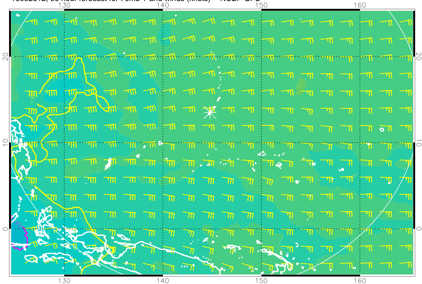
16092612, 96 hour forecast for 70mb T and winds (knots) -- NCEP GFS
