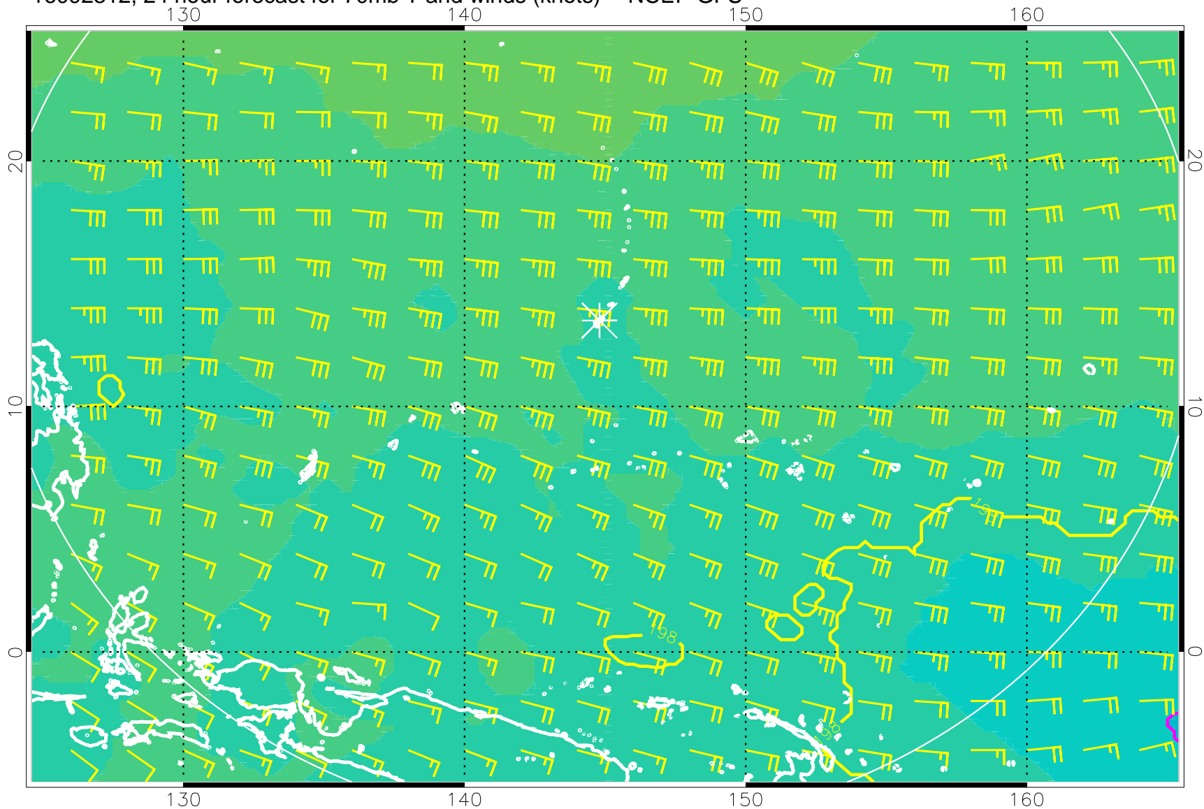
16092312, 24 hour forecast for 70mb T and winds (knots) -- NCEP GFS
