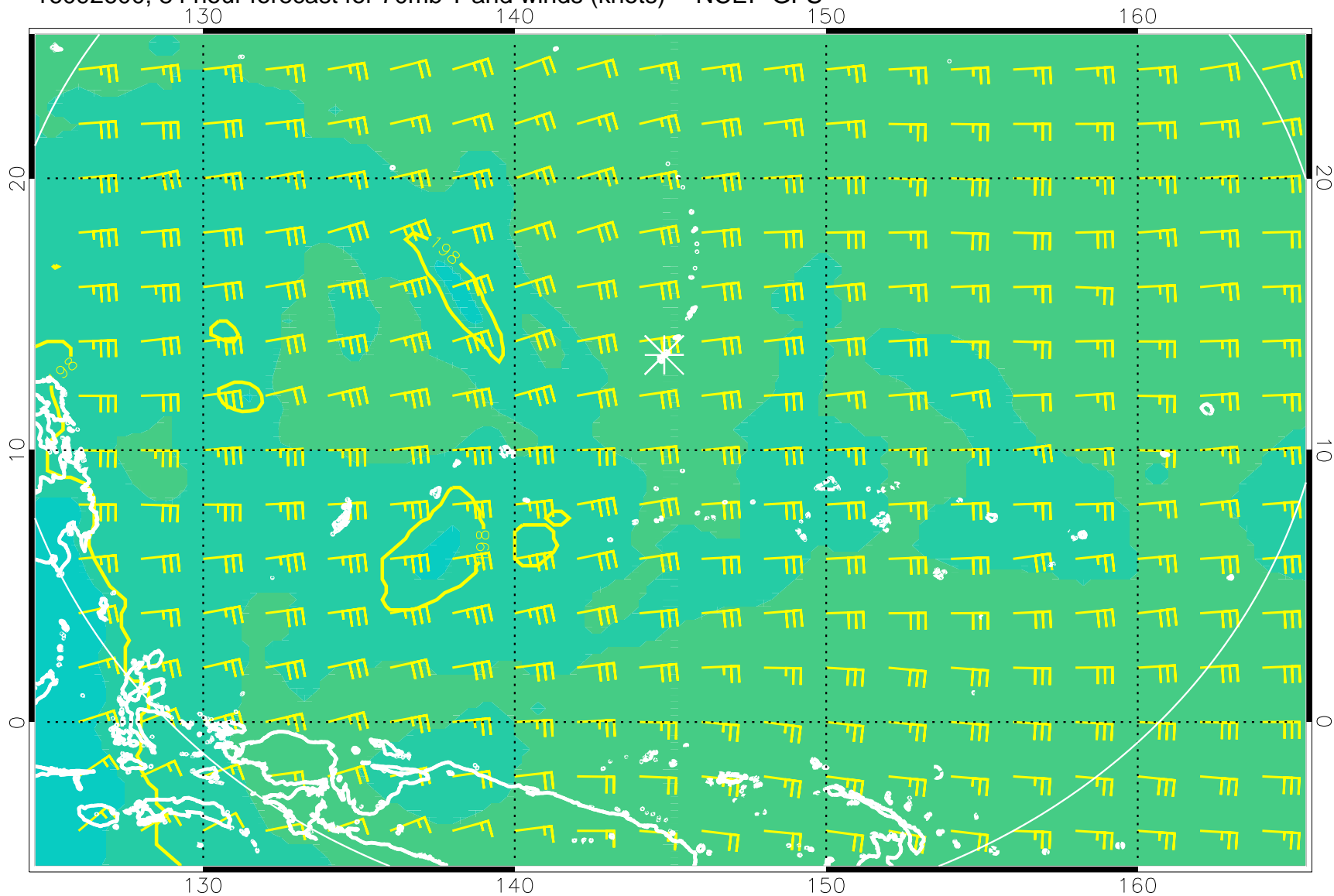
16092600, 84 hour forecast for 70mb T and winds (knots) -- NCEP GFS
