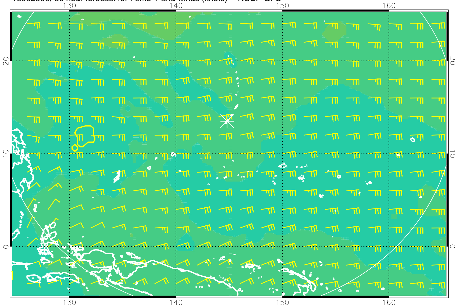
16092500, 60 hour forecast for 70mb T and winds (knots) -- NCEP GFS
