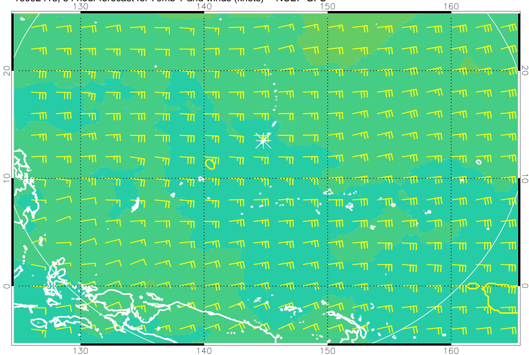
16092418, 54 hour forecast for 70mb T and winds (knots) -- NCEP GFS
