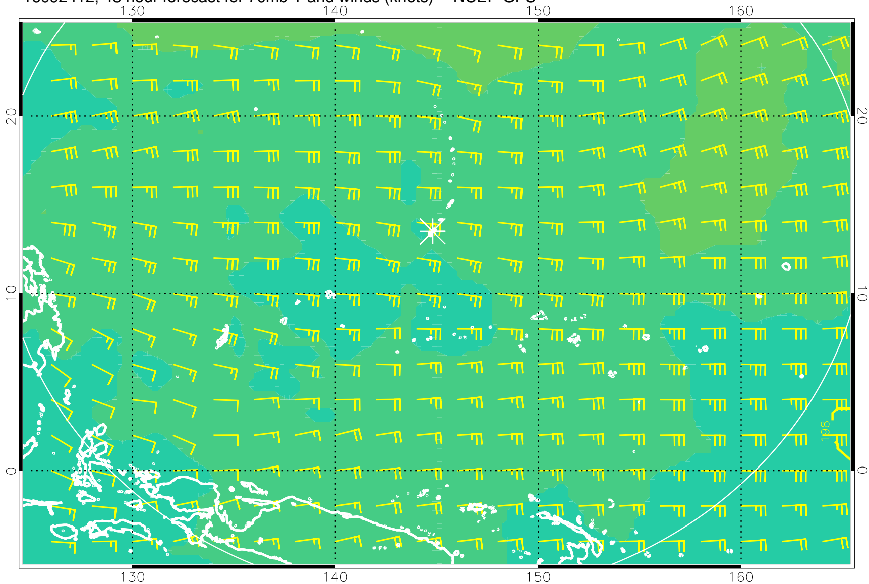
16092412, 48 hour forecast for 70mb T and winds (knots) -- NCEP GFS
