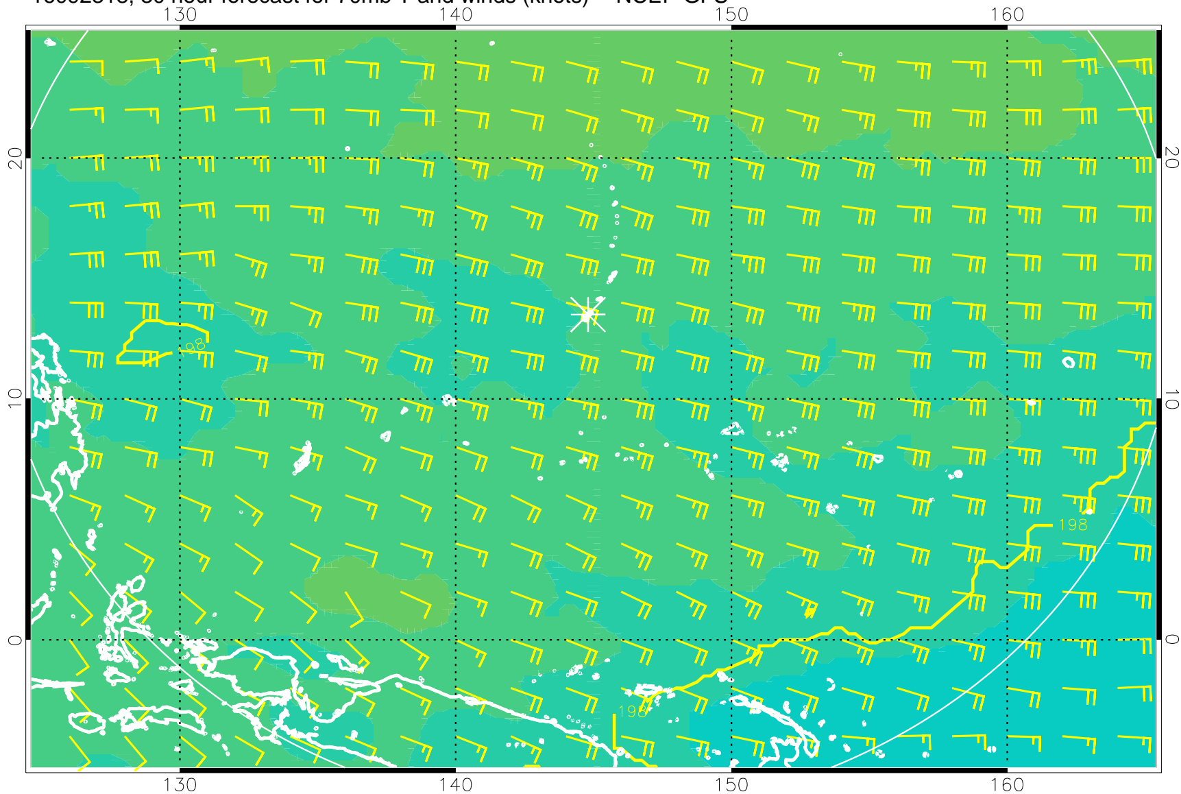
16092318, 30 hour forecast for 70mb T and winds (knots) -- NCEP GFS
