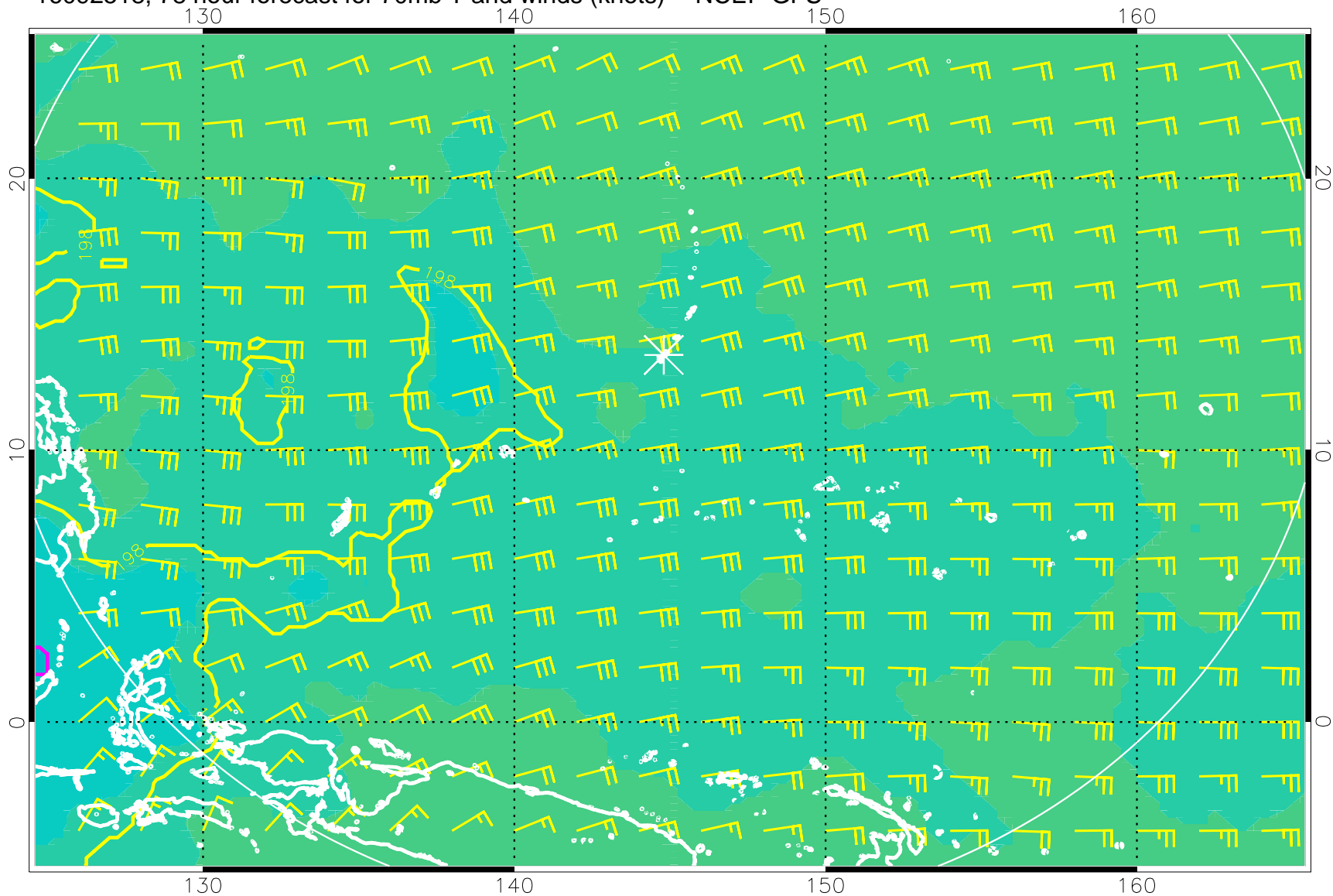
16092518, 78 hour forecast for 70mb T and winds (knots) -- NCEP GFS
