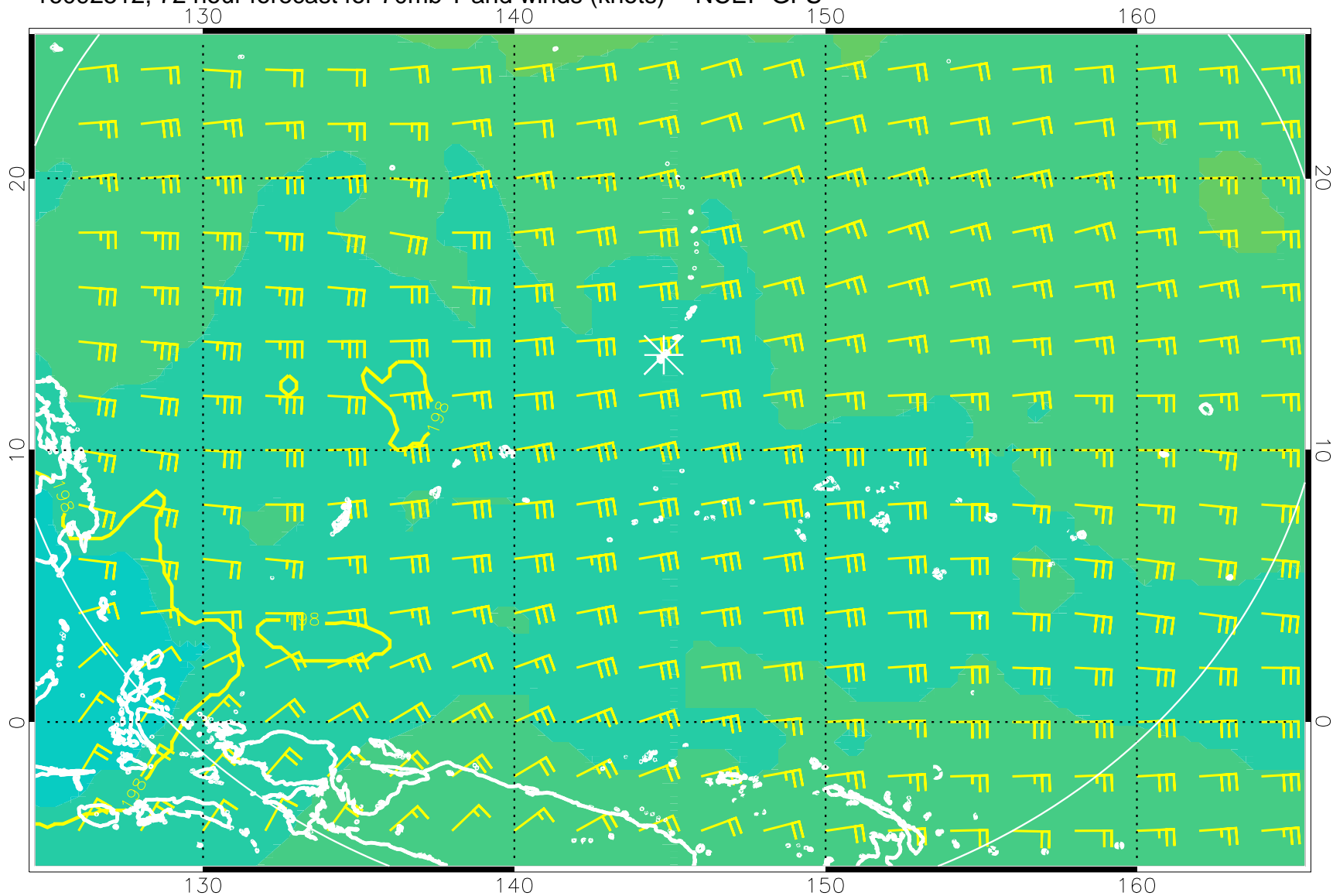
16092512, 72 hour forecast for 70mb T and winds (knots) -- NCEP GFS
