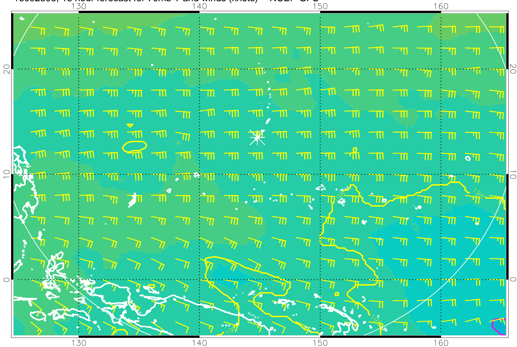
16092306, 18 hour forecast for 70mb T and winds (knots) -- NCEP GFS
