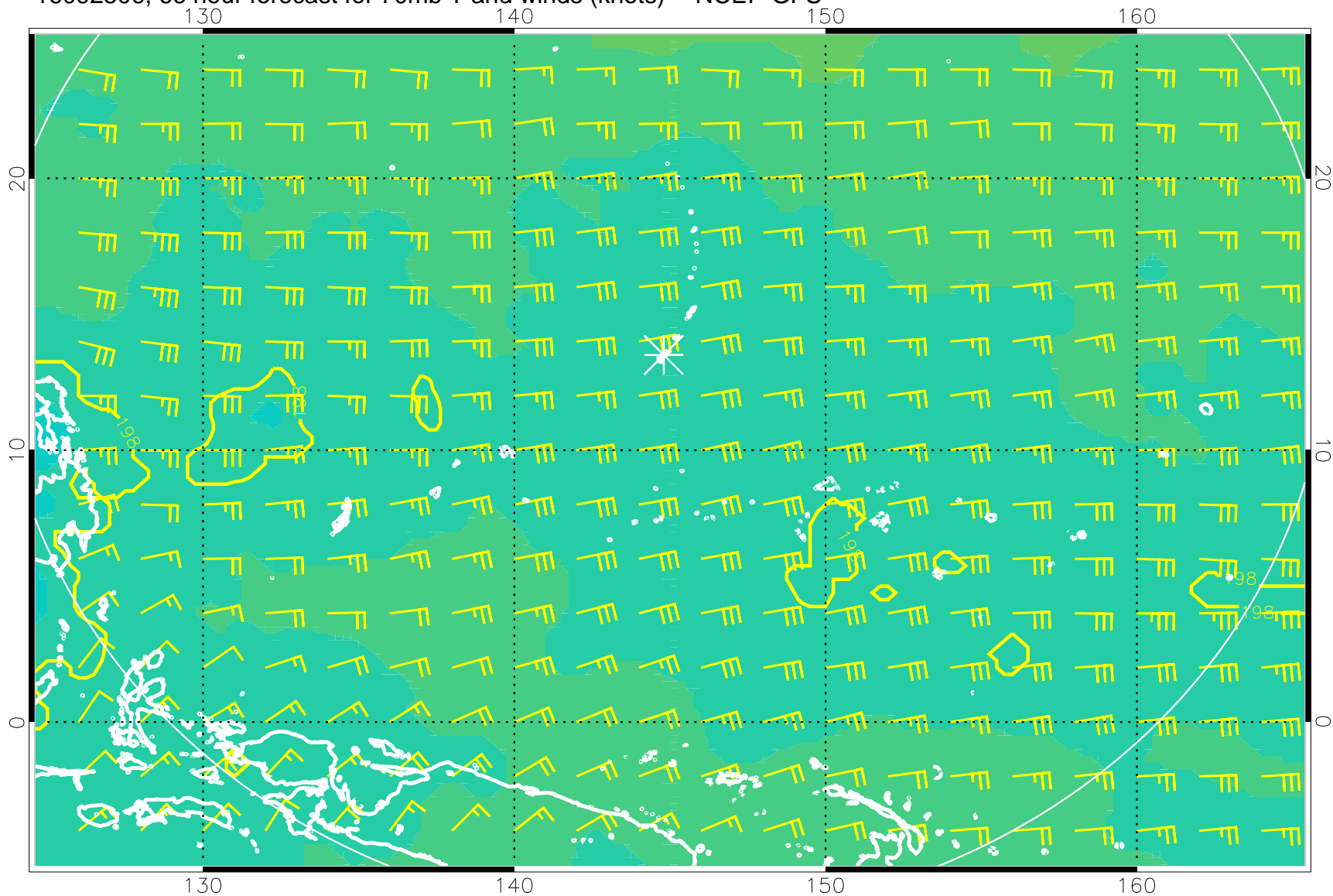
16092506, 66 hour forecast for 70mb T and winds (knots) -- NCEP GFS
