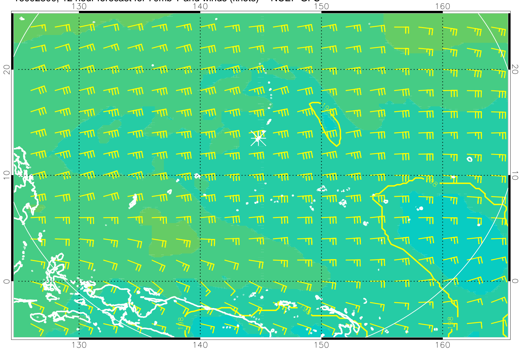
16092300, 12 hour forecast for 70mb T and winds (knots) -- NCEP GFS
