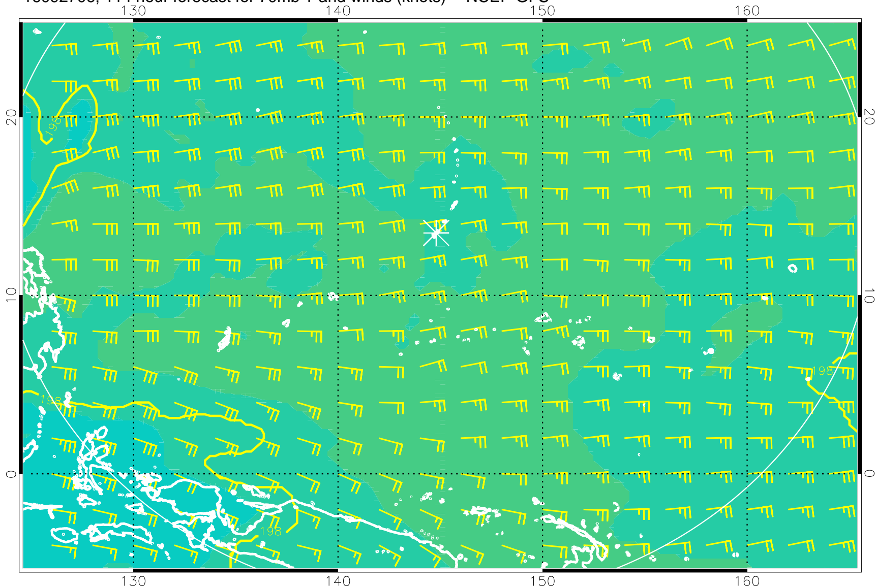
16092706, 114 hour forecast for 70mb T and winds (knots) -- NCEP GFS
