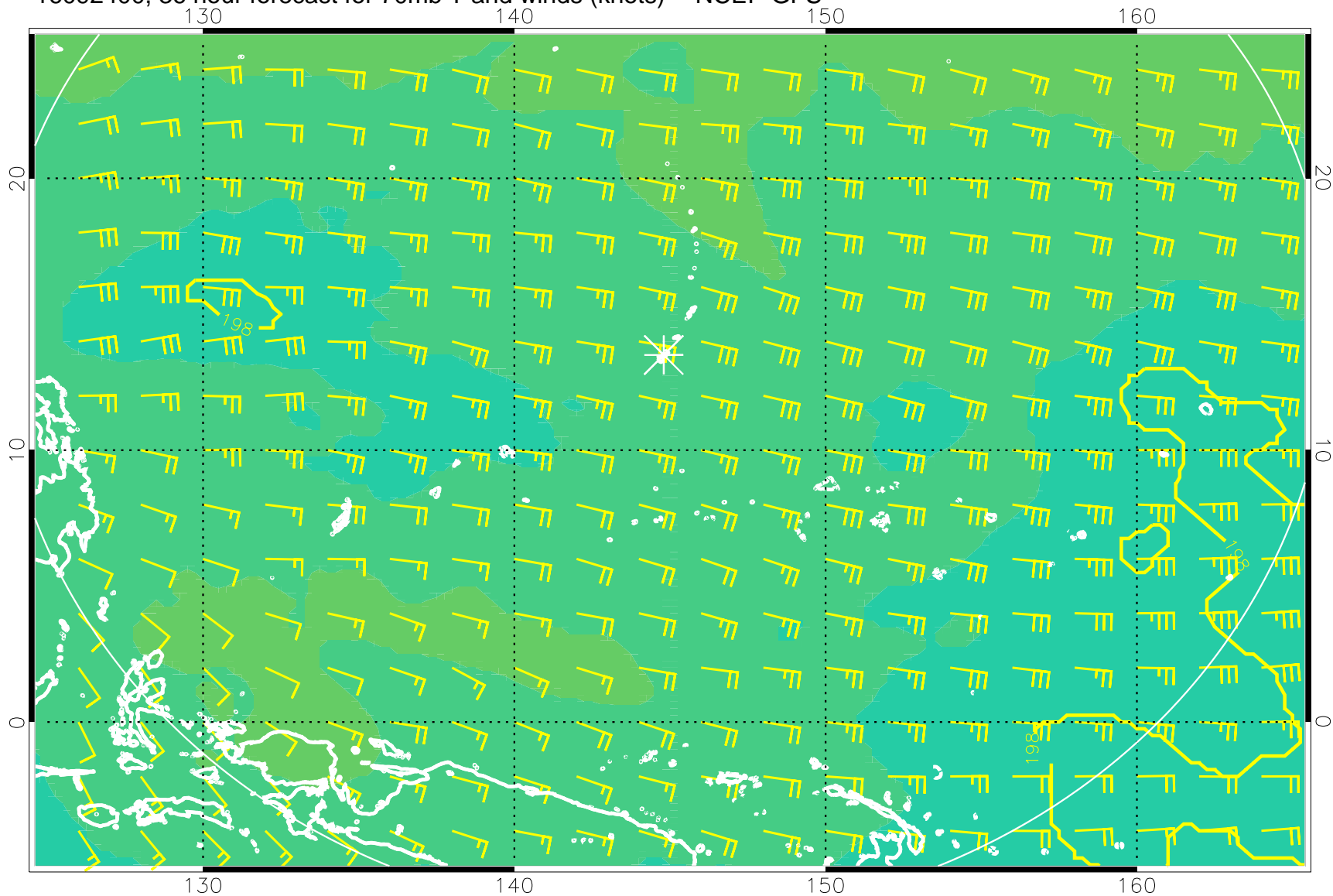
16092400, 36 hour forecast for 70mb T and winds (knots) -- NCEP GFS
