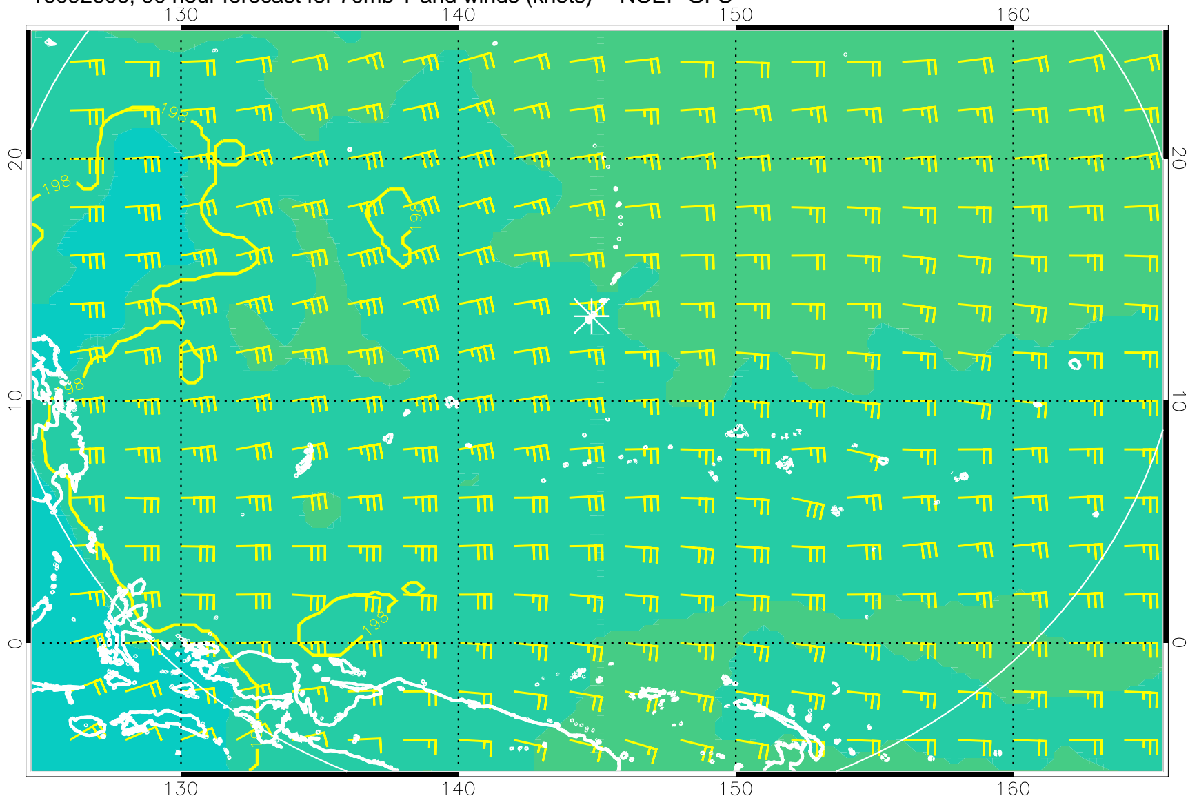
16092606, 90 hour forecast for 70mb T and winds (knots) -- NCEP GFS
