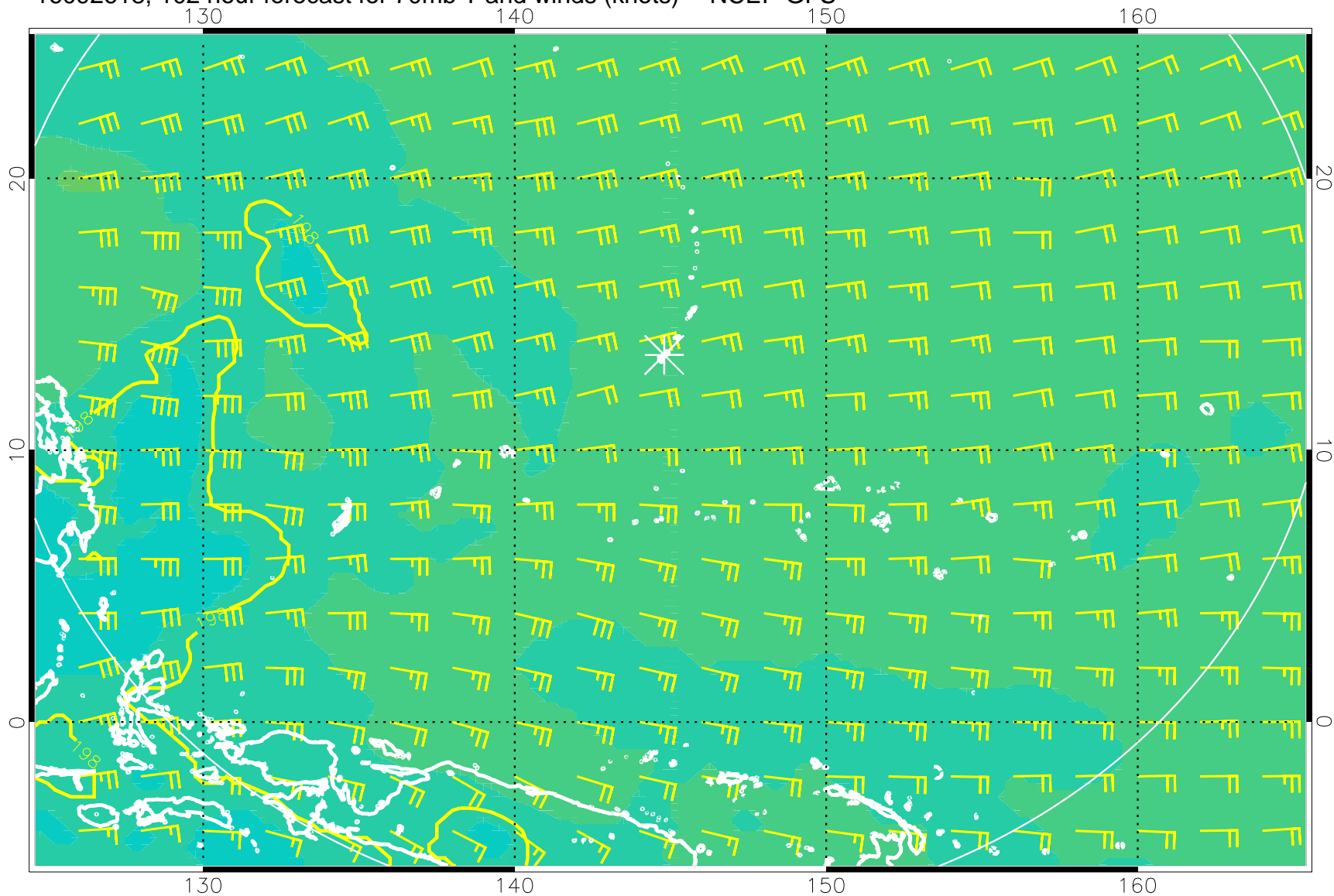
16092618, 102 hour forecast for 70mb T and winds (knots) -- NCEP GFS
