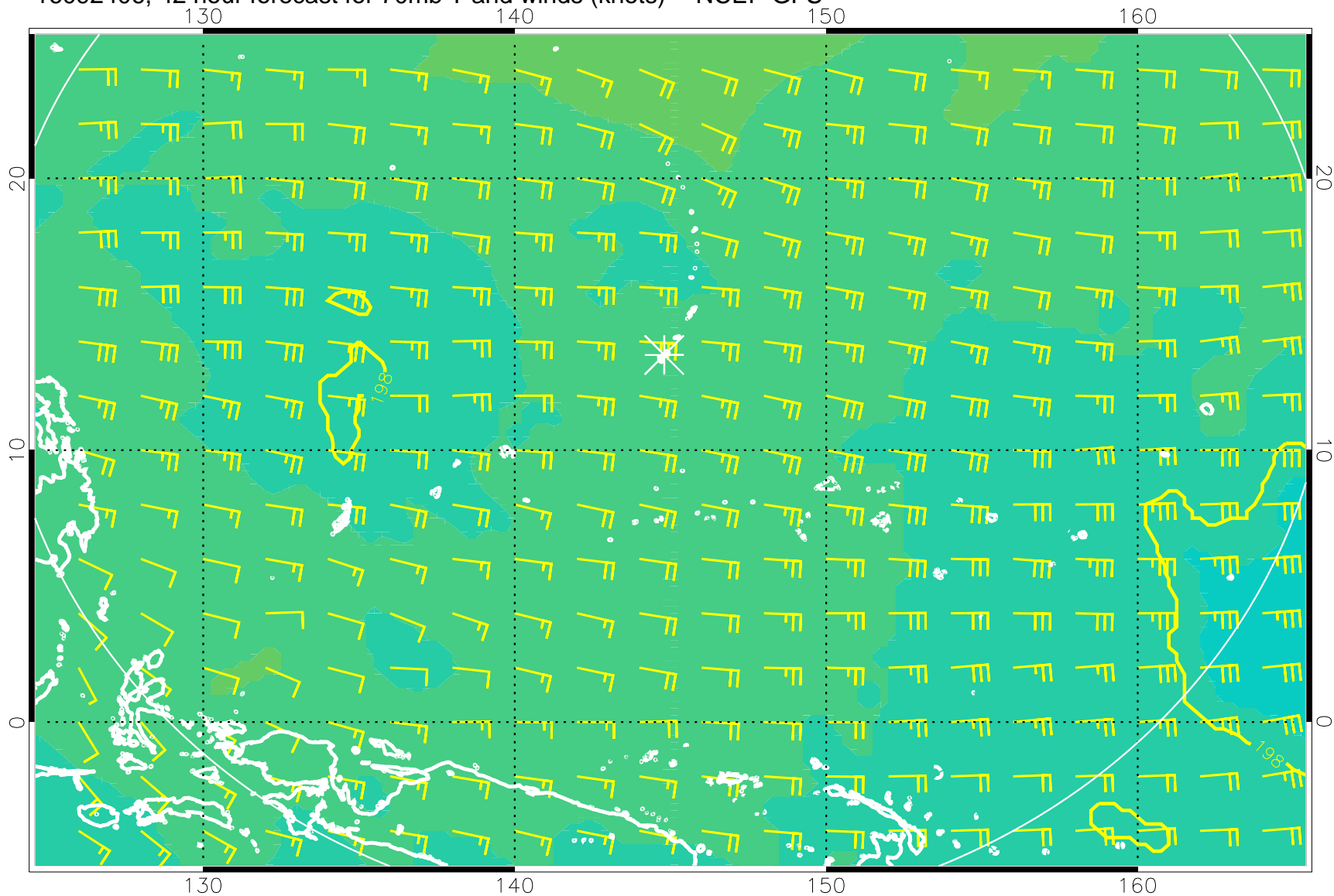
16092406, 42 hour forecast for 70mb T and winds (knots) -- NCEP GFS
