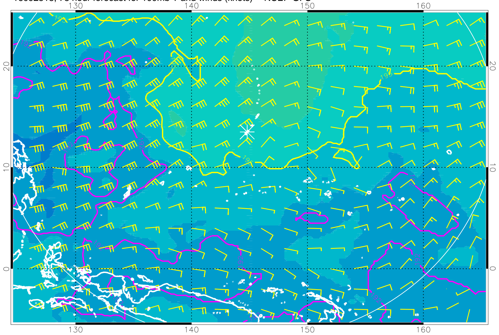
16092518, 78 hour forecast for 100mb T and winds (knots) -- NCEP GFS
