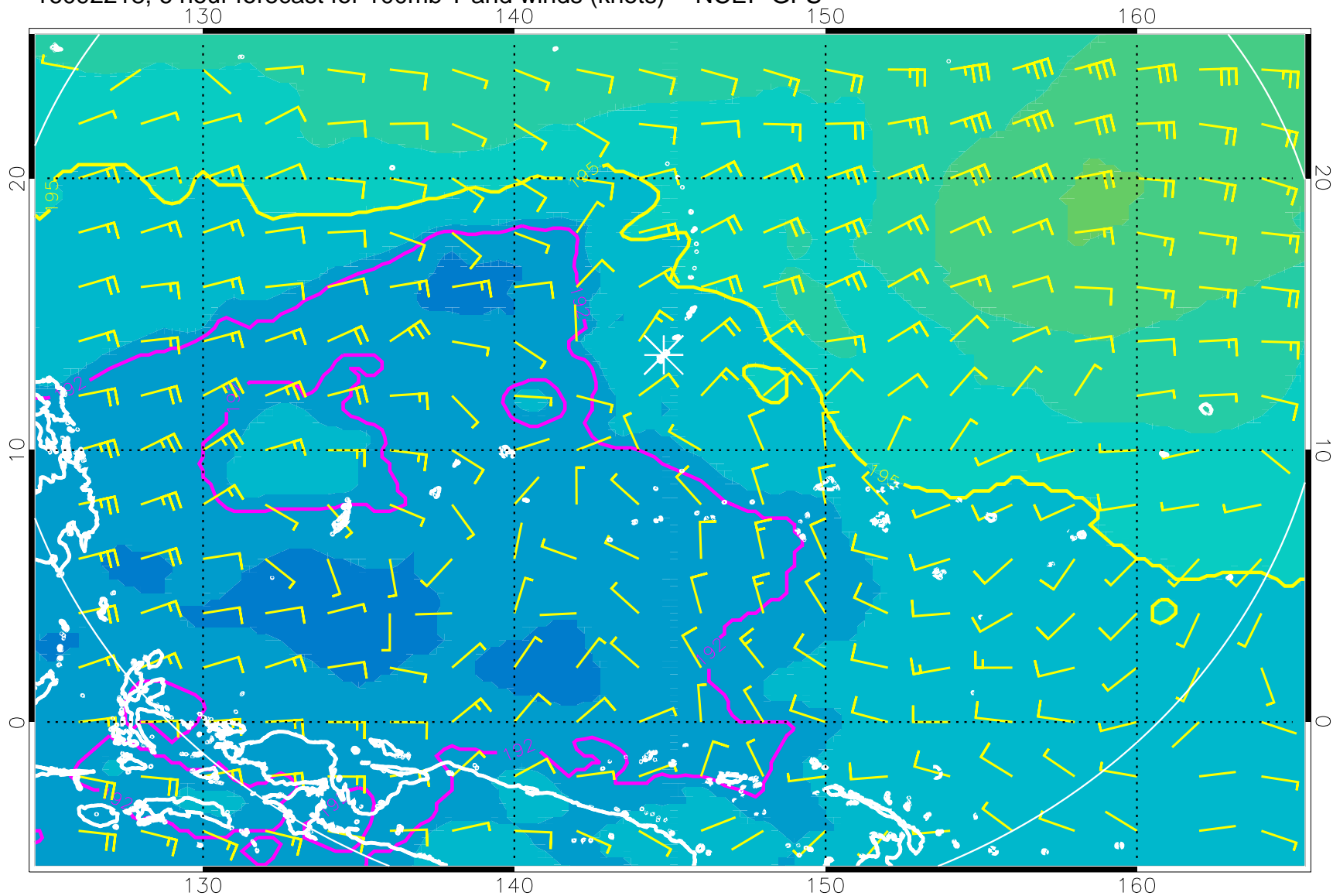
16092218, 6 hour forecast for 100mb T and winds (knots) -- NCEP GFS
