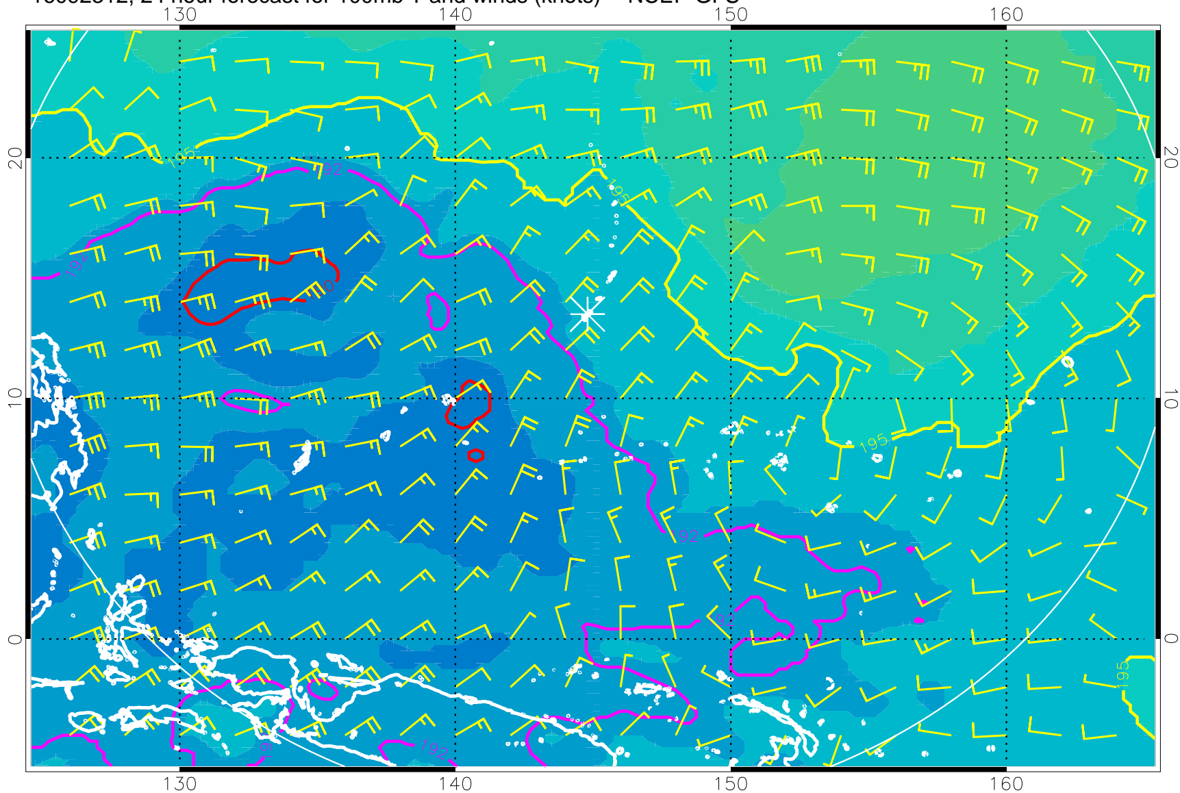
16092312, 24 hour forecast for 100mb T and winds (knots) -- NCEP GFS
