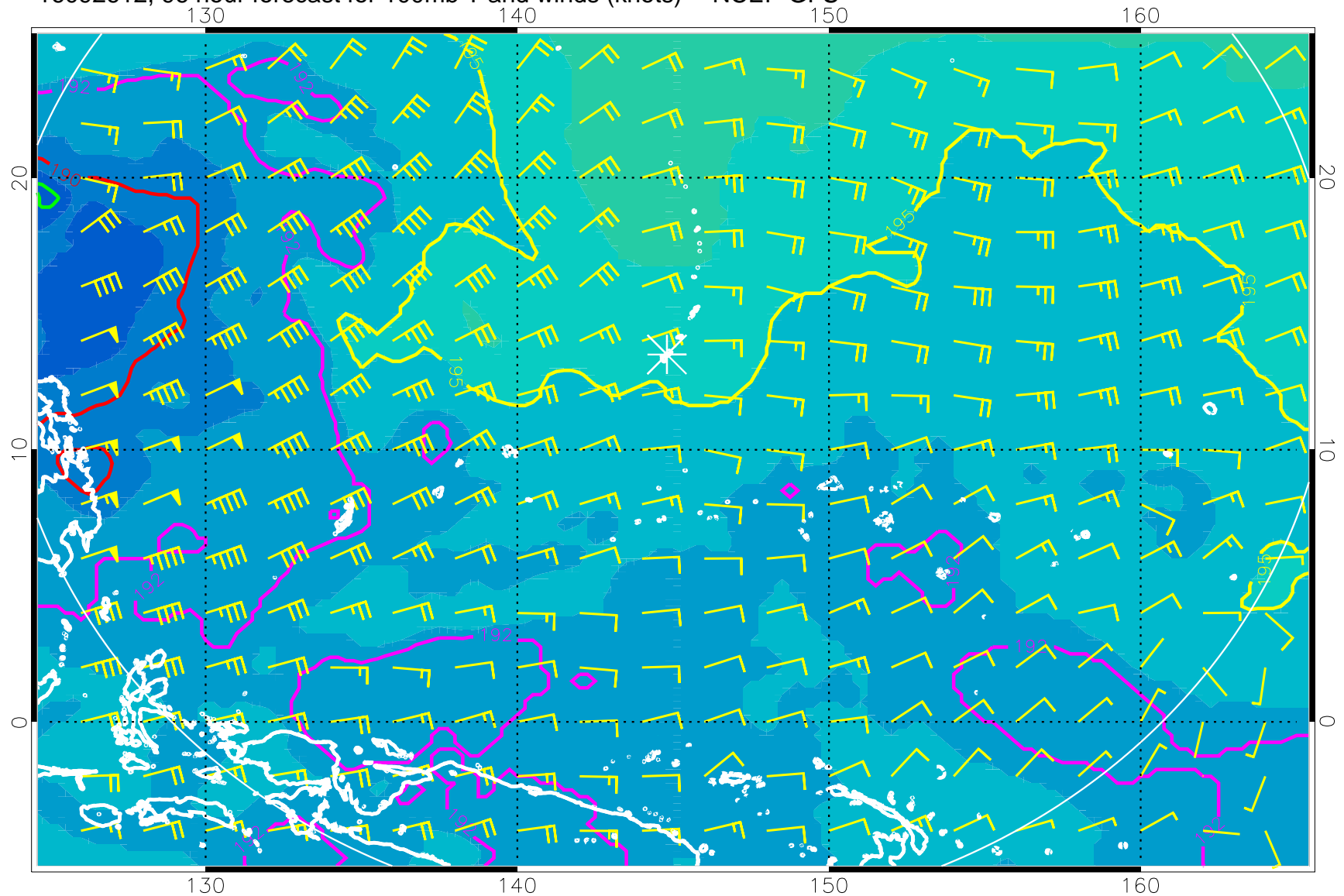
16092612, 96 hour forecast for 100mb T and winds (knots) -- NCEP GFS
