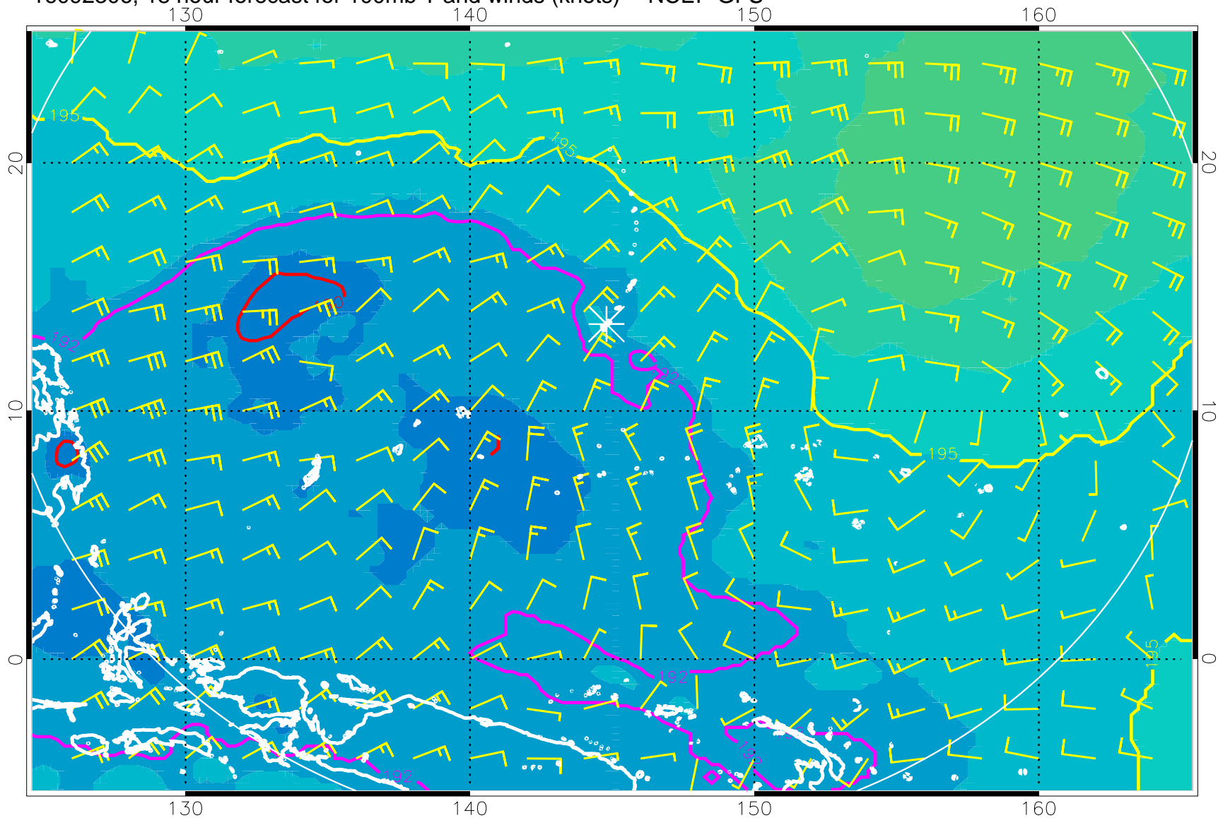
16092306, 18 hour forecast for 100mb T and winds (knots) -- NCEP GFS
