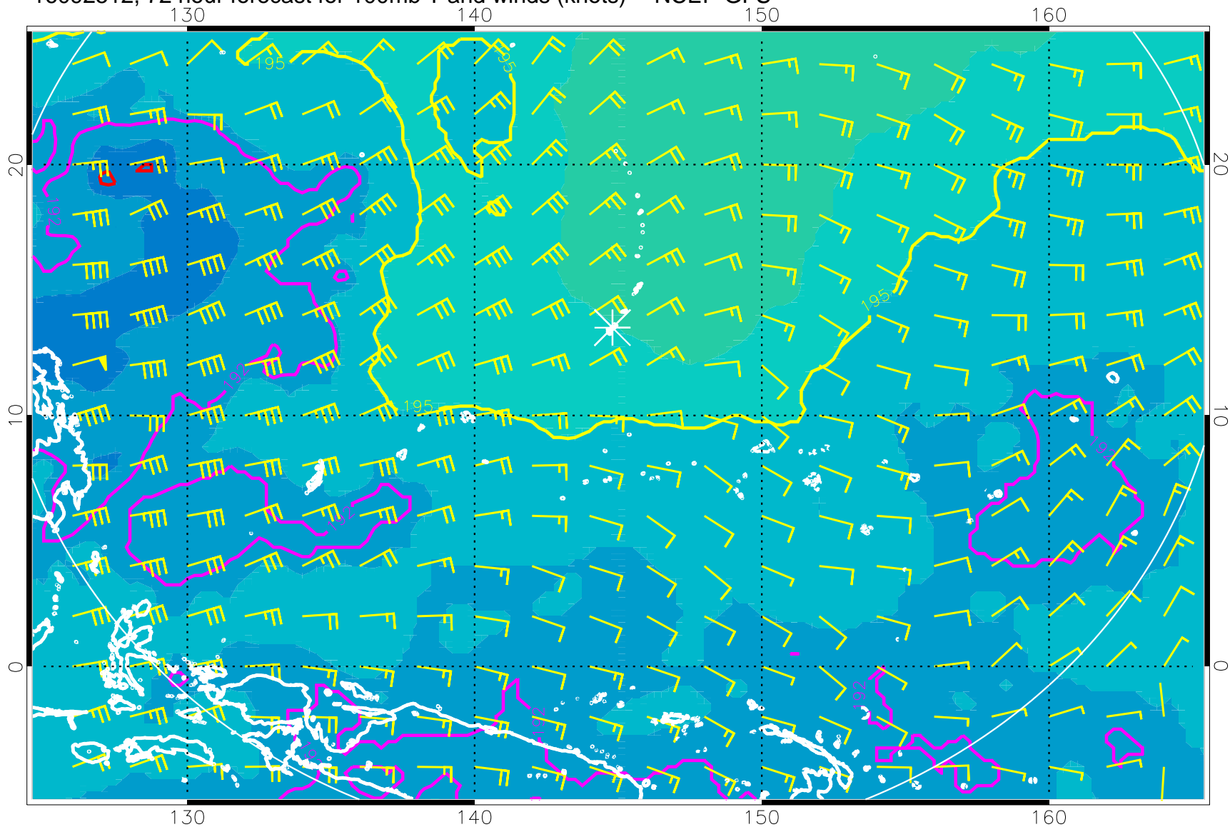
16092512, 72 hour forecast for 100mb T and winds (knots) -- NCEP GFS
