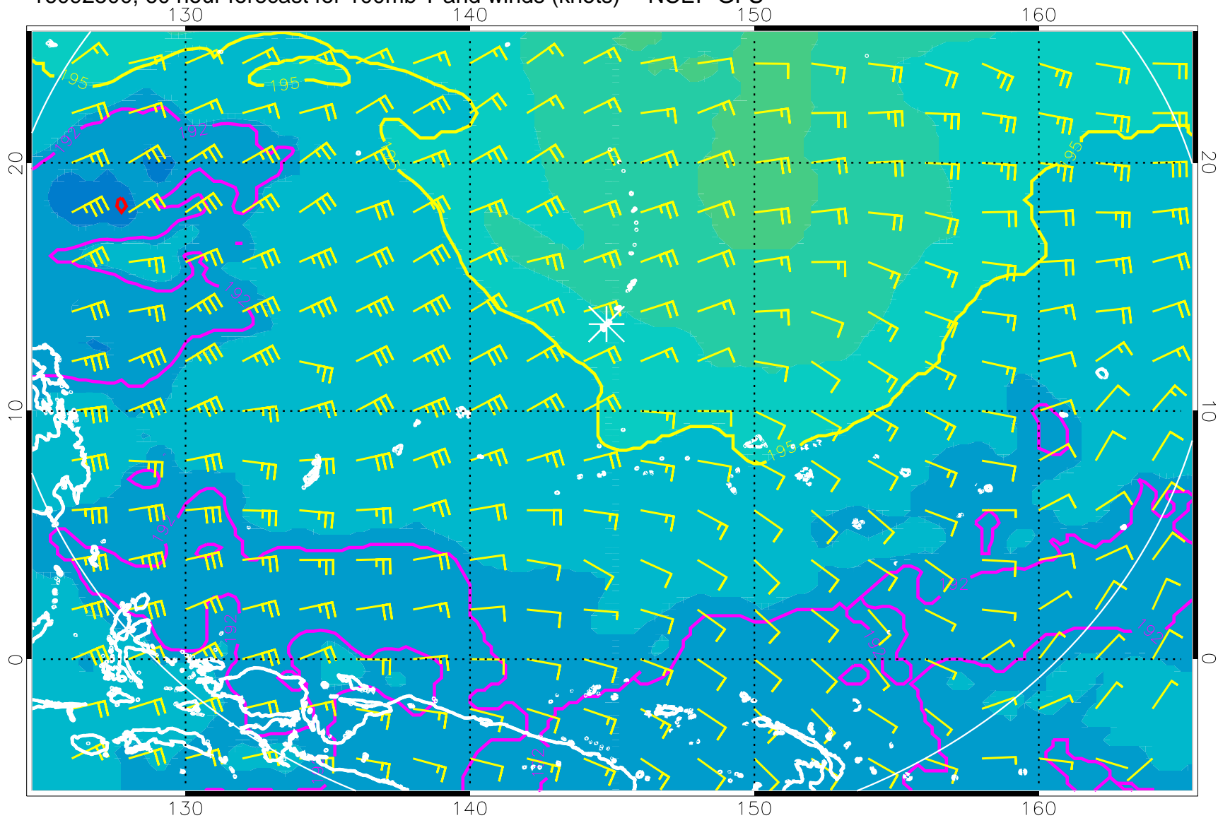
16092500, 60 hour forecast for 100mb T and winds (knots) -- NCEP GFS
