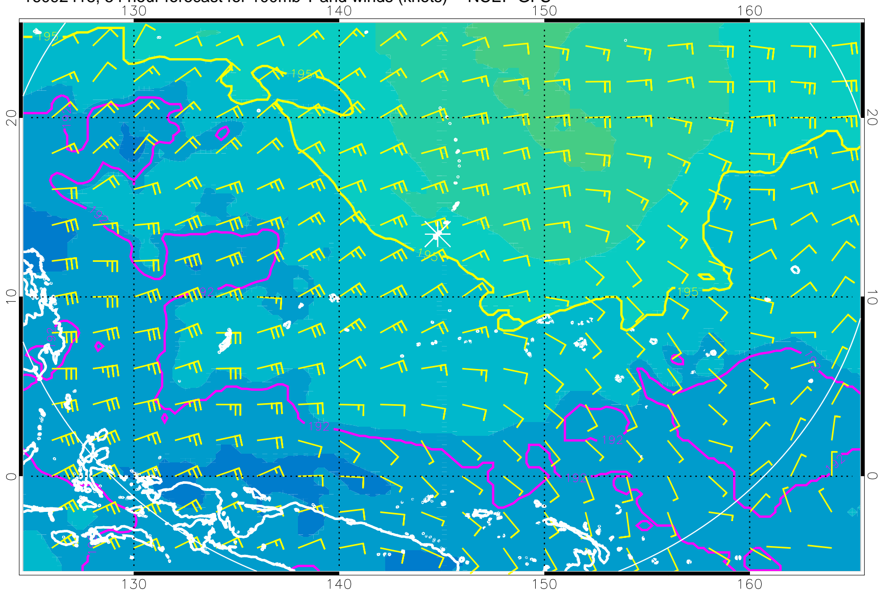
16092418, 54 hour forecast for 100mb T and winds (knots) -- NCEP GFS
