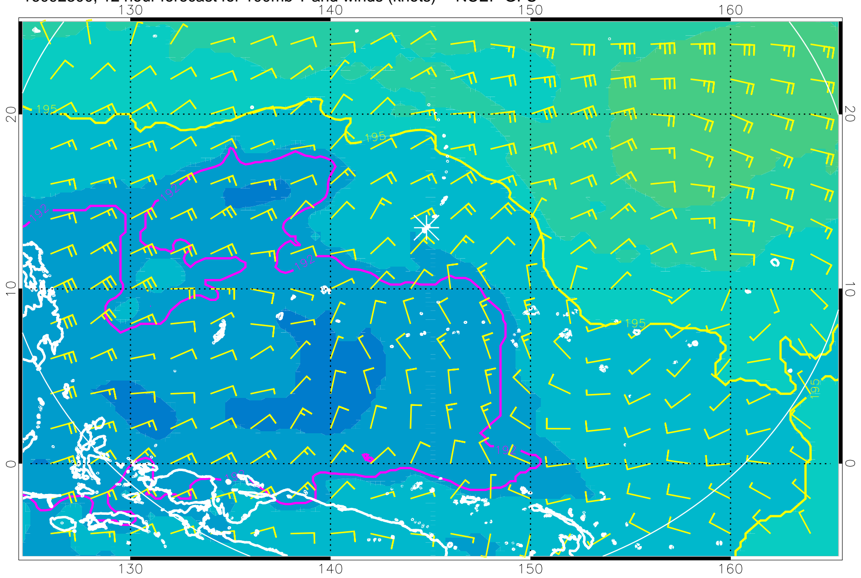
16092300, 12 hour forecast for 100mb T and winds (knots) -- NCEP GFS
