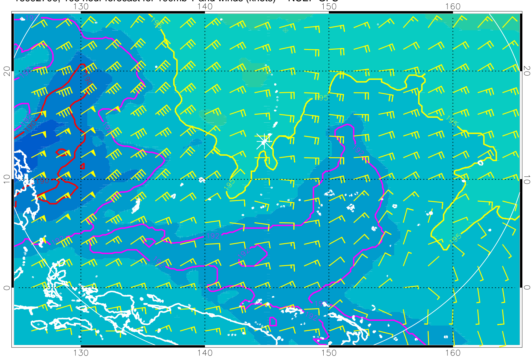
16092700, 108 hour forecast for 100mb T and winds (knots) -- NCEP GFS
