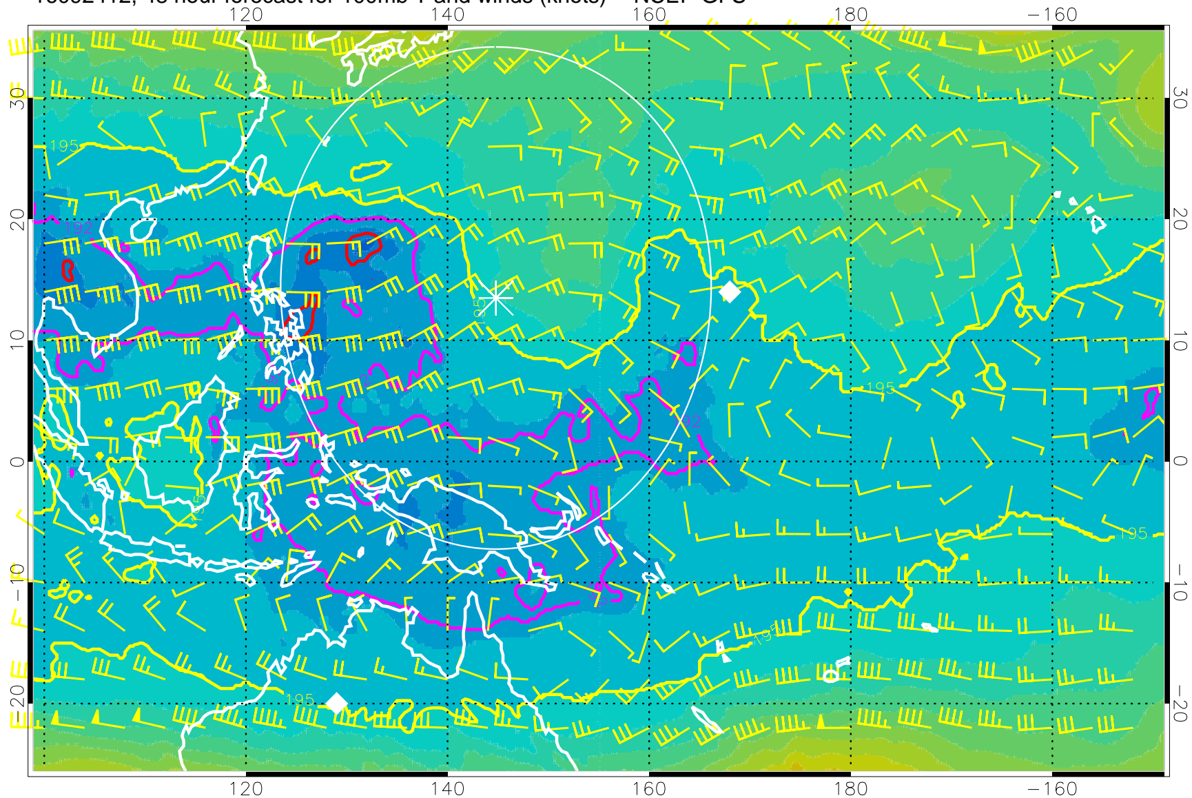
16092412, 48 hour forecast for 100mb T and winds (knots) -- NCEP GFS
