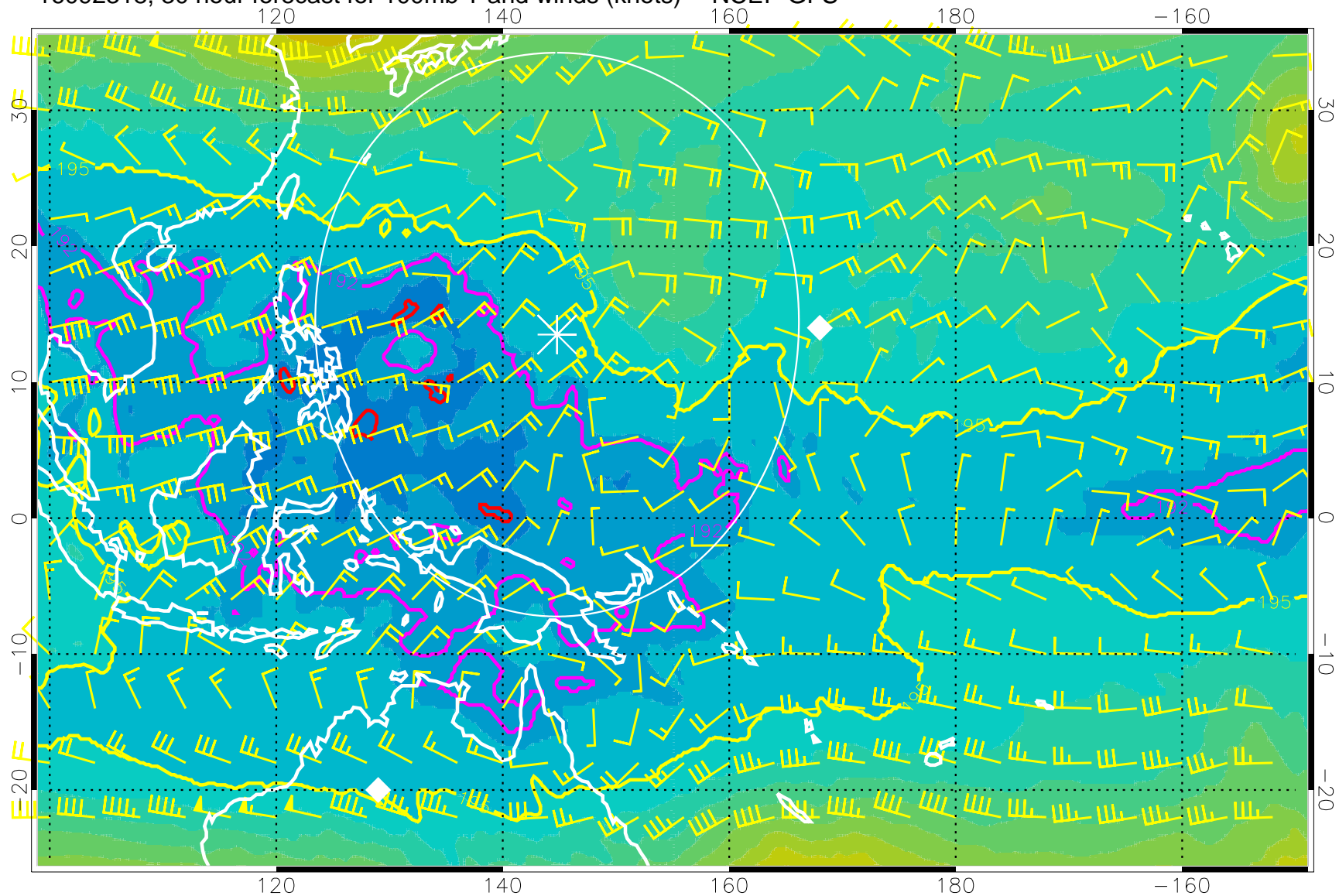
16092318, 30 hour forecast for 100mb T and winds (knots) -- NCEP GFS
