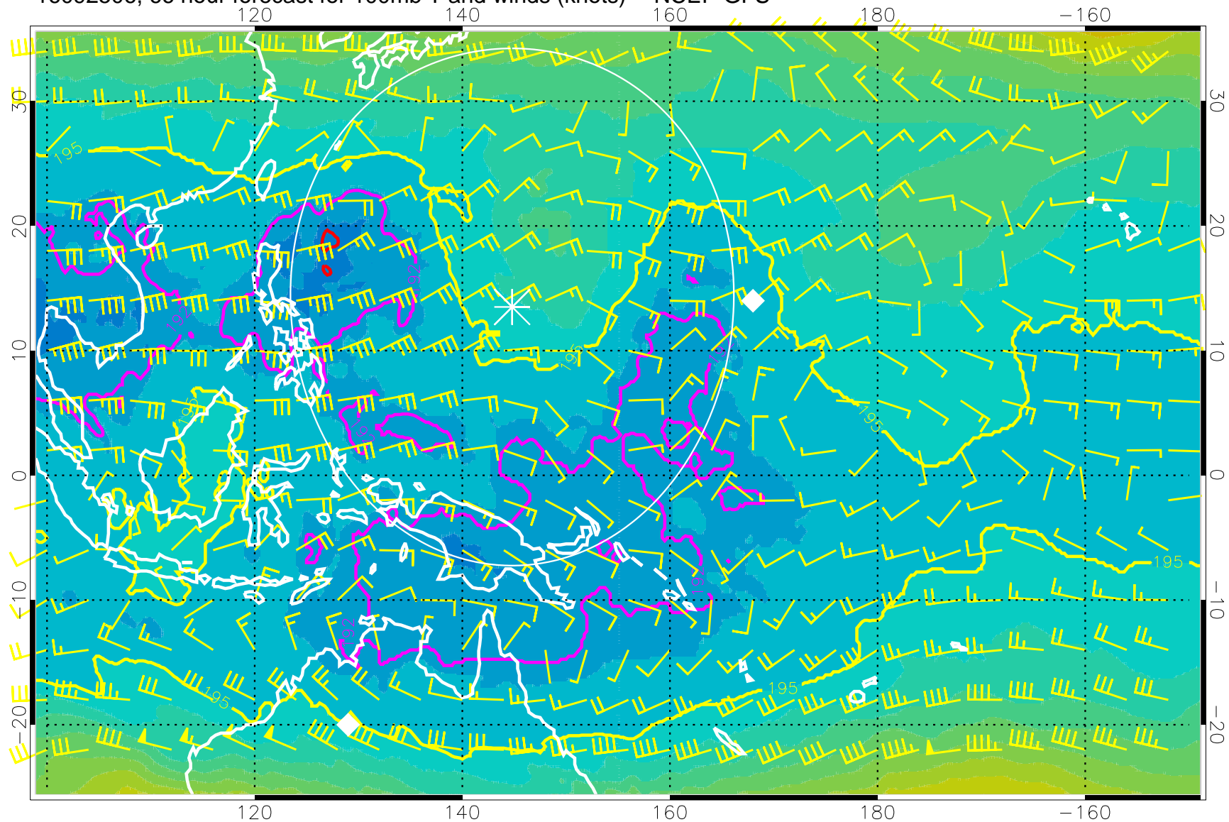
16092506, 66 hour forecast for 100mb T and winds (knots) -- NCEP GFS
