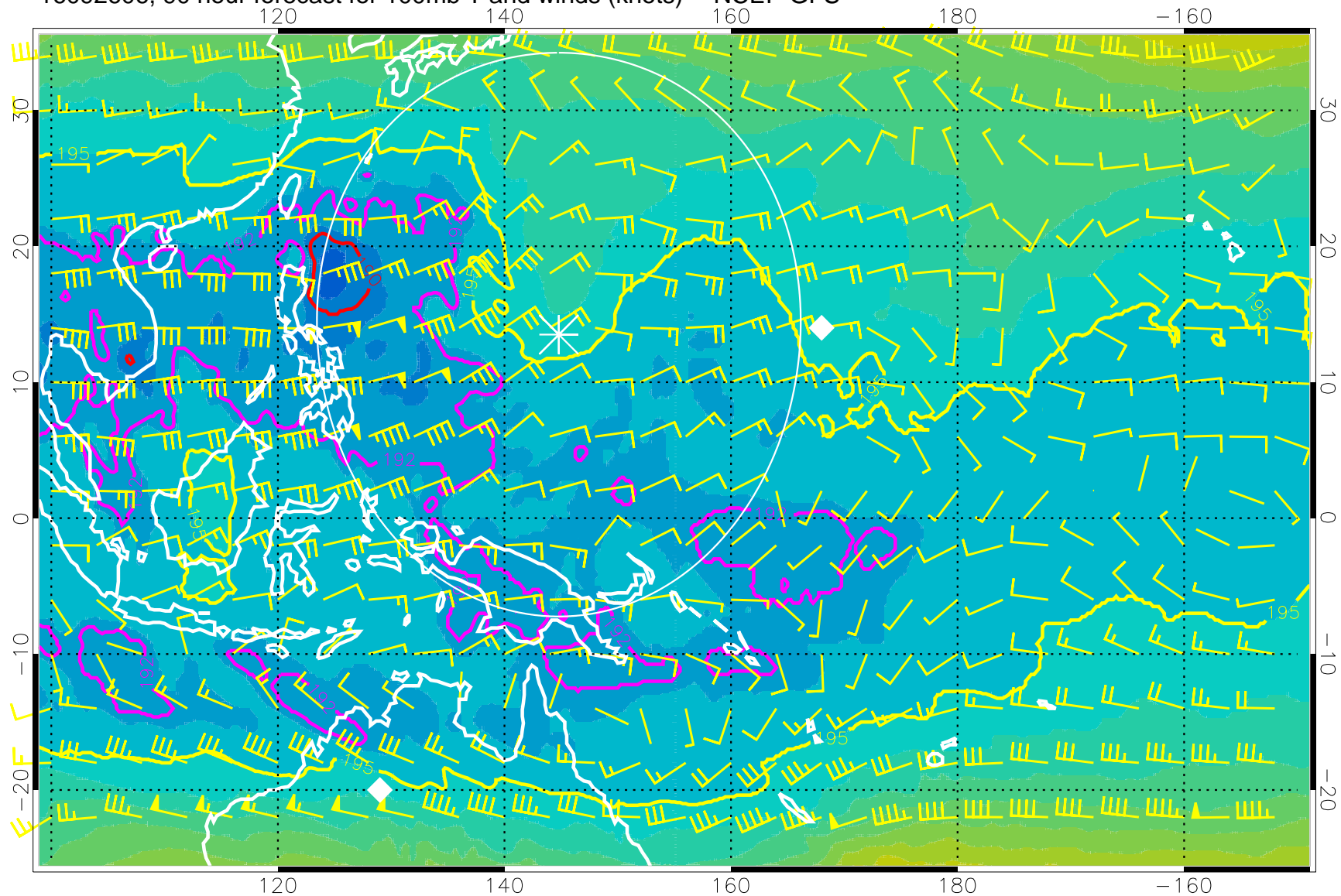
16092606, 90 hour forecast for 100mb T and winds (knots) -- NCEP GFS
