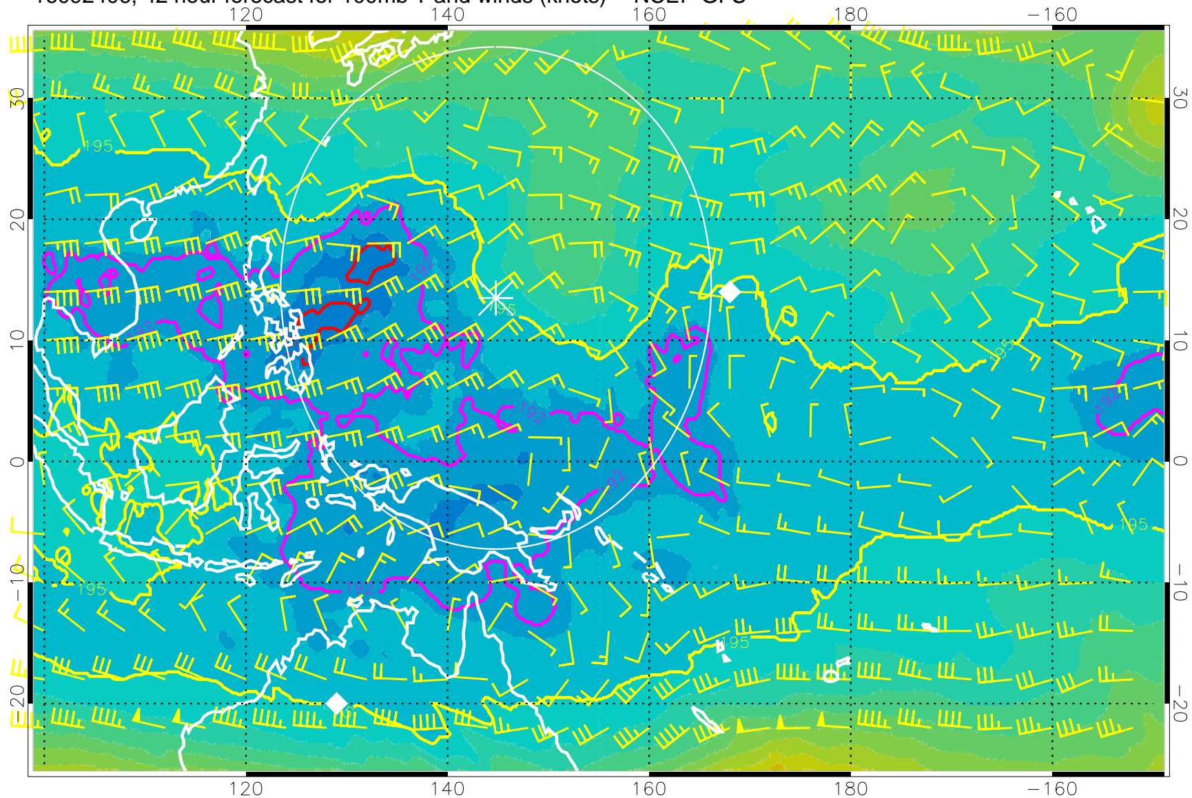
16092406, 42 hour forecast for 100mb T and winds (knots) -- NCEP GFS
