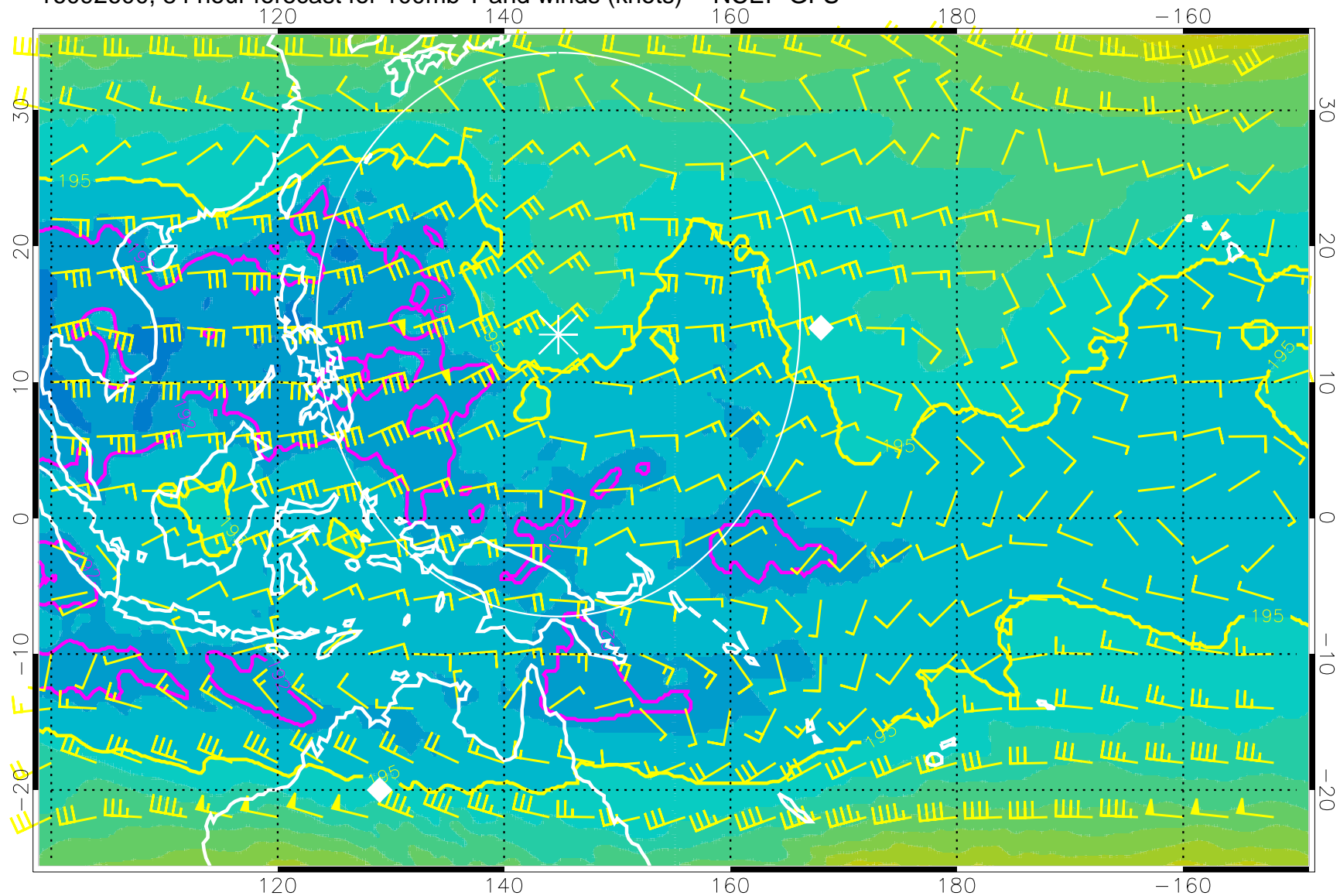
16092600, 84 hour forecast for 100mb T and winds (knots) -- NCEP GFS
