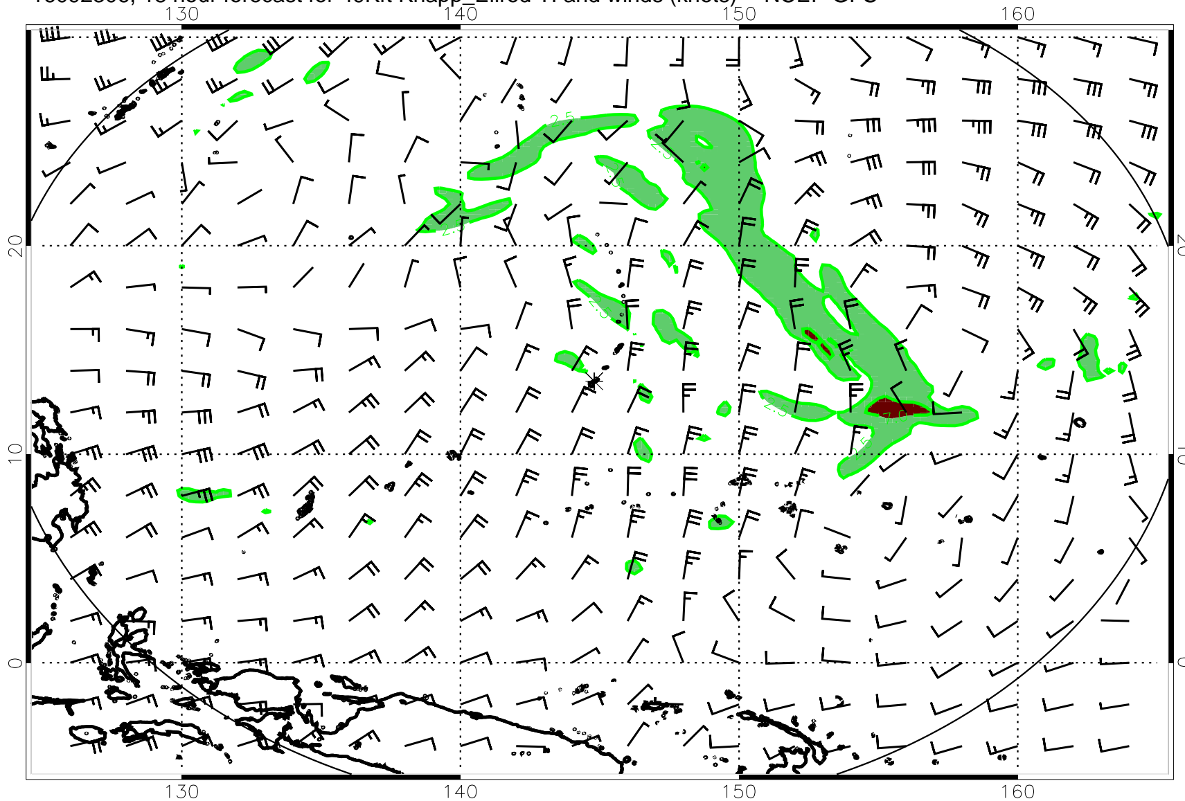
16092306, 18 hour forecast for 49Kft Knapp_Ellrod TI and winds (knots) -- NCEP GFS
