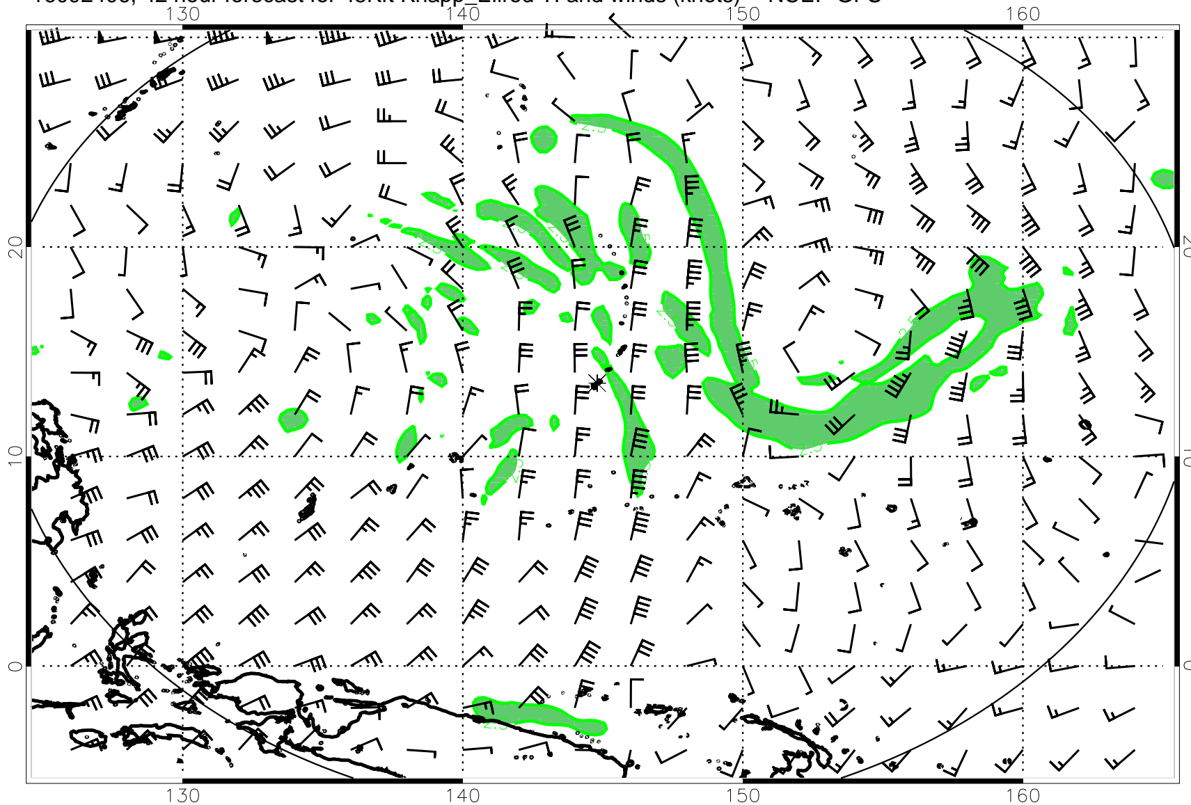
16092406, 42 hour forecast for 45Kft Knapp_Ellrod TI and winds (knots) -- NCEP GFS
