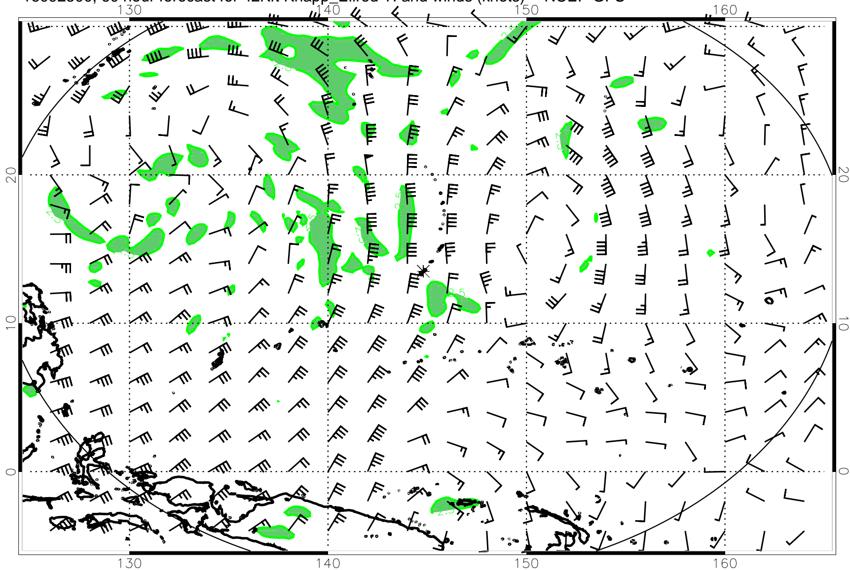
16092500, 60 hour forecast for 42Kft Knapp_Ellrod TI and winds (knots) -- NCEP GFS
