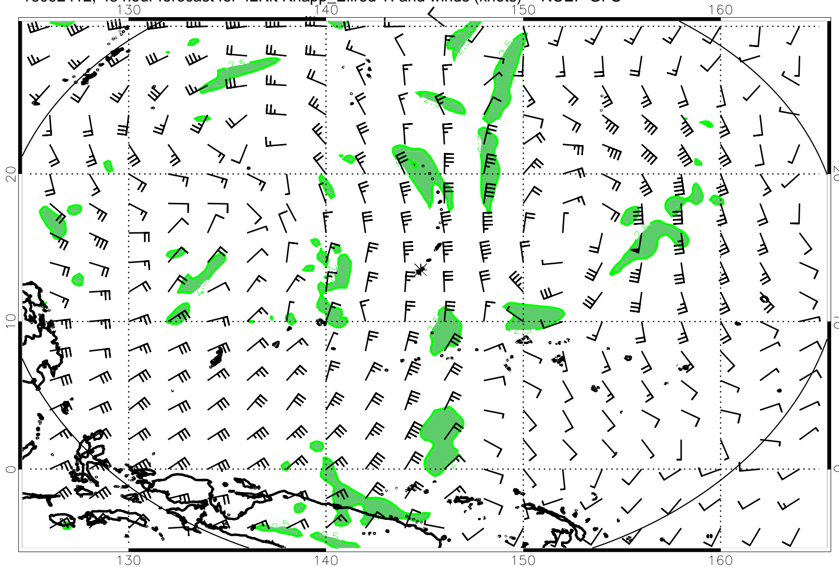
16092412, 48 hour forecast for 42Kft Knapp_Ellrod TI and winds (knots) -- NCEP GFS
