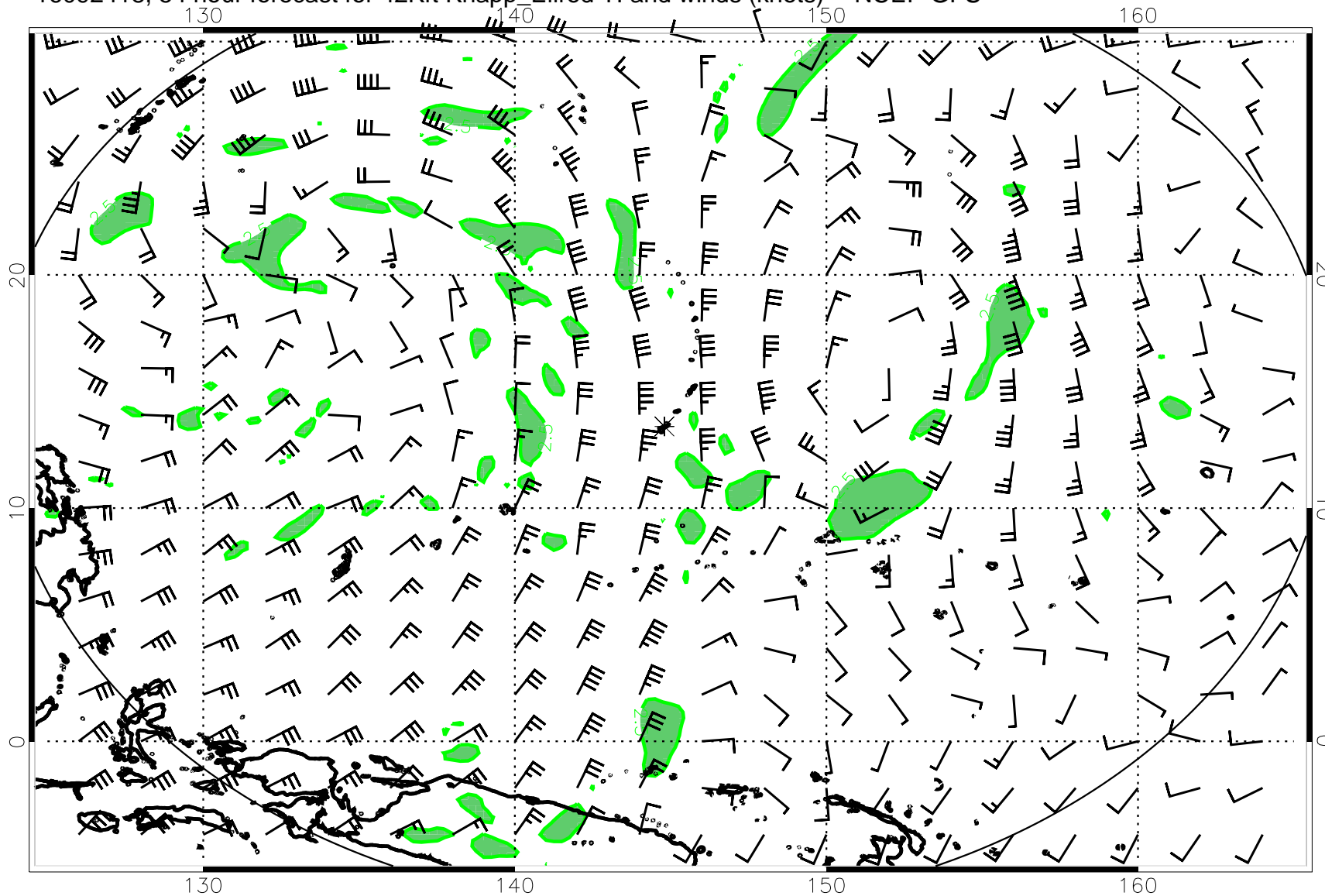
16092418, 54 hour forecast for 42Kft Knapp_Ellrod TI and winds (knots) -- NCEP GFS
