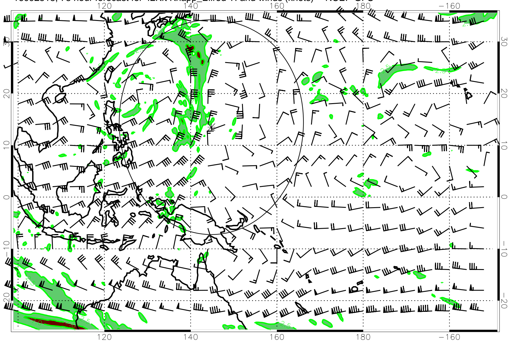
16092518, 78 hour forecast for 42Kft Knapp_Ellrod TI and winds (knots) -- NCEP GFS
