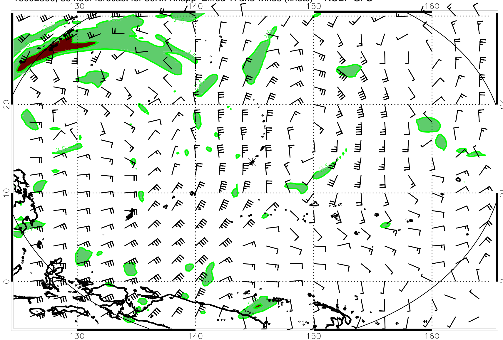
16092506, 66 hour forecast for 36Kft Knapp_Ellrod TI and winds (knots) -- NCEP GFS
