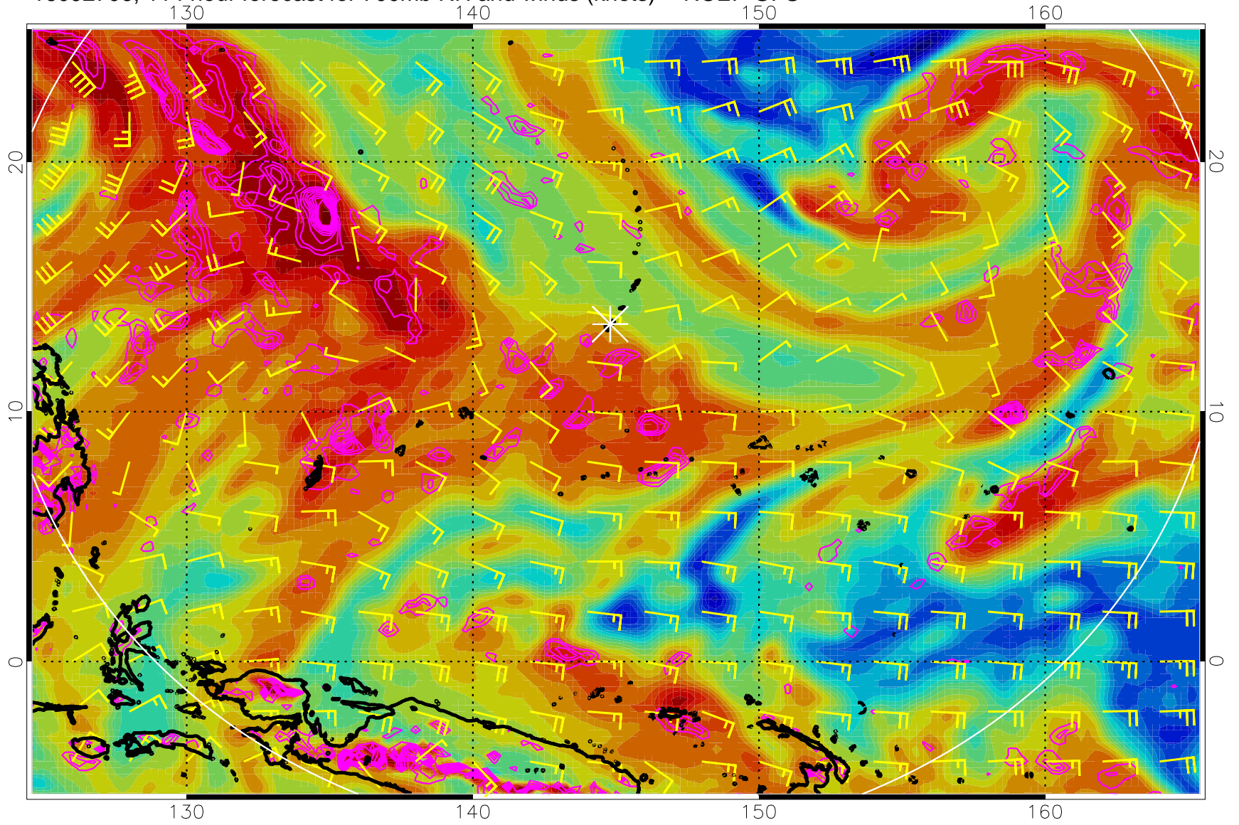
16092706, 114 hour forecast for 700mb RH and winds (knots) -- NCEP GFS
