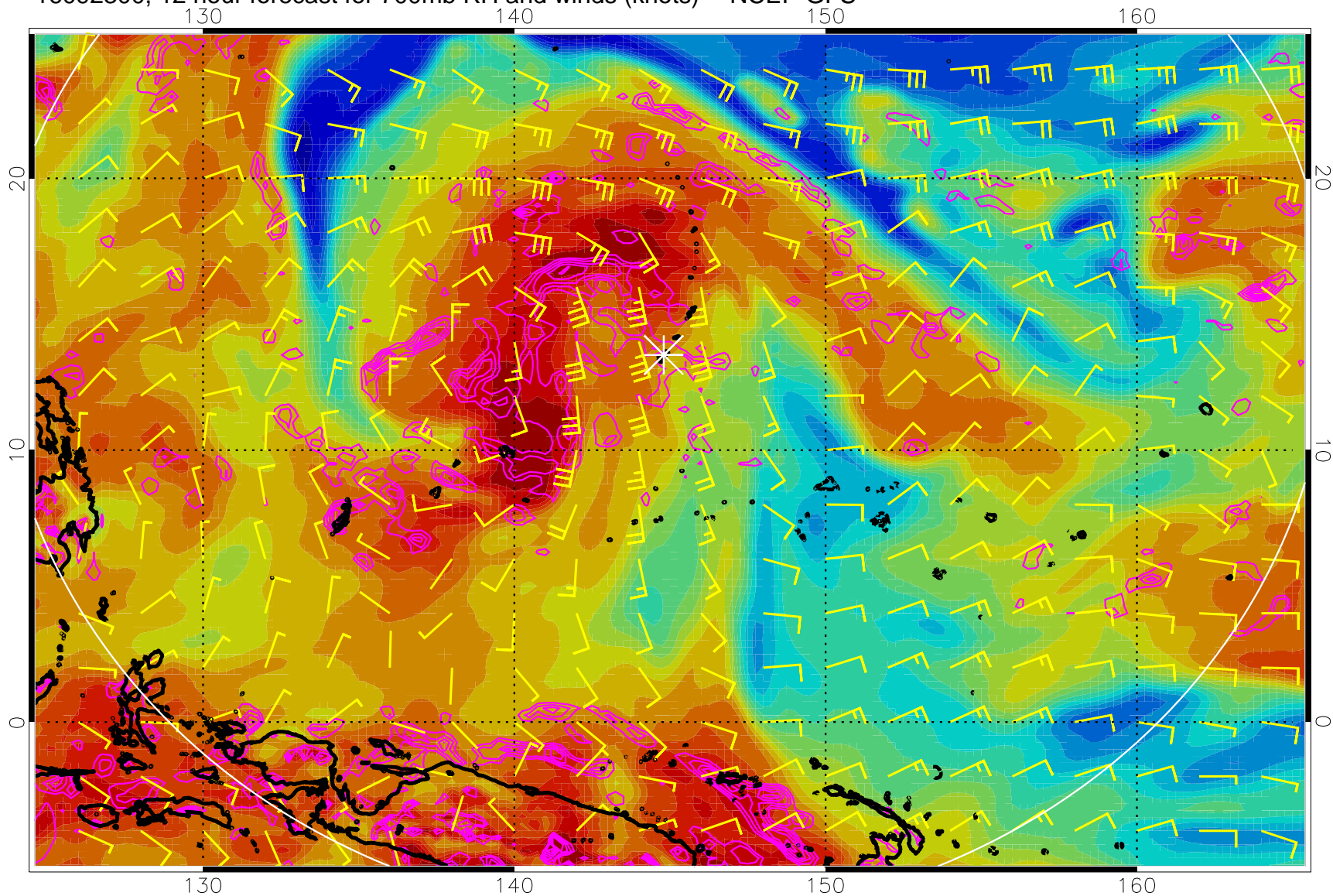
16092300, 12 hour forecast for 700mb RH and winds (knots) -- NCEP GFS
