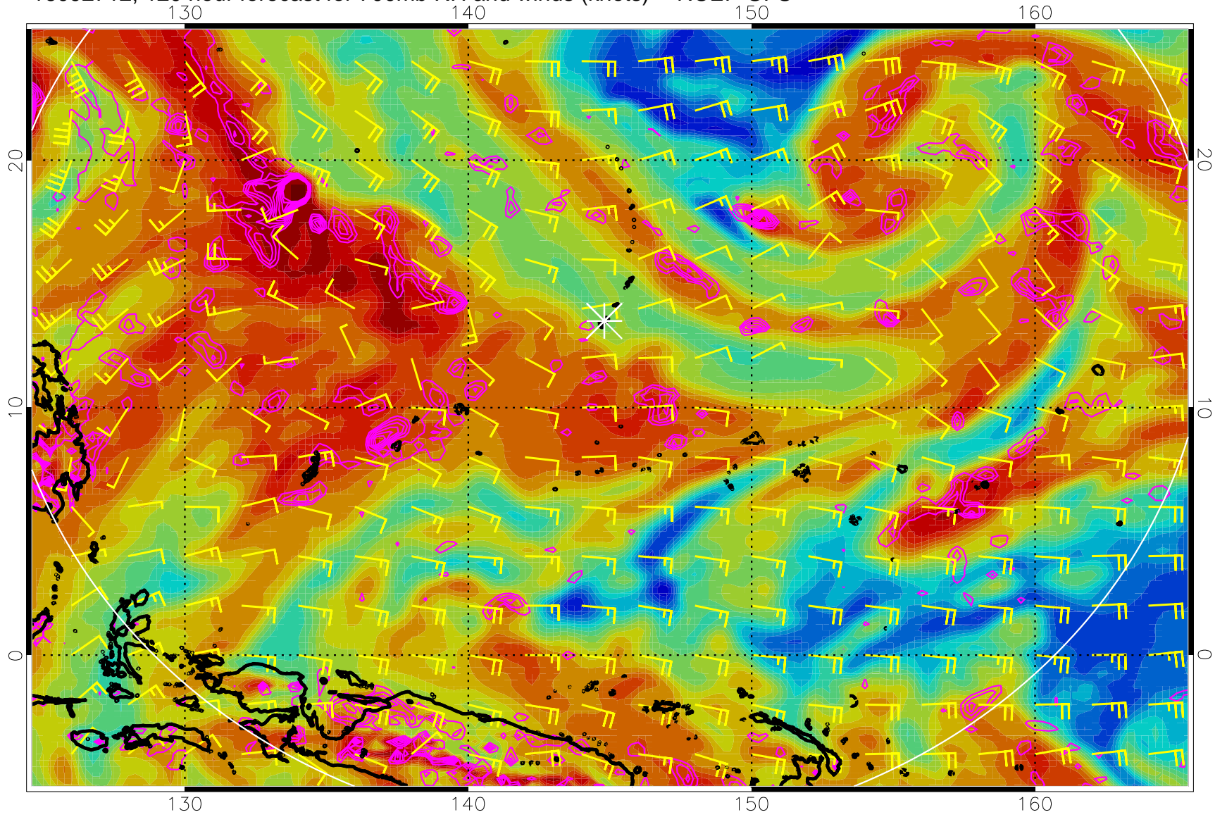
16092712, 120 hour forecast for 700mb RH and winds (knots) -- NCEP GFS
