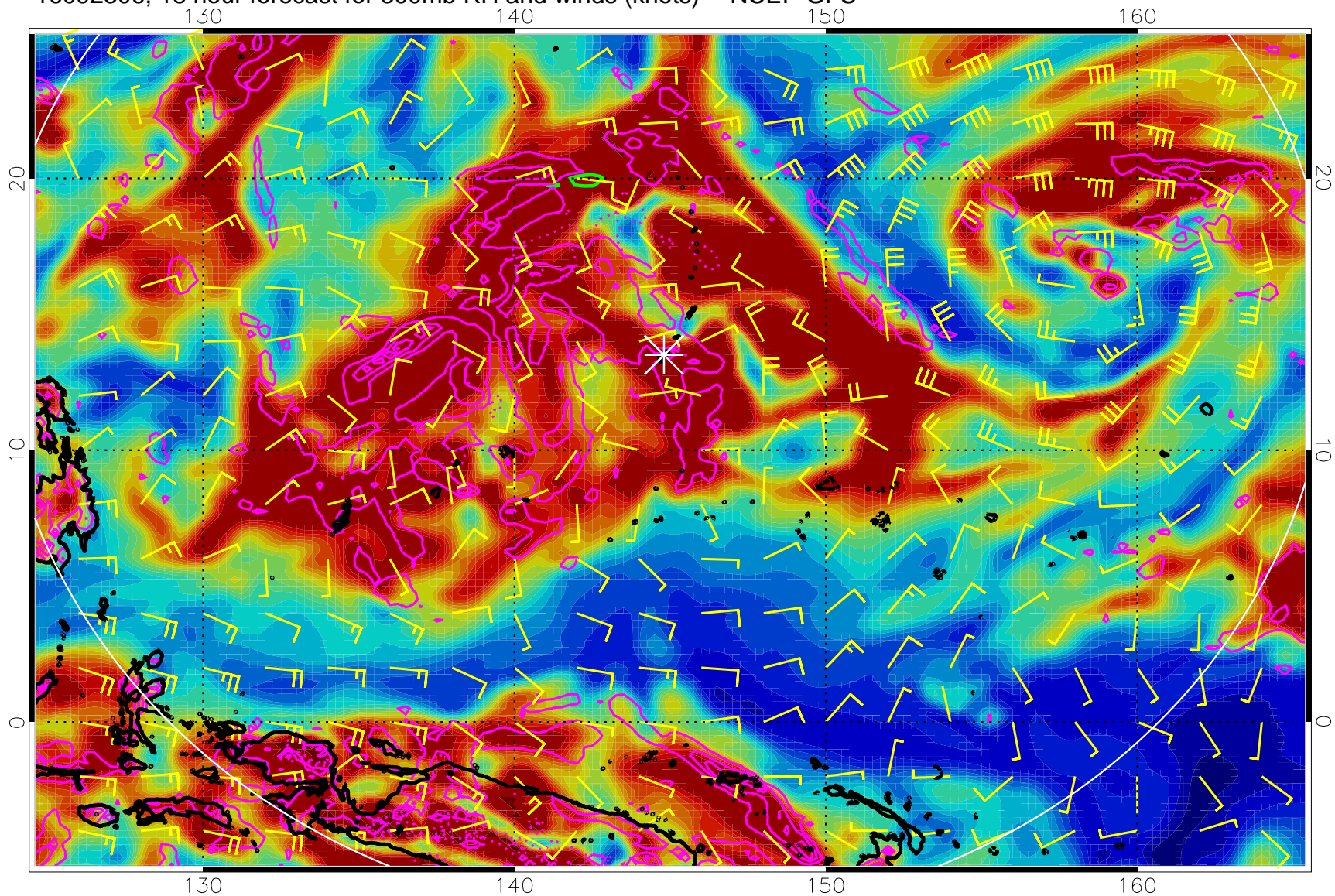
16092306, 18 hour forecast for 300mb RH and winds (knots) -- NCEP GFS
