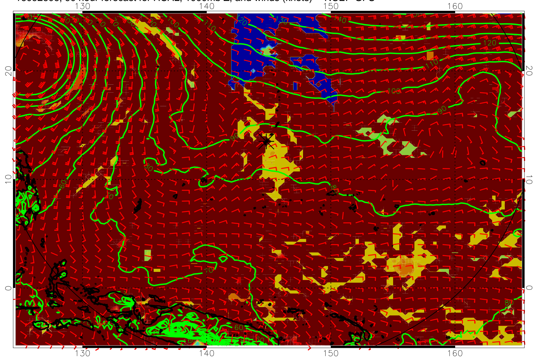
16092606, 90 hour forecast for HCAL, 1000mb Z, and winds (knots) -- NCEP GFS
