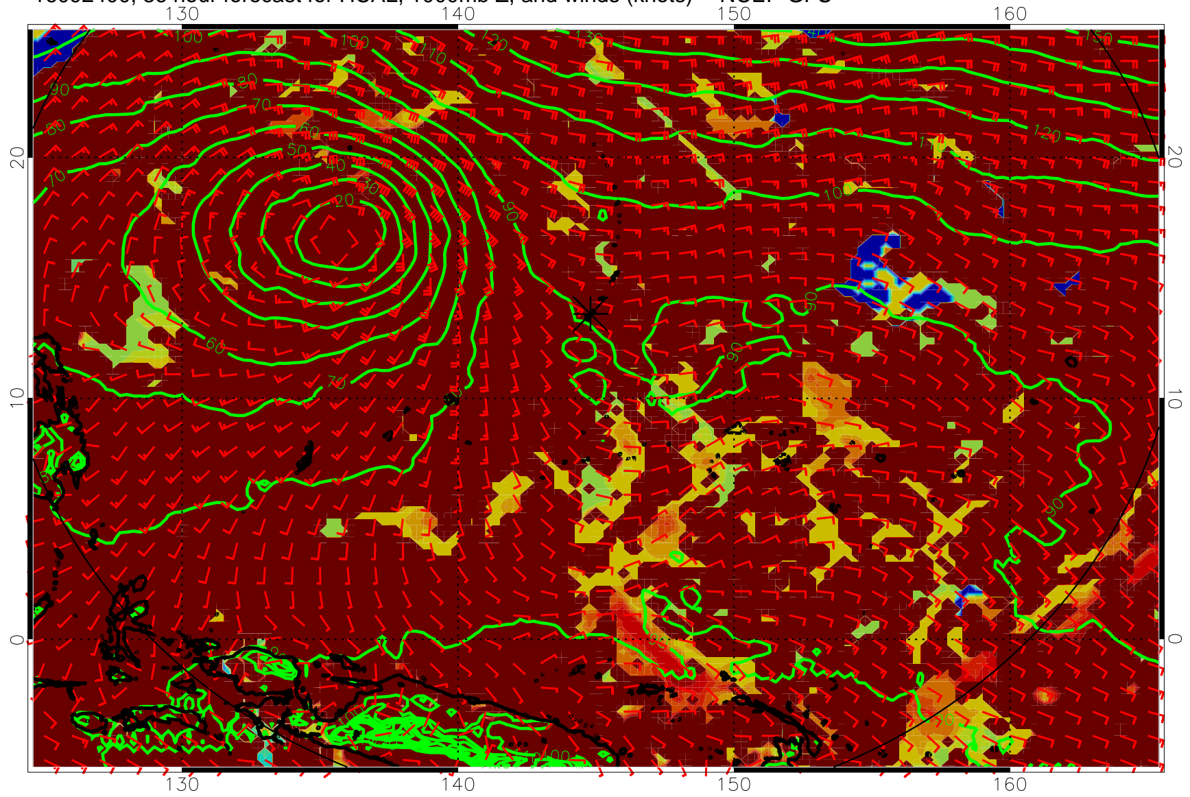
16092400, 36 hour forecast for HCAL, 1000mb Z, and winds (knots) -- NCEP GFS
