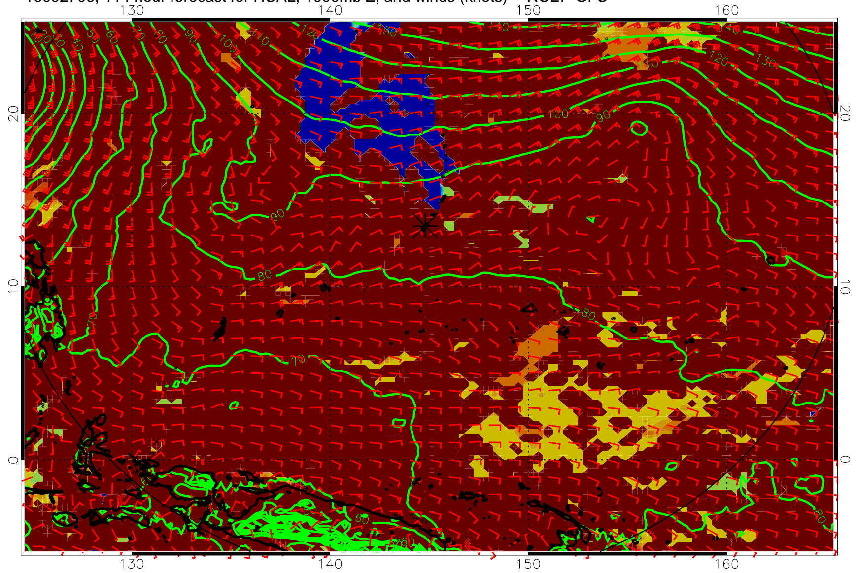
16092706, 114 hour forecast for HCAL, 1000mb Z, and winds (knots) -- NCEP GFS
