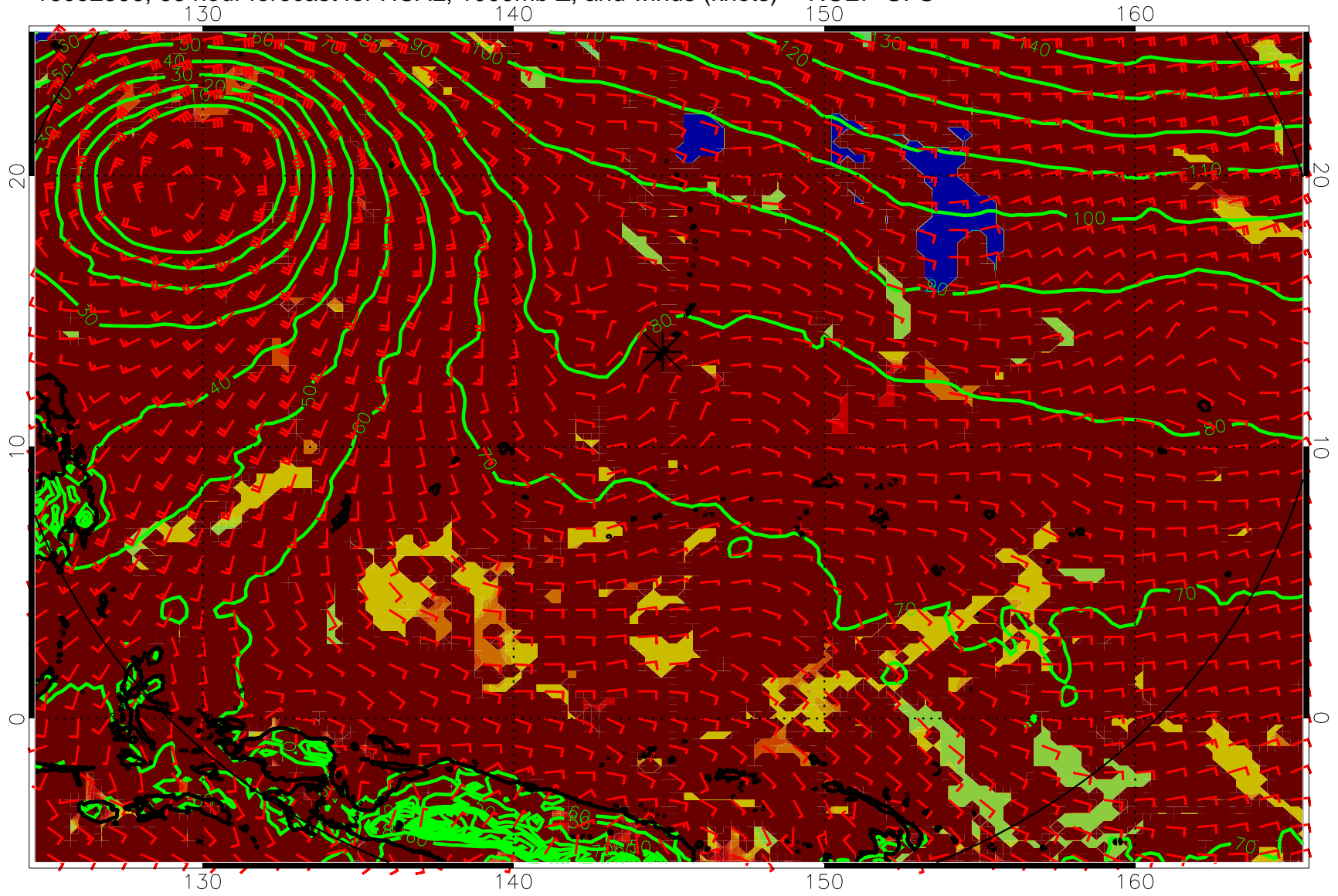
16092506, 66 hour forecast for HCAL, 1000mb Z, and winds (knots) -- NCEP GFS
