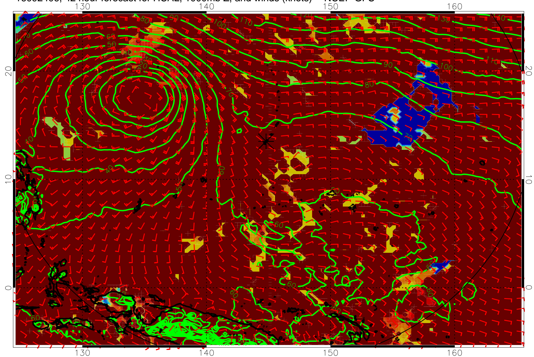
16092406, 42 hour forecast for HCAL, 1000mb Z, and winds (knots) -- NCEP GFS
