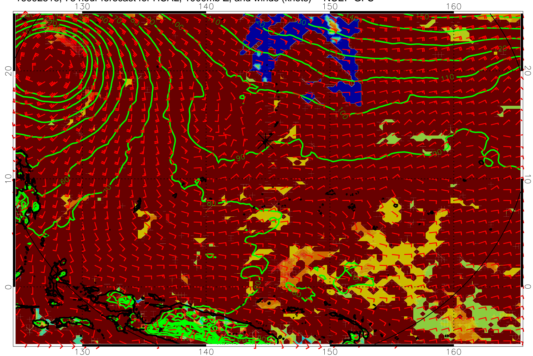
16092518, 78 hour forecast for HCAL, 1000mb Z, and winds (knots) -- NCEP GFS
