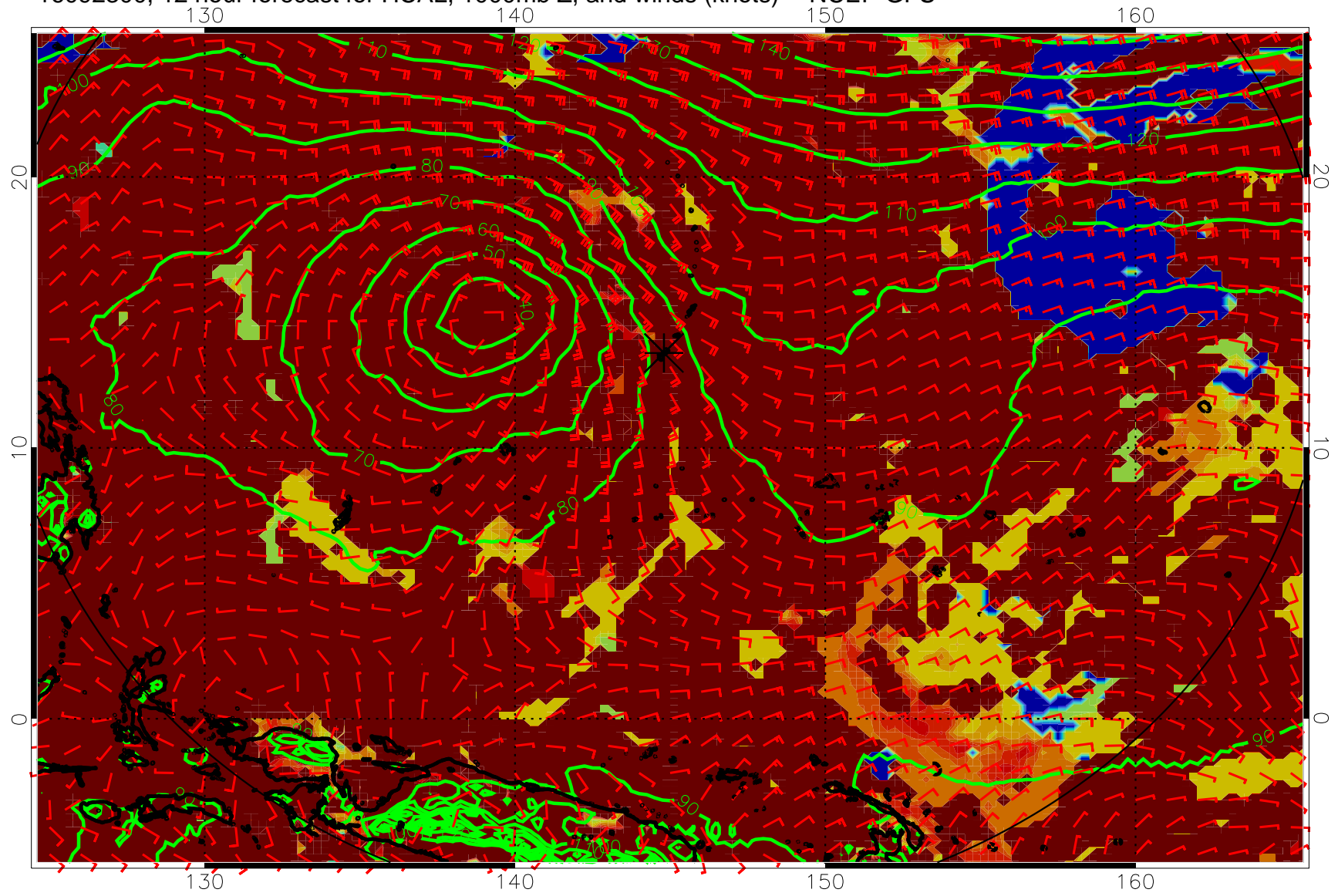
16092300, 12 hour forecast for HCAL, 1000mb Z, and winds (knots) -- NCEP GFS
