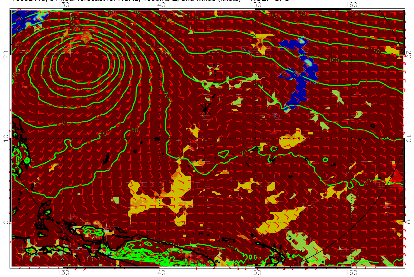
16092418, 54 hour forecast for HCAL, 1000mb Z, and winds (knots) -- NCEP GFS
