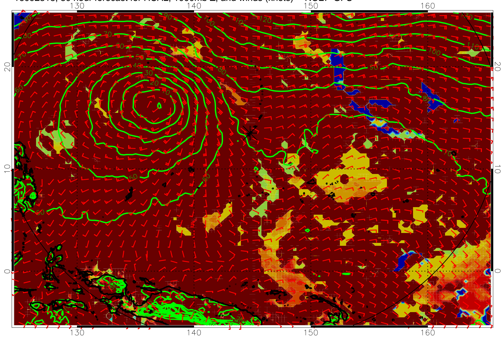
16092318, 30 hour forecast for HCAL, 1000mb Z, and winds (knots) -- NCEP GFS
