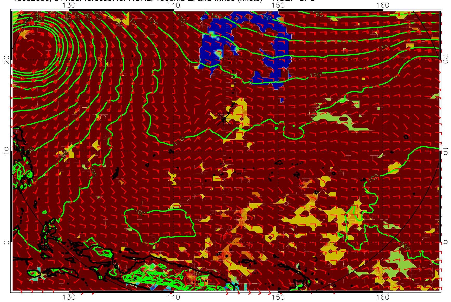
16092600, 84 hour forecast for HCAL, 1000mb Z, and winds (knots) -- NCEP GFS
