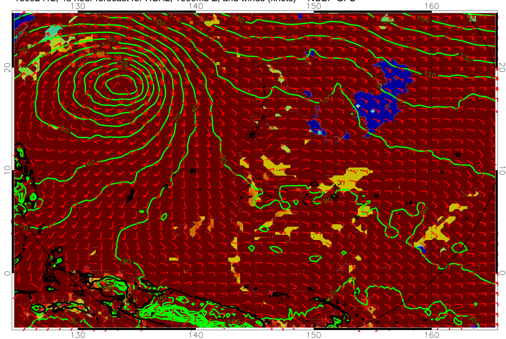
16092412, 48 hour forecast for HCAL, 1000mb Z, and winds (knots) -- NCEP GFS
