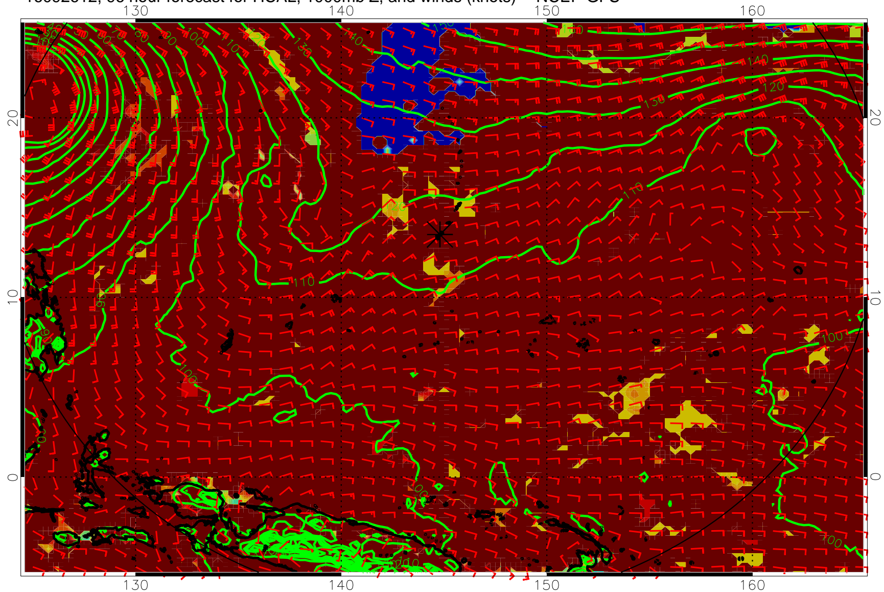
16092612, 96 hour forecast for HCAL, 1000mb Z, and winds (knots) -- NCEP GFS
