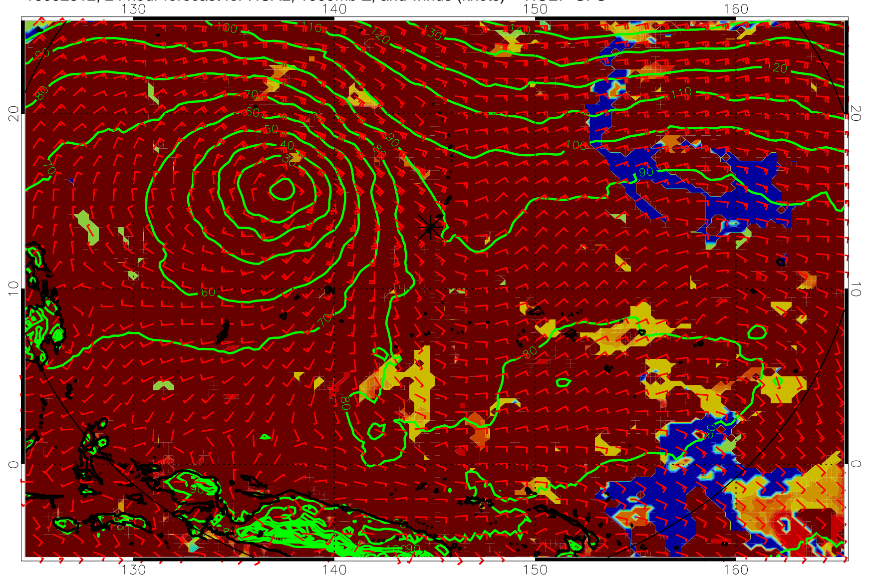
16092312, 24 hour forecast for HCAL, 1000mb Z, and winds (knots) -- NCEP GFS
