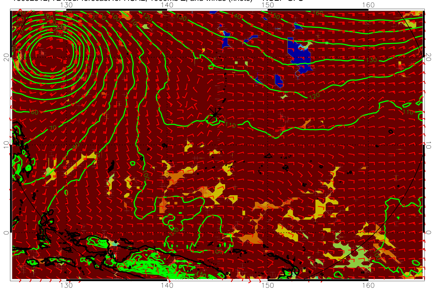
16092512, 72 hour forecast for HCAL, 1000mb Z, and winds (knots) -- NCEP GFS
