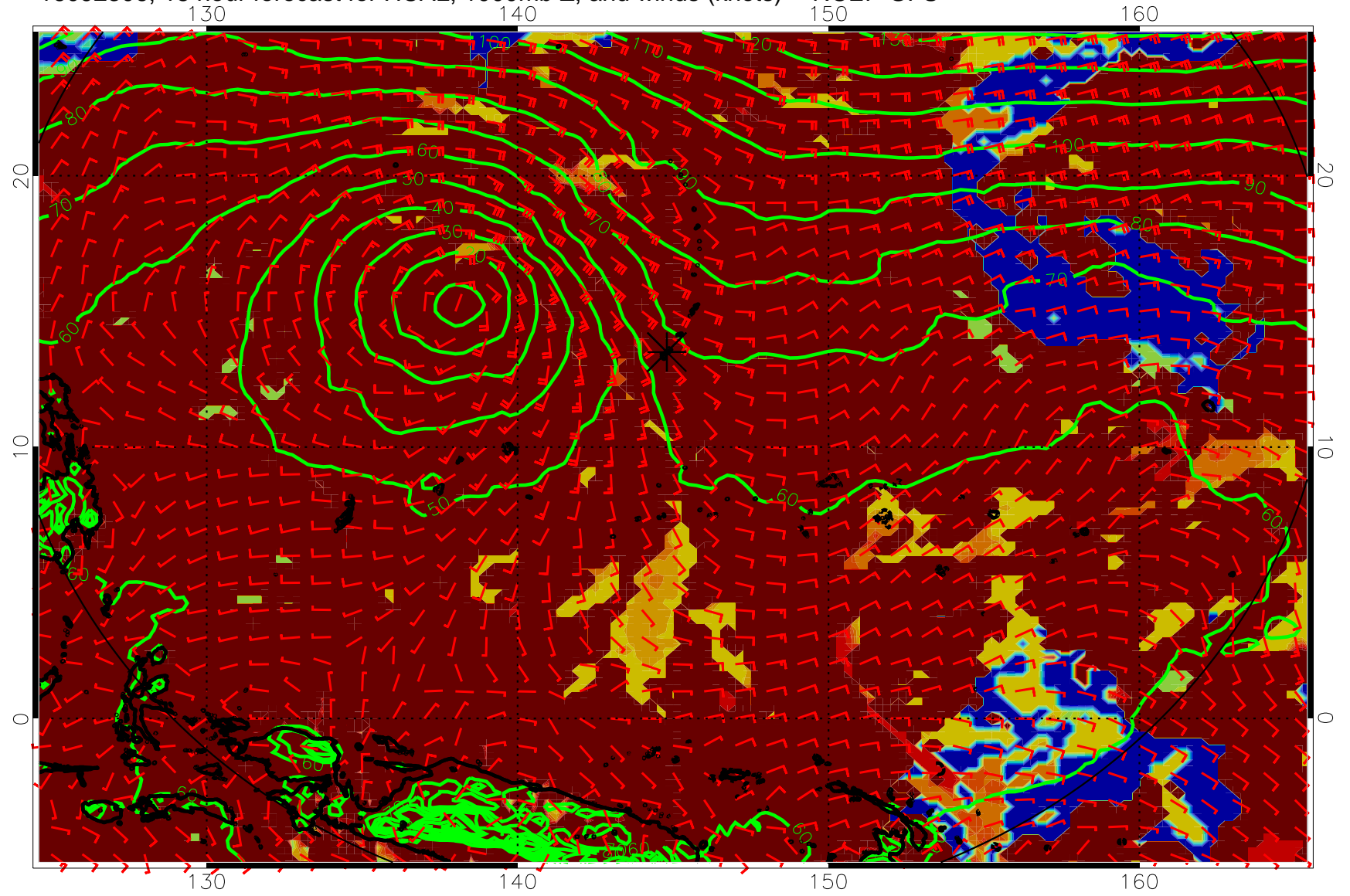
16092306, 18 hour forecast for HCAL, 1000mb Z, and winds (knots) -- NCEP GFS
