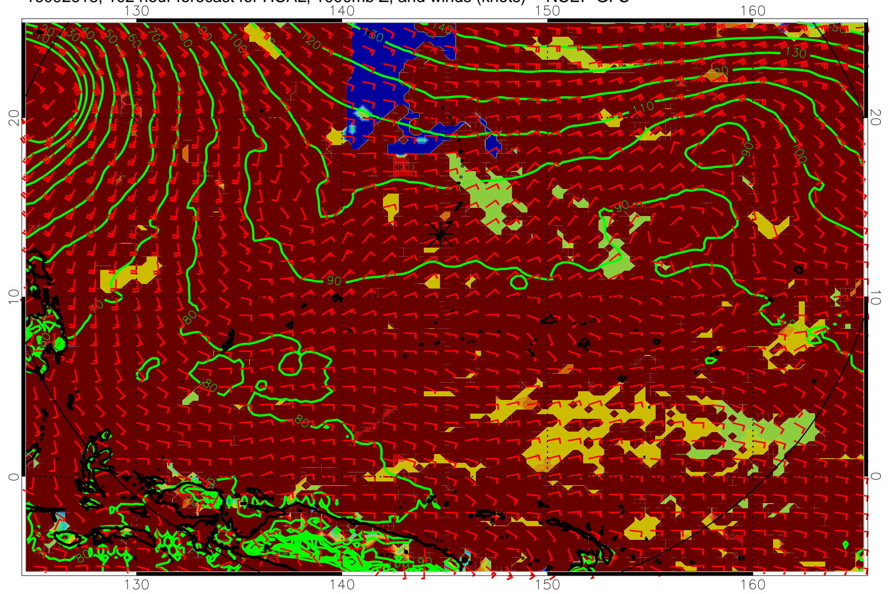
16092618, 102 hour forecast for HCAL, 1000mb Z, and winds (knots) -- NCEP GFS
