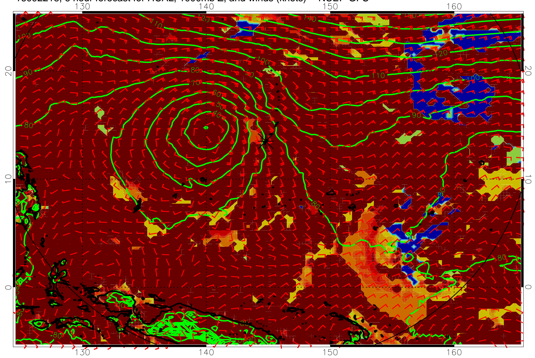
16092218, 6 hour forecast for HCAL, 1000mb Z, and winds (knots) -- NCEP GFS
