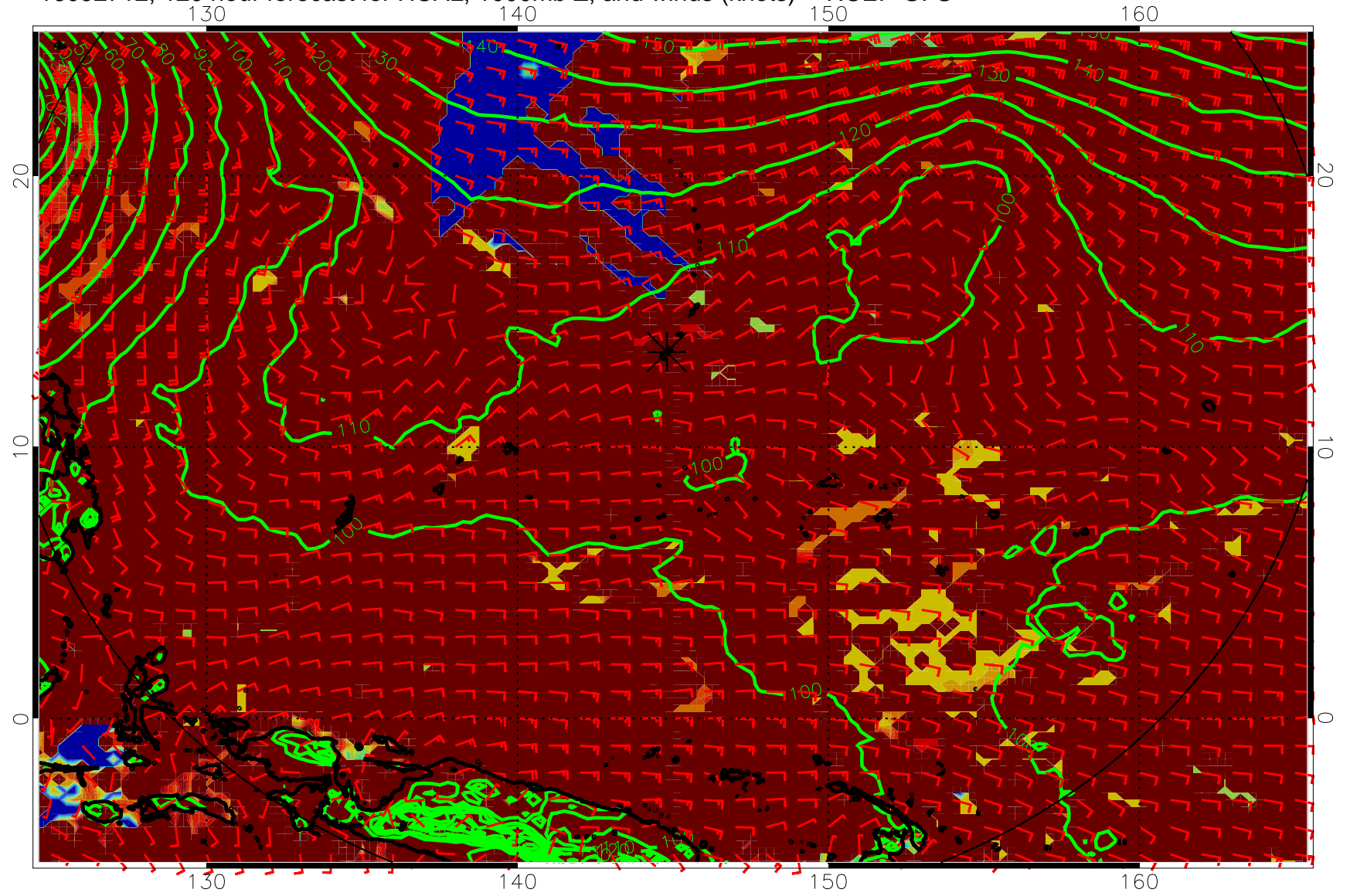
16092712, 120 hour forecast for HCAL, 1000mb Z, and winds (knots) -- NCEP GFS
