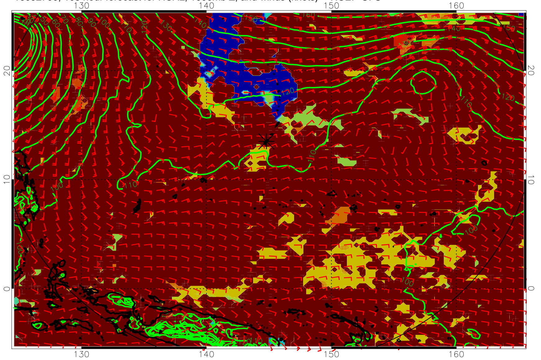
16092700, 108 hour forecast for HCAL, 1000mb Z, and winds (knots) -- NCEP GFS
