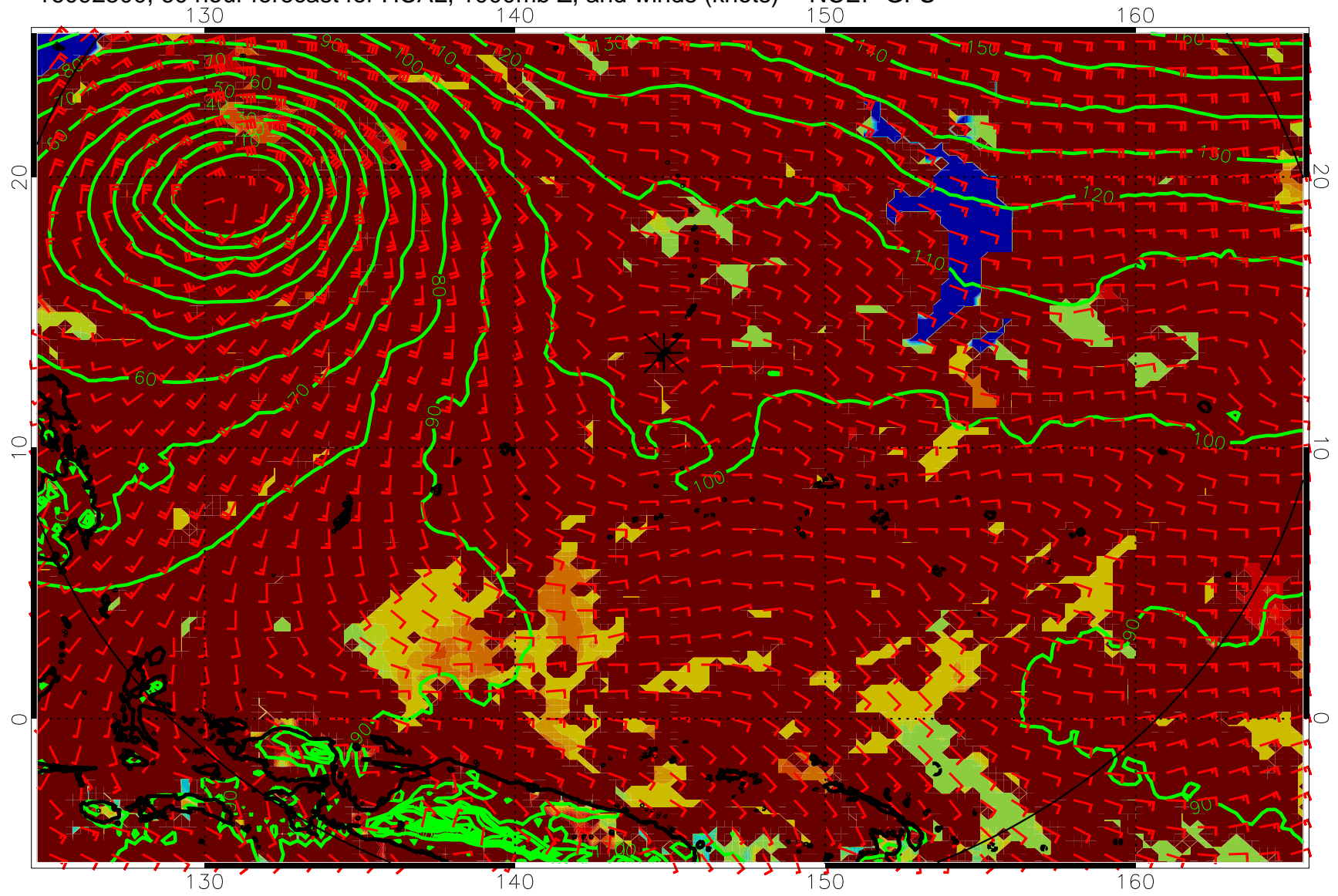
16092500, 60 hour forecast for HCAL, 1000mb Z, and winds (knots) -- NCEP GFS
