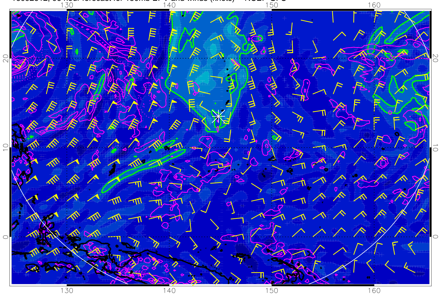
16092612, 96 hour forecast for 150mb EPV and winds (knots) -- NCEP GFS
