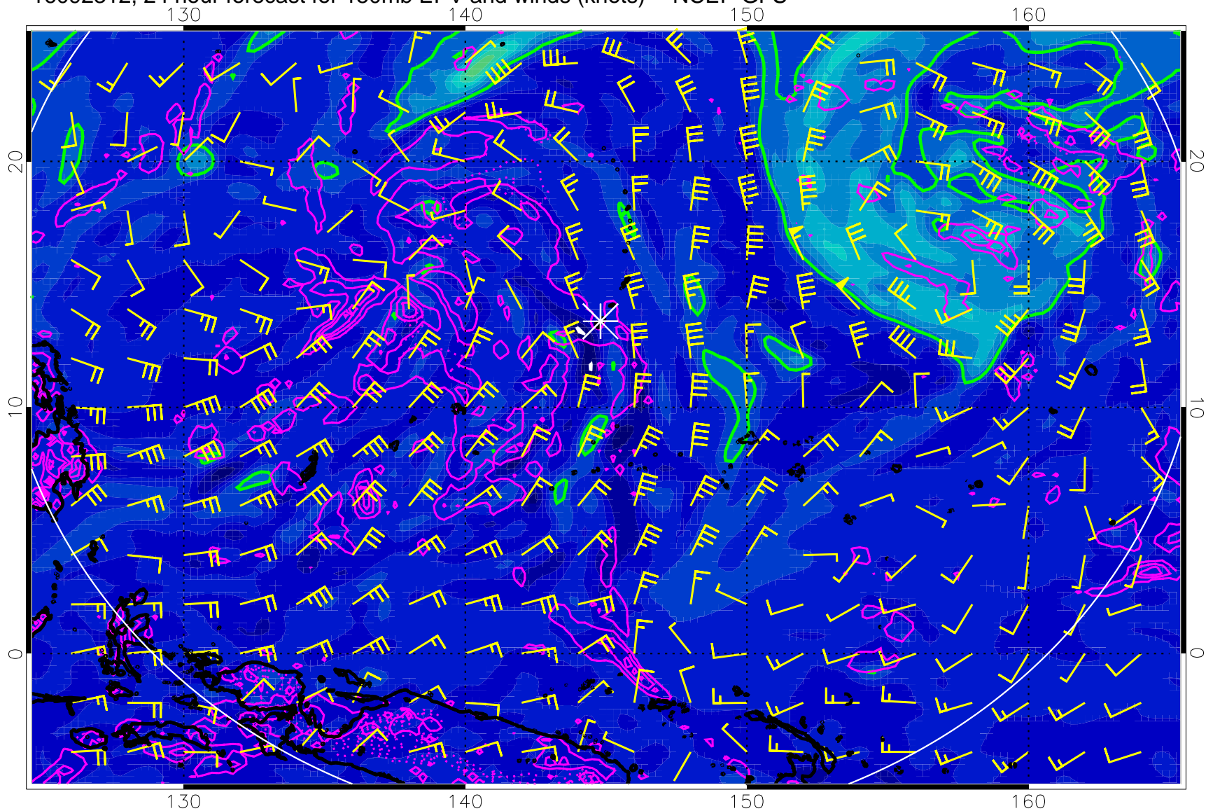
16092312, 24 hour forecast for 150mb EPV and winds (knots) -- NCEP GFS
