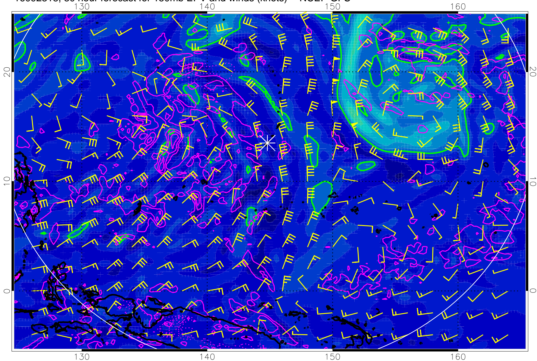
16092318, 30 hour forecast for 150mb EPV and winds (knots) -- NCEP GFS
