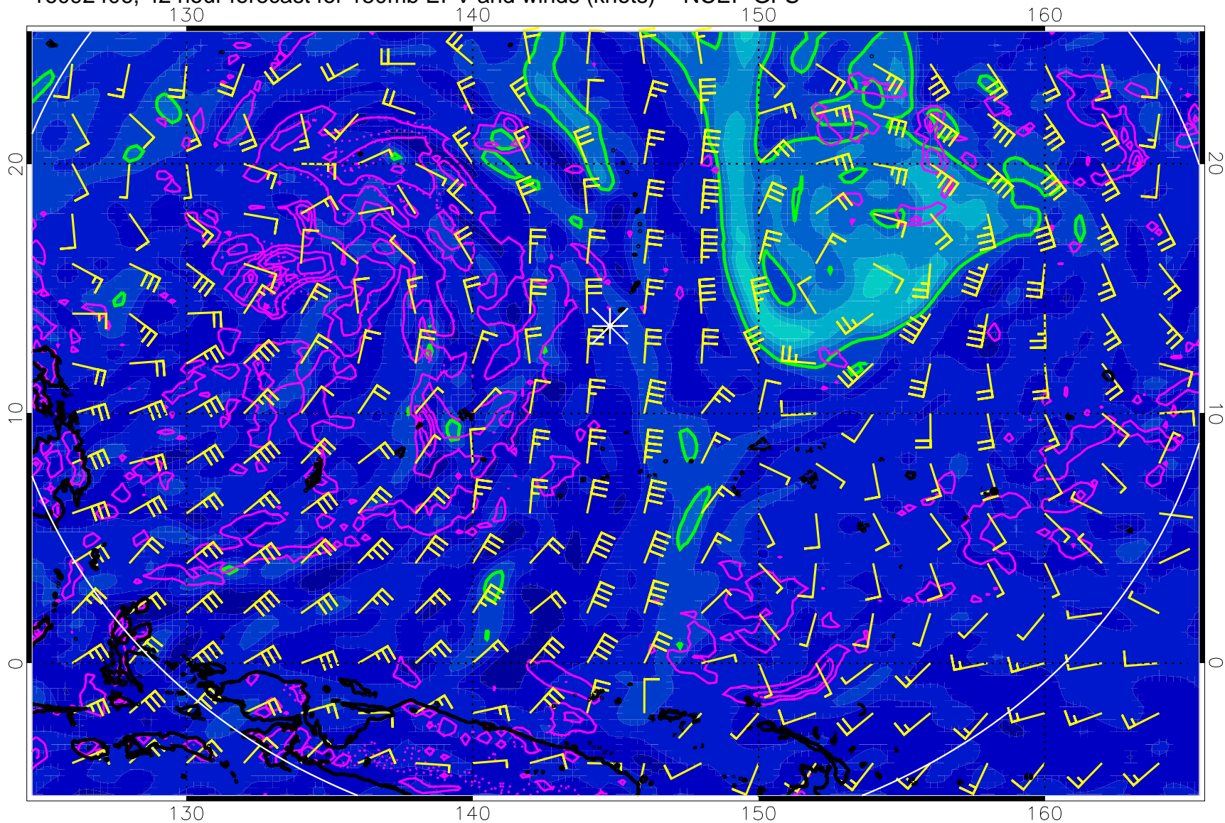
16092406, 42 hour forecast for 150mb EPV and winds (knots) -- NCEP GFS
