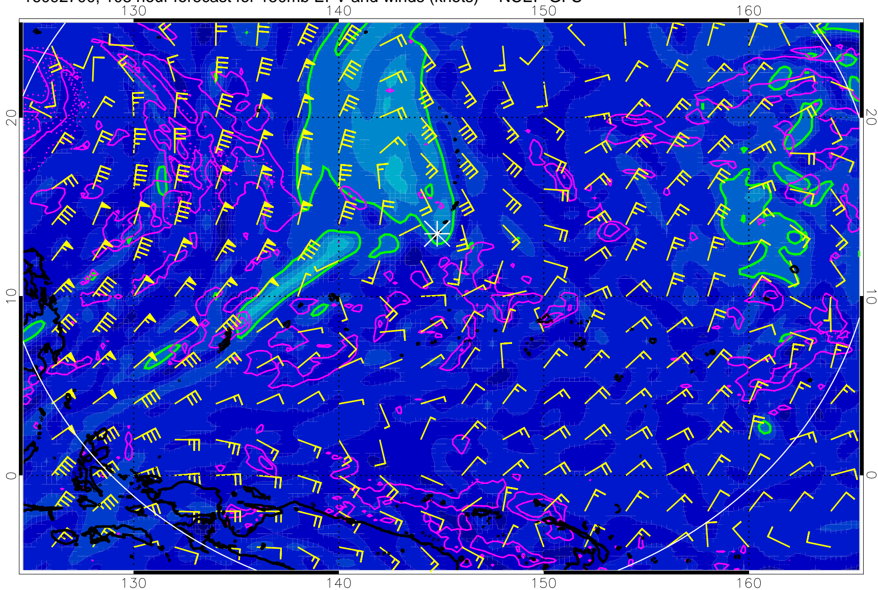
16092700, 108 hour forecast for 150mb EPV and winds (knots) -- NCEP GFS
