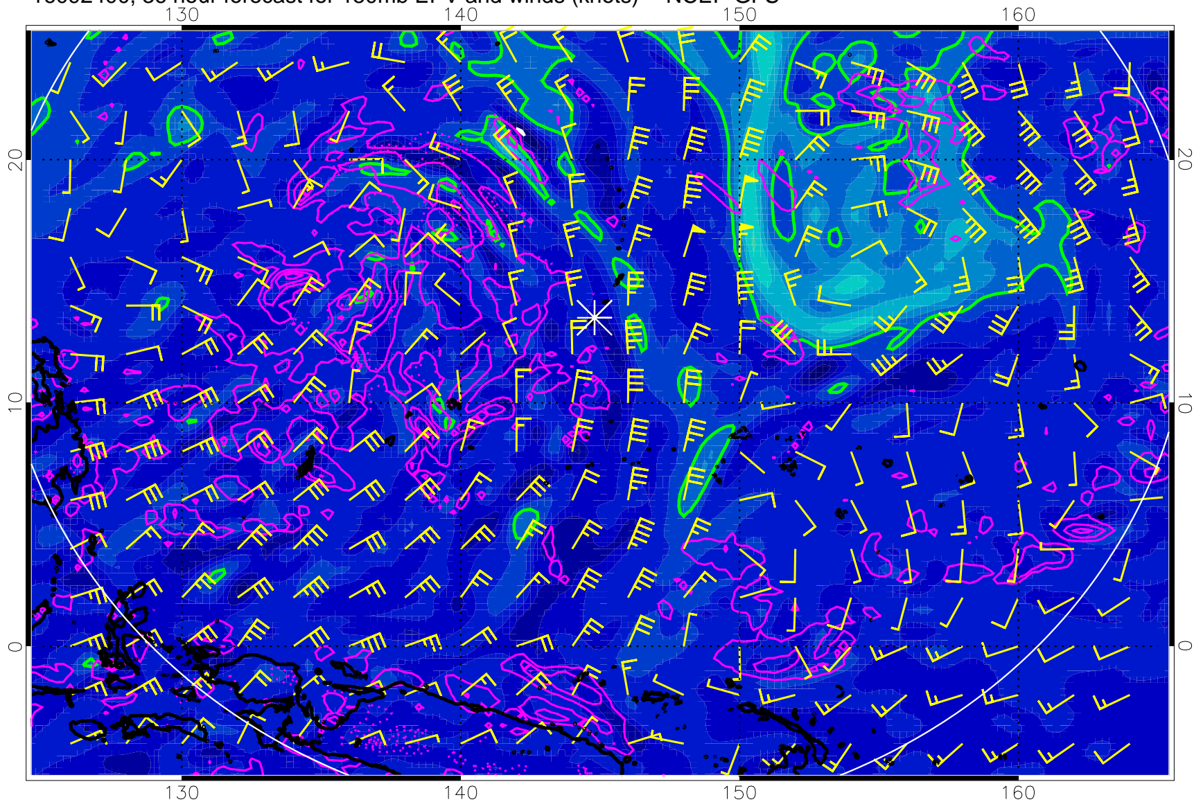
16092400, 36 hour forecast for 150mb EPV and winds (knots) -- NCEP GFS
