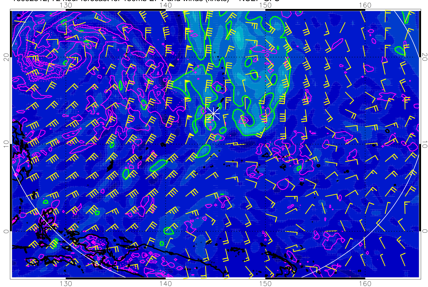
16092512, 72 hour forecast for 150mb EPV and winds (knots) -- NCEP GFS
