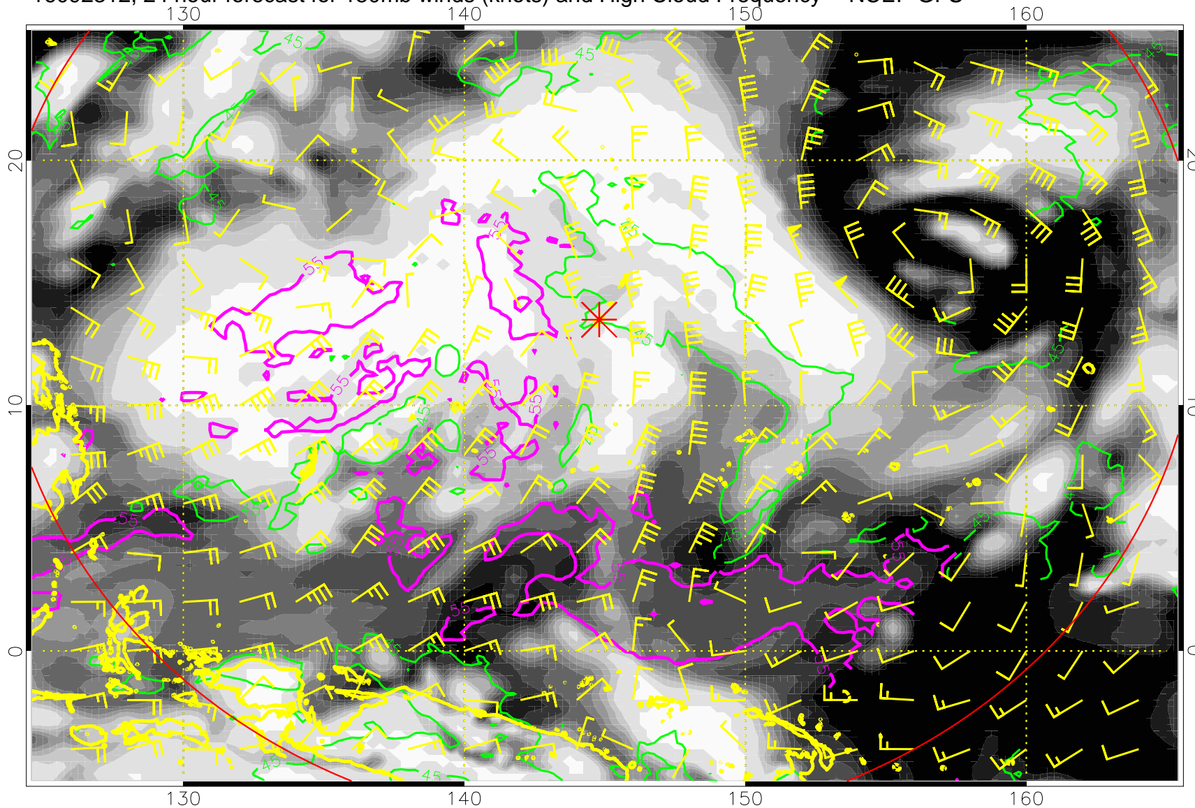
16092312, 24 hour forecast for 150mb winds (knots) and High Cloud Frequency -- NCEP GFS
