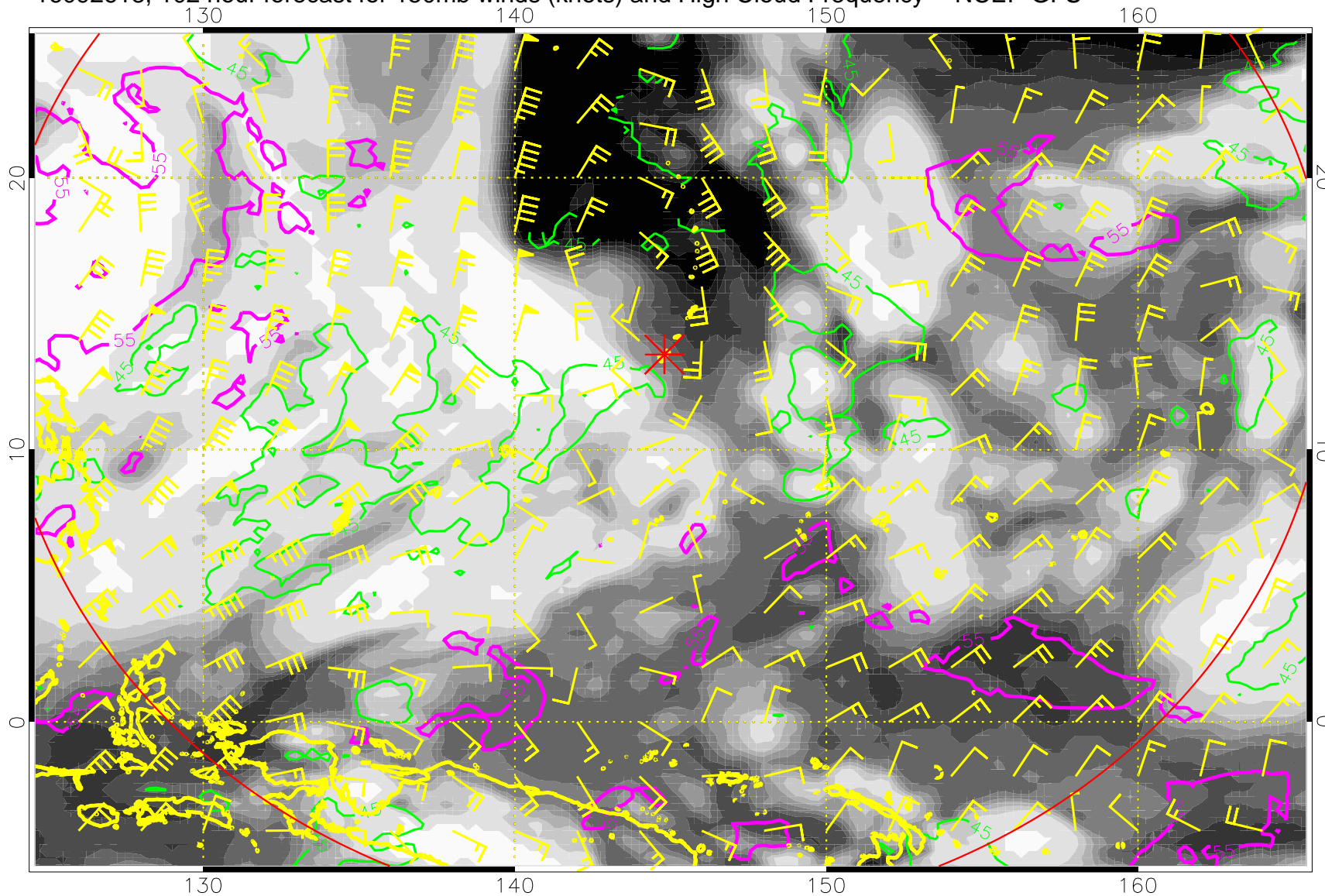
16092618, 102 hour forecast for 150mb winds (knots) and High Cloud Frequency -- NCEP GFS
