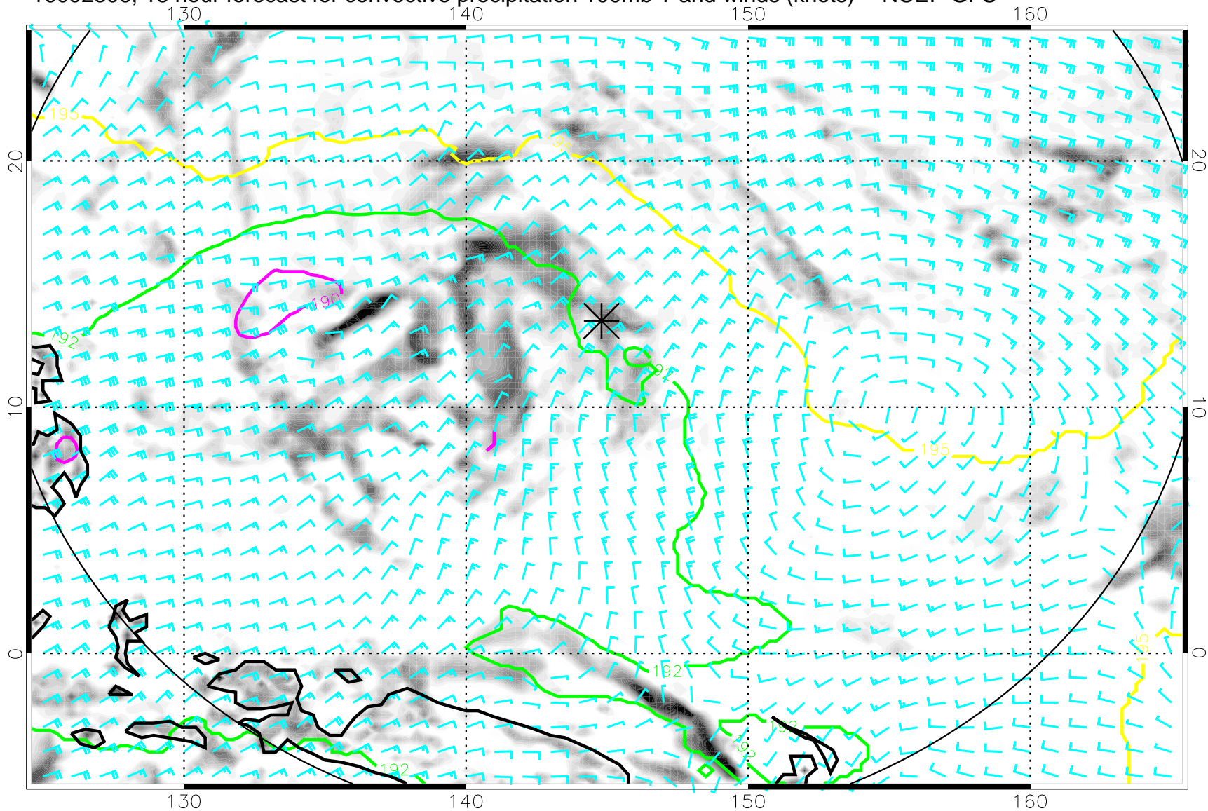
16092306, 18 hour forecast for convective precipitation 100mb T and winds (knots) -- NCEP GFS
