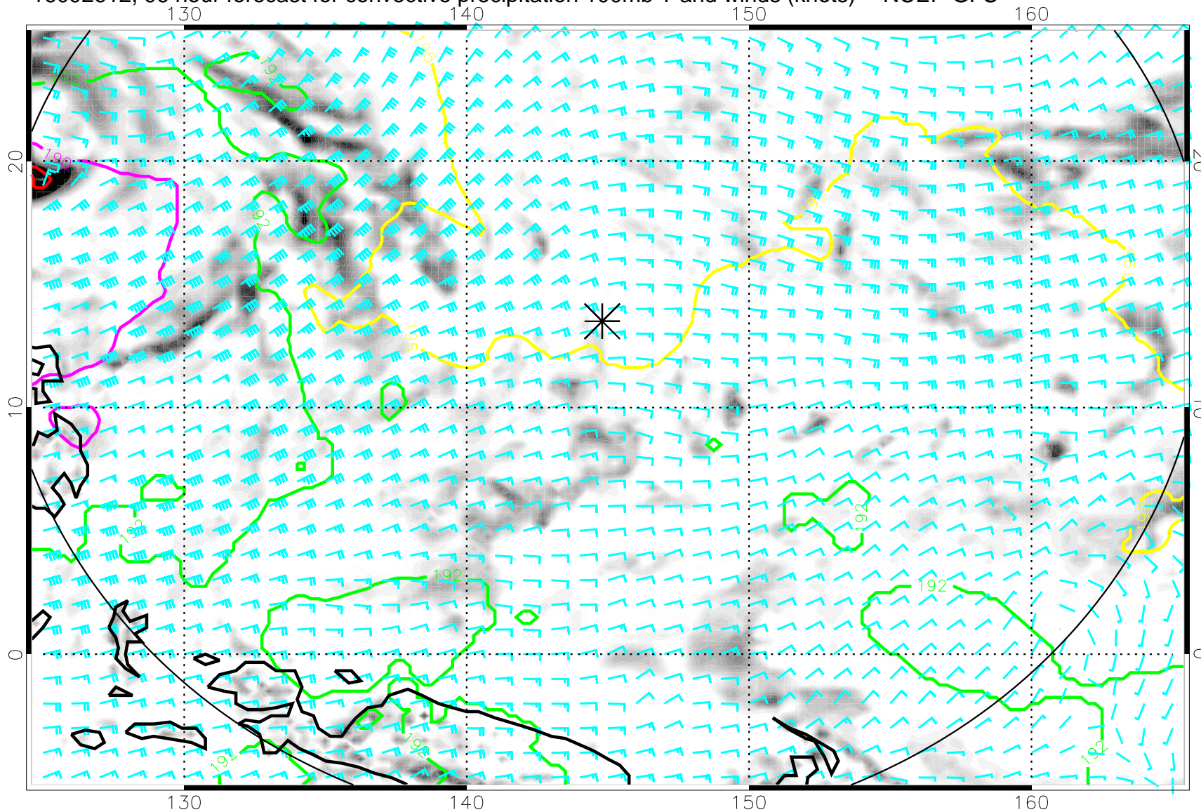
16092612, 96 hour forecast for convective precipitation 100mb T and winds (knots) -- NCEP GFS
