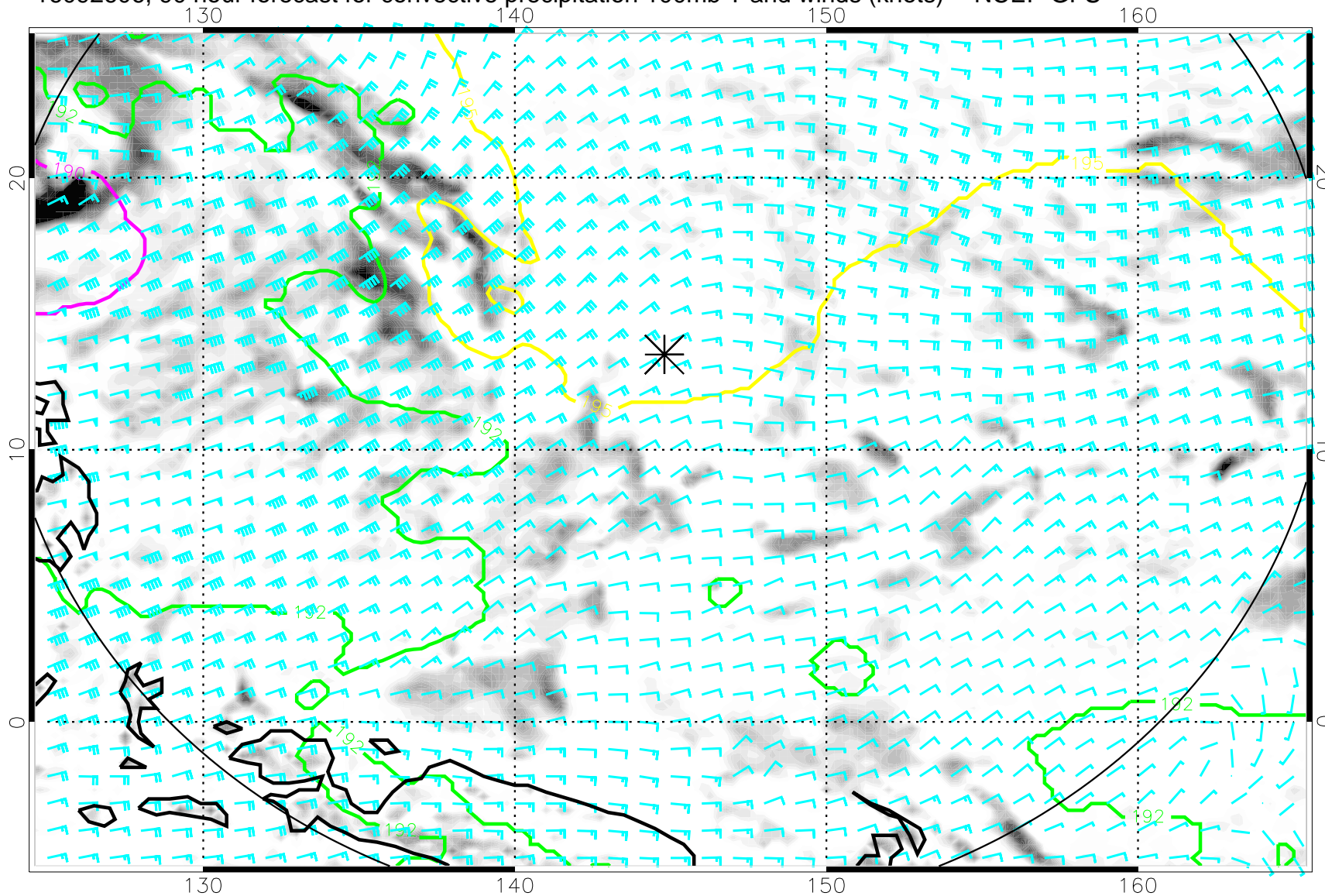
16092606, 90 hour forecast for convective precipitation 100mb T and winds (knots) -- NCEP GFS
