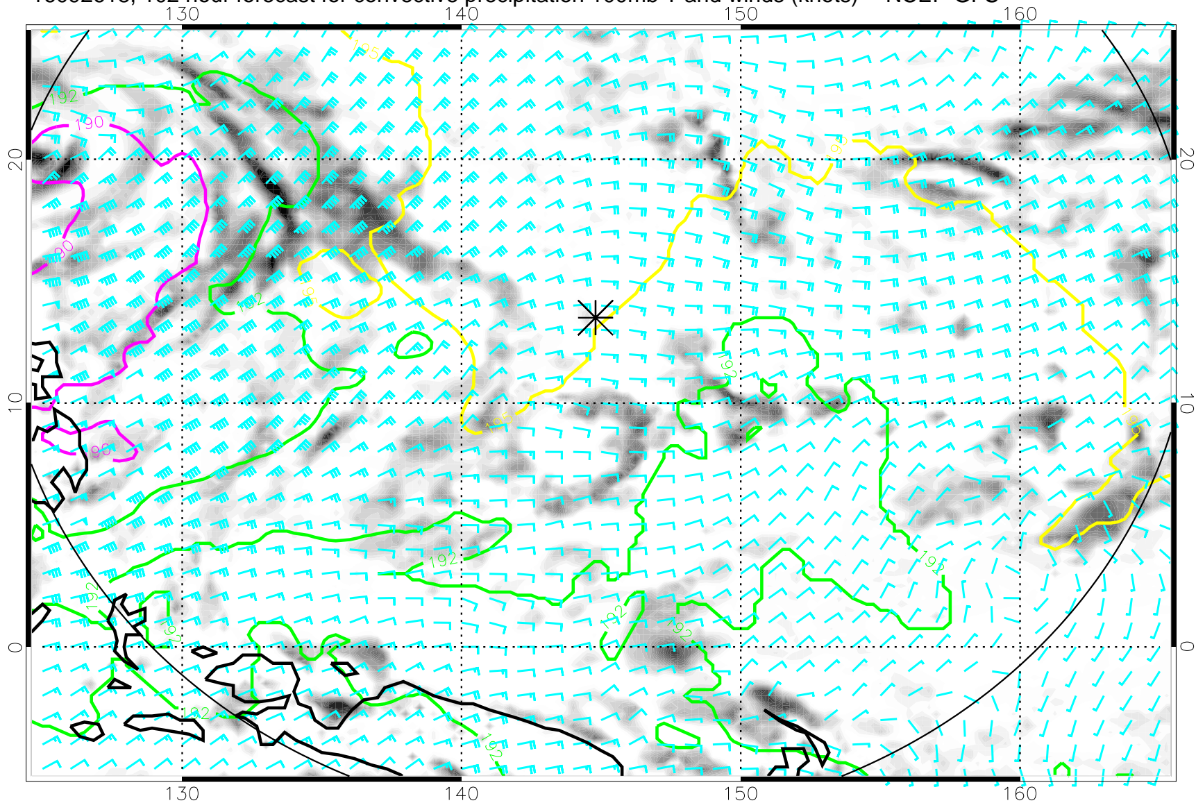
16092618, 102 hour forecast for convective precipitation 100mb T and winds (knots) -- NCEP GFS
