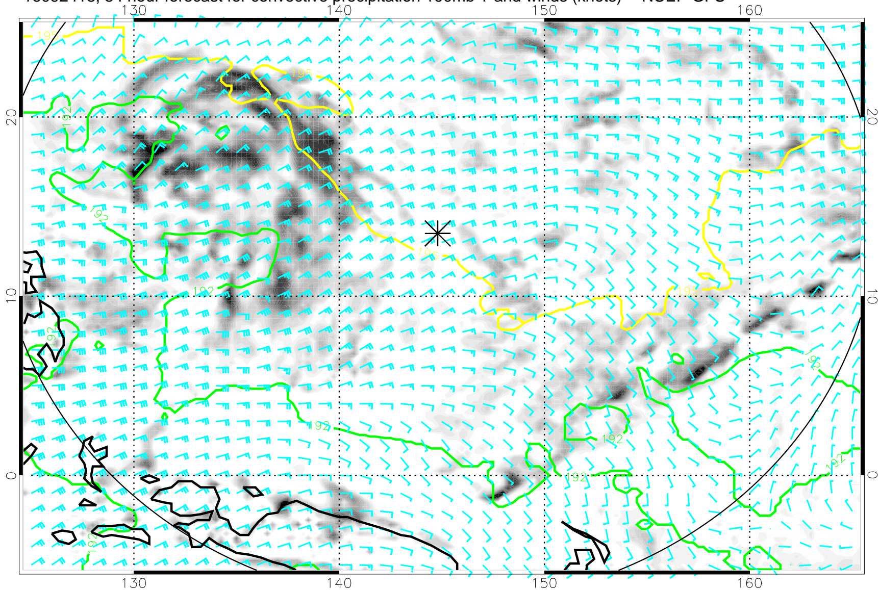
16092418, 54 hour forecast for convective precipitation 100mb T and winds (knots) -- NCEP GFS
