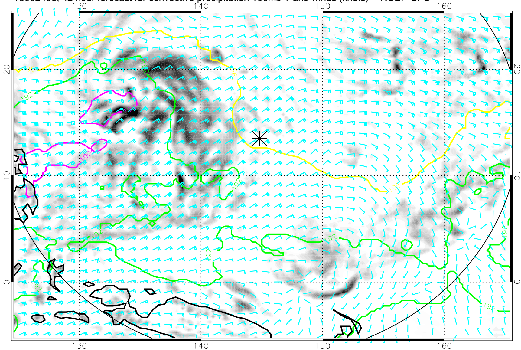
16092406, 42 hour forecast for convective precipitation 100mb T and winds (knots) -- NCEP GFS
