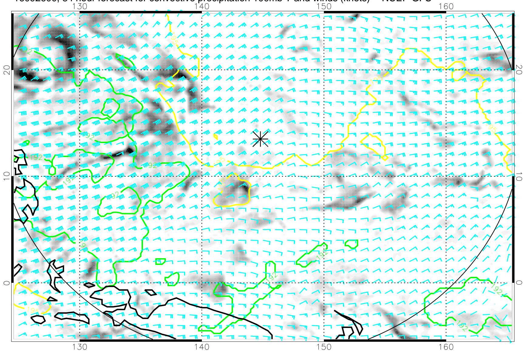
16092600, 84 hour forecast for convective precipitation 100mb T and winds (knots) -- NCEP GFS
