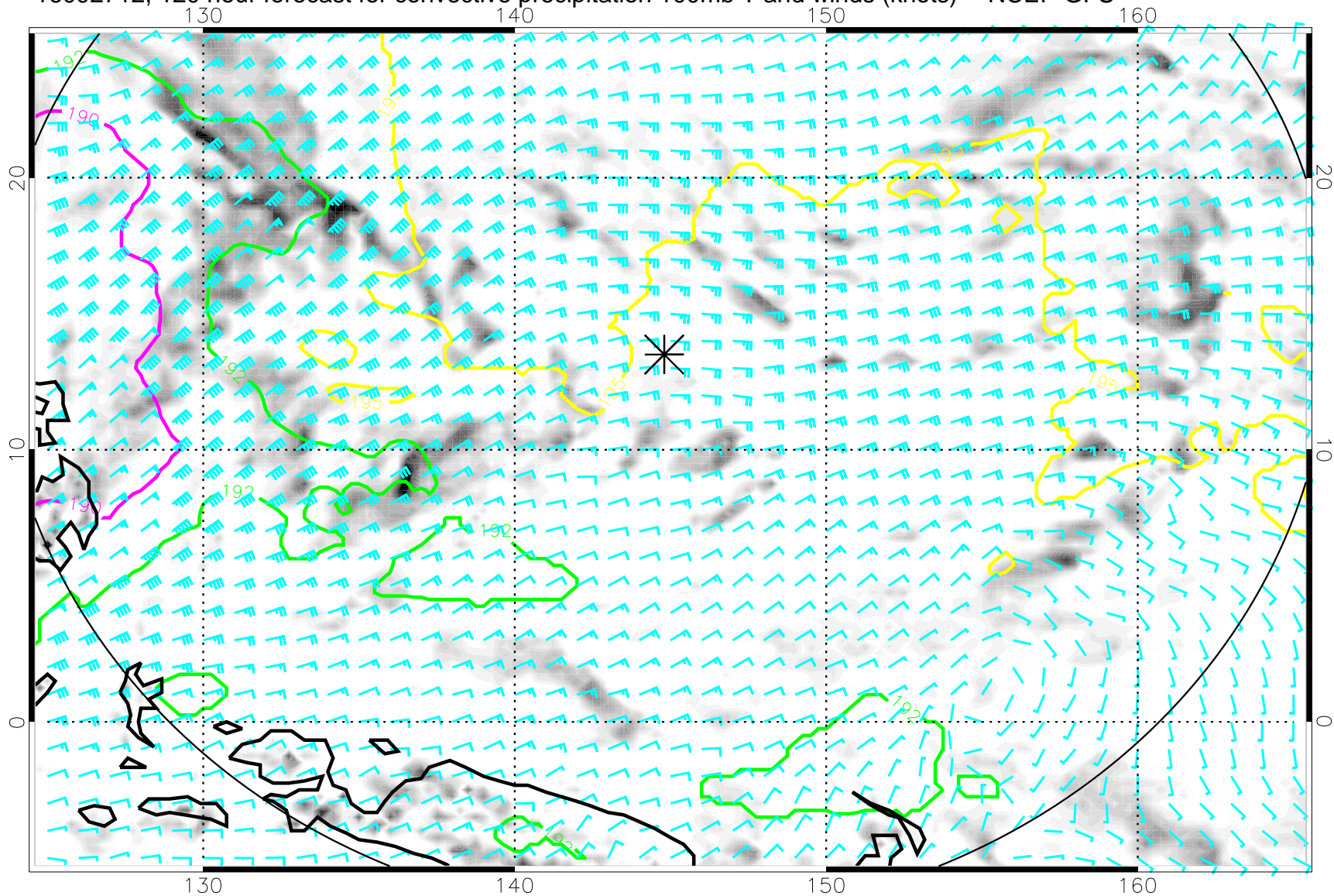
16092712, 120 hour forecast for convective precipitation 100mb T and winds (knots) -- NCEP GFS
