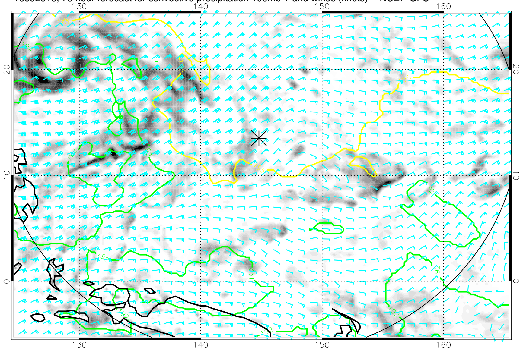
16092518, 78 hour forecast for convective precipitation 100mb T and winds (knots) -- NCEP GFS
