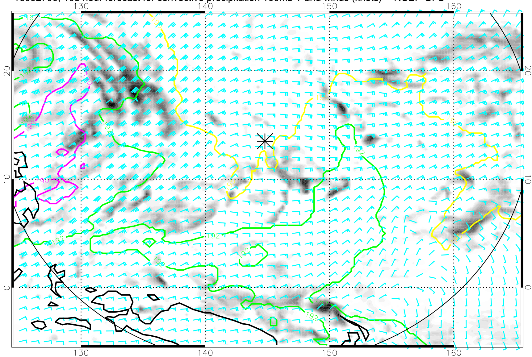
16092700, 108 hour forecast for convective precipitation 100mb T and winds (knots) -- NCEP GFS
