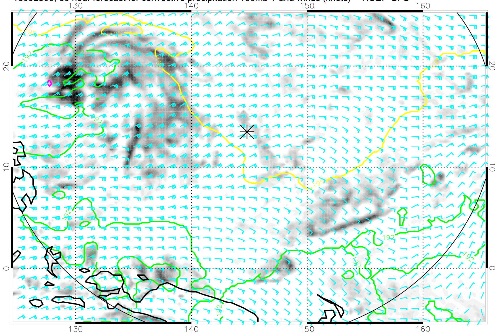
16092500, 60 hour forecast for convective precipitation 100mb T and winds (knots) -- NCEP GFS
