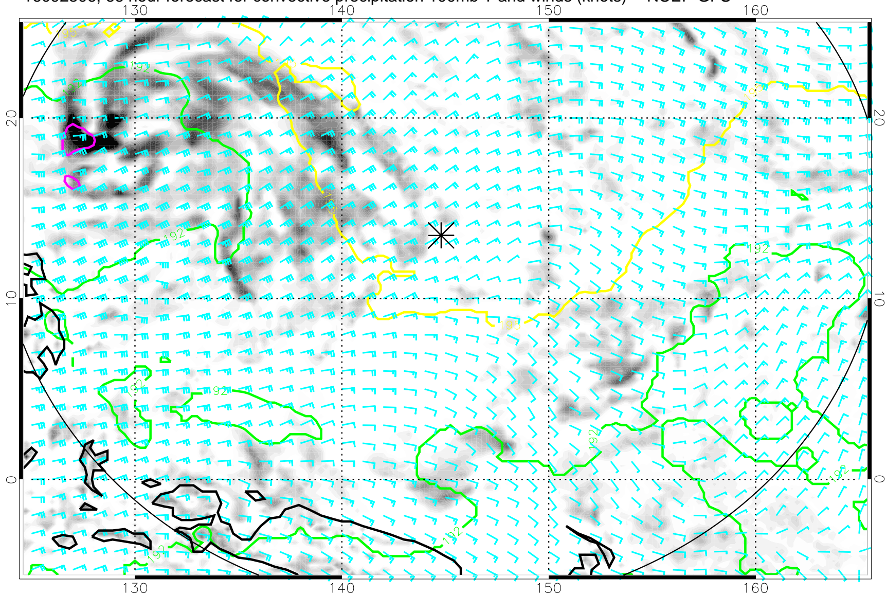
16092506, 66 hour forecast for convective precipitation 100mb T and winds (knots) -- NCEP GFS
