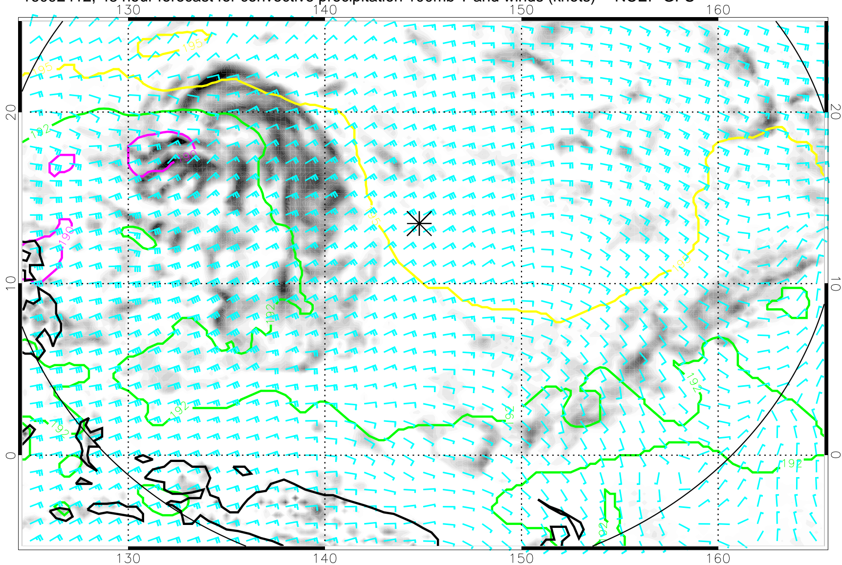
16092412, 48 hour forecast for convective precipitation 100mb T and winds (knots) -- NCEP GFS
