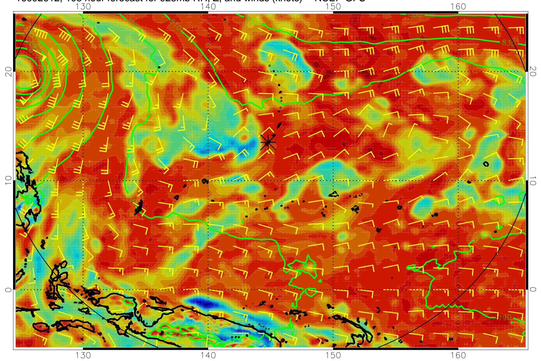
16092612, 108 hour forecast for 925mb RH, Z, and winds (knots) -- NCEP GFS
