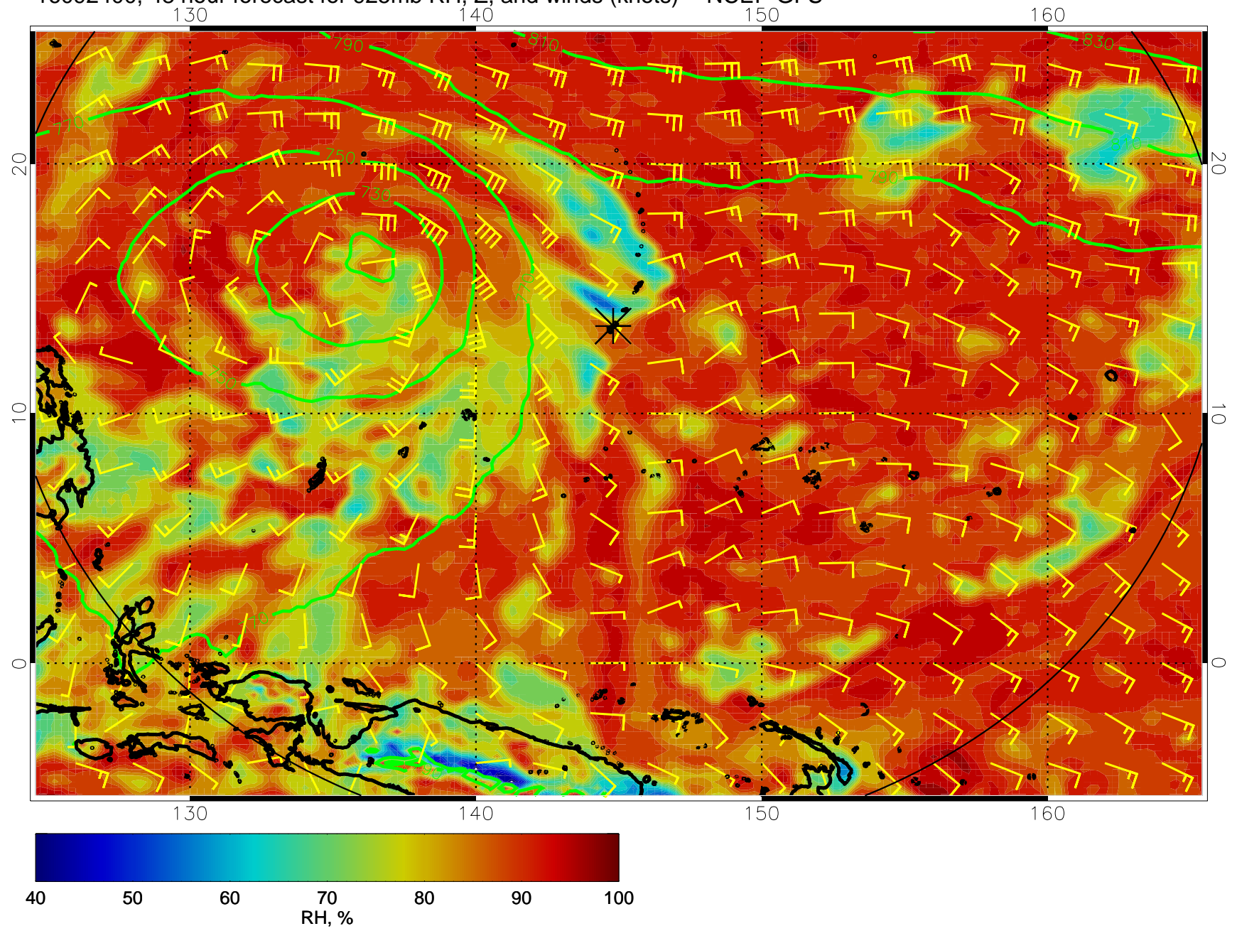
16092400, 48 hour forecast for 925mb RH, Z, and winds (knots) -- NCEP GFS
