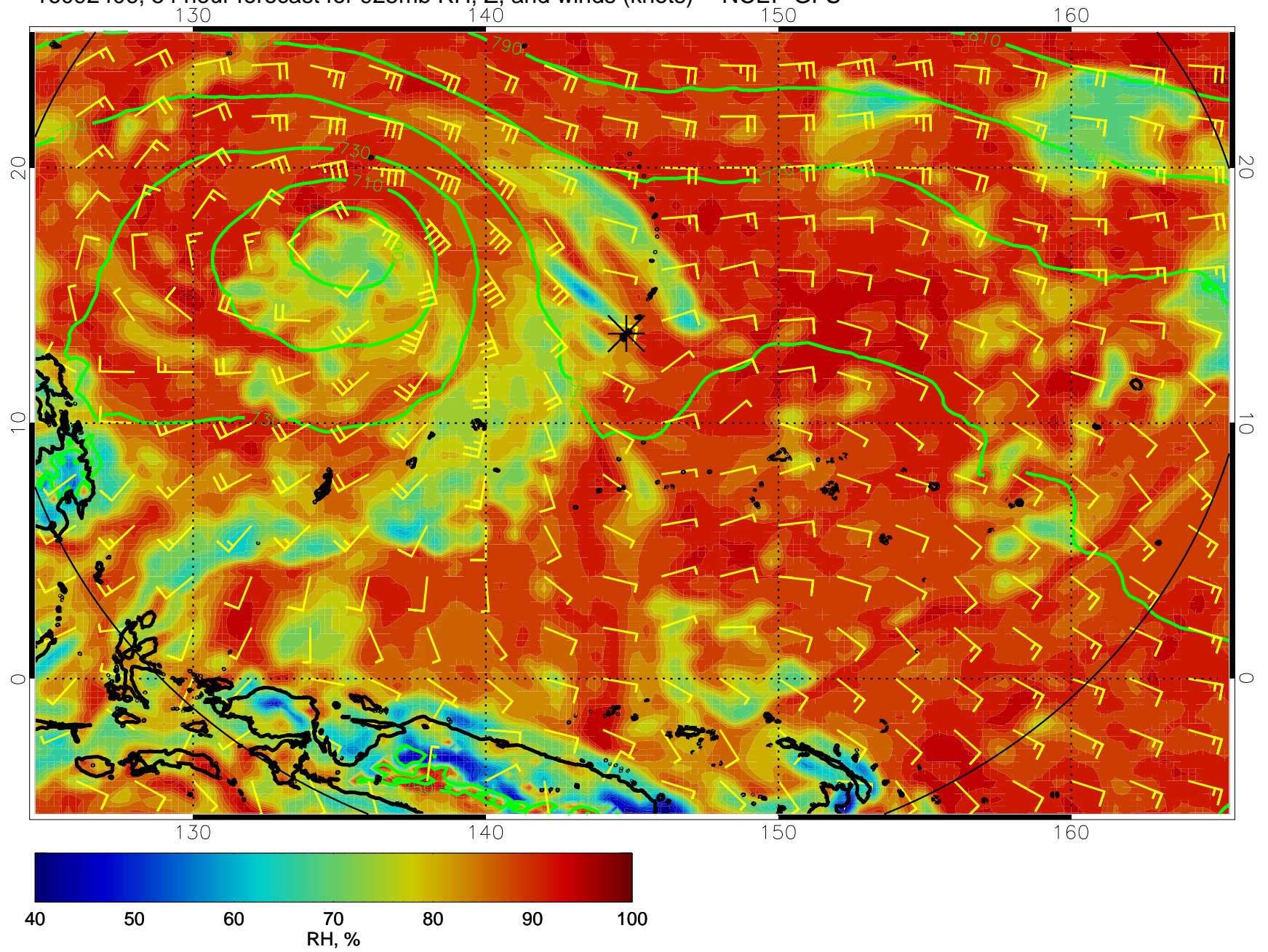
16092406, 54 hour forecast for 925mb RH, Z, and winds (knots) -- NCEP GFS
