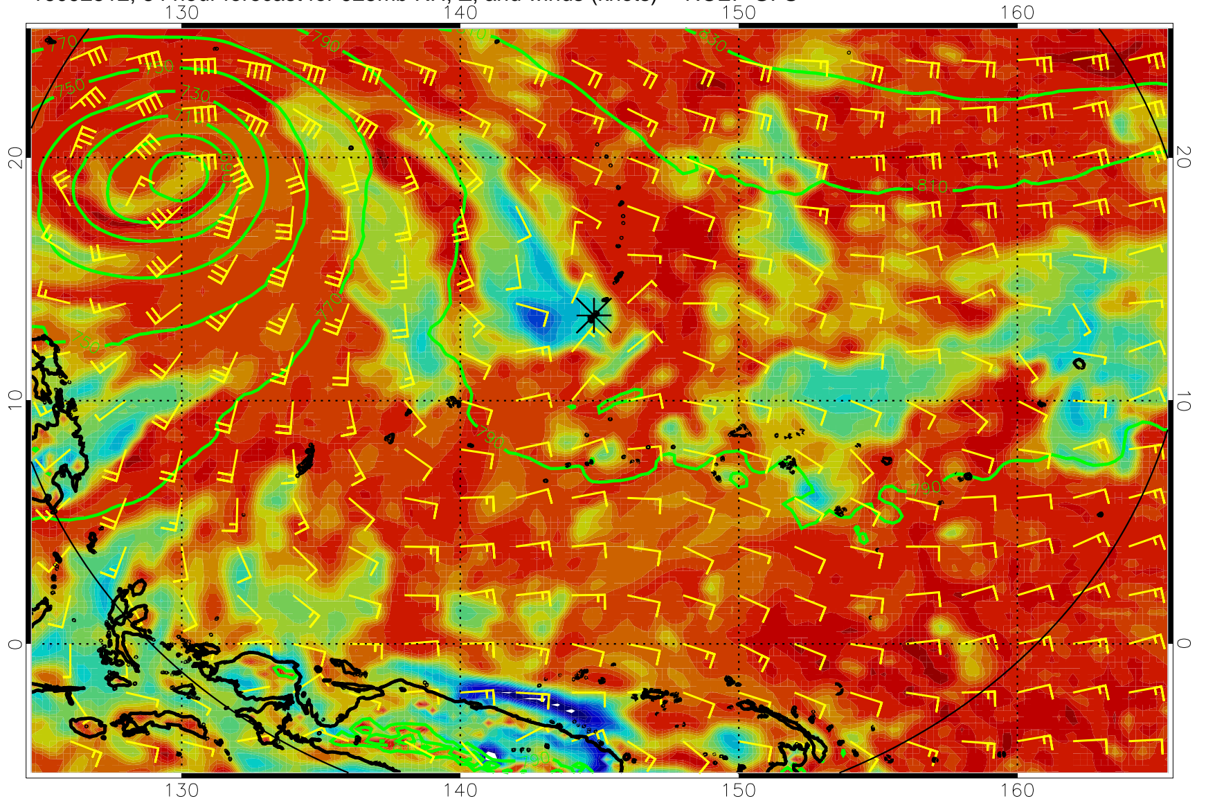
16092512, 84 hour forecast for 925mb RH, Z, and winds (knots) -- NCEP GFS
