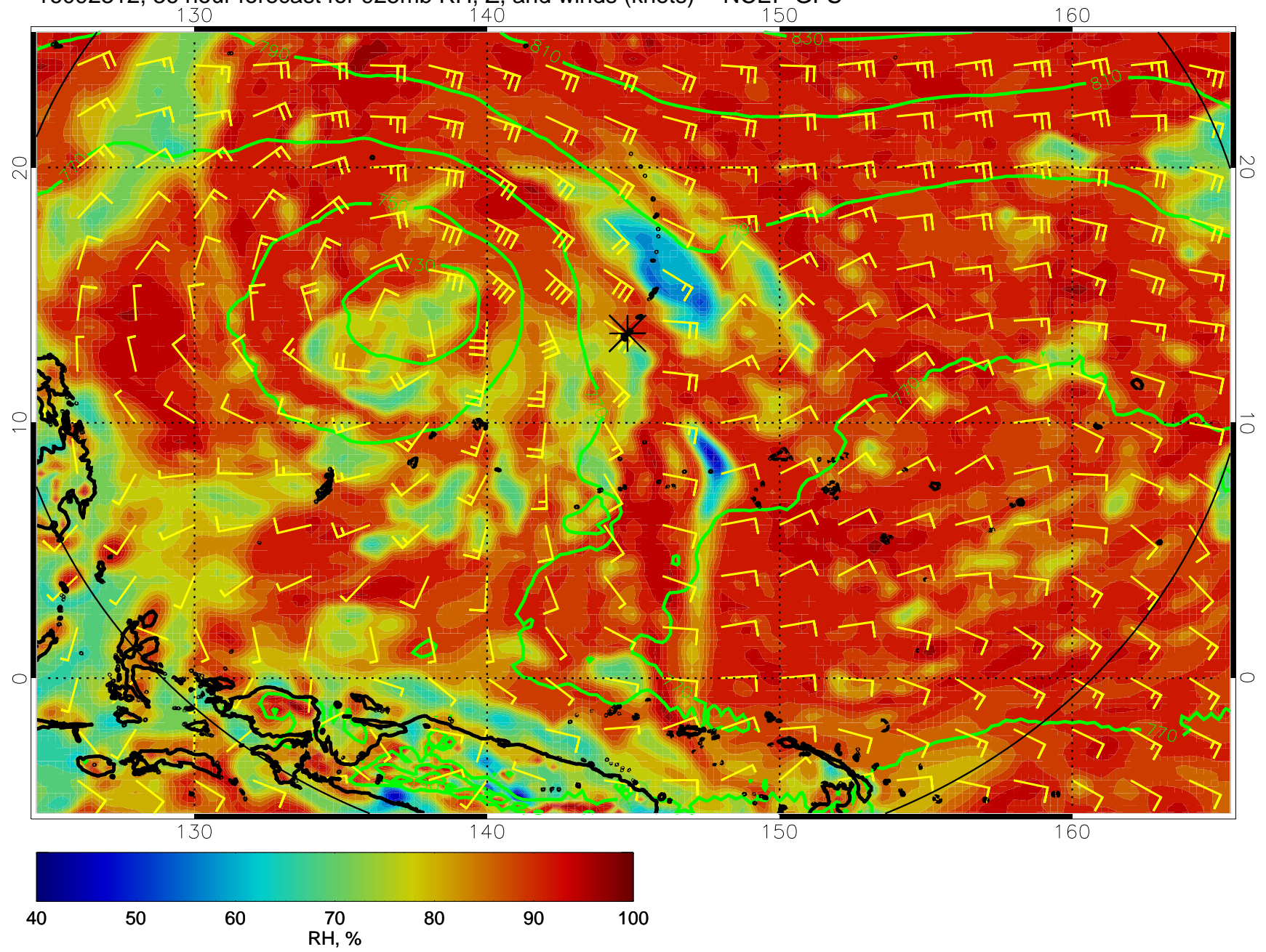
16092312, 36 hour forecast for 925mb RH, Z, and winds (knots) -- NCEP GFS
