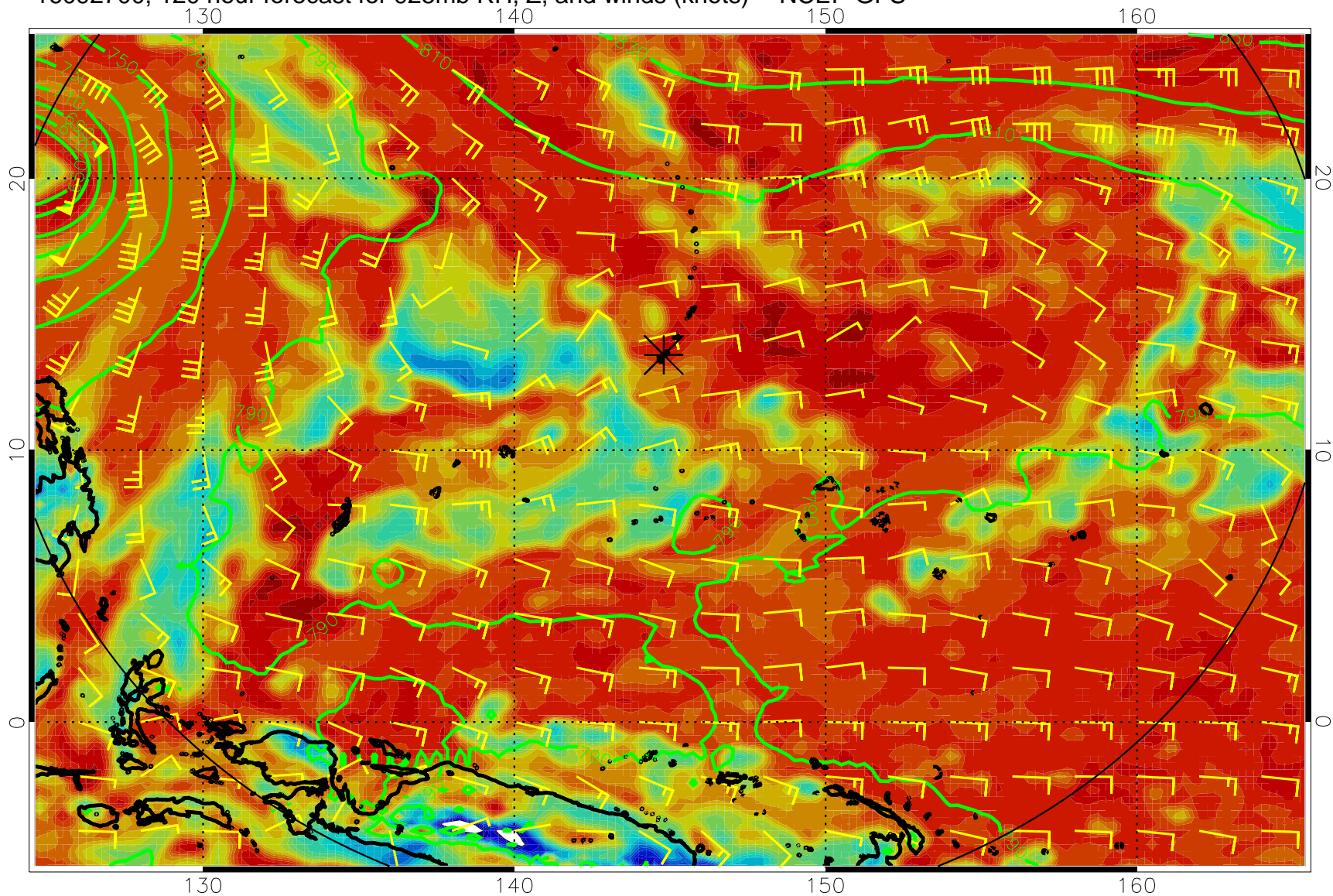
16092700, 120 hour forecast for 925mb RH, Z, and winds (knots) -- NCEP GFS
