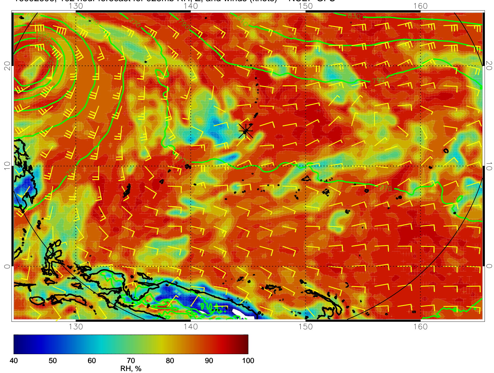
16092606, 102 hour forecast for 925mb RH, Z, and winds (knots) -- NCEP GFS
