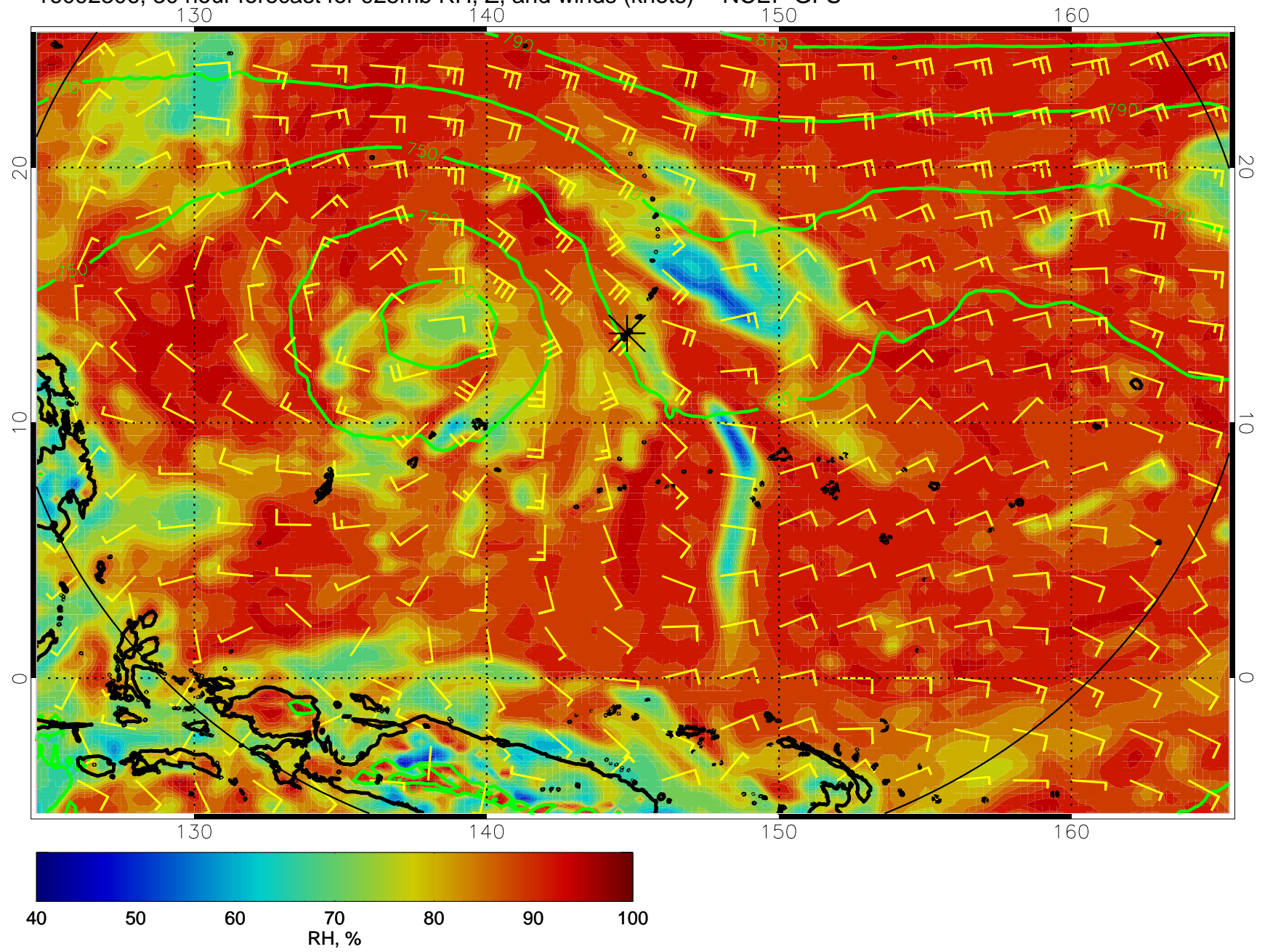
16092306, 30 hour forecast for 925mb RH, Z, and winds (knots) -- NCEP GFS
