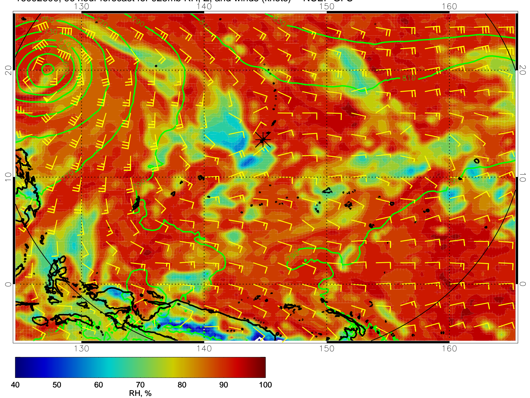
16092600, 96 hour forecast for 925mb RH, Z, and winds (knots) -- NCEP GFS
