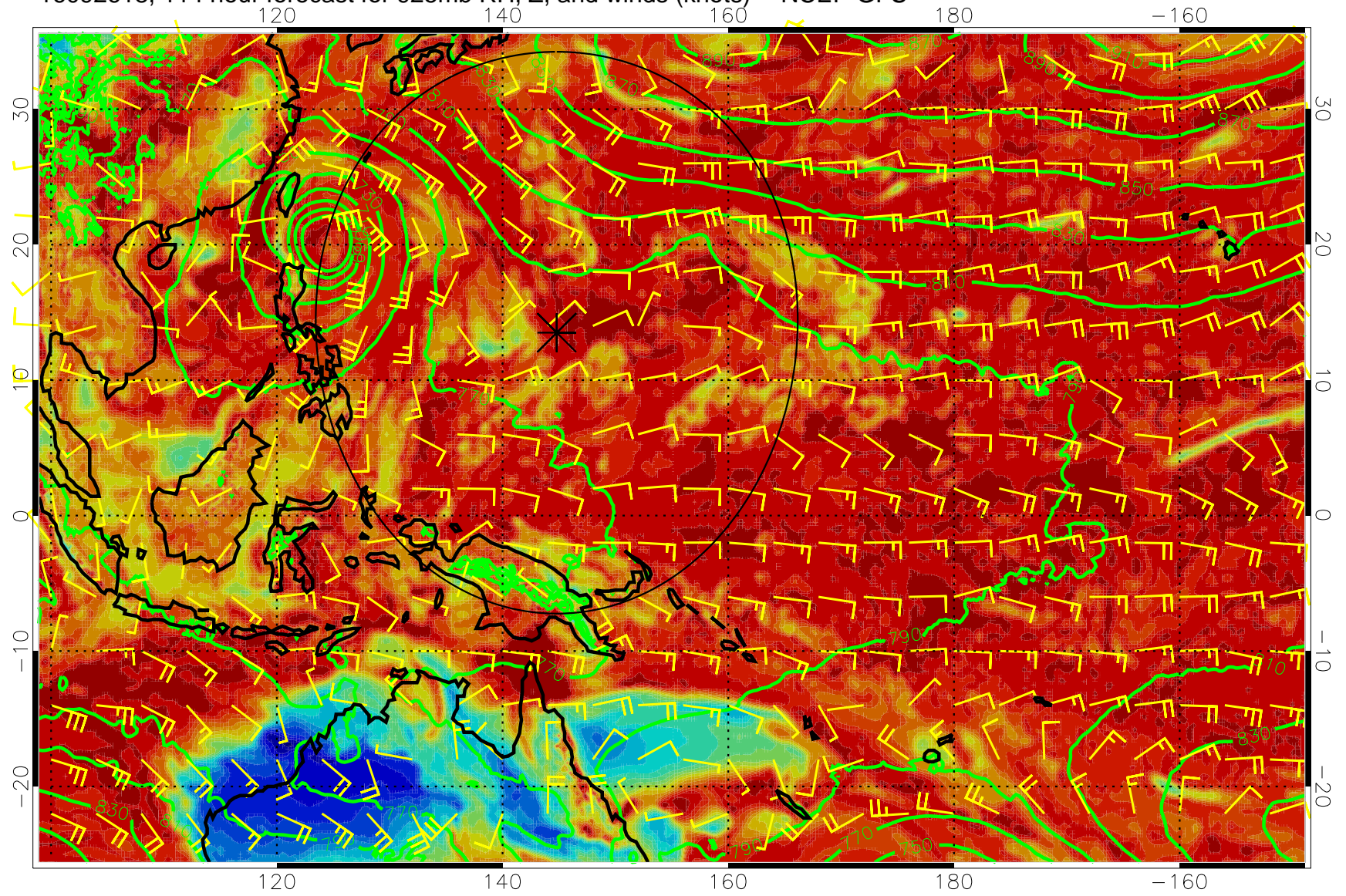
16092618, 114 hour forecast for 925mb RH, Z, and winds (knots) -- NCEP GFS
