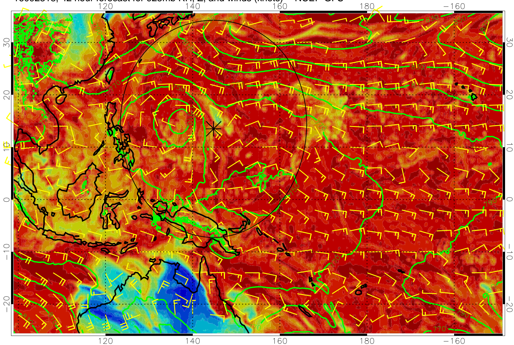
16092318, 42 hour forecast for 925mb RH, Z, and winds (knots) -- NCEP GFS
