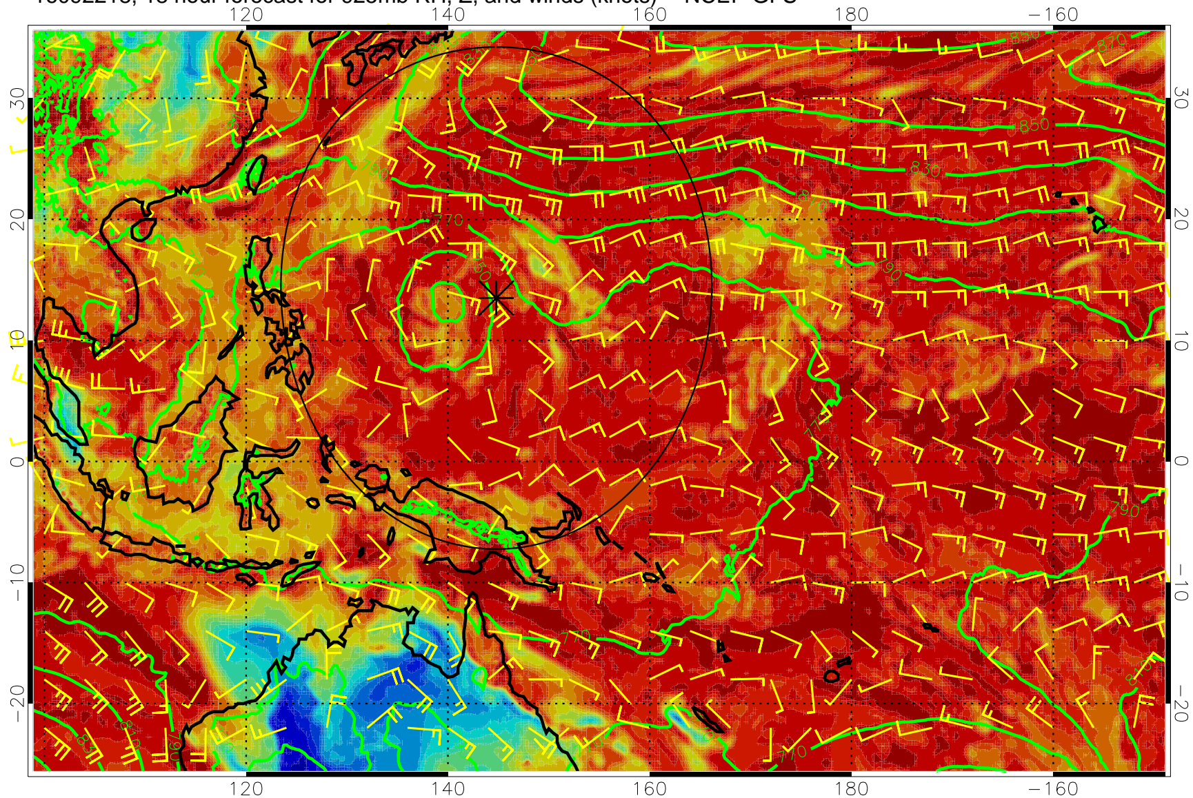
16092218, 18 hour forecast for 925mb RH, Z, and winds (knots) -- NCEP GFS
