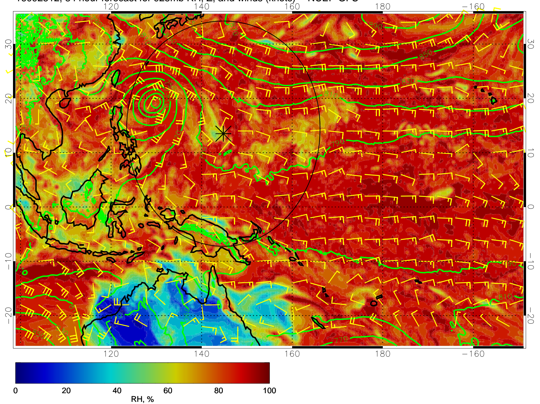
16092512, 84 hour forecast for 925mb RH, Z, and winds (knots) -- NCEP GFS
