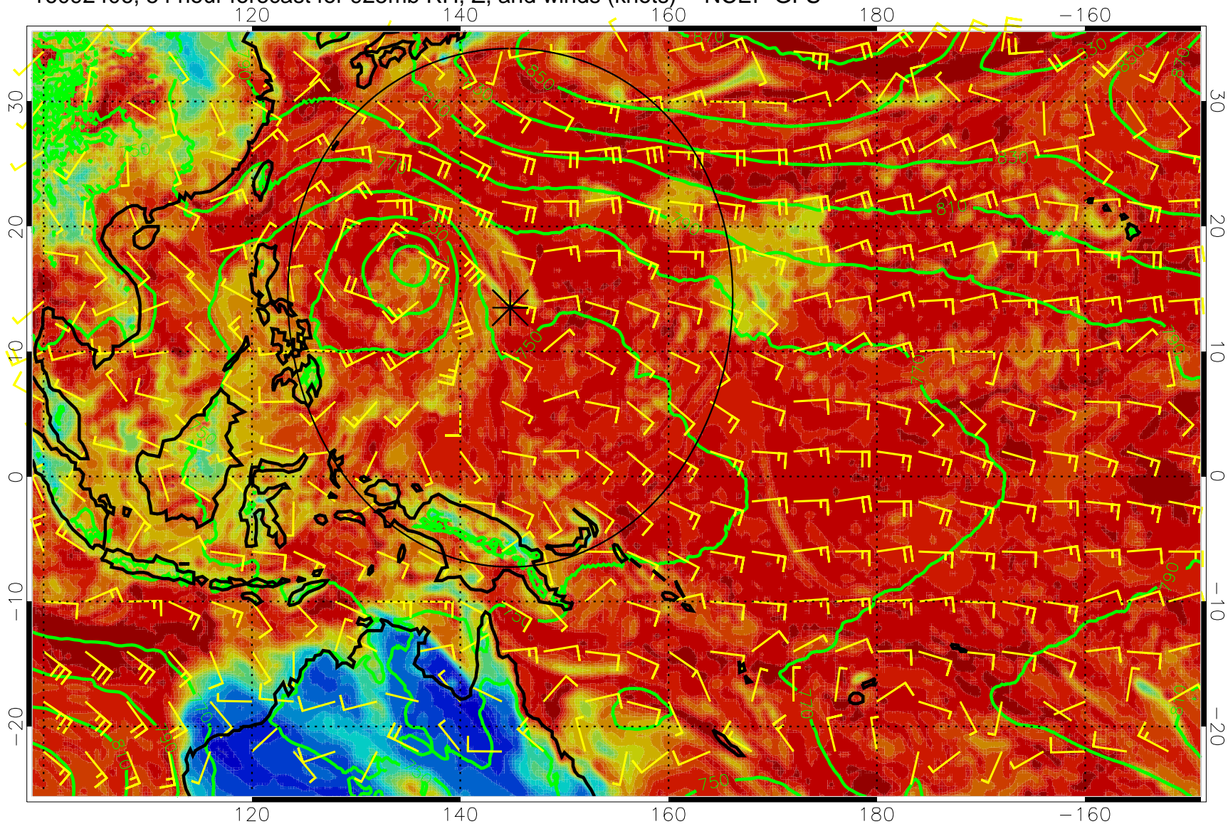
16092406, 54 hour forecast for 925mb RH, Z, and winds (knots) -- NCEP GFS
