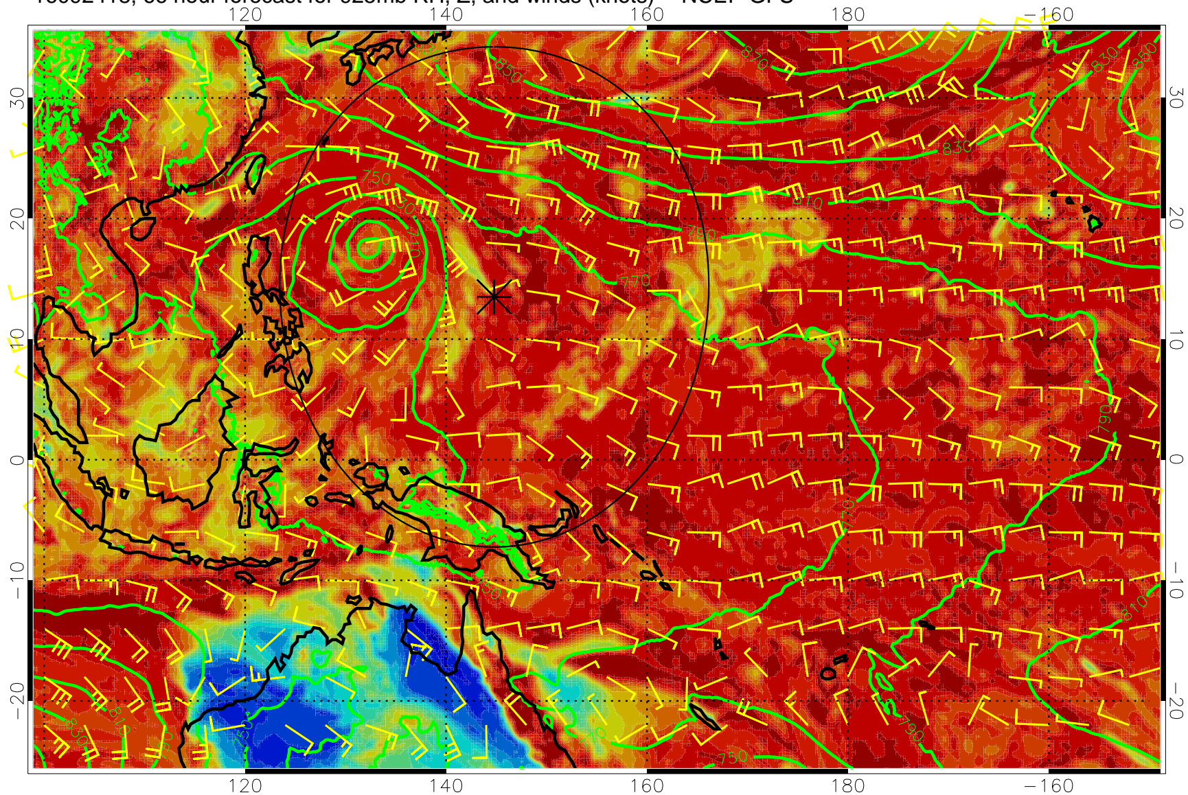
16092418, 66 hour forecast for 925mb RH, Z, and winds (knots) -- NCEP GFS
