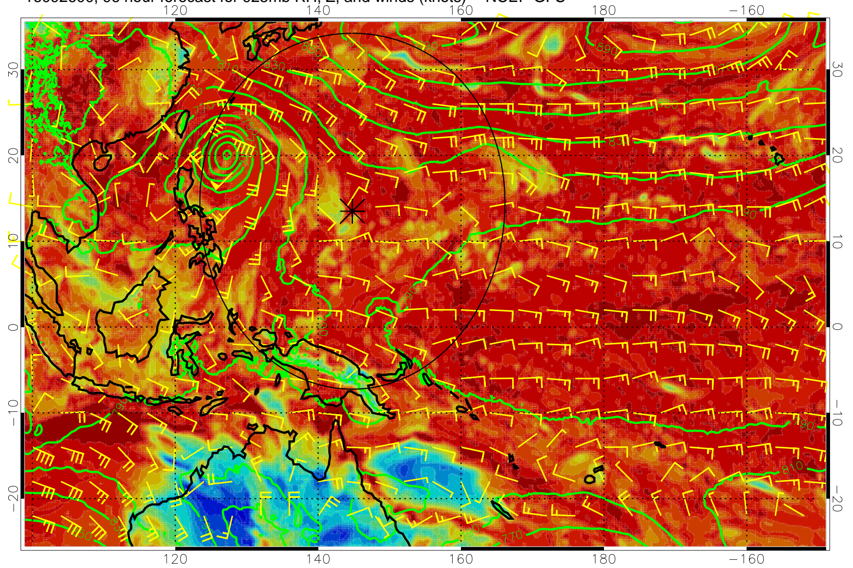
16092600, 96 hour forecast for 925mb RH, Z, and winds (knots) -- NCEP GFS
