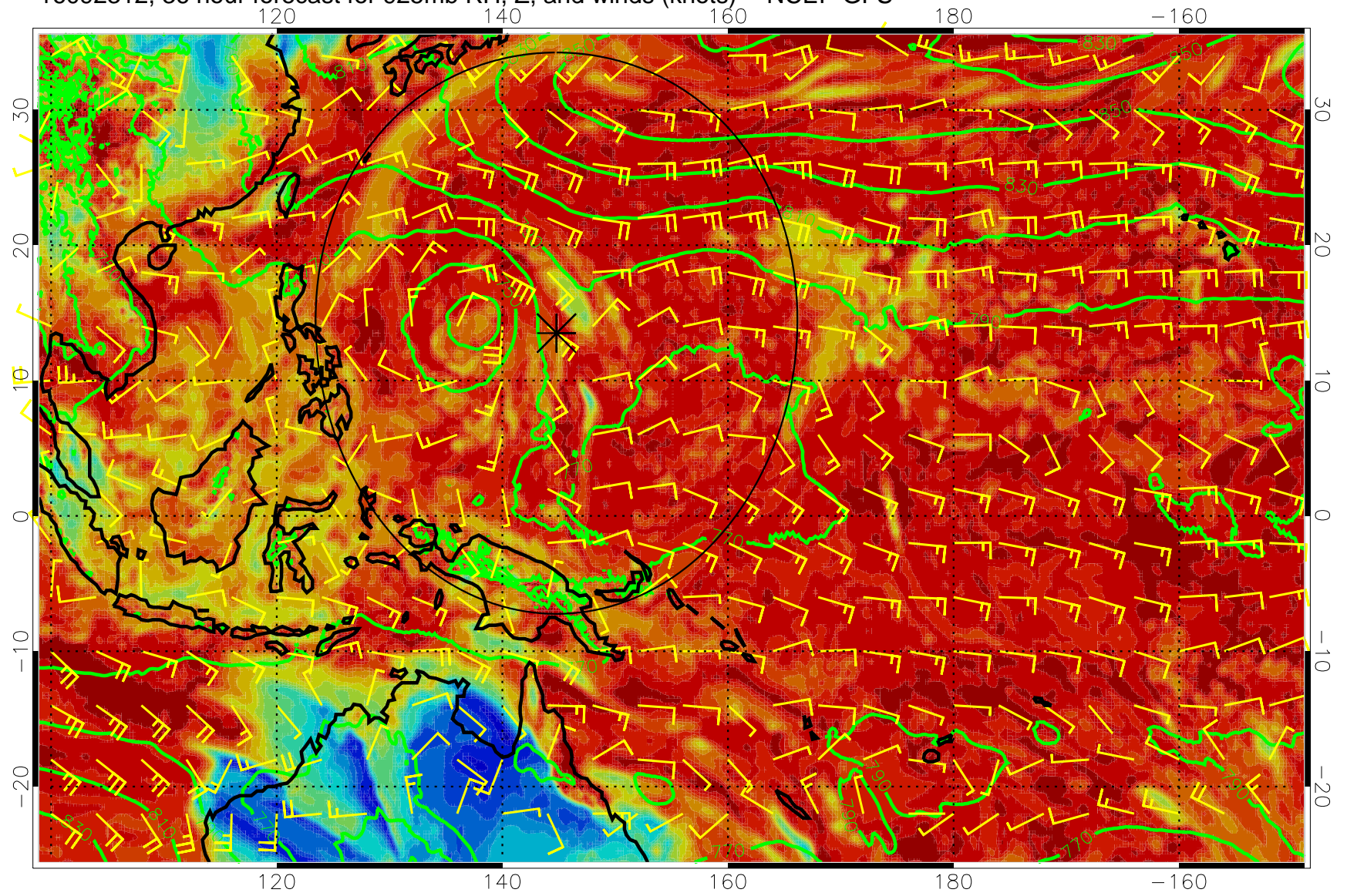
16092312, 36 hour forecast for 925mb RH, Z, and winds (knots) -- NCEP GFS
