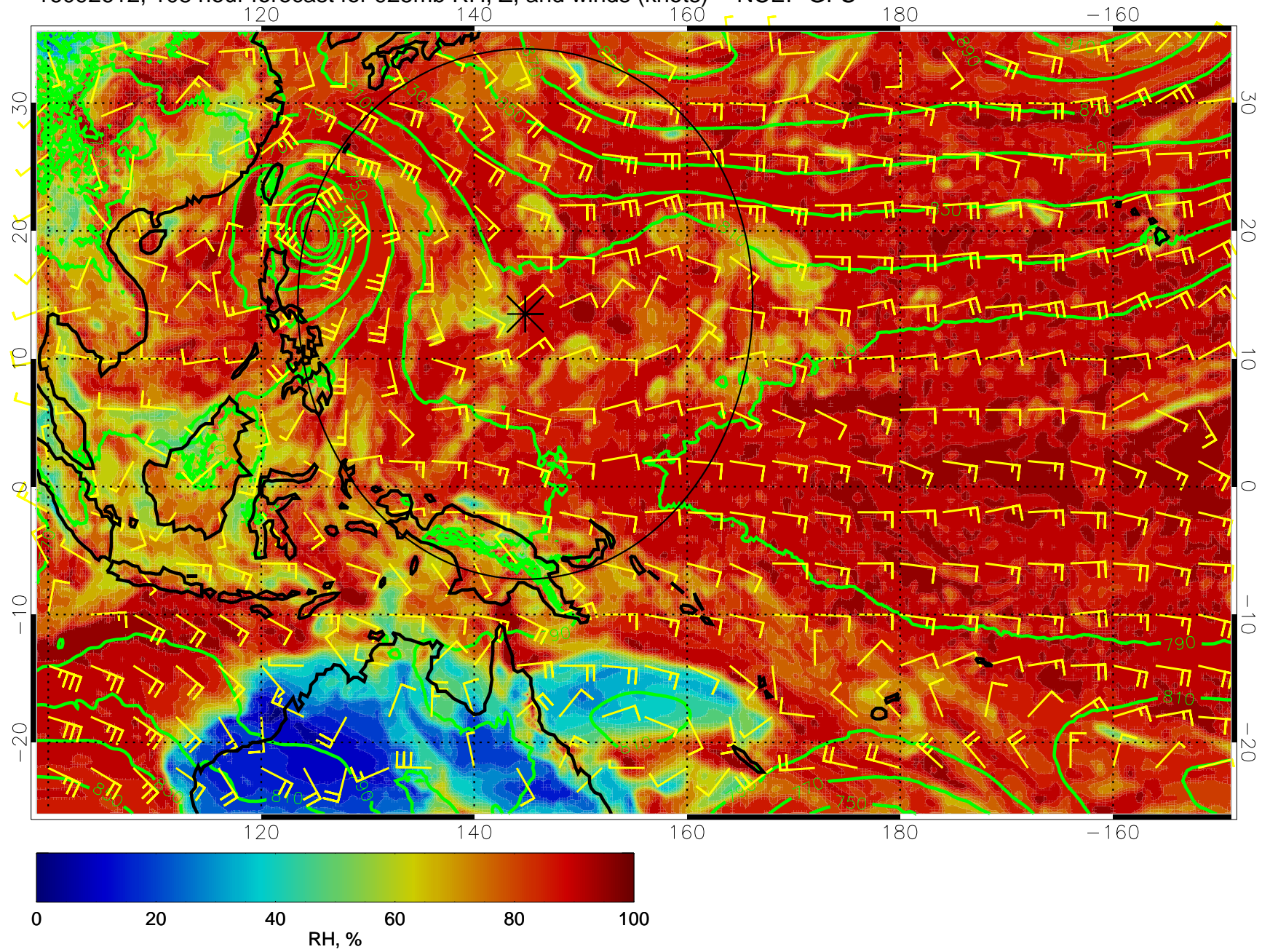
16092612, 108 hour forecast for 925mb RH, Z, and winds (knots) -- NCEP GFS
