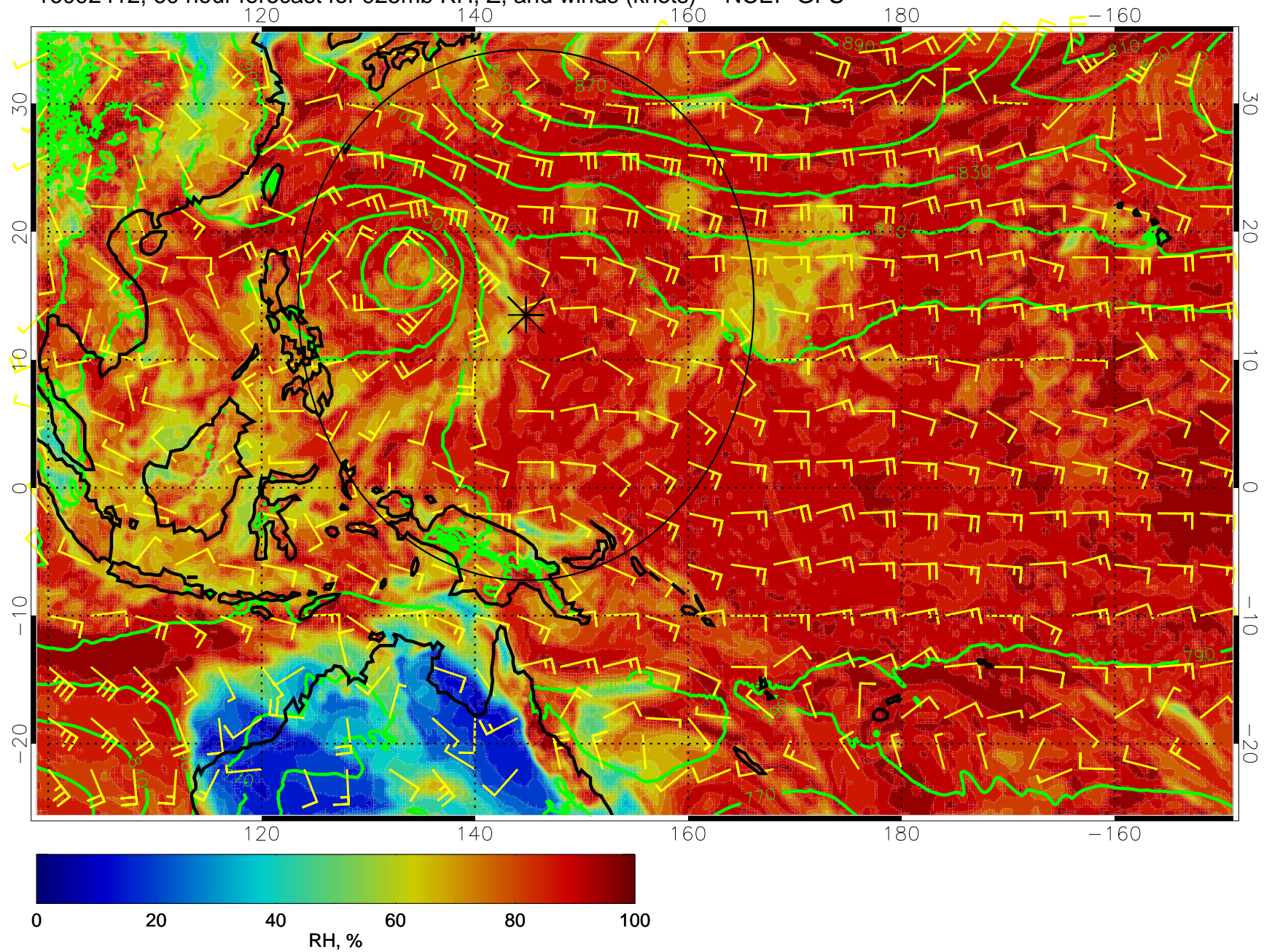
16092412, 60 hour forecast for 925mb RH, Z, and winds (knots) -- NCEP GFS
