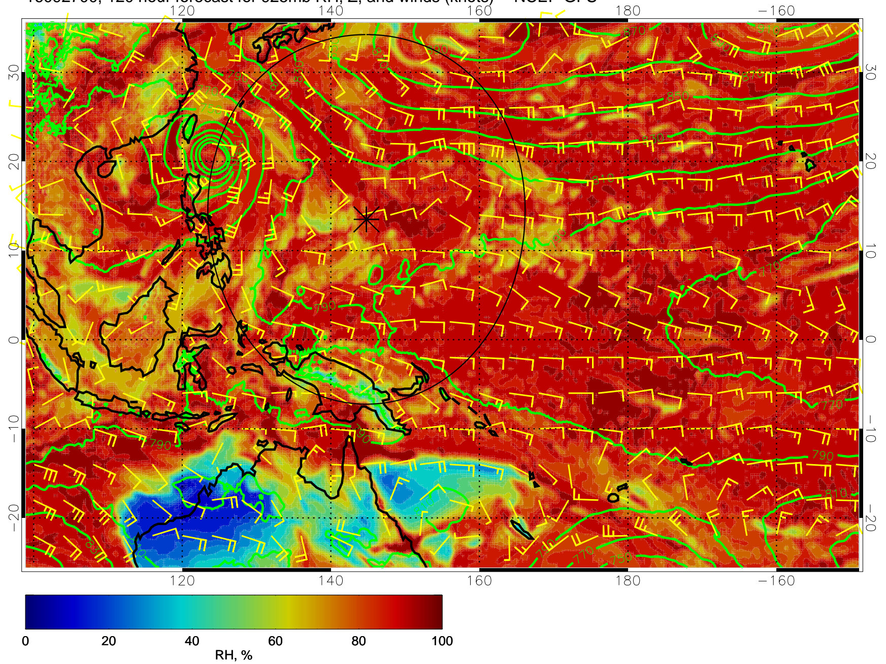
16092700, 120 hour forecast for 925mb RH, Z, and winds (knots) -- NCEP GFS
