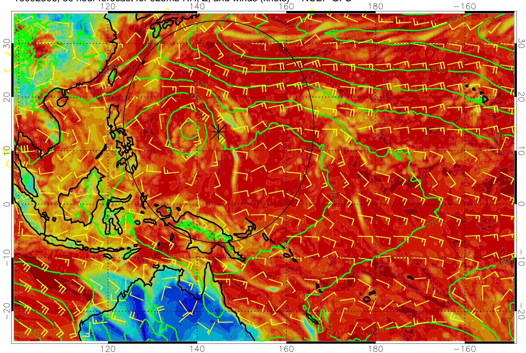
16092306, 30 hour forecast for 925mb RH, Z, and winds (knots) -- NCEP GFS
