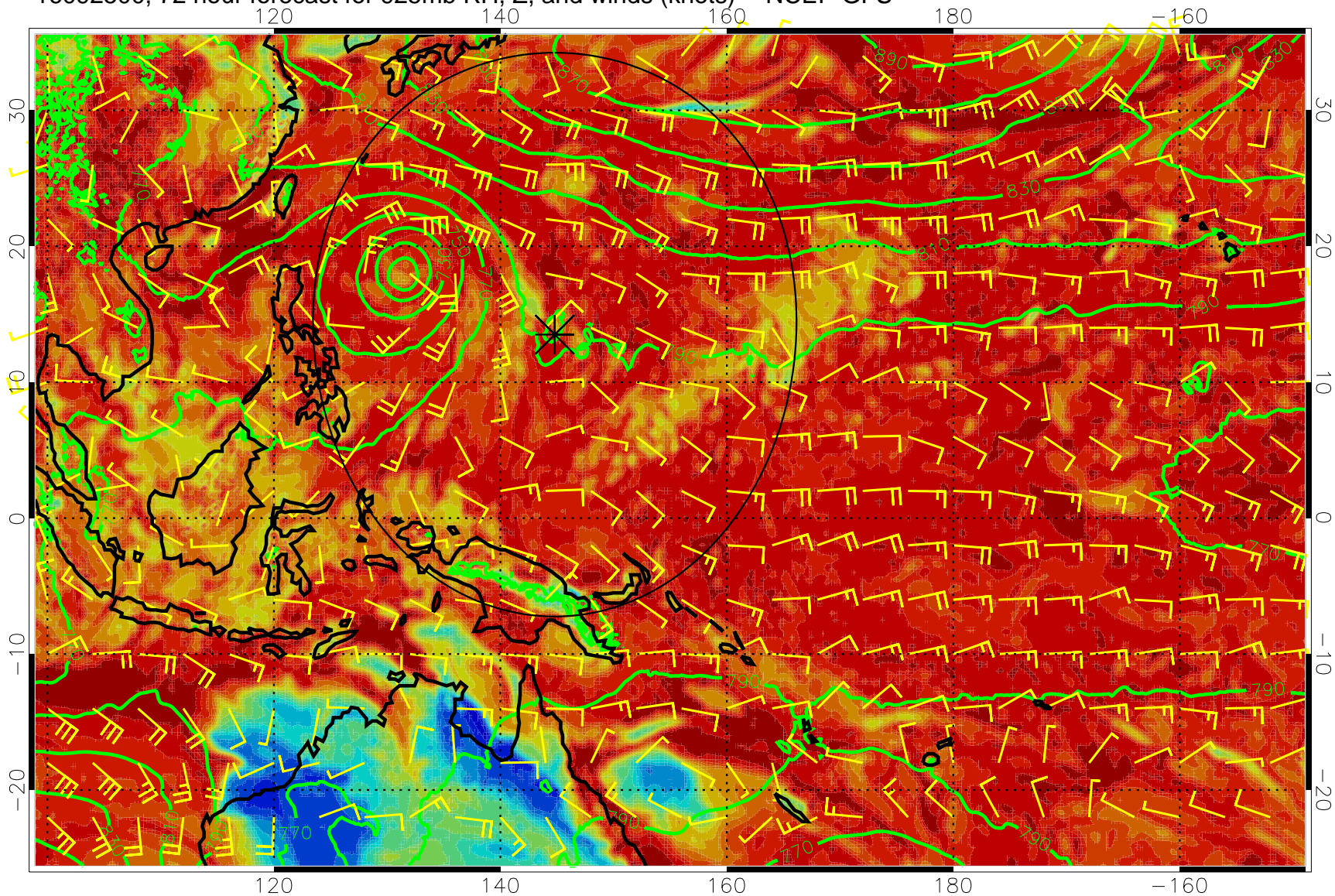
16092500, 72 hour forecast for 925mb RH, Z, and winds (knots) -- NCEP GFS
