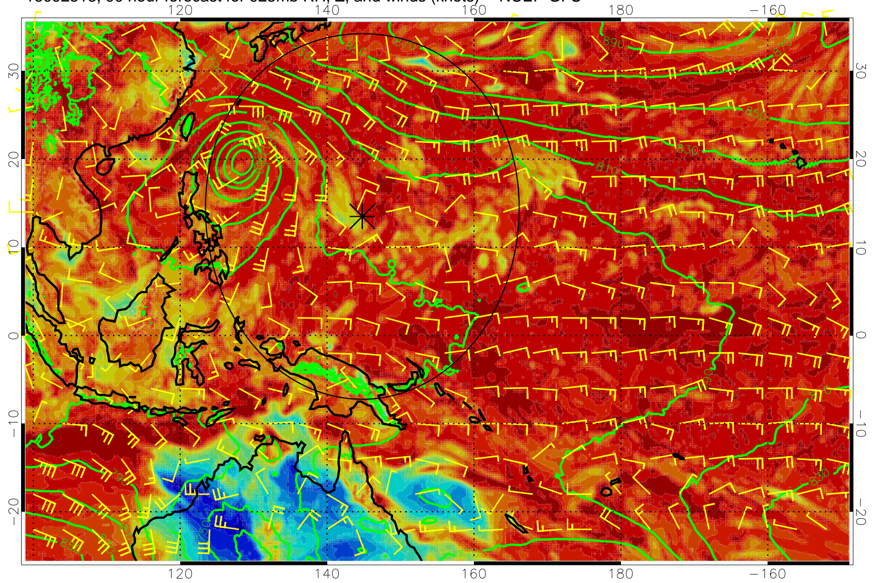
16092518, 90 hour forecast for 925mb RH, Z, and winds (knots) -- NCEP GFS
