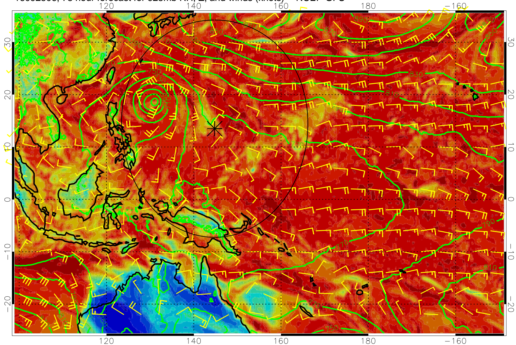
16092506, 78 hour forecast for 925mb RH, Z, and winds (knots) -- NCEP GFS
