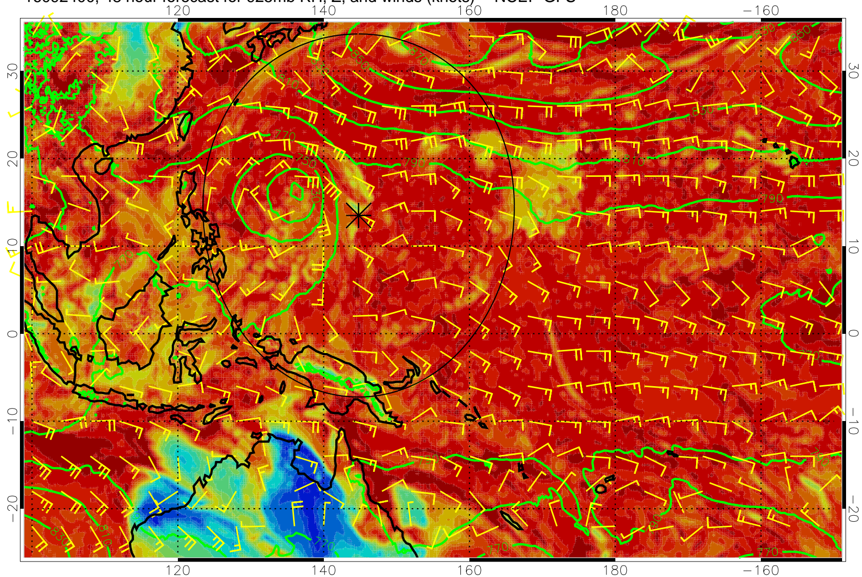
16092400, 48 hour forecast for 925mb RH, Z, and winds (knots) -- NCEP GFS
