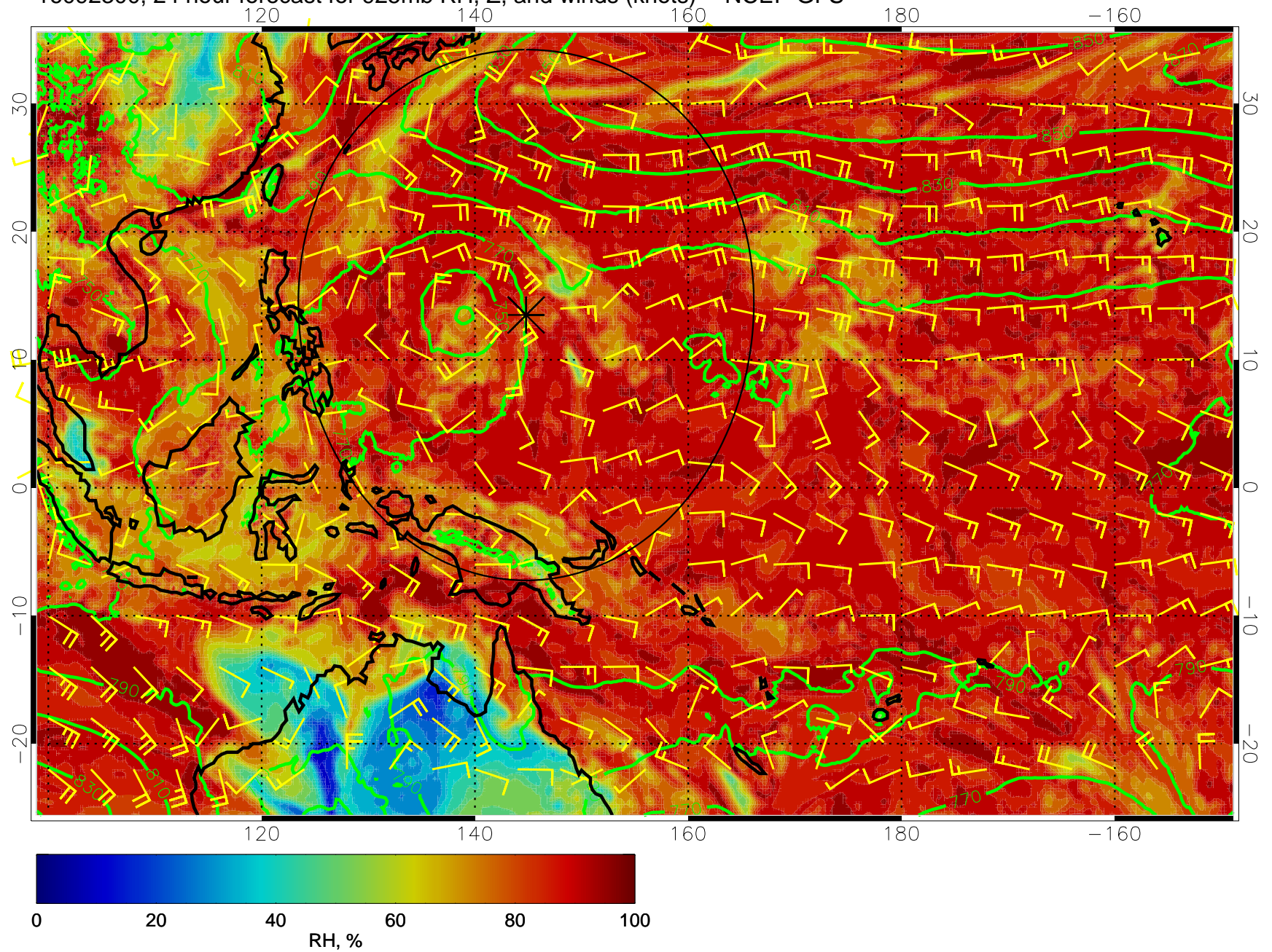
16092300, 24 hour forecast for 925mb RH, Z, and winds (knots) -- NCEP GFS
