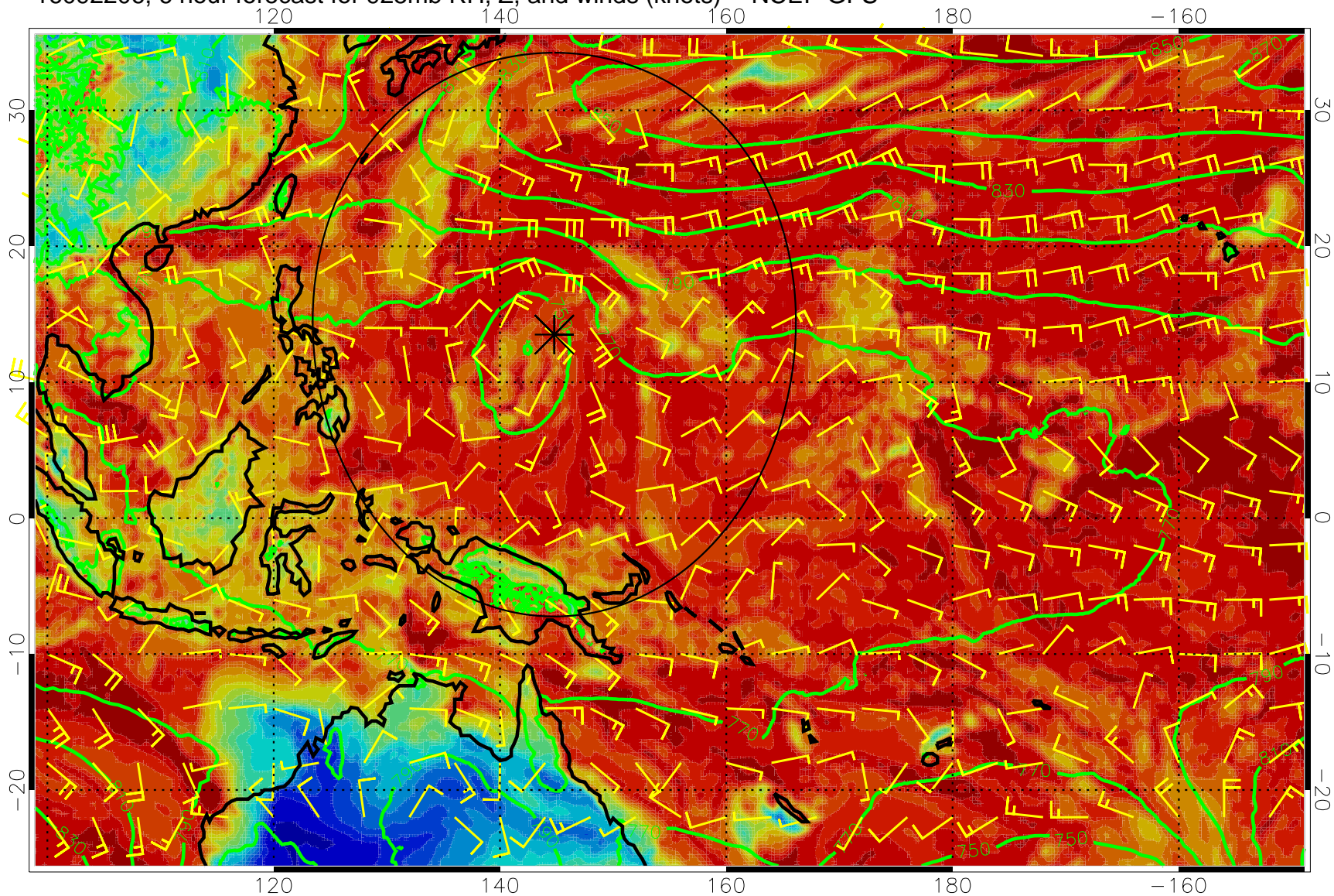
16092206, 6 hour forecast for 925mb RH, Z, and winds (knots) -- NCEP GFS
