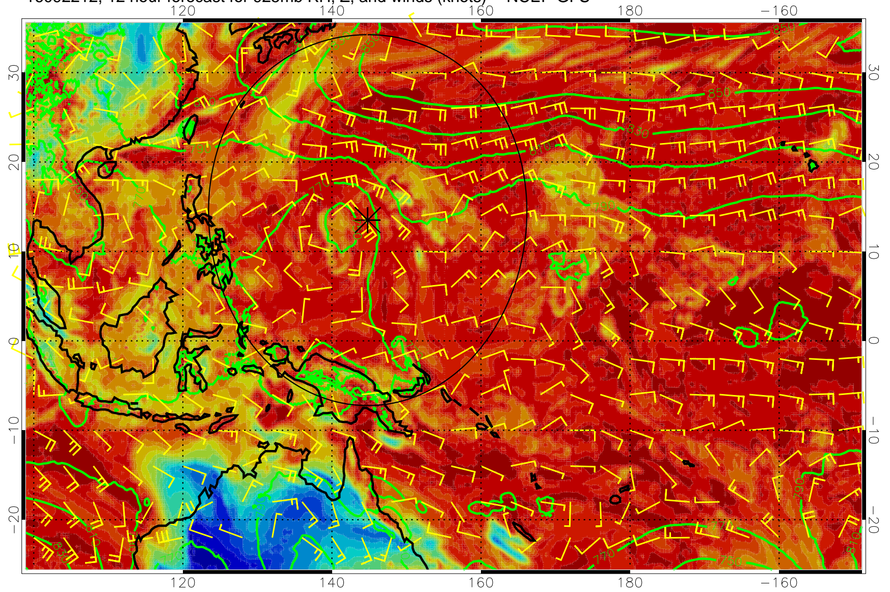
16092212, 12 hour forecast for 925mb RH, Z, and winds (knots) -- NCEP GFS
