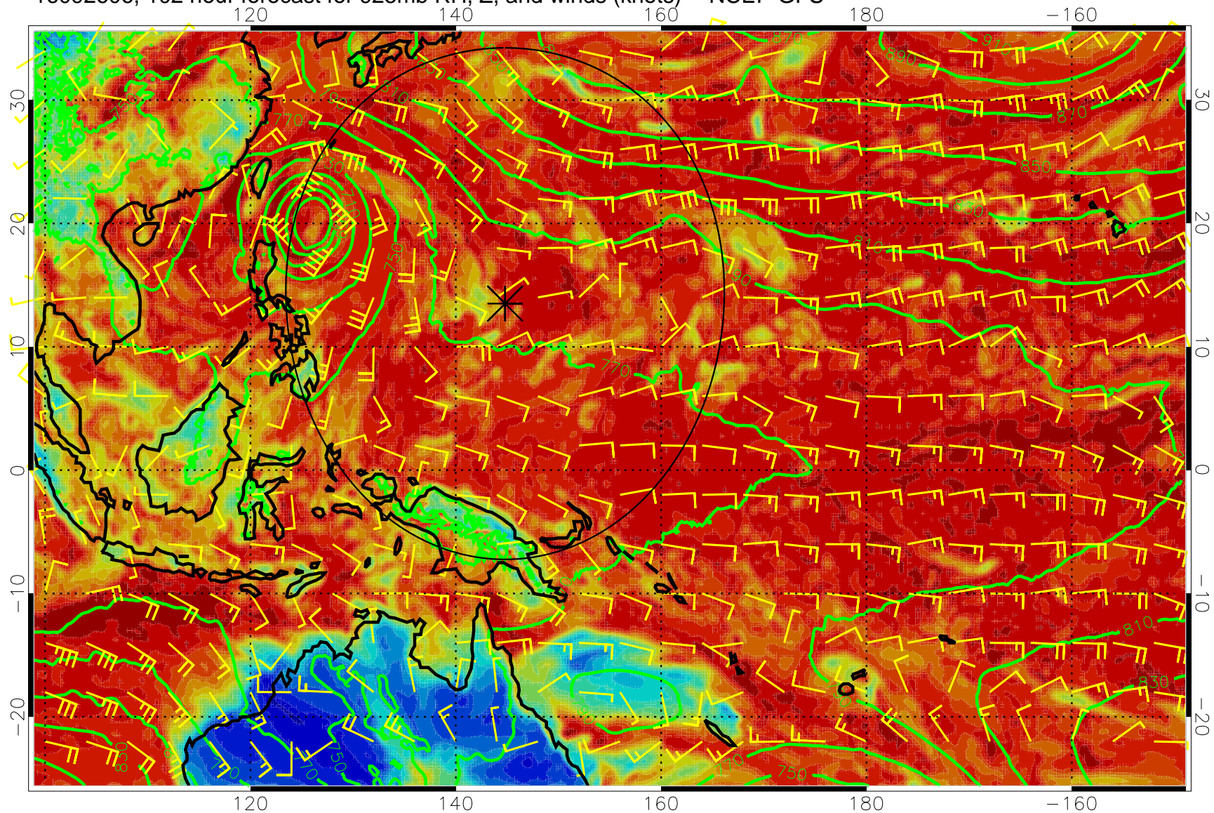
16092606, 102 hour forecast for 925mb RH, Z, and winds (knots) -- NCEP GFS
